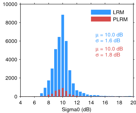
Figure 28. Histogram of science-valid sigma0 over oceans and lakes for LRM (blue) and PLRM (red) for 07/07/2015. The mean ( \mu ) and standard deviation ( \sigma ) are also shown. Note that values outside [4 20] dB are excluded from the histogram for the sake of readability but not from the computation of \mu and \sigma .
