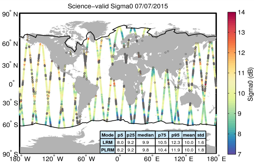
Figure 27. Geographical distribution of science-valid sigma0 data over oceans and lakes for 07/07/2015. The statistical values shown in the table refer to the sigma0 in dB and are calculated separately for LRM and PLRM regions. The black lines mark the outer limit of the Arctic and Antarctic polar polygons. Gray circles denote records that have been rejected based on the editing criteria described in Table 4.
