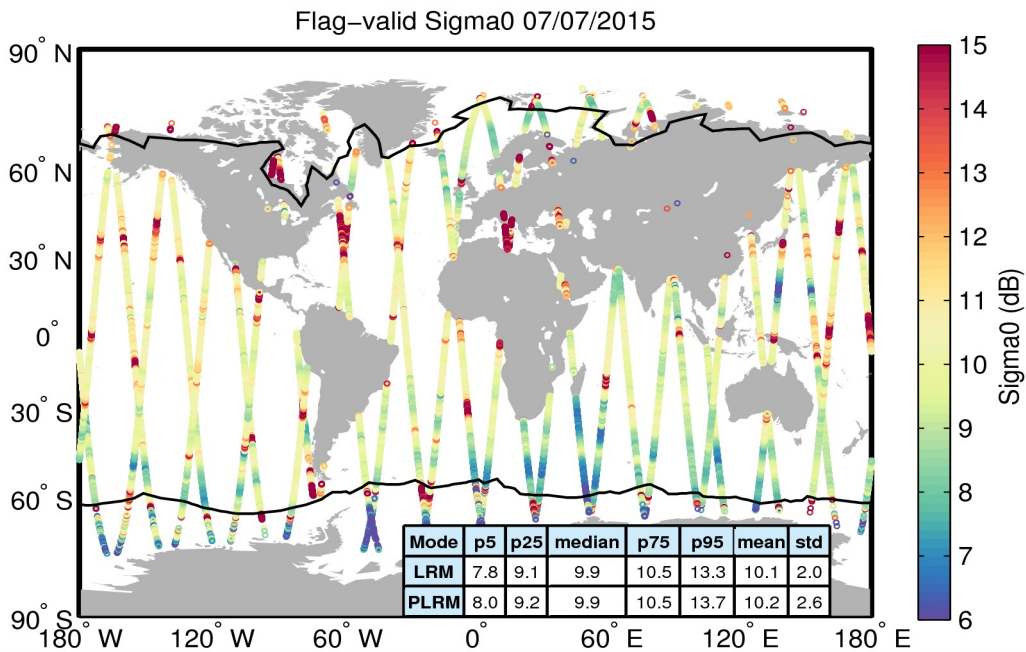
Figure 23. Geographical distribution of flag-valid sigma0 data over oceans and lakes for 07/07/2015. The statistical values shown in the table refer to the sigma0 in dB and are calculated separately for LRM and PLRM regions. Measurements taken over polar polygons have been excluded from the computation of the statistical values. The black lines mark the outer limit of the Arctic and Antarctic polar polygons.
