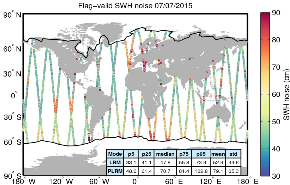
Figure 18. Geographical distribution of flag-valid 20-Hz SWH measurement noise over oceans and lakes for 07/07/2015. The statistical values shown in the table refer to the SWH noise and are calculated separately for LRM and PLRM regions. Measurements taken over polar polygons have been excluded from the computation of the statistical values. The black lines mark the outer limit of the Arctic and Antarctic polar polygons.
