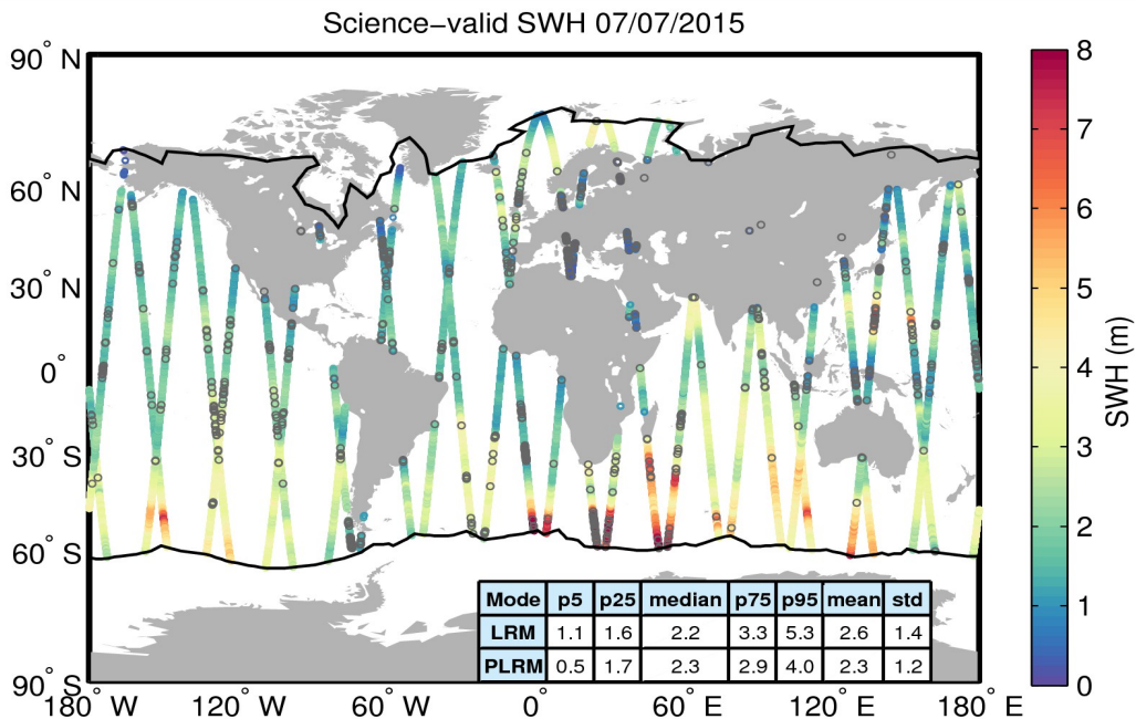
Figure 19. Geographical distribution of science-valid SWH data over oceans and lakes for 07/07/2015. The statistical values shown in the table refer to the SWH in m and are calculated separately for LRM and PLRM regions. The black lines mark the outer limit of the Arctic and Antarctic polar polygons. Gray circles denote records that have been rejected based on the editing criteria described in Table 3.
