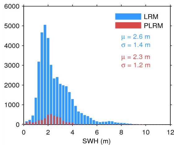
Figure 20. Histogram of science-valid SWH over oceans and lakes for LRM (blue) and PLRM (red) for 07/07/2015. The mean ( \mu ) and standard deviation ( \sigma ) are also shown. Note that values larger than 12 m are excluded from the histogram for the sake of readability but not from the computation of \mu and \sigma .
