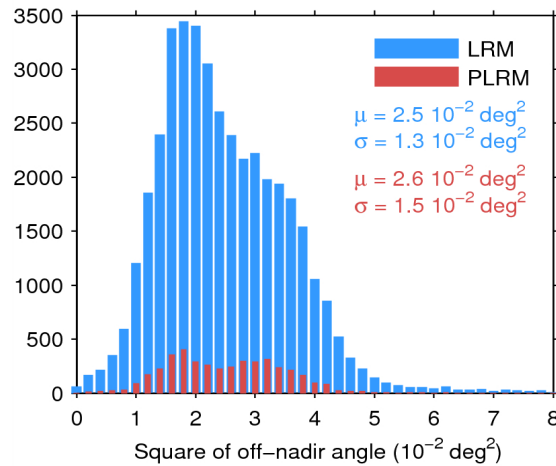
Figure 39. Histogram of flag-valid mispointing over oceans and lakes for LRM (blue) and PLRM (red) for 07/07/2015. Only positive values have been considered. The mean ( \mu ) and standard deviation ( \sigma ) are also shown. Note that values larger than 8 \cdot 10^{-2} \text{ deg}^2 are excluded from the histogram for the sake of readability but not from the computation of \mu and \sigma .
