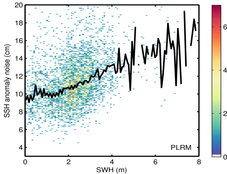
Figure 9. 2D histogram showing flag-valid SSH anomaly noise as a function of SWH for LRM (top) and PLRM (bottom) for 07/07/2015. The black line denotes the median SSH anomaly as a function of SWH.
