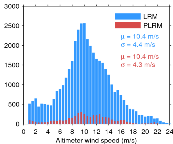
Figure 35. Histogram of science-valid wind over oceans and lakes for LRM (blue) and PLRM (red) for 07/07/2015. The mean ( \mu ) and standard deviation ( \sigma ) are also shown. Note that values larger than 24 m/s are excluded from the histogram for the sake of readability but not from the computation of \mu and \sigma .
