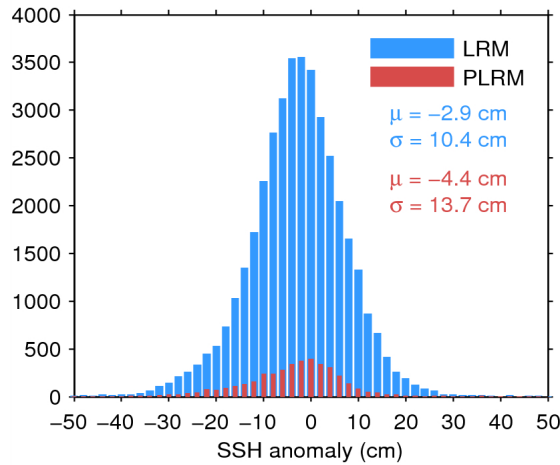
Figure 11. Histogram of science-valid SSH anomaly over oceans and lakes for LRM (blue) and PLRM (red) for 07/07/2015. The mean ( \mu ) and standard deviation ( \sigma ) are also shown. Note that values outside [-50 50] cm are excluded from the histogram for the sake of readability but not from the computation of \mu and \sigma .
