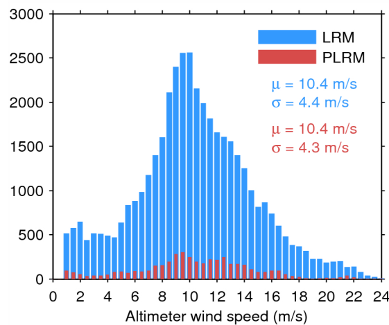
Figure 33. Histogram of flag-valid wind over oceans and lakes for LRM (blue) and PLRM (red) for 07/07/2015. The mean ( \mu ) and standard deviation ( \sigma ) are also shown. Note that values larger than 24 m/s are excluded from the histogram for the sake of readability but not from the computation of \mu and \sigma .
