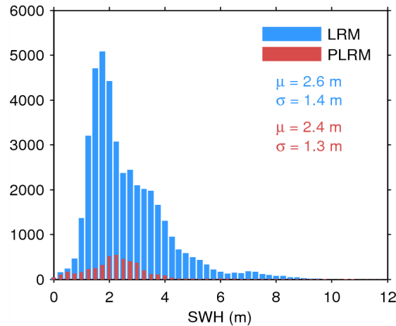
Figure 17. Histogram of flag-valid SWH over oceans and lakes for LRM (blue) and PLRM (red) for 07/07/2015. The mean ( \mu ) and standard deviation ( \sigma ) are also shown. Note that values larger than 12 m are excluded from the histogram for the sake of readability but not from the computation of \mu and \sigma .
