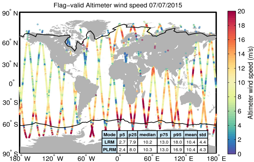
Figure 31. Geographical distribution of flag-valid wind data over oceans and lakes for 07/07/2015. The statistical values shown in the table refer to the wind in m/s and are calculated separately for LRM and PLRM regions. Measurements taken over polar polygons have been excluded from the computation of the statistical values. The black lines mark the outer limit of the Arctic and Antarctic polar polygons.
