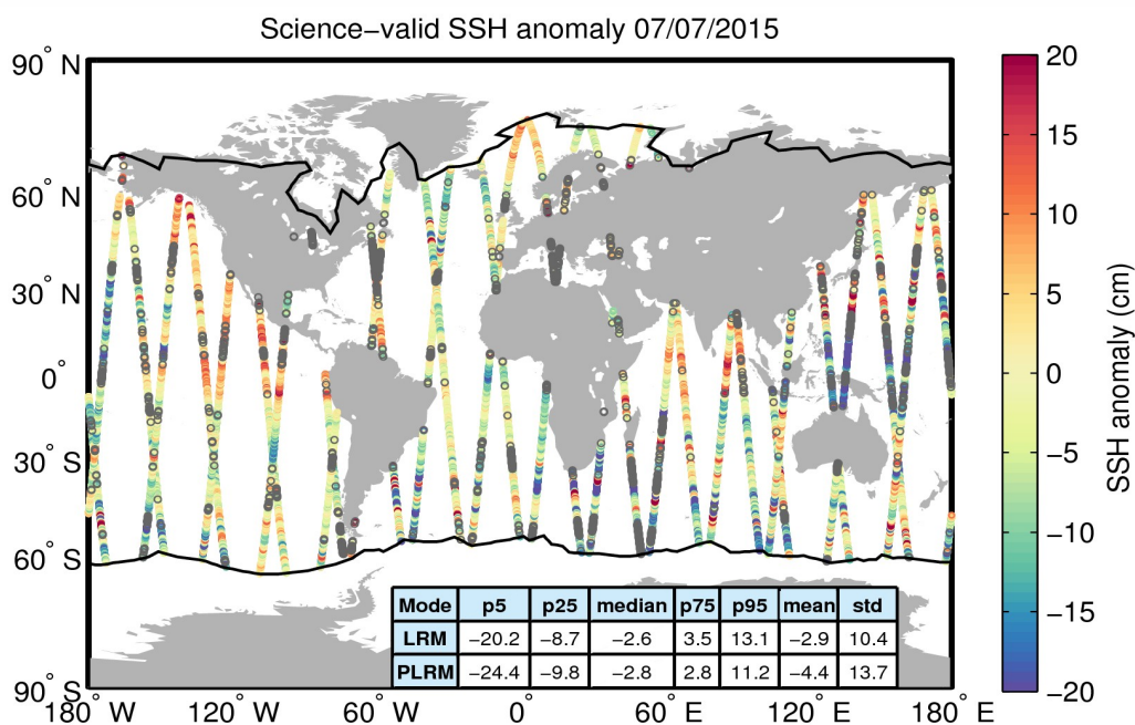
Figure 10. Geographical distribution of science-valid SSH anomaly data over oceans and lakes for 07/07/2015. The statistical values shown in the table refer to the SSH anomaly in cm and are calculated separately for LRM and PLRM regions. The black lines mark the outer limit of the Arctic and Antarctic polar polygons. Gray circles denote records that have been rejected based on the editing criteria described in Table 2.
