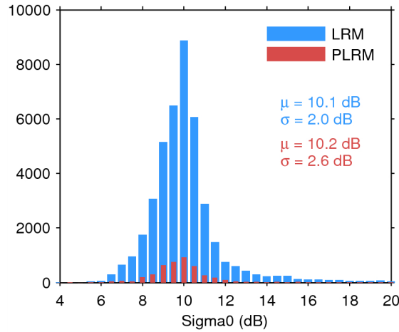
Figure 25. Histogram of flag-valid sigma0 over oceans and lakes for LRM (blue) and PLRM (red) for 07/07/2015. The mean ( \mu ) and standard deviation ( \sigma ) are also shown. Note that values outside [4 20] dB are excluded from the histogram for the sake of readability but not from the computation of \mu and \sigma .
