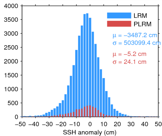
Figure 7. Histogram of flag-valid SSH anomaly over oceans and lakes for LRM (blue) and PLRM (red) for 07/07/2015. The mean ( \mu ) and standard deviation ( \sigma ) are also shown. Note that values outside [-50\ 50] cm are excluded from the histogram for the sake of readability but not from the computation of \mu and \sigma .
