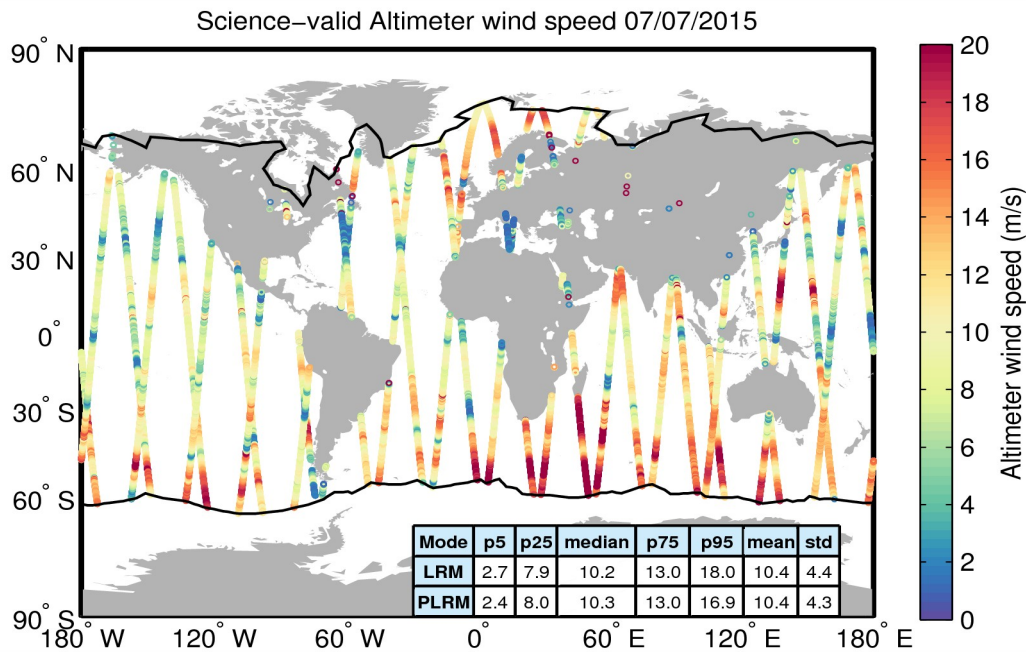
Figure 34. Geographical distribution of science-valid wind data over oceans and lakes for 07/07/2015. The statistical values shown in the table refer to the wind in m/s and are calculated separately for LRM and PLRM regions. The black lines mark the outer limit of the Arctic and Antarctic polar polygons. Gray circles denote records that have been rejected based on the editing criteria described in Table 5.
