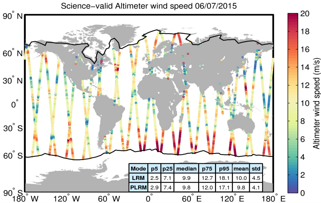
Figure 34. Geographical distribution of science-valid wind data over oceans and lakes for 06/07/2015. The statistical values shown in the table refer to the wind in m/s and are calculated separately for LRM and PLRM regions. The black lines mark the outer limit of the Arctic and Antarctic polar polygons. Gray circles denote records that have been rejected based on the editing criteria described in Table 5.
