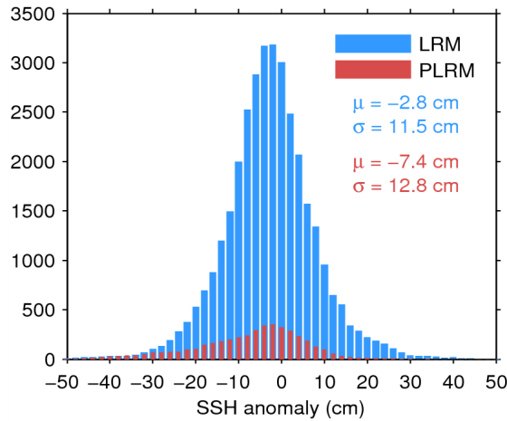
Figure 11. Histogram of science-valid SSH anomaly over oceans and lakes for LRM (blue) and PLRM (red) for 06/07/2015. The mean ( \mu ) and standard deviation ( \sigma ) are also shown. Note that values outside [-50\ 50] cm are excluded from the histogram for the sake of readability but not from the computation of \mu and \sigma .
