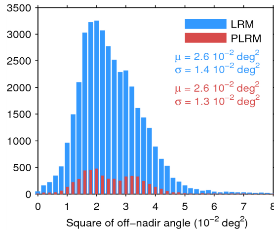
Figure 39. Histogram of flag-valid mispointing over oceans and lakes for LRM (blue) and PLRM (red) for 06/07/2015. Only positive values have been considered. The mean ( \mu ) and standard deviation ( \sigma ) are also shown. Note that values larger than 8 \cdot 10^{-2} \text{ deg}^2 are excluded from the histogram for the sake of readability but not from the computation of \mu and \sigma .
