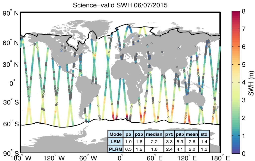
Figure 19. Geographical distribution of science-valid SWH data over oceans and lakes for 06/07/2015. The statistical values shown in the table refer to the SWH in m and are calculated separately for LRM and PLRM regions. The black lines mark the outer limit of the Arctic and Antarctic polar polygons. Gray circles denote records that have been rejected based on the editing criteria described in Table 3.
