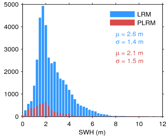
Figure 17. Histogram of flag-valid SWH over oceans and lakes for LRM (blue) and PLRM (red) for 06/07/2015. The mean ( \mu ) and standard deviation ( \sigma ) are also shown. Note that values larger than 12 m are excluded from the histogram for the sake of readability but not from the computation of \mu and \sigma .
