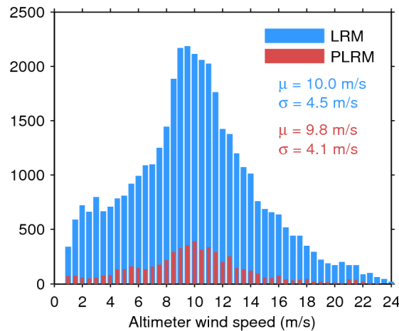
Figure 33. Histogram of flag-valid wind over oceans and lakes for LRM (blue) and PLRM (red) for 06/07/2015. The mean ( \mu ) and standard deviation ( \sigma ) are also shown. Note that values larger than 24 m/s are excluded from the histogram for the sake of readability but not from the computation of \mu and \sigma .
