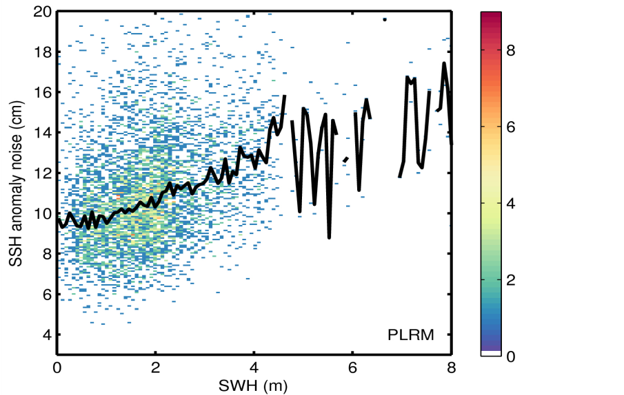
Figure 9. 2D histogram showing flag-valid SSH anomaly noise as a function of SWH for LRM (top) and PLRM (bottom) for 06/07/2015. The black line denotes the median SSH anomaly as a function of SWH.
