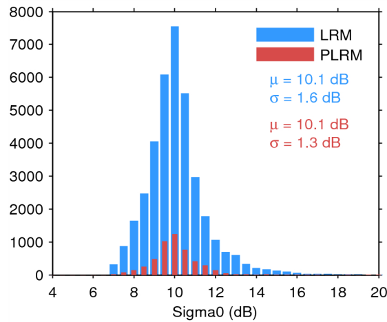
Figure 28. Histogram of science-valid sigma0 over oceans and lakes for LRM (blue) and PLRM (red) for 06/07/2015. The mean ( \mu ) and standard deviation ( \sigma ) are also shown. Note that values outside [4 20] dB are excluded from the histogram for the sake of readability but not from the computation of \mu and \sigma .
