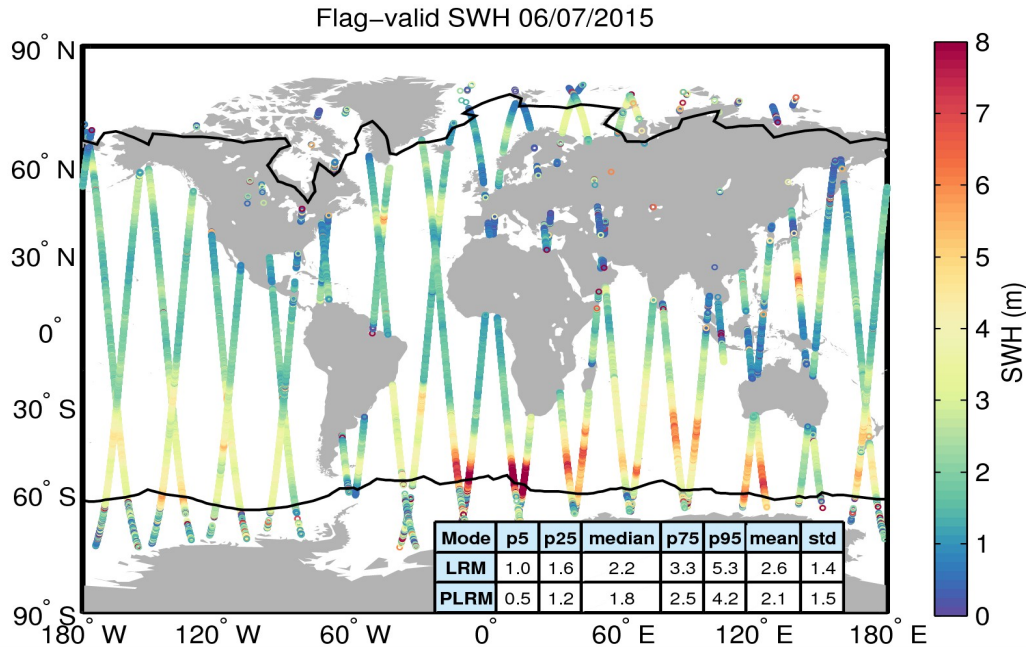
Figure 15. Geographical distribution of flag-valid SWH data over oceans and lakes for 06/07/2015. The statistical values shown in the table refer to the SWH in m and are calculated separately for LRM and PLRM regions. Measurements taken over polar polygons have been excluded from the computation of the statistical values. The black lines mark the outer limit of the Arctic and Antarctic polar polygons.
