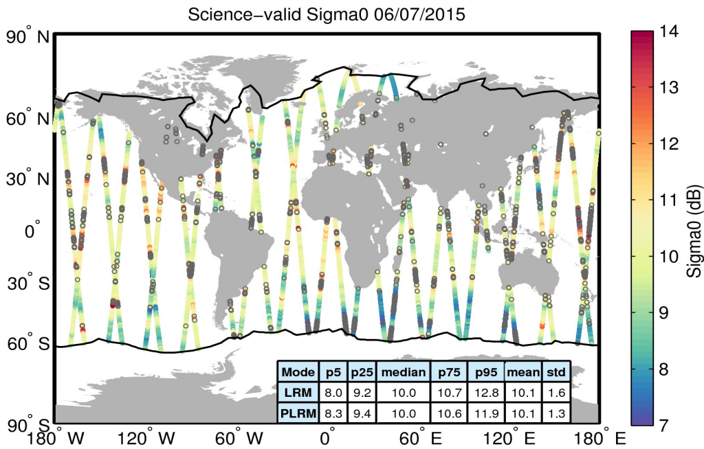
Figure 27. Geographical distribution of science-valid sigma0 data over oceans and lakes for 06/07/2015. The statistical values shown in the table refer to the sigma0 in dB and are calculated separately for LRM and PLRM regions. The black lines mark the outer limit of the Arctic and Antarctic polar polygons. Gray circles denote records that have been rejected based on the editing criteria described in Table 4.
