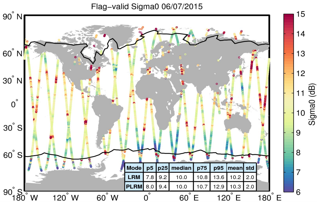
Figure 23. Geographical distribution of flag-valid sigma0 data over oceans and lakes for 06/07/2015. The statistical values shown in the table refer to the sigma0 in dB and are calculated separately for LRM and PLRM regions. Measurements taken over polar polygons have been excluded from the computation of the statistical values. The black lines mark the outer limit of the Arctic and Antarctic polar polygons.
