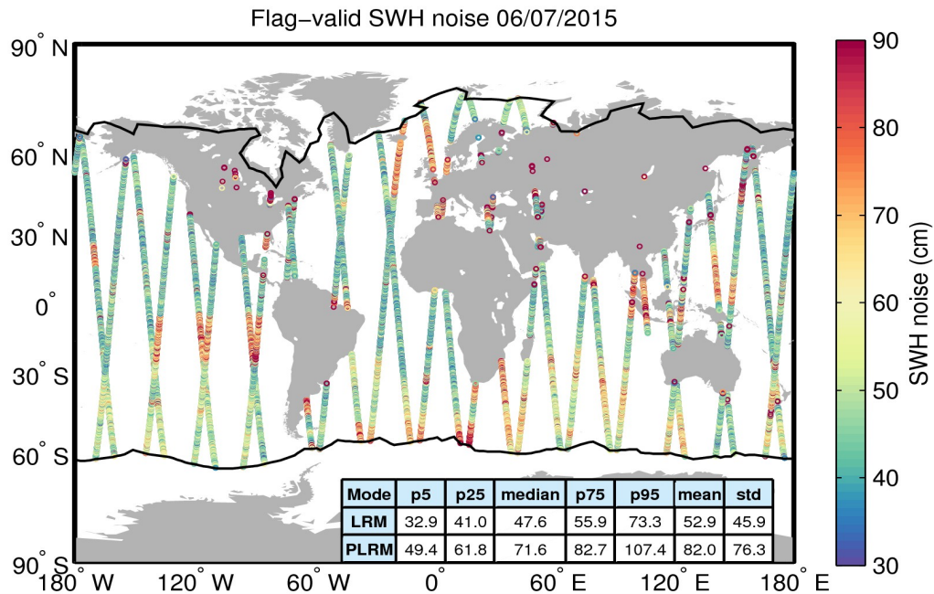
Figure 18. Geographical distribution of flag-valid 20-Hz SWH measurement noise over oceans and lakes for 06/07/2015. The statistical values shown in the table refer to the SWH noise and are calculated separately for LRM and PLRM regions. Measurements taken over polar polygons have been excluded from the computation of the statistical values. The black lines mark the outer limit of the Arctic and Antarctic polar polygons.
