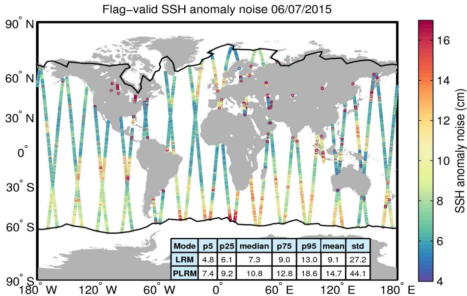
Figure 8. Geographical distribution of flag-valid 20-Hz SSH anomaly measurement noise over oceans and lakes for 06/07/2015. The statistical values shown in the table refer to the SSH anomaly noise and are calculated separately for LRM and PLRM regions. Measurements taken over polar polygons have been excluded from the computation of the statistical values. The black lines mark the outer limit of the Arctic and Antarctic polar polygons.
