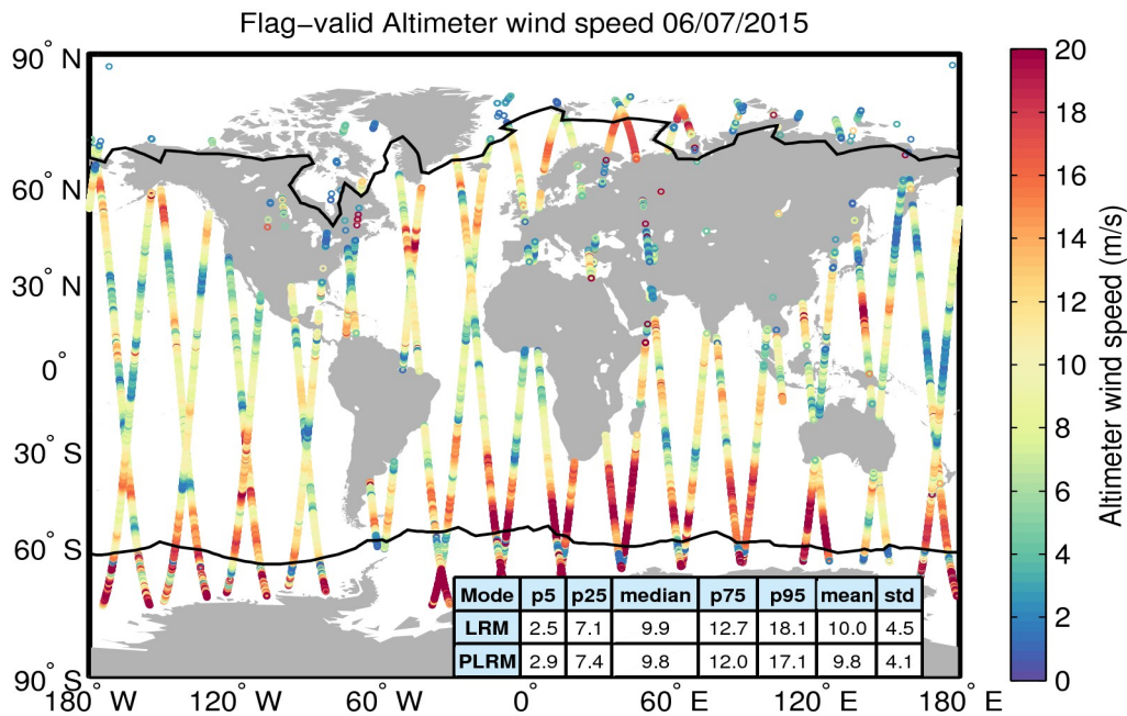
Figure 31. Geographical distribution of flag-valid wind data over oceans and lakes for 06/07/2015. The statistical values shown in the table refer to the wind in m/s and are calculated separately for LRM and PLRM regions. Measurements taken over polar polygons have been excluded from the computation of the statistical values. The black lines mark the outer limit of the Arctic and Antarctic polar polygons.
