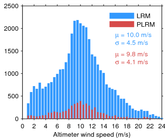
Figure 35. Histogram of science-valid wind over oceans and lakes for LRM (blue) and PLRM (red) for 06/07/2015. The mean ( \mu ) and standard deviation ( \sigma ) are also shown. Note that values larger than 24 m/s are excluded from the histogram for the sake of readability but not from the computation of \mu and \sigma .
