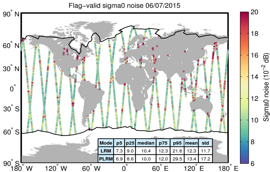
Figure 26. Geographical distribution of flag-valid 20-Hz sigma0 measurement noise over oceans and lakes for 06/07/2015. The statistical values shown in the table refer to the sigma0 noise and are calculated separately for LRM and PLRM regions. Measurements taken over polar polygons have been excluded from the computation of the statistical values. The black lines mark the outer limit of the Arctic and Antarctic polar polygons.
