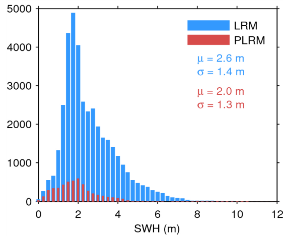
Figure 20. Histogram of science-valid SWH over oceans and lakes for LRM (blue) and PLRM (red) for 06/07/2015. The mean ( \mu ) and standard deviation ( \sigma ) are also shown. Note that values larger than 12 m are excluded from the histogram for the sake of readability but not from the computation of \mu and \sigma .
