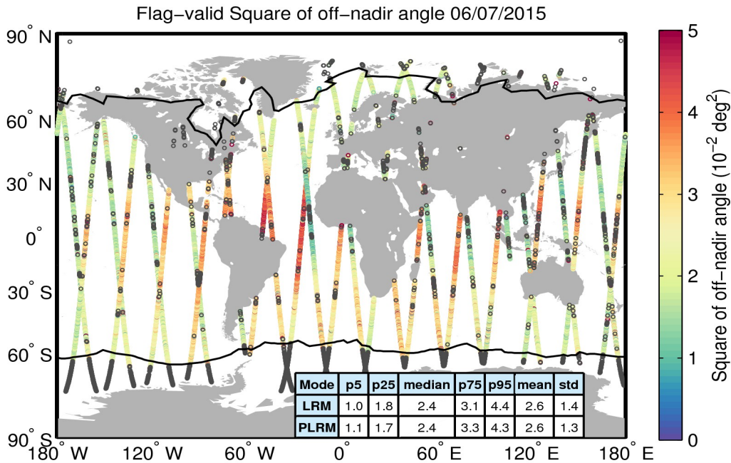
Figure 37. Geographical distribution of flag-valid mispointing data over oceans and lakes for 06/07/2015. The statistical values shown in the table refer to the mispointing in 10^{-2} \text{ deg}^2 and are calculated separately for LRM and PLRM regions. Measurements taken over polar polygons have been excluded from the computation of the statistical values. The black lines mark the outer limit of the Arctic and Antarctic polar polygons. Gray circles denote negative values.
