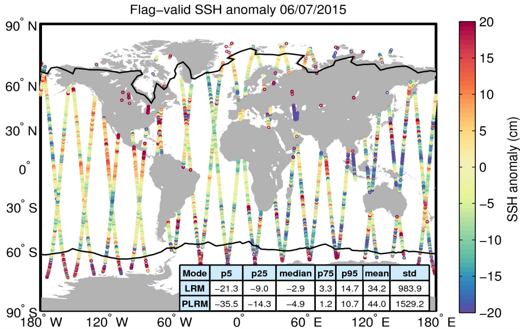
Figure 5. Geographical distribution of flag-valid 1-Hz SSH anomaly data over oceans and lakes for 06/07/2015. The statistical values shown in the table refer to the SSH anomaly in cm and are calculated separately for LRM and PLRM regions. Measurements taken over polar polygons have been excluded from the computation of the statistical values. The black lines mark the outer limit of the Arctic and Antarctic polar polygons.
