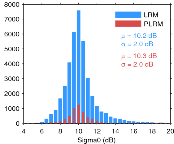
Figure 25. Histogram of flag-valid sigma0 over oceans and lakes for LRM (blue) and PLRM (red) for 06/07/2015. The mean ( \mu ) and standard deviation ( \sigma ) are also shown. Note that values outside [4 20] dB are excluded from the histogram for the sake of readability but not from the computation of \mu and \sigma .
