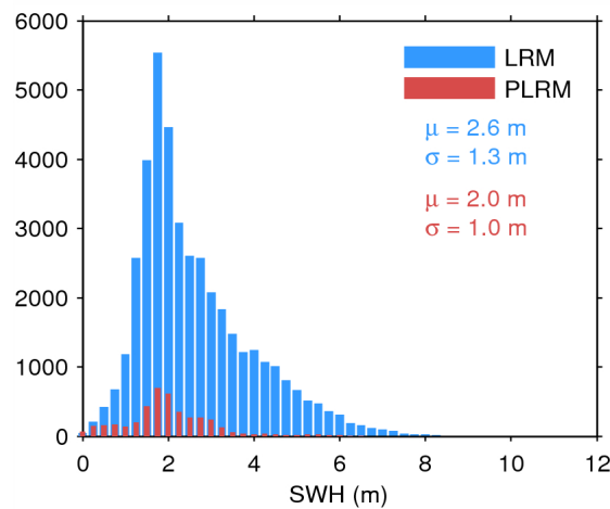
Figure 20. Histogram of science-valid SWH over oceans and lakes for LRM (blue) and PLRM (red) for 05/07/2015. The mean ( \mu ) and standard deviation ( \sigma ) are also shown. Note that values larger than 12 m are excluded from the histogram for the sake of readability but not from the computation of \mu and \sigma .
