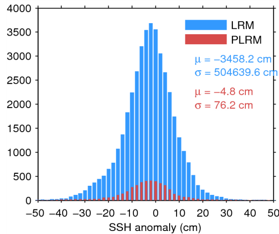
Figure 7. Histogram of flag-valid SSH anomaly over oceans and lakes for LRM (blue) and PLRM (red) for 05/07/2015. The mean ( \mu ) and standard deviation ( \sigma ) are also shown. Note that values outside [-50\ 50] cm are excluded from the histogram for the sake of readability but not from the computation of \mu and \sigma .
