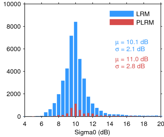
Figure 25. Histogram of flag-valid sigma0 over oceans and lakes for LRM (blue) and PLRM (red) for 05/07/2015. The mean ( \mu ) and standard deviation ( \sigma ) are also shown. Note that values outside [4 20] dB are excluded from the histogram for the sake of readability but not from the computation of \mu and \sigma .
