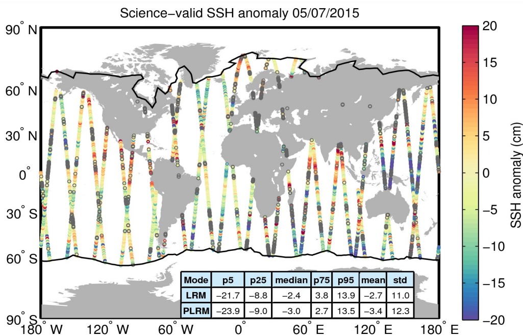
Figure 10. Geographical distribution of science-valid SSH anomaly data over oceans and lakes for 05/07/2015. The statistical values shown in the table refer to the SSH anomaly in cm and are calculated separately for LRM and PLRM regions. The black lines mark the outer limit of the Arctic and Antarctic polar polygons. Gray circles denote records that have been rejected based on the editing criteria described in Table 2.
