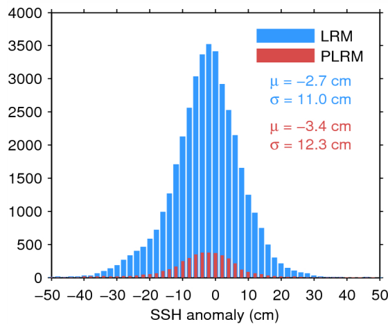
Figure 11. Histogram of science-valid SSH anomaly over oceans and lakes for LRM (blue) and PLRM (red) for 05/07/2015. The mean ( \mu ) and standard deviation ( \sigma ) are also shown. Note that values outside [-50 50] cm are excluded from the histogram for the sake of readability but not from the computation of \mu and \sigma .
