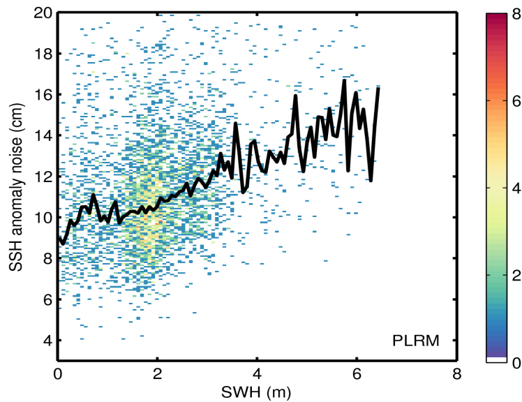
Figure 9. 2D histogram showing flag-valid SSH anomaly noise as a function of SWH for LRM (top) and PLRM (bottom) for 05/07/2015. The black line denotes the median SSH anomaly as a function of SWH.
