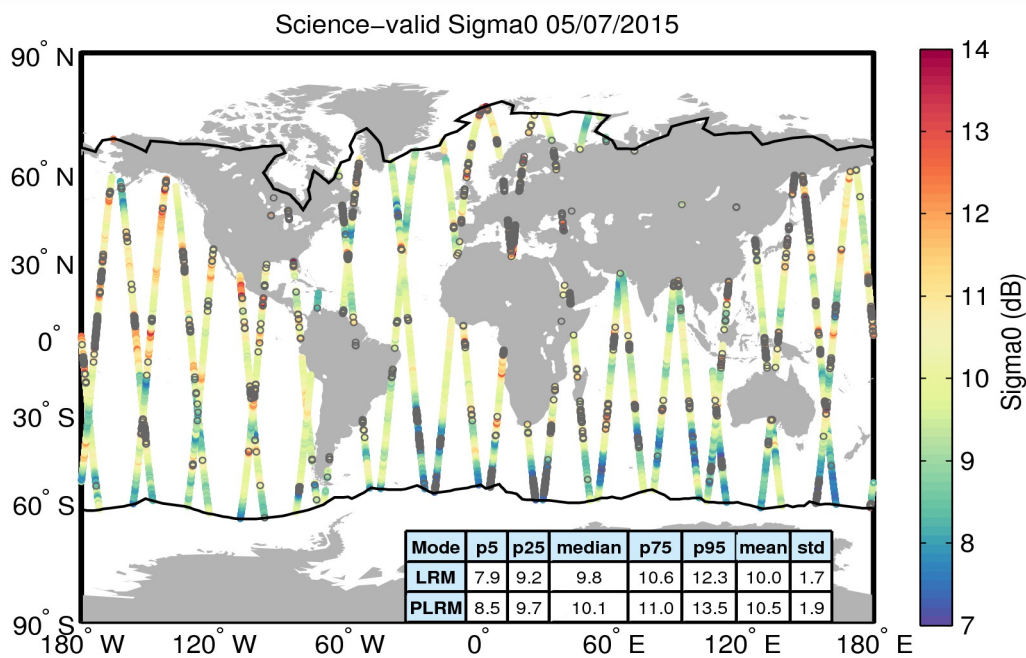
Figure 27. Geographical distribution of science-valid sigma0 data over oceans and lakes for 05/07/2015. The statistical values shown in the table refer to the sigma0 in dB and are calculated separately for LRM and PLRM regions. The black lines mark the outer limit of the Arctic and Antarctic polar polygons. Gray circles denote records that have been rejected based on the editing criteria described in Table 4.
