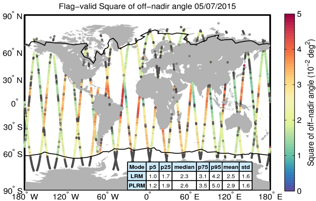
Figure 37. Geographical distribution of flag-valid mispointing data over oceans and lakes for 05/07/2015. The statistical values shown in the table refer to the mispointing in 10^{-2} deg 2 and are calculated separately for LRM and PLRM regions. Measurements taken over polar polygons have been excluded from the computation of the statistical values. The black lines mark the outer limit of the Arctic and Antarctic polar polygons. Gray circles denote negative values.
