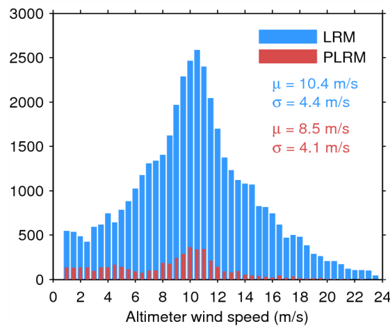
Figure 33. Histogram of flag-valid wind over oceans and lakes for LRM (blue) and PLRM (red) for 05/07/2015. The mean ( \mu ) and standard deviation ( \sigma ) are also shown. Note that values larger than 24 m/s are excluded from the histogram for the sake of readability but not from the computation of \mu and \sigma .
