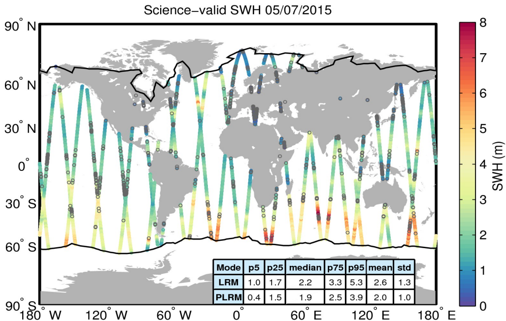
Figure 19. Geographical distribution of science-valid SWH data over oceans and lakes for 05/07/2015. The statistical values shown in the table refer to the SWH in m and are calculated separately for LRM and PLRM regions. The black lines mark the outer limit of the Arctic and Antarctic polar polygons. Gray circles denote records that have been rejected based on the editing criteria described in Table 3.
