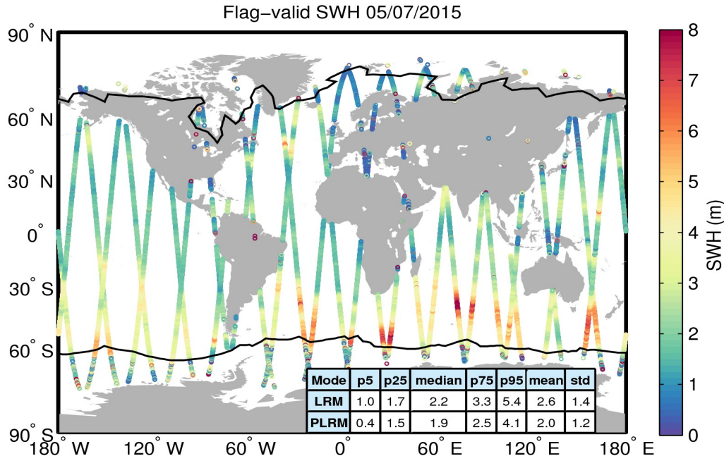
Figure 15. Geographical distribution of flag-valid SWH data over oceans and lakes for 05/07/2015. The statistical values shown in the table refer to the SWH in m and are calculated separately for LRM and PLRM regions. Measurements taken over polar polygons have been excluded from the computation of the statistical values. The black lines mark the outer limit of the Arctic and Antarctic polar polygons.
