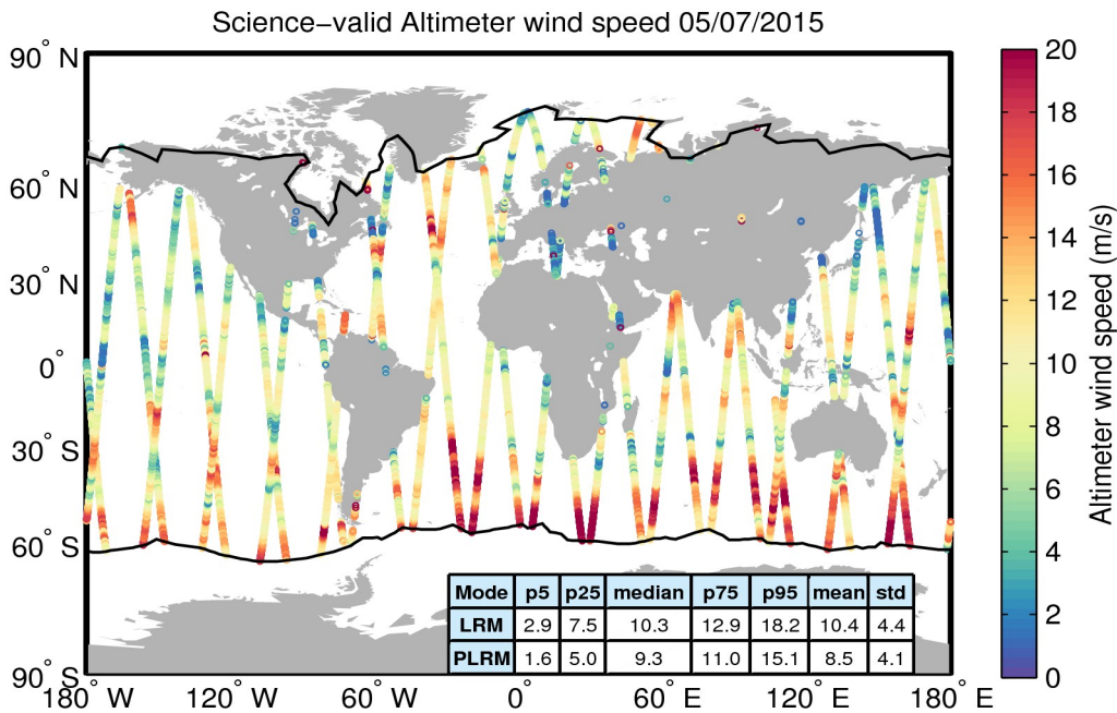
Figure 34. Geographical distribution of science-valid wind data over oceans and lakes for 05/07/2015. The statistical values shown in the table refer to the wind in m/s and are calculated separately for LRM and PLRM regions. The black lines mark the outer limit of the Arctic and Antarctic polar polygons. Gray circles denote records that have been rejected based on the editing criteria described in Table 5.
