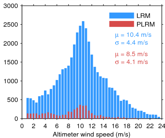
Figure 35. Histogram of science-valid wind over oceans and lakes for LRM (blue) and PLRM (red) for 05/07/2015. The mean ( \mu ) and standard deviation ( \sigma ) are also shown. Note that values larger than 24 m/s are excluded from the histogram for the sake of readability but not from the computation of \mu and \sigma .
