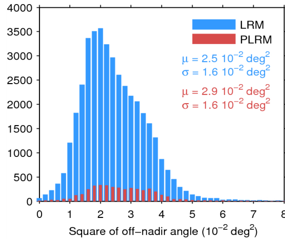
Figure 39. Histogram of flag-valid mispointing over oceans and lakes for LRM (blue) and PLRM (red) for 05/07/2015. Only positive values have been considered. The mean ( \mu ) and standard deviation ( \sigma ) are also shown. Note that values larger than 8 \cdot 10^{-2} \text{ deg}^2 are excluded from the histogram for the sake of readability but not from the computation of \mu and \sigma .
