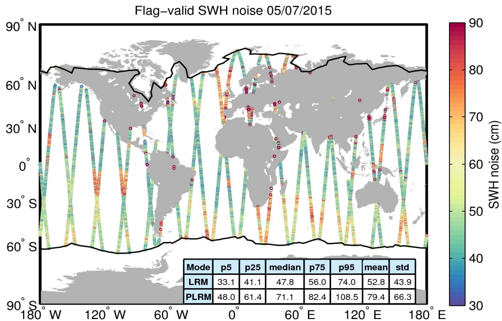
Figure 18. Geographical distribution of flag-valid 20-Hz SWH measurement noise over oceans and lakes for 05/07/2015. The statistical values shown in the table refer to the SWH noise and are calculated separately for LRM and PLRM regions. Measurements taken over polar polygons have been excluded from the computation of the statistical values. The black lines mark the outer limit of the Arctic and Antarctic polar polygons.
