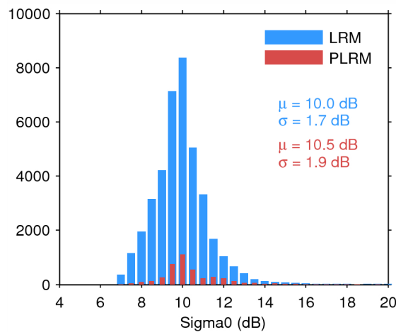
Figure 28. Histogram of science-valid sigma0 over oceans and lakes for LRM (blue) and PLRM (red) for 05/07/2015. The mean ( \mu ) and standard deviation ( \sigma ) are also shown. Note that values outside [4 20] dB are excluded from the histogram for the sake of readability but not from the computation of \mu and \sigma .
