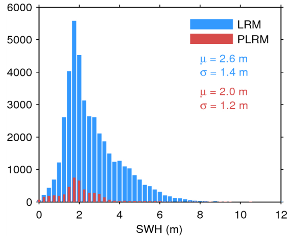
Figure 17. Histogram of flag-valid SWH over oceans and lakes for LRM (blue) and PLRM (red) for 05/07/2015. The mean ( \mu ) and standard deviation ( \sigma ) are also shown. Note that values larger than 12 m are excluded from the histogram for the sake of readability but not from the computation of \mu and \sigma .
