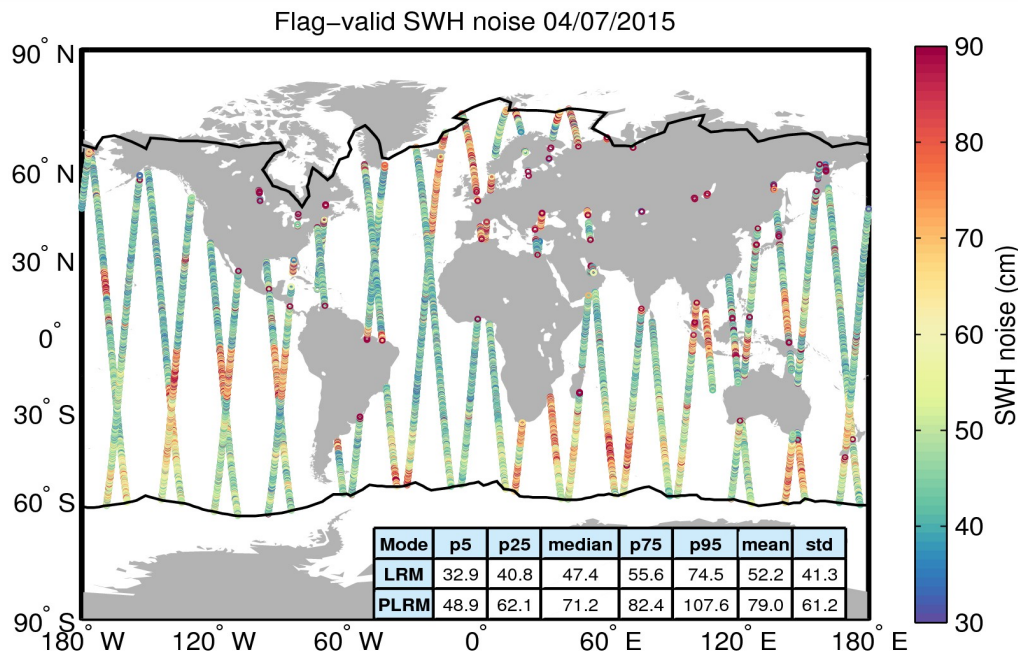
Figure 18. Geographical distribution of flag-valid 20-Hz SWH measurement noise over oceans and lakes for 04/07/2015. The statistical values shown in the table refer to the SWH noise and are calculated separately for LRM and PLRM regions. Measurements taken over polar polygons have been excluded from the computation of the statistical values. The black lines mark the outer limit of the Arctic and Antarctic polar polygons.
