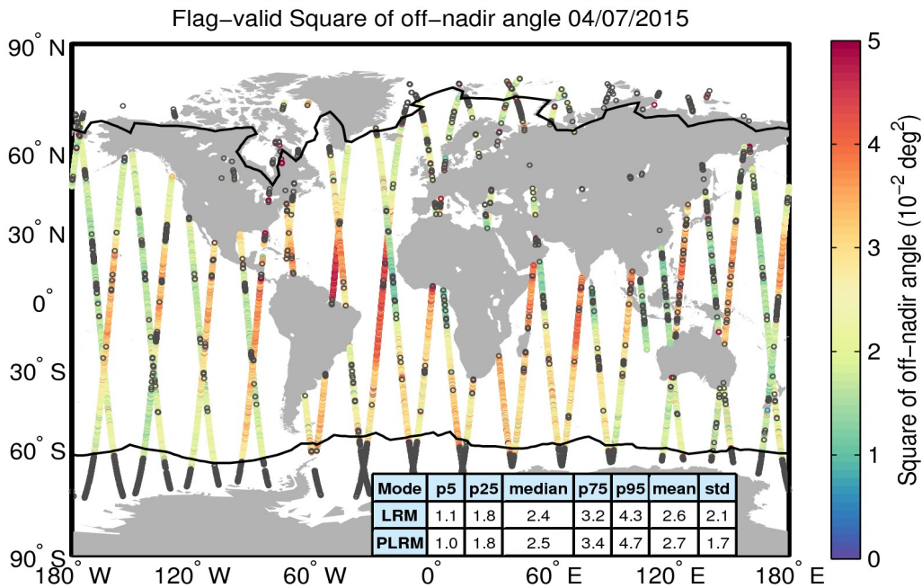
Figure 37. Geographical distribution of flag-valid mispointing data over oceans and lakes for 04/07/2015. The statistical values shown in the table refer to the mispointing in 10^{-2} deg 2 and are calculated separately for LRM and PLRM regions. Measurements taken over polar polygons have been excluded from the computation of the statistical values. The black lines mark the outer limit of the Arctic and Antarctic polar polygons. Gray circles denote negative values.
