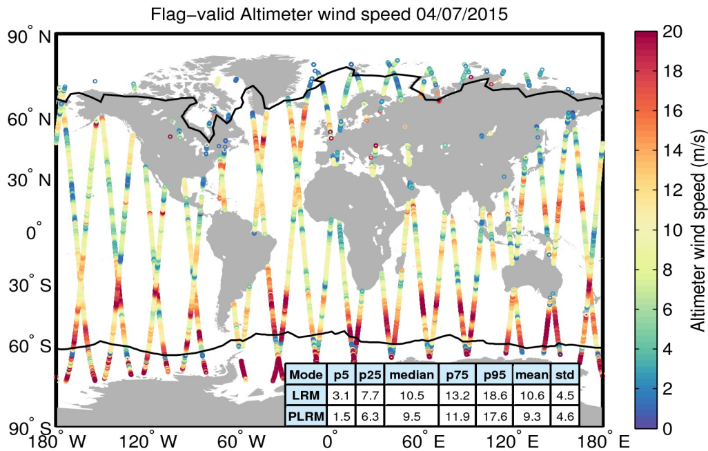
Figure 31. Geographical distribution of flag-valid wind data over oceans and lakes for 04/07/2015. The statistical values shown in the table refer to the wind in m/s and are calculated separately for LRM and PLRM regions. Measurements taken over polar polygons have been excluded from the computation of the statistical values. The black lines mark the outer limit of the Arctic and Antarctic polar polygons.
