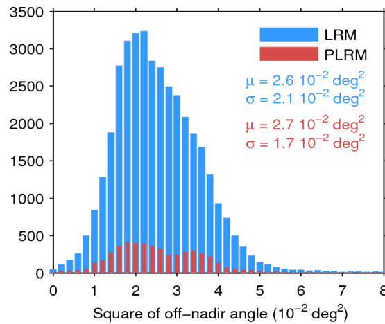
Figure 39. Histogram of flag-valid mispointing over oceans and lakes for LRM (blue) and PLRM (red) for 04/07/2015. Only positive values have been considered. The mean ( \mu ) and standard deviation ( \sigma ) are also shown. Note that values larger than 8 \cdot 10^{-2} \text{ deg}^2 are excluded from the histogram for the sake of readability but not from the computation of \mu and \sigma .
