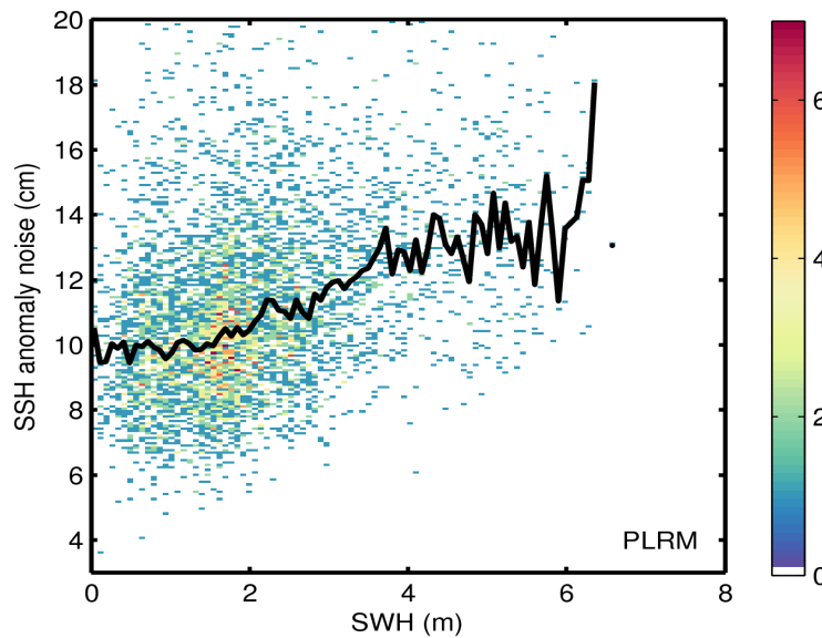
Figure 9. 2D histogram showing flag-valid SSH anomaly noise as a function of SWH for LRM (top) and PLRM (bottom) for 04/07/2015. The black line denotes the median SSH anomaly as a function of SWH.
