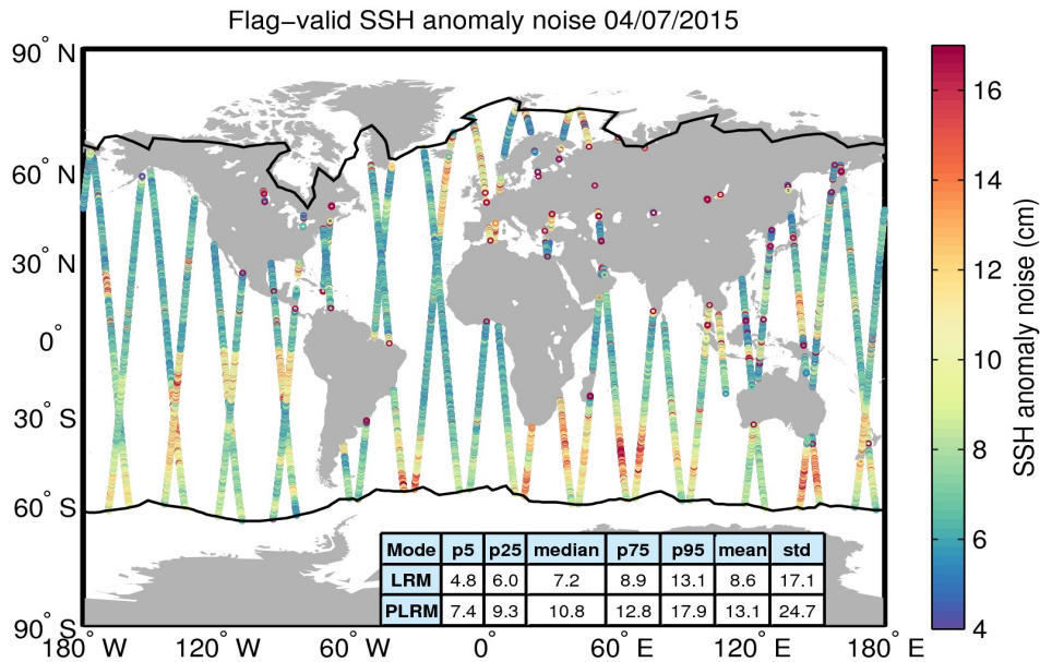
Figure 8. Geographical distribution of flag-valid 20-Hz SSH anomaly measurement noise over oceans and lakes for 04/07/2015. The statistical values shown in the table refer to the SSH anomaly noise and are calculated separately for LRM and PLRM regions. Measurements taken over polar polygons have been excluded from the computation of the statistical values. The black lines mark the outer limit of the Arctic and Antarctic polar polygons.
