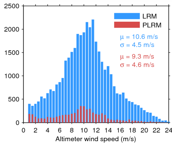
Figure 33. Histogram of flag-valid wind over oceans and lakes for LRM (blue) and PLRM (red) for 04/07/2015. The mean ( \mu ) and standard deviation ( \sigma ) are also shown. Note that values larger than 24 m/s are excluded from the histogram for the sake of readability but not from the computation of \mu and \sigma .
