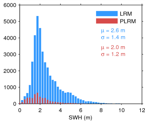
Figure 20. Histogram of science-valid SWH over oceans and lakes for LRM (blue) and PLRM (red) for 04/07/2015. The mean ( \mu ) and standard deviation ( \sigma ) are also shown. Note that values larger than 12 m are excluded from the histogram for the sake of readability but not from the computation of \mu and \sigma .
