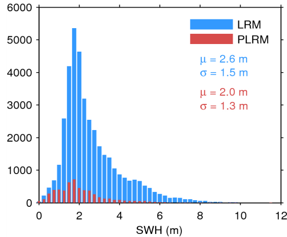
Figure 17. Histogram of flag-valid SWH over oceans and lakes for LRM (blue) and PLRM (red) for 04/07/2015. The mean ( \mu ) and standard deviation ( \sigma ) are also shown. Note that values larger than 12 m are excluded from the histogram for the sake of readability but not from the computation of \mu and \sigma .
