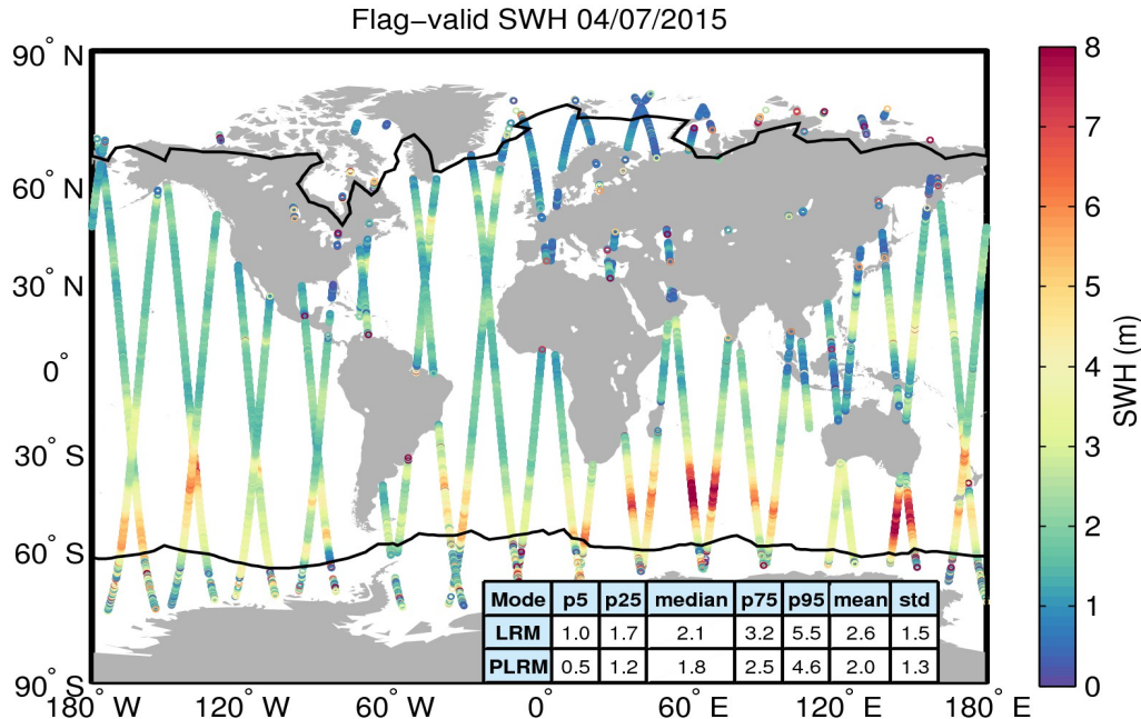
Figure 15. Geographical distribution of flag-valid SWH data over oceans and lakes for 04/07/2015. The statistical values shown in the table refer to the SWH in m and are calculated separately for LRM and PLRM regions. Measurements taken over polar polygons have been excluded from the computation of the statistical values. The black lines mark the outer limit of the Arctic and Antarctic polar polygons.
