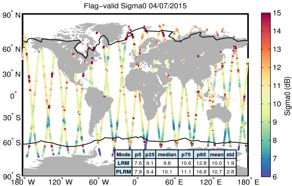
Figure 23. Geographical distribution of flag-valid sigma0 data over oceans and lakes for 04/07/2015. The statistical values shown in the table refer to the sigma0 in dB and are calculated separately for LRM and PLRM regions. Measurements taken over polar polygons have been excluded from the computation of the statistical values. The black lines mark the outer limit of the Arctic and Antarctic polar polygons.
