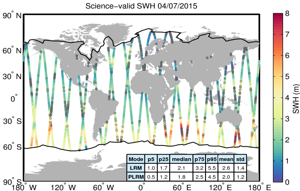
Figure 19. Geographical distribution of science-valid SWH data over oceans and lakes for 04/07/2015. The statistical values shown in the table refer to the SWH in m and are calculated separately for LRM and PLRM regions. The black lines mark the outer limit of the Arctic and Antarctic polar polygons. Gray circles denote records that have been rejected based on the editing criteria described in Table 3.
