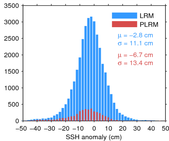
Figure 11. Histogram of science-valid SSH anomaly over oceans and lakes for LRM (blue) and PLRM (red) for 04/07/2015. The mean ( \mu ) and standard deviation ( \sigma ) are also shown. Note that values outside [-50 50] cm are excluded from the histogram for the sake of readability but not from the computation of \mu and \sigma .
