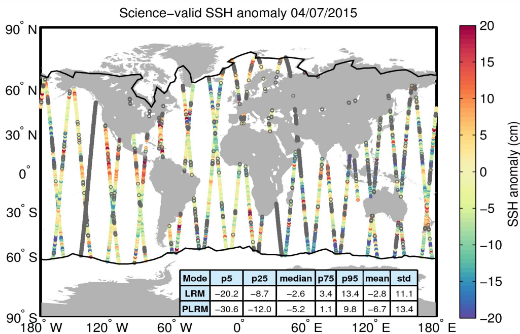
Figure 10. Geographical distribution of science-valid SSH anomaly data over oceans and lakes for 04/07/2015. The statistical values shown in the table refer to the SSH anomaly in cm and are calculated separately for LRM and PLRM regions. The black lines mark the outer limit of the Arctic and Antarctic polar polygons. Gray circles denote records that have been rejected based on the editing criteria described in Table 2.
