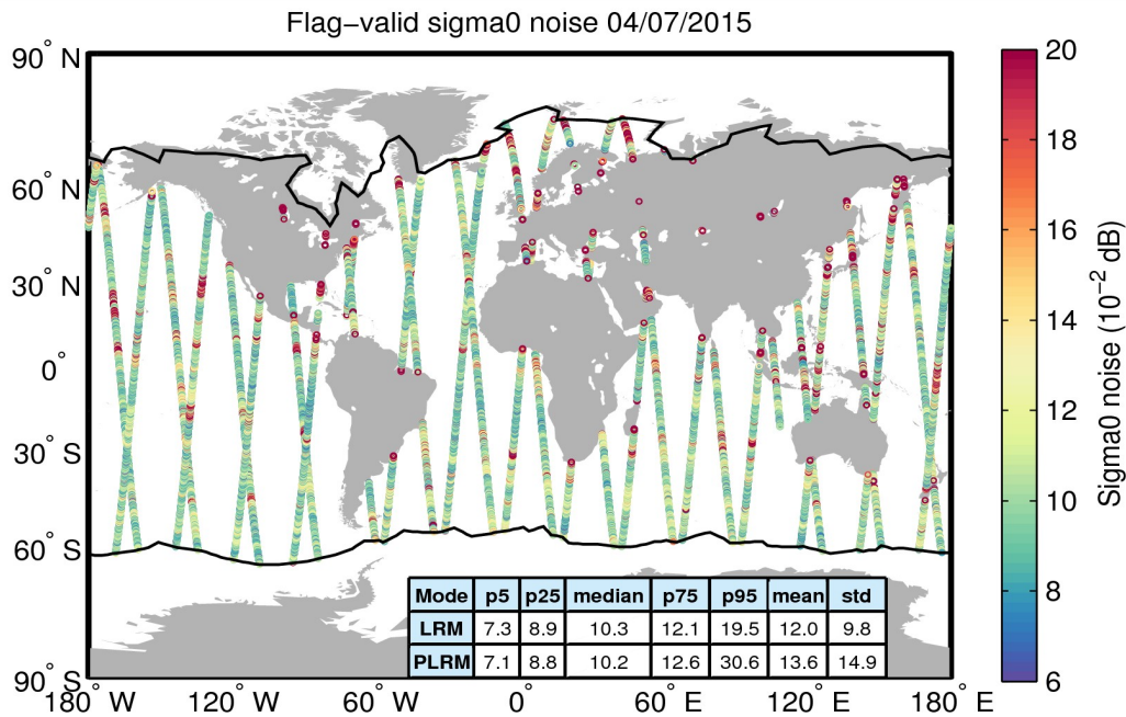
Figure 26. Geographical distribution of flag-valid 20-Hz sigma0 measurement noise over oceans and lakes for 04/07/2015. The statistical values shown in the table refer to the sigma0 noise and are calculated separately for LRM and PLRM regions. Measurements taken over polar polygons have been excluded from the computation of the statistical values. The black lines mark the outer limit of the Arctic and Antarctic polar polygons.
