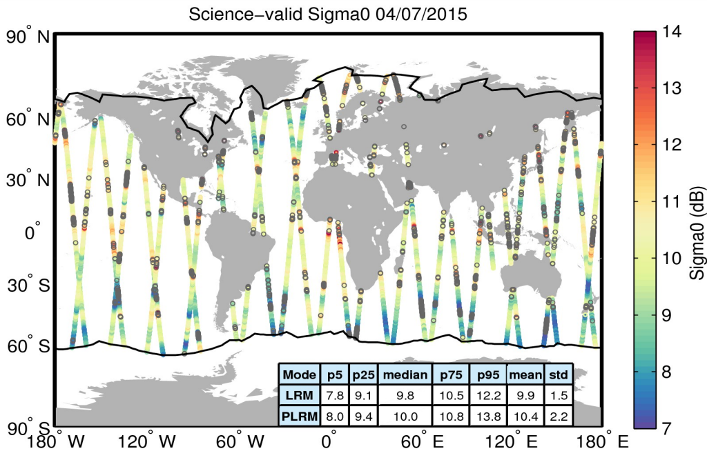
Figure 27. Geographical distribution of science-valid sigma0 data over oceans and lakes for 04/07/2015. The statistical values shown in the table refer to the sigma0 in dB and are calculated separately for LRM and PLRM regions. The black lines mark the outer limit of the Arctic and Antarctic polar polygons. Gray circles denote records that have been rejected based on the editing criteria described in Table 4.
