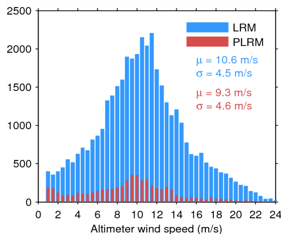
Figure 35. Histogram of science-valid wind over oceans and lakes for LRM (blue) and PLRM (red) for 04/07/2015. The mean ( \mu ) and standard deviation ( \sigma ) are also shown. Note that values larger than 24 m/s are excluded from the histogram for the sake of readability but not from the computation of \mu and \sigma .
