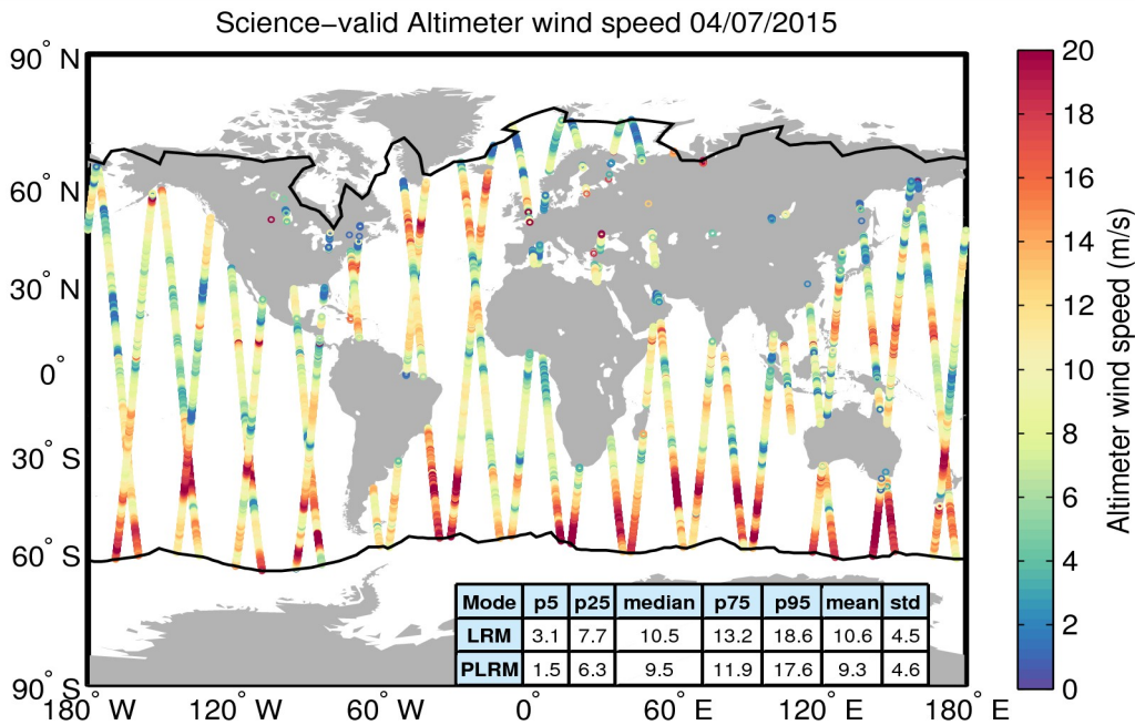
Figure 34. Geographical distribution of science-valid wind data over oceans and lakes for 04/07/2015. The statistical values shown in the table refer to the wind in m/s and are calculated separately for LRM and PLRM regions. The black lines mark the outer limit of the Arctic and Antarctic polar polygons. Gray circles denote records that have been rejected based on the editing criteria described in Table 5.
