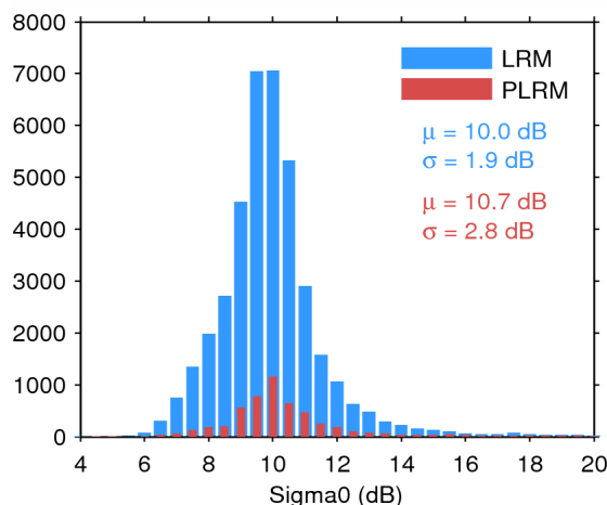
Figure 25. Histogram of flag-valid sigma0 over oceans and lakes for LRM (blue) and PLRM (red) for 04/07/2015. The mean ( \mu ) and standard deviation ( \sigma ) are also shown. Note that values outside [4 20] dB are excluded from the histogram for the sake of readability but not from the computation of \mu and \sigma .
