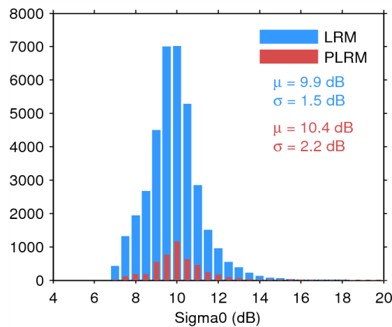
Figure 28. Histogram of science-valid sigma0 over oceans and lakes for LRM (blue) and PLRM (red) for 04/07/2015. The mean ( \mu ) and standard deviation ( \sigma ) are also shown. Note that values outside [4 20] dB are excluded from the histogram for the sake of readability but not from the computation of \mu and \sigma .
