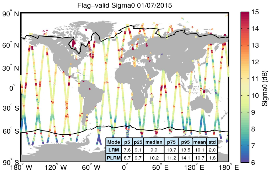
Figure 23. Geographical distribution of flag-valid sigma0 data over oceans and lakes for 01/07/2015. The statistical values shown in the table refer to the sigma0 in dB and are calculated separately for LRM and PLRM regions. Measurements taken over polar polygons have been excluded from the computation of the statistical values. The black lines mark the outer limit of the Arctic and Antarctic polar polygons.
