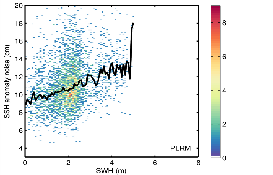
Figure 9. 2D histogram showing flag-valid SSH anomaly noise as a function of SWH for LRM (top) and PLRM (bottom) for 01/07/2015. The black line denotes the median SSH anomaly as a function of SWH.
