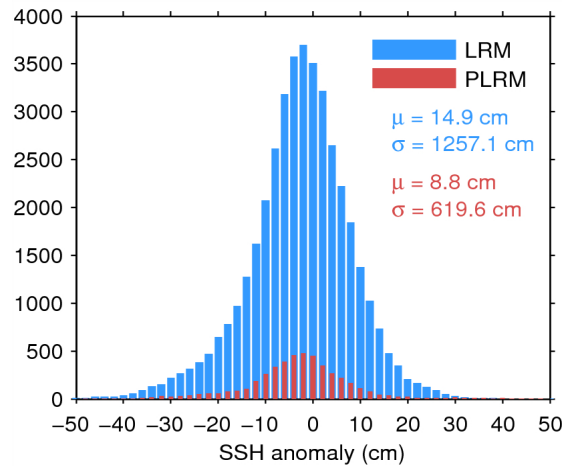
Figure 7. Histogram of flag-valid SSH anomaly over oceans and lakes for LRM (blue) and PLRM (red) for 01/07/2015. The mean ( \mu ) and standard deviation ( \sigma ) are also shown. Note that values outside [-50\ 50] cm are excluded from the histogram for the sake of readability but not from the computation of \mu and \sigma .
