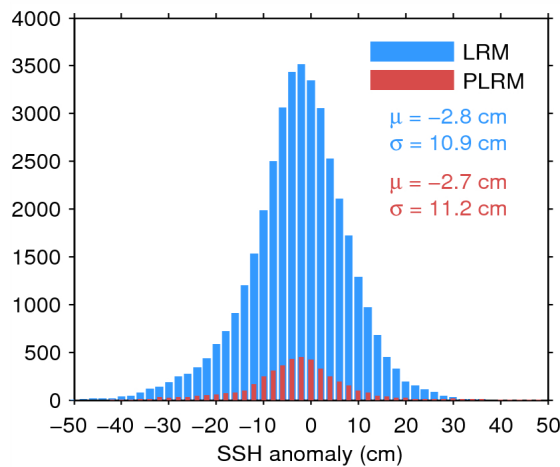
Figure 11. Histogram of science-valid SSH anomaly over oceans and lakes for LRM (blue) and PLRM (red) for 01/07/2015. The mean ( \mu ) and standard deviation ( \sigma ) are also shown. Note that values outside [-50\ 50] cm are excluded from the histogram for the sake of readability but not from the computation of \mu and \sigma .
