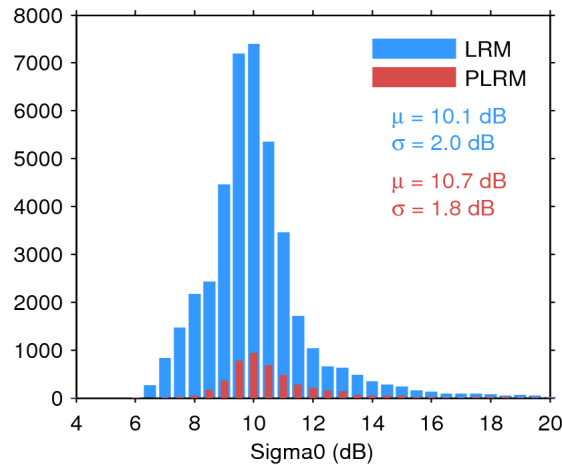
Figure 25. Histogram of flag-valid sigma0 over oceans and lakes for LRM (blue) and PLRM (red) for 01/07/2015. The mean ( \mu ) and standard deviation ( \sigma ) are also shown. Note that values outside [4 20] dB are excluded from the histogram for the sake of readability but not from the computation of \mu and \sigma .
