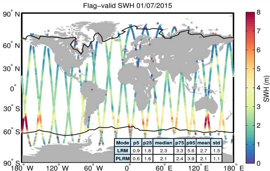
Figure 15. Geographical distribution of flag-valid SWH data over oceans and lakes for 01/07/2015. The statistical values shown in the table refer to the SWH in m and are calculated separately for LRM and PLRM regions. Measurements taken over polar polygons have been excluded from the computation of the statistical values. The black lines mark the outer limit of the Arctic and Antarctic polar polygons.
