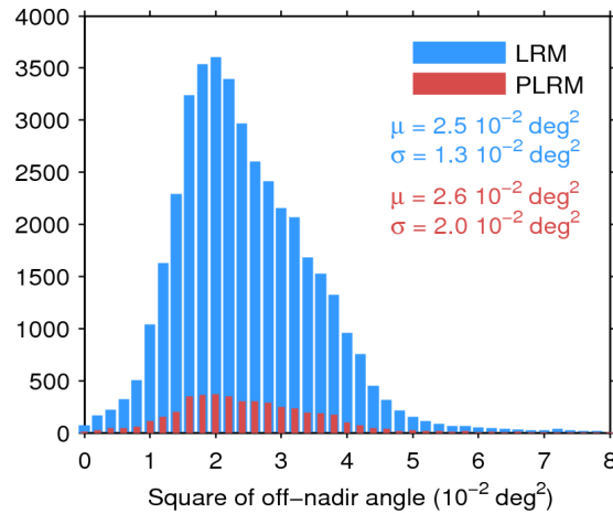
Figure 39. Histogram of flag-valid mispointing over oceans and lakes for LRM (blue) and PLRM (red) for 01/07/2015. Only positive values have been considered. The mean ( \mu ) and standard deviation ( \sigma ) are also shown. Note that values larger than 8 \cdot 10^{-2} \text{ deg}^2 are excluded from the histogram for the sake of readability but not from the computation of \mu and \sigma .
