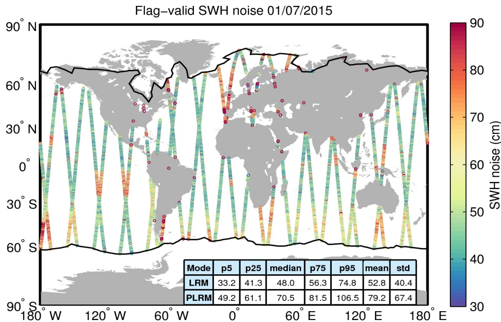
Figure 18. Geographical distribution of flag-valid 20-Hz SWH measurement noise over oceans and lakes for 01/07/2015. The statistical values shown in the table refer to the SWH noise and are calculated separately for LRM and PLRM regions. Measurements taken over polar polygons have been excluded from the computation of the statistical values. The black lines mark the outer limit of the Arctic and Antarctic polar polygons.
