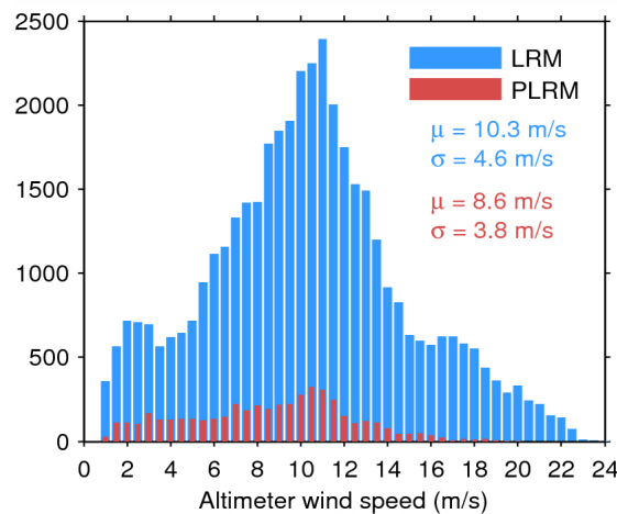
Figure 35. Histogram of science-valid wind over oceans and lakes for LRM (blue) and PLRM (red) for 01/07/2015. The mean ( \mu ) and standard deviation ( \sigma ) are also shown. Note that values larger than 24 m/s are excluded from the histogram for the sake of readability but not from the computation of \mu and \sigma .
