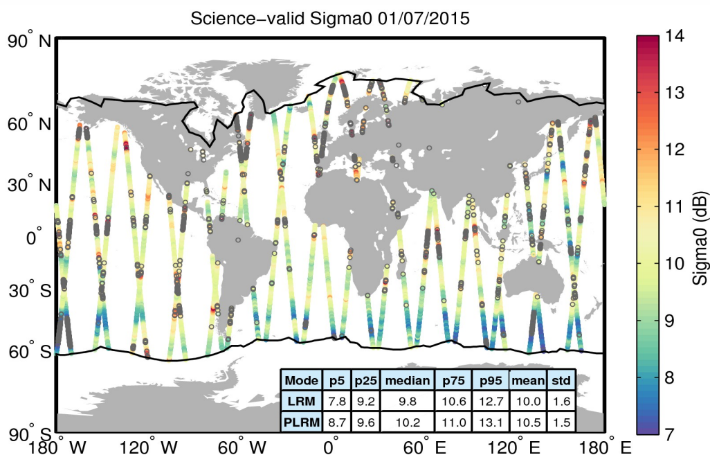
Figure 27. Geographical distribution of science-valid sigma0 data over oceans and lakes for 01/07/2015. The statistical values shown in the table refer to the sigma0 in dB and are calculated separately for LRM and PLRM regions. The black lines mark the outer limit of the Arctic and Antarctic polar polygons. Gray circles denote records that have been rejected based on the editing criteria described in Table 4.
