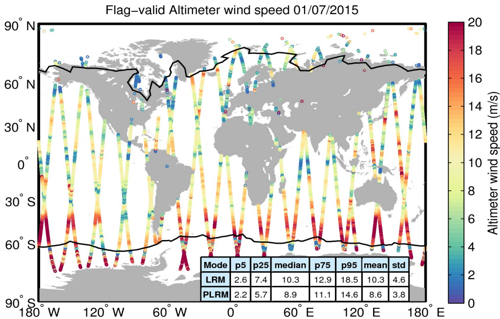
Figure 31. Geographical distribution of flag-valid wind data over oceans and lakes for 01/07/2015. The statistical values shown in the table refer to the wind in m/s and are calculated separately for LRM and PLRM regions. Measurements taken over polar polygons have been excluded from the computation of the statistical values. The black lines mark the outer limit of the Arctic and Antarctic polar polygons.
