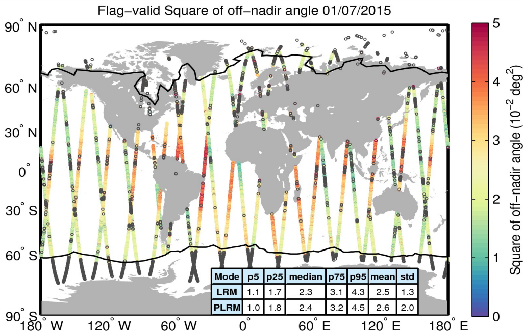
Figure 37. Geographical distribution of flag-valid mispointing data over oceans and lakes for 01/07/2015. The statistical values shown in the table refer to the mispointing in 10^{-2} deg 2 and are calculated separately for LRM and PLRM regions. Measurements taken over polar polygons have been excluded from the computation of the statistical values. The black lines mark the outer limit of the Arctic and Antarctic polar polygons. Gray circles denote negative values.
