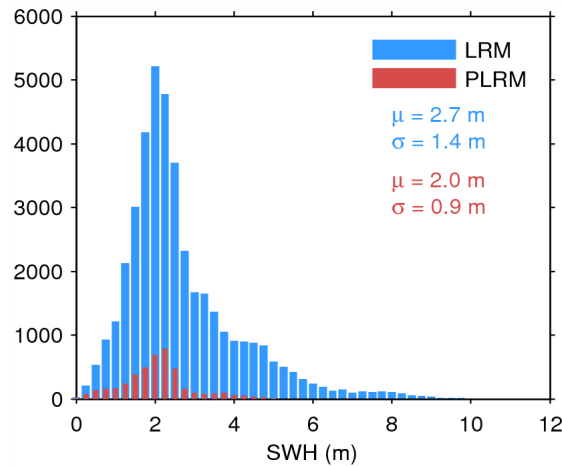
Figure 20. Histogram of science-valid SWH over oceans and lakes for LRM (blue) and PLRM (red) for 01/07/2015. The mean ( \mu ) and standard deviation ( \sigma ) are also shown. Note that values larger than 12 m are excluded from the histogram for the sake of readability but not from the computation of \mu and \sigma .
