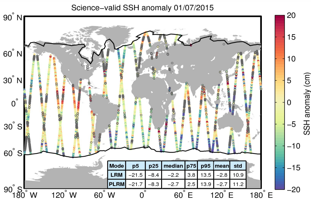
Figure 10. Geographical distribution of science-valid SSH anomaly data over oceans and lakes for 01/07/2015. The statistical values shown in the table refer to the SSH anomaly in cm and are calculated separately for LRM and PLRM regions. The black lines mark the outer limit of the Arctic and Antarctic polar polygons. Gray circles denote records that have been rejected based on the editing criteria described in Table 2.
