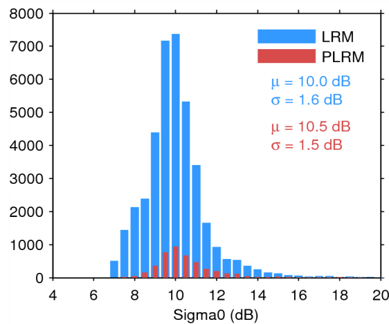
Figure 28. Histogram of science-valid sigma0 over oceans and lakes for LRM (blue) and PLRM (red) for 01/07/2015. The mean ( \mu ) and standard deviation ( \sigma ) are also shown. Note that values outside [4 20] dB are excluded from the histogram for the sake of readability but not from the computation of \mu and \sigma .
