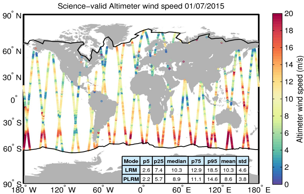
Figure 34. Geographical distribution of science-valid wind data over oceans and lakes for 01/07/2015. The statistical values shown in the table refer to the wind in m/s and are calculated separately for LRM and PLRM regions. The black lines mark the outer limit of the Arctic and Antarctic polar polygons. Gray circles denote records that have been rejected based on the editing criteria described in Table 5.
