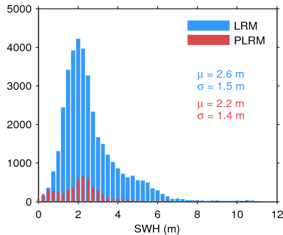
Figure 17. Histogram of flag-valid SWH over oceans and lakes for LRM (blue) and PLRM (red) for 30/06/2015. The mean ( \mu ) and standard deviation ( \sigma ) are also shown. Note that values larger than 12 m are excluded from the histogram for the sake of readability but not from the computation of \mu and \sigma .
