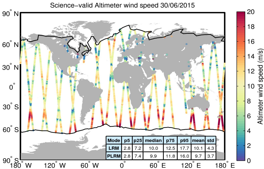
Figure 34. Geographical distribution of science-valid wind data over oceans and lakes for 30/06/2015. The statistical values shown in the table refer to the wind in m/s and are calculated separately for LRM and PLRM regions. The black lines mark the outer limit of the Arctic and Antarctic polar polygons. Gray circles denote records that have been rejected based on the editing criteria described in Table 5.
