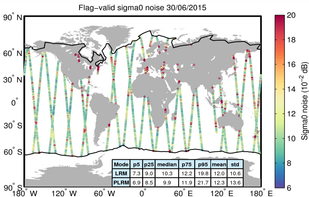
Figure 26. Geographical distribution of flag-valid 20-Hz sigma0 measurement noise over oceans and lakes for 30/06/2015. The statistical values shown in the table refer to the sigma0 noise and are calculated separately for LRM and PLRM regions. Measurements taken over polar polygons have been excluded from the computation of the statistical values. The black lines mark the outer limit of the Arctic and Antarctic polar polygons.
