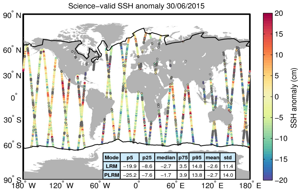
Figure 10. Geographical distribution of science-valid SSH anomaly data over oceans and lakes for 30/06/2015. The statistical values shown in the table refer to the SSH anomaly in cm and are calculated separately for LRM and PLRM regions. The black lines mark the outer limit of the Arctic and Antarctic polar polygons. Gray circles denote records that have been rejected based on the editing criteria described in Table 2.
