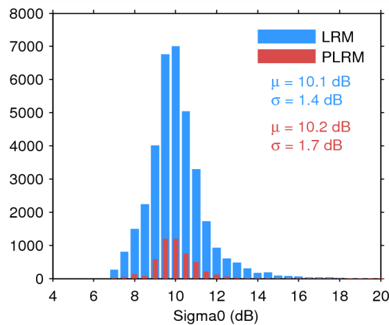
Figure 28. Histogram of science-valid sigma0 over oceans and lakes for LRM (blue) and PLRM (red) for 30/06/2015. The mean ( \mu ) and standard deviation ( \sigma ) are also shown. Note that values outside [4 20] dB are excluded from the histogram for the sake of readability but not from the computation of \mu and \sigma .
