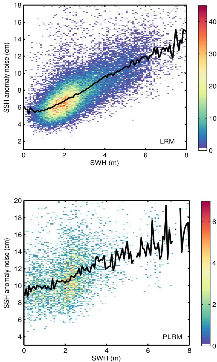
Figure 9. 2D histogram showing flag-valid SSH anomaly noise as a function of SWH for LRM (top) and PLRM (bottom) for 30/06/2015. The black line denotes the median SSH anomaly as a function of SWH.
