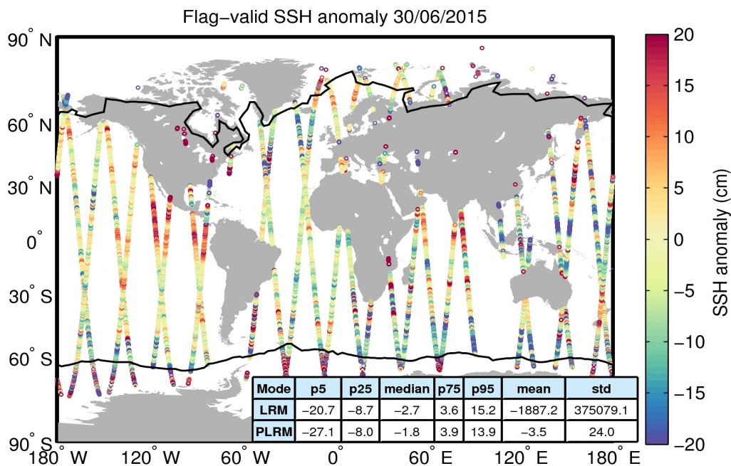
Figure 5. Geographical distribution of flag-valid 1-Hz SSH anomaly data over oceans and lakes for 30/06/2015. The statistical values shown in the table refer to the SSH anomaly in cm and are calculated separately for LRM and PLRM regions. Measurements taken over polar polygons have been excluded from the computation of the statistical values. The black lines mark the outer limit of the Arctic and Antarctic polar polygons.
