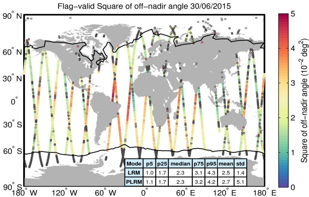
Figure 37. Geographical distribution of flag-valid mispointing data over oceans and lakes for 30/06/2015. The statistical values shown in the table refer to the mispointing in 10^{-2} \text{ deg}^2 and are calculated separately for LRM and PLRM regions. Measurements taken over polar polygons have been excluded from the computation of the statistical values. The black lines mark the outer limit of the Arctic and Antarctic polar polygons. Gray circles denote negative values.
