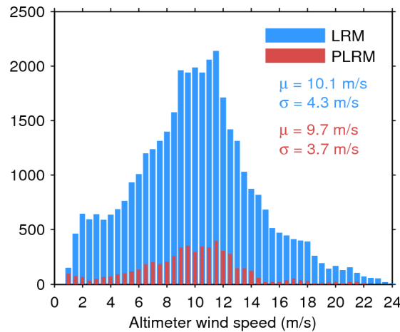
Figure 33. Histogram of flag-valid wind over oceans and lakes for LRM (blue) and PLRM (red) for 30/06/2015. The mean ( \mu ) and standard deviation ( \sigma ) are also shown. Note that values larger than 24 m/s are excluded from the histogram for the sake of readability but not from the computation of \mu and \sigma .
