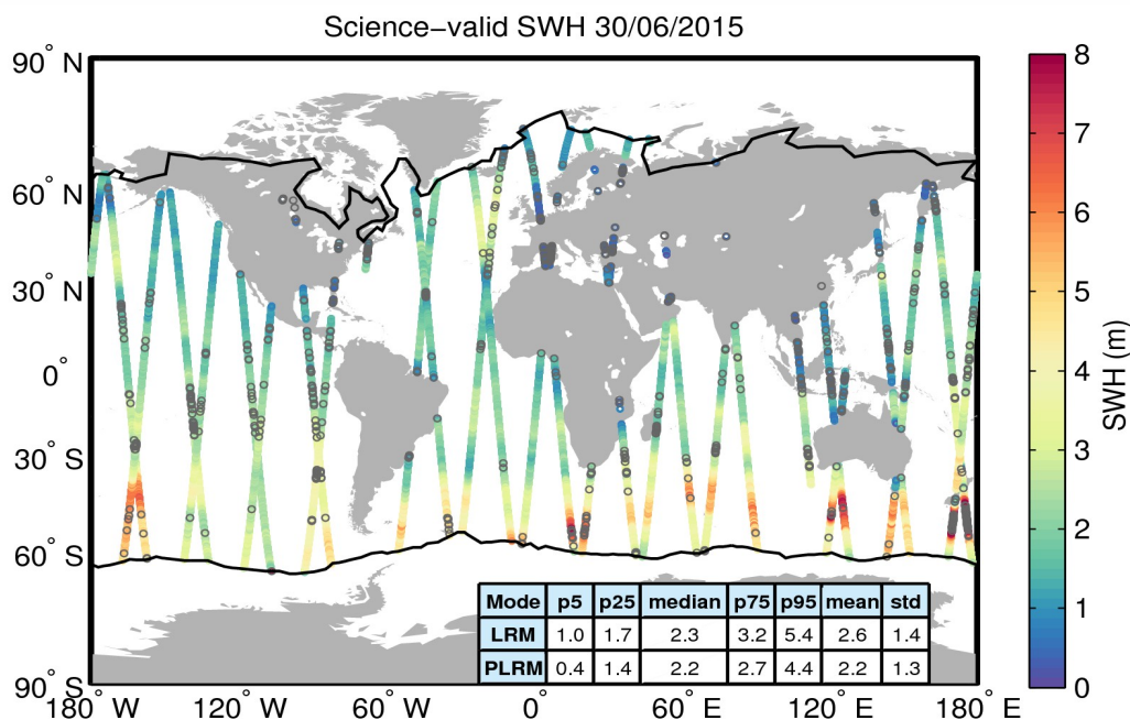
Figure 19. Geographical distribution of science-valid SWH data over oceans and lakes for 30/06/2015. The statistical values shown in the table refer to the SWH in m and are calculated separately for LRM and PLRM regions. The black lines mark the outer limit of the Arctic and Antarctic polar polygons. Gray circles denote records that have been rejected based on the editing criteria described in Table 3.
