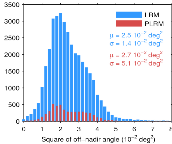
Figure 39. Histogram of flag-valid mispointing over oceans and lakes for LRM (blue) and PLRM (red) for 30/06/2015. Only positive values have been considered. The mean ( \mu ) and standard deviation ( \sigma ) are also shown. Note that values larger than 8 \cdot 10^{-2} \text{ deg}^2 are excluded from the histogram for the sake of readability but not from the computation of \mu and \sigma .
