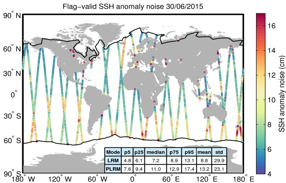
Figure 8. Geographical distribution of flag-valid 20-Hz SSH anomaly measurement noise over oceans and lakes for 30/06/2015. The statistical values shown in the table refer to the SSH anomaly noise and are calculated separately for LRM and PLRM regions. Measurements taken over polar polygons have been excluded from the computation of the statistical values. The black lines mark the outer limit of the Arctic and Antarctic polar polygons.
