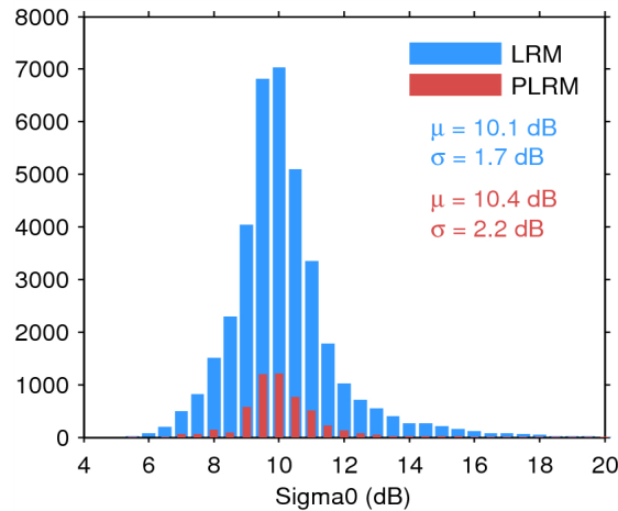
Figure 25. Histogram of flag-valid sigma0 over oceans and lakes for LRM (blue) and PLRM (red) for 30/06/2015. The mean ( \mu ) and standard deviation ( \sigma ) are also shown. Note that values outside [4 20] dB are excluded from the histogram for the sake of readability but not from the computation of \mu and \sigma .
