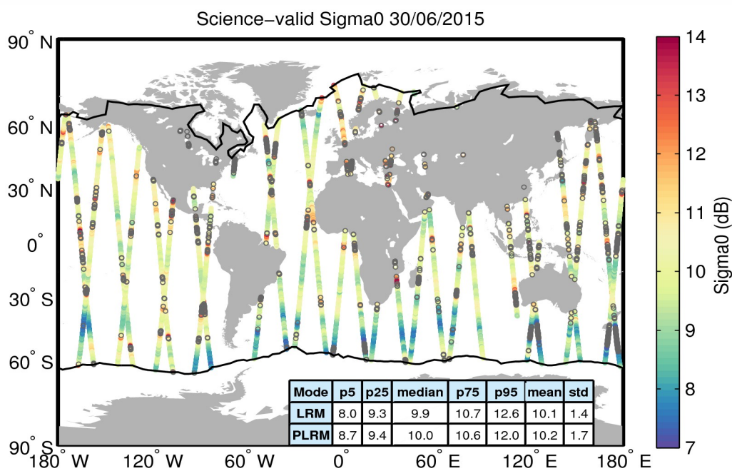
Figure 27. Geographical distribution of science-valid sigma0 data over oceans and lakes for 30/06/2015. The statistical values shown in the table refer to the sigma0 in dB and are calculated separately for LRM and PLRM regions. The black lines mark the outer limit of the Arctic and Antarctic polar polygons. Gray circles denote records that have been rejected based on the editing criteria described in Table 4.
