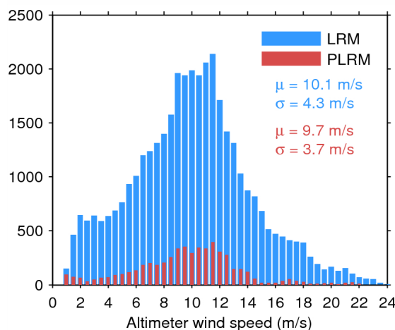
Figure 35. Histogram of science-valid wind over oceans and lakes for LRM (blue) and PLRM (red) for 30/06/2015. The mean ( \mu ) and standard deviation ( \sigma ) are also shown. Note that values larger than 24 m/s are excluded from the histogram for the sake of readability but not from the computation of \mu and \sigma .
