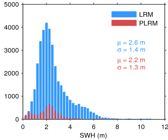
Figure 20. Histogram of science-valid SWH over oceans and lakes for LRM (blue) and PLRM (red) for 30/06/2015. The mean ( \mu ) and standard deviation ( \sigma ) are also shown. Note that values larger than 12 m are excluded from the histogram for the sake of readability but not from the computation of \mu and \sigma .
