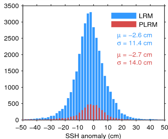
Figure 11. Histogram of science-valid SSH anomaly over oceans and lakes for LRM (blue) and PLRM (red) for 30/06/2015. The mean ( \mu ) and standard deviation ( \sigma ) are also shown. Note that values outside [-50 50] cm are excluded from the histogram for the sake of readability but not from the computation of \mu and \sigma .
