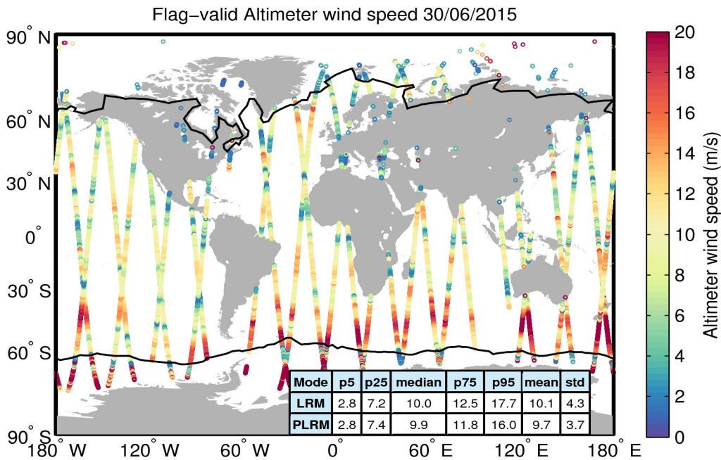
Figure 31. Geographical distribution of flag-valid wind data over oceans and lakes for 30/06/2015. The statistical values shown in the table refer to the wind in m/s and are calculated separately for LRM and PLRM regions. Measurements taken over polar polygons have been excluded from the computation of the statistical values. The black lines mark the outer limit of the Arctic and Antarctic polar polygons.
