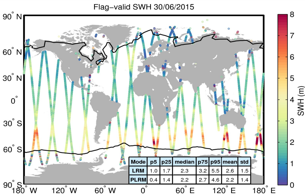
Figure 15. Geographical distribution of flag-valid SWH data over oceans and lakes for 30/06/2015. The statistical values shown in the table refer to the SWH in m and are calculated separately for LRM and PLRM regions. Measurements taken over polar polygons have been excluded from the computation of the statistical values. The black lines mark the outer limit of the Arctic and Antarctic polar polygons.
