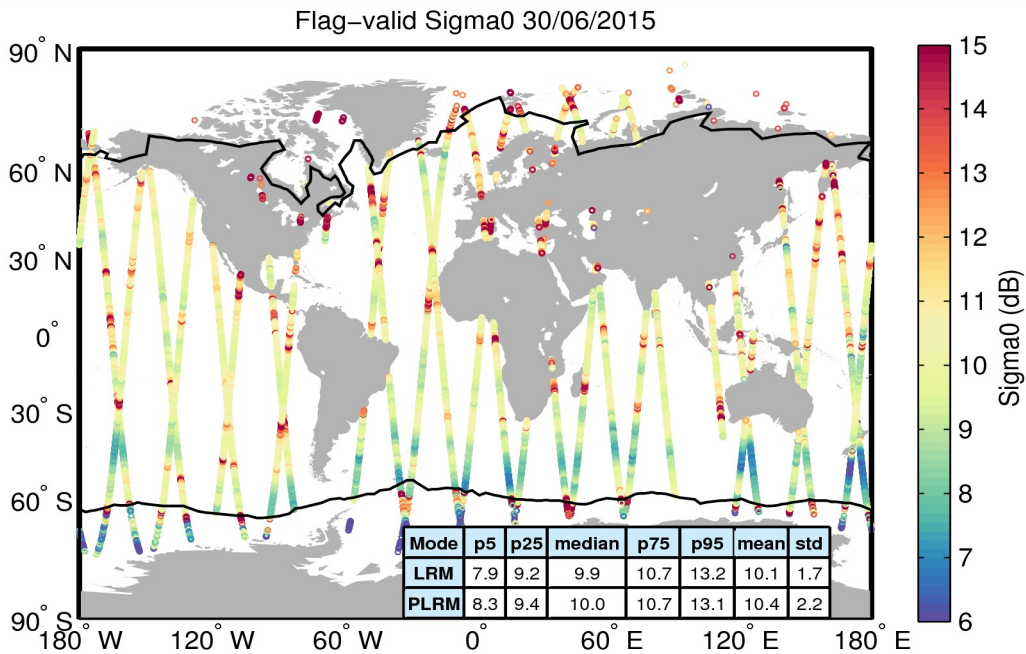
Figure 23. Geographical distribution of flag-valid sigma0 data over oceans and lakes for 30/06/2015. The statistical values shown in the table refer to the sigma0 in dB and are calculated separately for LRM and PLRM regions. Measurements taken over polar polygons have been excluded from the computation of the statistical values. The black lines mark the outer limit of the Arctic and Antarctic polar polygons.
