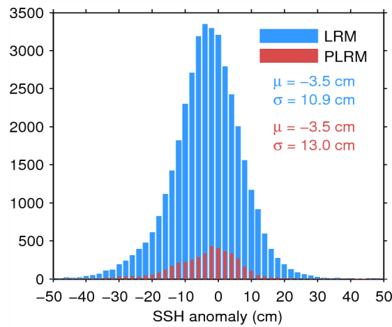
Figure 11. Histogram of science-valid SSH anomaly over oceans and lakes for LRM (blue) and PLRM (red) for 27/06/2015. The mean ( \mu ) and standard deviation ( \sigma ) are also shown. Note that values outside [-50\ 50] cm are excluded from the histogram for the sake of readability but not from the computation of \mu and \sigma .
