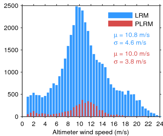
Figure 33. Histogram of flag-valid wind over oceans and lakes for LRM (blue) and PLRM (red) for 27/06/2015. The mean ( \mu ) and standard deviation ( \sigma ) are also shown. Note that values larger than 24 m/s are excluded from the histogram for the sake of readability but not from the computation of \mu and \sigma .
