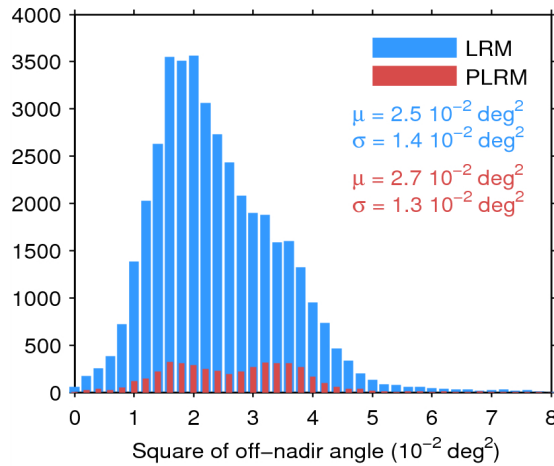
Figure 39. Histogram of flag-valid mispointing over oceans and lakes for LRM (blue) and PLRM (red) for 27/06/2015. Only positive values have been considered. The mean ( \mu ) and standard deviation ( \sigma ) are also shown. Note that values larger than 8 \cdot 10^{-2} \text{ deg}^2 are excluded from the histogram for the sake of readability but not from the computation of \mu and \sigma .
