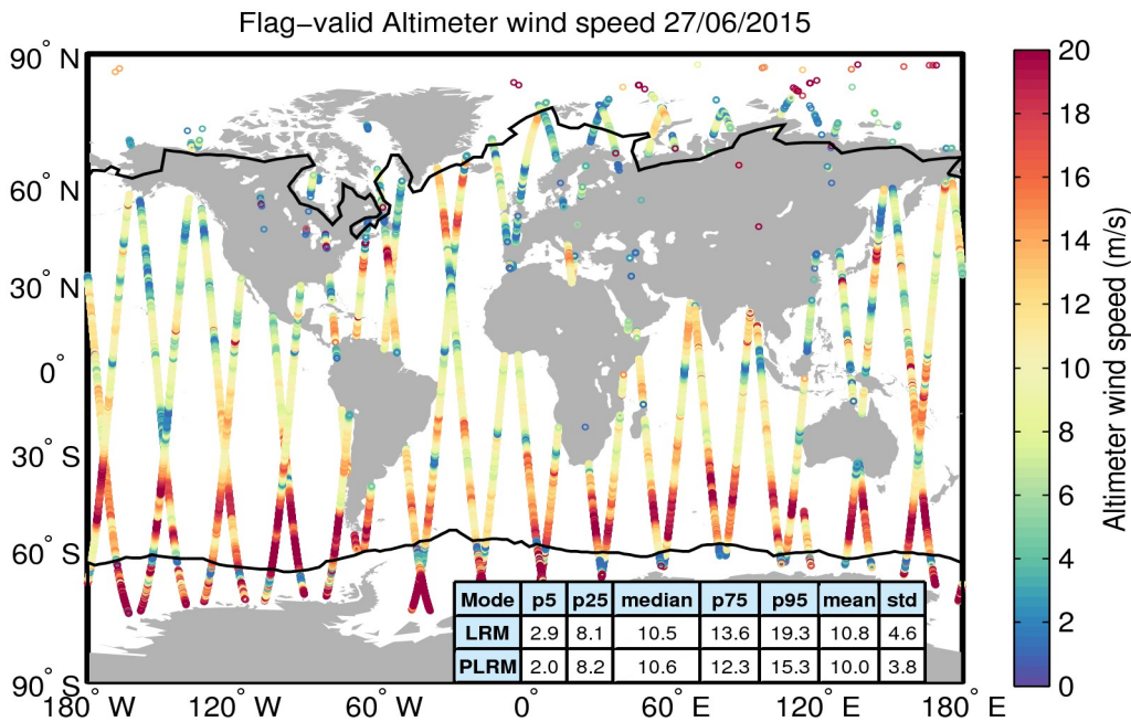
Figure 31. Geographical distribution of flag-valid wind data over oceans and lakes for 27/06/2015. The statistical values shown in the table refer to the wind in m/s and are calculated separately for LRM and PLRM regions. Measurements taken over polar polygons have been excluded from the computation of the statistical values. The black lines mark the outer limit of the Arctic and Antarctic polar polygons.
