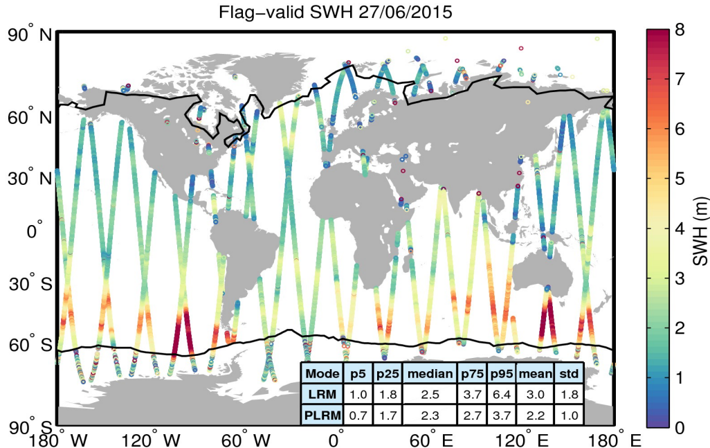
Figure 15. Geographical distribution of flag-valid SWH data over oceans and lakes for 27/06/2015. The statistical values shown in the table refer to the SWH in m and are calculated separately for LRM and PLRM regions. Measurements taken over polar polygons have been excluded from the computation of the statistical values. The black lines mark the outer limit of the Arctic and Antarctic polar polygons.
