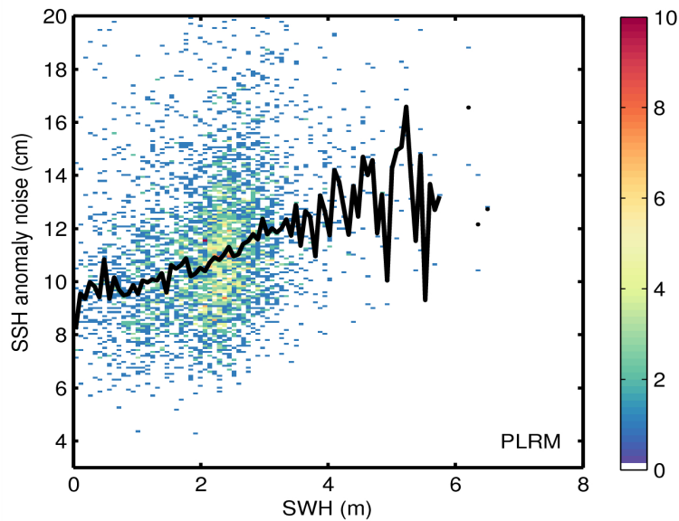
Figure 9. 2D histogram showing flag-valid SSH anomaly noise as a function of SWH for LRM (top) and PLRM (bottom) for 27/06/2015. The black line denotes the median SSH anomaly as a function of SWH.
