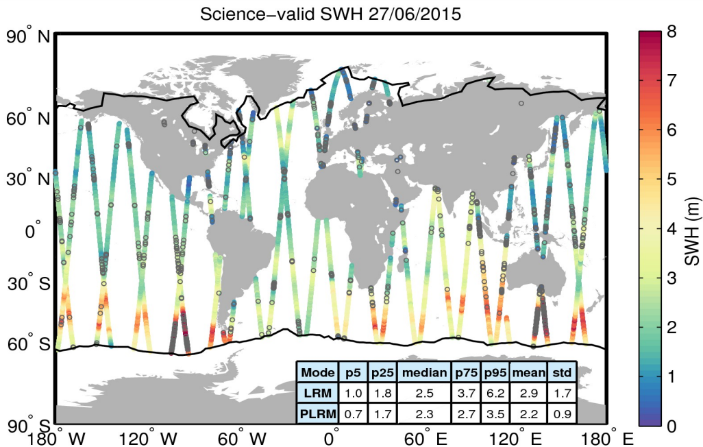
Figure 19. Geographical distribution of science-valid SWH data over oceans and lakes for 27/06/2015. The statistical values shown in the table refer to the SWH in m and are calculated separately for LRM and PLRM regions. The black lines mark the outer limit of the Arctic and Antarctic polar polygons. Gray circles denote records that have been rejected based on the editing criteria described in Table 3.
