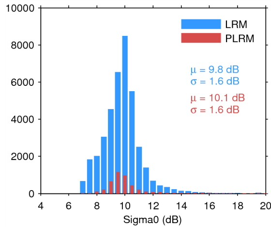
Figure 28. Histogram of science-valid sigma0 over oceans and lakes for LRM (blue) and PLRM (red) for 27/06/2015. The mean ( \mu ) and standard deviation ( \sigma ) are also shown. Note that values outside [4 20] dB are excluded from the histogram for the sake of readability but not from the computation of \mu and \sigma .
