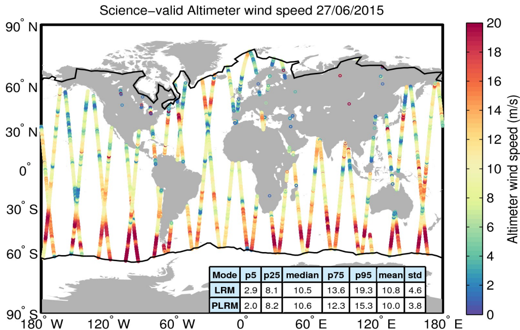
Figure 34. Geographical distribution of science-valid wind data over oceans and lakes for 27/06/2015. The statistical values shown in the table refer to the wind in m/s and are calculated separately for LRM and PLRM regions. The black lines mark the outer limit of the Arctic and Antarctic polar polygons. Gray circles denote records that have been rejected based on the editing criteria described in Table 5.
