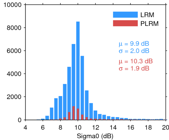
Figure 25. Histogram of flag-valid sigma0 over oceans and lakes for LRM (blue) and PLRM (red) for 27/06/2015. The mean ( \mu ) and standard deviation ( \sigma ) are also shown. Note that values outside [4 20] dB are excluded from the histogram for the sake of readability but not from the computation of \mu and \sigma .
