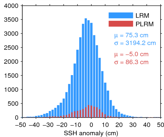
Figure 7. Histogram of flag-valid SSH anomaly over oceans and lakes for LRM (blue) and PLRM (red) for 27/06/2015. The mean ( \mu ) and standard deviation ( \sigma ) are also shown. Note that values outside [-50 50] cm are excluded from the histogram for the sake of readability but not from the computation of \mu and \sigma .
