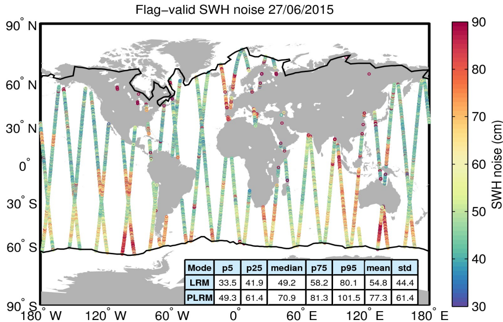
Figure 18. Geographical distribution of flag-valid 20-Hz SWH measurement noise over oceans and lakes for 27/06/2015. The statistical values shown in the table refer to the SWH noise and are calculated separately for LRM and PLRM regions. Measurements taken over polar polygons have been excluded from the computation of the statistical values. The black lines mark the outer limit of the Arctic and Antarctic polar polygons.
