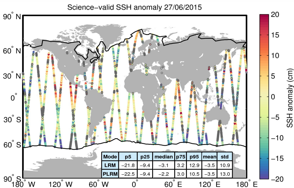
Figure 10. Geographical distribution of science-valid SSH anomaly data over oceans and lakes for 27/06/2015. The statistical values shown in the table refer to the SSH anomaly in cm and are calculated separately for LRM and PLRM regions. The black lines mark the outer limit of the Arctic and Antarctic polar polygons. Gray circles denote records that have been rejected based on the editing criteria described in Table 2.
