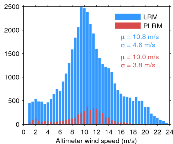
Figure 35. Histogram of science-valid wind over oceans and lakes for LRM (blue) and PLRM (red) for 27/06/2015. The mean ( \mu ) and standard deviation ( \sigma ) are also shown. Note that values larger than 24 m/s are excluded from the histogram for the sake of readability but not from the computation of \mu and \sigma .
