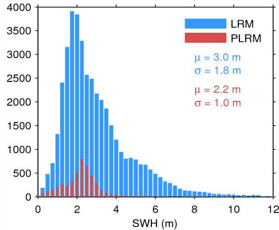
Figure 17. Histogram of flag-valid SWH over oceans and lakes for LRM (blue) and PLRM (red) for 27/06/2015. The mean ( \mu ) and standard deviation ( \sigma ) are also shown. Note that values larger than 12 m are excluded from the histogram for the sake of readability but not from the computation of \mu and \sigma .
