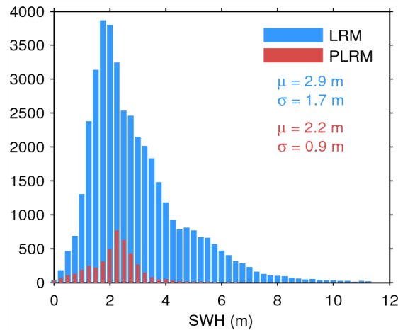
Figure 20. Histogram of science-valid SWH over oceans and lakes for LRM (blue) and PLRM (red) for 27/06/2015. The mean ( \mu ) and standard deviation ( \sigma ) are also shown. Note that values larger than 12 m are excluded from the histogram for the sake of readability but not from the computation of \mu and \sigma .
