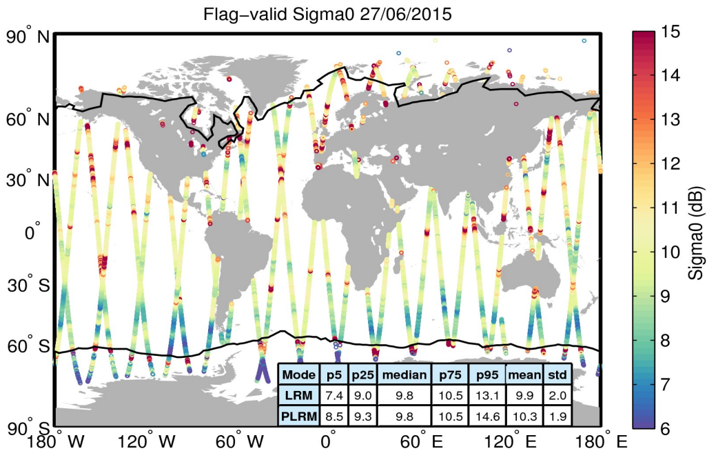
Figure 23. Geographical distribution of flag-valid sigma0 data over oceans and lakes for 27/06/2015. The statistical values shown in the table refer to the sigma0 in dB and are calculated separately for LRM and PLRM regions. Measurements taken over polar polygons have been excluded from the computation of the statistical values. The black lines mark the outer limit of the Arctic and Antarctic polar polygons.
