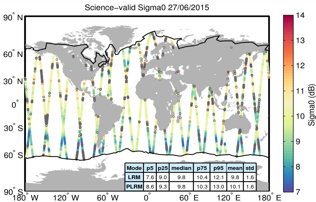
Figure 27. Geographical distribution of science-valid sigma0 data over oceans and lakes for 27/06/2015. The statistical values shown in the table refer to the sigma0 in dB and are calculated separately for LRM and PLRM regions. The black lines mark the outer limit of the Arctic and Antarctic polar polygons. Gray circles denote records that have been rejected based on the editing criteria described in Table 4.
