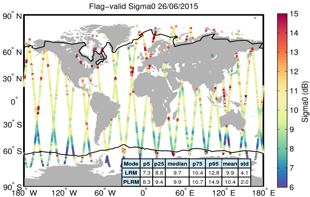
Figure 23. Geographical distribution of flag-valid sigma0 data over oceans and lakes for 26/06/2015. The statistical values shown in the table refer to the sigma0 in dB and are calculated separately for LRM and PLRM regions. Measurements taken over polar polygons have been excluded from the computation of the statistical values. The black lines mark the outer limit of the Arctic and Antarctic polar polygons.
