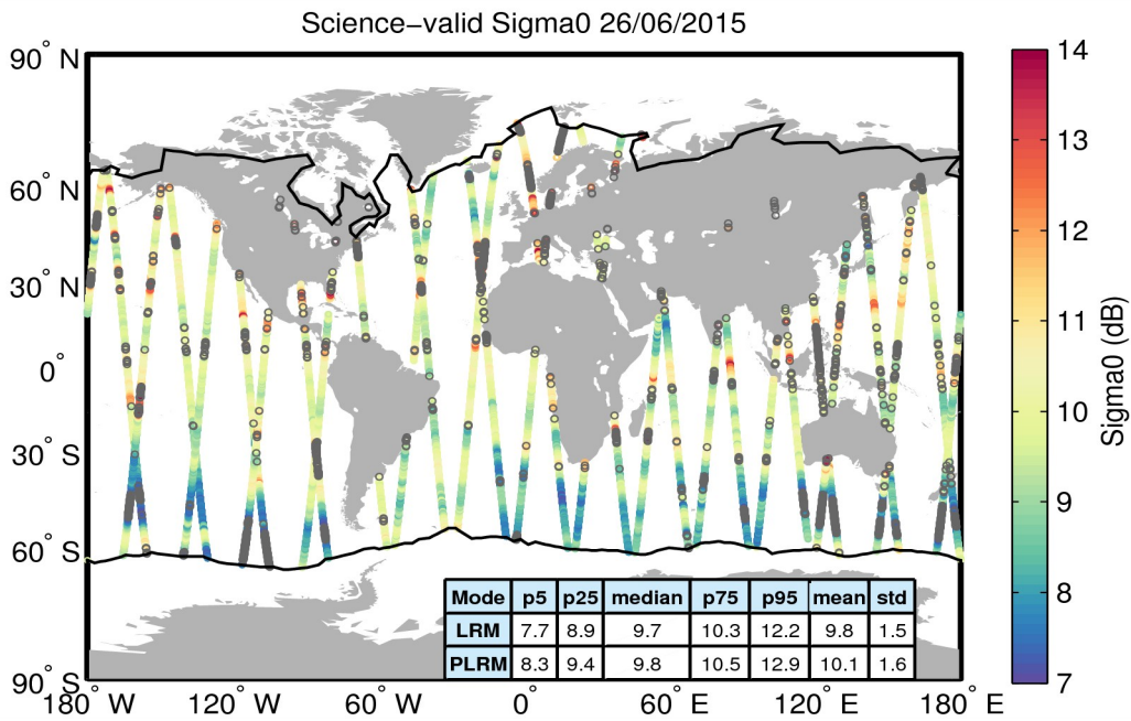
Figure 27. Geographical distribution of science-valid sigma0 data over oceans and lakes for 26/06/2015. The statistical values shown in the table refer to the sigma0 in dB and are calculated separately for LRM and PLRM regions. The black lines mark the outer limit of the Arctic and Antarctic polar polygons. Gray circles denote records that have been rejected based on the editing criteria described in Table 4.
