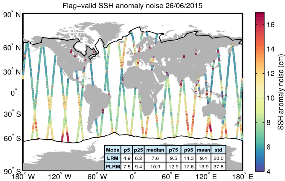
Figure 8. Geographical distribution of flag-valid 20-Hz SSH anomaly measurement noise over oceans and lakes for 26/06/2015. The statistical values shown in the table refer to the SSH anomaly noise and are calculated separately for LRM and PLRM regions. Measurements taken over polar polygons have been excluded from the computation of the statistical values. The black lines mark the outer limit of the Arctic and Antarctic polar polygons.
