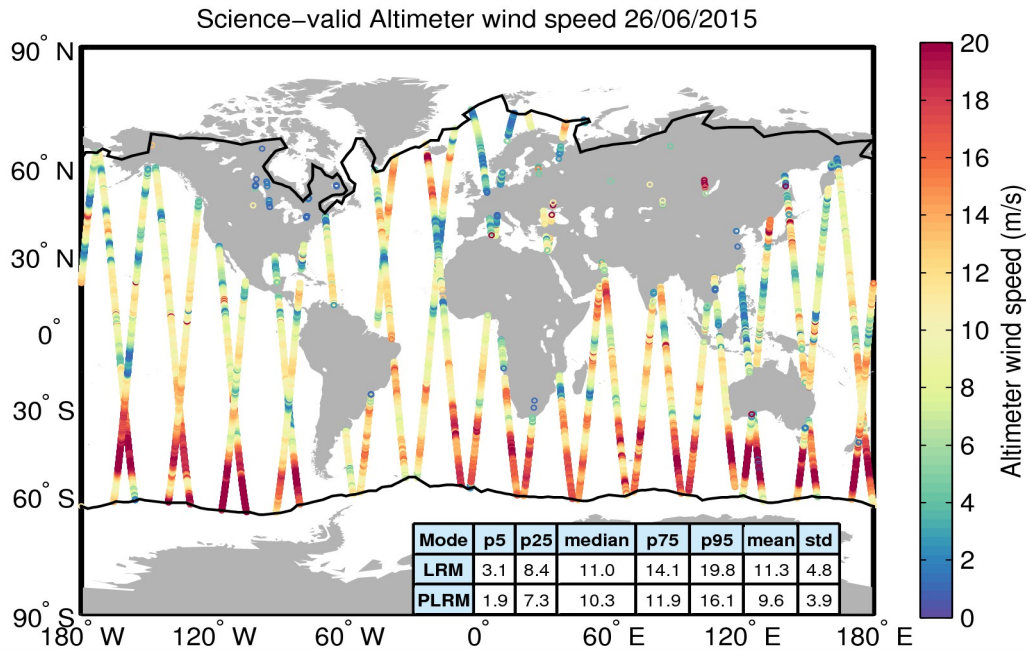
Figure 34. Geographical distribution of science-valid wind data over oceans and lakes for 26/06/2015. The statistical values shown in the table refer to the wind in m/s and are calculated separately for LRM and PLRM regions. The black lines mark the outer limit of the Arctic and Antarctic polar polygons. Gray circles denote records that have been rejected based on the editing criteria described in Table 5.
