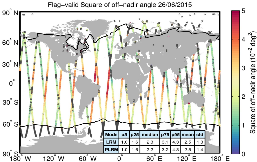
Figure 37. Geographical distribution of flag-valid mispointing data over oceans and lakes for 26/06/2015. The statistical values shown in the table refer to the mispointing in 10^{-2} deg 2 and are calculated separately for LRM and PLRM regions. Measurements taken over polar polygons have been excluded from the computation of the statistical values. The black lines mark the outer limit of the Arctic and Antarctic polar polygons. Gray circles denote negative values.
