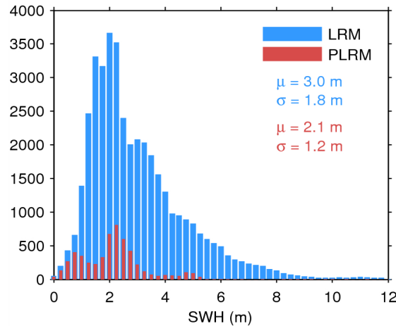
Figure 17. Histogram of flag-valid SWH over oceans and lakes for LRM (blue) and PLRM (red) for 26/06/2015. The mean ( \mu ) and standard deviation ( \sigma ) are also shown. Note that values larger than 12 m are excluded from the histogram for the sake of readability but not from the computation of \mu and \sigma .
