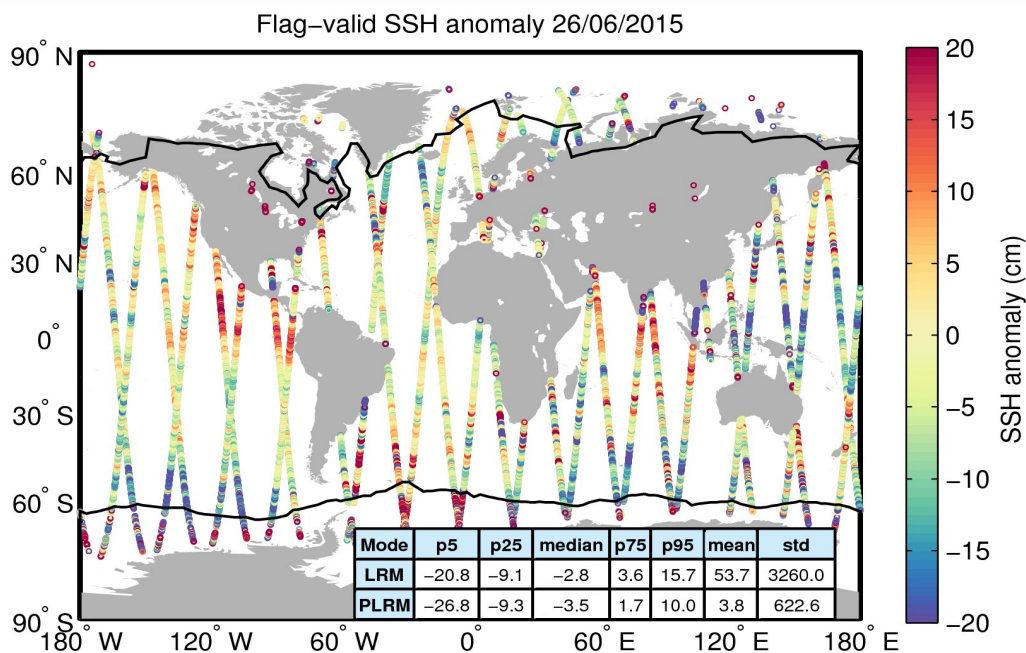
Figure 5. Geographical distribution of flag-valid 1-Hz SSH anomaly data over oceans and lakes for 26/06/2015. The statistical values shown in the table refer to the SSH anomaly in cm and are calculated separately for LRM and PLRM regions. Measurements taken over polar polygons have been excluded from the computation of the statistical values. The black lines mark the outer limit of the Arctic and Antarctic polar polygons.
