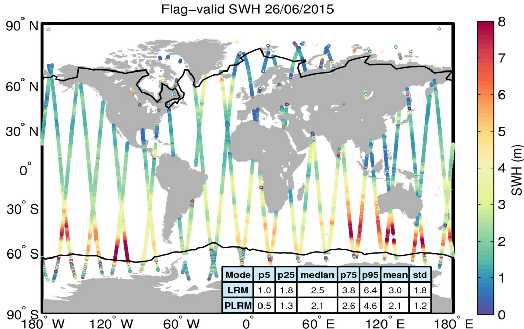
Figure 15. Geographical distribution of flag-valid SWH data over oceans and lakes for 26/06/2015. The statistical values shown in the table refer to the SWH in m and are calculated separately for LRM and PLRM regions. Measurements taken over polar polygons have been excluded from the computation of the statistical values. The black lines mark the outer limit of the Arctic and Antarctic polar polygons.
