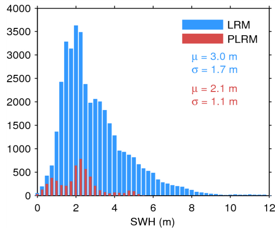
Figure 20. Histogram of science-valid SWH over oceans and lakes for LRM (blue) and PLRM (red) for 26/06/2015. The mean ( \mu ) and standard deviation ( \sigma ) are also shown. Note that values larger than 12 m are excluded from the histogram for the sake of readability but not from the computation of \mu and \sigma .
