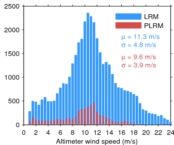
Figure 35. Histogram of science-valid wind over oceans and lakes for LRM (blue) and PLRM (red) for 26/06/2015. The mean ( \mu ) and standard deviation ( \sigma ) are also shown. Note that values larger than 24 m/s are excluded from the histogram for the sake of readability but not from the computation of \mu and \sigma .
