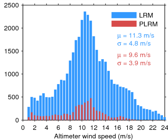
Figure 33. Histogram of flag-valid wind over oceans and lakes for LRM (blue) and PLRM (red) for 26/06/2015. The mean ( \mu ) and standard deviation ( \sigma ) are also shown. Note that values larger than 24 m/s are excluded from the histogram for the sake of readability but not from the computation of \mu and \sigma .
