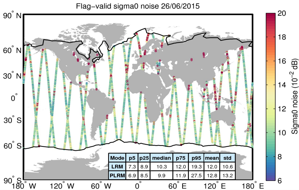
Figure 26. Geographical distribution of flag-valid 20-Hz sigma0 measurement noise over oceans and lakes for 26/06/2015. The statistical values shown in the table refer to the sigma0 noise and are calculated separately for LRM and PLRM regions. Measurements taken over polar polygons have been excluded from the computation of the statistical values. The black lines mark the outer limit of the Arctic and Antarctic polar polygons.
