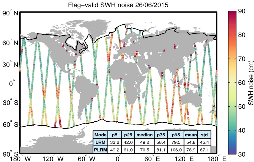
Figure 18. Geographical distribution of flag-valid 20-Hz SWH measurement noise over oceans and lakes for 26/06/2015. The statistical values shown in the table refer to the SWH noise and are calculated separately for LRM and PLRM regions. Measurements taken over polar polygons have been excluded from the computation of the statistical values. The black lines mark the outer limit of the Arctic and Antarctic polar polygons.
