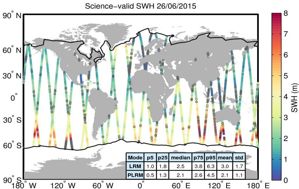
Figure 19. Geographical distribution of science-valid SWH data over oceans and lakes for 26/06/2015. The statistical values shown in the table refer to the SWH in m and are calculated separately for LRM and PLRM regions. The black lines mark the outer limit of the Arctic and Antarctic polar polygons. Gray circles denote records that have been rejected based on the editing criteria described in Table 3.
