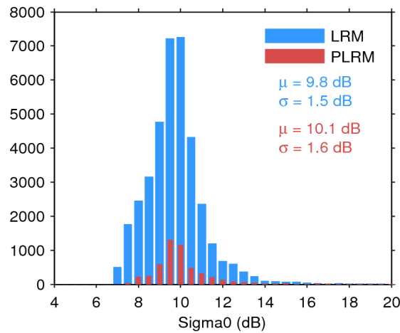
Figure 28. Histogram of science-valid sigma0 over oceans and lakes for LRM (blue) and PLRM (red) for 26/06/2015. The mean ( \mu ) and standard deviation ( \sigma ) are also shown. Note that values outside [4 20] dB are excluded from the histogram for the sake of readability but not from the computation of \mu and \sigma .
