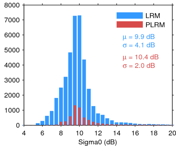
Figure 25. Histogram of flag-valid sigma0 over oceans and lakes for LRM (blue) and PLRM (red) for 26/06/2015. The mean ( \mu ) and standard deviation ( \sigma ) are also shown. Note that values outside [4 20] dB are excluded from the histogram for the sake of readability but not from the computation of \mu and \sigma .
