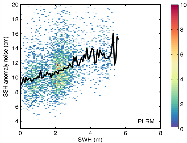
Figure 9. 2D histogram showing flag-valid SSH anomaly noise as a function of SWH for LRM (top) and PLRM (bottom) for 26/06/2015. The black line denotes the median SSH anomaly as a function of SWH.
