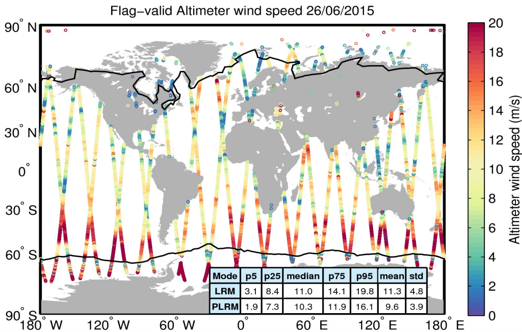
Figure 31. Geographical distribution of flag-valid wind data over oceans and lakes for 26/06/2015. The statistical values shown in the table refer to the wind in m/s and are calculated separately for LRM and PLRM regions. Measurements taken over polar polygons have been excluded from the computation of the statistical values. The black lines mark the outer limit of the Arctic and Antarctic polar polygons.
