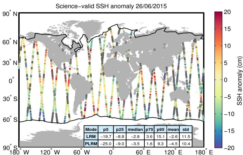
Figure 10. Geographical distribution of science-valid SSH anomaly data over oceans and lakes for 26/06/2015. The statistical values shown in the table refer to the SSH anomaly in cm and are calculated separately for LRM and PLRM regions. The black lines mark the outer limit of the Arctic and Antarctic polar polygons. Gray circles denote records that have been rejected based on the editing criteria described in Table 2.
