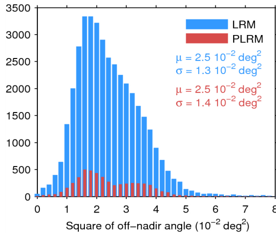
Figure 39. Histogram of flag-valid mispointing over oceans and lakes for LRM (blue) and PLRM (red) for 26/06/2015. Only positive values have been considered. The mean ( \mu ) and standard deviation ( \sigma ) are also shown. Note that values larger than 8 \cdot 10^{-2} \text{ deg}^2 are excluded from the histogram for the sake of readability but not from the computation of \mu and \sigma .
