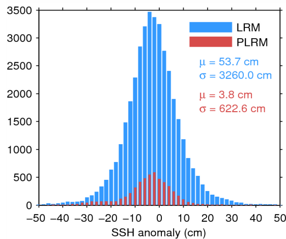
Figure 7. Histogram of flag-valid SSH anomaly over oceans and lakes for LRM (blue) and PLRM (red) for 26/06/2015. The mean ( \mu ) and standard deviation ( \sigma ) are also shown. Note that values outside [-50\ 50] cm are excluded from the histogram for the sake of readability but not from the computation of \mu and \sigma .
