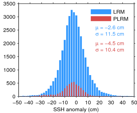
Figure 11. Histogram of science-valid SSH anomaly over oceans and lakes for LRM (blue) and PLRM (red) for 26/06/2015. The mean ( \mu ) and standard deviation ( \sigma ) are also shown. Note that values outside [-50 50] cm are excluded from the histogram for the sake of readability but not from the computation of \mu and \sigma .
