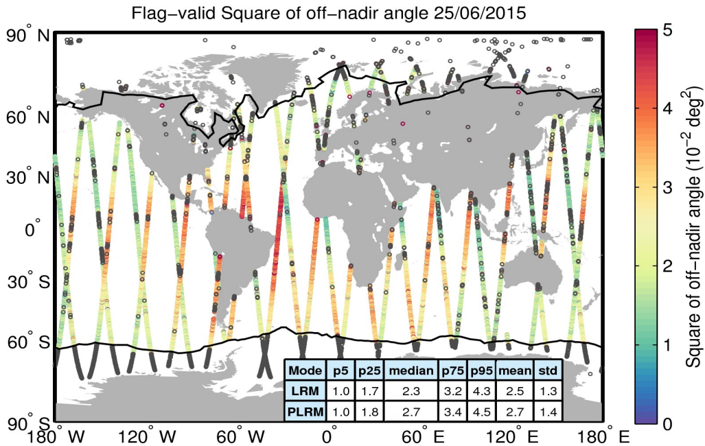
Figure 37. Geographical distribution of flag-valid mispointing data over oceans and lakes for 25/06/2015. The statistical values shown in the table refer to the mispointing in 10^{-2} \text{ deg}^2 and are calculated separately for LRM and PLRM regions. Measurements taken over polar polygons have been excluded from the computation of the statistical values. The black lines mark the outer limit of the Arctic and Antarctic polar polygons. Gray circles denote negative values.
