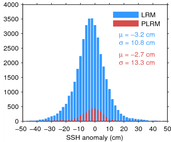
Figure 11. Histogram of science-valid SSH anomaly over oceans and lakes for LRM (blue) and PLRM (red) for 25/06/2015. The mean ( \mu ) and standard deviation ( \sigma ) are also shown. Note that values outside [-50 50] cm are excluded from the histogram for the sake of readability but not from the computation of \mu and \sigma .
