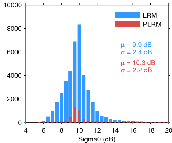
Figure 25. Histogram of flag-valid sigma0 over oceans and lakes for LRM (blue) and PLRM (red) for 25/06/2015. The mean ( \mu ) and standard deviation ( \sigma ) are also shown. Note that values outside [4 20] dB are excluded from the histogram for the sake of readability but not from the computation of \mu and \sigma .
