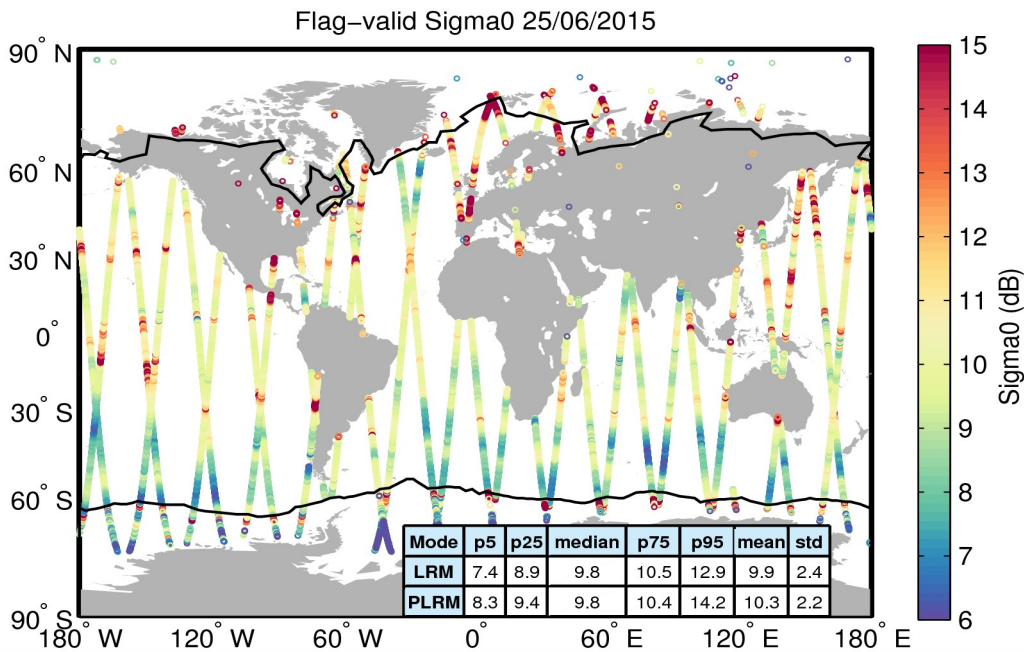
Figure 23. Geographical distribution of flag-valid sigma0 data over oceans and lakes for 25/06/2015. The statistical values shown in the table refer to the sigma0 in dB and are calculated separately for LRM and PLRM regions. Measurements taken over polar polygons have been excluded from the computation of the statistical values. The black lines mark the outer limit of the Arctic and Antarctic polar polygons.
