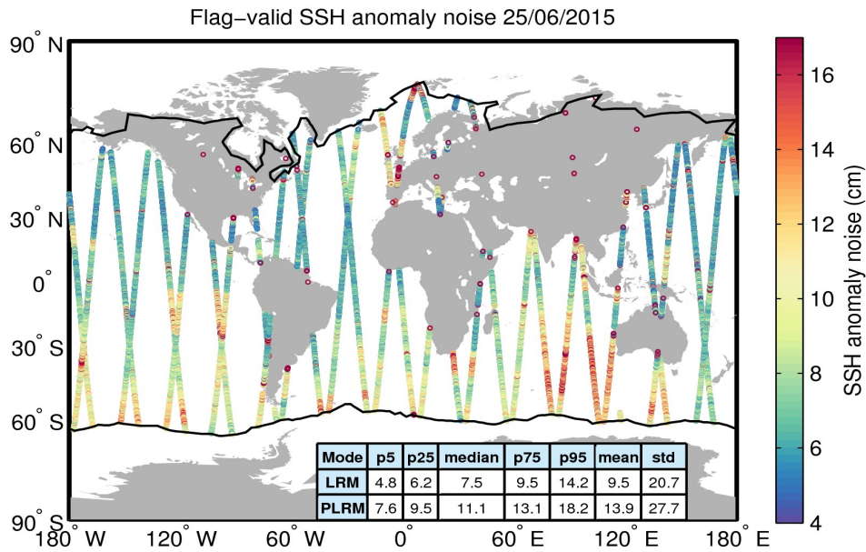
Figure 8. Geographical distribution of flag-valid 20-Hz SSH anomaly measurement noise over oceans and lakes for 25/06/2015. The statistical values shown in the table refer to the SSH anomaly noise and are calculated separately for LRM and PLRM regions. Measurements taken over polar polygons have been excluded from the computation of the statistical values. The black lines mark the outer limit of the Arctic and Antarctic polar polygons.
