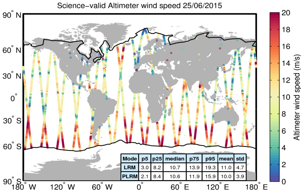
Figure 34. Geographical distribution of science-valid wind data over oceans and lakes for 25/06/2015. The statistical values shown in the table refer to the wind in m/s and are calculated separately for LRM and PLRM regions. The black lines mark the outer limit of the Arctic and Antarctic polar polygons. Gray circles denote records that have been rejected based on the editing criteria described in Table 5.
