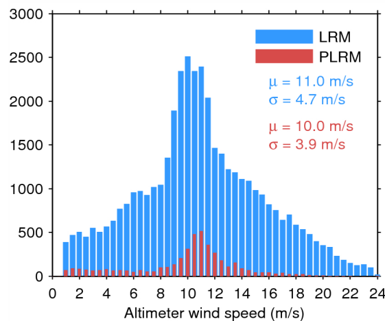
Figure 35. Histogram of science-valid wind over oceans and lakes for LRM (blue) and PLRM (red) for 25/06/2015. The mean ( \mu ) and standard deviation ( \sigma ) are also shown. Note that values larger than 24 m/s are excluded from the histogram for the sake of readability but not from the computation of \mu and \sigma .
