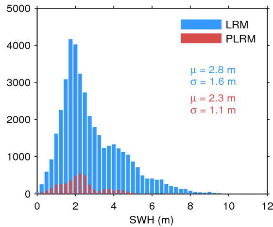
Figure 20. Histogram of science-valid SWH over oceans and lakes for LRM (blue) and PLRM (red) for 25/06/2015. The mean ( \mu ) and standard deviation ( \sigma ) are also shown. Note that values larger than 12 m are excluded from the histogram for the sake of readability but not from the computation of \mu and \sigma .
