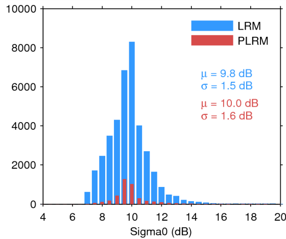
Figure 28. Histogram of science-valid sigma0 over oceans and lakes for LRM (blue) and PLRM (red) for 25/06/2015. The mean ( \mu ) and standard deviation ( \sigma ) are also shown. Note that values outside [4 20] dB are excluded from the histogram for the sake of readability but not from the computation of \mu and \sigma .
