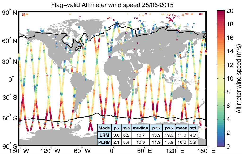
Figure 31. Geographical distribution of flag-valid wind data over oceans and lakes for 25/06/2015. The statistical values shown in the table refer to the wind in m/s and are calculated separately for LRM and PLRM regions. Measurements taken over polar polygons have been excluded from the computation of the statistical values. The black lines mark the outer limit of the Arctic and Antarctic polar polygons.
