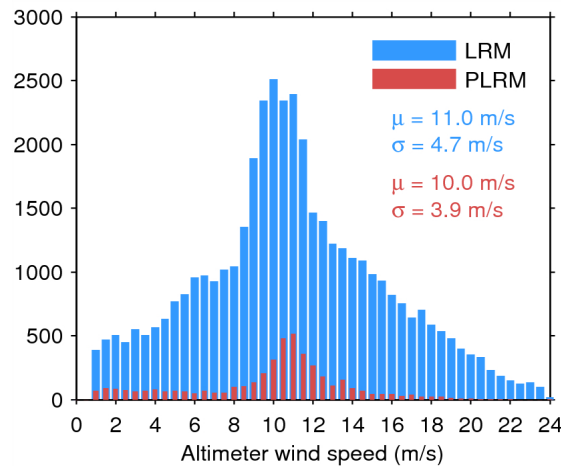
Figure 33. Histogram of flag-valid wind over oceans and lakes for LRM (blue) and PLRM (red) for 25/06/2015. The mean ( \mu ) and standard deviation ( \sigma ) are also shown. Note that values larger than 24 m/s are excluded from the histogram for the sake of readability but not from the computation of \mu and \sigma .
