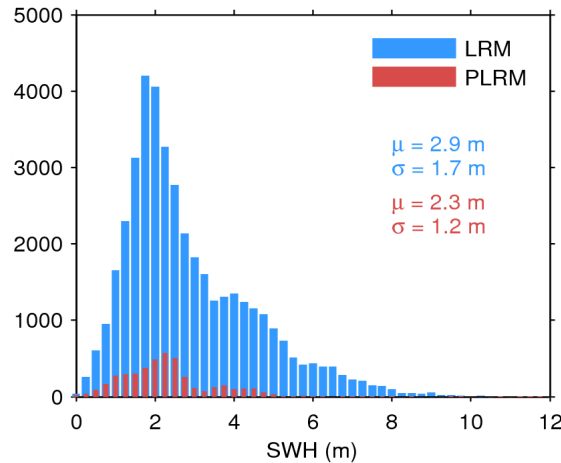
Figure 17. Histogram of flag-valid SWH over oceans and lakes for LRM (blue) and PLRM (red) for 25/06/2015. The mean ( \mu ) and standard deviation ( \sigma ) are also shown. Note that values larger than 12 m are excluded from the histogram for the sake of readability but not from the computation of \mu and \sigma .
