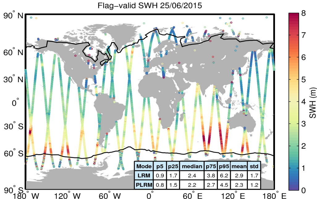
Figure 15. Geographical distribution of flag-valid SWH data over oceans and lakes for 25/06/2015. The statistical values shown in the table refer to the SWH in m and are calculated separately for LRM and PLRM regions. Measurements taken over polar polygons have been excluded from the computation of the statistical values. The black lines mark the outer limit of the Arctic and Antarctic polar polygons.
