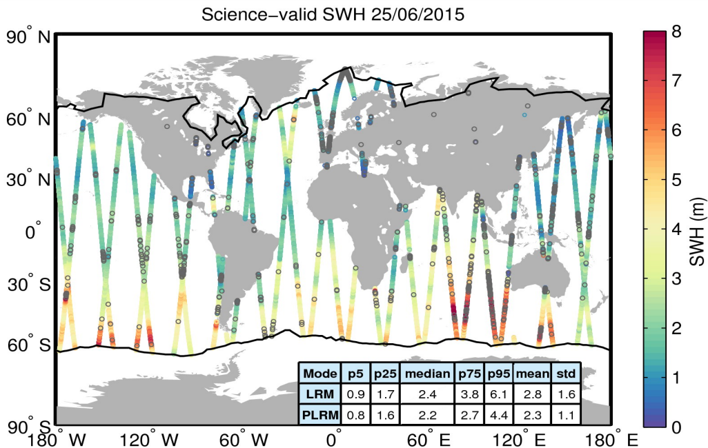
Figure 19. Geographical distribution of science-valid SWH data over oceans and lakes for 25/06/2015. The statistical values shown in the table refer to the SWH in m and are calculated separately for LRM and PLRM regions. The black lines mark the outer limit of the Arctic and Antarctic polar polygons. Gray circles denote records that have been rejected based on the editing criteria described in Table 3.
