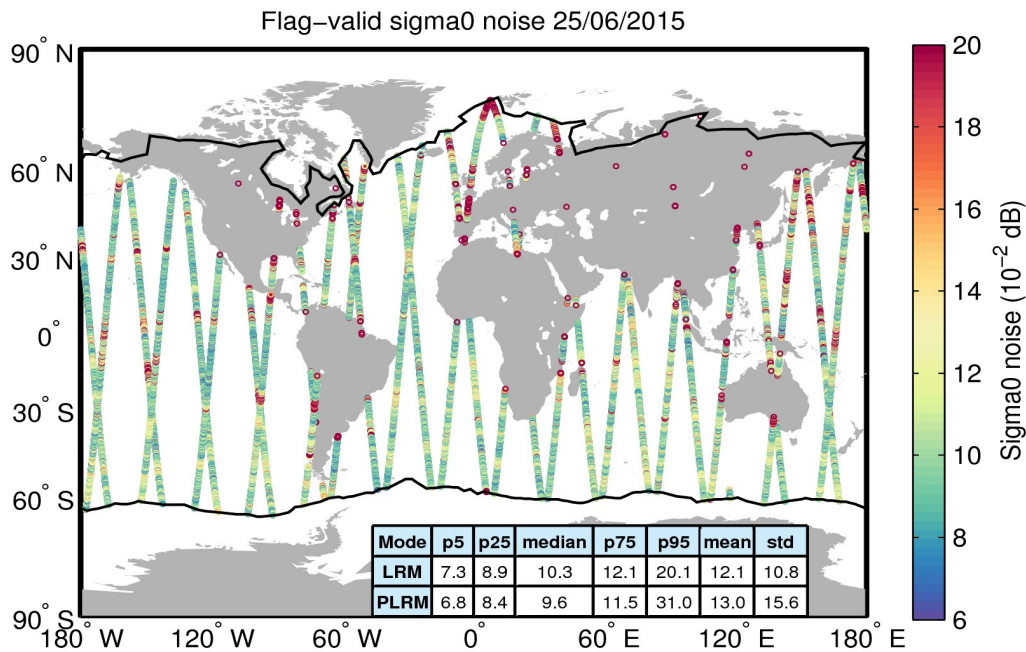
Figure 26. Geographical distribution of flag-valid 20-Hz sigma0 measurement noise over oceans and lakes for 25/06/2015. The statistical values shown in the table refer to the sigma0 noise and are calculated separately for LRM and PLRM regions. Measurements taken over polar polygons have been excluded from the computation of the statistical values. The black lines mark the outer limit of the Arctic and Antarctic polar polygons.
