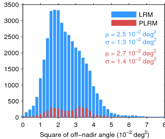
Figure 39. Histogram of flag-valid mispointing over oceans and lakes for LRM (blue) and PLRM (red) for 25/06/2015. Only positive values have been considered. The mean ( \mu ) and standard deviation ( \sigma ) are also shown. Note that values larger than 8 \cdot 10^{-2} \text{ deg}^2 are excluded from the histogram for the sake of readability but not from the computation of \mu and \sigma .
