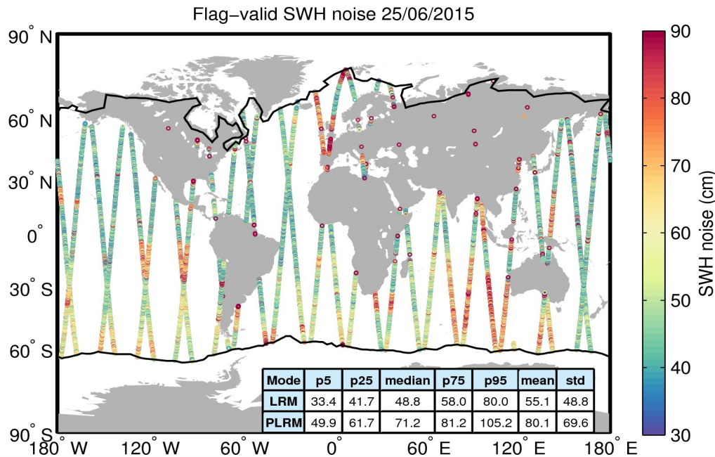
Figure 18. Geographical distribution of flag-valid 20-Hz SWH measurement noise over oceans and lakes for 25/06/2015. The statistical values shown in the table refer to the SWH noise and are calculated separately for LRM and PLRM regions. Measurements taken over polar polygons have been excluded from the computation of the statistical values. The black lines mark the outer limit of the Arctic and Antarctic polar polygons.
