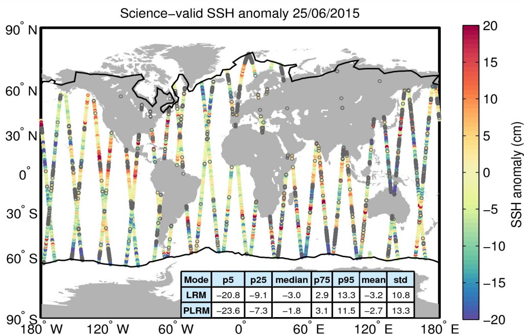
Figure 10. Geographical distribution of science-valid SSH anomaly data over oceans and lakes for 25/06/2015. The statistical values shown in the table refer to the SSH anomaly in cm and are calculated separately for LRM and PLRM regions. The black lines mark the outer limit of the Arctic and Antarctic polar polygons. Gray circles denote records that have been rejected based on the editing criteria described in Table 2.
