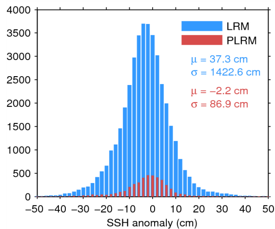
Figure 7. Histogram of flag-valid SSH anomaly over oceans and lakes for LRM (blue) and PLRM (red) for 25/06/2015. The mean ( \mu ) and standard deviation ( \sigma ) are also shown. Note that values outside [-50\ 50] cm are excluded from the histogram for the sake of readability but not from the computation of \mu and \sigma .
