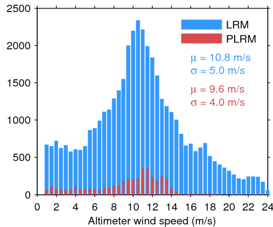
Figure 33. Histogram of flag-valid wind over oceans and lakes for LRM (blue) and PLRM (red) for 23/06/2015. The mean ( \mu ) and standard deviation ( \sigma ) are also shown. Note that values larger than 24 m/s are excluded from the histogram for the sake of readability but not from the computation of \mu and \sigma .
