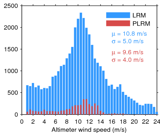
Figure 35. Histogram of science-valid wind over oceans and lakes for LRM (blue) and PLRM (red) for 23/06/2015. The mean ( \mu ) and standard deviation ( \sigma ) are also shown. Note that values larger than 24 m/s are excluded from the histogram for the sake of readability but not from the computation of \mu and \sigma .
