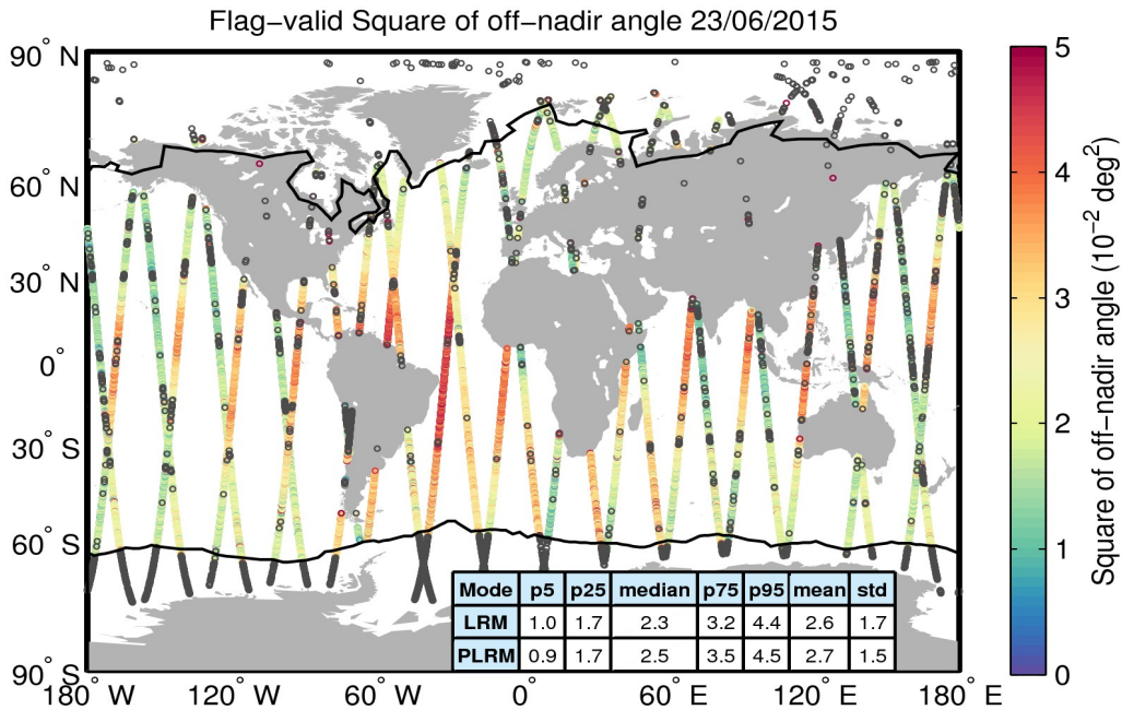
Figure 37. Geographical distribution of flag-valid mispointing data over oceans and lakes for 23/06/2015. The statistical values shown in the table refer to the mispointing in 10^{-2} \text{ deg}^2 and are calculated separately for LRM and PLRM regions. Measurements taken over polar polygons have been excluded from the computation of the statistical values. The black lines mark the outer limit of the Arctic and Antarctic polar polygons. Gray circles denote negative values.
