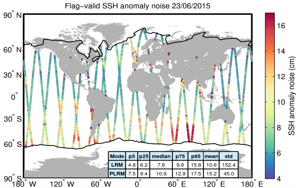
Figure 8. Geographical distribution of flag-valid 20-Hz SSH anomaly measurement noise over oceans and lakes for 23/06/2015. The statistical values shown in the table refer to the SSH anomaly noise and are calculated separately for LRM and PLRM regions. Measurements taken over polar polygons have been excluded from the computation of the statistical values. The black lines mark the outer limit of the Arctic and Antarctic polar polygons.
