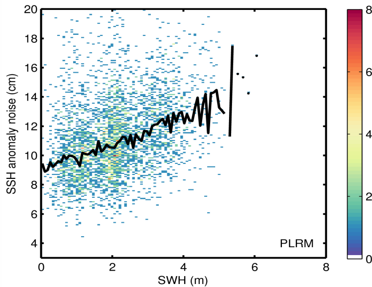
Figure 9. 2D histogram showing flag-valid SSH anomaly noise as a function of SWH for LRM (top) and PLRM (bottom) for 23/06/2015. The black line denotes the median SSH anomaly as a function of SWH.
