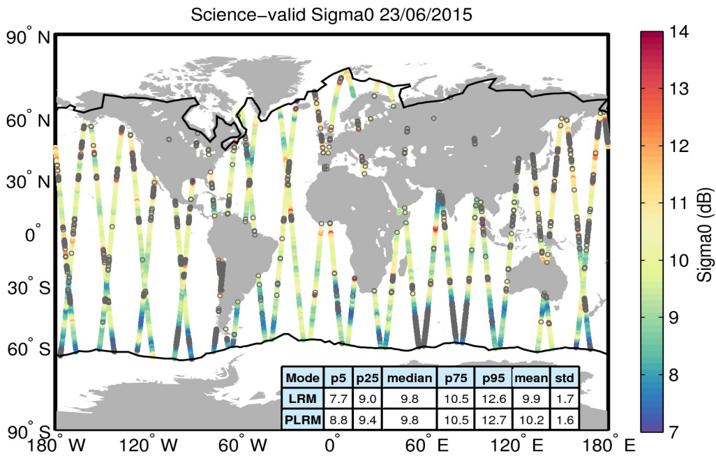
Figure 27. Geographical distribution of science-valid sigma0 data over oceans and lakes for 23/06/2015. The statistical values shown in the table refer to the sigma0 in dB and are calculated separately for LRM and PLRM regions. The black lines mark the outer limit of the Arctic and Antarctic polar polygons. Gray circles denote records that have been rejected based on the editing criteria described in Table 4.
