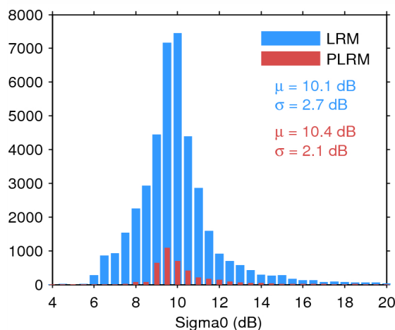
Figure 25. Histogram of flag-valid sigma0 over oceans and lakes for LRM (blue) and PLRM (red) for 23/06/2015. The mean ( \mu ) and standard deviation ( \sigma ) are also shown. Note that values outside [4 20] dB are excluded from the histogram for the sake of readability but not from the computation of \mu and \sigma .
