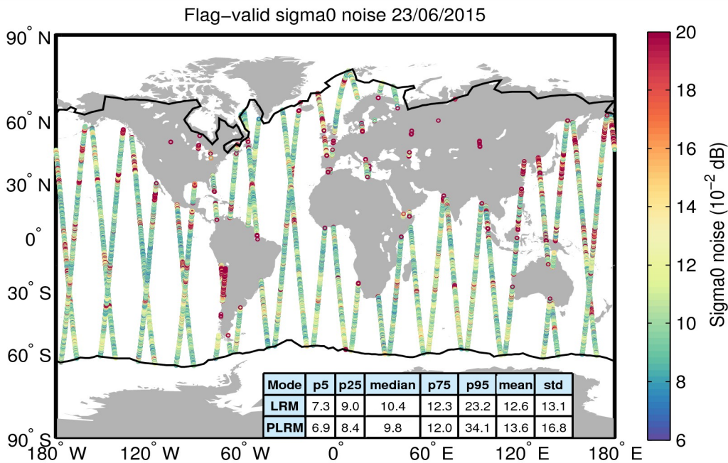
Figure 26. Geographical distribution of flag-valid 20-Hz sigma0 measurement noise over oceans and lakes for 23/06/2015. The statistical values shown in the table refer to the sigma0 noise and are calculated separately for LRM and PLRM regions. Measurements taken over polar polygons have been excluded from the computation of the statistical values. The black lines mark the outer limit of the Arctic and Antarctic polar polygons.
