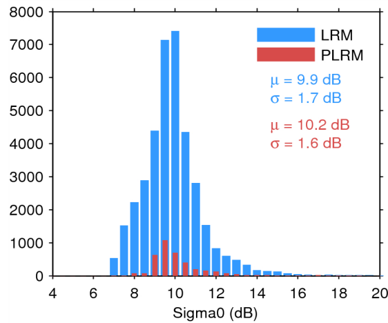
Figure 28. Histogram of science-valid sigma0 over oceans and lakes for LRM (blue) and PLRM (red) for 23/06/2015. The mean ( \mu ) and standard deviation ( \sigma ) are also shown. Note that values outside [4 20] dB are excluded from the histogram for the sake of readability but not from the computation of \mu and \sigma .
