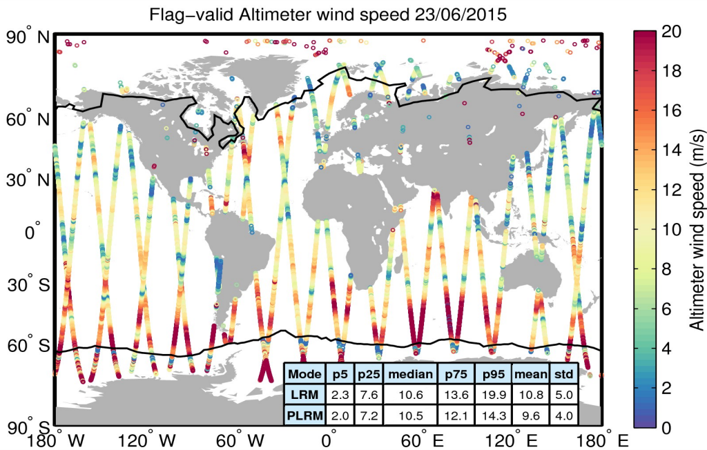
Figure 31. Geographical distribution of flag-valid wind data over oceans and lakes for 23/06/2015. The statistical values shown in the table refer to the wind in m/s and are calculated separately for LRM and PLRM regions. Measurements taken over polar polygons have been excluded from the computation of the statistical values. The black lines mark the outer limit of the Arctic and Antarctic polar polygons.
