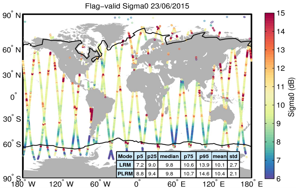
Figure 23. Geographical distribution of flag-valid sigma0 data over oceans and lakes for 23/06/2015. The statistical values shown in the table refer to the sigma0 in dB and are calculated separately for LRM and PLRM regions. Measurements taken over polar polygons have been excluded from the computation of the statistical values. The black lines mark the outer limit of the Arctic and Antarctic polar polygons.
