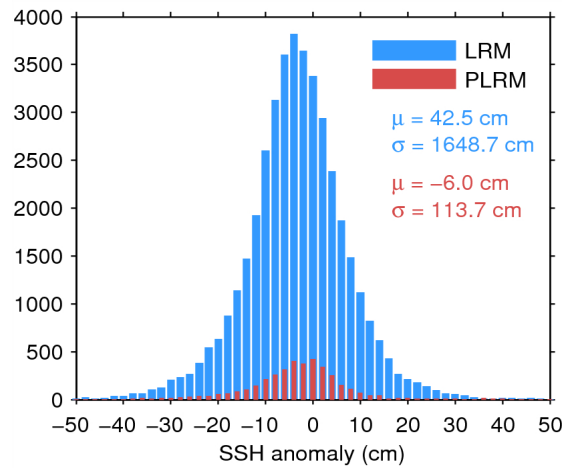
Figure 7. Histogram of flag-valid SSH anomaly over oceans and lakes for LRM (blue) and PLRM (red) for 23/06/2015. The mean ( \mu ) and standard deviation ( \sigma ) are also shown. Note that values outside [-50\ 50] cm are excluded from the histogram for the sake of readability but not from the computation of \mu and \sigma .
