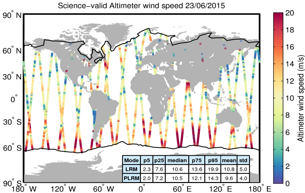
Figure 34. Geographical distribution of science-valid wind data over oceans and lakes for 23/06/2015. The statistical values shown in the table refer to the wind in m/s and are calculated separately for LRM and PLRM regions. The black lines mark the outer limit of the Arctic and Antarctic polar polygons. Gray circles denote records that have been rejected based on the editing criteria described in Table 5.
