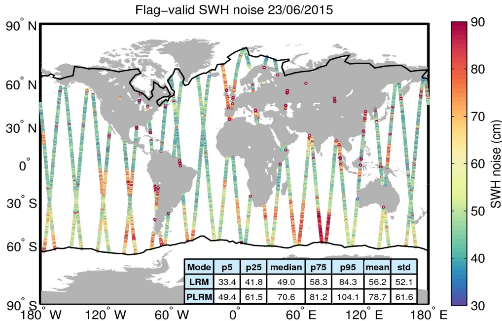
Figure 18. Geographical distribution of flag-valid 20-Hz SWH measurement noise over oceans and lakes for 23/06/2015. The statistical values shown in the table refer to the SWH noise and are calculated separately for LRM and PLRM regions. Measurements taken over polar polygons have been excluded from the computation of the statistical values. The black lines mark the outer limit of the Arctic and Antarctic polar polygons.
