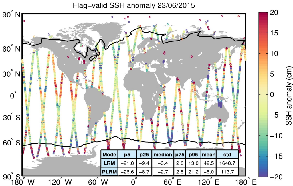
Figure 5. Geographical distribution of flag-valid 1-Hz SSH anomaly data over oceans and lakes for 23/06/2015. The statistical values shown in the table refer to the SSH anomaly in cm and are calculated separately for LRM and PLRM regions. Measurements taken over polar polygons have been excluded from the computation of the statistical values. The black lines mark the outer limit of the Arctic and Antarctic polar polygons.
