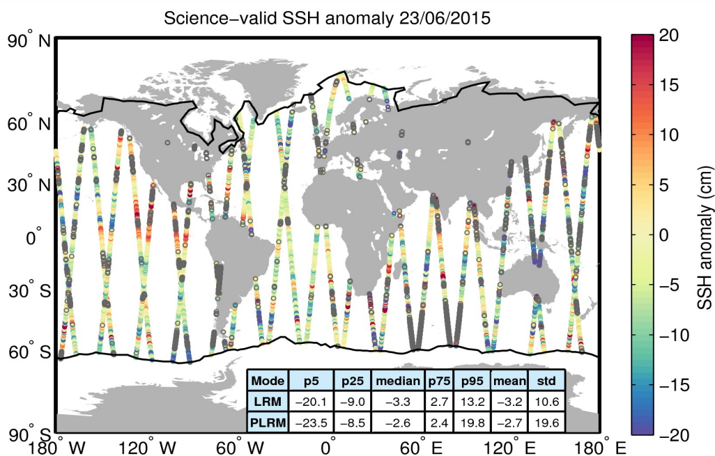
Figure 10. Geographical distribution of science-valid SSH anomaly data over oceans and lakes for 23/06/2015. The statistical values shown in the table refer to the SSH anomaly in cm and are calculated separately for LRM and PLRM regions. The black lines mark the outer limit of the Arctic and Antarctic polar polygons. Gray circles denote records that have been rejected based on the editing criteria described in Table 2.
