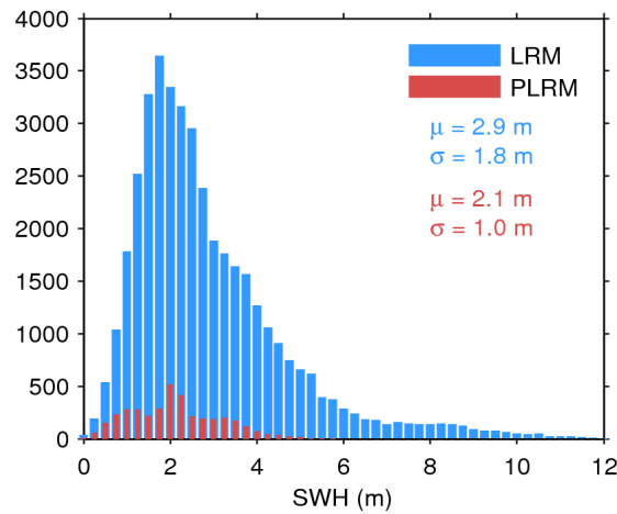
Figure 20. Histogram of science-valid SWH over oceans and lakes for LRM (blue) and PLRM (red) for 23/06/2015. The mean ( \mu ) and standard deviation ( \sigma ) are also shown. Note that values larger than 12 m are excluded from the histogram for the sake of readability but not from the computation of \mu and \sigma .
