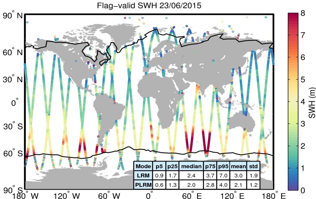
Figure 15. Geographical distribution of flag-valid SWH data over oceans and lakes for 23/06/2015. The statistical values shown in the table refer to the SWH in m and are calculated separately for LRM and PLRM regions. Measurements taken over polar polygons have been excluded from the computation of the statistical values. The black lines mark the outer limit of the Arctic and Antarctic polar polygons.
