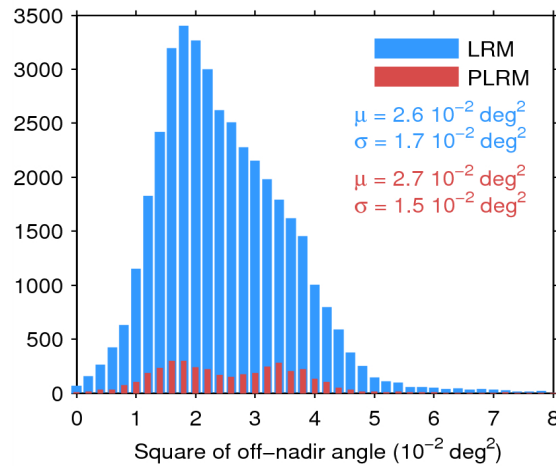
Figure 39. Histogram of flag-valid mispointing over oceans and lakes for LRM (blue) and PLRM (red) for 23/06/2015. Only positive values have been considered. The mean ( \mu ) and standard deviation ( \sigma ) are also shown. Note that values larger than 8 \cdot 10^{-2} \text{ deg}^2 are excluded from the histogram for the sake of readability but not from the computation of \mu and \sigma .
