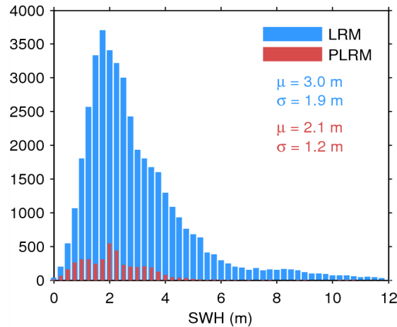
Figure 17. Histogram of flag-valid SWH over oceans and lakes for LRM (blue) and PLRM (red) for 23/06/2015. The mean ( \mu ) and standard deviation ( \sigma ) are also shown. Note that values larger than 12 m are excluded from the histogram for the sake of readability but not from the computation of \mu and \sigma .
