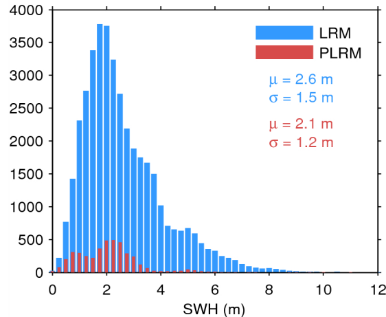
Figure 17. Histogram of flag-valid SWH over oceans and lakes for LRM (blue) and PLRM (red) for 19/06/2015. The mean ( \mu ) and standard deviation ( \sigma ) are also shown. Note that values larger than 12 m are excluded from the histogram for the sake of readability but not from the computation of \mu and \sigma .
