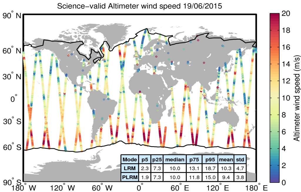
Figure 34. Geographical distribution of science-valid wind data over oceans and lakes for 19/06/2015. The statistical values shown in the table refer to the wind in m/s and are calculated separately for LRM and PLRM regions. The black lines mark the outer limit of the Arctic and Antarctic polar polygons. Gray circles denote records that have been rejected based on the editing criteria described in Table 5.
