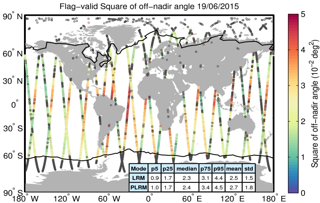
Figure 37. Geographical distribution of flag-valid mispointing data over oceans and lakes for 19/06/2015. The statistical values shown in the table refer to the mispointing in 10^{-2} deg 2 and are calculated separately for LRM and PLRM regions. Measurements taken over polar polygons have been excluded from the computation of the statistical values. The black lines mark the outer limit of the Arctic and Antarctic polar polygons. Gray circles denote negative values.
