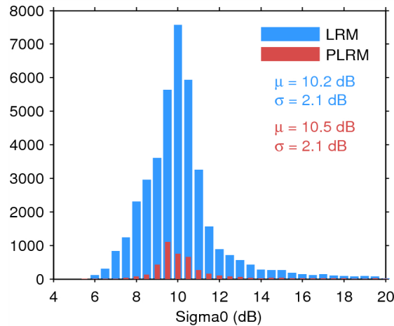
Figure 25. Histogram of flag-valid sigma0 over oceans and lakes for LRM (blue) and PLRM (red) for 19/06/2015. The mean ( \mu ) and standard deviation ( \sigma ) are also shown. Note that values outside [4 20] dB are excluded from the histogram for the sake of readability but not from the computation of \mu and \sigma .
