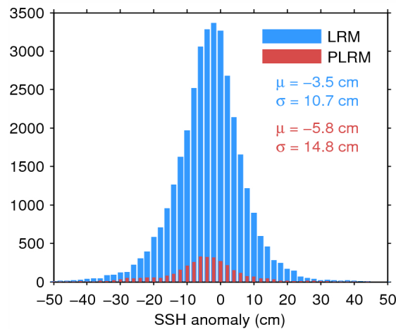
Figure 11. Histogram of science-valid SSH anomaly over oceans and lakes for LRM (blue) and PLRM (red) for 19/06/2015. The mean ( \mu ) and standard deviation ( \sigma ) are also shown. Note that values outside [-50\ 50] cm are excluded from the histogram for the sake of readability but not from the computation of \mu and \sigma .
