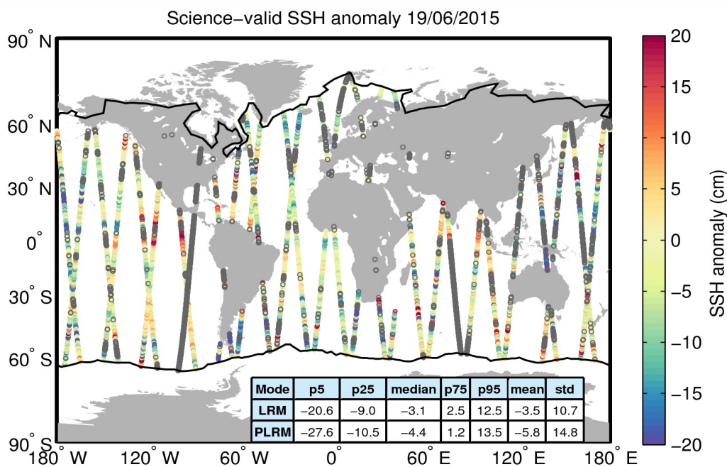
Figure 10. Geographical distribution of science-valid SSH anomaly data over oceans and lakes for 19/06/2015. The statistical values shown in the table refer to the SSH anomaly in cm and are calculated separately for LRM and PLRM regions. The black lines mark the outer limit of the Arctic and Antarctic polar polygons. Gray circles denote records that have been rejected based on the editing criteria described in Table 2.
