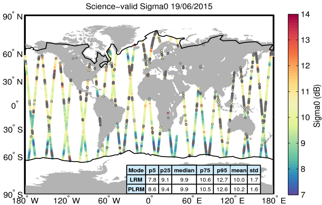
Figure 27. Geographical distribution of science-valid sigma0 data over oceans and lakes for 19/06/2015. The statistical values shown in the table refer to the sigma0 in dB and are calculated separately for LRM and PLRM regions. The black lines mark the outer limit of the Arctic and Antarctic polar polygons. Gray circles denote records that have been rejected based on the editing criteria described in Table 4.
