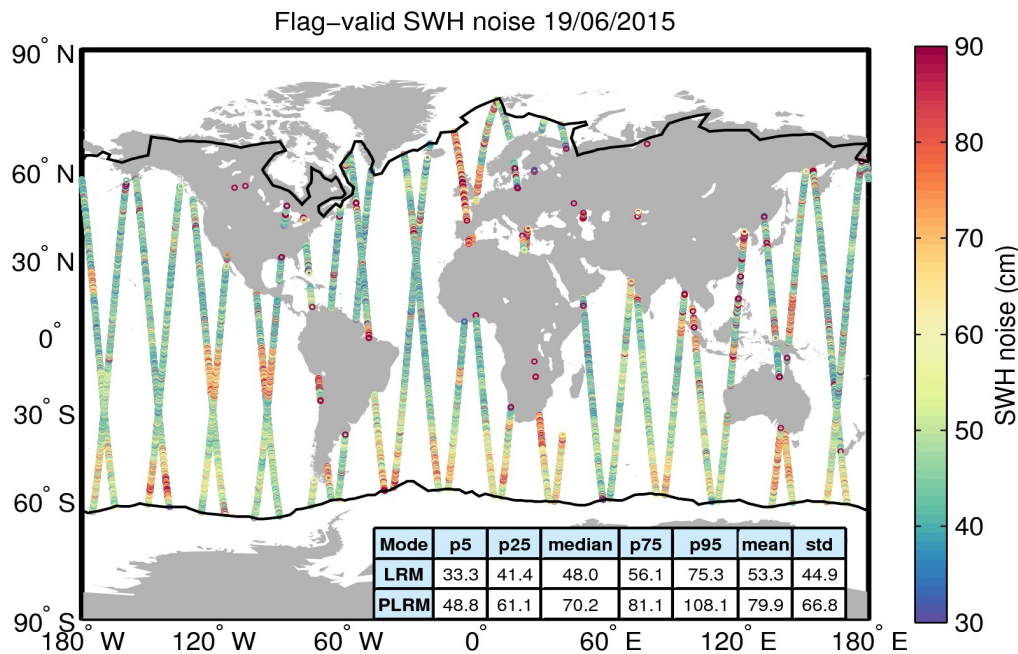
Figure 18. Geographical distribution of flag-valid 20-Hz SWH measurement noise over oceans and lakes for 19/06/2015. The statistical values shown in the table refer to the SWH noise and are calculated separately for LRM and PLRM regions. Measurements taken over polar polygons have been excluded from the computation of the statistical values. The black lines mark the outer limit of the Arctic and Antarctic polar polygons.
