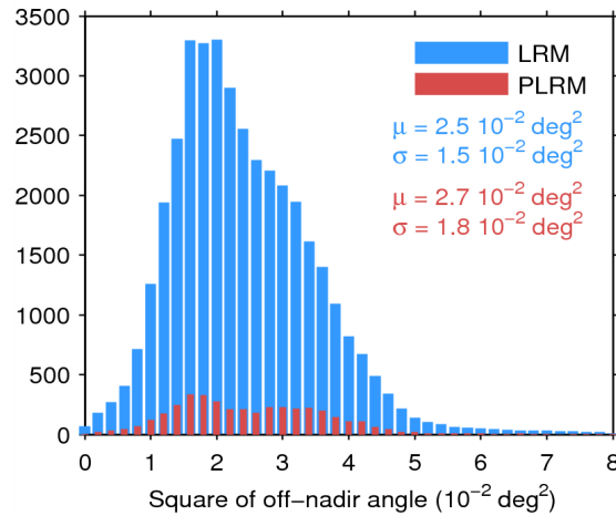
Figure 39. Histogram of flag-valid mispointing over oceans and lakes for LRM (blue) and PLRM (red) for 19/06/2015. Only positive values have been considered. The mean ( \mu ) and standard deviation ( \sigma ) are also shown. Note that values larger than 8 \cdot 10^{-2} \text{ deg}^2 are excluded from the histogram for the sake of readability but not from the computation of \mu and \sigma .
