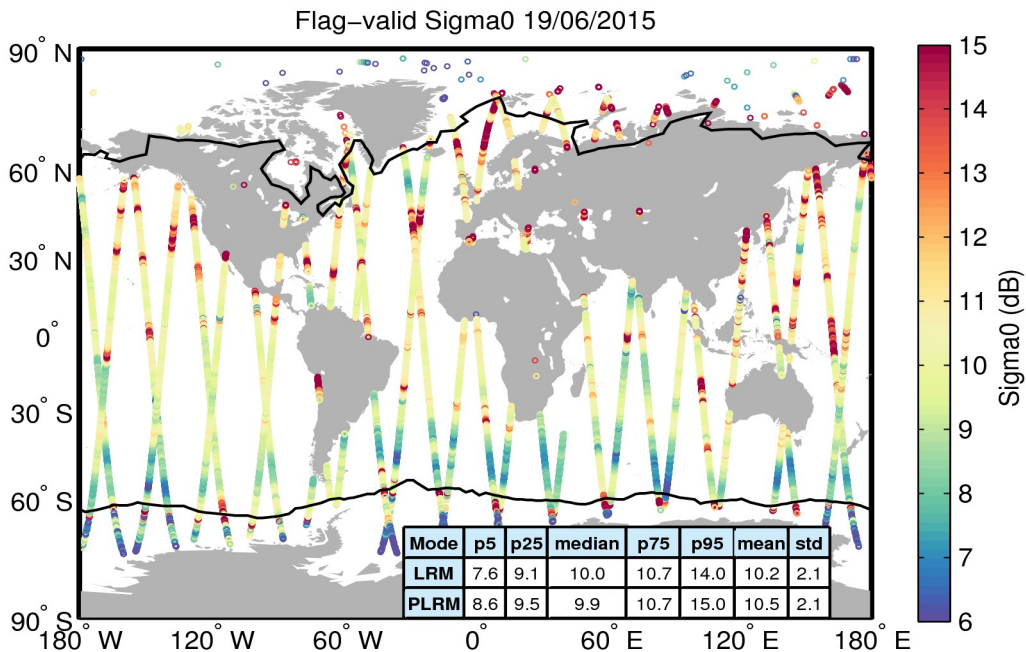
Figure 23. Geographical distribution of flag-valid sigma0 data over oceans and lakes for 19/06/2015. The statistical values shown in the table refer to the sigma0 in dB and are calculated separately for LRM and PLRM regions. Measurements taken over polar polygons have been excluded from the computation of the statistical values. The black lines mark the outer limit of the Arctic and Antarctic polar polygons.
