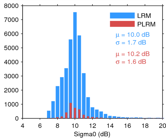
Figure 28. Histogram of science-valid sigma0 over oceans and lakes for LRM (blue) and PLRM (red) for 19/06/2015. The mean ( \mu ) and standard deviation ( \sigma ) are also shown. Note that values outside [4 20] dB are excluded from the histogram for the sake of readability but not from the computation of \mu and \sigma .
