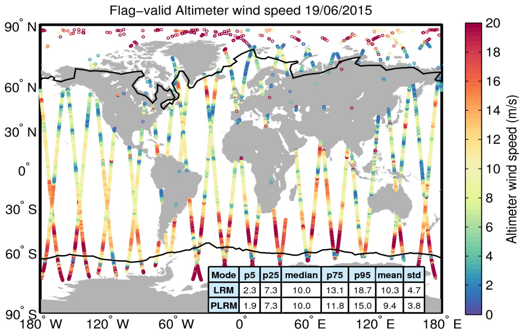
Figure 31. Geographical distribution of flag-valid wind data over oceans and lakes for 19/06/2015. The statistical values shown in the table refer to the wind in m/s and are calculated separately for LRM and PLRM regions. Measurements taken over polar polygons have been excluded from the computation of the statistical values. The black lines mark the outer limit of the Arctic and Antarctic polar polygons.
