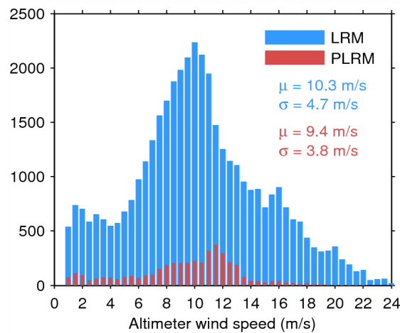
Figure 33. Histogram of flag-valid wind over oceans and lakes for LRM (blue) and PLRM (red) for 19/06/2015. The mean ( \mu ) and standard deviation ( \sigma ) are also shown. Note that values larger than 24 m/s are excluded from the histogram for the sake of readability but not from the computation of \mu and \sigma .
