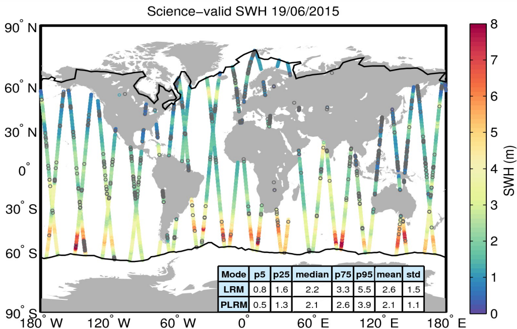
Figure 19. Geographical distribution of science-valid SWH data over oceans and lakes for 19/06/2015. The statistical values shown in the table refer to the SWH in m and are calculated separately for LRM and PLRM regions. The black lines mark the outer limit of the Arctic and Antarctic polar polygons. Gray circles denote records that have been rejected based on the editing criteria described in Table 3.
