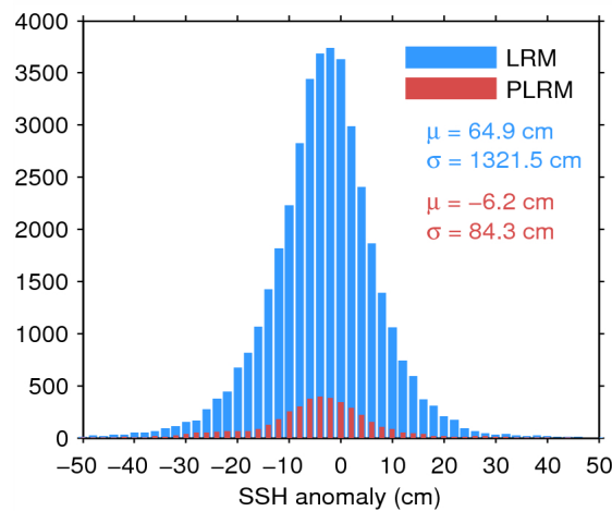
Figure 7. Histogram of flag-valid SSH anomaly over oceans and lakes for LRM (blue) and PLRM (red) for 19/06/2015. The mean ( \mu ) and standard deviation ( \sigma ) are also shown. Note that values outside [-50 50] cm are excluded from the histogram for the sake of readability but not from the computation of \mu and \sigma .
