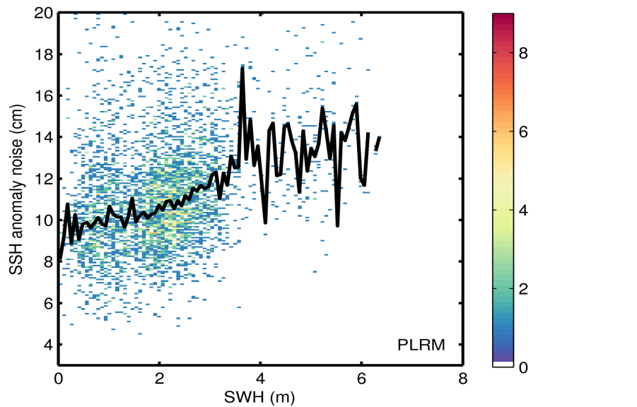
Figure 9. 2D histogram showing flag-valid SSH anomaly noise as a function of SWH for LRM (top) and PLRM (bottom) for 19/06/2015. The black line denotes the median SSH anomaly as a function of SWH.
