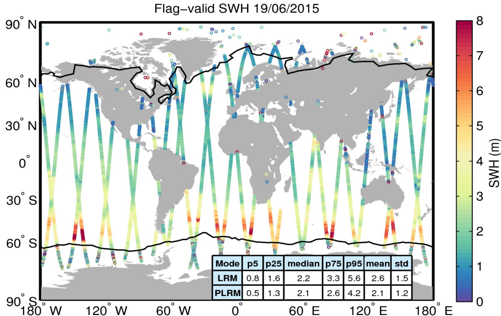
Figure 15. Geographical distribution of flag-valid SWH data over oceans and lakes for 19/06/2015. The statistical values shown in the table refer to the SWH in m and are calculated separately for LRM and PLRM regions. Measurements taken over polar polygons have been excluded from the computation of the statistical values. The black lines mark the outer limit of the Arctic and Antarctic polar polygons.
