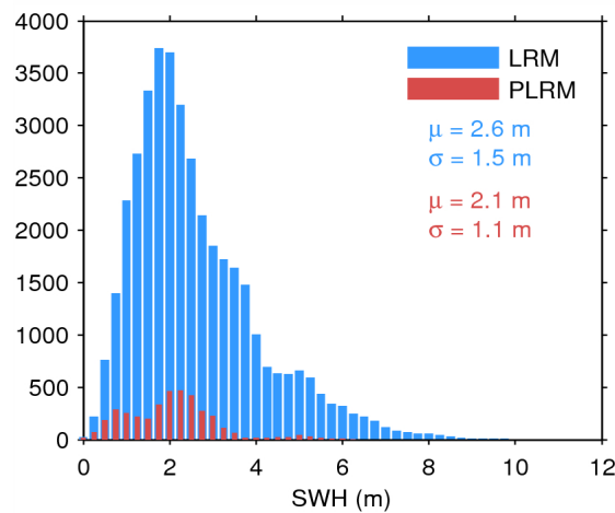
Figure 20. Histogram of science-valid SWH over oceans and lakes for LRM (blue) and PLRM (red) for 19/06/2015. The mean ( \mu ) and standard deviation ( \sigma ) are also shown. Note that values larger than 12 m are excluded from the histogram for the sake of readability but not from the computation of \mu and \sigma .
