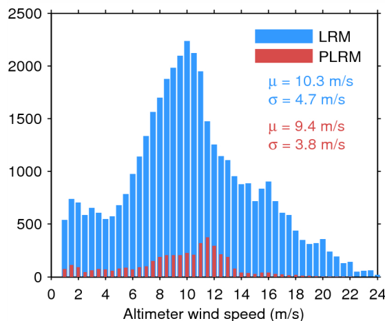
Figure 35. Histogram of science-valid wind over oceans and lakes for LRM (blue) and PLRM (red) for 19/06/2015. The mean ( \mu ) and standard deviation ( \sigma ) are also shown. Note that values larger than 24 m/s are excluded from the histogram for the sake of readability but not from the computation of \mu and \sigma .
