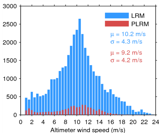
Figure 35. Histogram of science-valid wind over oceans and lakes for LRM (blue) and PLRM (red) for 15/06/2015. The mean ( \mu ) and standard deviation ( \sigma ) are also shown. Note that values larger than 24 m/s are excluded from the histogram for the sake of readability but not from the computation of \mu and \sigma .
