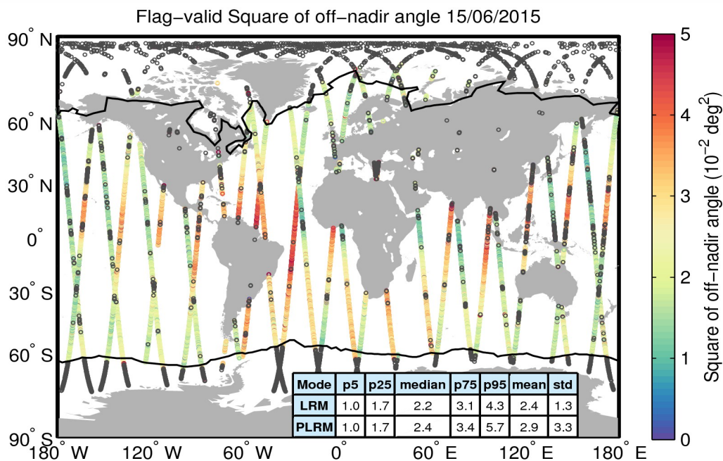
Figure 37. Geographical distribution of flag-valid mispointing data over oceans and lakes for 15/06/2015. The statistical values shown in the table refer to the mispointing in 10^{-2} \text{ deg}^2 and are calculated separately for LRM and PLRM regions. Measurements taken over polar polygons have been excluded from the computation of the statistical values. The black lines mark the outer limit of the Arctic and Antarctic polar polygons. Gray circles denote negative values.
