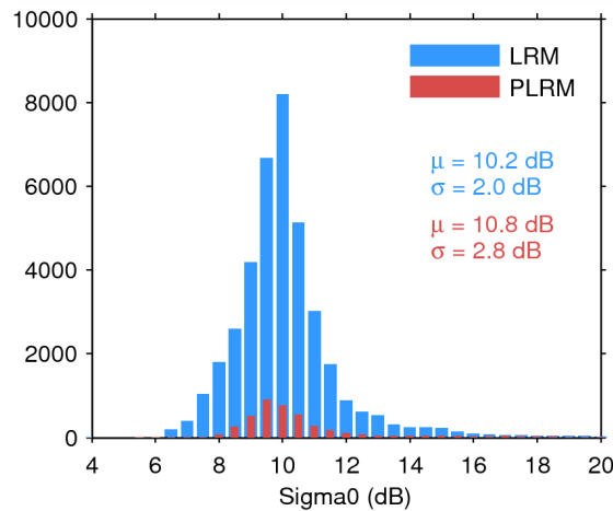
Figure 25. Histogram of flag-valid sigma0 over oceans and lakes for LRM (blue) and PLRM (red) for 15/06/2015. The mean ( \mu ) and standard deviation ( \sigma ) are also shown. Note that values outside [4 20] dB are excluded from the histogram for the sake of readability but not from the computation of \mu and \sigma .
