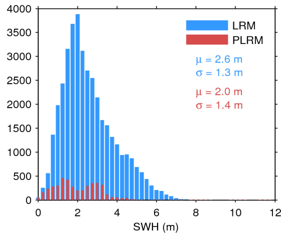
Figure 17. Histogram of flag-valid SWH over oceans and lakes for LRM (blue) and PLRM (red) for 15/06/2015. The mean ( \mu ) and standard deviation ( \sigma ) are also shown. Note that values larger than 12 m are excluded from the histogram for the sake of readability but not from the computation of \mu and \sigma .
