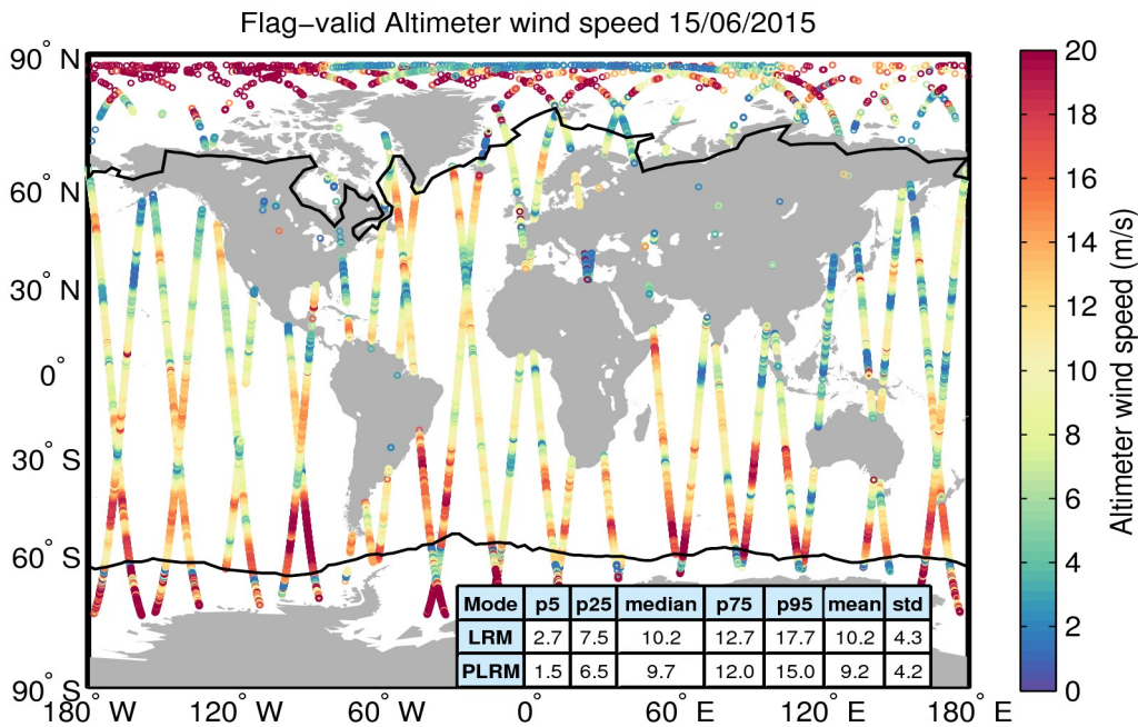
Figure 31. Geographical distribution of flag-valid wind data over oceans and lakes for 15/06/2015. The statistical values shown in the table refer to the wind in m/s and are calculated separately for LRM and PLRM regions. Measurements taken over polar polygons have been excluded from the computation of the statistical values. The black lines mark the outer limit of the Arctic and Antarctic polar polygons.
