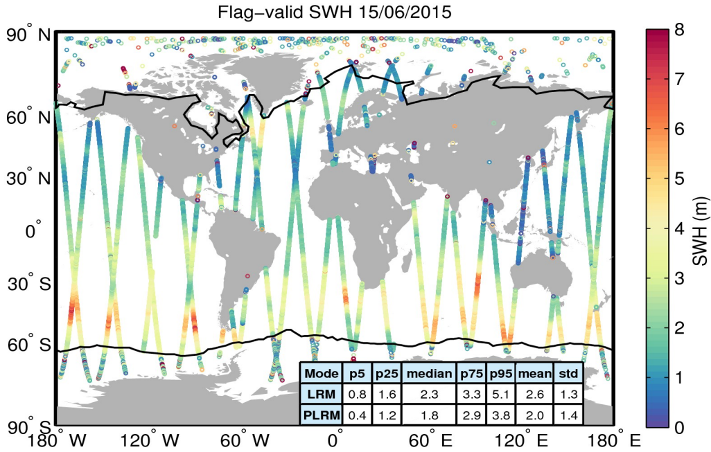
Figure 15. Geographical distribution of flag-valid SWH data over oceans and lakes for 15/06/2015. The statistical values shown in the table refer to the SWH in m and are calculated separately for LRM and PLRM regions. Measurements taken over polar polygons have been excluded from the computation of the statistical values. The black lines mark the outer limit of the Arctic and Antarctic polar polygons.
