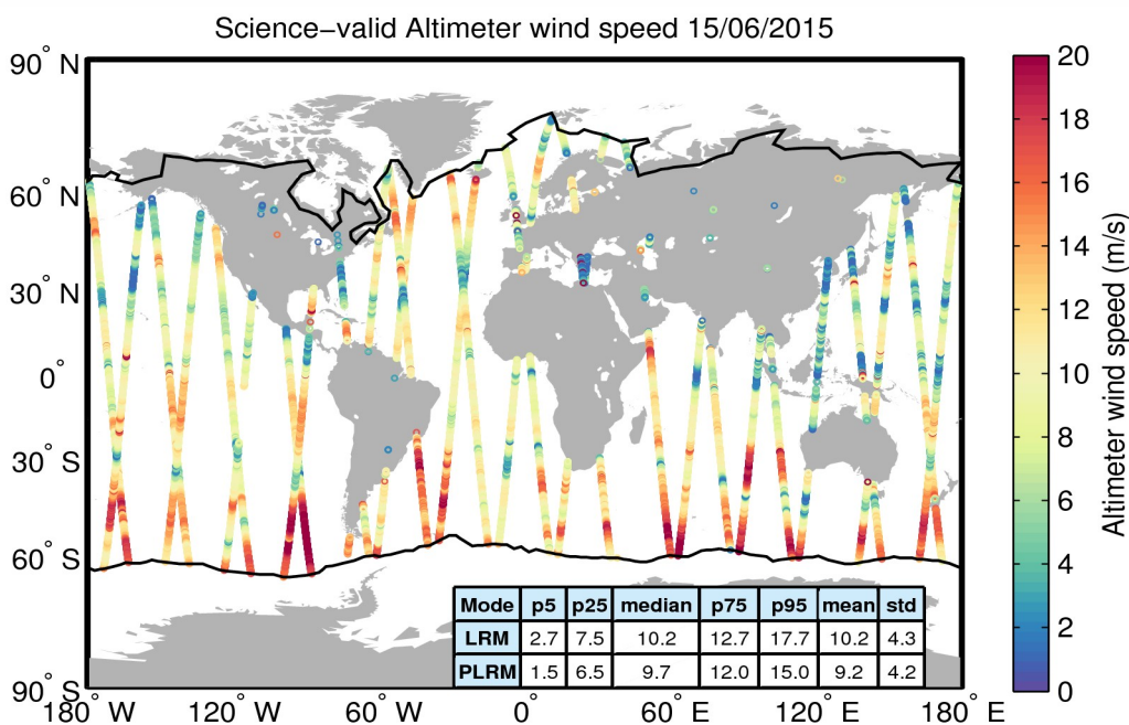
Figure 34. Geographical distribution of science-valid wind data over oceans and lakes for 15/06/2015. The statistical values shown in the table refer to the wind in m/s and are calculated separately for LRM and PLRM regions. The black lines mark the outer limit of the Arctic and Antarctic polar polygons. Gray circles denote records that have been rejected based on the editing criteria described in Table 5.
