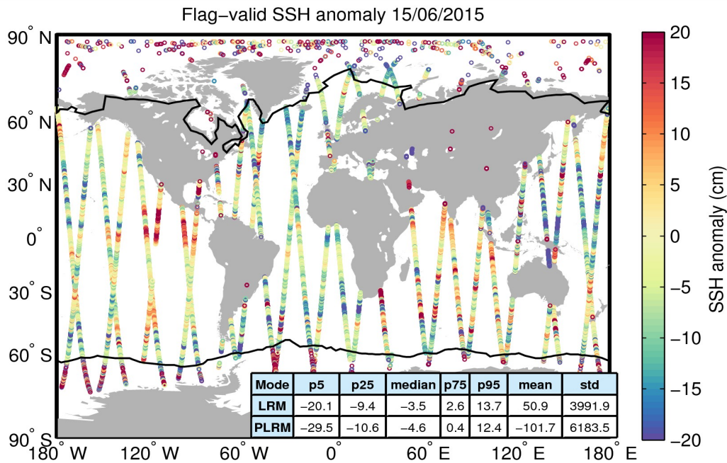
Figure 5. Geographical distribution of flag-valid 1-Hz SSH anomaly data over oceans and lakes for 15/06/2015. The statistical values shown in the table refer to the SSH anomaly in cm and are calculated separately for LRM and PLRM regions. Measurements taken over polar polygons have been excluded from the computation of the statistical values. The black lines mark the outer limit of the Arctic and Antarctic polar polygons.
