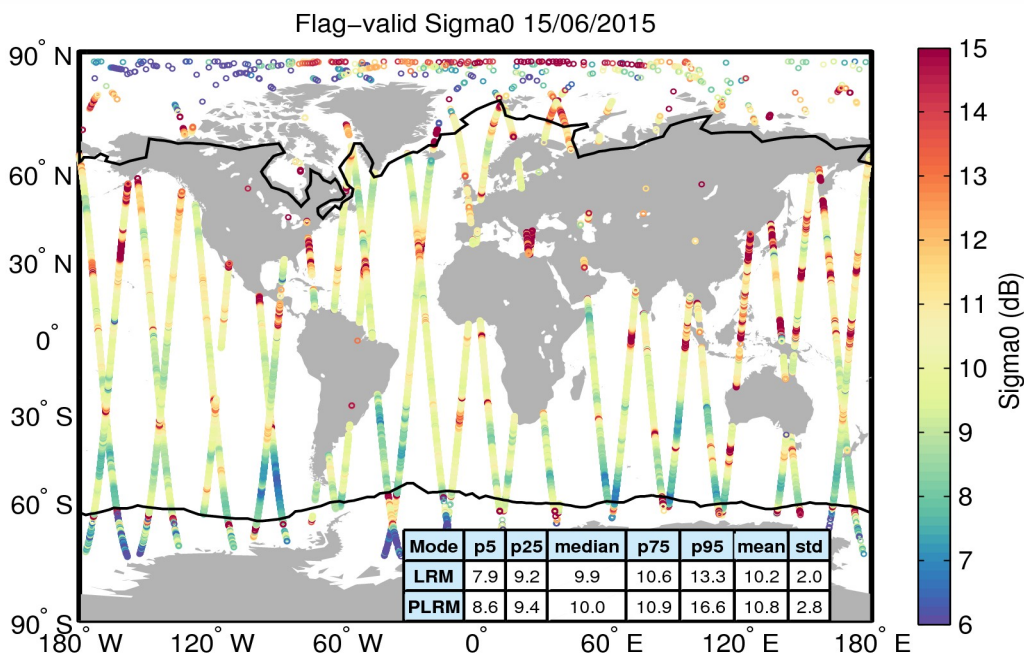
Figure 23. Geographical distribution of flag-valid sigma0 data over oceans and lakes for 15/06/2015. The statistical values shown in the table refer to the sigma0 in dB and are calculated separately for LRM and PLRM regions. Measurements taken over polar polygons have been excluded from the computation of the statistical values. The black lines mark the outer limit of the Arctic and Antarctic polar polygons.
