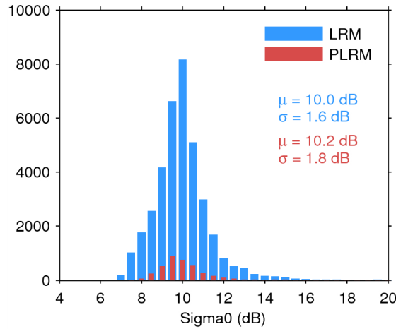
Figure 28. Histogram of science-valid sigma0 over oceans and lakes for LRM (blue) and PLRM (red) for 15/06/2015. The mean ( \mu ) and standard deviation ( \sigma ) are also shown. Note that values outside [4 20] dB are excluded from the histogram for the sake of readability but not from the computation of \mu and \sigma .
