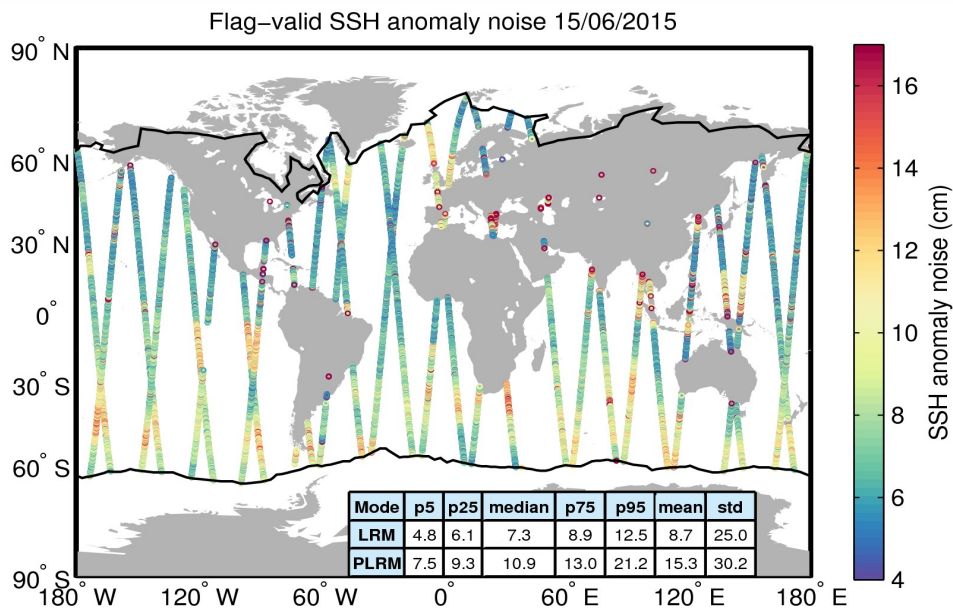
Figure 8. Geographical distribution of flag-valid 20-Hz SSH anomaly measurement noise over oceans and lakes for 15/06/2015. The statistical values shown in the table refer to the SSH anomaly noise and are calculated separately for LRM and PLRM regions. Measurements taken over polar polygons have been excluded from the computation of the statistical values. The black lines mark the outer limit of the Arctic and Antarctic polar polygons.
