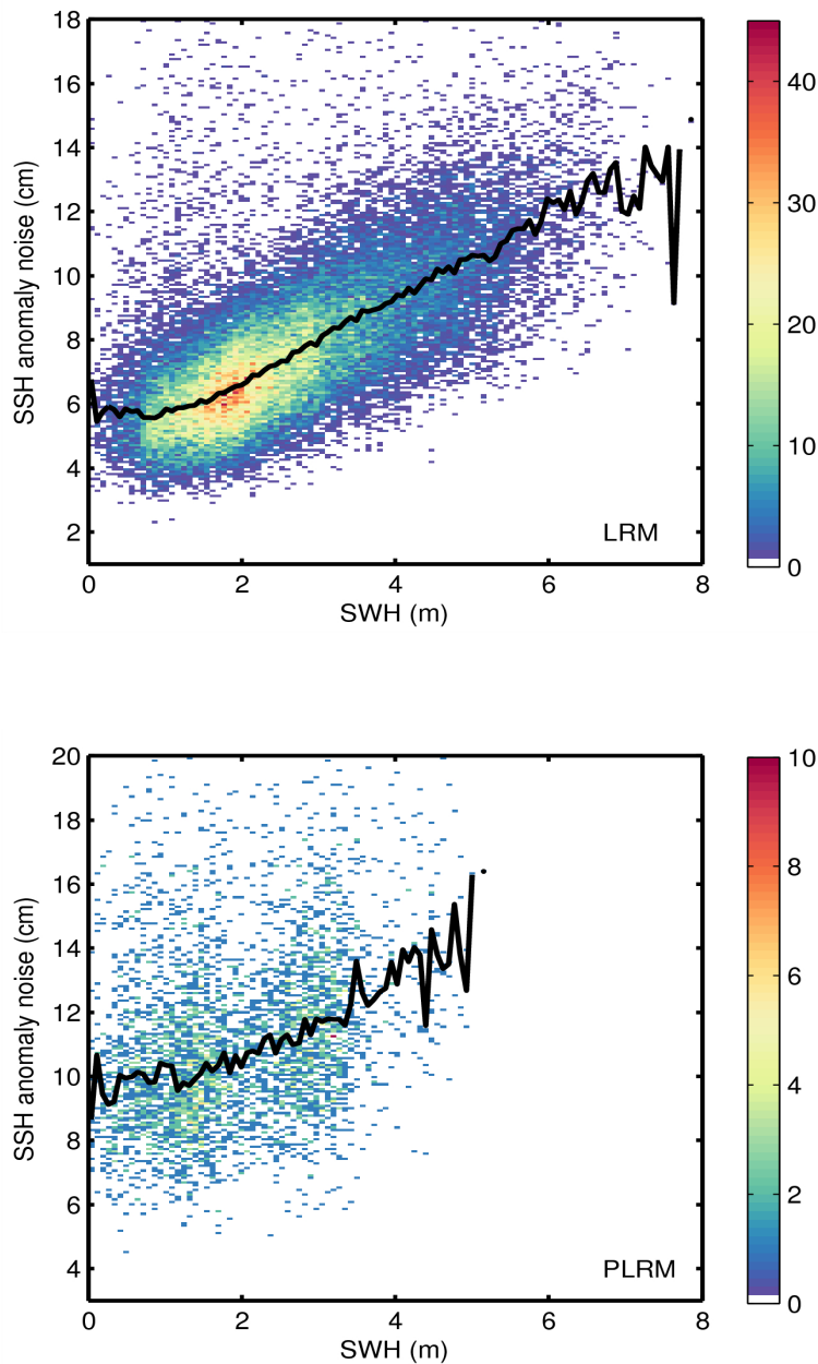
Figure 9. 2D histogram showing flag-valid SSH anomaly noise as a function of SWH for LRM (top) and PLRM (bottom) for 15/06/2015. The black line denotes the median SSH anomaly as a function of SWH.
