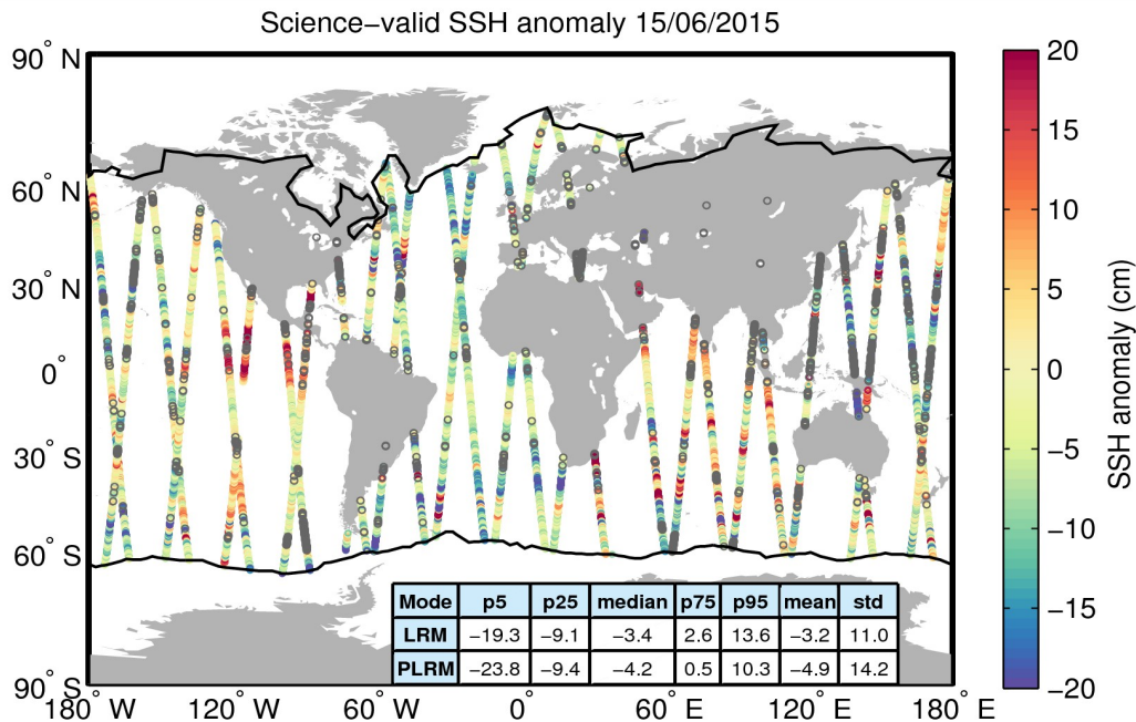
Figure 10. Geographical distribution of science-valid SSH anomaly data over oceans and lakes for 15/06/2015. The statistical values shown in the table refer to the SSH anomaly in cm and are calculated separately for LRM and PLRM regions. The black lines mark the outer limit of the Arctic and Antarctic polar polygons. Gray circles denote records that have been rejected based on the editing criteria described in Table 2.
