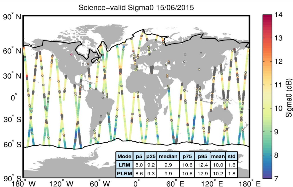
Figure 27. Geographical distribution of science-valid sigma0 data over oceans and lakes for 15/06/2015. The statistical values shown in the table refer to the sigma0 in dB and are calculated separately for LRM and PLRM regions. The black lines mark the outer limit of the Arctic and Antarctic polar polygons. Gray circles denote records that have been rejected based on the editing criteria described in Table 4.
