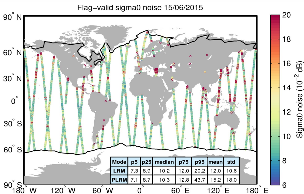
Figure 26. Geographical distribution of flag-valid 20-Hz sigma0 measurement noise over oceans and lakes for 15/06/2015. The statistical values shown in the table refer to the sigma0 noise and are calculated separately for LRM and PLRM regions. Measurements taken over polar polygons have been excluded from the computation of the statistical values. The black lines mark the outer limit of the Arctic and Antarctic polar polygons.
