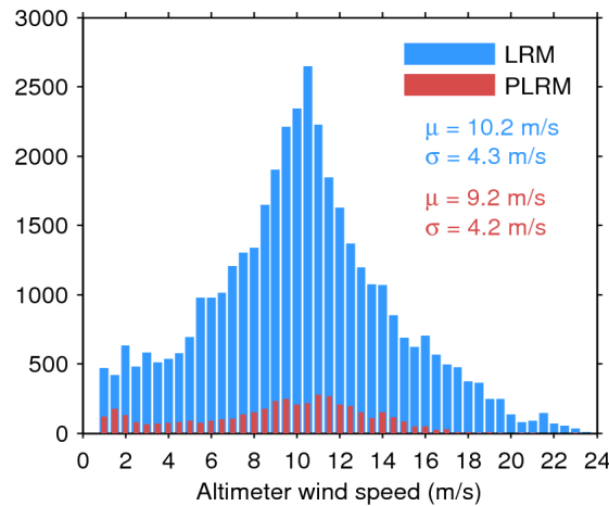
Figure 33. Histogram of flag-valid wind over oceans and lakes for LRM (blue) and PLRM (red) for 15/06/2015. The mean ( \mu ) and standard deviation ( \sigma ) are also shown. Note that values larger than 24 m/s are excluded from the histogram for the sake of readability but not from the computation of \mu and \sigma .
