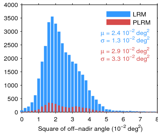
Figure 39. Histogram of flag-valid mispointing over oceans and lakes for LRM (blue) and PLRM (red) for 15/06/2015. Only positive values have been considered. The mean ( \mu ) and standard deviation ( \sigma ) are also shown. Note that values larger than 8 \cdot 10^{-2} \text{ deg}^2 are excluded from the histogram for the sake of readability but not from the computation of \mu and \sigma .
