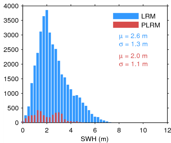
Figure 20. Histogram of science-valid SWH over oceans and lakes for LRM (blue) and PLRM (red) for 15/06/2015. The mean ( \mu ) and standard deviation ( \sigma ) are also shown. Note that values larger than 12 m are excluded from the histogram for the sake of readability but not from the computation of \mu and \sigma .
