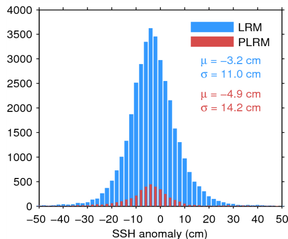
Figure 11. Histogram of science-valid SSH anomaly over oceans and lakes for LRM (blue) and PLRM (red) for 15/06/2015. The mean ( \mu ) and standard deviation ( \sigma ) are also shown. Note that values outside [-50 50] cm are excluded from the histogram for the sake of readability but not from the computation of \mu and \sigma .
