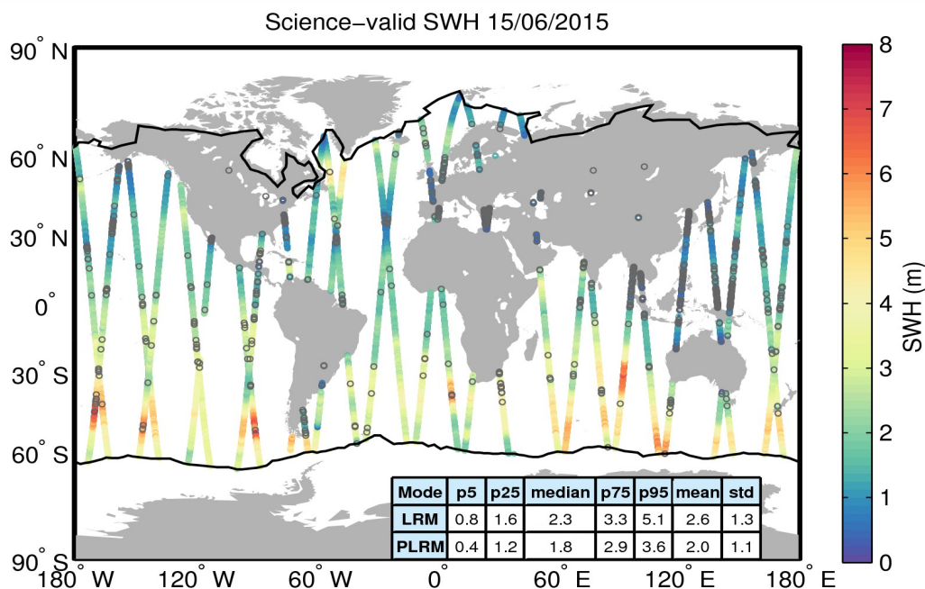
Figure 19. Geographical distribution of science-valid SWH data over oceans and lakes for 15/06/2015. The statistical values shown in the table refer to the SWH in m and are calculated separately for LRM and PLRM regions. The black lines mark the outer limit of the Arctic and Antarctic polar polygons. Gray circles denote records that have been rejected based on the editing criteria described in Table 3.
