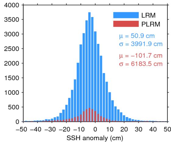
Figure 7. Histogram of flag-valid SSH anomaly over oceans and lakes for LRM (blue) and PLRM (red) for 15/06/2015. The mean ( \mu ) and standard deviation ( \sigma ) are also shown. Note that values outside [-50\ 50] cm are excluded from the histogram for the sake of readability but not from the computation of \mu and \sigma .
