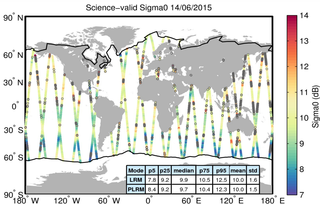
Figure 27. Geographical distribution of science-valid sigma0 data over oceans and lakes for 14/06/2015. The statistical values shown in the table refer to the sigma0 in dB and are calculated separately for LRM and PLRM regions. The black lines mark the outer limit of the Arctic and Antarctic polar polygons. Gray circles denote records that have been rejected based on the editing criteria described in Table 4.
