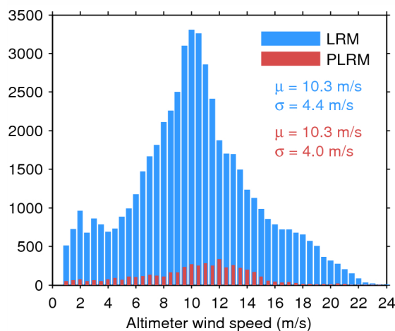
Figure 33. Histogram of flag-valid wind over oceans and lakes for LRM (blue) and PLRM (red) for 14/06/2015. The mean ( \mu ) and standard deviation ( \sigma ) are also shown. Note that values larger than 24 m/s are excluded from the histogram for the sake of readability but not from the computation of \mu and \sigma .
