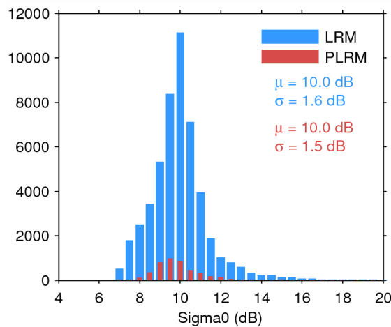
Figure 28. Histogram of science-valid sigma0 over oceans and lakes for LRM (blue) and PLRM (red) for 14/06/2015. The mean ( \mu ) and standard deviation ( \sigma ) are also shown. Note that values outside [4 20] dB are excluded from the histogram for the sake of readability but not from the computation of \mu and \sigma .
