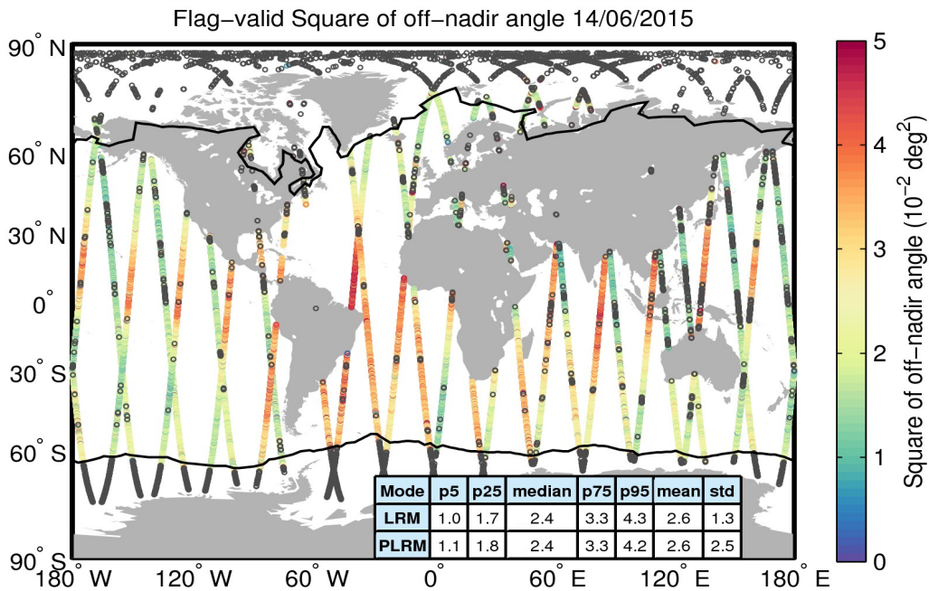
Figure 37. Geographical distribution of flag-valid mispointing data over oceans and lakes for 14/06/2015. The statistical values shown in the table refer to the mispointing in 10^{-2} \text{ deg}^2 and are calculated separately for LRM and PLRM regions. Measurements taken over polar polygons have been excluded from the computation of the statistical values. The black lines mark the outer limit of the Arctic and Antarctic polar polygons. Gray circles denote negative values.
