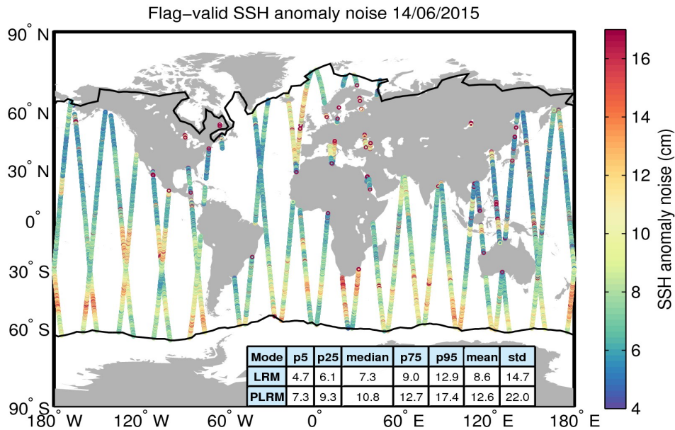
Figure 8. Geographical distribution of flag-valid 20-Hz SSH anomaly measurement noise over oceans and lakes for 14/06/2015. The statistical values shown in the table refer to the SSH anomaly noise and are calculated separately for LRM and PLRM regions. Measurements taken over polar polygons have been excluded from the computation of the statistical values. The black lines mark the outer limit of the Arctic and Antarctic polar polygons.
