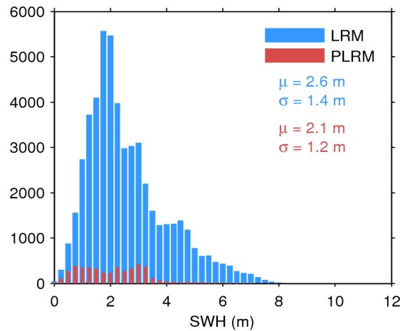
Figure 20. Histogram of science-valid SWH over oceans and lakes for LRM (blue) and PLRM (red) for 14/06/2015. The mean ( \mu ) and standard deviation ( \sigma ) are also shown. Note that values larger than 12 m are excluded from the histogram for the sake of readability but not from the computation of \mu and \sigma .
