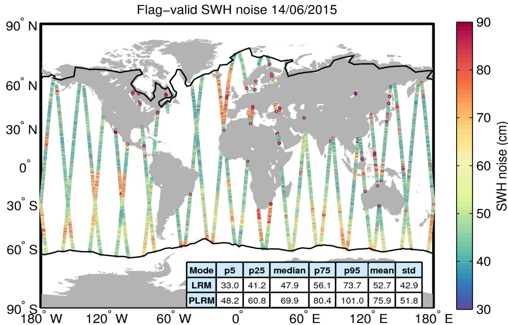
Figure 18. Geographical distribution of flag-valid 20-Hz SWH measurement noise over oceans and lakes for 14/06/2015. The statistical values shown in the table refer to the SWH noise and are calculated separately for LRM and PLRM regions. Measurements taken over polar polygons have been excluded from the computation of the statistical values. The black lines mark the outer limit of the Arctic and Antarctic polar polygons.
