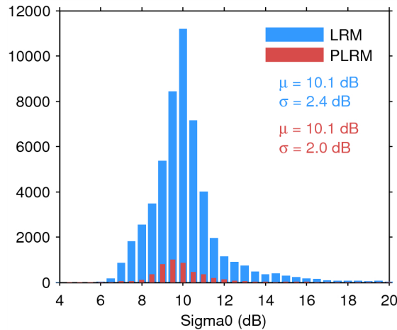
Figure 25. Histogram of flag-valid sigma0 over oceans and lakes for LRM (blue) and PLRM (red) for 14/06/2015. The mean ( \mu ) and standard deviation ( \sigma ) are also shown. Note that values outside [4 20] dB are excluded from the histogram for the sake of readability but not from the computation of \mu and \sigma .
