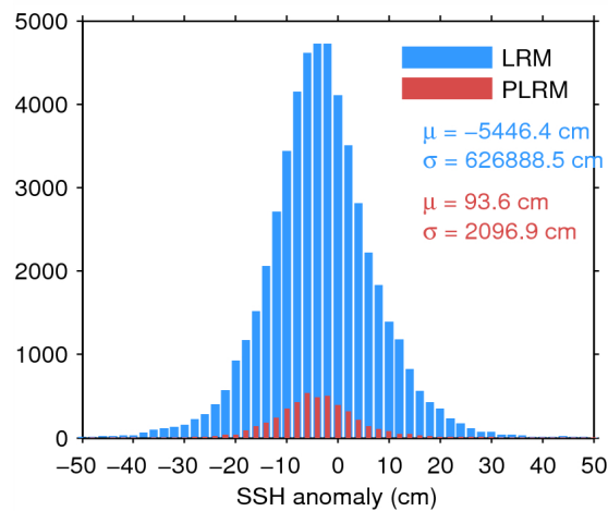
Figure 7. Histogram of flag-valid SSH anomaly over oceans and lakes for LRM (blue) and PLRM (red) for 14/06/2015. The mean ( \mu ) and standard deviation ( \sigma ) are also shown. Note that values outside [-50 50] cm are excluded from the histogram for the sake of readability but not from the computation of \mu and \sigma .
