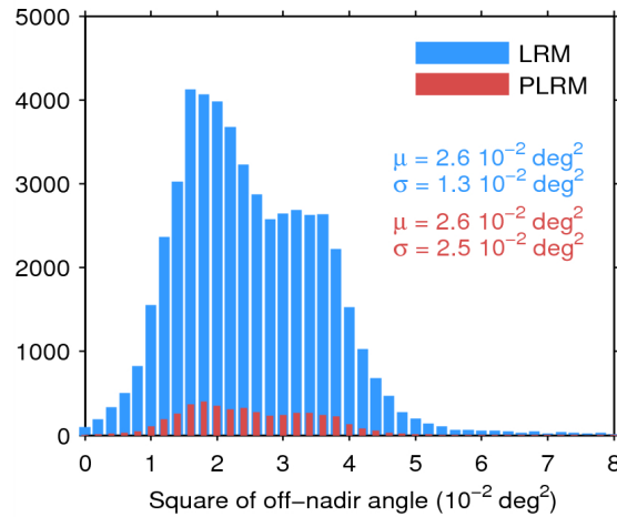
Figure 39. Histogram of flag-valid mispointing over oceans and lakes for LRM (blue) and PLRM (red) for 14/06/2015. Only positive values have been considered. The mean ( \mu ) and standard deviation ( \sigma ) are also shown. Note that values larger than 8 \cdot 10^{-2} \text{ deg}^2 are excluded from the histogram for the sake of readability but not from the computation of \mu and \sigma .
