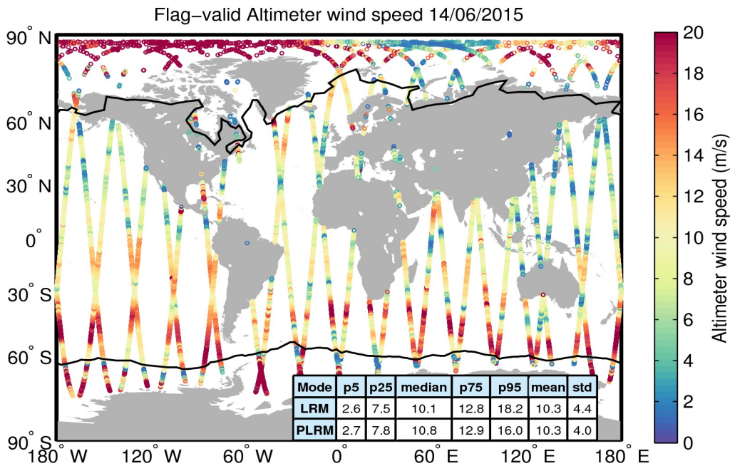
Figure 31. Geographical distribution of flag-valid wind data over oceans and lakes for 14/06/2015. The statistical values shown in the table refer to the wind in m/s and are calculated separately for LRM and PLRM regions. Measurements taken over polar polygons have been excluded from the computation of the statistical values. The black lines mark the outer limit of the Arctic and Antarctic polar polygons.
