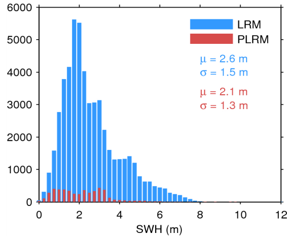
Figure 17. Histogram of flag-valid SWH over oceans and lakes for LRM (blue) and PLRM (red) for 14/06/2015. The mean ( \mu ) and standard deviation ( \sigma ) are also shown. Note that values larger than 12 m are excluded from the histogram for the sake of readability but not from the computation of \mu and \sigma .
