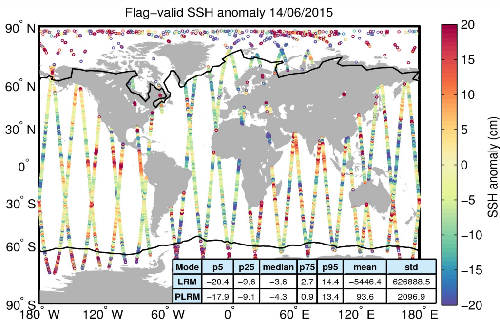
Figure 5. Geographical distribution of flag-valid 1-Hz SSH anomaly data over oceans and lakes for 14/06/2015. The statistical values shown in the table refer to the SSH anomaly in cm and are calculated separately for LRM and PLRM regions. Measurements taken over polar polygons have been excluded from the computation of the statistical values. The black lines mark the outer limit of the Arctic and Antarctic polar polygons.
