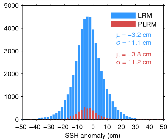
Figure 11. Histogram of science-valid SSH anomaly over oceans and lakes for LRM (blue) and PLRM (red) for 14/06/2015. The mean ( \mu ) and standard deviation ( \sigma ) are also shown. Note that values outside [-50\ 50] cm are excluded from the histogram for the sake of readability but not from the computation of \mu and \sigma .
