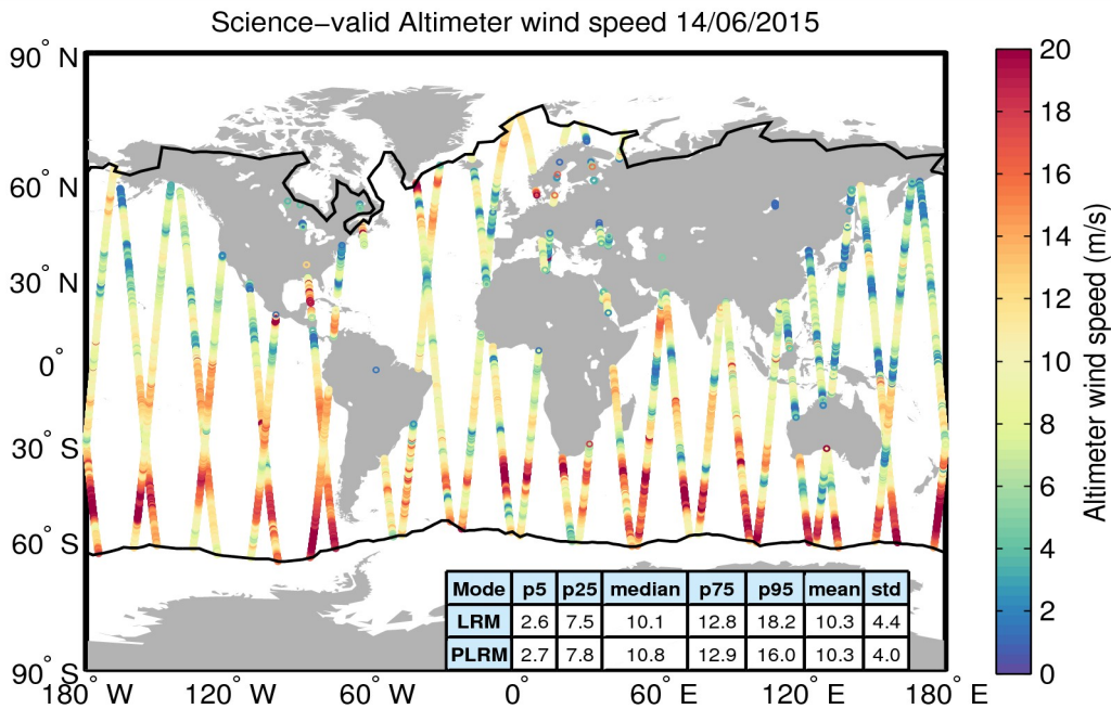
Figure 34. Geographical distribution of science-valid wind data over oceans and lakes for 14/06/2015. The statistical values shown in the table refer to the wind in m/s and are calculated separately for LRM and PLRM regions. The black lines mark the outer limit of the Arctic and Antarctic polar polygons. Gray circles denote records that have been rejected based on the editing criteria described in Table 5.
