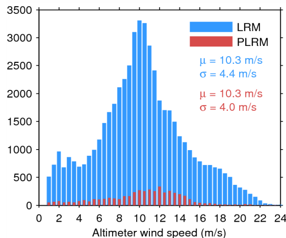
Figure 35. Histogram of science-valid wind over oceans and lakes for LRM (blue) and PLRM (red) for 14/06/2015. The mean ( \mu ) and standard deviation ( \sigma ) are also shown. Note that values larger than 24 m/s are excluded from the histogram for the sake of readability but not from the computation of \mu and \sigma .
