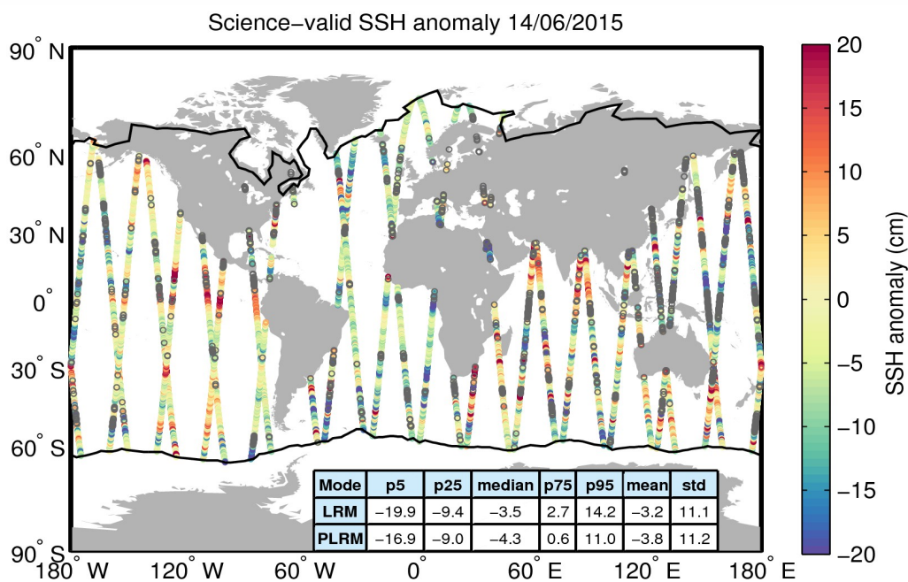
Figure 10. Geographical distribution of science-valid SSH anomaly data over oceans and lakes for 14/06/2015. The statistical values shown in the table refer to the SSH anomaly in cm and are calculated separately for LRM and PLRM regions. The black lines mark the outer limit of the Arctic and Antarctic polar polygons. Gray circles denote records that have been rejected based on the editing criteria described in Table 2.
