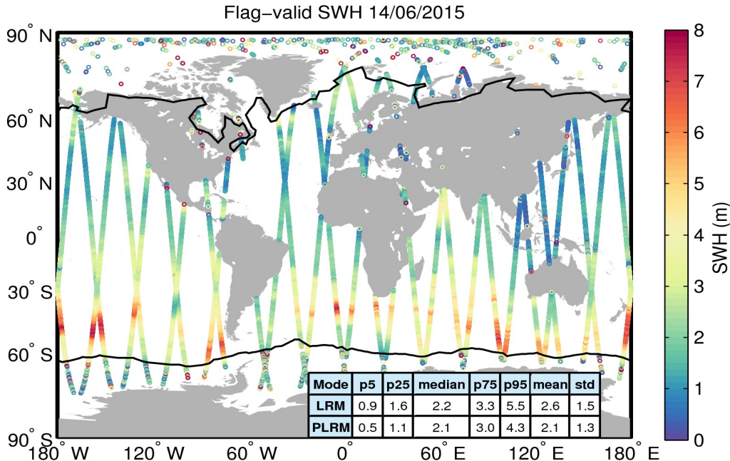
Figure 15. Geographical distribution of flag-valid SWH data over oceans and lakes for 14/06/2015. The statistical values shown in the table refer to the SWH in m and are calculated separately for LRM and PLRM regions. Measurements taken over polar polygons have been excluded from the computation of the statistical values. The black lines mark the outer limit of the Arctic and Antarctic polar polygons.
