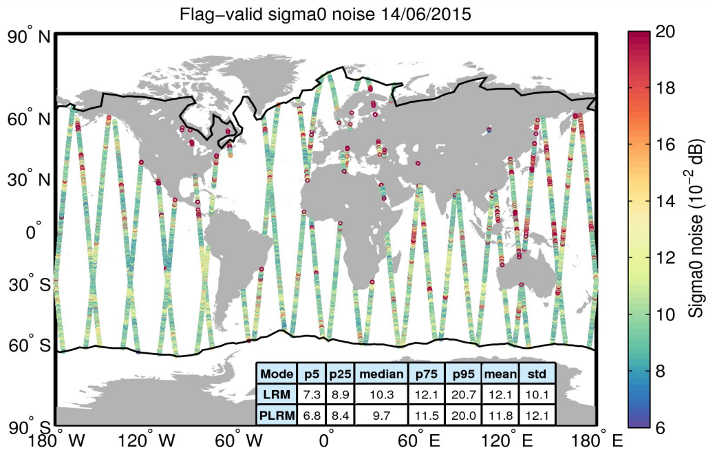
Figure 26. Geographical distribution of flag-valid 20-Hz sigma0 measurement noise over oceans and lakes for 14/06/2015. The statistical values shown in the table refer to the sigma0 noise and are calculated separately for LRM and PLRM regions. Measurements taken over polar polygons have been excluded from the computation of the statistical values. The black lines mark the outer limit of the Arctic and Antarctic polar polygons.
