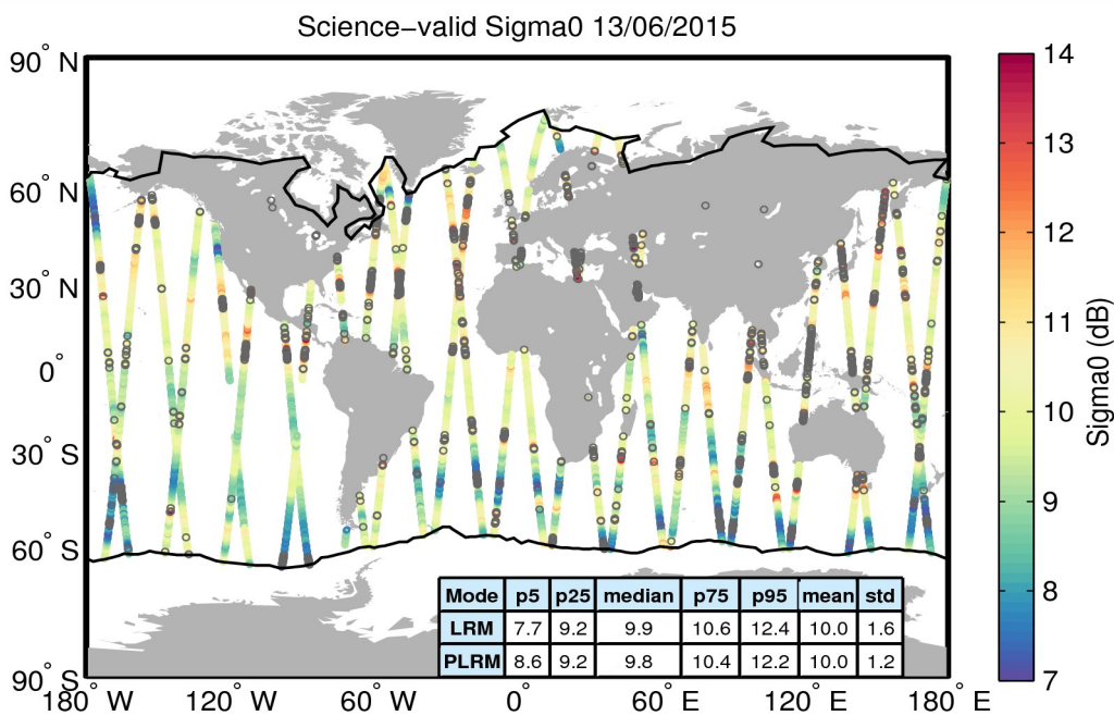
Figure 27. Geographical distribution of science-valid sigma0 data over oceans and lakes for 13/06/2015. The statistical values shown in the table refer to the sigma0 in dB and are calculated separately for LRM and PLRM regions. The black lines mark the outer limit of the Arctic and Antarctic polar polygons. Gray circles denote records that have been rejected based on the editing criteria described in Table 4.
