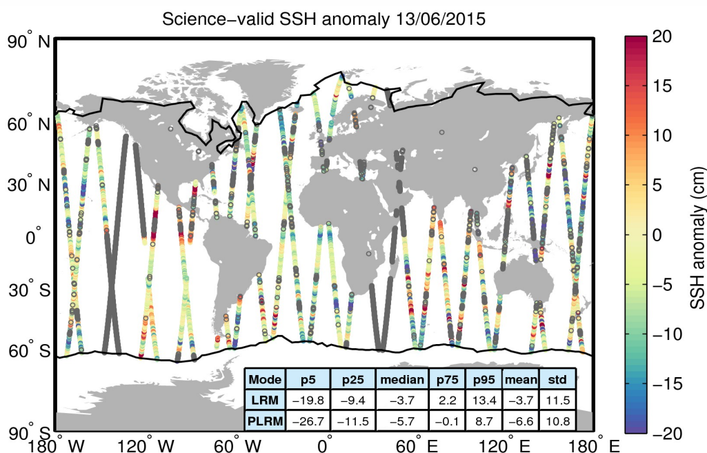
Figure 10. Geographical distribution of science-valid SSH anomaly data over oceans and lakes for 13/06/2015. The statistical values shown in the table refer to the SSH anomaly in cm and are calculated separately for LRM and PLRM regions. The black lines mark the outer limit of the Arctic and Antarctic polar polygons. Gray circles denote records that have been rejected based on the editing criteria described in Table 2.
