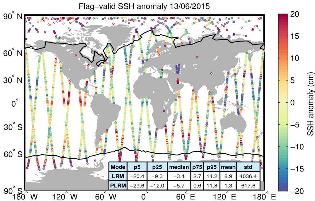
Figure 5. Geographical distribution of flag-valid 1-Hz SSH anomaly data over oceans and lakes for 13/06/2015. The statistical values shown in the table refer to the SSH anomaly in cm and are calculated separately for LRM and PLRM regions. Measurements taken over polar polygons have been excluded from the computation of the statistical values. The black lines mark the outer limit of the Arctic and Antarctic polar polygons.
