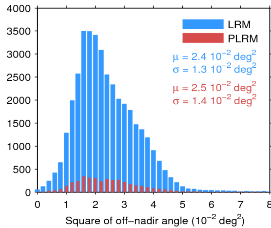
Figure 39. Histogram of flag-valid mispointing over oceans and lakes for LRM (blue) and PLRM (red) for 13/06/2015. Only positive values have been considered. The mean ( \mu ) and standard deviation ( \sigma ) are also shown. Note that values larger than 8 \cdot 10^{-2} \text{ deg}^2 are excluded from the histogram for the sake of readability but not from the computation of \mu and \sigma .
