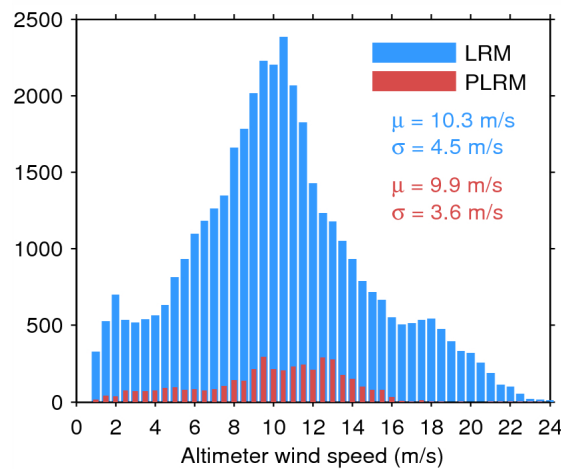
Figure 33. Histogram of flag-valid wind over oceans and lakes for LRM (blue) and PLRM (red) for 13/06/2015. The mean ( \mu ) and standard deviation ( \sigma ) are also shown. Note that values larger than 24 m/s are excluded from the histogram for the sake of readability but not from the computation of \mu and \sigma .
