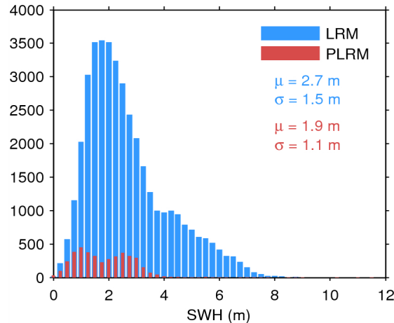
Figure 17. Histogram of flag-valid SWH over oceans and lakes for LRM (blue) and PLRM (red) for 13/06/2015. The mean ( \mu ) and standard deviation ( \sigma ) are also shown. Note that values larger than 12 m are excluded from the histogram for the sake of readability but not from the computation of \mu and \sigma .
