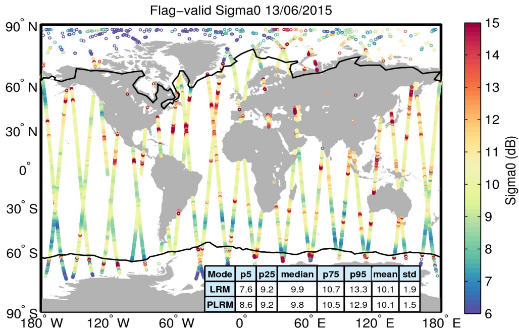
Figure 23. Geographical distribution of flag-valid sigma0 data over oceans and lakes for 13/06/2015. The statistical values shown in the table refer to the sigma0 in dB and are calculated separately for LRM and PLRM regions. Measurements taken over polar polygons have been excluded from the computation of the statistical values. The black lines mark the outer limit of the Arctic and Antarctic polar polygons.
