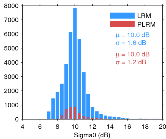
Figure 28. Histogram of science-valid sigma0 over oceans and lakes for LRM (blue) and PLRM (red) for 13/06/2015. The mean ( \mu ) and standard deviation ( \sigma ) are also shown. Note that values outside [4 20] dB are excluded from the histogram for the sake of readability but not from the computation of \mu and \sigma .
