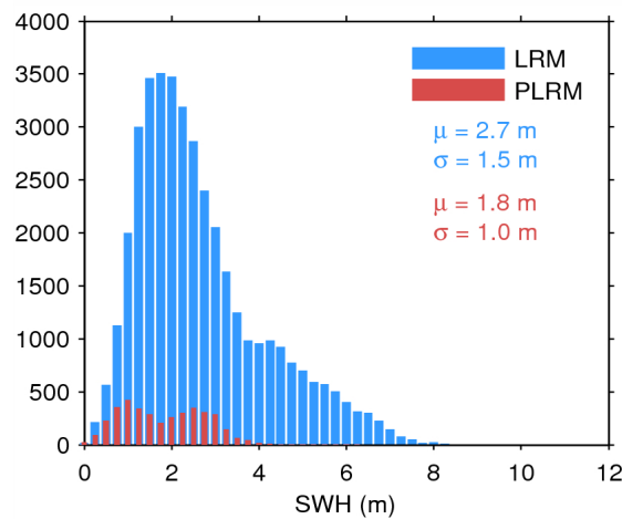
Figure 20. Histogram of science-valid SWH over oceans and lakes for LRM (blue) and PLRM (red) for 13/06/2015. The mean ( \mu ) and standard deviation ( \sigma ) are also shown. Note that values larger than 12 m are excluded from the histogram for the sake of readability but not from the computation of \mu and \sigma .
