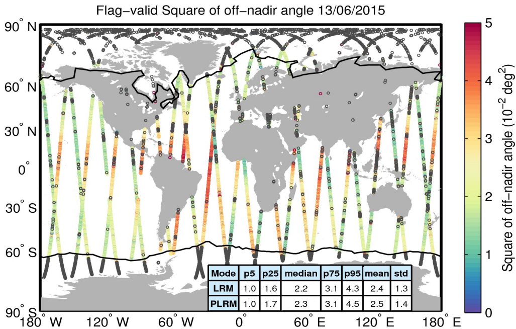
Figure 37. Geographical distribution of flag-valid mispointing data over oceans and lakes for 13/06/2015. The statistical values shown in the table refer to the mispointing in 10^{-2} deg 2 and are calculated separately for LRM and PLRM regions. Measurements taken over polar polygons have been excluded from the computation of the statistical values. The black lines mark the outer limit of the Arctic and Antarctic polar polygons. Gray circles denote negative values.
