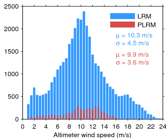
Figure 35. Histogram of science-valid wind over oceans and lakes for LRM (blue) and PLRM (red) for 13/06/2015. The mean ( \mu ) and standard deviation ( \sigma ) are also shown. Note that values larger than 24 m/s are excluded from the histogram for the sake of readability but not from the computation of \mu and \sigma .
