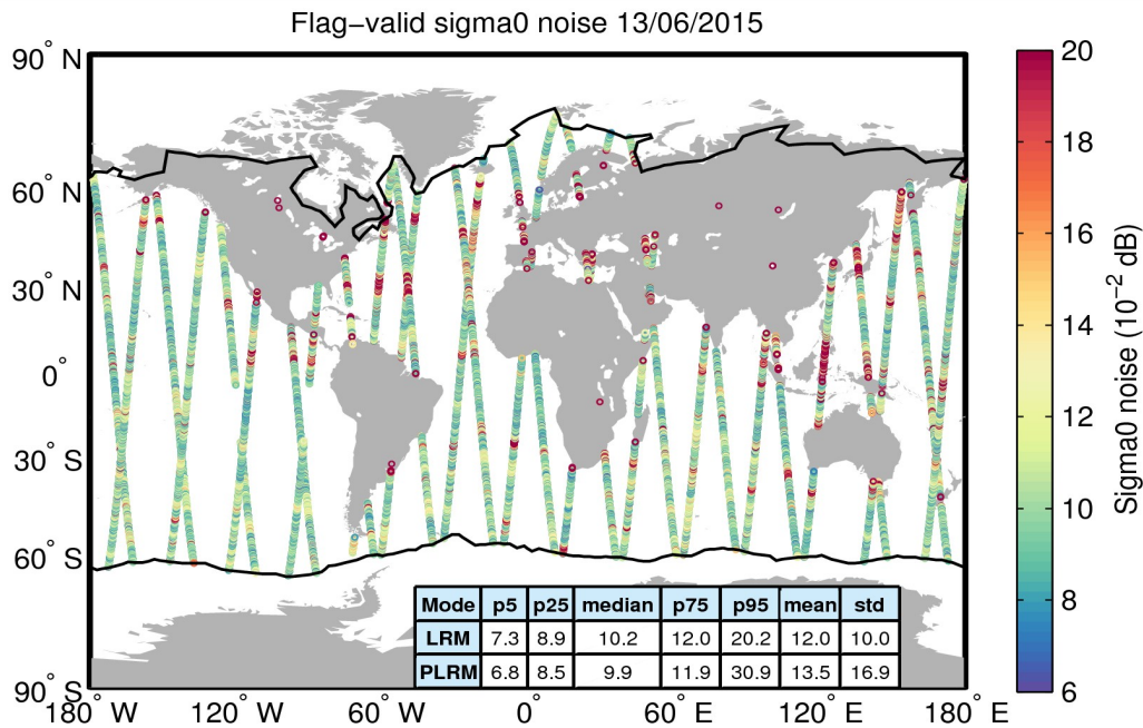
Figure 26. Geographical distribution of flag-valid 20-Hz sigma0 measurement noise over oceans and lakes for 13/06/2015. The statistical values shown in the table refer to the sigma0 noise and are calculated separately for LRM and PLRM regions. Measurements taken over polar polygons have been excluded from the computation of the statistical values. The black lines mark the outer limit of the Arctic and Antarctic polar polygons.
