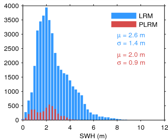
Figure 20. Histogram of science-valid SWH over oceans and lakes for LRM (blue) and PLRM (red) for 12/06/2015. The mean ( \mu ) and standard deviation ( \sigma ) are also shown. Note that values larger than 12 m are excluded from the histogram for the sake of readability but not from the computation of \mu and \sigma .
