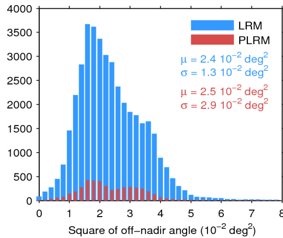
Figure 39. Histogram of flag-valid mispointing over oceans and lakes for LRM (blue) and PLRM (red) for 12/06/2015. Only positive values have been considered. The mean ( \mu ) and standard deviation ( \sigma ) are also shown. Note that values larger than 8 \cdot 10^{-2} \text{ deg}^2 are excluded from the histogram for the sake of readability but not from the computation of \mu and \sigma .
