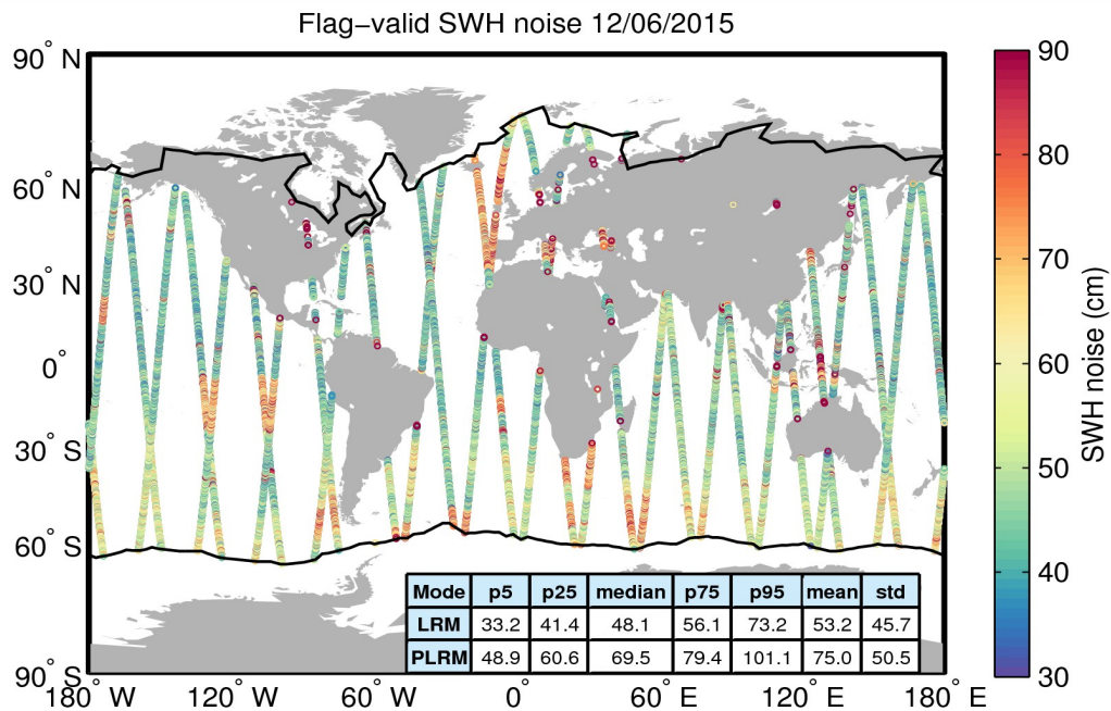
Figure 18. Geographical distribution of flag-valid 20-Hz SWH measurement noise over oceans and lakes for 12/06/2015. The statistical values shown in the table refer to the SWH noise and are calculated separately for LRM and PLRM regions. Measurements taken over polar polygons have been excluded from the computation of the statistical values. The black lines mark the outer limit of the Arctic and Antarctic polar polygons.
