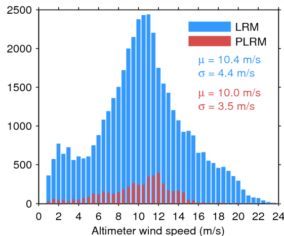
Figure 35. Histogram of science-valid wind over oceans and lakes for LRM (blue) and PLRM (red) for 12/06/2015. The mean ( \mu ) and standard deviation ( \sigma ) are also shown. Note that values larger than 24 m/s are excluded from the histogram for the sake of readability but not from the computation of \mu and \sigma .
