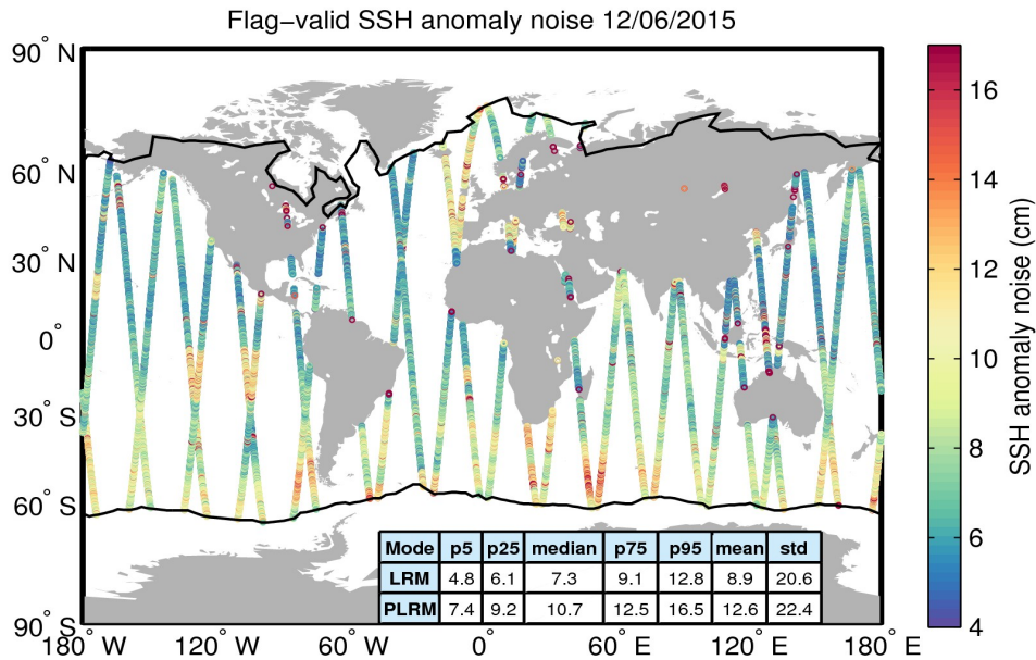
Figure 8. Geographical distribution of flag-valid 20-Hz SSH anomaly measurement noise over oceans and lakes for 12/06/2015. The statistical values shown in the table refer to the SSH anomaly noise and are calculated separately for LRM and PLRM regions. Measurements taken over polar polygons have been excluded from the computation of the statistical values. The black lines mark the outer limit of the Arctic and Antarctic polar polygons.
