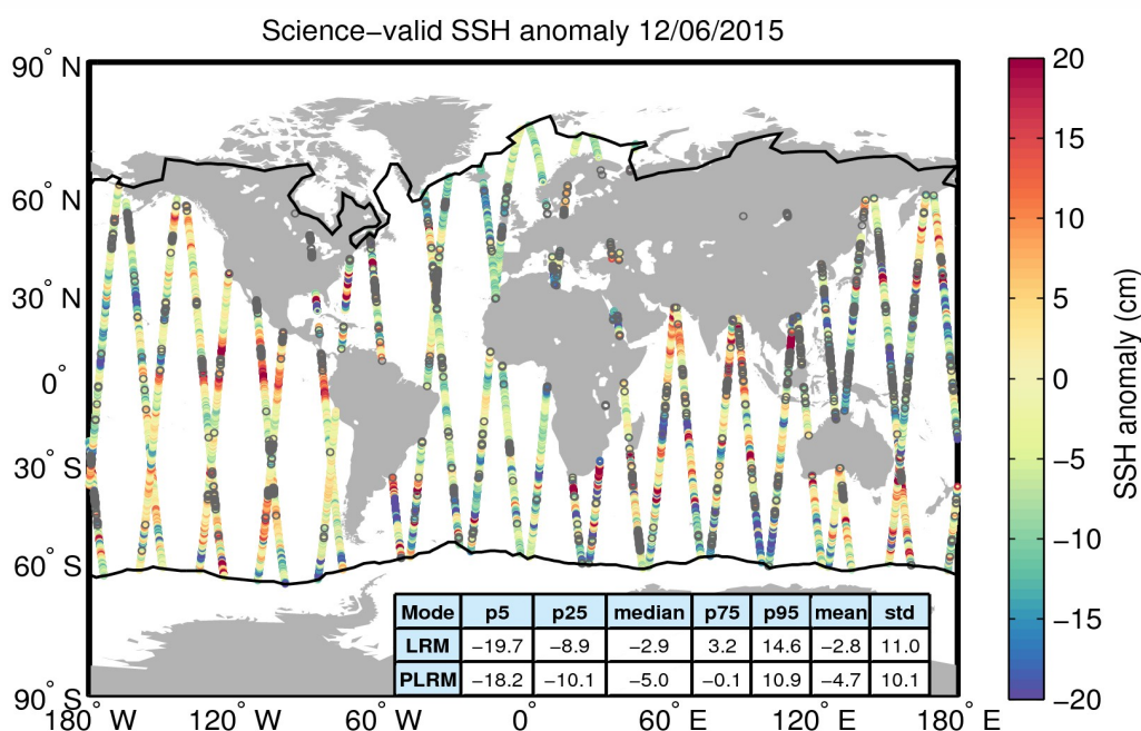
Figure 10. Geographical distribution of science-valid SSH anomaly data over oceans and lakes for 12/06/2015. The statistical values shown in the table refer to the SSH anomaly in cm and are calculated separately for LRM and PLRM regions. The black lines mark the outer limit of the Arctic and Antarctic polar polygons. Gray circles denote records that have been rejected based on the editing criteria described in Table 2.
