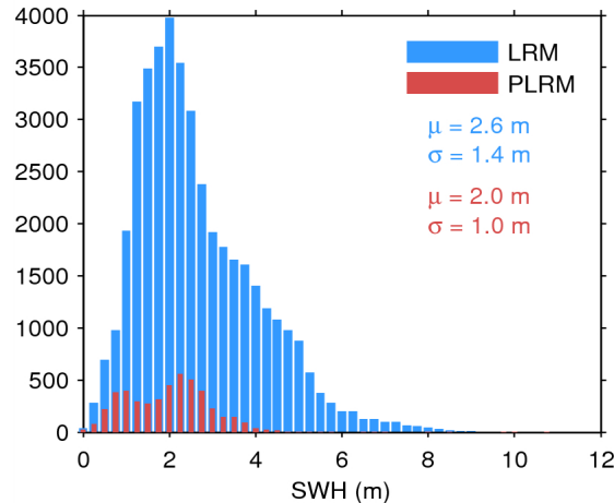
Figure 17. Histogram of flag-valid SWH over oceans and lakes for LRM (blue) and PLRM (red) for 12/06/2015. The mean ( \mu ) and standard deviation ( \sigma ) are also shown. Note that values larger than 12 m are excluded from the histogram for the sake of readability but not from the computation of \mu and \sigma .
