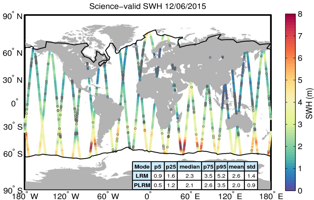
Figure 19. Geographical distribution of science-valid SWH data over oceans and lakes for 12/06/2015. The statistical values shown in the table refer to the SWH in m and are calculated separately for LRM and PLRM regions. The black lines mark the outer limit of the Arctic and Antarctic polar polygons. Gray circles denote records that have been rejected based on the editing criteria described in Table 3.
