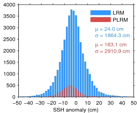
Figure 7. Histogram of flag-valid SSH anomaly over oceans and lakes for LRM (blue) and PLRM (red) for 12/06/2015. The mean ( \mu ) and standard deviation ( \sigma ) are also shown. Note that values outside [-50\ 50] cm are excluded from the histogram for the sake of readability but not from the computation of \mu and \sigma .
