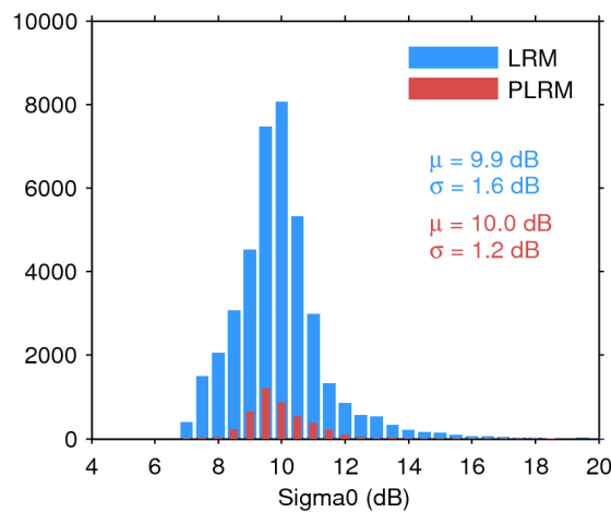
Figure 28. Histogram of science-valid sigma0 over oceans and lakes for LRM (blue) and PLRM (red) for 12/06/2015. The mean ( \mu ) and standard deviation ( \sigma ) are also shown. Note that values outside [4 20] dB are excluded from the histogram for the sake of readability but not from the computation of \mu and \sigma .
