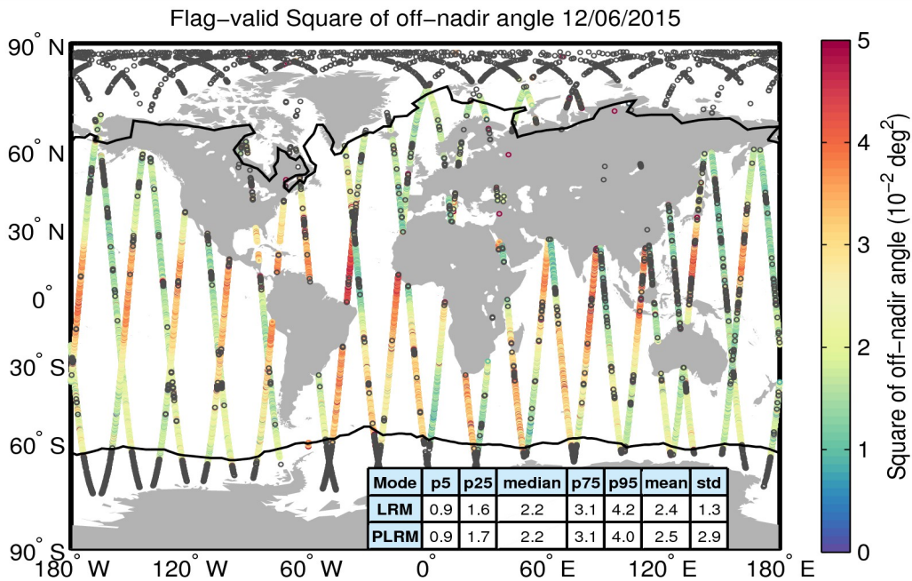
Figure 37. Geographical distribution of flag-valid mispointing data over oceans and lakes for 12/06/2015. The statistical values shown in the table refer to the mispointing in 10^{-2} \text{ deg}^2 and are calculated separately for LRM and PLRM regions. Measurements taken over polar polygons have been excluded from the computation of the statistical values. The black lines mark the outer limit of the Arctic and Antarctic polar polygons. Gray circles denote negative values.
