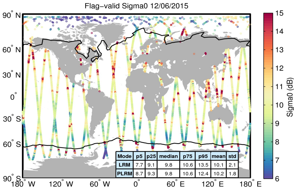
Figure 23. Geographical distribution of flag-valid sigma0 data over oceans and lakes for 12/06/2015. The statistical values shown in the table refer to the sigma0 in dB and are calculated separately for LRM and PLRM regions. Measurements taken over polar polygons have been excluded from the computation of the statistical values. The black lines mark the outer limit of the Arctic and Antarctic polar polygons.
