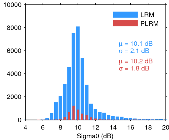
Figure 25. Histogram of flag-valid sigma0 over oceans and lakes for LRM (blue) and PLRM (red) for 12/06/2015. The mean ( \mu ) and standard deviation ( \sigma ) are also shown. Note that values outside [4 20] dB are excluded from the histogram for the sake of readability but not from the computation of \mu and \sigma .
