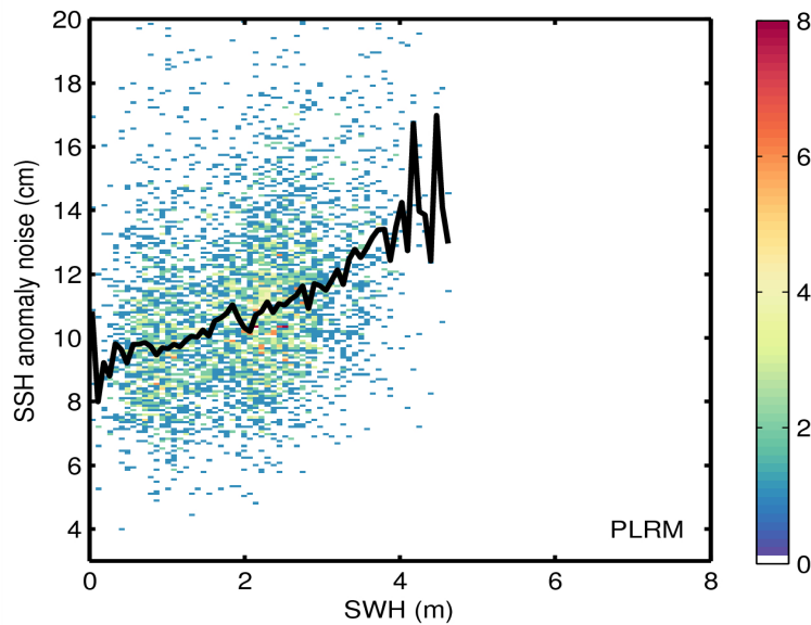
Figure 9. 2D histogram showing flag-valid SSH anomaly noise as a function of SWH for LRM (top) and PLRM (bottom) for 12/06/2015. The black line denotes the median SSH anomaly as a function of SWH.
