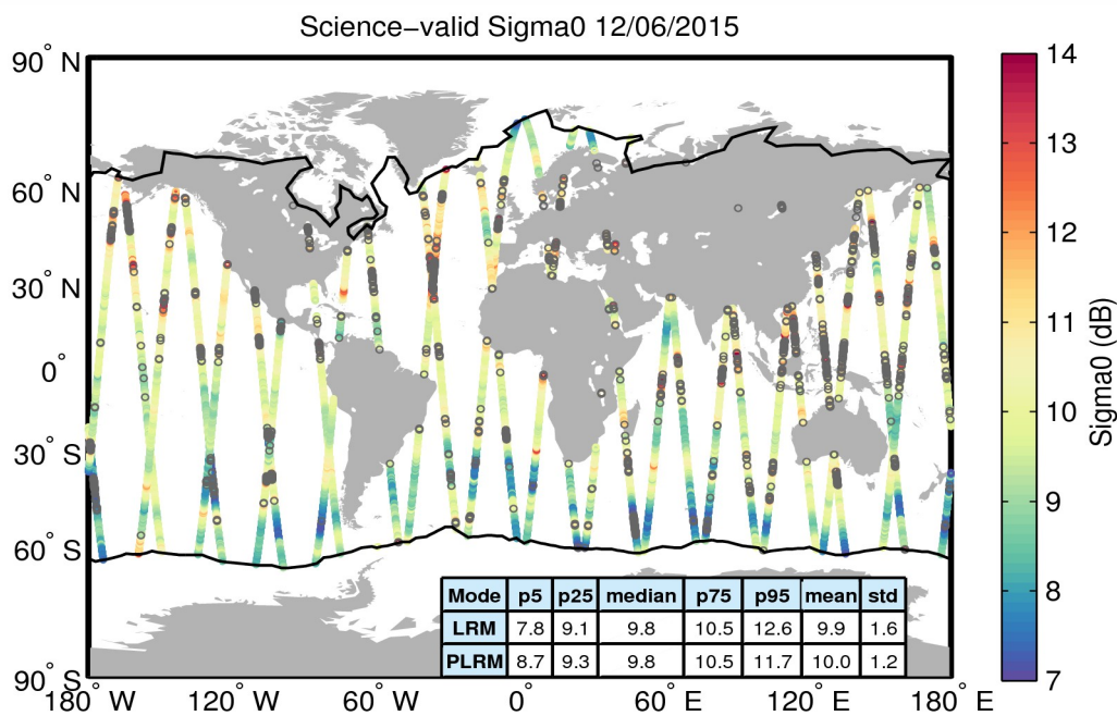
Figure 27. Geographical distribution of science-valid sigma0 data over oceans and lakes for 12/06/2015. The statistical values shown in the table refer to the sigma0 in dB and are calculated separately for LRM and PLRM regions. The black lines mark the outer limit of the Arctic and Antarctic polar polygons. Gray circles denote records that have been rejected based on the editing criteria described in Table 4.
