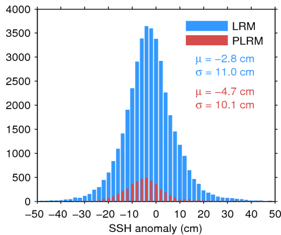
Figure 11. Histogram of science-valid SSH anomaly over oceans and lakes for LRM (blue) and PLRM (red) for 12/06/2015. The mean ( \mu ) and standard deviation ( \sigma ) are also shown. Note that values outside [-50 50] cm are excluded from the histogram for the sake of readability but not from the computation of \mu and \sigma .
