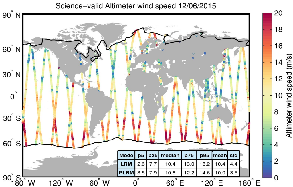
Figure 34. Geographical distribution of science-valid wind data over oceans and lakes for 12/06/2015. The statistical values shown in the table refer to the wind in m/s and are calculated separately for LRM and PLRM regions. The black lines mark the outer limit of the Arctic and Antarctic polar polygons. Gray circles denote records that have been rejected based on the editing criteria described in Table 5.
