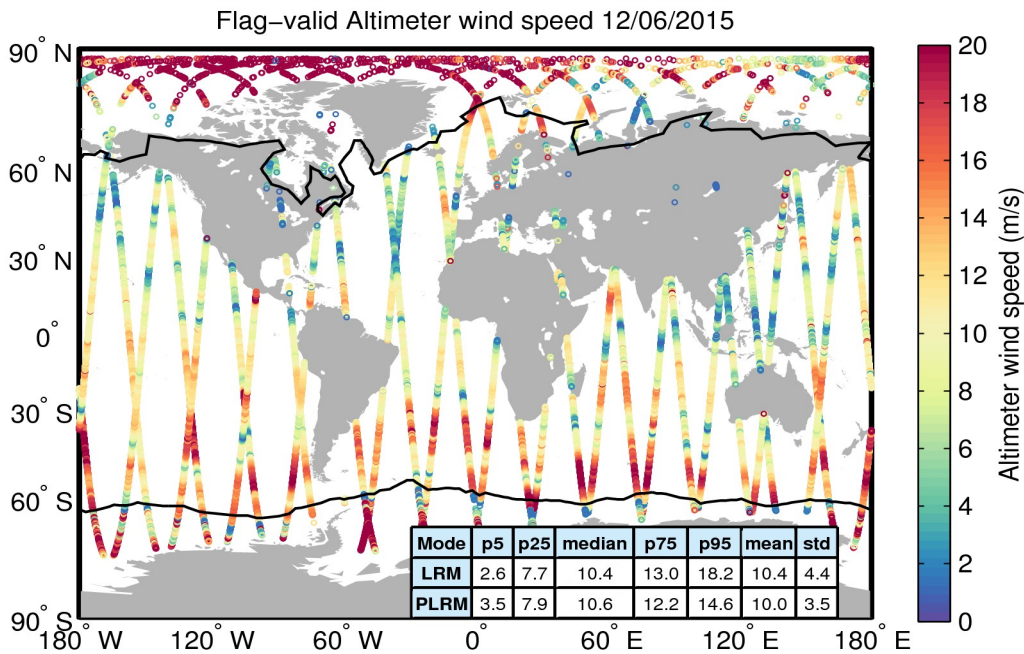
Figure 31. Geographical distribution of flag-valid wind data over oceans and lakes for 12/06/2015. The statistical values shown in the table refer to the wind in m/s and are calculated separately for LRM and PLRM regions. Measurements taken over polar polygons have been excluded from the computation of the statistical values. The black lines mark the outer limit of the Arctic and Antarctic polar polygons.
