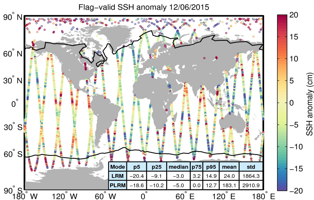
Figure 5. Geographical distribution of flag-valid 1-Hz SSH anomaly data over oceans and lakes for 12/06/2015. The statistical values shown in the table refer to the SSH anomaly in cm and are calculated separately for LRM and PLRM regions. Measurements taken over polar polygons have been excluded from the computation of the statistical values. The black lines mark the outer limit of the Arctic and Antarctic polar polygons.
