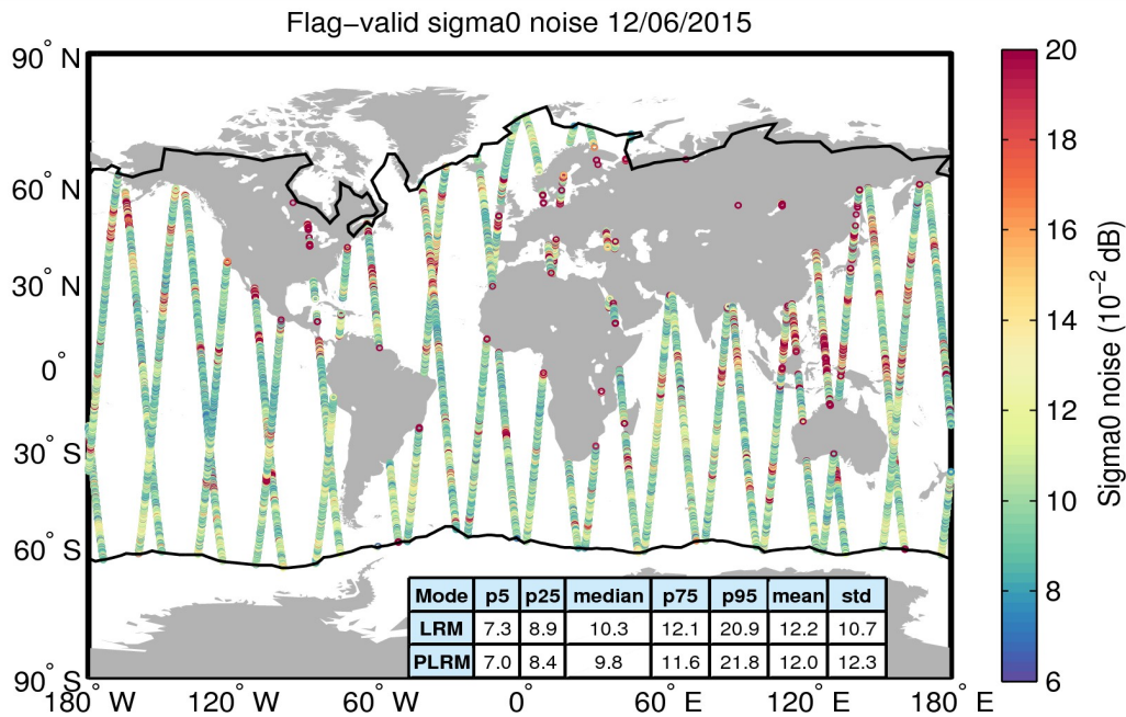
Figure 26. Geographical distribution of flag-valid 20-Hz sigma0 measurement noise over oceans and lakes for 12/06/2015. The statistical values shown in the table refer to the sigma0 noise and are calculated separately for LRM and PLRM regions. Measurements taken over polar polygons have been excluded from the computation of the statistical values. The black lines mark the outer limit of the Arctic and Antarctic polar polygons.
