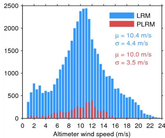
Figure 33. Histogram of flag-valid wind over oceans and lakes for LRM (blue) and PLRM (red) for 12/06/2015. The mean ( \mu ) and standard deviation ( \sigma ) are also shown. Note that values larger than 24 m/s are excluded from the histogram for the sake of readability but not from the computation of \mu and \sigma .
