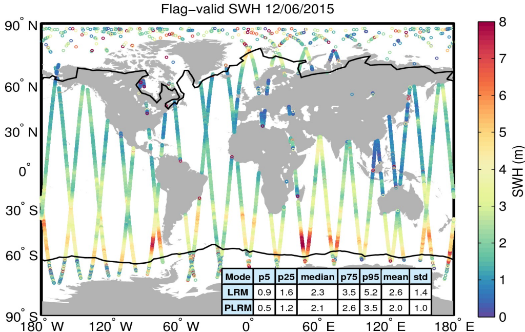
Figure 15. Geographical distribution of flag-valid SWH data over oceans and lakes for 12/06/2015. The statistical values shown in the table refer to the SWH in m and are calculated separately for LRM and PLRM regions. Measurements taken over polar polygons have been excluded from the computation of the statistical values. The black lines mark the outer limit of the Arctic and Antarctic polar polygons.
