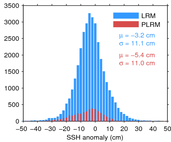
Figure 11. Histogram of science-valid SSH anomaly over oceans and lakes for LRM (blue) and PLRM (red) for 09/06/2015. The mean ( \mu ) and standard deviation ( \sigma ) are also shown. Note that values outside [-50 50] cm are excluded from the histogram for the sake of readability but not from the computation of \mu and \sigma .
