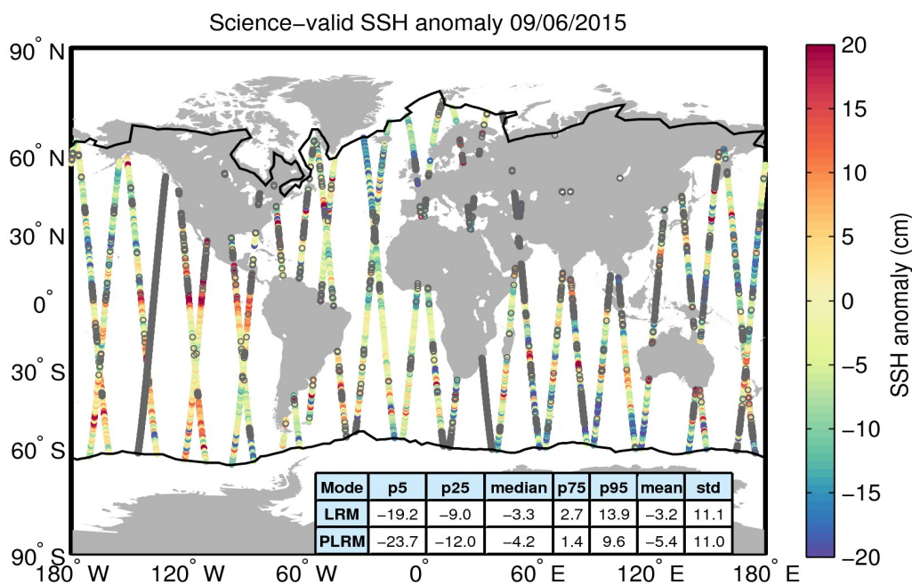
Figure 10. Geographical distribution of science-valid SSH anomaly data over oceans and lakes for 09/06/2015. The statistical values shown in the table refer to the SSH anomaly in cm and are calculated separately for LRM and PLRM regions. The black lines mark the outer limit of the Arctic and Antarctic polar polygons. Gray circles denote records that have been rejected based on the editing criteria described in Table 2.
