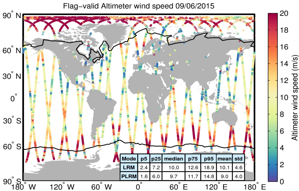
Figure 31. Geographical distribution of flag-valid wind data over oceans and lakes for 09/06/2015. The statistical values shown in the table refer to the wind in m/s and are calculated separately for LRM and PLRM regions. Measurements taken over polar polygons have been excluded from the computation of the statistical values. The black lines mark the outer limit of the Arctic and Antarctic polar polygons.
