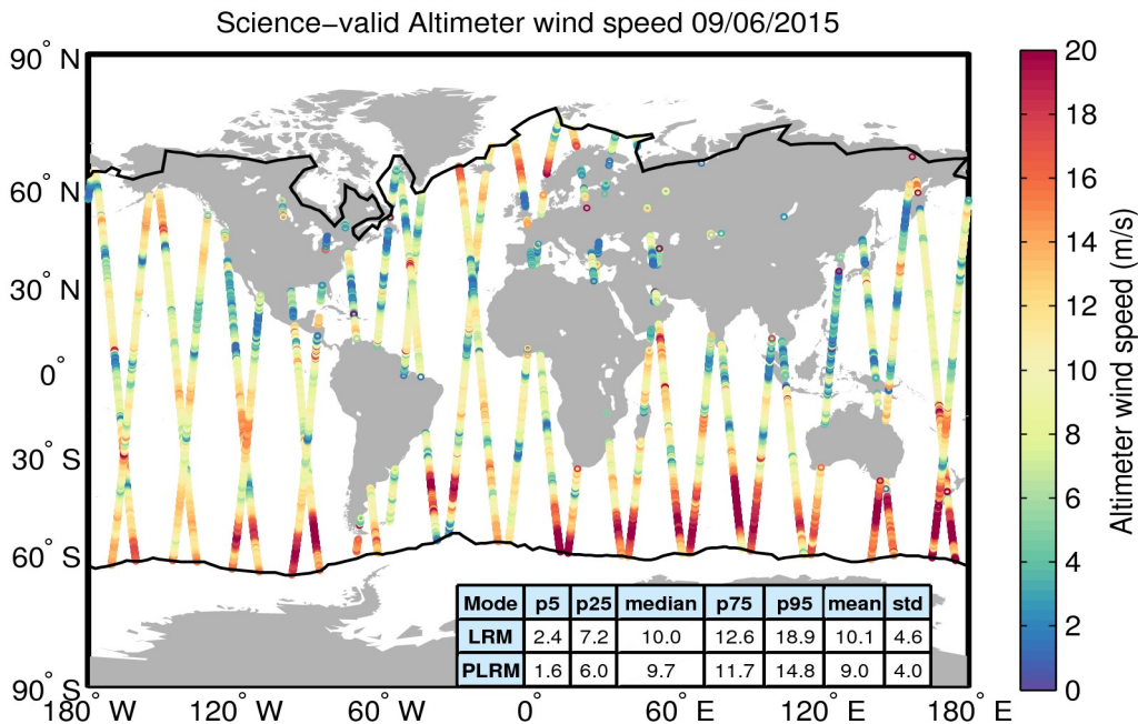
Figure 34. Geographical distribution of science-valid wind data over oceans and lakes for 09/06/2015. The statistical values shown in the table refer to the wind in m/s and are calculated separately for LRM and PLRM regions. The black lines mark the outer limit of the Arctic and Antarctic polar polygons. Gray circles denote records that have been rejected based on the editing criteria described in Table 5.
