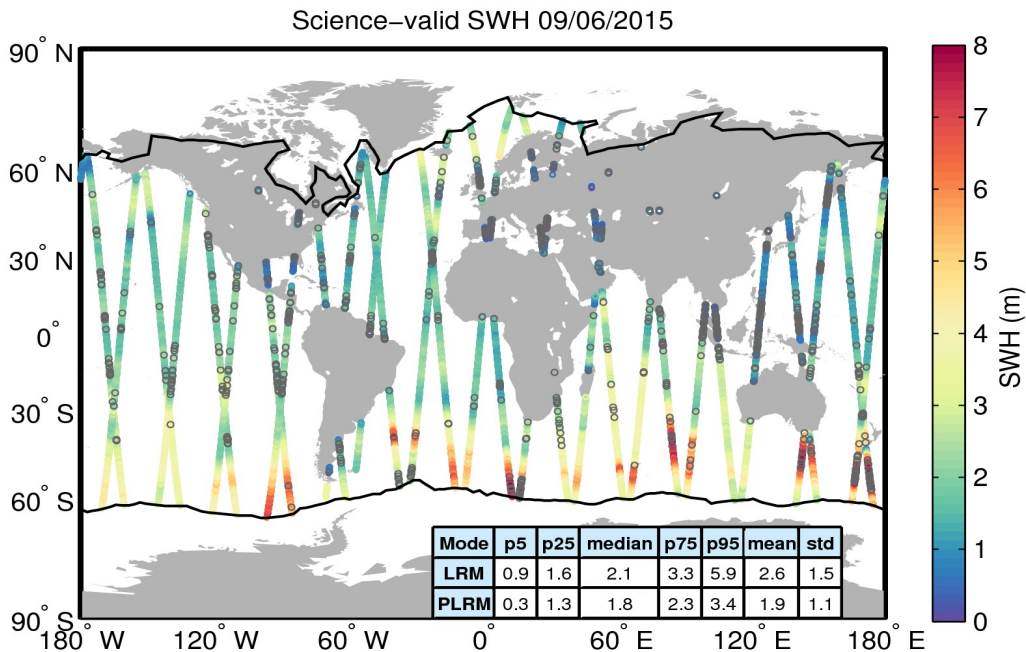
Figure 19. Geographical distribution of science-valid SWH data over oceans and lakes for 09/06/2015. The statistical values shown in the table refer to the SWH in m and are calculated separately for LRM and PLRM regions. The black lines mark the outer limit of the Arctic and Antarctic polar polygons. Gray circles denote records that have been rejected based on the editing criteria described in Table 3.
