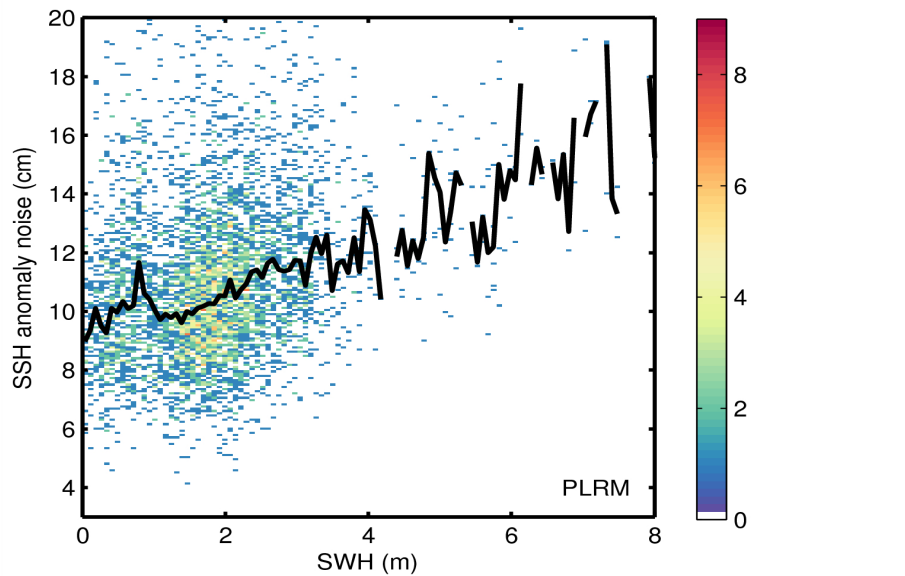
Figure 9. 2D histogram showing flag-valid SSH anomaly noise as a function of SWH for LRM (top) and PLRM (bottom) for 09/06/2015. The black line denotes the median SSH anomaly as a function of SWH.
