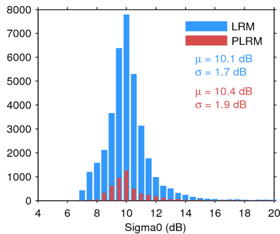
Figure 28. Histogram of science-valid sigma0 over oceans and lakes for LRM (blue) and PLRM (red) for 09/06/2015. The mean ( \mu ) and standard deviation ( \sigma ) are also shown. Note that values outside [4 20] dB are excluded from the histogram for the sake of readability but not from the computation of \mu and \sigma .
