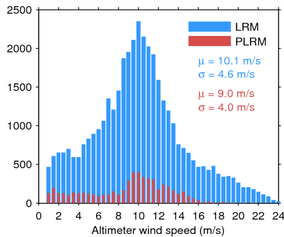
Figure 33. Histogram of flag-valid wind over oceans and lakes for LRM (blue) and PLRM (red) for 09/06/2015. The mean ( \mu ) and standard deviation ( \sigma ) are also shown. Note that values larger than 24 m/s are excluded from the histogram for the sake of readability but not from the computation of \mu and \sigma .
