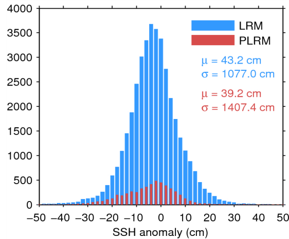
Figure 7. Histogram of flag-valid SSH anomaly over oceans and lakes for LRM (blue) and PLRM (red) for 09/06/2015. The mean ( \mu ) and standard deviation ( \sigma ) are also shown. Note that values outside [-50\ 50] cm are excluded from the histogram for the sake of readability but not from the computation of \mu and \sigma .
