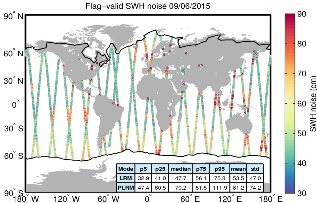
Figure 18. Geographical distribution of flag-valid 20-Hz SWH measurement noise over oceans and lakes for 09/06/2015. The statistical values shown in the table refer to the SWH noise and are calculated separately for LRM and PLRM regions. Measurements taken over polar polygons have been excluded from the computation of the statistical values. The black lines mark the outer limit of the Arctic and Antarctic polar polygons.
