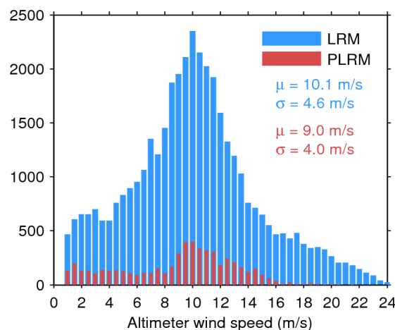
Figure 35. Histogram of science-valid wind over oceans and lakes for LRM (blue) and PLRM (red) for 09/06/2015. The mean ( \mu ) and standard deviation ( \sigma ) are also shown. Note that values larger than 24 m/s are excluded from the histogram for the sake of readability but not from the computation of \mu and \sigma .
