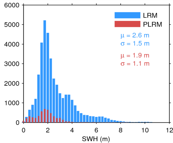
Figure 20. Histogram of science-valid SWH over oceans and lakes for LRM (blue) and PLRM (red) for 09/06/2015. The mean ( \mu ) and standard deviation ( \sigma ) are also shown. Note that values larger than 12 m are excluded from the histogram for the sake of readability but not from the computation of \mu and \sigma .
