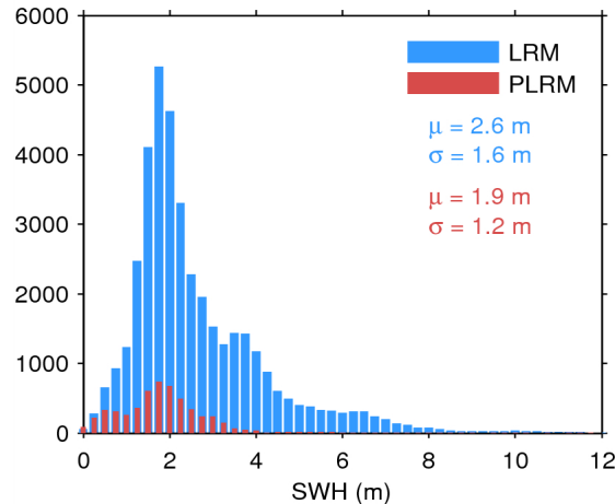
Figure 17. Histogram of flag-valid SWH over oceans and lakes for LRM (blue) and PLRM (red) for 09/06/2015. The mean ( \mu ) and standard deviation ( \sigma ) are also shown. Note that values larger than 12 m are excluded from the histogram for the sake of readability but not from the computation of \mu and \sigma .
