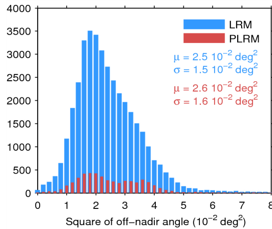
Figure 39. Histogram of flag-valid mispointing over oceans and lakes for LRM (blue) and PLRM (red) for 09/06/2015. Only positive values have been considered. The mean ( \mu ) and standard deviation ( \sigma ) are also shown. Note that values larger than 8 \cdot 10^{-2} \text{ deg}^2 are excluded from the histogram for the sake of readability but not from the computation of \mu and \sigma .
