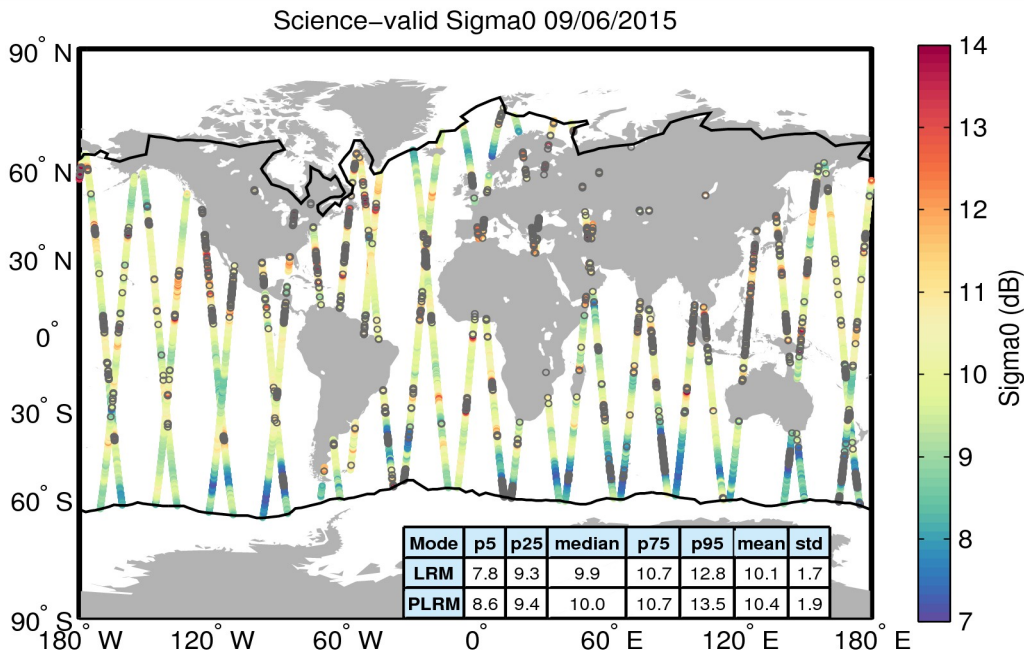
Figure 27. Geographical distribution of science-valid sigma0 data over oceans and lakes for 09/06/2015. The statistical values shown in the table refer to the sigma0 in dB and are calculated separately for LRM and PLRM regions. The black lines mark the outer limit of the Arctic and Antarctic polar polygons. Gray circles denote records that have been rejected based on the editing criteria described in Table 4.
