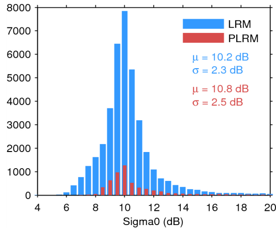
Figure 25. Histogram of flag-valid sigma0 over oceans and lakes for LRM (blue) and PLRM (red) for 09/06/2015. The mean ( \mu ) and standard deviation ( \sigma ) are also shown. Note that values outside [4 20] dB are excluded from the histogram for the sake of readability but not from the computation of \mu and \sigma .
