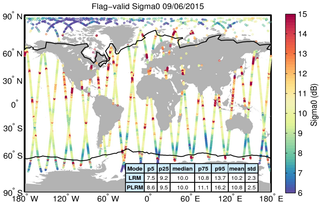
Figure 23. Geographical distribution of flag-valid sigma0 data over oceans and lakes for 09/06/2015. The statistical values shown in the table refer to the sigma0 in dB and are calculated separately for LRM and PLRM regions. Measurements taken over polar polygons have been excluded from the computation of the statistical values. The black lines mark the outer limit of the Arctic and Antarctic polar polygons.
