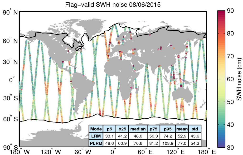
Figure 18. Geographical distribution of flag-valid 20-Hz SWH measurement noise over oceans and lakes for 08/06/2015. The statistical values shown in the table refer to the SWH noise and are calculated separately for LRM and PLRM regions. Measurements taken over polar polygons have been excluded from the computation of the statistical values. The black lines mark the outer limit of the Arctic and Antarctic polar polygons.
