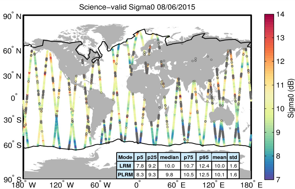
Figure 27. Geographical distribution of science-valid sigma0 data over oceans and lakes for 08/06/2015. The statistical values shown in the table refer to the sigma0 in dB and are calculated separately for LRM and PLRM regions. The black lines mark the outer limit of the Arctic and Antarctic polar polygons. Gray circles denote records that have been rejected based on the editing criteria described in Table 4.
