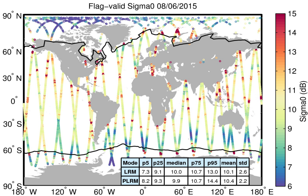
Figure 23. Geographical distribution of flag-valid sigma0 data over oceans and lakes for 08/06/2015. The statistical values shown in the table refer to the sigma0 in dB and are calculated separately for LRM and PLRM regions. Measurements taken over polar polygons have been excluded from the computation of the statistical values. The black lines mark the outer limit of the Arctic and Antarctic polar polygons.
