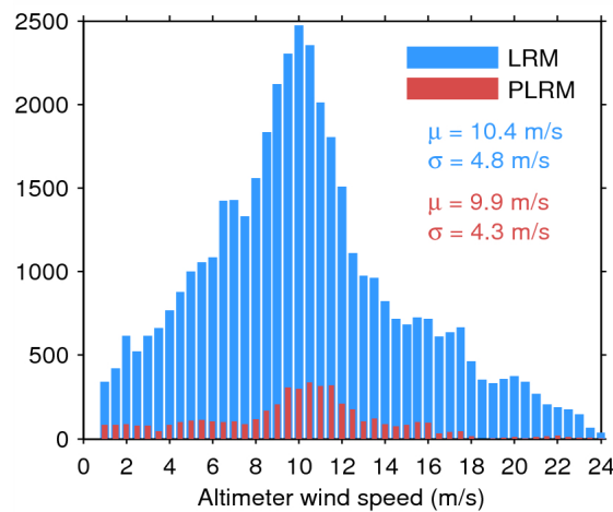
Figure 33. Histogram of flag-valid wind over oceans and lakes for LRM (blue) and PLRM (red) for 08/06/2015. The mean ( \mu ) and standard deviation ( \sigma ) are also shown. Note that values larger than 24 m/s are excluded from the histogram for the sake of readability but not from the computation of \mu and \sigma .
