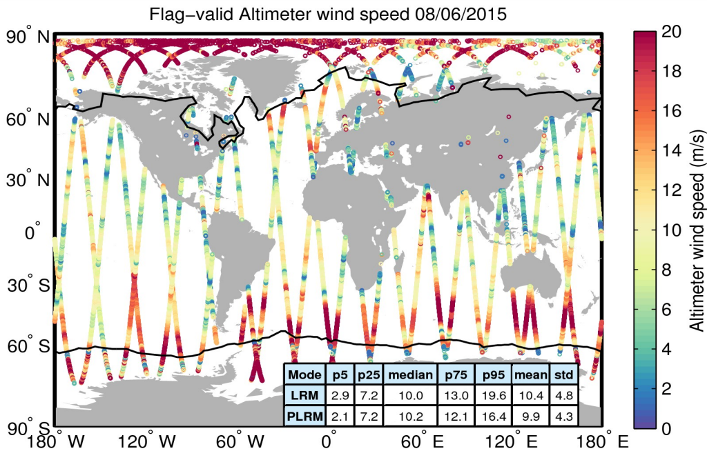
Figure 31. Geographical distribution of flag-valid wind data over oceans and lakes for 08/06/2015. The statistical values shown in the table refer to the wind in m/s and are calculated separately for LRM and PLRM regions. Measurements taken over polar polygons have been excluded from the computation of the statistical values. The black lines mark the outer limit of the Arctic and Antarctic polar polygons.
