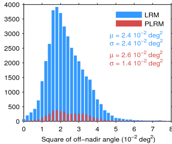
Figure 39. Histogram of flag-valid mispointing over oceans and lakes for LRM (blue) and PLRM (red) for 08/06/2015. Only positive values have been considered. The mean ( \mu ) and standard deviation ( \sigma ) are also shown. Note that values larger than 8 \cdot 10^{-2} \text{ deg}^2 are excluded from the histogram for the sake of readability but not from the computation of \mu and \sigma .
