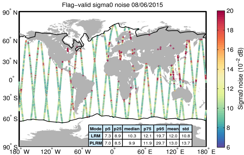
Figure 26. Geographical distribution of flag-valid 20-Hz sigma0 measurement noise over oceans and lakes for 08/06/2015. The statistical values shown in the table refer to the sigma0 noise and are calculated separately for LRM and PLRM regions. Measurements taken over polar polygons have been excluded from the computation of the statistical values. The black lines mark the outer limit of the Arctic and Antarctic polar polygons.
