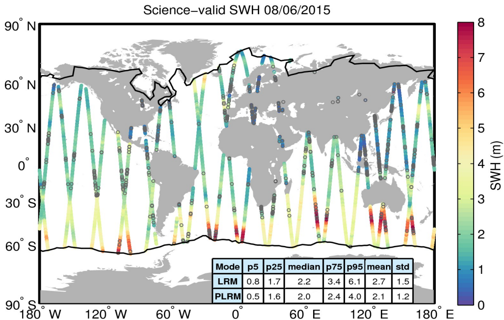
Figure 19. Geographical distribution of science-valid SWH data over oceans and lakes for 08/06/2015. The statistical values shown in the table refer to the SWH in m and are calculated separately for LRM and PLRM regions. The black lines mark the outer limit of the Arctic and Antarctic polar polygons. Gray circles denote records that have been rejected based on the editing criteria described in Table 3.
