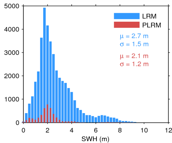
Figure 20. Histogram of science-valid SWH over oceans and lakes for LRM (blue) and PLRM (red) for 08/06/2015. The mean ( \mu ) and standard deviation ( \sigma ) are also shown. Note that values larger than 12 m are excluded from the histogram for the sake of readability but not from the computation of \mu and \sigma .
