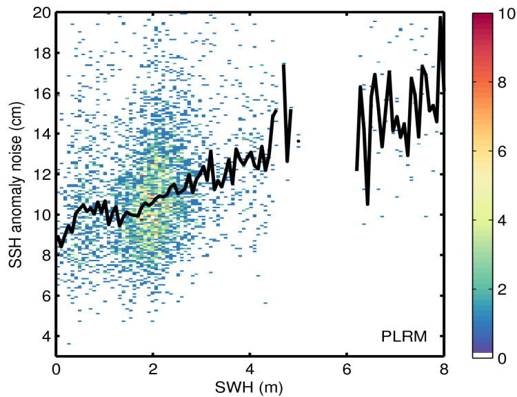
Figure 9. 2D histogram showing flag-valid SSH anomaly noise as a function of SWH for LRM (top) and PLRM (bottom) for 08/06/2015. The black line denotes the median SSH anomaly as a function of SWH.
