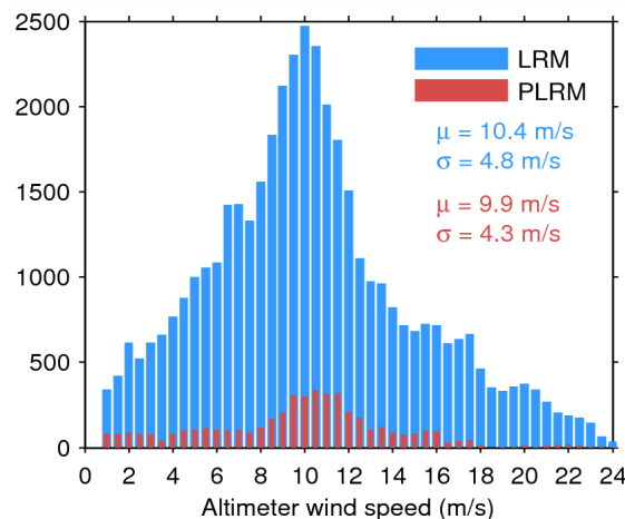
Figure 35. Histogram of science-valid wind over oceans and lakes for LRM (blue) and PLRM (red) for 08/06/2015. The mean ( \mu ) and standard deviation ( \sigma ) are also shown. Note that values larger than 24 m/s are excluded from the histogram for the sake of readability but not from the computation of \mu and \sigma .
