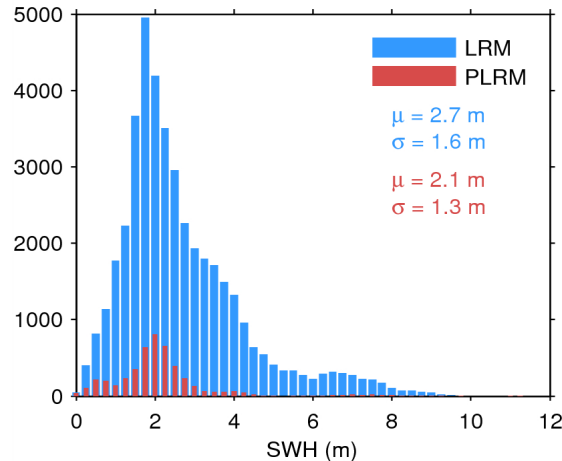
Figure 17. Histogram of flag-valid SWH over oceans and lakes for LRM (blue) and PLRM (red) for 08/06/2015. The mean ( \mu ) and standard deviation ( \sigma ) are also shown. Note that values larger than 12 m are excluded from the histogram for the sake of readability but not from the computation of \mu and \sigma .
