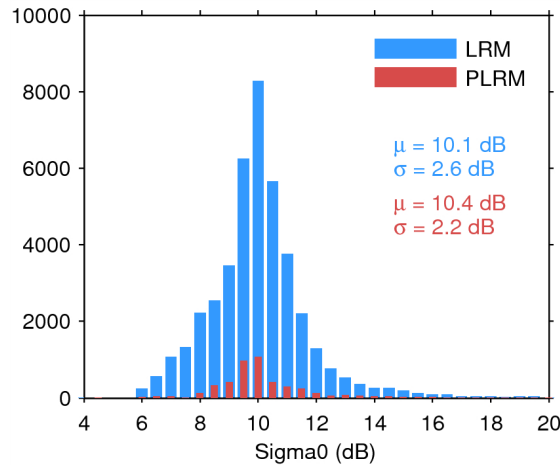
Figure 25. Histogram of flag-valid sigma0 over oceans and lakes for LRM (blue) and PLRM (red) for 08/06/2015. The mean ( \mu ) and standard deviation ( \sigma ) are also shown. Note that values outside [4 20] dB are excluded from the histogram for the sake of readability but not from the computation of \mu and \sigma .
