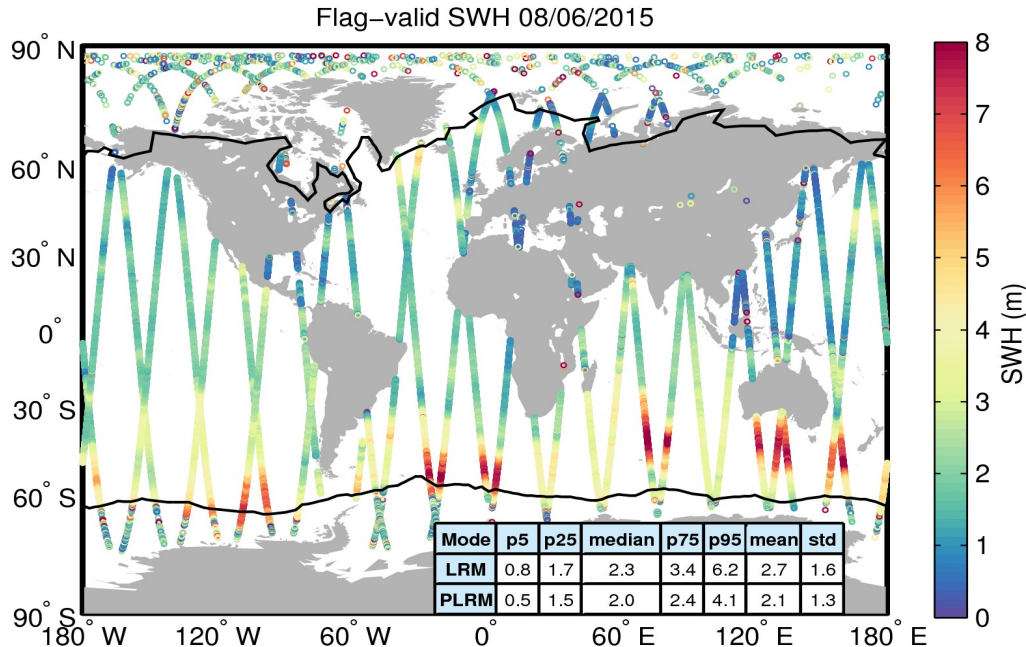
Figure 15. Geographical distribution of flag-valid SWH data over oceans and lakes for 08/06/2015. The statistical values shown in the table refer to the SWH in m and are calculated separately for LRM and PLRM regions. Measurements taken over polar polygons have been excluded from the computation of the statistical values. The black lines mark the outer limit of the Arctic and Antarctic polar polygons.
