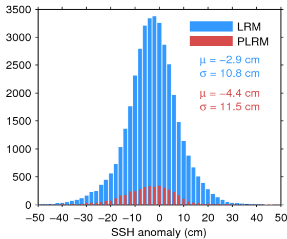
Figure 11. Histogram of science-valid SSH anomaly over oceans and lakes for LRM (blue) and PLRM (red) for 08/06/2015. The mean ( \mu ) and standard deviation ( \sigma ) are also shown. Note that values outside [-50 50] cm are excluded from the histogram for the sake of readability but not from the computation of \mu and \sigma .
