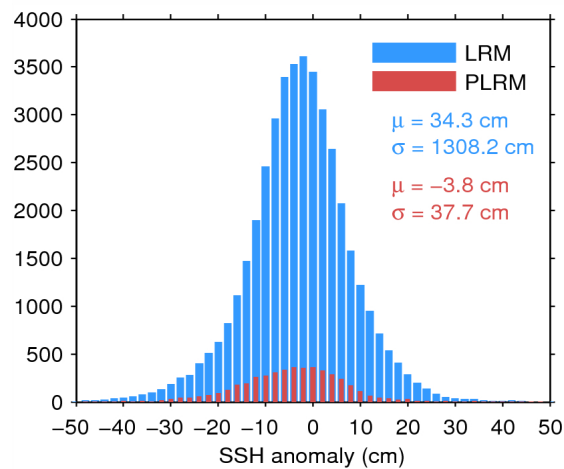
Figure 7. Histogram of flag-valid SSH anomaly over oceans and lakes for LRM (blue) and PLRM (red) for 08/06/2015. The mean ( \mu ) and standard deviation ( \sigma ) are also shown. Note that values outside [-50\ 50] cm are excluded from the histogram for the sake of readability but not from the computation of \mu and \sigma .
