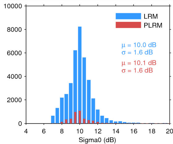
Figure 28. Histogram of science-valid sigma0 over oceans and lakes for LRM (blue) and PLRM (red) for 08/06/2015. The mean ( \mu ) and standard deviation ( \sigma ) are also shown. Note that values outside [4 20] dB are excluded from the histogram for the sake of readability but not from the computation of \mu and \sigma .
