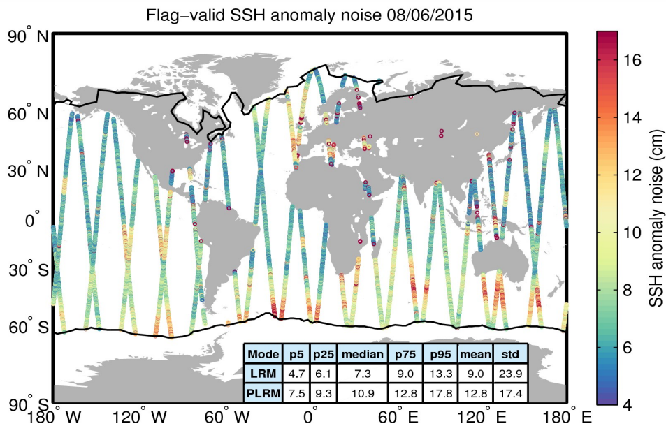
Figure 8. Geographical distribution of flag-valid 20-Hz SSH anomaly measurement noise over oceans and lakes for 08/06/2015. The statistical values shown in the table refer to the SSH anomaly noise and are calculated separately for LRM and PLRM regions. Measurements taken over polar polygons have been excluded from the computation of the statistical values. The black lines mark the outer limit of the Arctic and Antarctic polar polygons.
