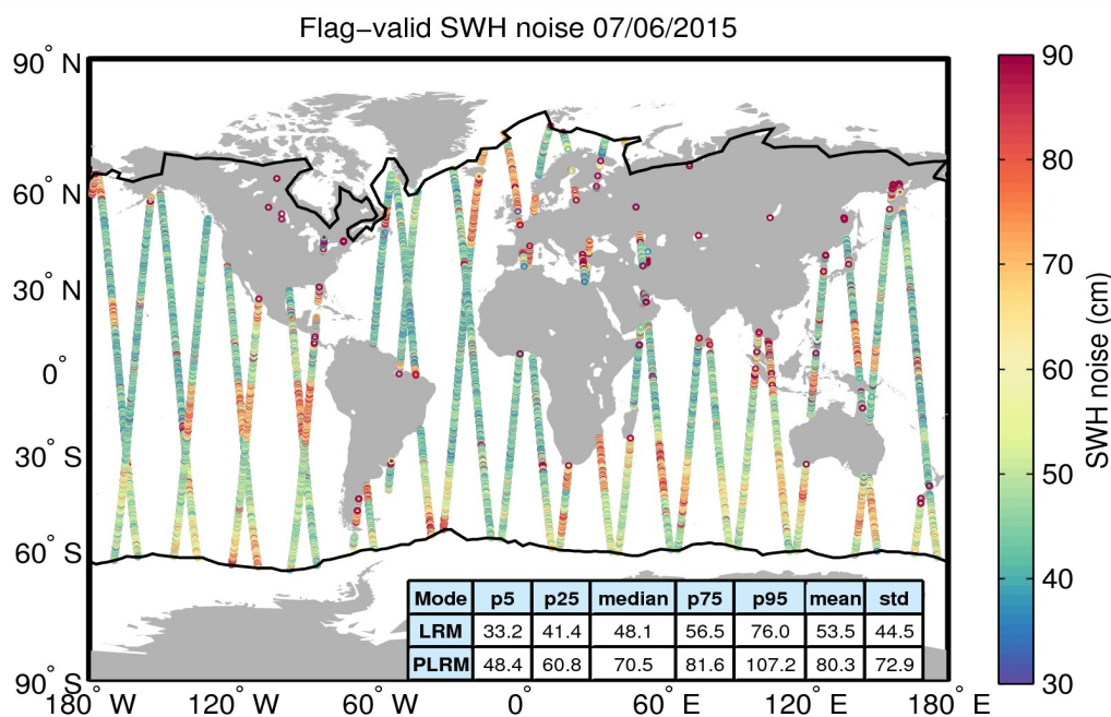
Figure 18. Geographical distribution of flag-valid 20-Hz SWH measurement noise over oceans and lakes for 07/06/2015. The statistical values shown in the table refer to the SWH noise and are calculated separately for LRM and PLRM regions. Measurements taken over polar polygons have been excluded from the computation of the statistical values. The black lines mark the outer limit of the Arctic and Antarctic polar polygons.
