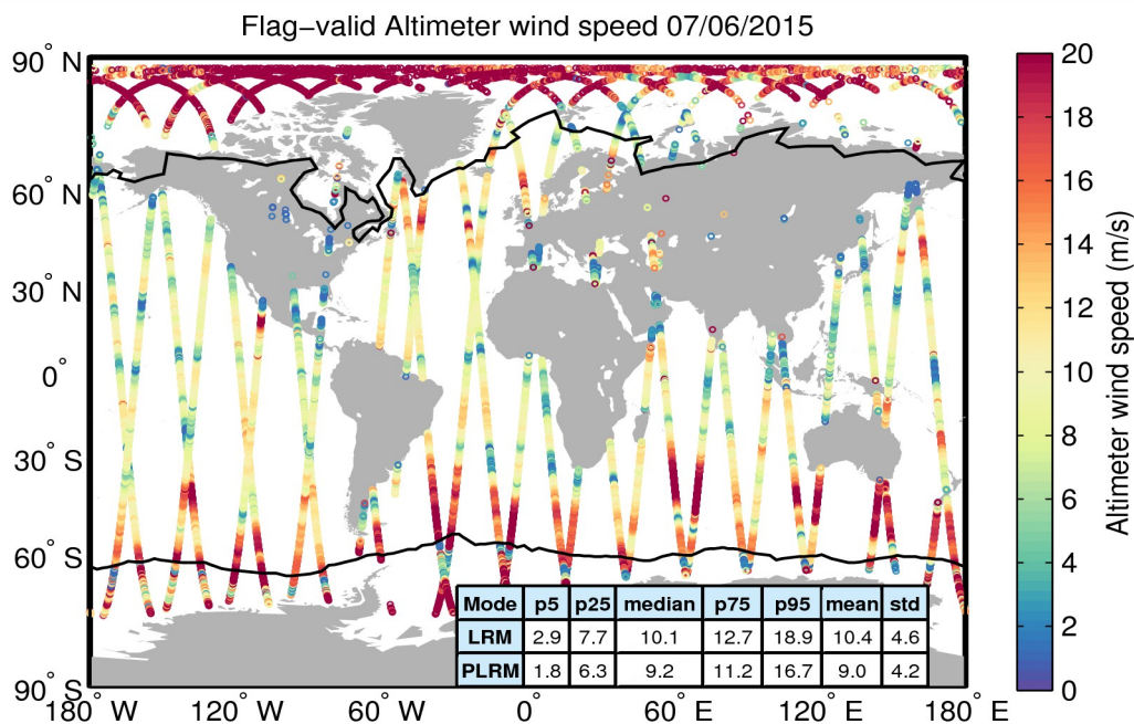
Figure 31. Geographical distribution of flag-valid wind data over oceans and lakes for 07/06/2015. The statistical values shown in the table refer to the wind in m/s and are calculated separately for LRM and PLRM regions. Measurements taken over polar polygons have been excluded from the computation of the statistical values. The black lines mark the outer limit of the Arctic and Antarctic polar polygons.
