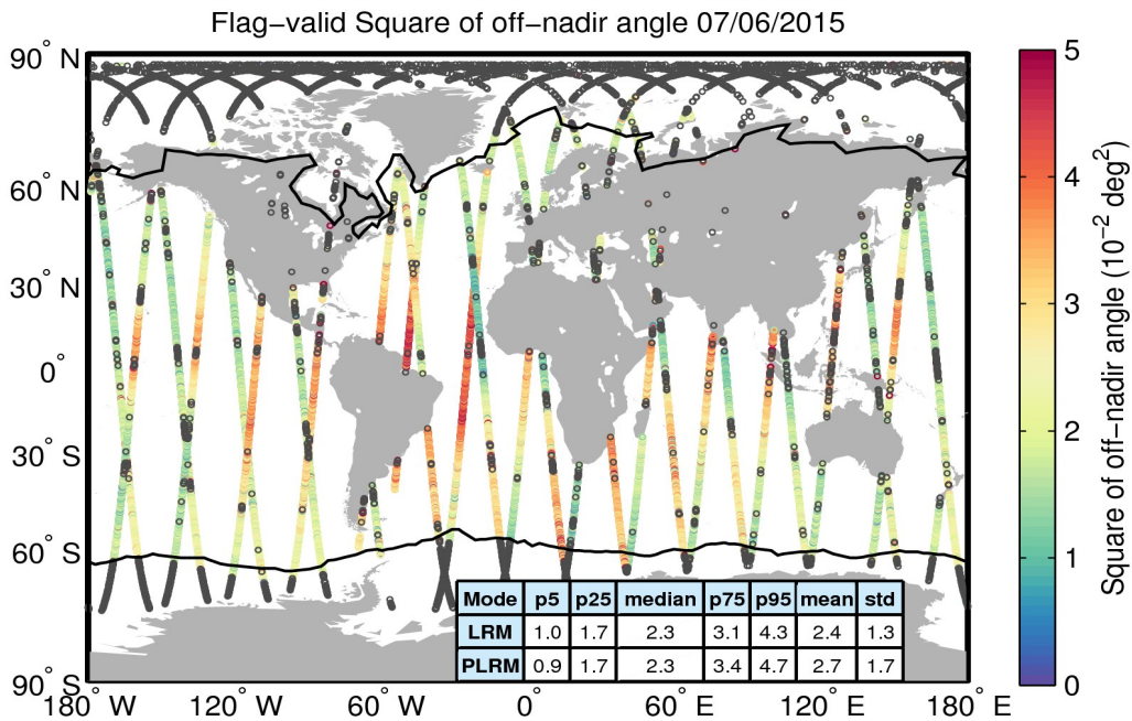
Figure 37. Geographical distribution of flag-valid mispointing data over oceans and lakes for 07/06/2015. The statistical values shown in the table refer to the mispointing in 10^{-2} \text{ deg}^2 and are calculated separately for LRM and PLRM regions. Measurements taken over polar polygons have been excluded from the computation of the statistical values. The black lines mark the outer limit of the Arctic and Antarctic polar polygons. Gray circles denote negative values.
