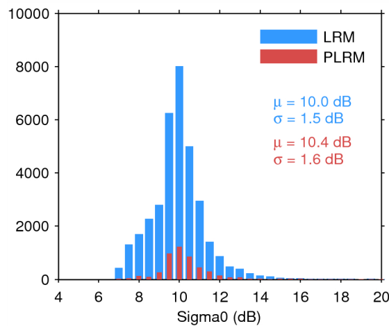
Figure 28. Histogram of science-valid sigma0 over oceans and lakes for LRM (blue) and PLRM (red) for 07/06/2015. The mean ( \mu ) and standard deviation ( \sigma ) are also shown. Note that values outside [4 20] dB are excluded from the histogram for the sake of readability but not from the computation of \mu and \sigma .
