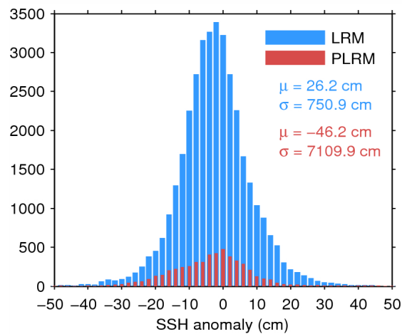
Figure 7. Histogram of flag-valid SSH anomaly over oceans and lakes for LRM (blue) and PLRM (red) for 07/06/2015. The mean ( \mu ) and standard deviation ( \sigma ) are also shown. Note that values outside [-50\ 50] cm are excluded from the histogram for the sake of readability but not from the computation of \mu and \sigma .
