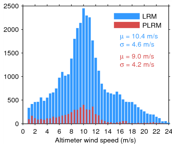
Figure 35. Histogram of science-valid wind over oceans and lakes for LRM (blue) and PLRM (red) for 07/06/2015. The mean ( \mu ) and standard deviation ( \sigma ) are also shown. Note that values larger than 24 m/s are excluded from the histogram for the sake of readability but not from the computation of \mu and \sigma .
