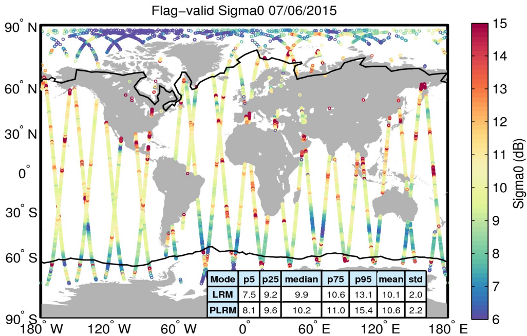
Figure 23. Geographical distribution of flag-valid sigma0 data over oceans and lakes for 07/06/2015. The statistical values shown in the table refer to the sigma0 in dB and are calculated separately for LRM and PLRM regions. Measurements taken over polar polygons have been excluded from the computation of the statistical values. The black lines mark the outer limit of the Arctic and Antarctic polar polygons.
