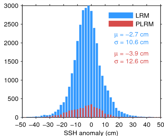
Figure 11. Histogram of science-valid SSH anomaly over oceans and lakes for LRM (blue) and PLRM (red) for 07/06/2015. The mean ( \mu ) and standard deviation ( \sigma ) are also shown. Note that values outside [-50 50] cm are excluded from the histogram for the sake of readability but not from the computation of \mu and \sigma .
