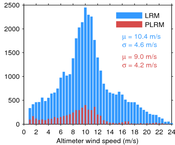
Figure 33. Histogram of flag-valid wind over oceans and lakes for LRM (blue) and PLRM (red) for 07/06/2015. The mean ( \mu ) and standard deviation ( \sigma ) are also shown. Note that values larger than 24 m/s are excluded from the histogram for the sake of readability but not from the computation of \mu and \sigma .
