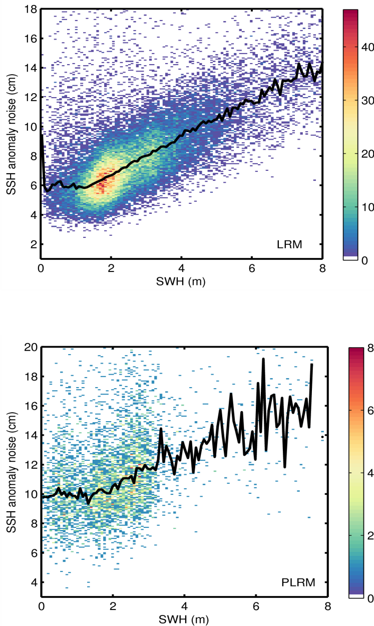
Figure 9. 2D histogram showing flag-valid SSH anomaly noise as a function of SWH for LRM (top) and PLRM (bottom) for 07/06/2015. The black line denotes the median SSH anomaly as a function of SWH.
