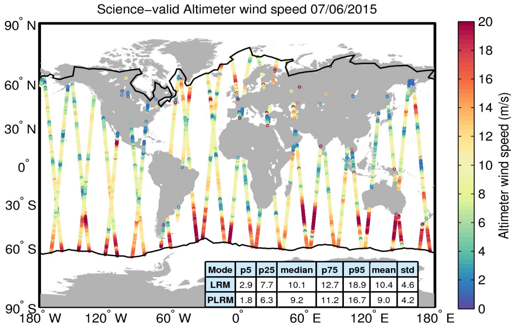
Figure 34. Geographical distribution of science-valid wind data over oceans and lakes for 07/06/2015. The statistical values shown in the table refer to the wind in m/s and are calculated separately for LRM and PLRM regions. The black lines mark the outer limit of the Arctic and Antarctic polar polygons. Gray circles denote records that have been rejected based on the editing criteria described in Table 5.
