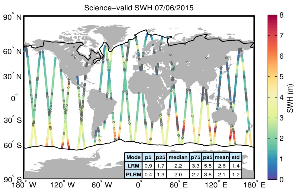
Figure 19. Geographical distribution of science-valid SWH data over oceans and lakes for 07/06/2015. The statistical values shown in the table refer to the SWH in m and are calculated separately for LRM and PLRM regions. The black lines mark the outer limit of the Arctic and Antarctic polar polygons. Gray circles denote records that have been rejected based on the editing criteria described in Table 3.
