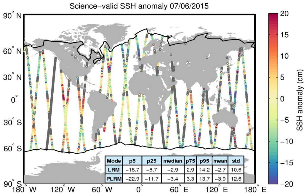
Figure 10. Geographical distribution of science-valid SSH anomaly data over oceans and lakes for 07/06/2015. The statistical values shown in the table refer to the SSH anomaly in cm and are calculated separately for LRM and PLRM regions. The black lines mark the outer limit of the Arctic and Antarctic polar polygons. Gray circles denote records that have been rejected based on the editing criteria described in Table 2.
