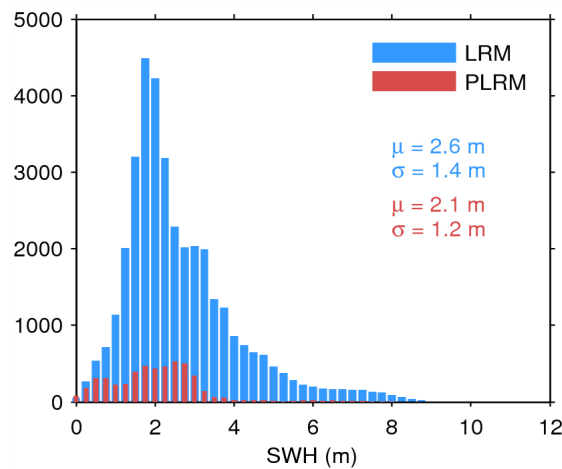
Figure 20. Histogram of science-valid SWH over oceans and lakes for LRM (blue) and PLRM (red) for 07/06/2015. The mean ( \mu ) and standard deviation ( \sigma ) are also shown. Note that values larger than 12 m are excluded from the histogram for the sake of readability but not from the computation of \mu and \sigma .
