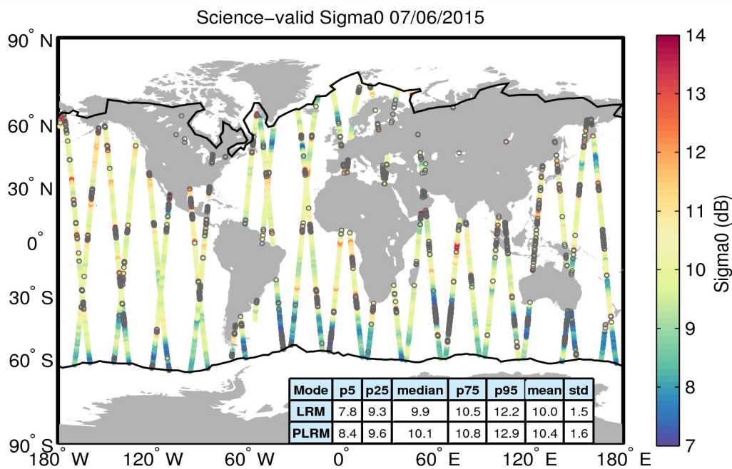
Figure 27. Geographical distribution of science-valid sigma0 data over oceans and lakes for 07/06/2015. The statistical values shown in the table refer to the sigma0 in dB and are calculated separately for LRM and PLRM regions. The black lines mark the outer limit of the Arctic and Antarctic polar polygons. Gray circles denote records that have been rejected based on the editing criteria described in Table 4.
