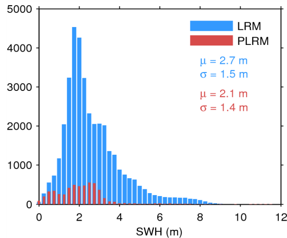
Figure 17. Histogram of flag-valid SWH over oceans and lakes for LRM (blue) and PLRM (red) for 07/06/2015. The mean ( \mu ) and standard deviation ( \sigma ) are also shown. Note that values larger than 12 m are excluded from the histogram for the sake of readability but not from the computation of \mu and \sigma .
