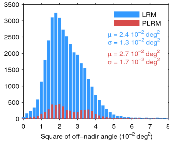
Figure 39. Histogram of flag-valid mispointing over oceans and lakes for LRM (blue) and PLRM (red) for 07/06/2015. Only positive values have been considered. The mean ( \mu ) and standard deviation ( \sigma ) are also shown. Note that values larger than 8 \cdot 10^{-2} \text{ deg}^2 are excluded from the histogram for the sake of readability but not from the computation of \mu and \sigma .
