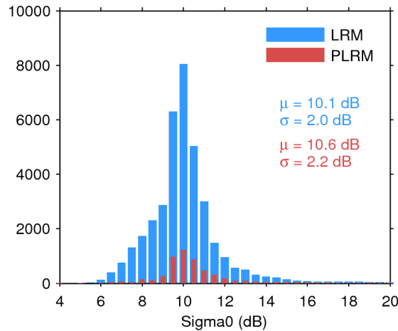
Figure 25. Histogram of flag-valid sigma0 over oceans and lakes for LRM (blue) and PLRM (red) for 07/06/2015. The mean ( \mu ) and standard deviation ( \sigma ) are also shown. Note that values outside [4 20] dB are excluded from the histogram for the sake of readability but not from the computation of \mu and \sigma .
