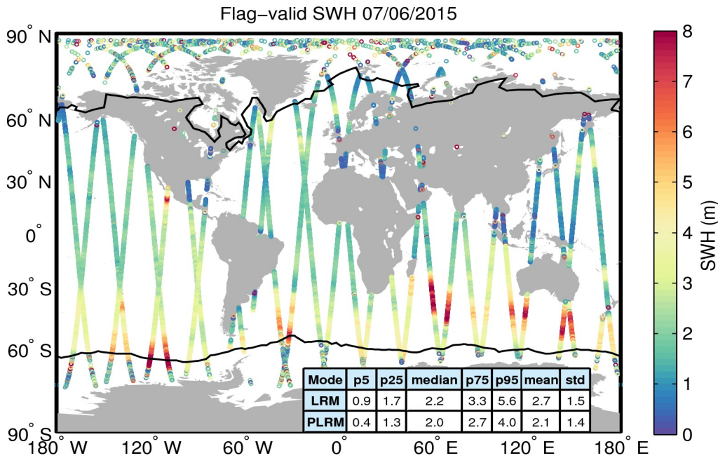
Figure 15. Geographical distribution of flag-valid SWH data over oceans and lakes for 07/06/2015. The statistical values shown in the table refer to the SWH in m and are calculated separately for LRM and PLRM regions. Measurements taken over polar polygons have been excluded from the computation of the statistical values. The black lines mark the outer limit of the Arctic and Antarctic polar polygons.
