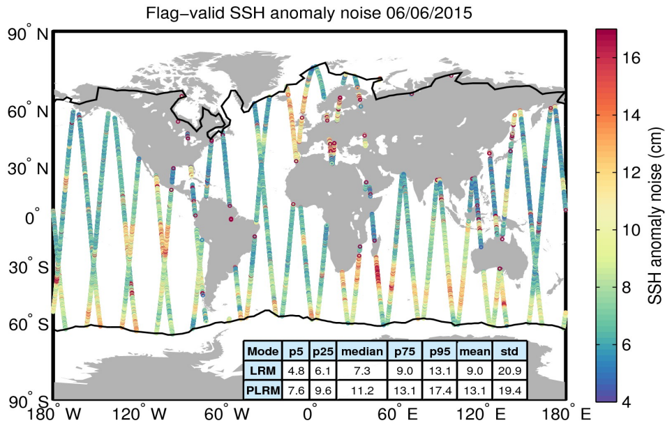
Figure 8. Geographical distribution of flag-valid 20-Hz SSH anomaly measurement noise over oceans and lakes for 06/06/2015. The statistical values shown in the table refer to the SSH anomaly noise and are calculated separately for LRM and PLRM regions. Measurements taken over polar polygons have been excluded from the computation of the statistical values. The black lines mark the outer limit of the Arctic and Antarctic polar polygons.
