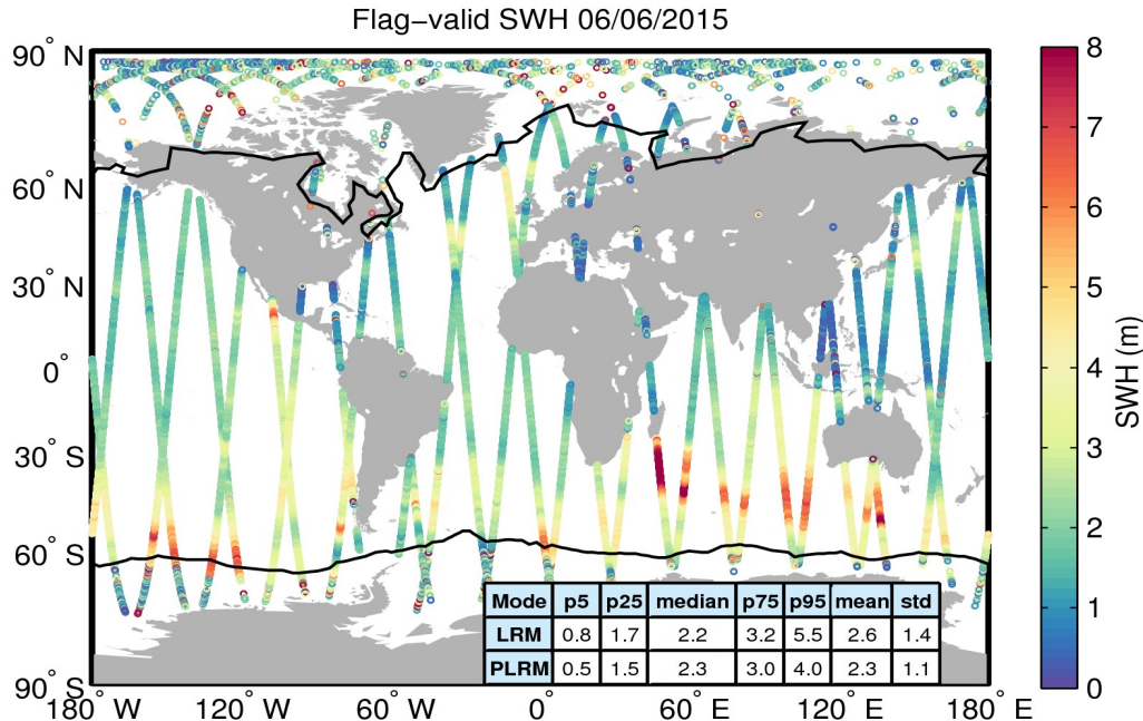
Figure 15. Geographical distribution of flag-valid SWH data over oceans and lakes for 06/06/2015. The statistical values shown in the table refer to the SWH in m and are calculated separately for LRM and PLRM regions. Measurements taken over polar polygons have been excluded from the computation of the statistical values. The black lines mark the outer limit of the Arctic and Antarctic polar polygons.
