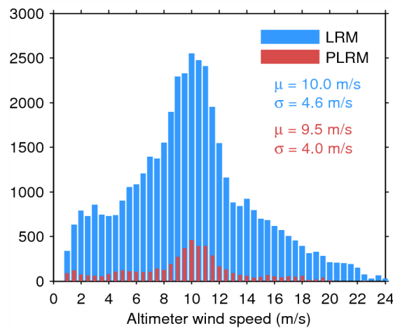
Figure 33. Histogram of flag-valid wind over oceans and lakes for LRM (blue) and PLRM (red) for 06/06/2015. The mean ( \mu ) and standard deviation ( \sigma ) are also shown. Note that values larger than 24 m/s are excluded from the histogram for the sake of readability but not from the computation of \mu and \sigma .
