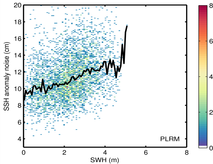
Figure 9. 2D histogram showing flag-valid SSH anomaly noise as a function of SWH for LRM (top) and PLRM (bottom) for 06/06/2015. The black line denotes the median SSH anomaly as a function of SWH.
