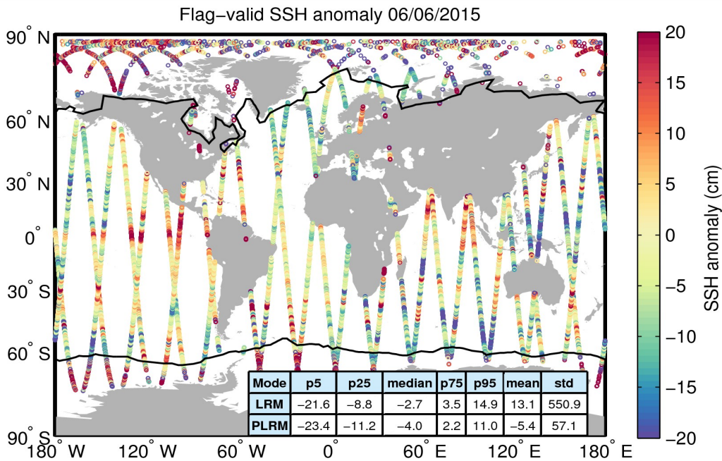
Figure 5. Geographical distribution of flag-valid 1-Hz SSH anomaly data over oceans and lakes for 06/06/2015. The statistical values shown in the table refer to the SSH anomaly in cm and are calculated separately for LRM and PLRM regions. Measurements taken over polar polygons have been excluded from the computation of the statistical values. The black lines mark the outer limit of the Arctic and Antarctic polar polygons.
