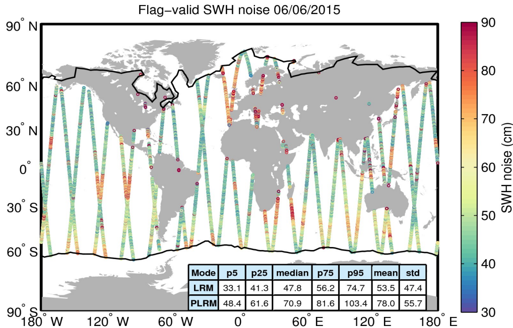
Figure 18. Geographical distribution of flag-valid 20-Hz SWH measurement noise over oceans and lakes for 06/06/2015. The statistical values shown in the table refer to the SWH noise and are calculated separately for LRM and PLRM regions. Measurements taken over polar polygons have been excluded from the computation of the statistical values. The black lines mark the outer limit of the Arctic and Antarctic polar polygons.
