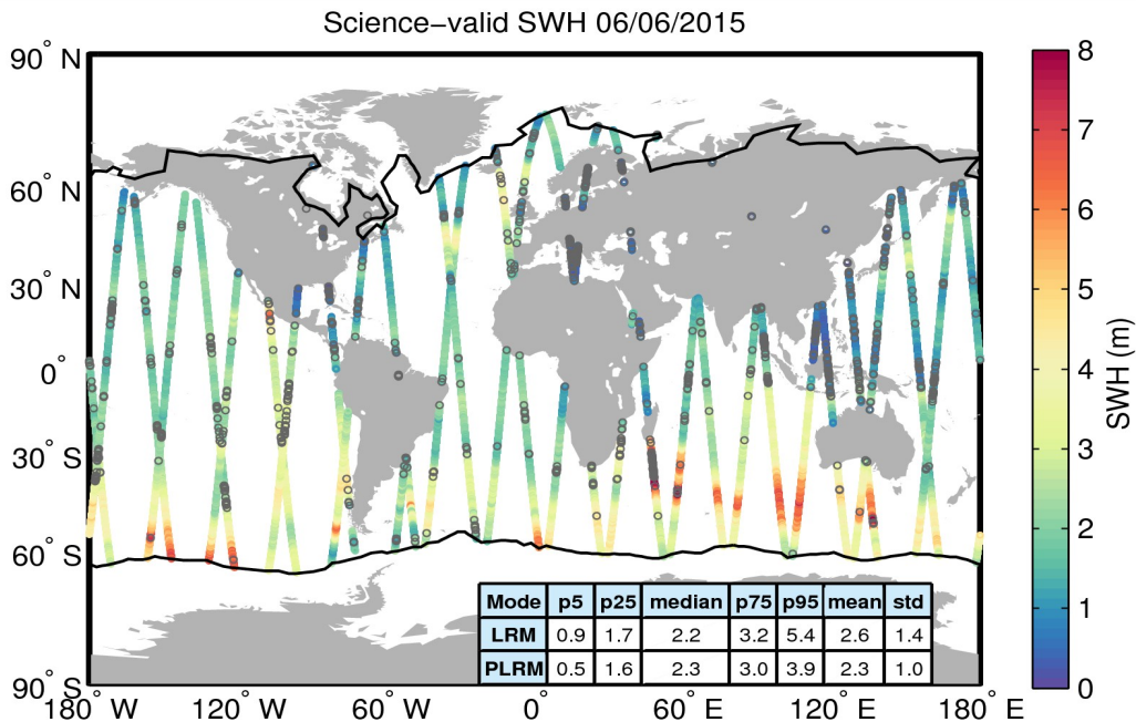
Figure 19. Geographical distribution of science-valid SWH data over oceans and lakes for 06/06/2015. The statistical values shown in the table refer to the SWH in m and are calculated separately for LRM and PLRM regions. The black lines mark the outer limit of the Arctic and Antarctic polar polygons. Gray circles denote records that have been rejected based on the editing criteria described in Table 3.
