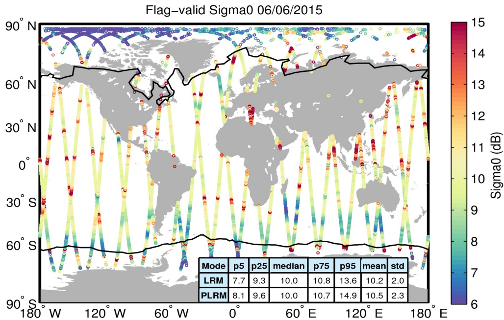
Figure 23. Geographical distribution of flag-valid sigma0 data over oceans and lakes for 06/06/2015. The statistical values shown in the table refer to the sigma0 in dB and are calculated separately for LRM and PLRM regions. Measurements taken over polar polygons have been excluded from the computation of the statistical values. The black lines mark the outer limit of the Arctic and Antarctic polar polygons.
