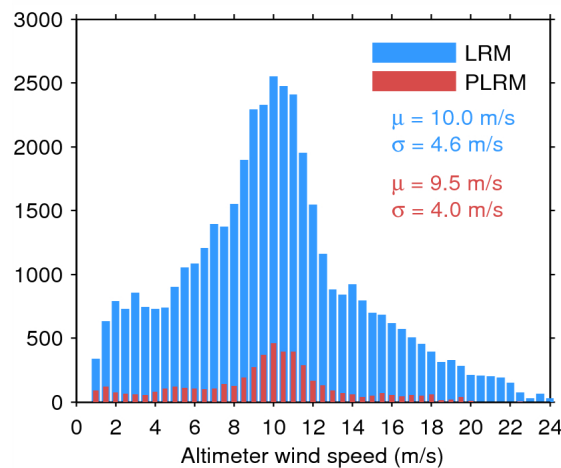
Figure 35. Histogram of science-valid wind over oceans and lakes for LRM (blue) and PLRM (red) for 06/06/2015. The mean ( \mu ) and standard deviation ( \sigma ) are also shown. Note that values larger than 24 m/s are excluded from the histogram for the sake of readability but not from the computation of \mu and \sigma .
