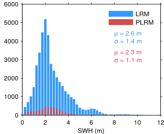
Figure 17. Histogram of flag-valid SWH over oceans and lakes for LRM (blue) and PLRM (red) for 06/06/2015. The mean ( \mu ) and standard deviation ( \sigma ) are also shown. Note that values larger than 12 m are excluded from the histogram for the sake of readability but not from the computation of \mu and \sigma .
