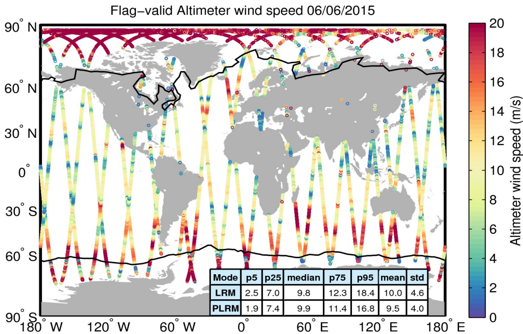
Figure 31. Geographical distribution of flag-valid wind data over oceans and lakes for 06/06/2015. The statistical values shown in the table refer to the wind in m/s and are calculated separately for LRM and PLRM regions. Measurements taken over polar polygons have been excluded from the computation of the statistical values. The black lines mark the outer limit of the Arctic and Antarctic polar polygons.
