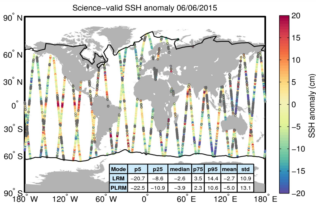
Figure 10. Geographical distribution of science-valid SSH anomaly data over oceans and lakes for 06/06/2015. The statistical values shown in the table refer to the SSH anomaly in cm and are calculated separately for LRM and PLRM regions. The black lines mark the outer limit of the Arctic and Antarctic polar polygons. Gray circles denote records that have been rejected based on the editing criteria described in Table 2.
