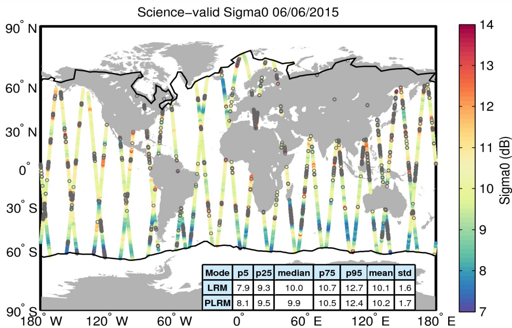
Figure 27. Geographical distribution of science-valid sigma0 data over oceans and lakes for 06/06/2015. The statistical values shown in the table refer to the sigma0 in dB and are calculated separately for LRM and PLRM regions. The black lines mark the outer limit of the Arctic and Antarctic polar polygons. Gray circles denote records that have been rejected based on the editing criteria described in Table 4.
