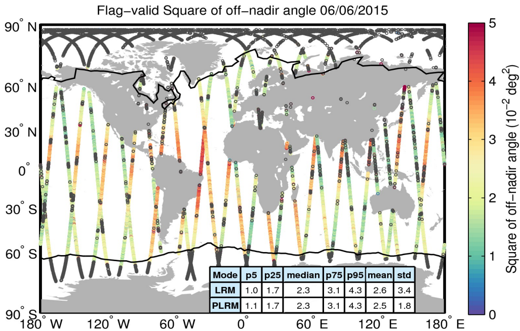
Figure 37. Geographical distribution of flag-valid mispointing data over oceans and lakes for 06/06/2015. The statistical values shown in the table refer to the mispointing in 10^{-2} deg 2 and are calculated separately for LRM and PLRM regions. Measurements taken over polar polygons have been excluded from the computation of the statistical values. The black lines mark the outer limit of the Arctic and Antarctic polar polygons. Gray circles denote negative values.
