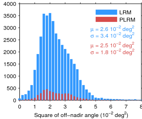
Figure 39. Histogram of flag-valid mispointing over oceans and lakes for LRM (blue) and PLRM (red) for 06/06/2015. Only positive values have been considered. The mean ( \mu ) and standard deviation ( \sigma ) are also shown. Note that values larger than 8 \cdot 10^{-2} \text{ deg}^2 are excluded from the histogram for the sake of readability but not from the computation of \mu and \sigma .
