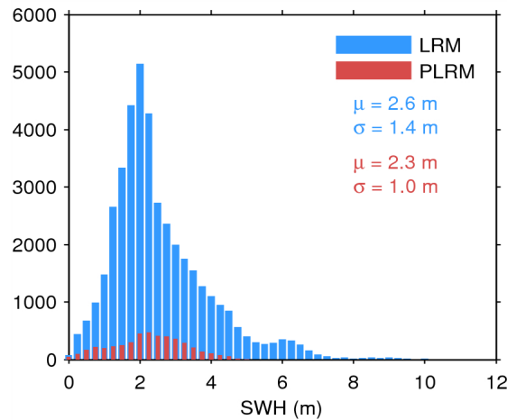
Figure 20. Histogram of science-valid SWH over oceans and lakes for LRM (blue) and PLRM (red) for 06/06/2015. The mean ( \mu ) and standard deviation ( \sigma ) are also shown. Note that values larger than 12 m are excluded from the histogram for the sake of readability but not from the computation of \mu and \sigma .
