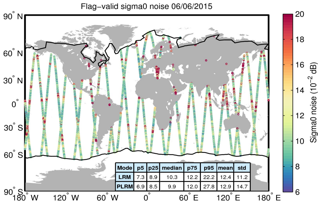
Figure 26. Geographical distribution of flag-valid 20-Hz sigma0 measurement noise over oceans and lakes for 06/06/2015. The statistical values shown in the table refer to the sigma0 noise and are calculated separately for LRM and PLRM regions. Measurements taken over polar polygons have been excluded from the computation of the statistical values. The black lines mark the outer limit of the Arctic and Antarctic polar polygons.
