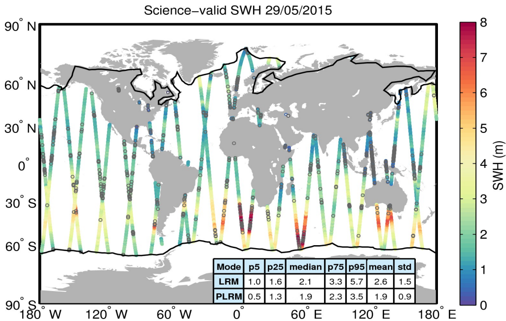
Figure 19. Geographical distribution of science-valid SWH data over oceans and lakes for 29/05/2015. The statistical values shown in the table refer to the SWH in m and are calculated separately for LRM and PLRM regions. The black lines mark the outer limit of the Arctic and Antarctic polar polygons. Gray circles denote records that have been rejected based on the editing criteria described in Table 3.
