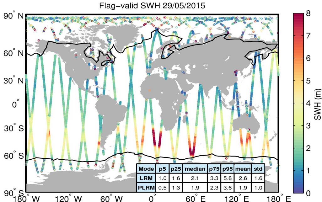
Figure 15. Geographical distribution of flag-valid SWH data over oceans and lakes for 29/05/2015. The statistical values shown in the table refer to the SWH in m and are calculated separately for LRM and PLRM regions. Measurements taken over polar polygons have been excluded from the computation of the statistical values. The black lines mark the outer limit of the Arctic and Antarctic polar polygons.
