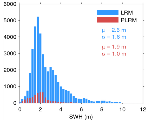
Figure 17. Histogram of flag-valid SWH over oceans and lakes for LRM (blue) and PLRM (red) for 29/05/2015. The mean ( \mu ) and standard deviation ( \sigma ) are also shown. Note that values larger than 12 m are excluded from the histogram for the sake of readability but not from the computation of \mu and \sigma .
