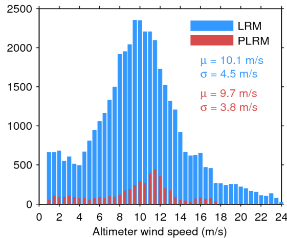
Figure 33. Histogram of flag-valid wind over oceans and lakes for LRM (blue) and PLRM (red) for 29/05/2015. The mean ( \mu ) and standard deviation ( \sigma ) are also shown. Note that values larger than 24 m/s are excluded from the histogram for the sake of readability but not from the computation of \mu and \sigma .
