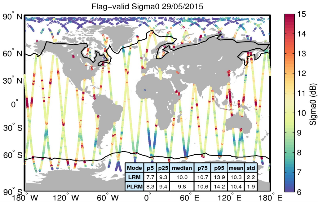
Figure 23. Geographical distribution of flag-valid sigma0 data over oceans and lakes for 29/05/2015. The statistical values shown in the table refer to the sigma0 in dB and are calculated separately for LRM and PLRM regions. Measurements taken over polar polygons have been excluded from the computation of the statistical values. The black lines mark the outer limit of the Arctic and Antarctic polar polygons.
