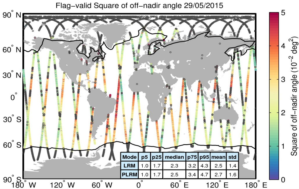
Figure 37. Geographical distribution of flag-valid mispointing data over oceans and lakes for 29/05/2015. The statistical values shown in the table refer to the mispointing in 10^{-2} \text{ deg}^2 and are calculated separately for LRM and PLRM regions. Measurements taken over polar polygons have been excluded from the computation of the statistical values. The black lines mark the outer limit of the Arctic and Antarctic polar polygons. Gray circles denote negative values.
