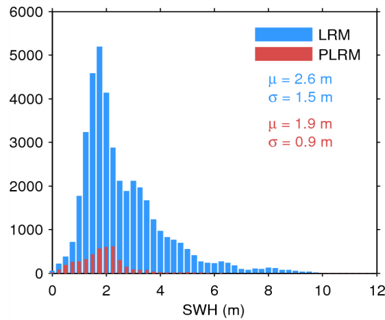
Figure 20. Histogram of science-valid SWH over oceans and lakes for LRM (blue) and PLRM (red) for 29/05/2015. The mean ( \mu ) and standard deviation ( \sigma ) are also shown. Note that values larger than 12 m are excluded from the histogram for the sake of readability but not from the computation of \mu and \sigma .
