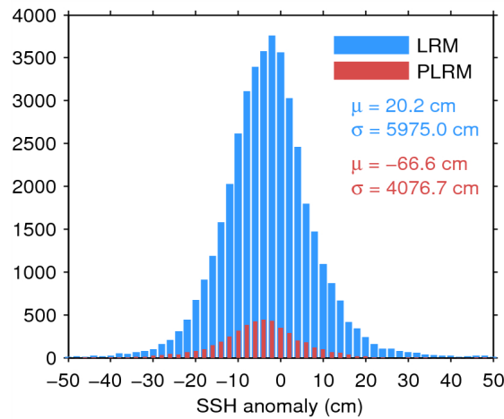
Figure 7. Histogram of flag-valid SSH anomaly over oceans and lakes for LRM (blue) and PLRM (red) for 29/05/2015. The mean ( \mu ) and standard deviation ( \sigma ) are also shown. Note that values outside [-50 \ 50] cm are excluded from the histogram for the sake of readability but not from the computation of \mu and \sigma .
