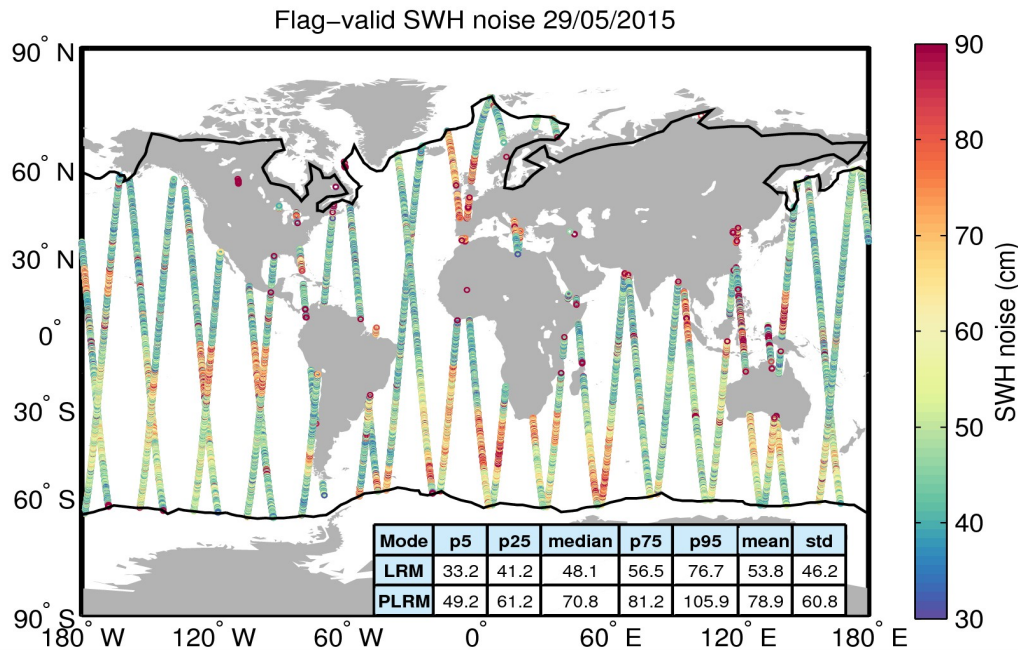
Figure 18. Geographical distribution of flag-valid 20-Hz SWH measurement noise over oceans and lakes for 29/05/2015. The statistical values shown in the table refer to the SWH noise and are calculated separately for LRM and PLRM regions. Measurements taken over polar polygons have been excluded from the computation of the statistical values. The black lines mark the outer limit of the Arctic and Antarctic polar polygons.
