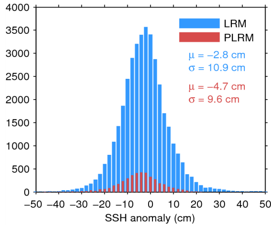
Figure 11. Histogram of science-valid SSH anomaly over oceans and lakes for LRM (blue) and PLRM (red) for 29/05/2015. The mean ( \mu ) and standard deviation ( \sigma ) are also shown. Note that values outside [-50 50] cm are excluded from the histogram for the sake of readability but not from the computation of \mu and \sigma .
