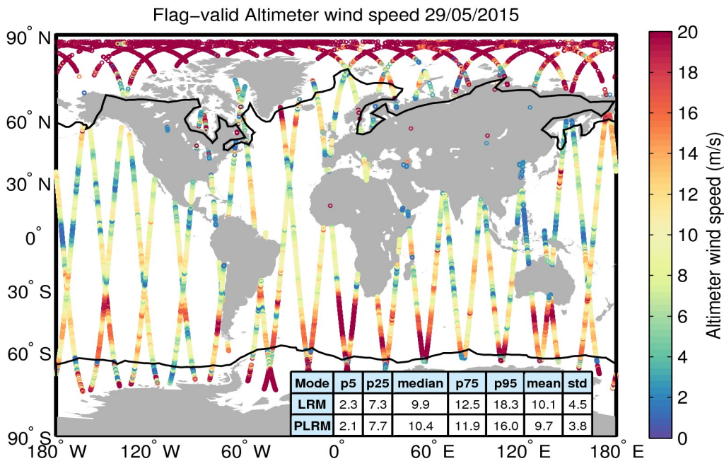
Figure 31. Geographical distribution of flag-valid wind data over oceans and lakes for 29/05/2015. The statistical values shown in the table refer to the wind in m/s and are calculated separately for LRM and PLRM regions. Measurements taken over polar polygons have been excluded from the computation of the statistical values. The black lines mark the outer limit of the Arctic and Antarctic polar polygons.
