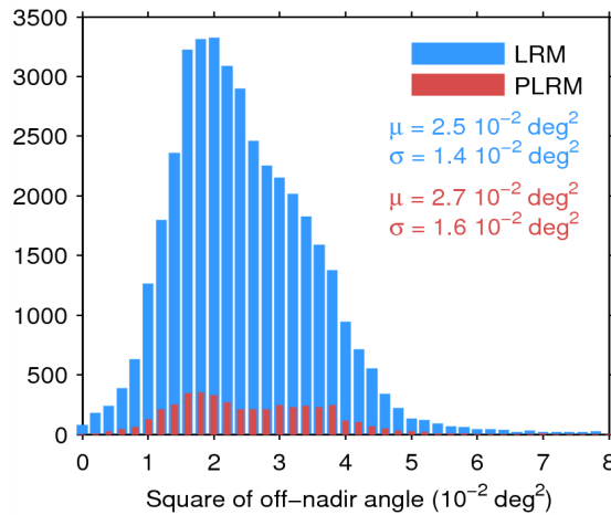
Figure 39. Histogram of flag-valid mispointing over oceans and lakes for LRM (blue) and PLRM (red) for 29/05/2015. Only positive values have been considered. The mean ( \mu ) and standard deviation ( \sigma ) are also shown. Note that values larger than 8 \cdot 10^{-2} \text{ deg}^2 are excluded from the histogram for the sake of readability but not from the computation of \mu and \sigma .
