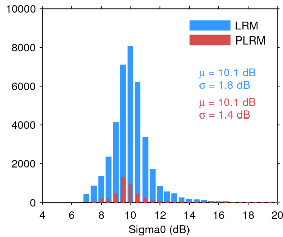
Figure 28. Histogram of science-valid sigma0 over oceans and lakes for LRM (blue) and PLRM (red) for 29/05/2015. The mean ( \mu ) and standard deviation ( \sigma ) are also shown. Note that values outside [4 20] dB are excluded from the histogram for the sake of readability but not from the computation of \mu and \sigma .
