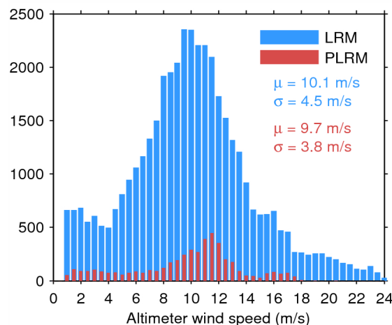
Figure 35. Histogram of science-valid wind over oceans and lakes for LRM (blue) and PLRM (red) for 29/05/2015. The mean ( \mu ) and standard deviation ( \sigma ) are also shown. Note that values larger than 24 m/s are excluded from the histogram for the sake of readability but not from the computation of \mu and \sigma .
