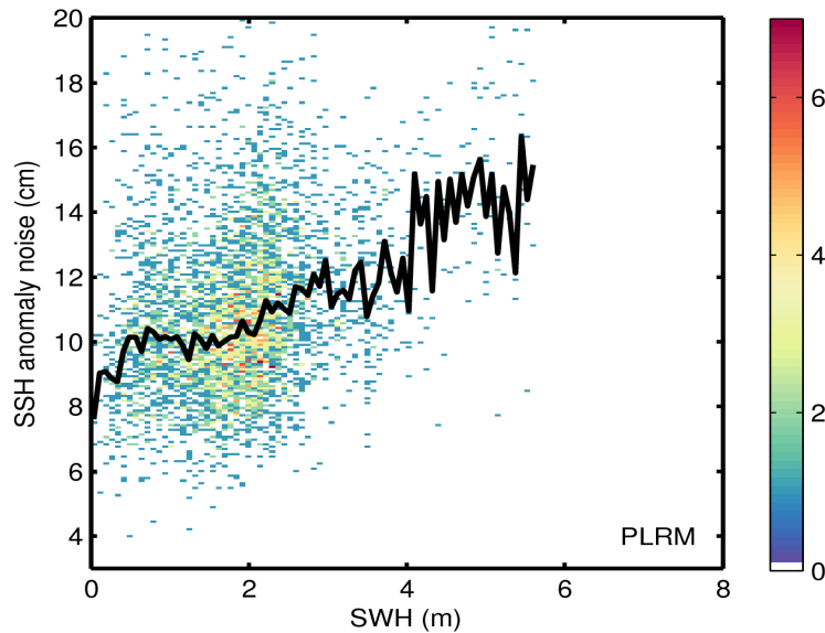
Figure 9. 2D histogram showing flag-valid SSH anomaly noise as a function of SWH for LRM (top) and PLRM (bottom) for 29/05/2015. The black line denotes the median SSH anomaly as a function of SWH.
