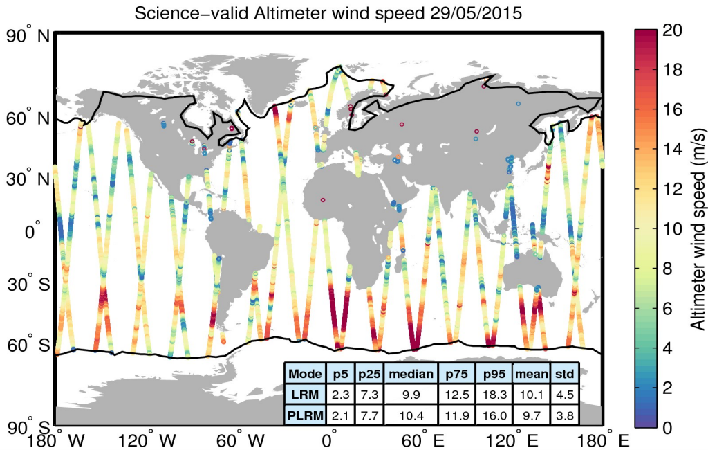
Figure 34. Geographical distribution of science-valid wind data over oceans and lakes for 29/05/2015. The statistical values shown in the table refer to the wind in m/s and are calculated separately for LRM and PLRM regions. The black lines mark the outer limit of the Arctic and Antarctic polar polygons. Gray circles denote records that have been rejected based on the editing criteria described in Table 5.
