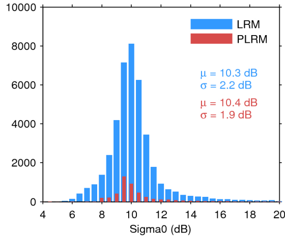
Figure 25. Histogram of flag-valid sigma0 over oceans and lakes for LRM (blue) and PLRM (red) for 29/05/2015. The mean ( \mu ) and standard deviation ( \sigma ) are also shown. Note that values outside [4 20] dB are excluded from the histogram for the sake of readability but not from the computation of \mu and \sigma .
