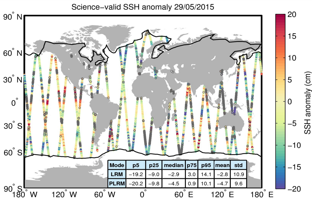
Figure 10. Geographical distribution of science-valid SSH anomaly data over oceans and lakes for 29/05/2015. The statistical values shown in the table refer to the SSH anomaly in cm and are calculated separately for LRM and PLRM regions. The black lines mark the outer limit of the Arctic and Antarctic polar polygons. Gray circles denote records that have been rejected based on the editing criteria described in Table 2.
