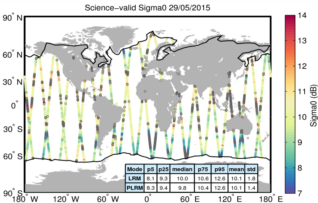
Figure 27. Geographical distribution of science-valid sigma0 data over oceans and lakes for 29/05/2015. The statistical values shown in the table refer to the sigma0 in dB and are calculated separately for LRM and PLRM regions. The black lines mark the outer limit of the Arctic and Antarctic polar polygons. Gray circles denote records that have been rejected based on the editing criteria described in Table 4.
