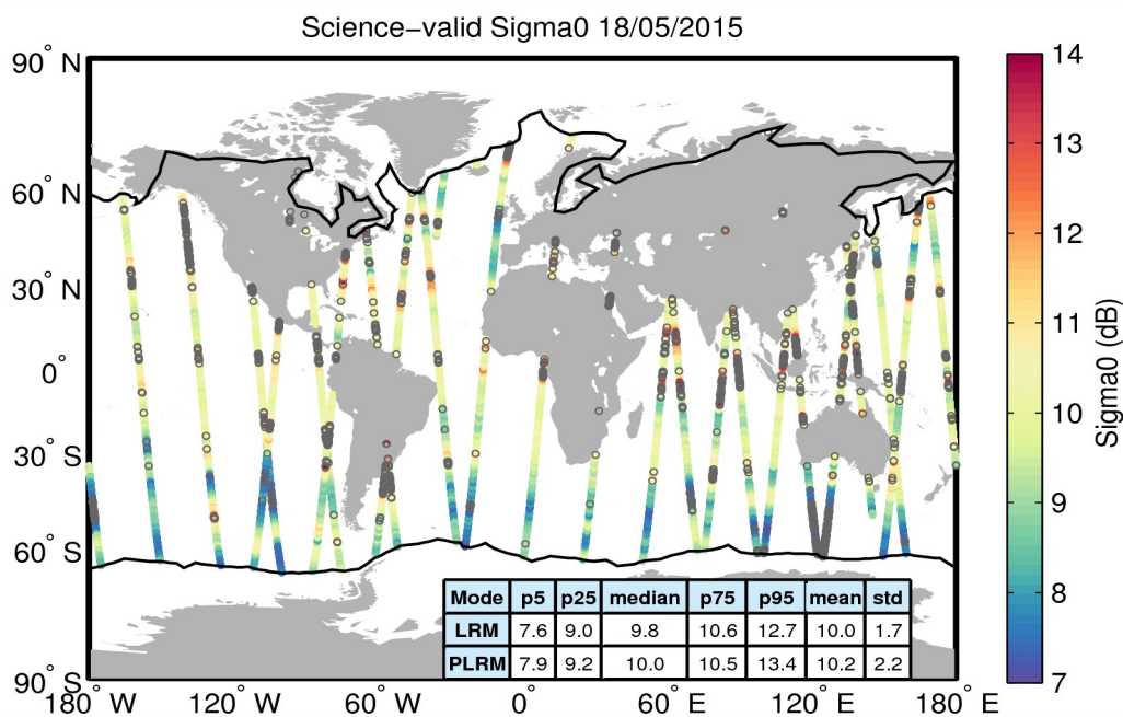
Figure 27. Geographical distribution of science-valid sigma0 data over oceans and lakes for 18/05/2015. The statistical values shown in the table refer to the sigma0 in dB and are calculated separately for LRM and PLRM regions. The black lines mark the outer limit of the Arctic and Antarctic polar polygons. Gray circles denote records that have been rejected based on the editing criteria described in Table 4.
