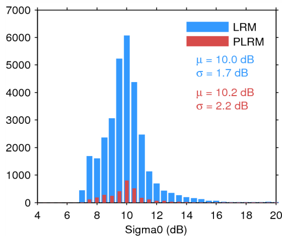
Figure 28. Histogram of science-valid sigma0 over oceans and lakes for LRM (blue) and PLRM (red) for 18/05/2015. The mean ( \mu ) and standard deviation ( \sigma ) are also shown. Note that values outside [4 20] dB are excluded from the histogram for the sake of readability but not from the computation of \mu and \sigma .
