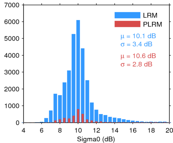
Figure 25. Histogram of flag-valid sigma0 over oceans and lakes for LRM (blue) and PLRM (red) for 18/05/2015. The mean ( \mu ) and standard deviation ( \sigma ) are also shown. Note that values outside [4 20] dB are excluded from the histogram for the sake of readability but not from the computation of \mu and \sigma .
