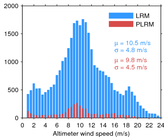
Figure 35. Histogram of science-valid wind over oceans and lakes for LRM (blue) and PLRM (red) for 18/05/2015. The mean ( \mu ) and standard deviation ( \sigma ) are also shown. Note that values larger than 24 m/s are excluded from the histogram for the sake of readability but not from the computation of \mu and \sigma .
