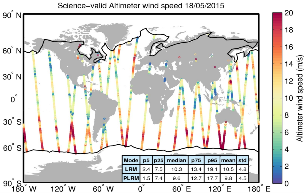
Figure 34. Geographical distribution of science-valid wind data over oceans and lakes for 18/05/2015. The statistical values shown in the table refer to the wind in m/s and are calculated separately for LRM and PLRM regions. The black lines mark the outer limit of the Arctic and Antarctic polar polygons. Gray circles denote records that have been rejected based on the editing criteria described in Table 5.
