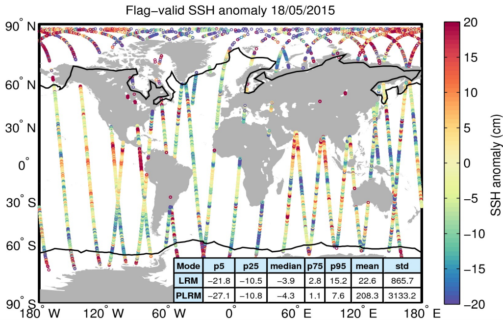
Figure 5. Geographical distribution of flag-valid 1-Hz SSH anomaly data over oceans and lakes for 18/05/2015. The statistical values shown in the table refer to the SSH anomaly in cm and are calculated separately for LRM and PLRM regions. Measurements taken over polar polygons have been excluded from the computation of the statistical values. The black lines mark the outer limit of the Arctic and Antarctic polar polygons.
