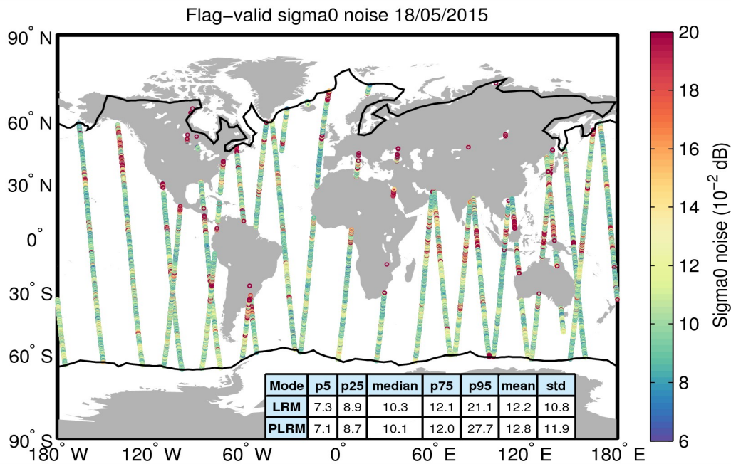
Figure 26. Geographical distribution of flag-valid 20-Hz sigma0 measurement noise over oceans and lakes for 18/05/2015. The statistical values shown in the table refer to the sigma0 noise and are calculated separately for LRM and PLRM regions. Measurements taken over polar polygons have been excluded from the computation of the statistical values. The black lines mark the outer limit of the Arctic and Antarctic polar polygons.
