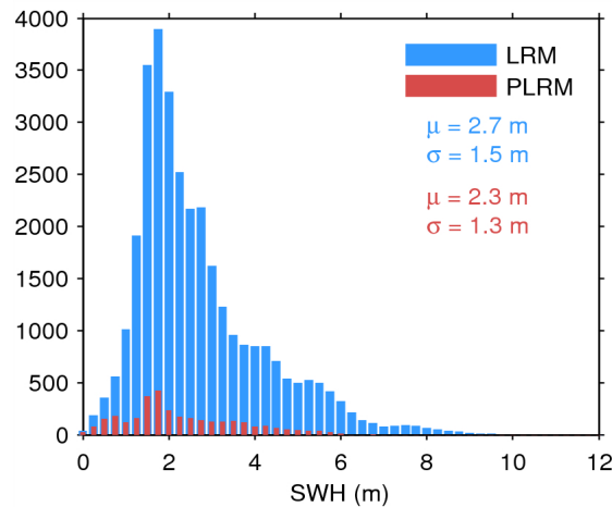
Figure 20. Histogram of science-valid SWH over oceans and lakes for LRM (blue) and PLRM (red) for 18/05/2015. The mean ( \mu ) and standard deviation ( \sigma ) are also shown. Note that values larger than 12 m are excluded from the histogram for the sake of readability but not from the computation of \mu and \sigma .
