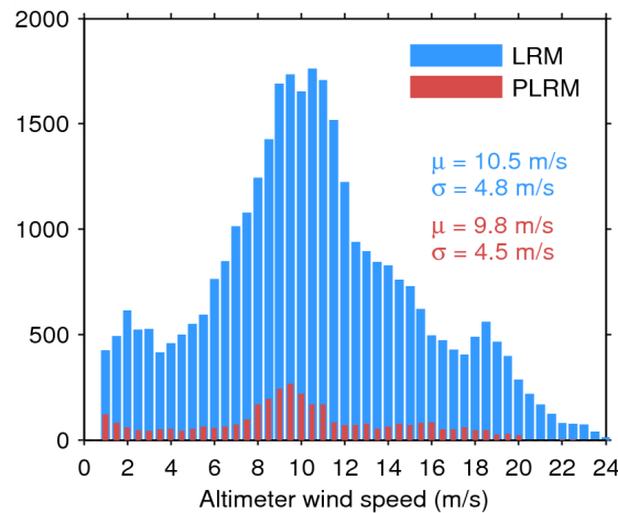
Figure 33. Histogram of flag-valid wind over oceans and lakes for LRM (blue) and PLRM (red) for 18/05/2015. The mean ( \mu ) and standard deviation ( \sigma ) are also shown. Note that values larger than 24 m/s are excluded from the histogram for the sake of readability but not from the computation of \mu and \sigma .
