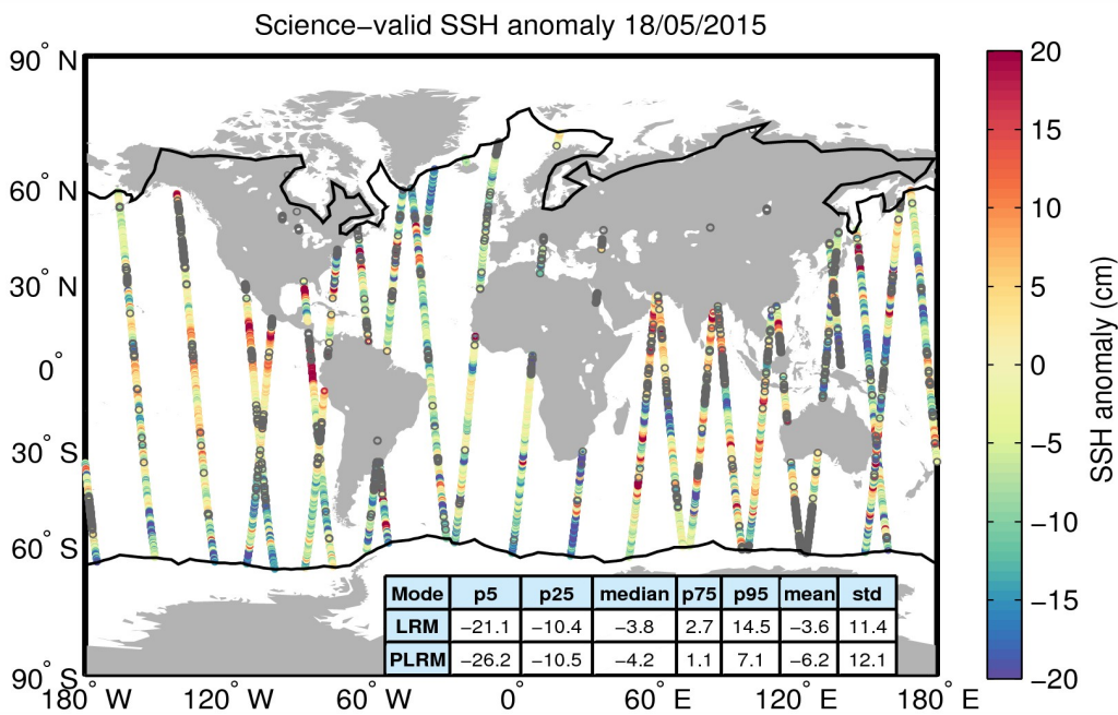
Figure 10. Geographical distribution of science-valid SSH anomaly data over oceans and lakes for 18/05/2015. The statistical values shown in the table refer to the SSH anomaly in cm and are calculated separately for LRM and PLRM regions. The black lines mark the outer limit of the Arctic and Antarctic polar polygons. Gray circles denote records that have been rejected based on the editing criteria described in Table 2.
