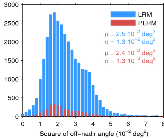
Figure 39. Histogram of flag-valid mispointing over oceans and lakes for LRM (blue) and PLRM (red) for 18/05/2015. Only positive values have been considered. The mean ( \mu ) and standard deviation ( \sigma ) are also shown. Note that values larger than 8 \cdot 10^{-2} \text{ deg}^2 are excluded from the histogram for the sake of readability but not from the computation of \mu and \sigma .
