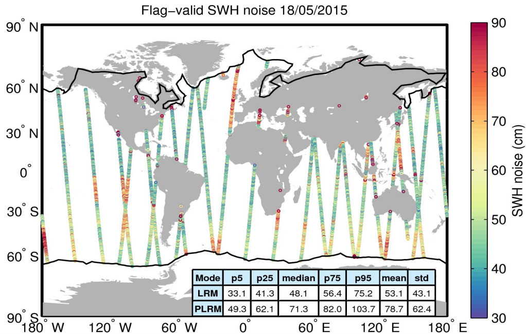
Figure 18. Geographical distribution of flag-valid 20-Hz SWH measurement noise over oceans and lakes for 18/05/2015. The statistical values shown in the table refer to the SWH noise and are calculated separately for LRM and PLRM regions. Measurements taken over polar polygons have been excluded from the computation of the statistical values. The black lines mark the outer limit of the Arctic and Antarctic polar polygons.
