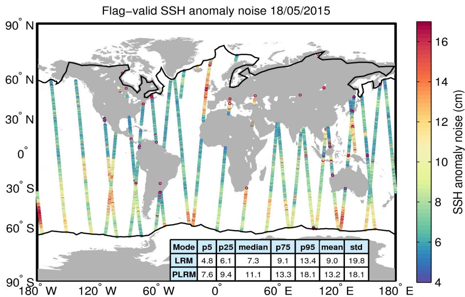
Figure 8. Geographical distribution of flag-valid 20-Hz SSH anomaly measurement noise over oceans and lakes for 18/05/2015. The statistical values shown in the table refer to the SSH anomaly noise and are calculated separately for LRM and PLRM regions. Measurements taken over polar polygons have been excluded from the computation of the statistical values. The black lines mark the outer limit of the Arctic and Antarctic polar polygons.
