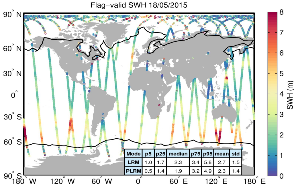
Figure 15. Geographical distribution of flag-valid SWH data over oceans and lakes for 18/05/2015. The statistical values shown in the table refer to the SWH in m and are calculated separately for LRM and PLRM regions. Measurements taken over polar polygons have been excluded from the computation of the statistical values. The black lines mark the outer limit of the Arctic and Antarctic polar polygons.
