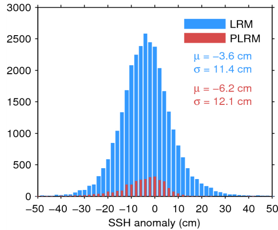
Figure 11. Histogram of science-valid SSH anomaly over oceans and lakes for LRM (blue) and PLRM (red) for 18/05/2015. The mean ( \mu ) and standard deviation ( \sigma ) are also shown. Note that values outside [-50 50] cm are excluded from the histogram for the sake of readability but not from the computation of \mu and \sigma .
