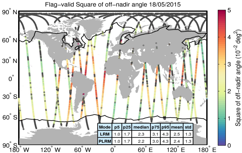
Figure 37. Geographical distribution of flag-valid mispointing data over oceans and lakes for 18/05/2015. The statistical values shown in the table refer to the mispointing in 10^{-2} \text{ deg}^2 and are calculated separately for LRM and PLRM regions. Measurements taken over polar polygons have been excluded from the computation of the statistical values. The black lines mark the outer limit of the Arctic and Antarctic polar polygons. Gray circles denote negative values.
