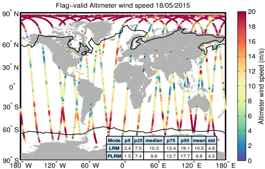
Figure 31. Geographical distribution of flag-valid wind data over oceans and lakes for 18/05/2015. The statistical values shown in the table refer to the wind in m/s and are calculated separately for LRM and PLRM regions. Measurements taken over polar polygons have been excluded from the computation of the statistical values. The black lines mark the outer limit of the Arctic and Antarctic polar polygons.
