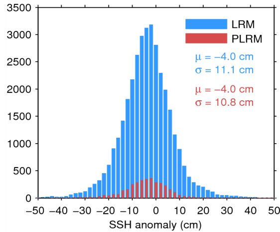
Figure 11. Histogram of science-valid SSH anomaly over oceans and lakes for LRM (blue) and PLRM (red) for 14/05/2015. The mean ( \mu ) and standard deviation ( \sigma ) are also shown. Note that values outside [-50 50] cm are excluded from the histogram for the sake of readability but not from the computation of \mu and \sigma .
