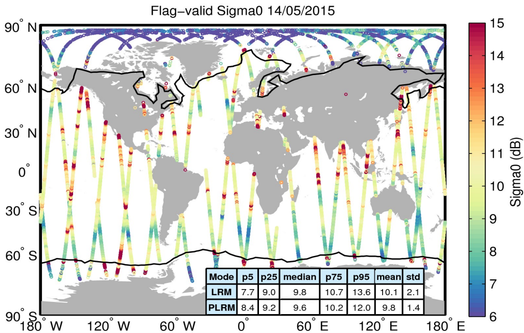
Figure 23. Geographical distribution of flag-valid sigma0 data over oceans and lakes for 14/05/2015. The statistical values shown in the table refer to the sigma0 in dB and are calculated separately for LRM and PLRM regions. Measurements taken over polar polygons have been excluded from the computation of the statistical values. The black lines mark the outer limit of the Arctic and Antarctic polar polygons.
