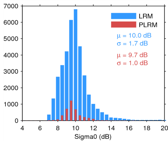
Figure 28. Histogram of science-valid sigma0 over oceans and lakes for LRM (blue) and PLRM (red) for 14/05/2015. The mean ( \mu ) and standard deviation ( \sigma ) are also shown. Note that values outside [4 20] dB are excluded from the histogram for the sake of readability but not from the computation of \mu and \sigma .
