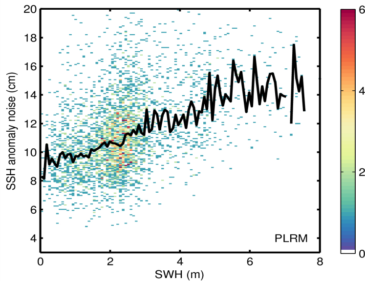
Figure 9. 2D histogram showing flag-valid SSH anomaly noise as a function of SWH for LRM (top) and PLRM (bottom) for 14/05/2015. The black line denotes the median SSH anomaly as a function of SWH.
