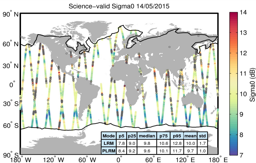
Figure 27. Geographical distribution of science-valid sigma0 data over oceans and lakes for 14/05/2015. The statistical values shown in the table refer to the sigma0 in dB and are calculated separately for LRM and PLRM regions. The black lines mark the outer limit of the Arctic and Antarctic polar polygons. Gray circles denote records that have been rejected based on the editing criteria described in Table 4.
