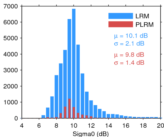
Figure 25. Histogram of flag-valid sigma0 over oceans and lakes for LRM (blue) and PLRM (red) for 14/05/2015. The mean ( \mu ) and standard deviation ( \sigma ) are also shown. Note that values outside [4 20] dB are excluded from the histogram for the sake of readability but not from the computation of \mu and \sigma .
