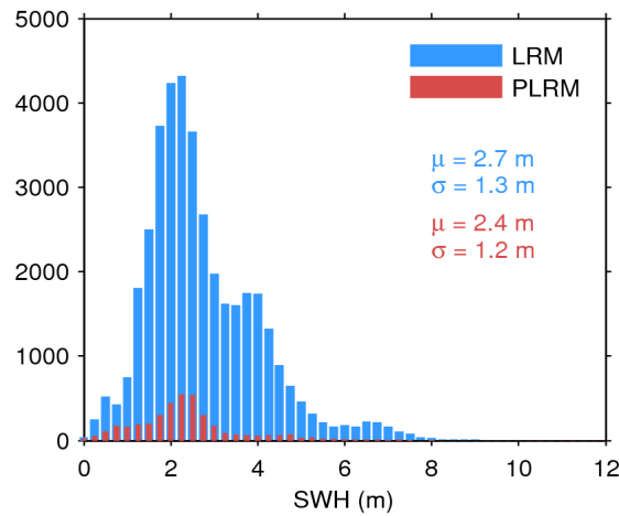
Figure 20. Histogram of science-valid SWH over oceans and lakes for LRM (blue) and PLRM (red) for 14/05/2015. The mean ( \mu ) and standard deviation ( \sigma ) are also shown. Note that values larger than 12 m are excluded from the histogram for the sake of readability but not from the computation of \mu and \sigma .
