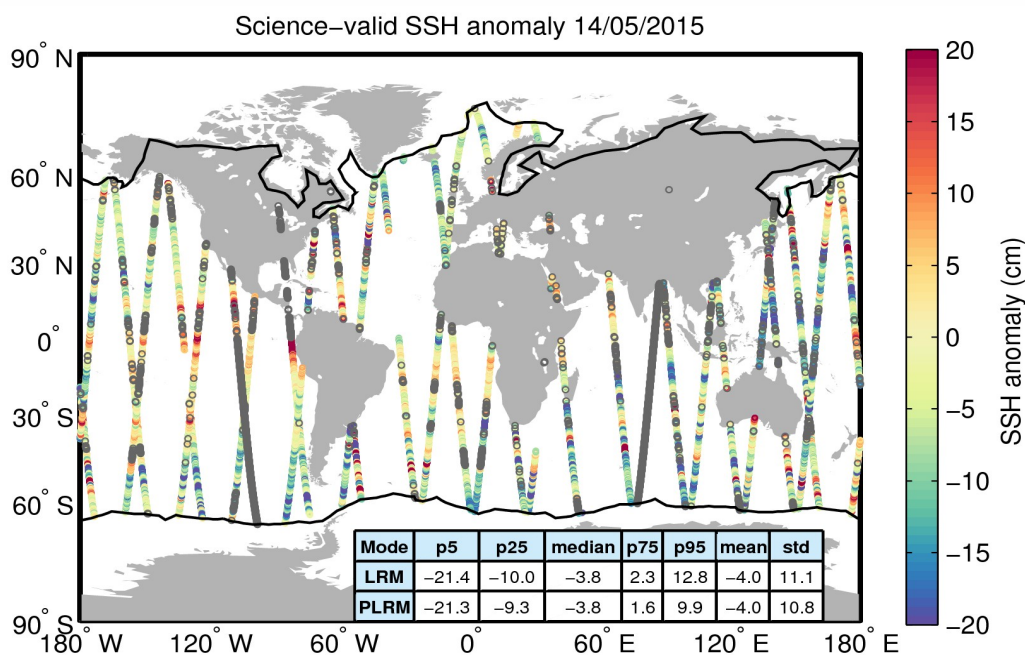
Figure 10. Geographical distribution of science-valid SSH anomaly data over oceans and lakes for 14/05/2015. The statistical values shown in the table refer to the SSH anomaly in cm and are calculated separately for LRM and PLRM regions. The black lines mark the outer limit of the Arctic and Antarctic polar polygons. Gray circles denote records that have been rejected based on the editing criteria described in Table 2.
