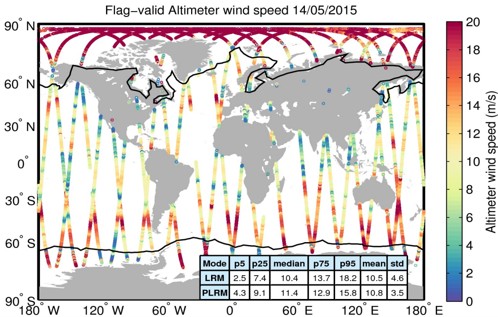
Figure 31. Geographical distribution of flag-valid wind data over oceans and lakes for 14/05/2015. The statistical values shown in the table refer to the wind in m/s and are calculated separately for LRM and PLRM regions. Measurements taken over polar polygons have been excluded from the computation of the statistical values. The black lines mark the outer limit of the Arctic and Antarctic polar polygons.
