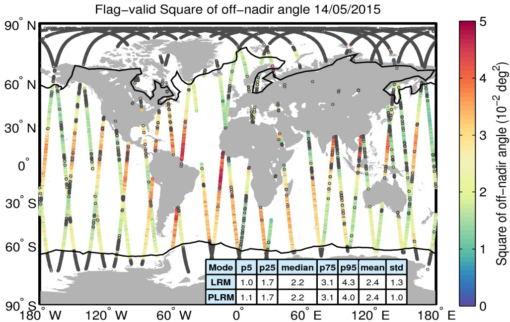
Figure 37. Geographical distribution of flag-valid mispointing data over oceans and lakes for 14/05/2015. The statistical values shown in the table refer to the mispointing in 10^{-2} \text{ deg}^2 and are calculated separately for LRM and PLRM regions. Measurements taken over polar polygons have been excluded from the computation of the statistical values. The black lines mark the outer limit of the Arctic and Antarctic polar polygons. Gray circles denote negative values.
