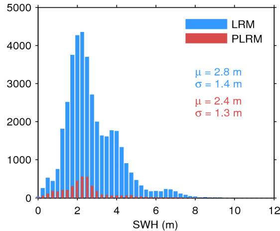
Figure 17. Histogram of flag-valid SWH over oceans and lakes for LRM (blue) and PLRM (red) for 14/05/2015. The mean ( \mu ) and standard deviation ( \sigma ) are also shown. Note that values larger than 12 m are excluded from the histogram for the sake of readability but not from the computation of \mu and \sigma .
