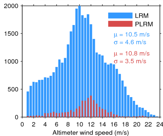
Figure 35. Histogram of science-valid wind over oceans and lakes for LRM (blue) and PLRM (red) for 14/05/2015. The mean ( \mu ) and standard deviation ( \sigma ) are also shown. Note that values larger than 24 m/s are excluded from the histogram for the sake of readability but not from the computation of \mu and \sigma .
