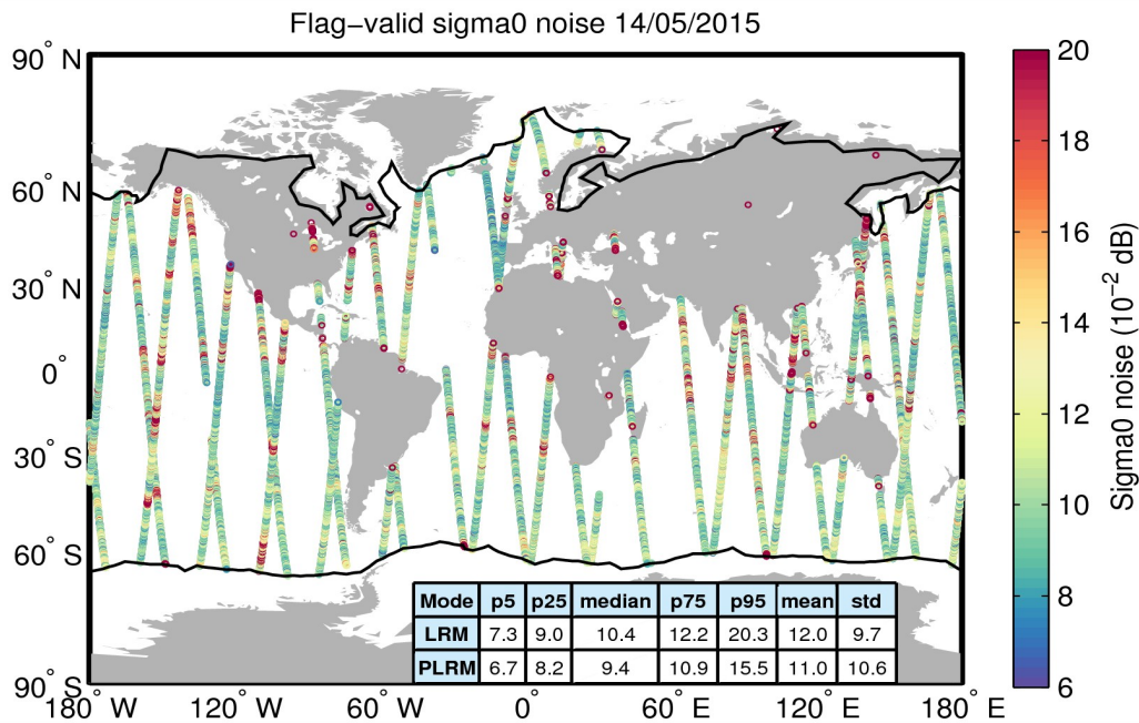
Figure 26. Geographical distribution of flag-valid 20-Hz sigma0 measurement noise over oceans and lakes for 14/05/2015. The statistical values shown in the table refer to the sigma0 noise and are calculated separately for LRM and PLRM regions. Measurements taken over polar polygons have been excluded from the computation of the statistical values. The black lines mark the outer limit of the Arctic and Antarctic polar polygons.
