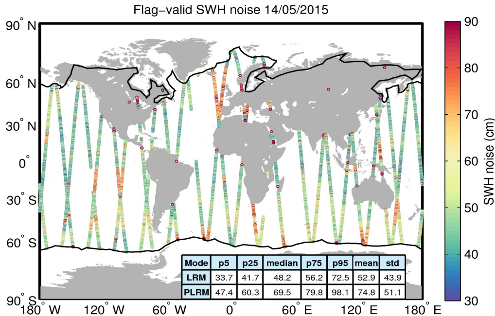
Figure 18. Geographical distribution of flag-valid 20-Hz SWH measurement noise over oceans and lakes for 14/05/2015. The statistical values shown in the table refer to the SWH noise and are calculated separately for LRM and PLRM regions. Measurements taken over polar polygons have been excluded from the computation of the statistical values. The black lines mark the outer limit of the Arctic and Antarctic polar polygons.
