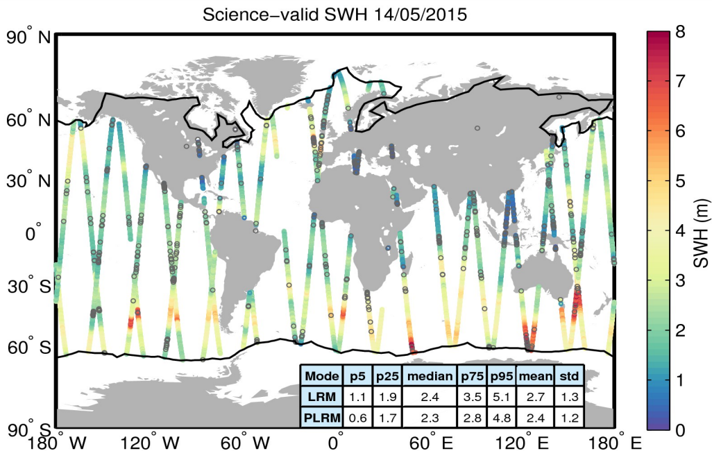
Figure 19. Geographical distribution of science-valid SWH data over oceans and lakes for 14/05/2015. The statistical values shown in the table refer to the SWH in m and are calculated separately for LRM and PLRM regions. The black lines mark the outer limit of the Arctic and Antarctic polar polygons. Gray circles denote records that have been rejected based on the editing criteria described in Table 3.
