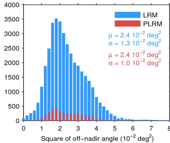
Figure 39. Histogram of flag-valid mispointing over oceans and lakes for LRM (blue) and PLRM (red) for 14/05/2015. Only positive values have been considered. The mean ( \mu ) and standard deviation ( \sigma ) are also shown. Note that values larger than 8 \cdot 10^{-2} \text{ deg}^2 are excluded from the histogram for the sake of readability but not from the computation of \mu and \sigma .
