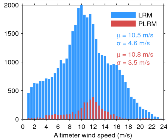
Figure 33. Histogram of flag-valid wind over oceans and lakes for LRM (blue) and PLRM (red) for 14/05/2015. The mean ( \mu ) and standard deviation ( \sigma ) are also shown. Note that values larger than 24 m/s are excluded from the histogram for the sake of readability but not from the computation of \mu and \sigma .
