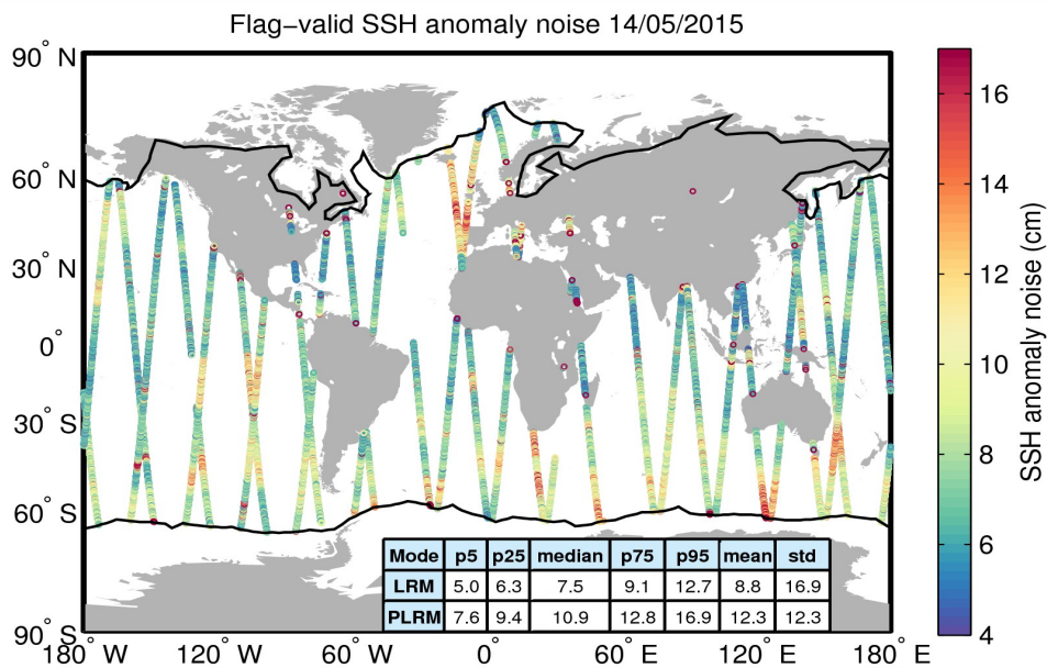
Figure 8. Geographical distribution of flag-valid 20-Hz SSH anomaly measurement noise over oceans and lakes for 14/05/2015. The statistical values shown in the table refer to the SSH anomaly noise and are calculated separately for LRM and PLRM regions. Measurements taken over polar polygons have been excluded from the computation of the statistical values. The black lines mark the outer limit of the Arctic and Antarctic polar polygons.
