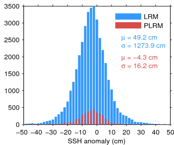
Figure 7. Histogram of flag-valid SSH anomaly over oceans and lakes for LRM (blue) and PLRM (red) for 14/05/2015. The mean ( \mu ) and standard deviation ( \sigma ) are also shown. Note that values outside [-50 50] cm are excluded from the histogram for the sake of readability but not from the computation of \mu and \sigma .
