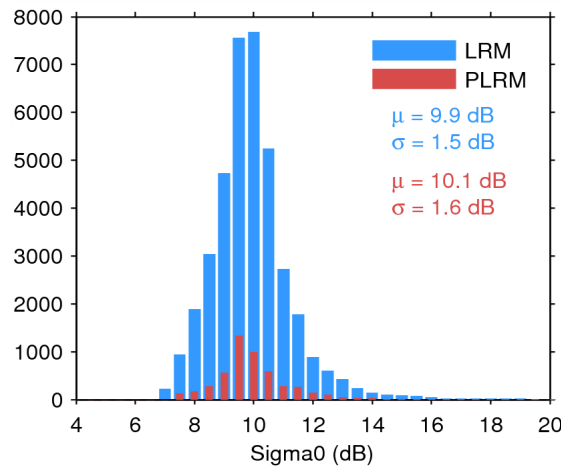
Figure 28. Histogram of science-valid sigma0 over oceans and lakes for LRM (blue) and PLRM (red) for 11/05/2015. The mean ( \mu ) and standard deviation ( \sigma ) are also shown. Note that values outside [4 20] dB are excluded from the histogram for the sake of readability but not from the computation of \mu and \sigma .
