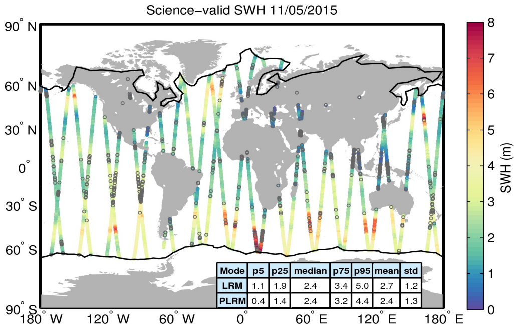
Figure 19. Geographical distribution of science-valid SWH data over oceans and lakes for 11/05/2015. The statistical values shown in the table refer to the SWH in m and are calculated separately for LRM and PLRM regions. The black lines mark the outer limit of the Arctic and Antarctic polar polygons. Gray circles denote records that have been rejected based on the editing criteria described in Table 3.
