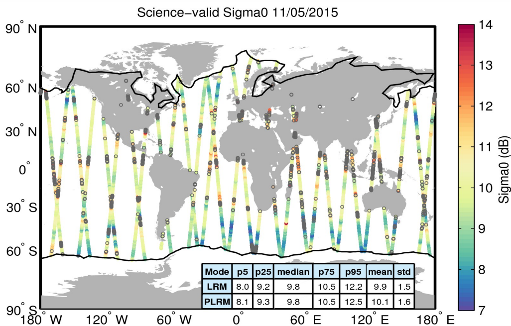
Figure 27. Geographical distribution of science-valid sigma0 data over oceans and lakes for 11/05/2015. The statistical values shown in the table refer to the sigma0 in dB and are calculated separately for LRM and PLRM regions. The black lines mark the outer limit of the Arctic and Antarctic polar polygons. Gray circles denote records that have been rejected based on the editing criteria described in Table 4.
