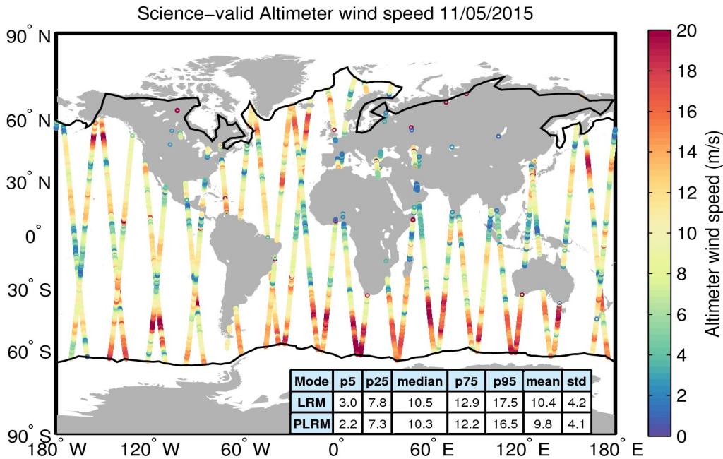
Figure 34. Geographical distribution of science-valid wind data over oceans and lakes for 11/05/2015. The statistical values shown in the table refer to the wind in m/s and are calculated separately for LRM and PLRM regions. The black lines mark the outer limit of the Arctic and Antarctic polar polygons. Gray circles denote records that have been rejected based on the editing criteria described in Table 5.
