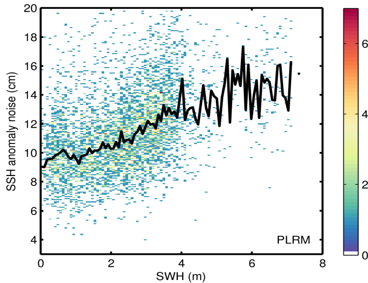
Figure 9. 2D histogram showing flag-valid SSH anomaly noise as a function of SWH for LRM (top) and PLRM (bottom) for 11/05/2015. The black line denotes the median SSH anomaly as a function of SWH.
