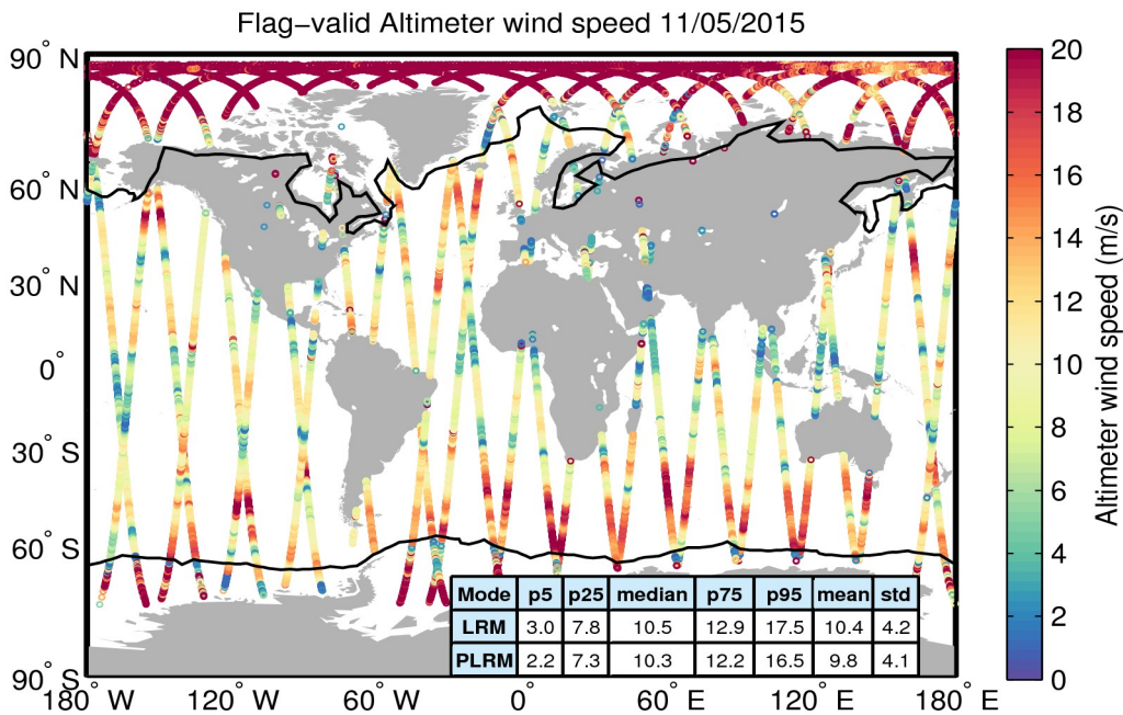
Figure 31. Geographical distribution of flag-valid wind data over oceans and lakes for 11/05/2015. The statistical values shown in the table refer to the wind in m/s and are calculated separately for LRM and PLRM regions. Measurements taken over polar polygons have been excluded from the computation of the statistical values. The black lines mark the outer limit of the Arctic and Antarctic polar polygons.
