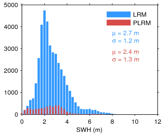
Figure 20. Histogram of science-valid SWH over oceans and lakes for LRM (blue) and PLRM (red) for 11/05/2015. The mean ( \mu ) and standard deviation ( \sigma ) are also shown. Note that values larger than 12 m are excluded from the histogram for the sake of readability but not from the computation of \mu and \sigma .
