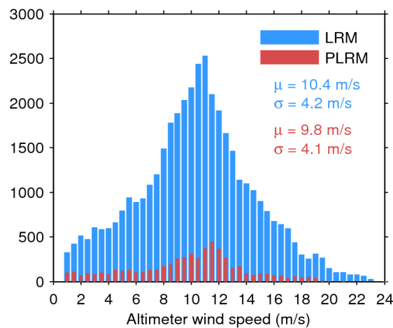
Figure 33. Histogram of flag-valid wind over oceans and lakes for LRM (blue) and PLRM (red) for 11/05/2015. The mean ( \mu ) and standard deviation ( \sigma ) are also shown. Note that values larger than 24 m/s are excluded from the histogram for the sake of readability but not from the computation of \mu and \sigma .
