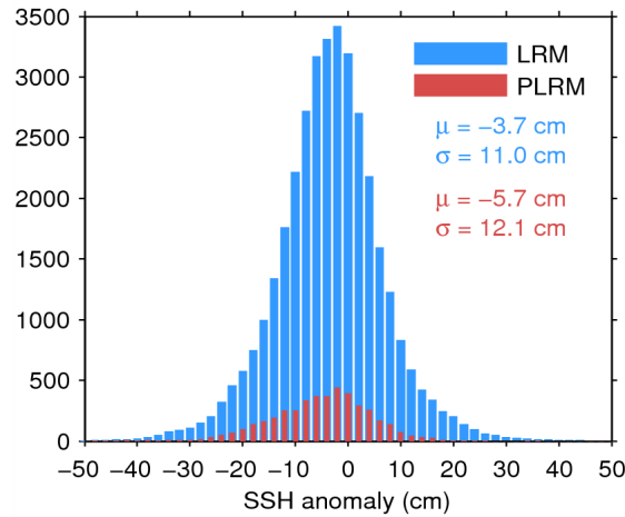
Figure 11. Histogram of science-valid SSH anomaly over oceans and lakes for LRM (blue) and PLRM (red) for 11/05/2015. The mean ( \mu ) and standard deviation ( \sigma ) are also shown. Note that values outside [-50\ 50] cm are excluded from the histogram for the sake of readability but not from the computation of \mu and \sigma .
