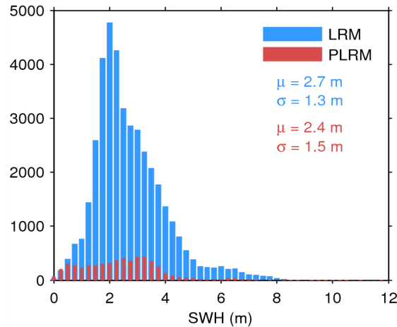
Figure 17. Histogram of flag-valid SWH over oceans and lakes for LRM (blue) and PLRM (red) for 11/05/2015. The mean ( \mu ) and standard deviation ( \sigma ) are also shown. Note that values larger than 12 m are excluded from the histogram for the sake of readability but not from the computation of \mu and \sigma .
