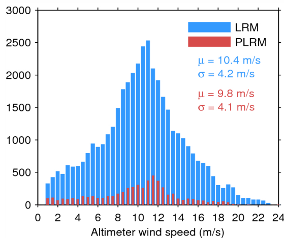
Figure 35. Histogram of science-valid wind over oceans and lakes for LRM (blue) and PLRM (red) for 11/05/2015. The mean ( \mu ) and standard deviation ( \sigma ) are also shown. Note that values larger than 24 m/s are excluded from the histogram for the sake of readability but not from the computation of \mu and \sigma .
