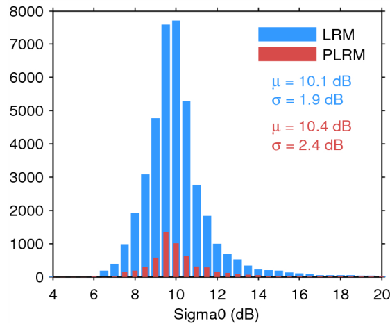
Figure 25. Histogram of flag-valid sigma0 over oceans and lakes for LRM (blue) and PLRM (red) for 11/05/2015. The mean ( \mu ) and standard deviation ( \sigma ) are also shown. Note that values outside [4 20] dB are excluded from the histogram for the sake of readability but not from the computation of \mu and \sigma .
