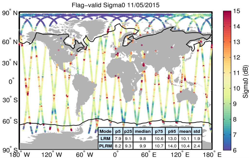
Figure 23. Geographical distribution of flag-valid sigma0 data over oceans and lakes for 11/05/2015. The statistical values shown in the table refer to the sigma0 in dB and are calculated separately for LRM and PLRM regions. Measurements taken over polar polygons have been excluded from the computation of the statistical values. The black lines mark the outer limit of the Arctic and Antarctic polar polygons.
