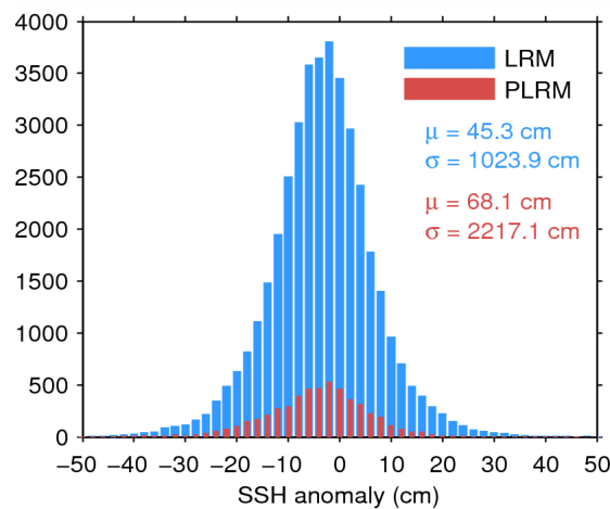
Figure 7. Histogram of flag-valid SSH anomaly over oceans and lakes for LRM (blue) and PLRM (red) for 11/05/2015. The mean ( \mu ) and standard deviation ( \sigma ) are also shown. Note that values outside [-50\ 50] cm are excluded from the histogram for the sake of readability but not from the computation of \mu and \sigma .
