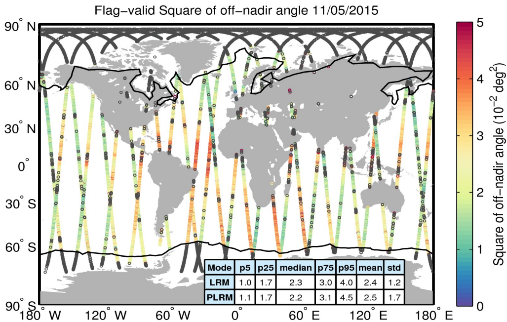
Figure 37. Geographical distribution of flag-valid mispointing data over oceans and lakes for 11/05/2015. The statistical values shown in the table refer to the mispointing in 10^{-2} \text{ deg}^2 and are calculated separately for LRM and PLRM regions. Measurements taken over polar polygons have been excluded from the computation of the statistical values. The black lines mark the outer limit of the Arctic and Antarctic polar polygons. Gray circles denote negative values.
