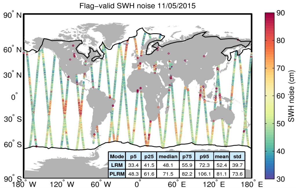
Figure 18. Geographical distribution of flag-valid 20-Hz SWH measurement noise over oceans and lakes for 11/05/2015. The statistical values shown in the table refer to the SWH noise and are calculated separately for LRM and PLRM regions. Measurements taken over polar polygons have been excluded from the computation of the statistical values. The black lines mark the outer limit of the Arctic and Antarctic polar polygons.
