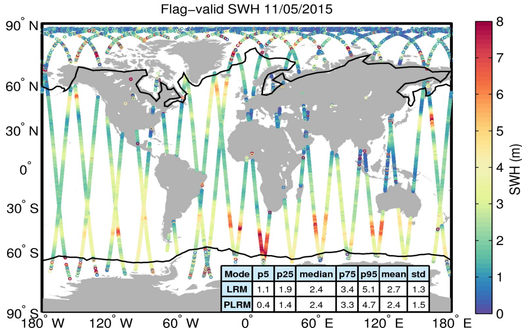
Figure 15. Geographical distribution of flag-valid SWH data over oceans and lakes for 11/05/2015. The statistical values shown in the table refer to the SWH in m and are calculated separately for LRM and PLRM regions. Measurements taken over polar polygons have been excluded from the computation of the statistical values. The black lines mark the outer limit of the Arctic and Antarctic polar polygons.
