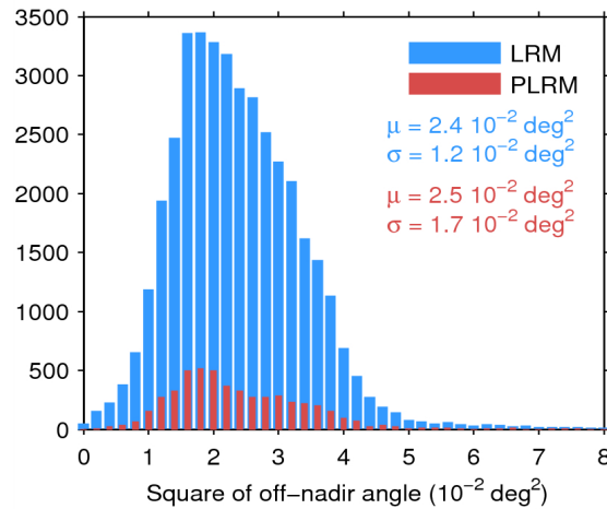
Figure 39. Histogram of flag-valid mispointing over oceans and lakes for LRM (blue) and PLRM (red) for 11/05/2015. Only positive values have been considered. The mean ( \mu ) and standard deviation ( \sigma ) are also shown. Note that values larger than 8 \cdot 10^{-2} \text{ deg}^2 are excluded from the histogram for the sake of readability but not from the computation of \mu and \sigma .
