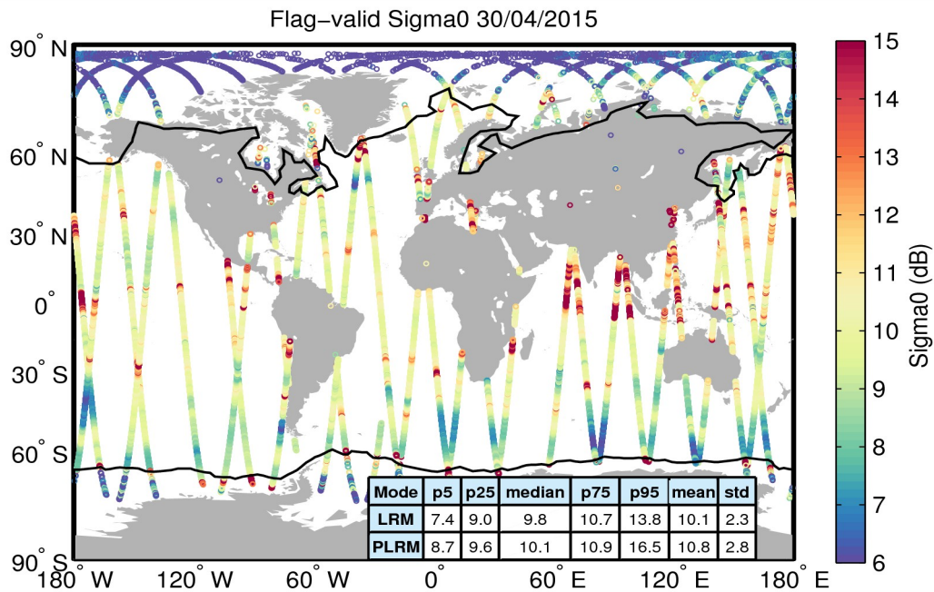
Figure 23. Geographical distribution of flag-valid sigma0 data over oceans and lakes for 30/04/2015. The statistical values shown in the table refer to the sigma0 in dB and are calculated separately for LRM and PLRM regions. Measurements taken over polar polygons have been excluded from the computation of the statistical values. The black lines mark the outer limit of the Arctic and Antarctic polar polygons.
