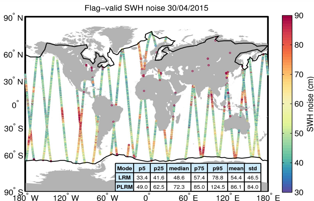
Figure 18. Geographical distribution of flag-valid 20-Hz SWH measurement noise over oceans and lakes for 30/04/2015. The statistical values shown in the table refer to the SWH noise and are calculated separately for LRM and PLRM regions. Measurements taken over polar polygons have been excluded from the computation of the statistical values. The black lines mark the outer limit of the Arctic and Antarctic polar polygons.
