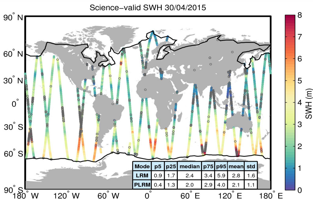
Figure 19. Geographical distribution of science-valid SWH data over oceans and lakes for 30/04/2015. The statistical values shown in the table refer to the SWH in m and are calculated separately for LRM and PLRM regions. The black lines mark the outer limit of the Arctic and Antarctic polar polygons. Gray circles denote records that have been rejected based on the editing criteria described in Table 3.
