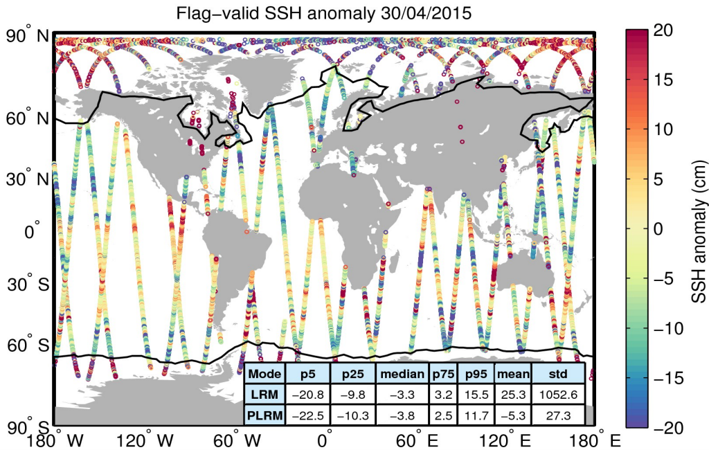
Figure 5. Geographical distribution of flag-valid 1-Hz SSH anomaly data over oceans and lakes for 30/04/2015. The statistical values shown in the table refer to the SSH anomaly in cm and are calculated separately for LRM and PLRM regions. Measurements taken over polar polygons have been excluded from the computation of the statistical values. The black lines mark the outer limit of the Arctic and Antarctic polar polygons.
