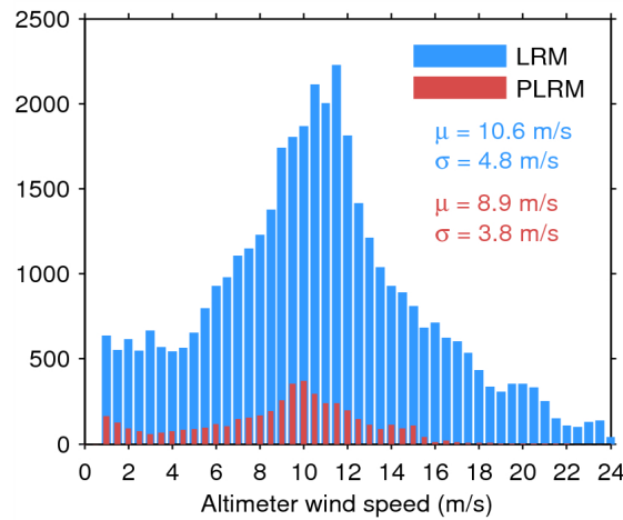
Figure 33. Histogram of flag-valid wind over oceans and lakes for LRM (blue) and PLRM (red) for 30/04/2015. The mean ( \mu ) and standard deviation ( \sigma ) are also shown. Note that values larger than 24 m/s are excluded from the histogram for the sake of readability but not from the computation of \mu and \sigma .
