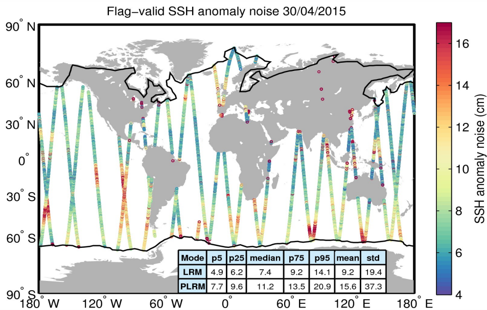
Figure 8. Geographical distribution of flag-valid 20-Hz SSH anomaly measurement noise over oceans and lakes for 30/04/2015. The statistical values shown in the table refer to the SSH anomaly noise and are calculated separately for LRM and PLRM regions. Measurements taken over polar polygons have been excluded from the computation of the statistical values. The black lines mark the outer limit of the Arctic and Antarctic polar polygons.
