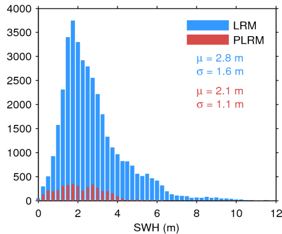
Figure 20. Histogram of science-valid SWH over oceans and lakes for LRM (blue) and PLRM (red) for 30/04/2015. The mean ( \mu ) and standard deviation ( \sigma ) are also shown. Note that values larger than 12 m are excluded from the histogram for the sake of readability but not from the computation of \mu and \sigma .
