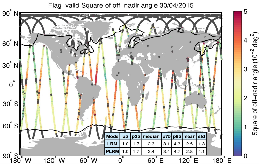
Figure 37. Geographical distribution of flag-valid mispointing data over oceans and lakes for 30/04/2015. The statistical values shown in the table refer to the mispointing in 10^{-2} \text{ deg}^2 and are calculated separately for LRM and PLRM regions. Measurements taken over polar polygons have been excluded from the computation of the statistical values. The black lines mark the outer limit of the Arctic and Antarctic polar polygons. Gray circles denote negative values.
