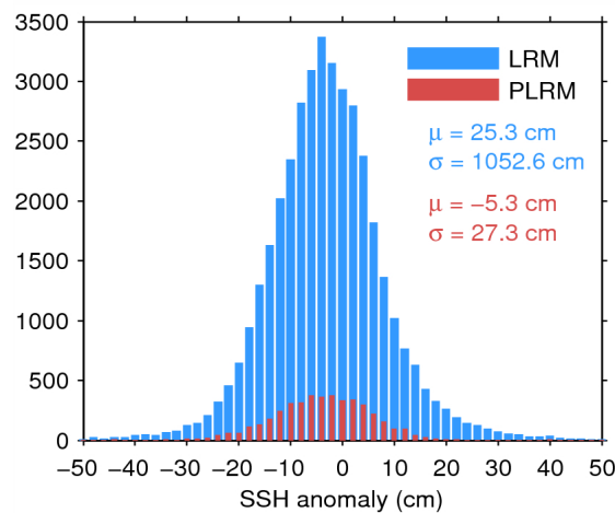
Figure 7. Histogram of flag-valid SSH anomaly over oceans and lakes for LRM (blue) and PLRM (red) for 30/04/2015. The mean ( \mu ) and standard deviation ( \sigma ) are also shown. Note that values outside [-50\ 50] cm are excluded from the histogram for the sake of readability but not from the computation of \mu and \sigma .
