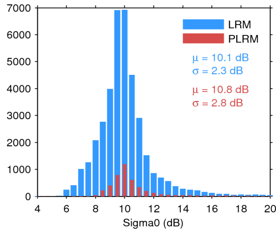
Figure 25. Histogram of flag-valid sigma0 over oceans and lakes for LRM (blue) and PLRM (red) for 30/04/2015. The mean ( \mu ) and standard deviation ( \sigma ) are also shown. Note that values outside [4 20] dB are excluded from the histogram for the sake of readability but not from the computation of \mu and \sigma .
