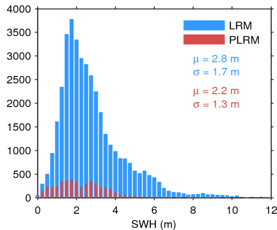
Figure 17. Histogram of flag-valid SWH over oceans and lakes for LRM (blue) and PLRM (red) for 30/04/2015. The mean ( \mu ) and standard deviation ( \sigma ) are also shown. Note that values larger than 12 m are excluded from the histogram for the sake of readability but not from the computation of \mu and \sigma .
