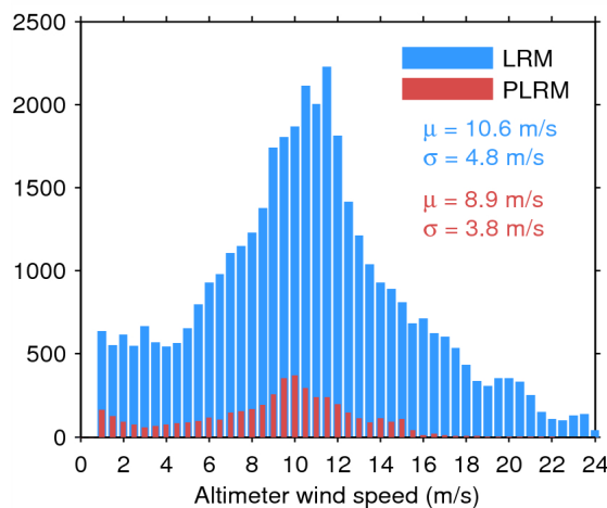
Figure 35. Histogram of science-valid wind over oceans and lakes for LRM (blue) and PLRM (red) for 30/04/2015. The mean ( \mu ) and standard deviation ( \sigma ) are also shown. Note that values larger than 24 m/s are excluded from the histogram for the sake of readability but not from the computation of \mu and \sigma .
