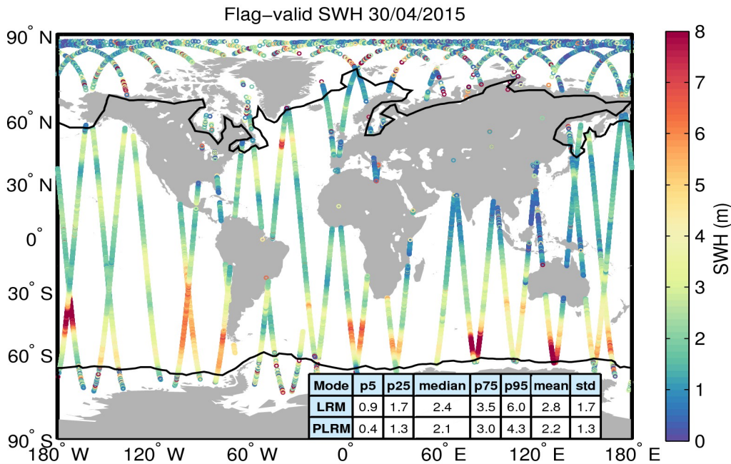
Figure 15. Geographical distribution of flag-valid SWH data over oceans and lakes for 30/04/2015. The statistical values shown in the table refer to the SWH in m and are calculated separately for LRM and PLRM regions. Measurements taken over polar polygons have been excluded from the computation of the statistical values. The black lines mark the outer limit of the Arctic and Antarctic polar polygons.
