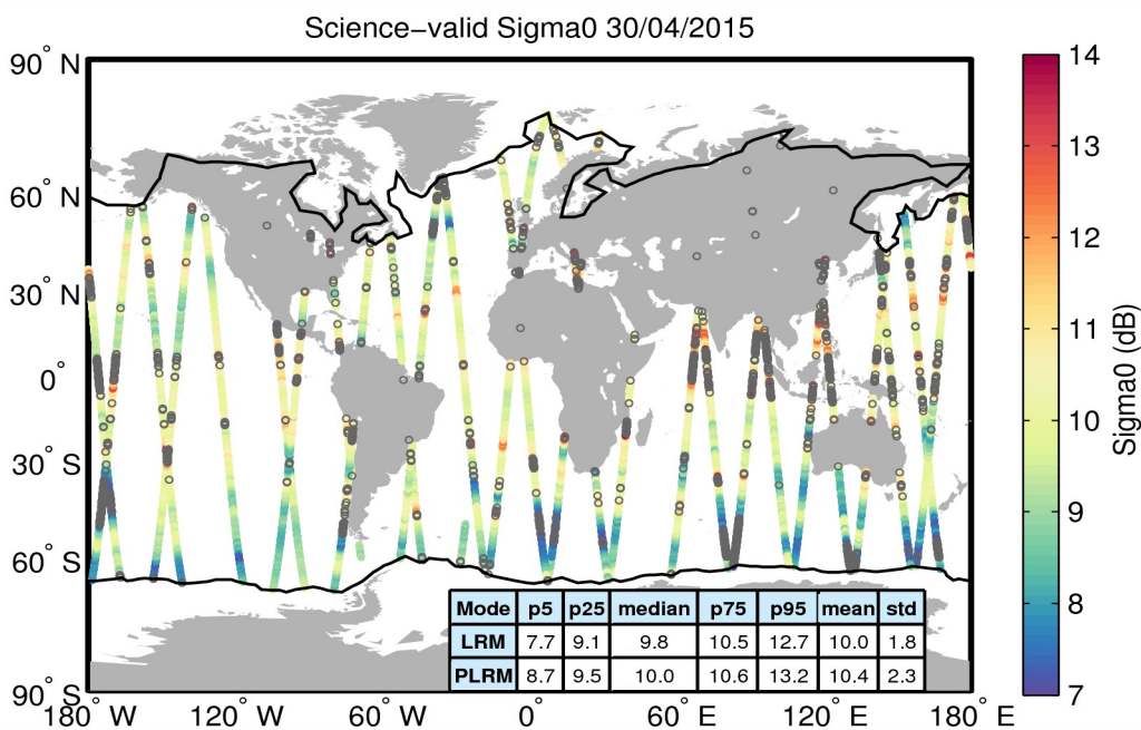
Figure 27. Geographical distribution of science-valid sigma0 data over oceans and lakes for 30/04/2015. The statistical values shown in the table refer to the sigma0 in dB and are calculated separately for LRM and PLRM regions. The black lines mark the outer limit of the Arctic and Antarctic polar polygons. Gray circles denote records that have been rejected based on the editing criteria described in Table 4.
