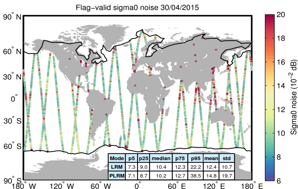
Figure 26. Geographical distribution of flag-valid 20-Hz sigma0 measurement noise over oceans and lakes for 30/04/2015. The statistical values shown in the table refer to the sigma0 noise and are calculated separately for LRM and PLRM regions. Measurements taken over polar polygons have been excluded from the computation of the statistical values. The black lines mark the outer limit of the Arctic and Antarctic polar polygons.
