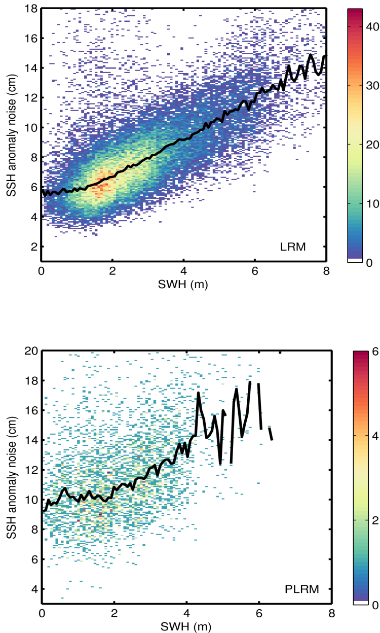
Figure 9. 2D histogram showing flag-valid SSH anomaly noise as a function of SWH for LRM (top) and PLRM (bottom) for 30/04/2015. The black line denotes the median SSH anomaly as a function of SWH.
