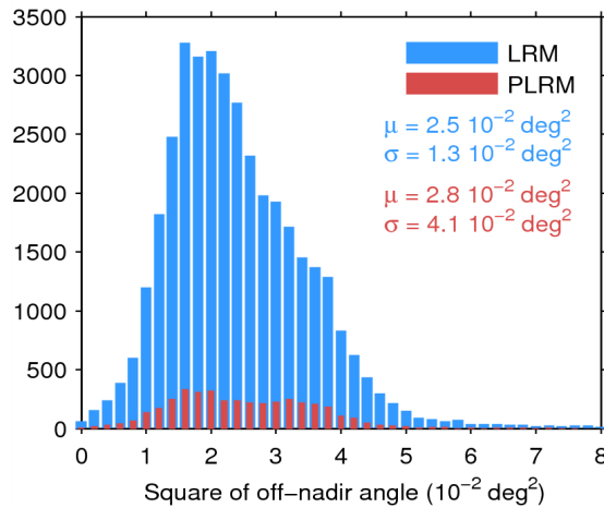
Figure 39. Histogram of flag-valid mispointing over oceans and lakes for LRM (blue) and PLRM (red) for 30/04/2015. Only positive values have been considered. The mean ( \mu ) and standard deviation ( \sigma ) are also shown. Note that values larger than 8 \cdot 10^{-2} \text{ deg}^2 are excluded from the histogram for the sake of readability but not from the computation of \mu and \sigma .
