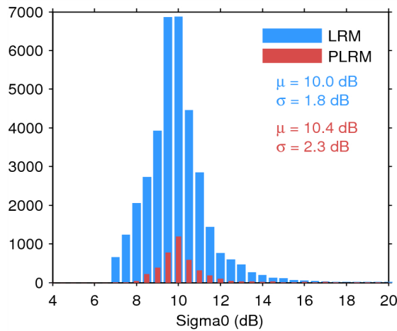
Figure 28. Histogram of science-valid sigma0 over oceans and lakes for LRM (blue) and PLRM (red) for 30/04/2015. The mean ( \mu ) and standard deviation ( \sigma ) are also shown. Note that values outside [4 20] dB are excluded from the histogram for the sake of readability but not from the computation of \mu and \sigma .
