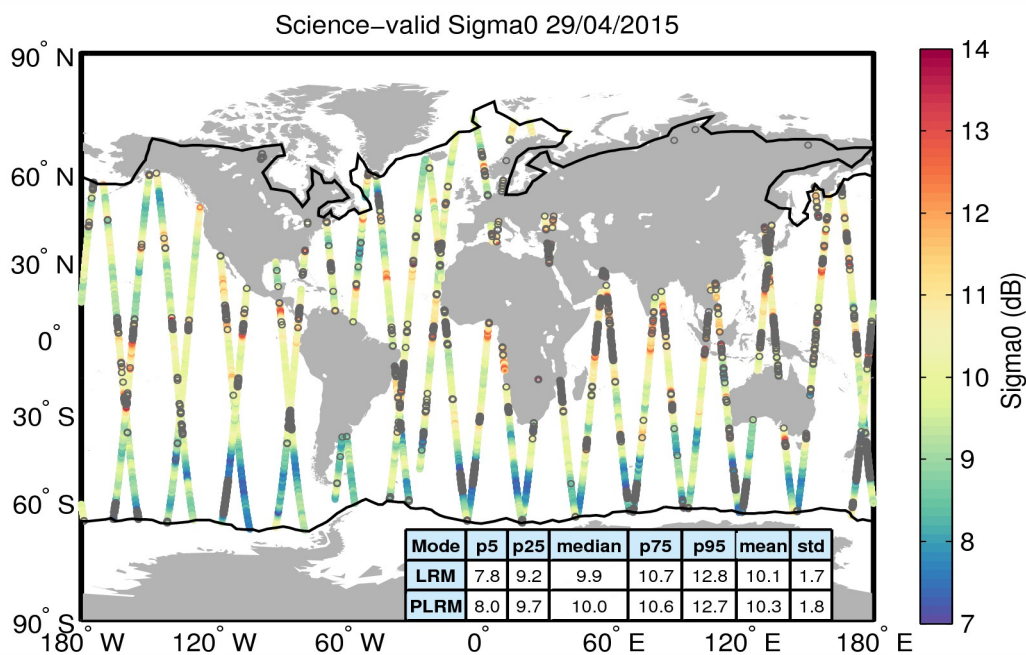
Figure 27. Geographical distribution of science-valid sigma0 data over oceans and lakes for 29/04/2015. The statistical values shown in the table refer to the sigma0 in dB and are calculated separately for LRM and PLRM regions. The black lines mark the outer limit of the Arctic and Antarctic polar polygons. Gray circles denote records that have been rejected based on the editing criteria described in Table 4.
