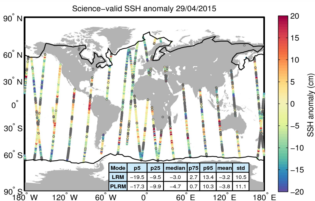
Figure 10. Geographical distribution of science-valid SSH anomaly data over oceans and lakes for 29/04/2015. The statistical values shown in the table refer to the SSH anomaly in cm and are calculated separately for LRM and PLRM regions. The black lines mark the outer limit of the Arctic and Antarctic polar polygons. Gray circles denote records that have been rejected based on the editing criteria described in Table 2.
