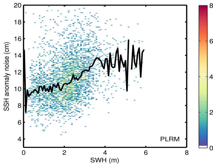
Figure 9. 2D histogram showing flag-valid SSH anomaly noise as a function of SWH for LRM (top) and PLRM (bottom) for 29/04/2015. The black line denotes the median SSH anomaly as a function of SWH.
