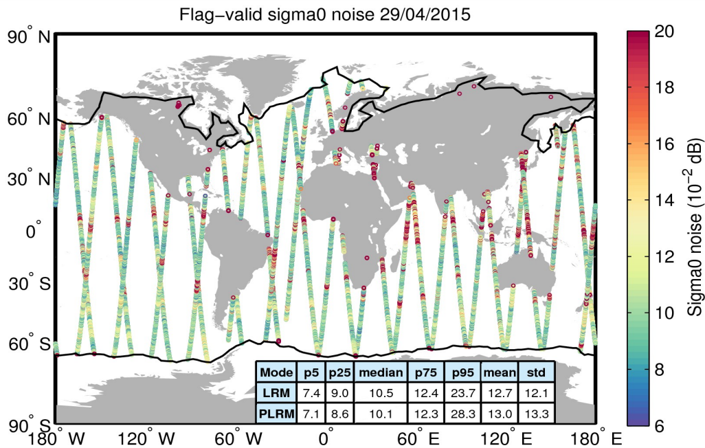
Figure 26. Geographical distribution of flag-valid 20-Hz sigma0 measurement noise over oceans and lakes for 29/04/2015. The statistical values shown in the table refer to the sigma0 noise and are calculated separately for LRM and PLRM regions. Measurements taken over polar polygons have been excluded from the computation of the statistical values. The black lines mark the outer limit of the Arctic and Antarctic polar polygons.
