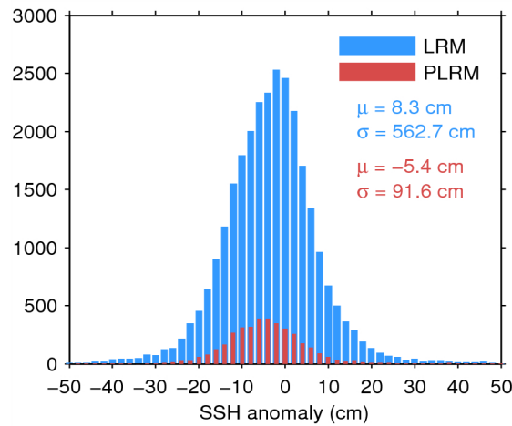
Figure 7. Histogram of flag-valid SSH anomaly over oceans and lakes for LRM (blue) and PLRM (red) for 29/04/2015. The mean ( \mu ) and standard deviation ( \sigma ) are also shown. Note that values outside [-50\ 50] cm are excluded from the histogram for the sake of readability but not from the computation of \mu and \sigma .
