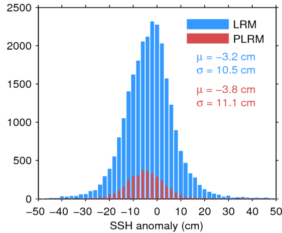
Figure 11. Histogram of science-valid SSH anomaly over oceans and lakes for LRM (blue) and PLRM (red) for 29/04/2015. The mean ( \mu ) and standard deviation ( \sigma ) are also shown. Note that values outside [-50\ 50] cm are excluded from the histogram for the sake of readability but not from the computation of \mu and \sigma .
