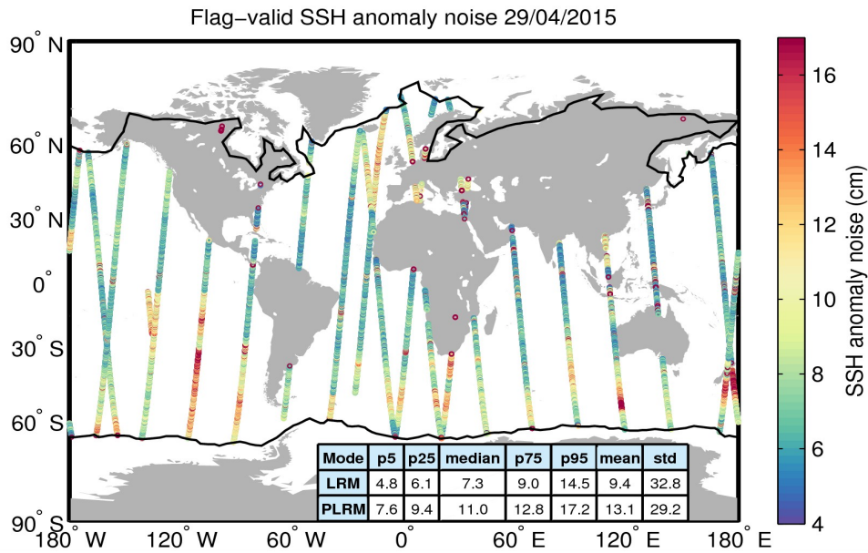
Figure 8. Geographical distribution of flag-valid 20-Hz SSH anomaly measurement noise over oceans and lakes for 29/04/2015. The statistical values shown in the table refer to the SSH anomaly noise and are calculated separately for LRM and PLRM regions. Measurements taken over polar polygons have been excluded from the computation of the statistical values. The black lines mark the outer limit of the Arctic and Antarctic polar polygons.
