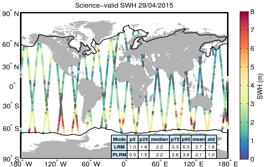
Figure 19. Geographical distribution of science-valid SWH data over oceans and lakes for 29/04/2015. The statistical values shown in the table refer to the SWH in m and are calculated separately for LRM and PLRM regions. The black lines mark the outer limit of the Arctic and Antarctic polar polygons. Gray circles denote records that have been rejected based on the editing criteria described in Table 3.
