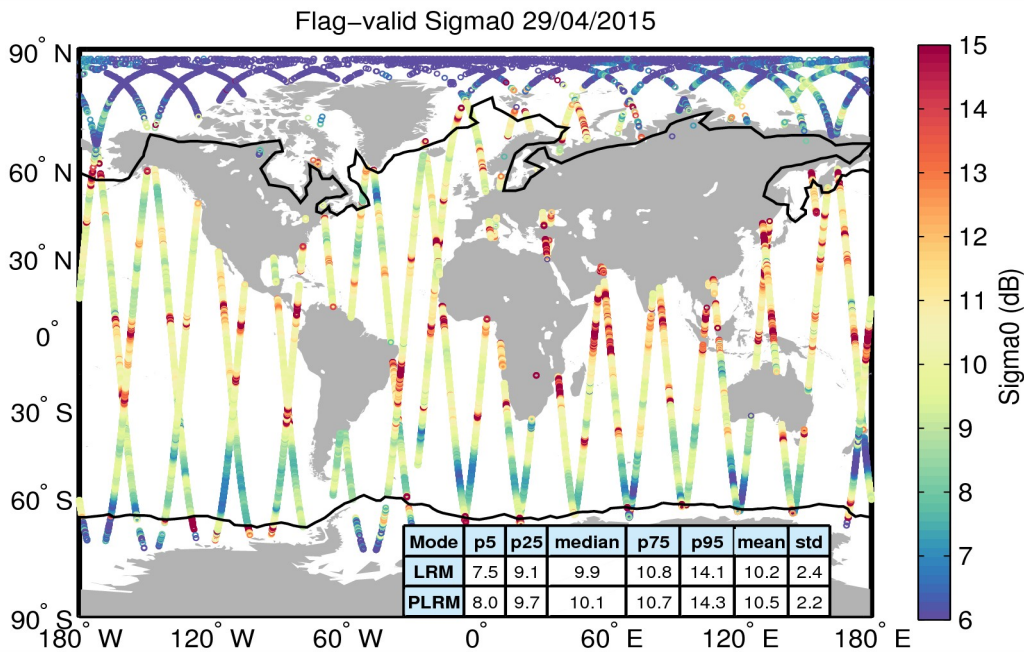
Figure 23. Geographical distribution of flag-valid sigma0 data over oceans and lakes for 29/04/2015. The statistical values shown in the table refer to the sigma0 in dB and are calculated separately for LRM and PLRM regions. Measurements taken over polar polygons have been excluded from the computation of the statistical values. The black lines mark the outer limit of the Arctic and Antarctic polar polygons.
