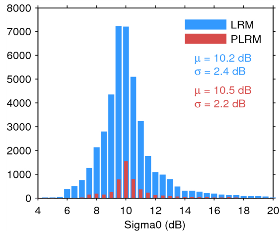
Figure 25. Histogram of flag-valid sigma0 over oceans and lakes for LRM (blue) and PLRM (red) for 29/04/2015. The mean ( \mu ) and standard deviation ( \sigma ) are also shown. Note that values outside [4 20] dB are excluded from the histogram for the sake of readability but not from the computation of \mu and \sigma .
