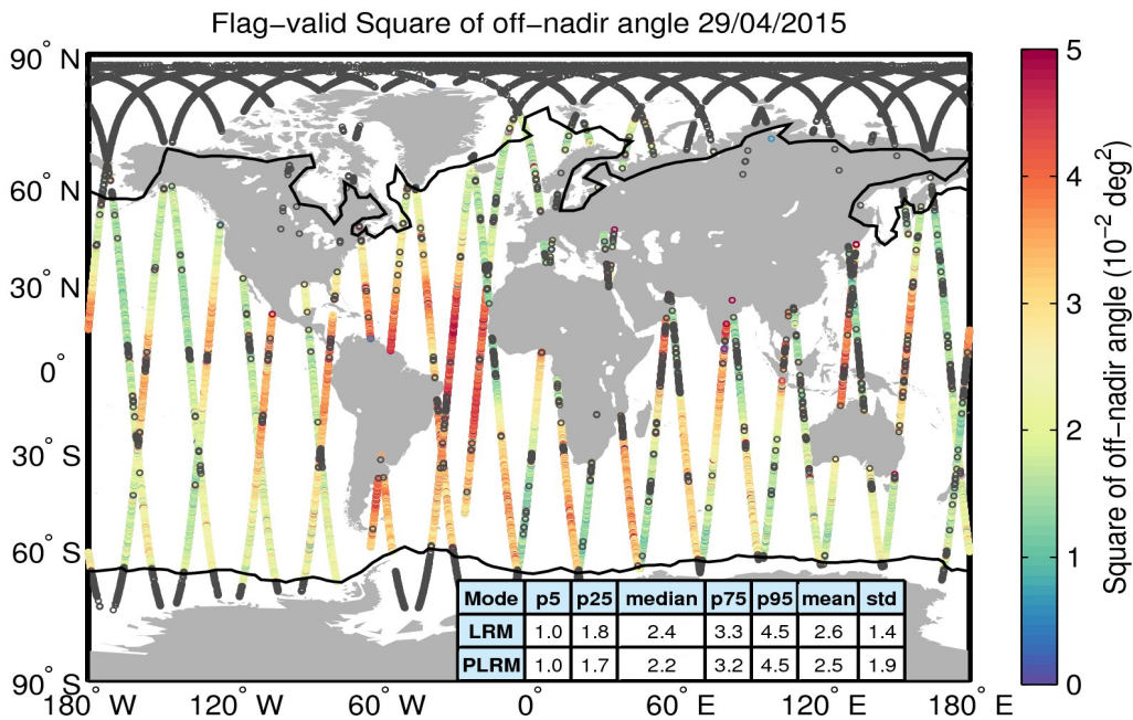
Figure 37. Geographical distribution of flag-valid mispointing data over oceans and lakes for 29/04/2015. The statistical values shown in the table refer to the mispointing in 10^{-2} \text{ deg}^2 and are calculated separately for LRM and PLRM regions. Measurements taken over polar polygons have been excluded from the computation of the statistical values. The black lines mark the outer limit of the Arctic and Antarctic polar polygons. Gray circles denote negative values.
