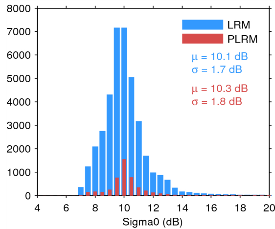
Figure 28. Histogram of science-valid sigma0 over oceans and lakes for LRM (blue) and PLRM (red) for 29/04/2015. The mean ( \mu ) and standard deviation ( \sigma ) are also shown. Note that values outside [4 20] dB are excluded from the histogram for the sake of readability but not from the computation of \mu and \sigma .
