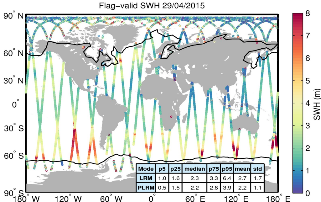
Figure 15. Geographical distribution of flag-valid SWH data over oceans and lakes for 29/04/2015. The statistical values shown in the table refer to the SWH in m and are calculated separately for LRM and PLRM regions. Measurements taken over polar polygons have been excluded from the computation of the statistical values. The black lines mark the outer limit of the Arctic and Antarctic polar polygons.
