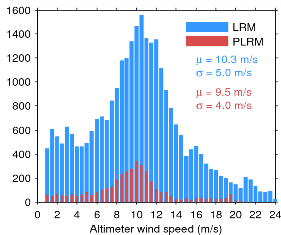
Figure 35. Histogram of science-valid wind over oceans and lakes for LRM (blue) and PLRM (red) for 29/04/2015. The mean ( \mu ) and standard deviation ( \sigma ) are also shown. Note that values larger than 24 m/s are excluded from the histogram for the sake of readability but not from the computation of \mu and \sigma .
