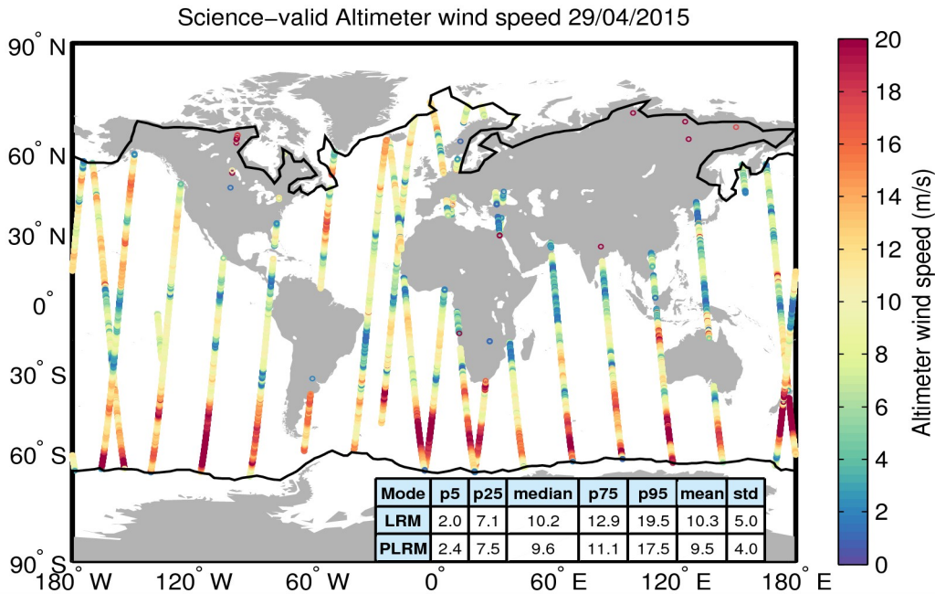
Figure 34. Geographical distribution of science-valid wind data over oceans and lakes for 29/04/2015. The statistical values shown in the table refer to the wind in m/s and are calculated separately for LRM and PLRM regions. The black lines mark the outer limit of the Arctic and Antarctic polar polygons. Gray circles denote records that have been rejected based on the editing criteria described in Table 5.
