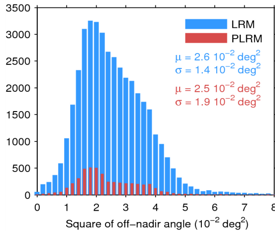
Figure 39. Histogram of flag-valid mispointing over oceans and lakes for LRM (blue) and PLRM (red) for 29/04/2015. Only positive values have been considered. The mean ( \mu ) and standard deviation ( \sigma ) are also shown. Note that values larger than 8 \cdot 10^{-2} \text{ deg}^2 are excluded from the histogram for the sake of readability but not from the computation of \mu and \sigma .
