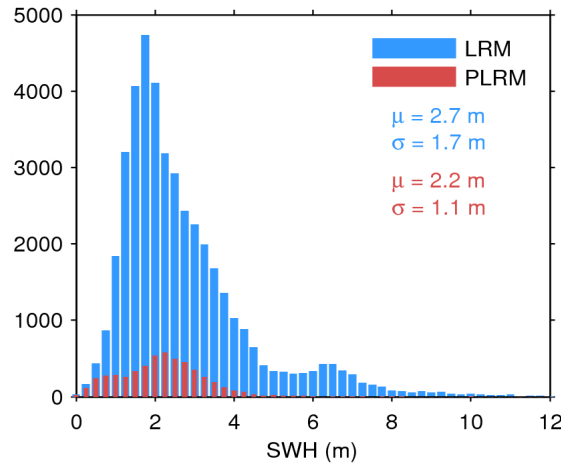
Figure 17. Histogram of flag-valid SWH over oceans and lakes for LRM (blue) and PLRM (red) for 29/04/2015. The mean ( \mu ) and standard deviation ( \sigma ) are also shown. Note that values larger than 12 m are excluded from the histogram for the sake of readability but not from the computation of \mu and \sigma .
