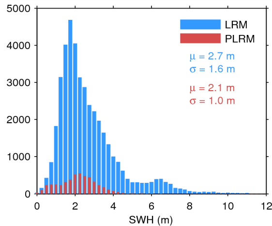
Figure 20. Histogram of science-valid SWH over oceans and lakes for LRM (blue) and PLRM (red) for 29/04/2015. The mean ( \mu ) and standard deviation ( \sigma ) are also shown. Note that values larger than 12 m are excluded from the histogram for the sake of readability but not from the computation of \mu and \sigma .
