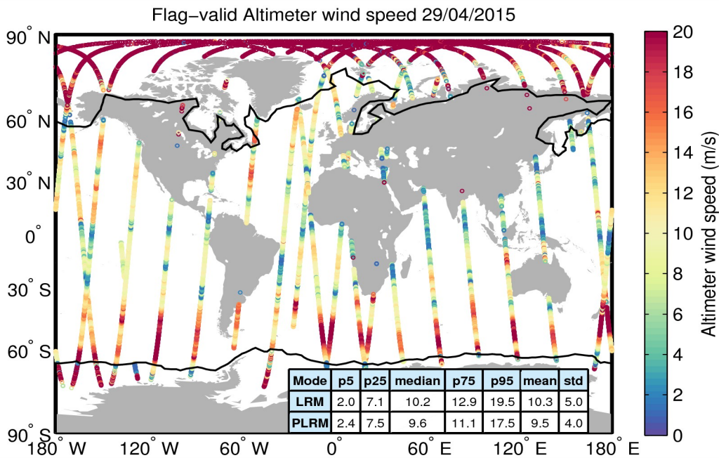
Figure 31. Geographical distribution of flag-valid wind data over oceans and lakes for 29/04/2015. The statistical values shown in the table refer to the wind in m/s and are calculated separately for LRM and PLRM regions. Measurements taken over polar polygons have been excluded from the computation of the statistical values. The black lines mark the outer limit of the Arctic and Antarctic polar polygons.
