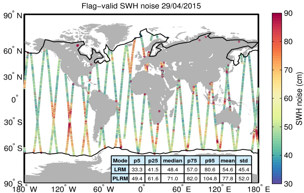
Figure 18. Geographical distribution of flag-valid 20-Hz SWH measurement noise over oceans and lakes for 29/04/2015. The statistical values shown in the table refer to the SWH noise and are calculated separately for LRM and PLRM regions. Measurements taken over polar polygons have been excluded from the computation of the statistical values. The black lines mark the outer limit of the Arctic and Antarctic polar polygons.
