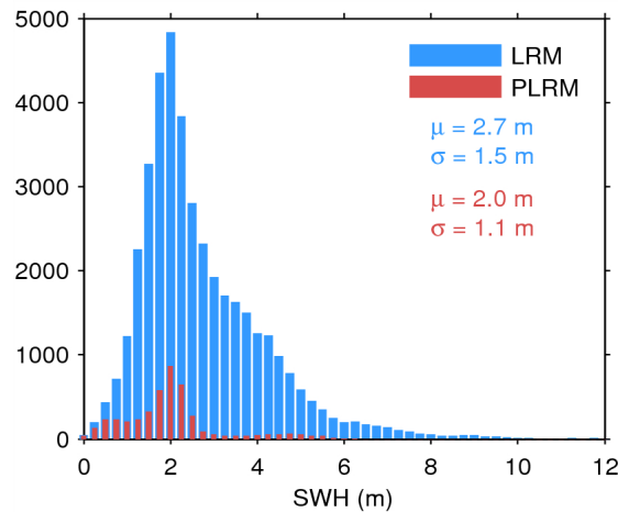
Figure 20. Histogram of science-valid SWH over oceans and lakes for LRM (blue) and PLRM (red) for 26/04/2015. The mean ( \mu ) and standard deviation ( \sigma ) are also shown. Note that values larger than 12 m are excluded from the histogram for the sake of readability but not from the computation of \mu and \sigma .
