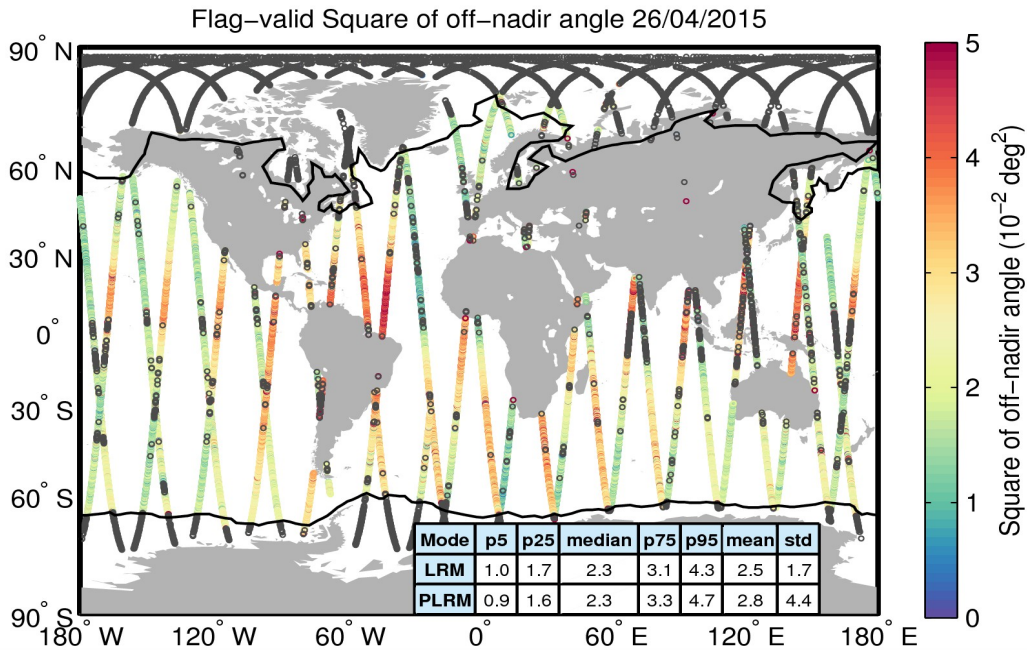
Figure 37. Geographical distribution of flag-valid mispointing data over oceans and lakes for 26/04/2015. The statistical values shown in the table refer to the mispointing in 10^{-2} \text{ deg}^2 and are calculated separately for LRM and PLRM regions. Measurements taken over polar polygons have been excluded from the computation of the statistical values. The black lines mark the outer limit of the Arctic and Antarctic polar polygons. Gray circles denote negative values.
