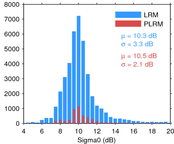
Figure 25. Histogram of flag-valid sigma0 over oceans and lakes for LRM (blue) and PLRM (red) for 26/04/2015. The mean ( \mu ) and standard deviation ( \sigma ) are also shown. Note that values outside [4 20] dB are excluded from the histogram for the sake of readability but not from the computation of \mu and \sigma .
