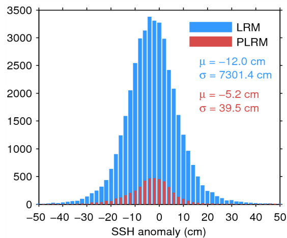
Figure 7. Histogram of flag-valid SSH anomaly over oceans and lakes for LRM (blue) and PLRM (red) for 26/04/2015. The mean ( \mu ) and standard deviation ( \sigma ) are also shown. Note that values outside [-50\ 50] cm are excluded from the histogram for the sake of readability but not from the computation of \mu and \sigma .
