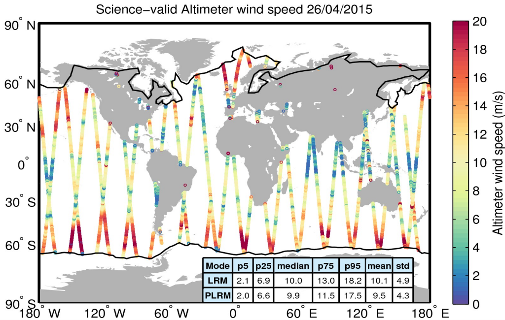
Figure 34. Geographical distribution of science-valid wind data over oceans and lakes for 26/04/2015. The statistical values shown in the table refer to the wind in m/s and are calculated separately for LRM and PLRM regions. The black lines mark the outer limit of the Arctic and Antarctic polar polygons. Gray circles denote records that have been rejected based on the editing criteria described in Table 5.
