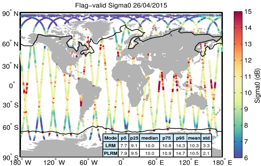
Figure 23. Geographical distribution of flag-valid sigma0 data over oceans and lakes for 26/04/2015. The statistical values shown in the table refer to the sigma0 in dB and are calculated separately for LRM and PLRM regions. Measurements taken over polar polygons have been excluded from the computation of the statistical values. The black lines mark the outer limit of the Arctic and Antarctic polar polygons.
