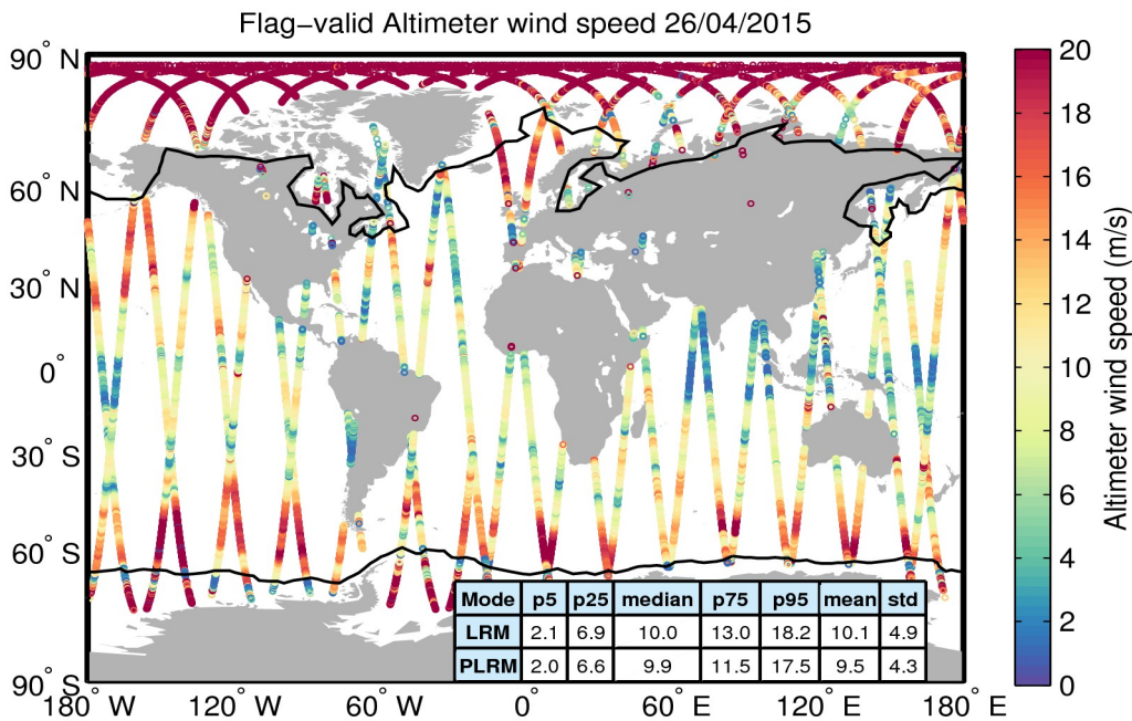
Figure 31. Geographical distribution of flag-valid wind data over oceans and lakes for 26/04/2015. The statistical values shown in the table refer to the wind in m/s and are calculated separately for LRM and PLRM regions. Measurements taken over polar polygons have been excluded from the computation of the statistical values. The black lines mark the outer limit of the Arctic and Antarctic polar polygons.
