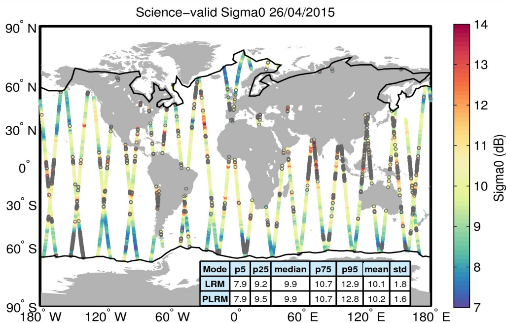
Figure 27. Geographical distribution of science-valid sigma0 data over oceans and lakes for 26/04/2015. The statistical values shown in the table refer to the sigma0 in dB and are calculated separately for LRM and PLRM regions. The black lines mark the outer limit of the Arctic and Antarctic polar polygons. Gray circles denote records that have been rejected based on the editing criteria described in Table 4.
