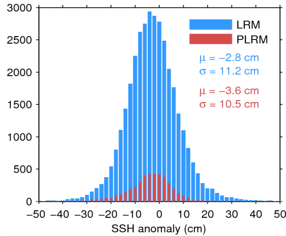
Figure 11. Histogram of science-valid SSH anomaly over oceans and lakes for LRM (blue) and PLRM (red) for 26/04/2015. The mean ( \mu ) and standard deviation ( \sigma ) are also shown. Note that values outside [-50 50] cm are excluded from the histogram for the sake of readability but not from the computation of \mu and \sigma .
