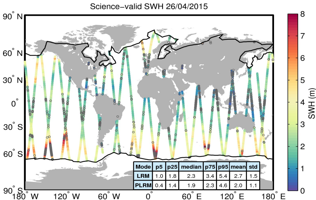
Figure 19. Geographical distribution of science-valid SWH data over oceans and lakes for 26/04/2015. The statistical values shown in the table refer to the SWH in m and are calculated separately for LRM and PLRM regions. The black lines mark the outer limit of the Arctic and Antarctic polar polygons. Gray circles denote records that have been rejected based on the editing criteria described in Table 3.
