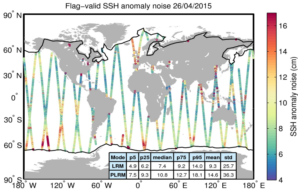
Figure 8. Geographical distribution of flag-valid 20-Hz SSH anomaly measurement noise over oceans and lakes for 26/04/2015. The statistical values shown in the table refer to the SSH anomaly noise and are calculated separately for LRM and PLRM regions. Measurements taken over polar polygons have been excluded from the computation of the statistical values. The black lines mark the outer limit of the Arctic and Antarctic polar polygons.
