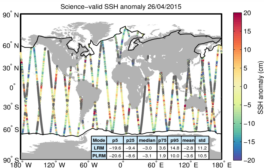
Figure 10. Geographical distribution of science-valid SSH anomaly data over oceans and lakes for 26/04/2015. The statistical values shown in the table refer to the SSH anomaly in cm and are calculated separately for LRM and PLRM regions. The black lines mark the outer limit of the Arctic and Antarctic polar polygons. Gray circles denote records that have been rejected based on the editing criteria described in Table 2.
