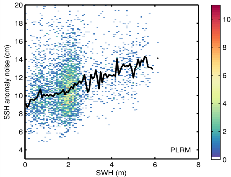
Figure 9. 2D histogram showing flag-valid SSH anomaly noise as a function of SWH for LRM (top) and PLRM (bottom) for 26/04/2015. The black line denotes the median SSH anomaly as a function of SWH.
