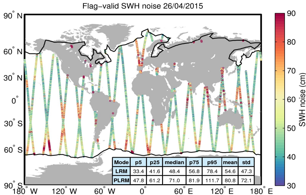
Figure 18. Geographical distribution of flag-valid 20-Hz SWH measurement noise over oceans and lakes for 26/04/2015. The statistical values shown in the table refer to the SWH noise and are calculated separately for LRM and PLRM regions. Measurements taken over polar polygons have been excluded from the computation of the statistical values. The black lines mark the outer limit of the Arctic and Antarctic polar polygons.
