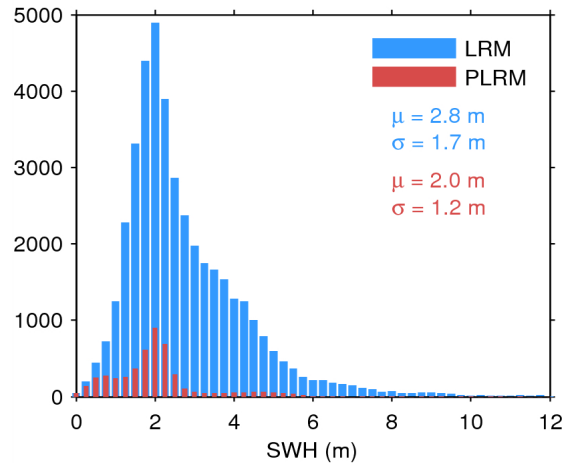
Figure 17. Histogram of flag-valid SWH over oceans and lakes for LRM (blue) and PLRM (red) for 26/04/2015. The mean ( \mu ) and standard deviation ( \sigma ) are also shown. Note that values larger than 12 m are excluded from the histogram for the sake of readability but not from the computation of \mu and \sigma .
