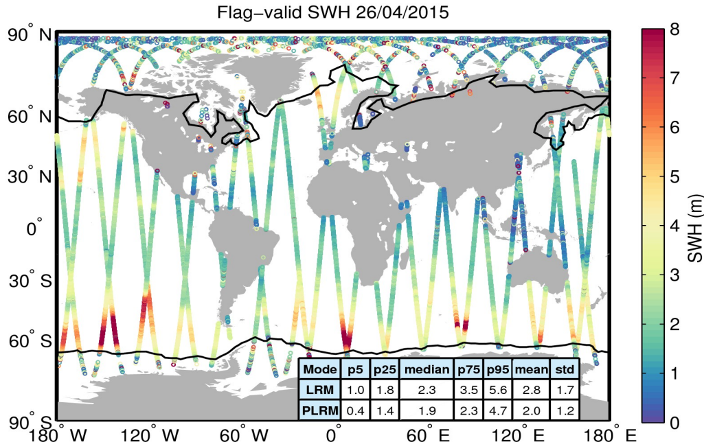
Figure 15. Geographical distribution of flag-valid SWH data over oceans and lakes for 26/04/2015. The statistical values shown in the table refer to the SWH in m and are calculated separately for LRM and PLRM regions. Measurements taken over polar polygons have been excluded from the computation of the statistical values. The black lines mark the outer limit of the Arctic and Antarctic polar polygons.
