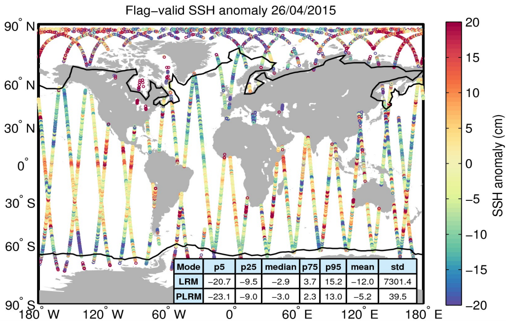
Figure 5. Geographical distribution of flag-valid 1-Hz SSH anomaly data over oceans and lakes for 26/04/2015. The statistical values shown in the table refer to the SSH anomaly in cm and are calculated separately for LRM and PLRM regions. Measurements taken over polar polygons have been excluded from the computation of the statistical values. The black lines mark the outer limit of the Arctic and Antarctic polar polygons.
