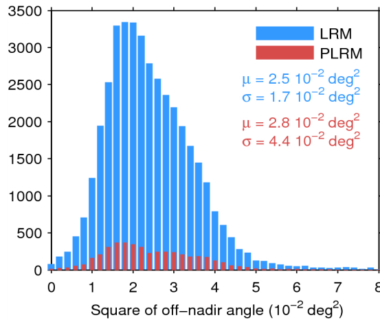
Figure 39. Histogram of flag-valid mispointing over oceans and lakes for LRM (blue) and PLRM (red) for 26/04/2015. Only positive values have been considered. The mean ( \mu ) and standard deviation ( \sigma ) are also shown. Note that values larger than 8 \cdot 10^{-2} \text{ deg}^2 are excluded from the histogram for the sake of readability but not from the computation of \mu and \sigma .
