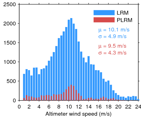
Figure 33. Histogram of flag-valid wind over oceans and lakes for LRM (blue) and PLRM (red) for 26/04/2015. The mean ( \mu ) and standard deviation ( \sigma ) are also shown. Note that values larger than 24 m/s are excluded from the histogram for the sake of readability but not from the computation of \mu and \sigma .
