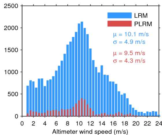
Figure 35. Histogram of science-valid wind over oceans and lakes for LRM (blue) and PLRM (red) for 26/04/2015. The mean ( \mu ) and standard deviation ( \sigma ) are also shown. Note that values larger than 24 m/s are excluded from the histogram for the sake of readability but not from the computation of \mu and \sigma .
