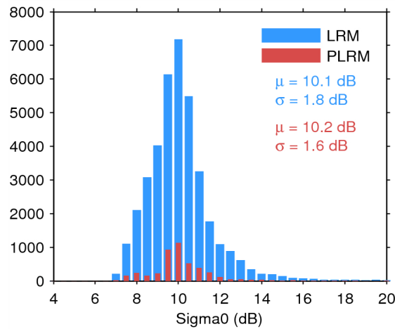
Figure 28. Histogram of science-valid sigma0 over oceans and lakes for LRM (blue) and PLRM (red) for 26/04/2015. The mean ( \mu ) and standard deviation ( \sigma ) are also shown. Note that values outside [4 20] dB are excluded from the histogram for the sake of readability but not from the computation of \mu and \sigma .
