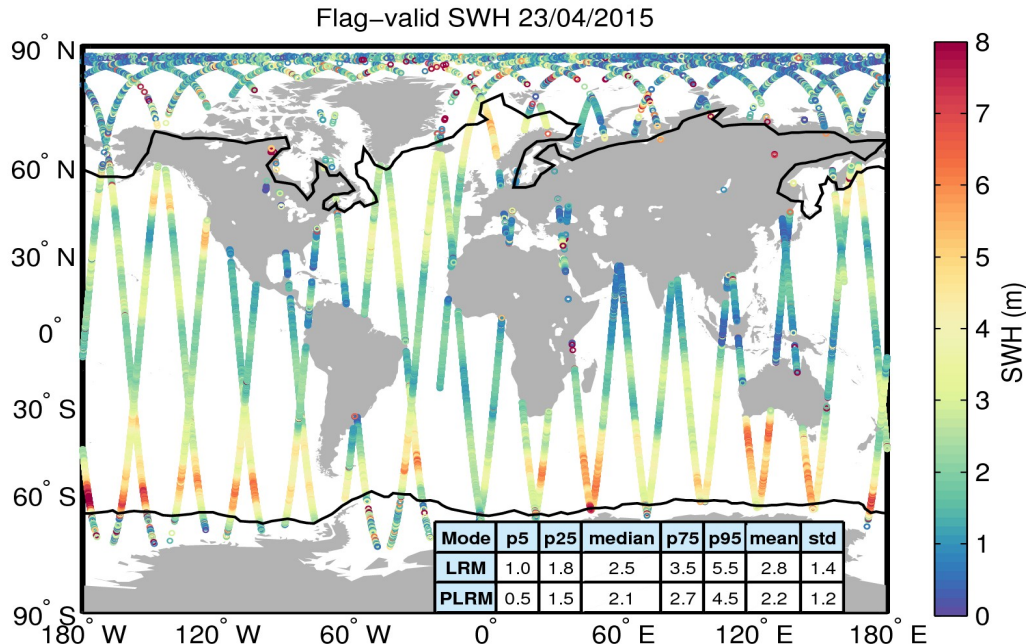
Figure 15. Geographical distribution of flag-valid SWH data over oceans and lakes for 23/04/2015. The statistical values shown in the table refer to the SWH in m and are calculated separately for LRM and PLRM regions. Measurements taken over polar polygons have been excluded from the computation of the statistical values. The black lines mark the outer limit of the Arctic and Antarctic polar polygons.
