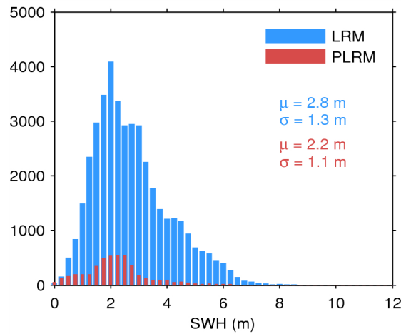
Figure 20. Histogram of science-valid SWH over oceans and lakes for LRM (blue) and PLRM (red) for 23/04/2015. The mean ( \mu ) and standard deviation ( \sigma ) are also shown. Note that values larger than 12 m are excluded from the histogram for the sake of readability but not from the computation of \mu and \sigma .
