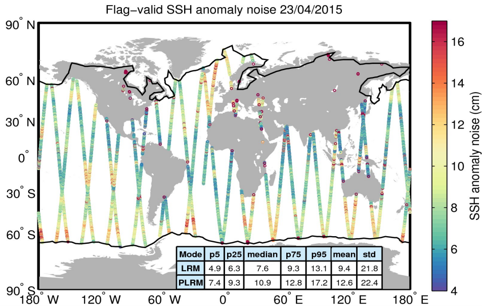
Figure 8. Geographical distribution of flag-valid 20-Hz SSH anomaly measurement noise over oceans and lakes for 23/04/2015. The statistical values shown in the table refer to the SSH anomaly noise and are calculated separately for LRM and PLRM regions. Measurements taken over polar polygons have been excluded from the computation of the statistical values. The black lines mark the outer limit of the Arctic and Antarctic polar polygons.
