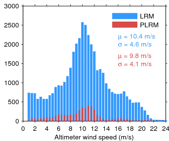
Figure 33. Histogram of flag-valid wind over oceans and lakes for LRM (blue) and PLRM (red) for 23/04/2015. The mean ( \mu ) and standard deviation ( \sigma ) are also shown. Note that values larger than 24 m/s are excluded from the histogram for the sake of readability but not from the computation of \mu and \sigma .
