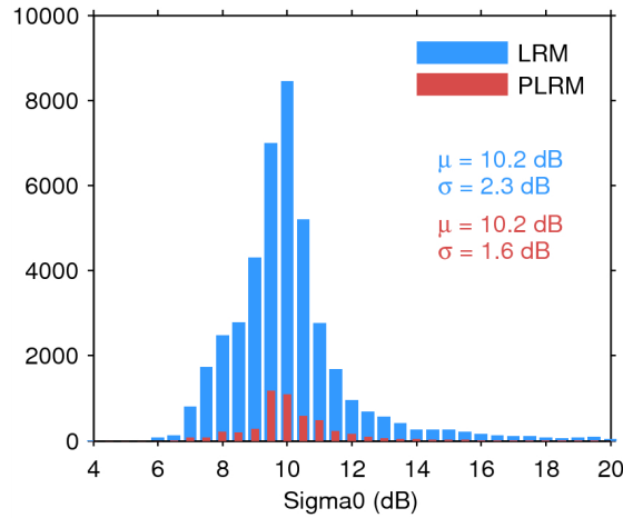
Figure 25. Histogram of flag-valid sigma0 over oceans and lakes for LRM (blue) and PLRM (red) for 23/04/2015. The mean ( \mu ) and standard deviation ( \sigma ) are also shown. Note that values outside [4 20] dB are excluded from the histogram for the sake of readability but not from the computation of \mu and \sigma .
