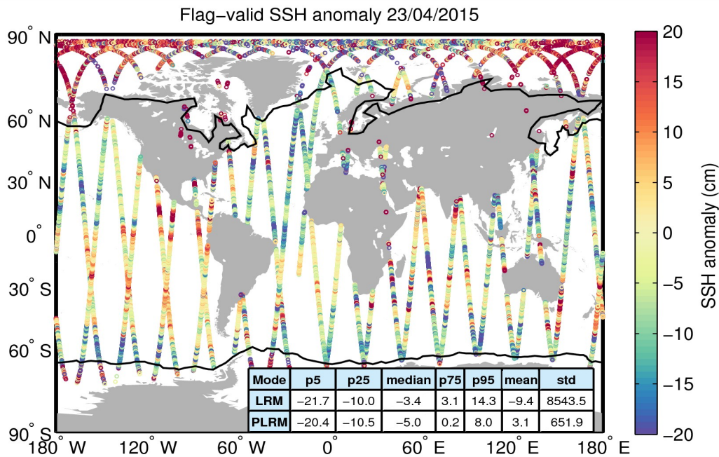
Figure 5. Geographical distribution of flag-valid 1-Hz SSH anomaly data over oceans and lakes for 23/04/2015. The statistical values shown in the table refer to the SSH anomaly in cm and are calculated separately for LRM and PLRM regions. Measurements taken over polar polygons have been excluded from the computation of the statistical values. The black lines mark the outer limit of the Arctic and Antarctic polar polygons.
