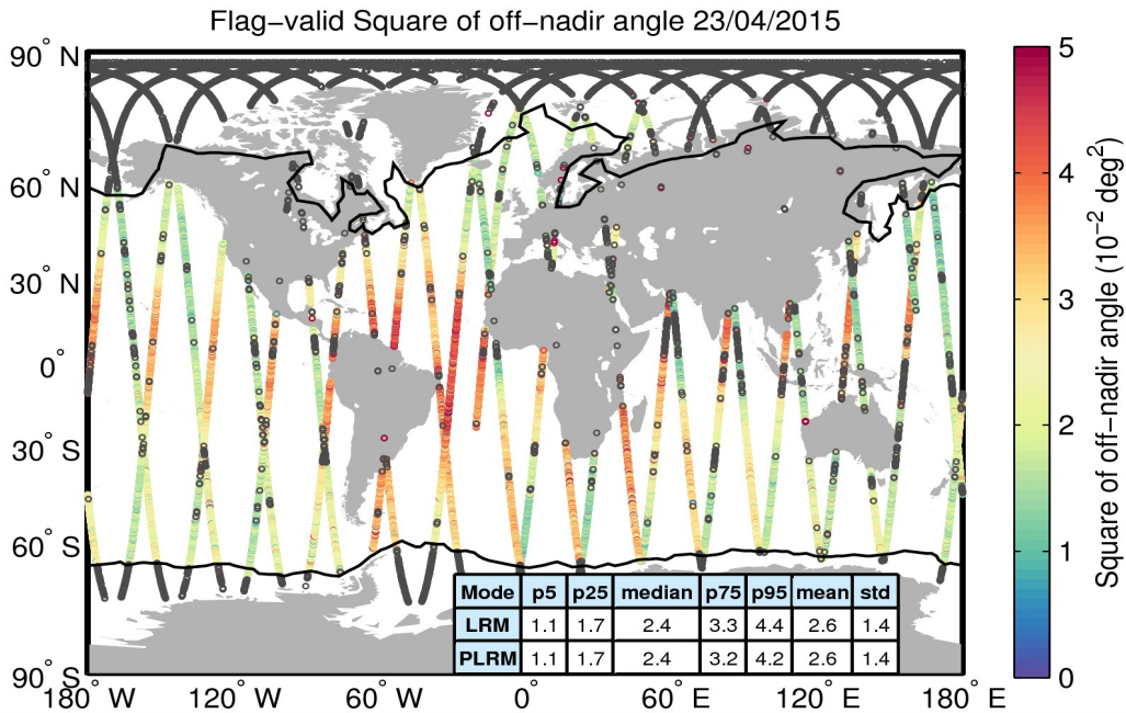
Figure 37. Geographical distribution of flag-valid mispointing data over oceans and lakes for 23/04/2015. The statistical values shown in the table refer to the mispointing in 10^{-2} \text{ deg}^2 and are calculated separately for LRM and PLRM regions. Measurements taken over polar polygons have been excluded from the computation of the statistical values. The black lines mark the outer limit of the Arctic and Antarctic polar polygons. Gray circles denote negative values.
