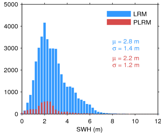
Figure 17. Histogram of flag-valid SWH over oceans and lakes for LRM (blue) and PLRM (red) for 23/04/2015. The mean ( \mu ) and standard deviation ( \sigma ) are also shown. Note that values larger than 12 m are excluded from the histogram for the sake of readability but not from the computation of \mu and \sigma .
