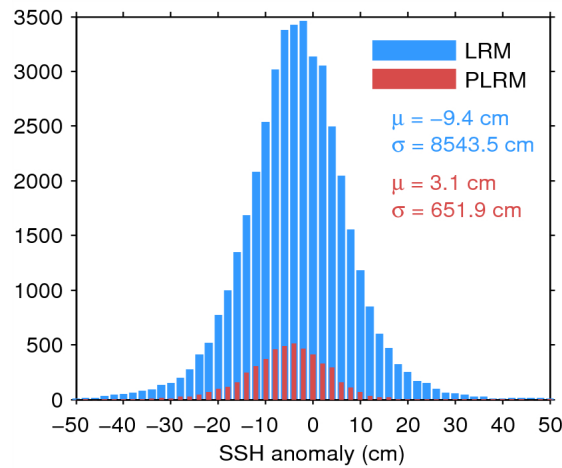
Figure 7. Histogram of flag-valid SSH anomaly over oceans and lakes for LRM (blue) and PLRM (red) for 23/04/2015. The mean ( \mu ) and standard deviation ( \sigma ) are also shown. Note that values outside [-50\ 50] cm are excluded from the histogram for the sake of readability but not from the computation of \mu and \sigma .
