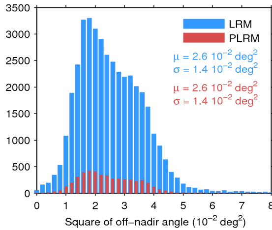
Figure 39. Histogram of flag-valid mispointing over oceans and lakes for LRM (blue) and PLRM (red) for 23/04/2015. Only positive values have been considered. The mean ( \mu ) and standard deviation ( \sigma ) are also shown. Note that values larger than 8 \cdot 10^{-2} \text{ deg}^2 are excluded from the histogram for the sake of readability but not from the computation of \mu and \sigma .
