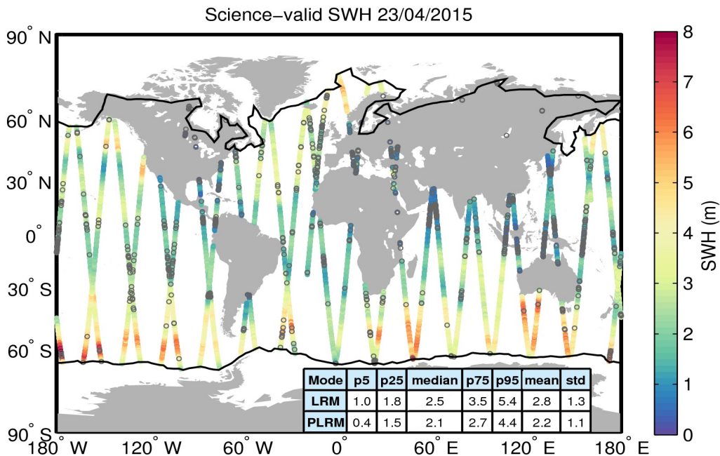
Figure 19. Geographical distribution of science-valid SWH data over oceans and lakes for 23/04/2015. The statistical values shown in the table refer to the SWH in m and are calculated separately for LRM and PLRM regions. The black lines mark the outer limit of the Arctic and Antarctic polar polygons. Gray circles denote records that have been rejected based on the editing criteria described in Table 3.
