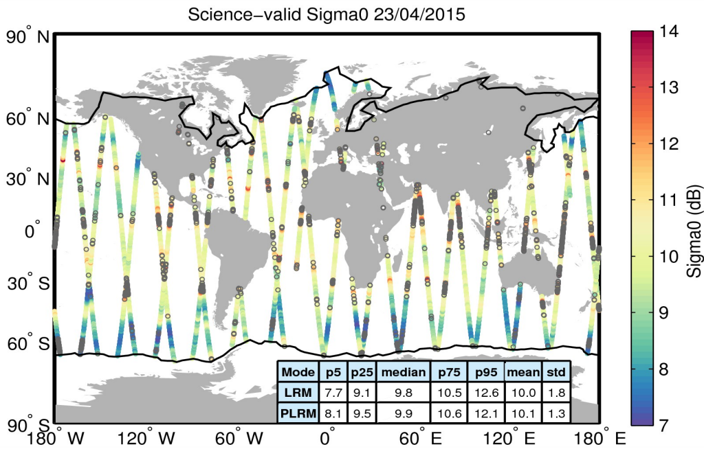
Figure 27. Geographical distribution of science-valid sigma0 data over oceans and lakes for 23/04/2015. The statistical values shown in the table refer to the sigma0 in dB and are calculated separately for LRM and PLRM regions. The black lines mark the outer limit of the Arctic and Antarctic polar polygons. Gray circles denote records that have been rejected based on the editing criteria described in Table 4.
