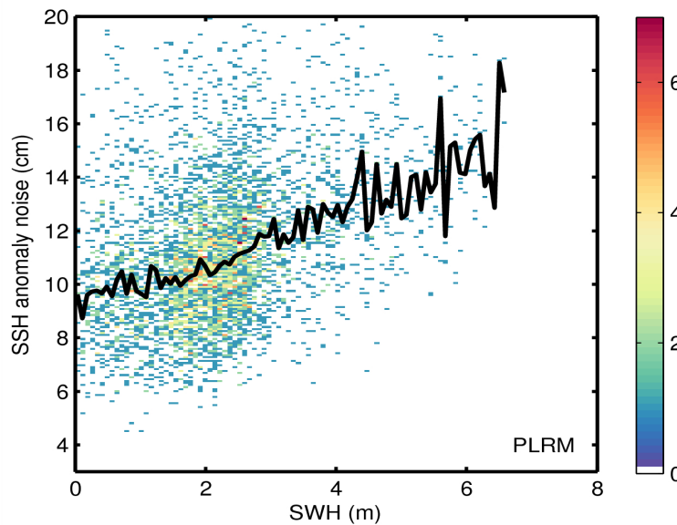
Figure 9. 2D histogram showing flag-valid SSH anomaly noise as a function of SWH for LRM (top) and PLRM (bottom) for 23/04/2015. The black line denotes the median SSH anomaly as a function of SWH.
