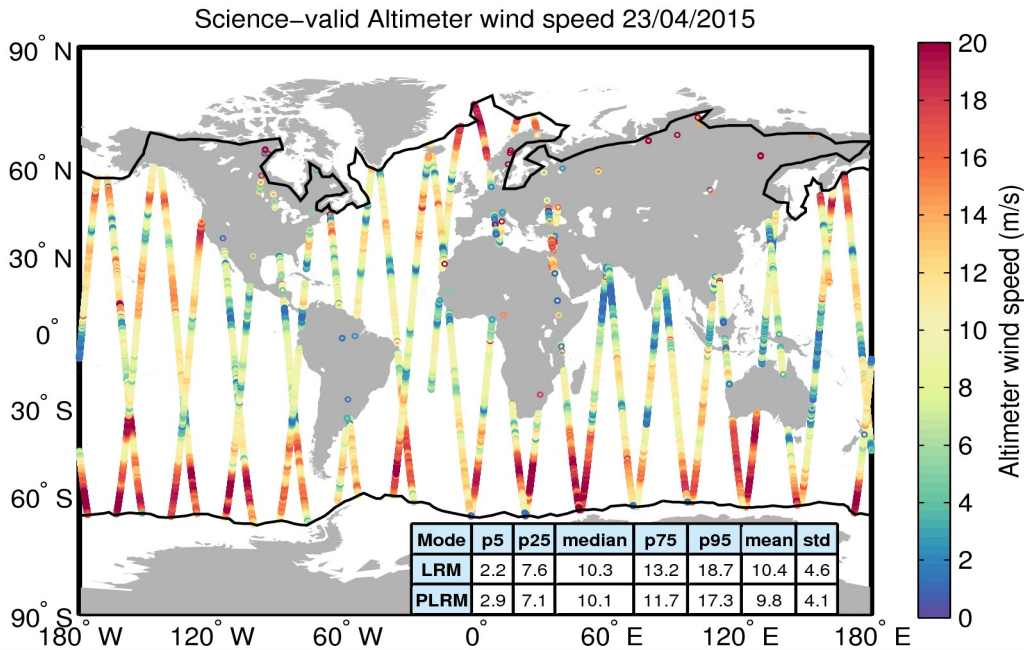
Figure 34. Geographical distribution of science-valid wind data over oceans and lakes for 23/04/2015. The statistical values shown in the table refer to the wind in m/s and are calculated separately for LRM and PLRM regions. The black lines mark the outer limit of the Arctic and Antarctic polar polygons. Gray circles denote records that have been rejected based on the editing criteria described in Table 5.
