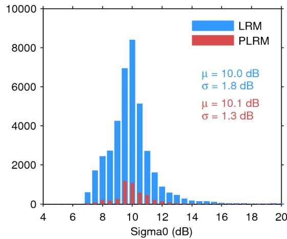
Figure 28. Histogram of science-valid sigma0 over oceans and lakes for LRM (blue) and PLRM (red) for 23/04/2015. The mean ( \mu ) and standard deviation ( \sigma ) are also shown. Note that values outside [4 20] dB are excluded from the histogram for the sake of readability but not from the computation of \mu and \sigma .
