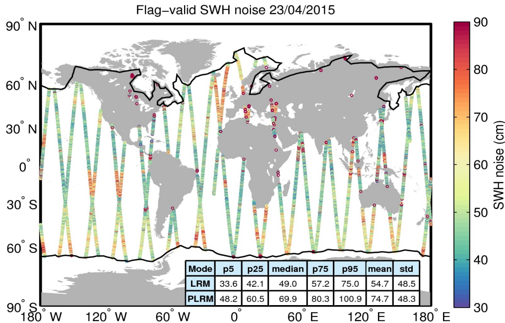
Figure 18. Geographical distribution of flag-valid 20-Hz SWH measurement noise over oceans and lakes for 23/04/2015. The statistical values shown in the table refer to the SWH noise and are calculated separately for LRM and PLRM regions. Measurements taken over polar polygons have been excluded from the computation of the statistical values. The black lines mark the outer limit of the Arctic and Antarctic polar polygons.
