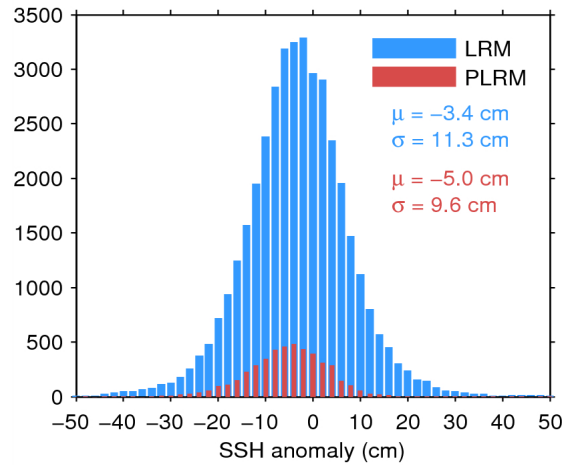
Figure 11. Histogram of science-valid SSH anomaly over oceans and lakes for LRM (blue) and PLRM (red) for 23/04/2015. The mean ( \mu ) and standard deviation ( \sigma ) are also shown. Note that values outside [-50 50] cm are excluded from the histogram for the sake of readability but not from the computation of \mu and \sigma .
