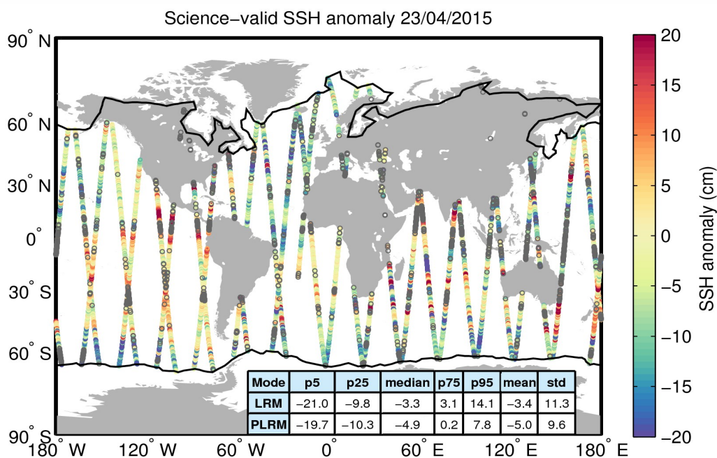
Figure 10. Geographical distribution of science-valid SSH anomaly data over oceans and lakes for 23/04/2015. The statistical values shown in the table refer to the SSH anomaly in cm and are calculated separately for LRM and PLRM regions. The black lines mark the outer limit of the Arctic and Antarctic polar polygons. Gray circles denote records that have been rejected based on the editing criteria described in Table 2.
