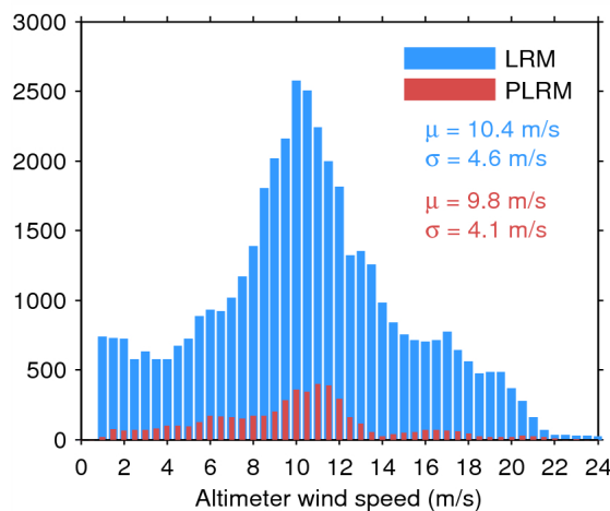
Figure 35. Histogram of science-valid wind over oceans and lakes for LRM (blue) and PLRM (red) for 23/04/2015. The mean ( \mu ) and standard deviation ( \sigma ) are also shown. Note that values larger than 24 m/s are excluded from the histogram for the sake of readability but not from the computation of \mu and \sigma .
