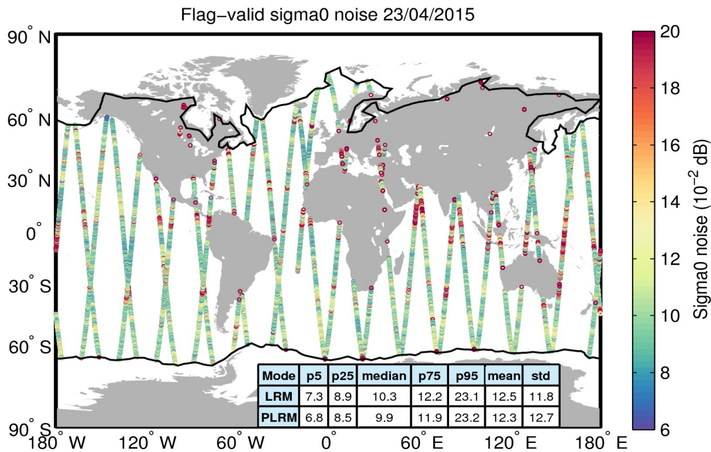
Figure 26. Geographical distribution of flag-valid 20-Hz sigma0 measurement noise over oceans and lakes for 23/04/2015. The statistical values shown in the table refer to the sigma0 noise and are calculated separately for LRM and PLRM regions. Measurements taken over polar polygons have been excluded from the computation of the statistical values. The black lines mark the outer limit of the Arctic and Antarctic polar polygons.
