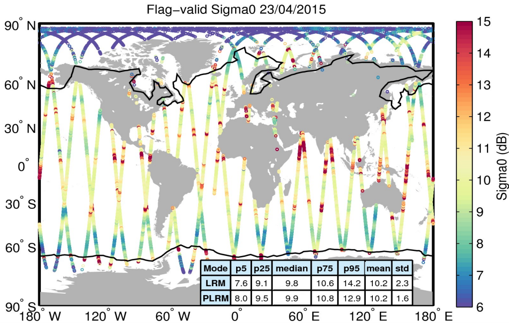
Figure 23. Geographical distribution of flag-valid sigma0 data over oceans and lakes for 23/04/2015. The statistical values shown in the table refer to the sigma0 in dB and are calculated separately for LRM and PLRM regions. Measurements taken over polar polygons have been excluded from the computation of the statistical values. The black lines mark the outer limit of the Arctic and Antarctic polar polygons.
