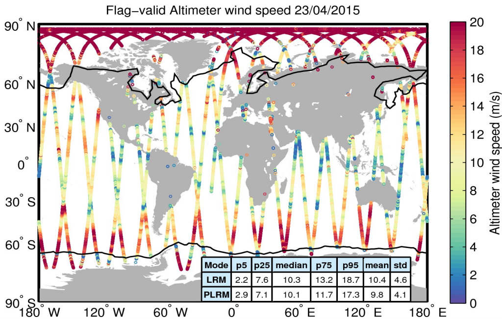
Figure 31. Geographical distribution of flag-valid wind data over oceans and lakes for 23/04/2015. The statistical values shown in the table refer to the wind in m/s and are calculated separately for LRM and PLRM regions. Measurements taken over polar polygons have been excluded from the computation of the statistical values. The black lines mark the outer limit of the Arctic and Antarctic polar polygons.
