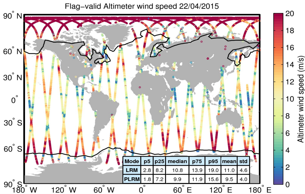
Figure 31. Geographical distribution of flag-valid wind data over oceans and lakes for 22/04/2015. The statistical values shown in the table refer to the wind in m/s and are calculated separately for LRM and PLRM regions. Measurements taken over polar polygons have been excluded from the computation of the statistical values. The black lines mark the outer limit of the Arctic and Antarctic polar polygons.
