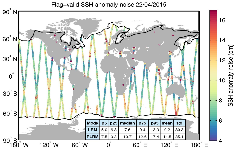
Figure 8. Geographical distribution of flag-valid 20-Hz SSH anomaly measurement noise over oceans and lakes for 22/04/2015. The statistical values shown in the table refer to the SSH anomaly noise and are calculated separately for LRM and PLRM regions. Measurements taken over polar polygons have been excluded from the computation of the statistical values. The black lines mark the outer limit of the Arctic and Antarctic polar polygons.
