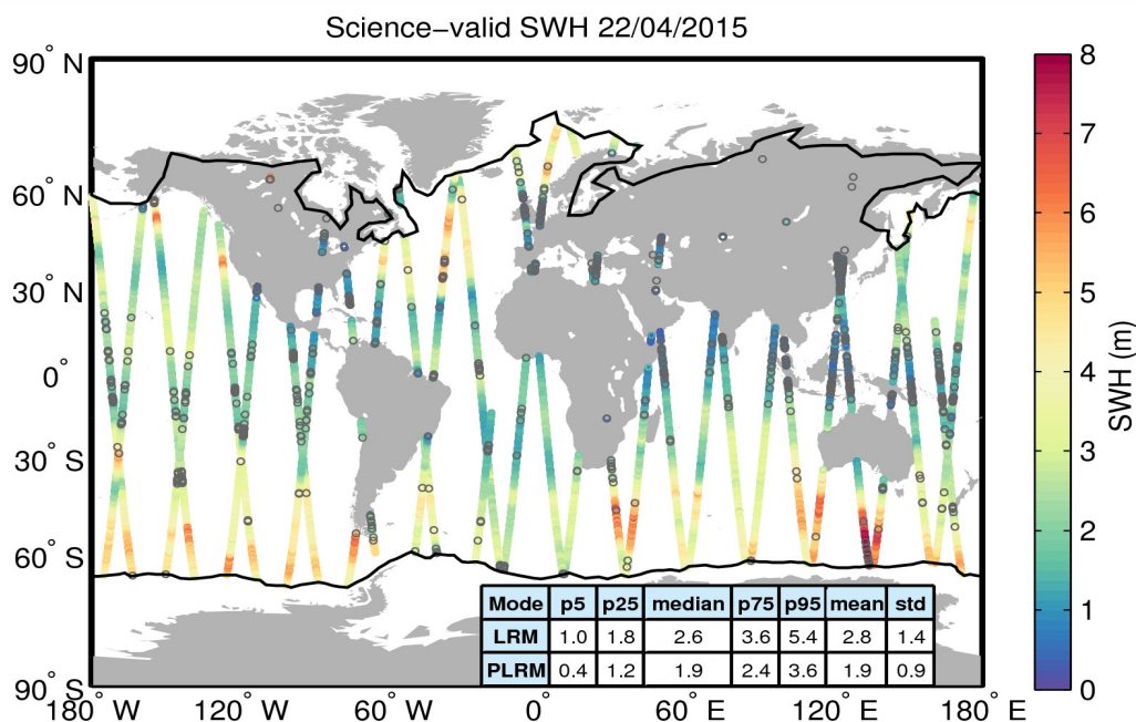
Figure 19. Geographical distribution of science-valid SWH data over oceans and lakes for 22/04/2015. The statistical values shown in the table refer to the SWH in m and are calculated separately for LRM and PLRM regions. The black lines mark the outer limit of the Arctic and Antarctic polar polygons. Gray circles denote records that have been rejected based on the editing criteria described in Table 3.
