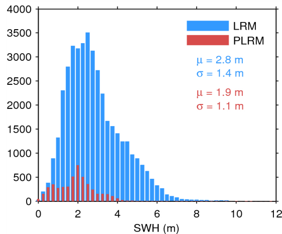
Figure 17. Histogram of flag-valid SWH over oceans and lakes for LRM (blue) and PLRM (red) for 22/04/2015. The mean ( \mu ) and standard deviation ( \sigma ) are also shown. Note that values larger than 12 m are excluded from the histogram for the sake of readability but not from the computation of \mu and \sigma .
