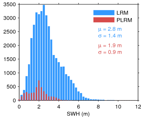
Figure 20. Histogram of science-valid SWH over oceans and lakes for LRM (blue) and PLRM (red) for 22/04/2015. The mean ( \mu ) and standard deviation ( \sigma ) are also shown. Note that values larger than 12 m are excluded from the histogram for the sake of readability but not from the computation of \mu and \sigma .
