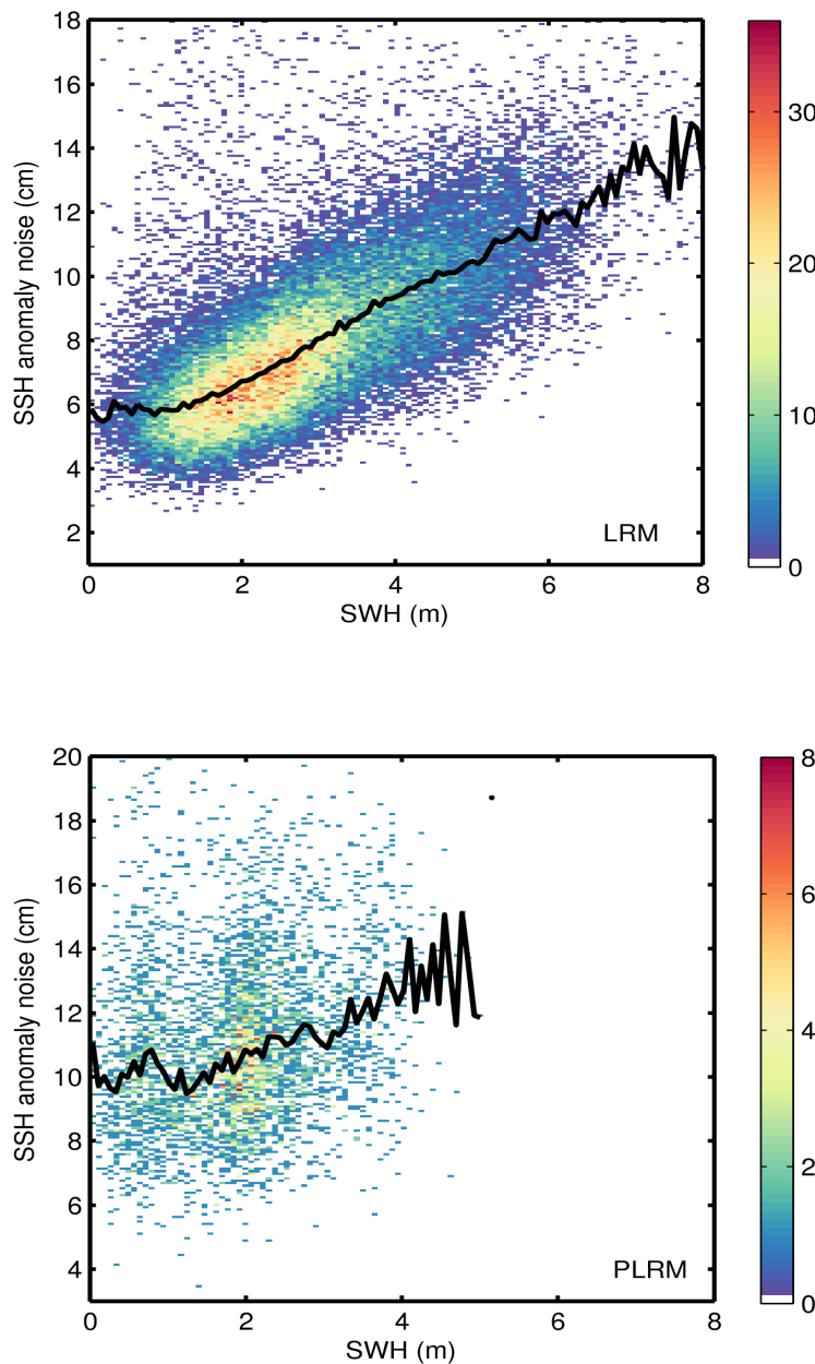
Figure 9. 2D histogram showing flag-valid SSH anomaly noise as a function of SWH for LRM (top) and PLRM (bottom) for 22/04/2015. The black line denotes the median SSH anomaly as a function of SWH.
