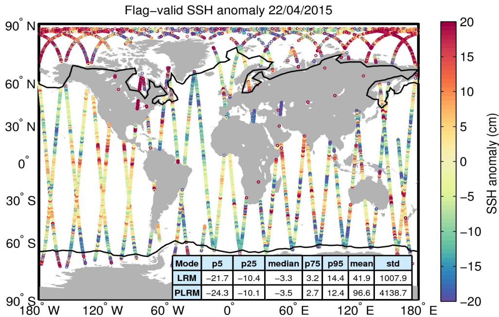
Figure 5. Geographical distribution of flag-valid 1-Hz SSH anomaly data over oceans and lakes for 22/04/2015. The statistical values shown in the table refer to the SSH anomaly in cm and are calculated separately for LRM and PLRM regions. Measurements taken over polar polygons have been excluded from the computation of the statistical values. The black lines mark the outer limit of the Arctic and Antarctic polar polygons.
