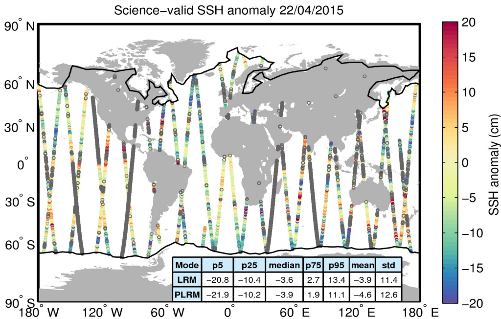
Figure 10. Geographical distribution of science-valid SSH anomaly data over oceans and lakes for 22/04/2015. The statistical values shown in the table refer to the SSH anomaly in cm and are calculated separately for LRM and PLRM regions. The black lines mark the outer limit of the Arctic and Antarctic polar polygons. Gray circles denote records that have been rejected based on the editing criteria described in Table 2.
