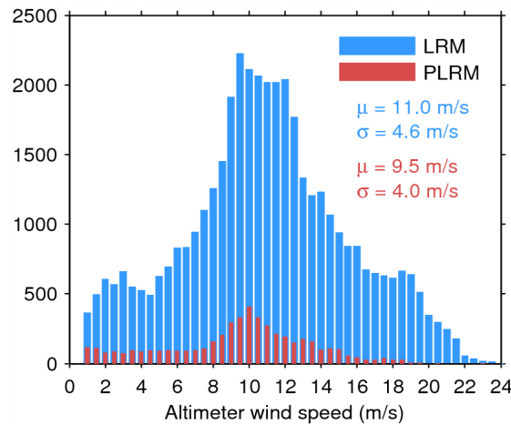
Figure 33. Histogram of flag-valid wind over oceans and lakes for LRM (blue) and PLRM (red) for 22/04/2015. The mean ( \mu ) and standard deviation ( \sigma ) are also shown. Note that values larger than 24 m/s are excluded from the histogram for the sake of readability but not from the computation of \mu and \sigma .
