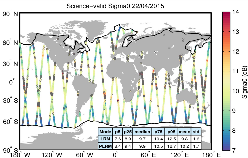
Figure 27. Geographical distribution of science-valid sigma0 data over oceans and lakes for 22/04/2015. The statistical values shown in the table refer to the sigma0 in dB and are calculated separately for LRM and PLRM regions. The black lines mark the outer limit of the Arctic and Antarctic polar polygons. Gray circles denote records that have been rejected based on the editing criteria described in Table 4.
