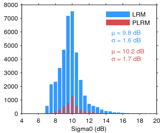
Figure 28. Histogram of science-valid sigma0 over oceans and lakes for LRM (blue) and PLRM (red) for 22/04/2015. The mean ( \mu ) and standard deviation ( \sigma ) are also shown. Note that values outside [4 20] dB are excluded from the histogram for the sake of readability but not from the computation of \mu and \sigma .
