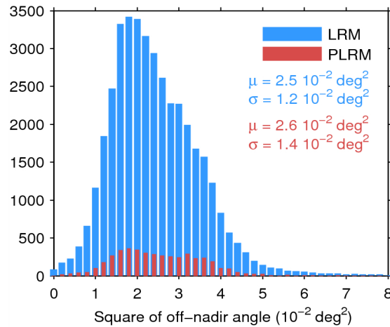
Figure 39. Histogram of flag-valid mispointing over oceans and lakes for LRM (blue) and PLRM (red) for 22/04/2015. Only positive values have been considered. The mean ( \mu ) and standard deviation ( \sigma ) are also shown. Note that values larger than 8 \cdot 10^{-2} \text{ deg}^2 are excluded from the histogram for the sake of readability but not from the computation of \mu and \sigma .
