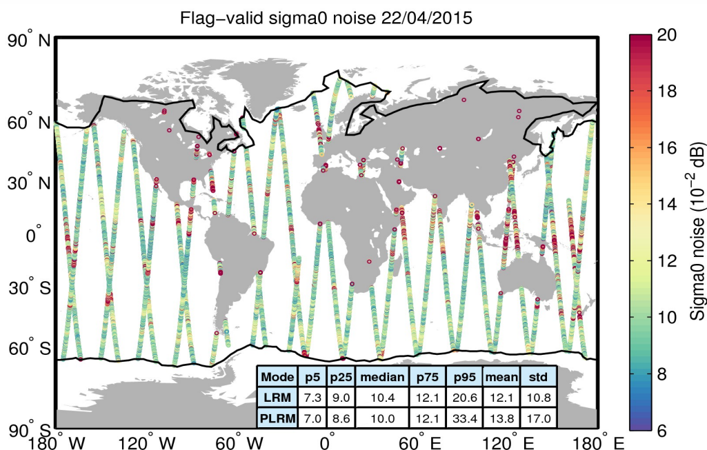
Figure 26. Geographical distribution of flag-valid 20-Hz sigma0 measurement noise over oceans and lakes for 22/04/2015. The statistical values shown in the table refer to the sigma0 noise and are calculated separately for LRM and PLRM regions. Measurements taken over polar polygons have been excluded from the computation of the statistical values. The black lines mark the outer limit of the Arctic and Antarctic polar polygons.
