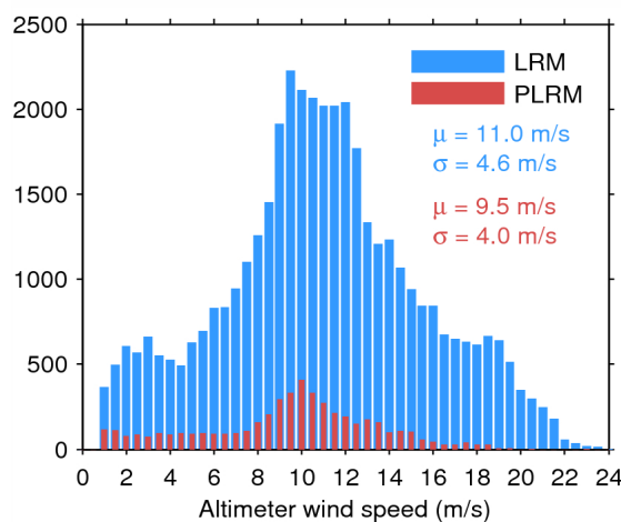
Figure 35. Histogram of science-valid wind over oceans and lakes for LRM (blue) and PLRM (red) for 22/04/2015. The mean ( \mu ) and standard deviation ( \sigma ) are also shown. Note that values larger than 24 m/s are excluded from the histogram for the sake of readability but not from the computation of \mu and \sigma .
