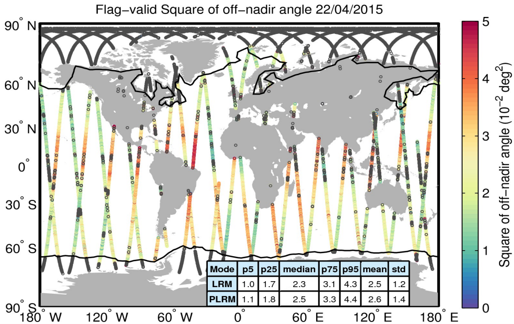
Figure 37. Geographical distribution of flag-valid mispointing data over oceans and lakes for 22/04/2015. The statistical values shown in the table refer to the mispointing in 10^{-2} \text{ deg}^2 and are calculated separately for LRM and PLRM regions. Measurements taken over polar polygons have been excluded from the computation of the statistical values. The black lines mark the outer limit of the Arctic and Antarctic polar polygons. Gray circles denote negative values.
