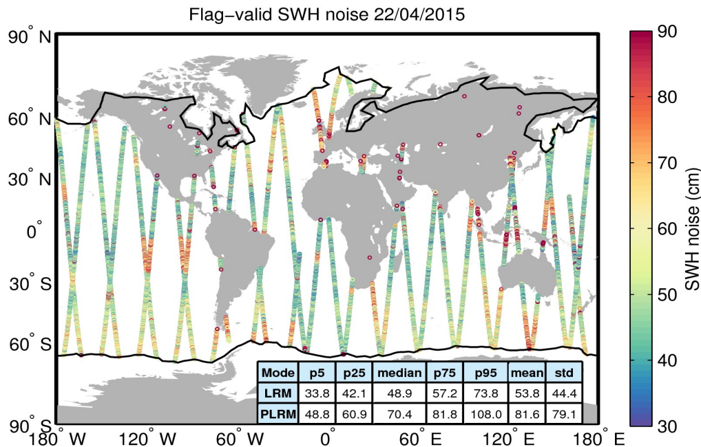
Figure 18. Geographical distribution of flag-valid 20-Hz SWH measurement noise over oceans and lakes for 22/04/2015. The statistical values shown in the table refer to the SWH noise and are calculated separately for LRM and PLRM regions. Measurements taken over polar polygons have been excluded from the computation of the statistical values. The black lines mark the outer limit of the Arctic and Antarctic polar polygons.
