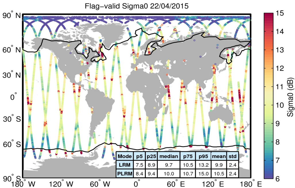
Figure 23. Geographical distribution of flag-valid sigma0 data over oceans and lakes for 22/04/2015. The statistical values shown in the table refer to the sigma0 in dB and are calculated separately for LRM and PLRM regions. Measurements taken over polar polygons have been excluded from the computation of the statistical values. The black lines mark the outer limit of the Arctic and Antarctic polar polygons.
