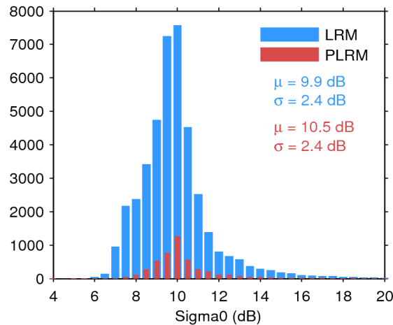
Figure 25. Histogram of flag-valid sigma0 over oceans and lakes for LRM (blue) and PLRM (red) for 22/04/2015. The mean ( \mu ) and standard deviation ( \sigma ) are also shown. Note that values outside [4 20] dB are excluded from the histogram for the sake of readability but not from the computation of \mu and \sigma .
