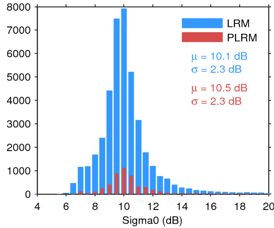
Figure 25. Histogram of flag-valid sigma0 over oceans and lakes for LRM (blue) and PLRM (red) for 21/04/2015. The mean ( \mu ) and standard deviation ( \sigma ) are also shown. Note that values outside [4 20] dB are excluded from the histogram for the sake of readability but not from the computation of \mu and \sigma .
