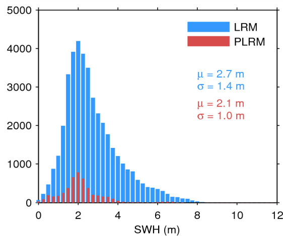
Figure 20. Histogram of science-valid SWH over oceans and lakes for LRM (blue) and PLRM (red) for 21/04/2015. The mean ( \mu ) and standard deviation ( \sigma ) are also shown. Note that values larger than 12 m are excluded from the histogram for the sake of readability but not from the computation of \mu and \sigma .
