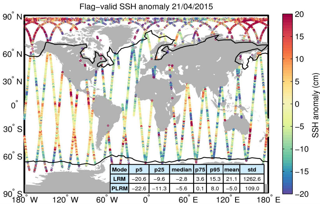
Figure 5. Geographical distribution of flag-valid 1-Hz SSH anomaly data over oceans and lakes for 21/04/2015. The statistical values shown in the table refer to the SSH anomaly in cm and are calculated separately for LRM and PLRM regions. Measurements taken over polar polygons have been excluded from the computation of the statistical values. The black lines mark the outer limit of the Arctic and Antarctic polar polygons.
