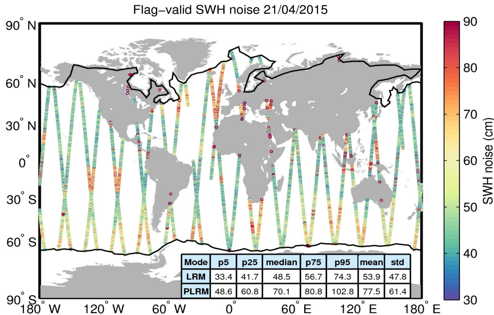
Figure 18. Geographical distribution of flag-valid 20-Hz SWH measurement noise over oceans and lakes for 21/04/2015. The statistical values shown in the table refer to the SWH noise and are calculated separately for LRM and PLRM regions. Measurements taken over polar polygons have been excluded from the computation of the statistical values. The black lines mark the outer limit of the Arctic and Antarctic polar polygons.
