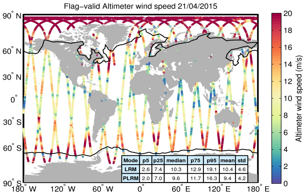
Figure 31. Geographical distribution of flag-valid wind data over oceans and lakes for 21/04/2015. The statistical values shown in the table refer to the wind in m/s and are calculated separately for LRM and PLRM regions. Measurements taken over polar polygons have been excluded from the computation of the statistical values. The black lines mark the outer limit of the Arctic and Antarctic polar polygons.
