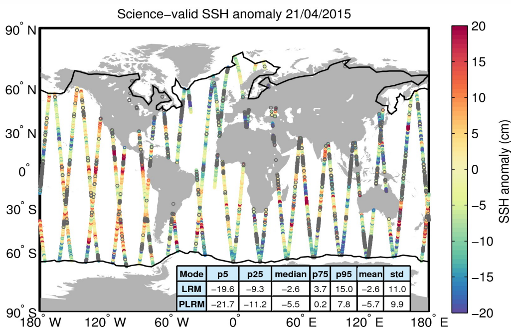
Figure 10. Geographical distribution of science-valid SSH anomaly data over oceans and lakes for 21/04/2015. The statistical values shown in the table refer to the SSH anomaly in cm and are calculated separately for LRM and PLRM regions. The black lines mark the outer limit of the Arctic and Antarctic polar polygons. Gray circles denote records that have been rejected based on the editing criteria described in Table 2.
