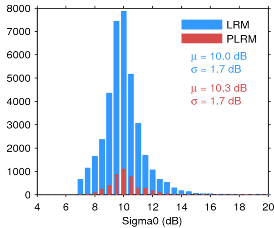
Figure 28. Histogram of science-valid sigma0 over oceans and lakes for LRM (blue) and PLRM (red) for 21/04/2015. The mean ( \mu ) and standard deviation ( \sigma ) are also shown. Note that values outside [4 20] dB are excluded from the histogram for the sake of readability but not from the computation of \mu and \sigma .
