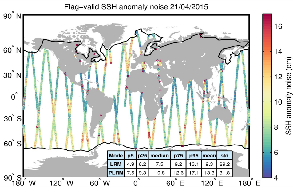
Figure 8. Geographical distribution of flag-valid 20-Hz SSH anomaly measurement noise over oceans and lakes for 21/04/2015. The statistical values shown in the table refer to the SSH anomaly noise and are calculated separately for LRM and PLRM regions. Measurements taken over polar polygons have been excluded from the computation of the statistical values. The black lines mark the outer limit of the Arctic and Antarctic polar polygons.
