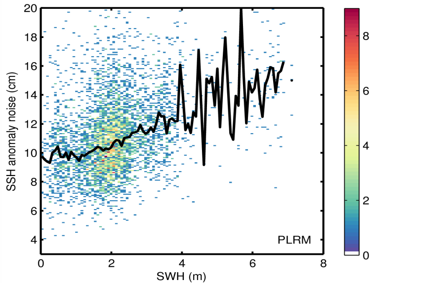
Figure 9. 2D histogram showing flag-valid SSH anomaly noise as a function of SWH for LRM (top) and PLRM (bottom) for 21/04/2015. The black line denotes the median SSH anomaly as a function of SWH.
