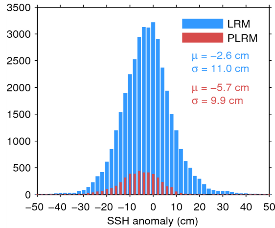
Figure 11. Histogram of science-valid SSH anomaly over oceans and lakes for LRM (blue) and PLRM (red) for 21/04/2015. The mean ( \mu ) and standard deviation ( \sigma ) are also shown. Note that values outside [-50 50] cm are excluded from the histogram for the sake of readability but not from the computation of \mu and \sigma .
