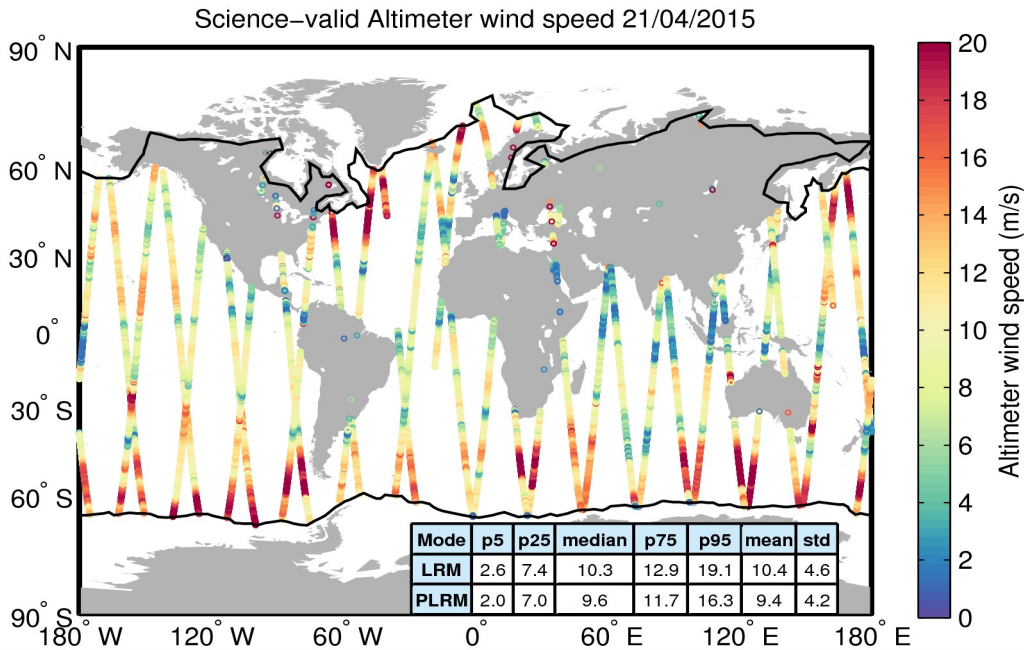
Figure 34. Geographical distribution of science-valid wind data over oceans and lakes for 21/04/2015. The statistical values shown in the table refer to the wind in m/s and are calculated separately for LRM and PLRM regions. The black lines mark the outer limit of the Arctic and Antarctic polar polygons. Gray circles denote records that have been rejected based on the editing criteria described in Table 5.
