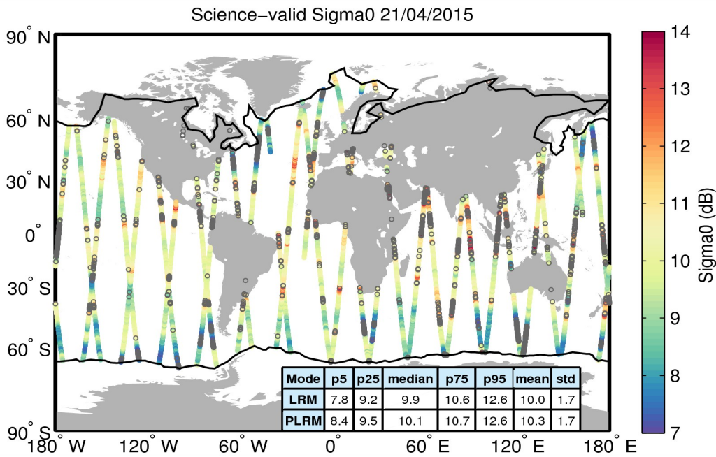
Figure 27. Geographical distribution of science-valid sigma0 data over oceans and lakes for 21/04/2015. The statistical values shown in the table refer to the sigma0 in dB and are calculated separately for LRM and PLRM regions. The black lines mark the outer limit of the Arctic and Antarctic polar polygons. Gray circles denote records that have been rejected based on the editing criteria described in Table 4.
