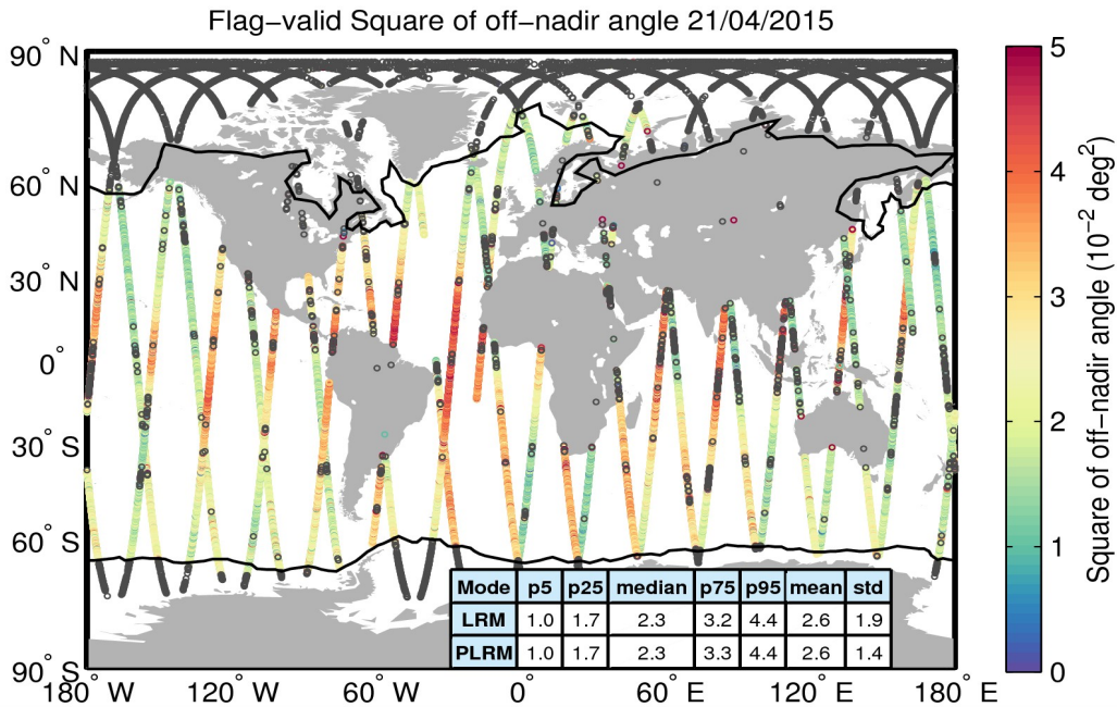
Figure 37. Geographical distribution of flag-valid mispointing data over oceans and lakes for 21/04/2015. The statistical values shown in the table refer to the mispointing in 10^{-2} \text{ deg}^2 and are calculated separately for LRM and PLRM regions. Measurements taken over polar polygons have been excluded from the computation of the statistical values. The black lines mark the outer limit of the Arctic and Antarctic polar polygons. Gray circles denote negative values.
