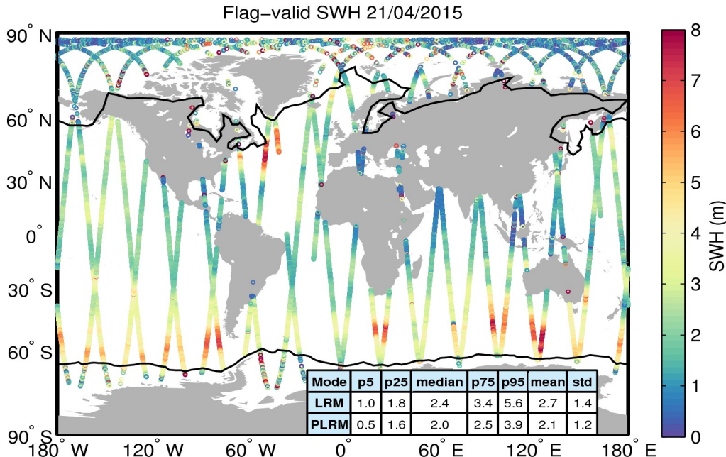
Figure 15. Geographical distribution of flag-valid SWH data over oceans and lakes for 21/04/2015. The statistical values shown in the table refer to the SWH in m and are calculated separately for LRM and PLRM regions. Measurements taken over polar polygons have been excluded from the computation of the statistical values. The black lines mark the outer limit of the Arctic and Antarctic polar polygons.
