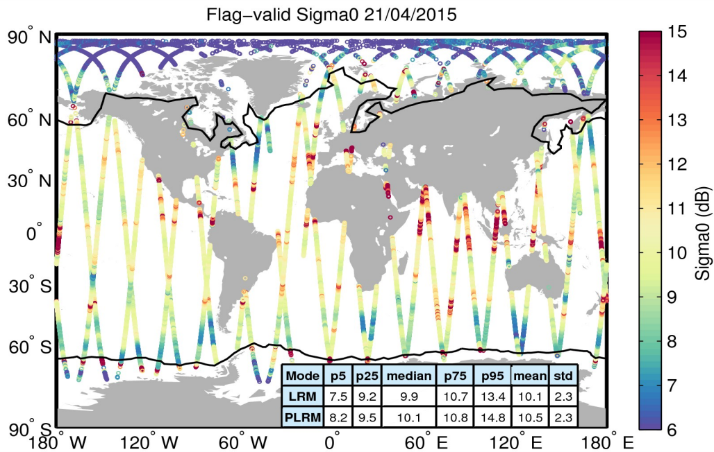
Figure 23. Geographical distribution of flag-valid sigma0 data over oceans and lakes for 21/04/2015. The statistical values shown in the table refer to the sigma0 in dB and are calculated separately for LRM and PLRM regions. Measurements taken over polar polygons have been excluded from the computation of the statistical values. The black lines mark the outer limit of the Arctic and Antarctic polar polygons.
