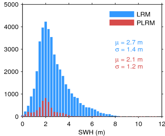
Figure 17. Histogram of flag-valid SWH over oceans and lakes for LRM (blue) and PLRM (red) for 21/04/2015. The mean ( \mu ) and standard deviation ( \sigma ) are also shown. Note that values larger than 12 m are excluded from the histogram for the sake of readability but not from the computation of \mu and \sigma .
