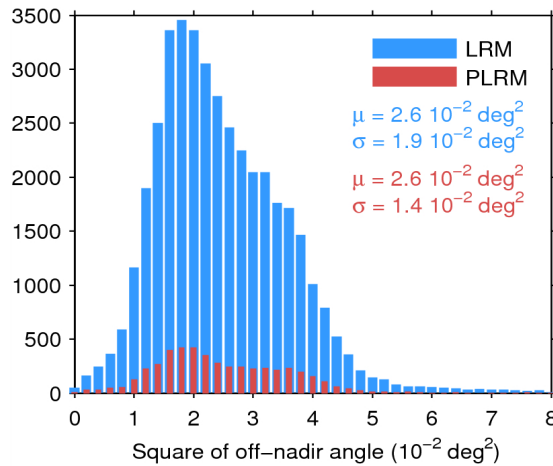
Figure 39. Histogram of flag-valid mispointing over oceans and lakes for LRM (blue) and PLRM (red) for 21/04/2015. Only positive values have been considered. The mean ( \mu ) and standard deviation ( \sigma ) are also shown. Note that values larger than 8 \cdot 10^{-2} \text{ deg}^2 are excluded from the histogram for the sake of readability but not from the computation of \mu and \sigma .
