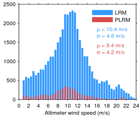
Figure 33. Histogram of flag-valid wind over oceans and lakes for LRM (blue) and PLRM (red) for 21/04/2015. The mean ( \mu ) and standard deviation ( \sigma ) are also shown. Note that values larger than 24 m/s are excluded from the histogram for the sake of readability but not from the computation of \mu and \sigma .
