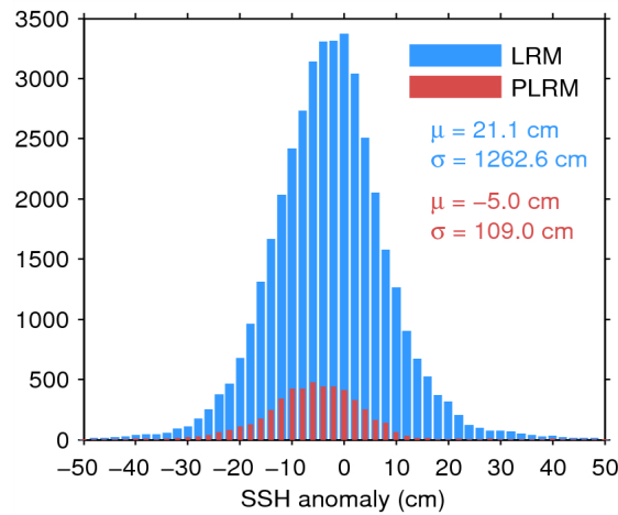
Figure 7. Histogram of flag-valid SSH anomaly over oceans and lakes for LRM (blue) and PLRM (red) for 21/04/2015. The mean ( \mu ) and standard deviation ( \sigma ) are also shown. Note that values outside [-50 50] cm are excluded from the histogram for the sake of readability but not from the computation of \mu and \sigma .
