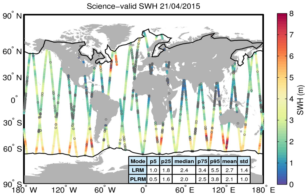
Figure 19. Geographical distribution of science-valid SWH data over oceans and lakes for 21/04/2015. The statistical values shown in the table refer to the SWH in m and are calculated separately for LRM and PLRM regions. The black lines mark the outer limit of the Arctic and Antarctic polar polygons. Gray circles denote records that have been rejected based on the editing criteria described in Table 3.
