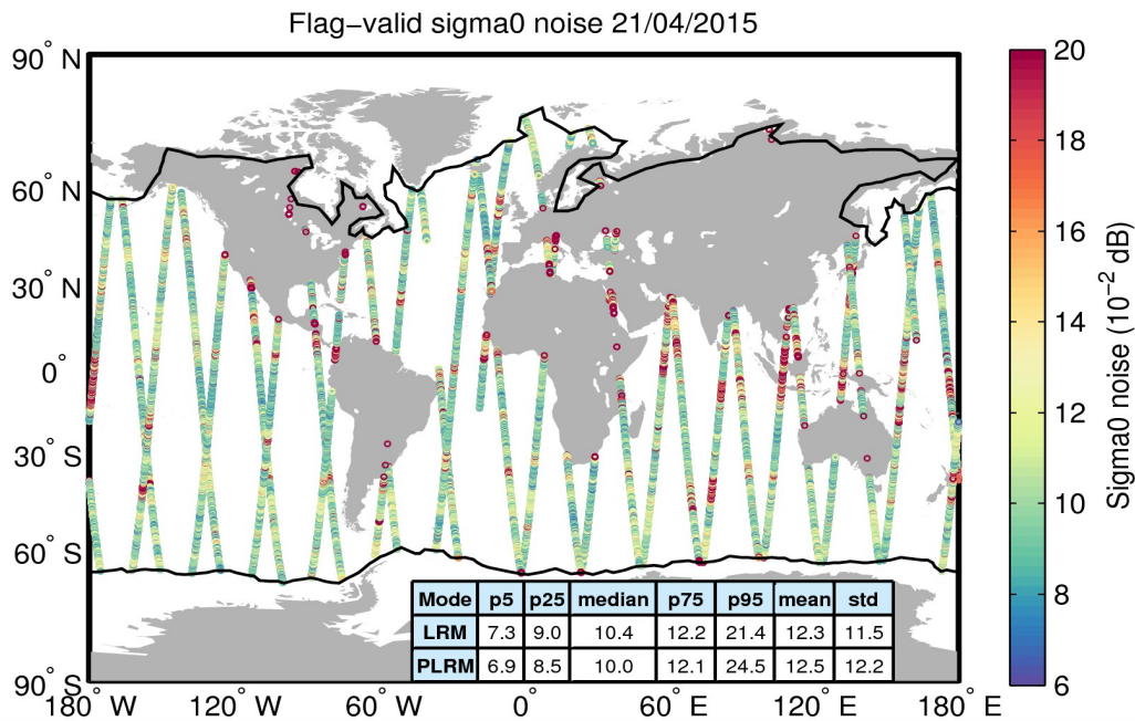
Figure 26. Geographical distribution of flag-valid 20-Hz sigma0 measurement noise over oceans and lakes for 21/04/2015. The statistical values shown in the table refer to the sigma0 noise and are calculated separately for LRM and PLRM regions. Measurements taken over polar polygons have been excluded from the computation of the statistical values. The black lines mark the outer limit of the Arctic and Antarctic polar polygons.
