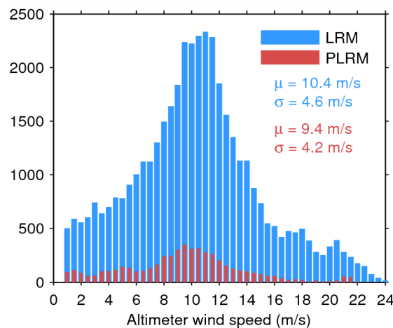
Figure 35. Histogram of science-valid wind over oceans and lakes for LRM (blue) and PLRM (red) for 21/04/2015. The mean ( \mu ) and standard deviation ( \sigma ) are also shown. Note that values larger than 24 m/s are excluded from the histogram for the sake of readability but not from the computation of \mu and \sigma .
