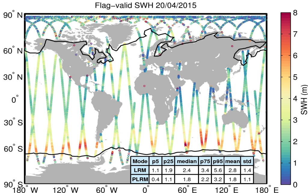
Figure 15. Geographical distribution of flag-valid SWH data over oceans and lakes for 20/04/2015. The statistical values shown in the table refer to the SWH in m and are calculated separately for LRM and PLRM regions. Measurements taken over polar polygons have been excluded from the computation of the statistical values. The black lines mark the outer limit of the Arctic and Antarctic polar polygons.
