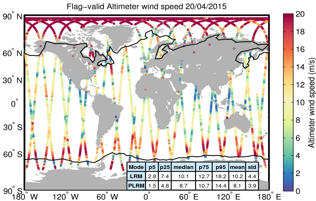
Figure 31. Geographical distribution of flag-valid wind data over oceans and lakes for 20/04/2015. The statistical values shown in the table refer to the wind in m/s and are calculated separately for LRM and PLRM regions. Measurements taken over polar polygons have been excluded from the computation of the statistical values. The black lines mark the outer limit of the Arctic and Antarctic polar polygons.
