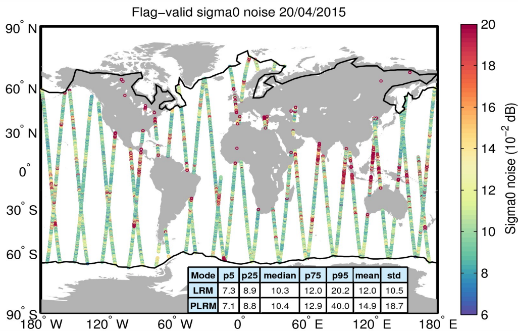
Figure 26. Geographical distribution of flag-valid 20-Hz sigma0 measurement noise over oceans and lakes for 20/04/2015. The statistical values shown in the table refer to the sigma0 noise and are calculated separately for LRM and PLRM regions. Measurements taken over polar polygons have been excluded from the computation of the statistical values. The black lines mark the outer limit of the Arctic and Antarctic polar polygons.
