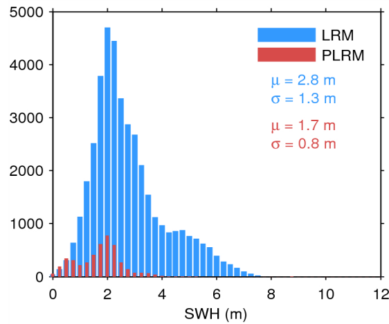
Figure 20. Histogram of science-valid SWH over oceans and lakes for LRM (blue) and PLRM (red) for 20/04/2015. The mean ( \mu ) and standard deviation ( \sigma ) are also shown. Note that values larger than 12 m are excluded from the histogram for the sake of readability but not from the computation of \mu and \sigma .
