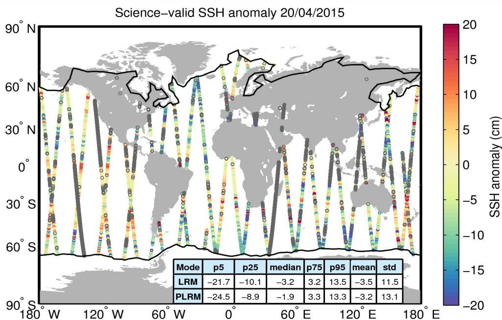
Figure 10. Geographical distribution of science-valid SSH anomaly data over oceans and lakes for 20/04/2015. The statistical values shown in the table refer to the SSH anomaly in cm and are calculated separately for LRM and PLRM regions. The black lines mark the outer limit of the Arctic and Antarctic polar polygons. Gray circles denote records that have been rejected based on the editing criteria described in Table 2.
