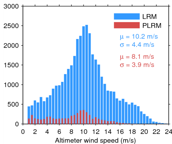
Figure 35. Histogram of science-valid wind over oceans and lakes for LRM (blue) and PLRM (red) for 20/04/2015. The mean ( \mu ) and standard deviation ( \sigma ) are also shown. Note that values larger than 24 m/s are excluded from the histogram for the sake of readability but not from the computation of \mu and \sigma .
