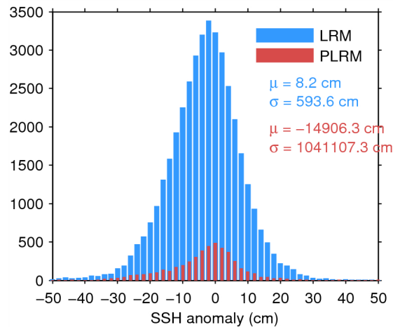
Figure 7. Histogram of flag-valid SSH anomaly over oceans and lakes for LRM (blue) and PLRM (red) for 20/04/2015. The mean ( \mu ) and standard deviation ( \sigma ) are also shown. Note that values outside [-50\ 50] cm are excluded from the histogram for the sake of readability but not from the computation of \mu and \sigma .
