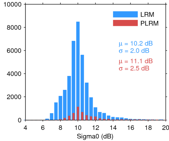
Figure 25. Histogram of flag-valid sigma0 over oceans and lakes for LRM (blue) and PLRM (red) for 20/04/2015. The mean ( \mu ) and standard deviation ( \sigma ) are also shown. Note that values outside [4 20] dB are excluded from the histogram for the sake of readability but not from the computation of \mu and \sigma .
