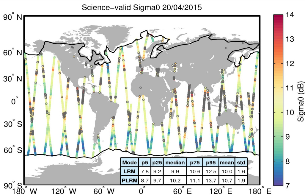
Figure 27. Geographical distribution of science-valid sigma0 data over oceans and lakes for 20/04/2015. The statistical values shown in the table refer to the sigma0 in dB and are calculated separately for LRM and PLRM regions. The black lines mark the outer limit of the Arctic and Antarctic polar polygons. Gray circles denote records that have been rejected based on the editing criteria described in Table 4.
