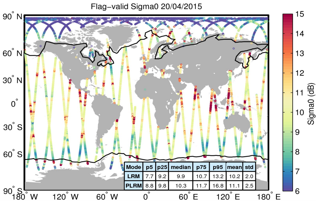
Figure 23. Geographical distribution of flag-valid sigma0 data over oceans and lakes for 20/04/2015. The statistical values shown in the table refer to the sigma0 in dB and are calculated separately for LRM and PLRM regions. Measurements taken over polar polygons have been excluded from the computation of the statistical values. The black lines mark the outer limit of the Arctic and Antarctic polar polygons.
