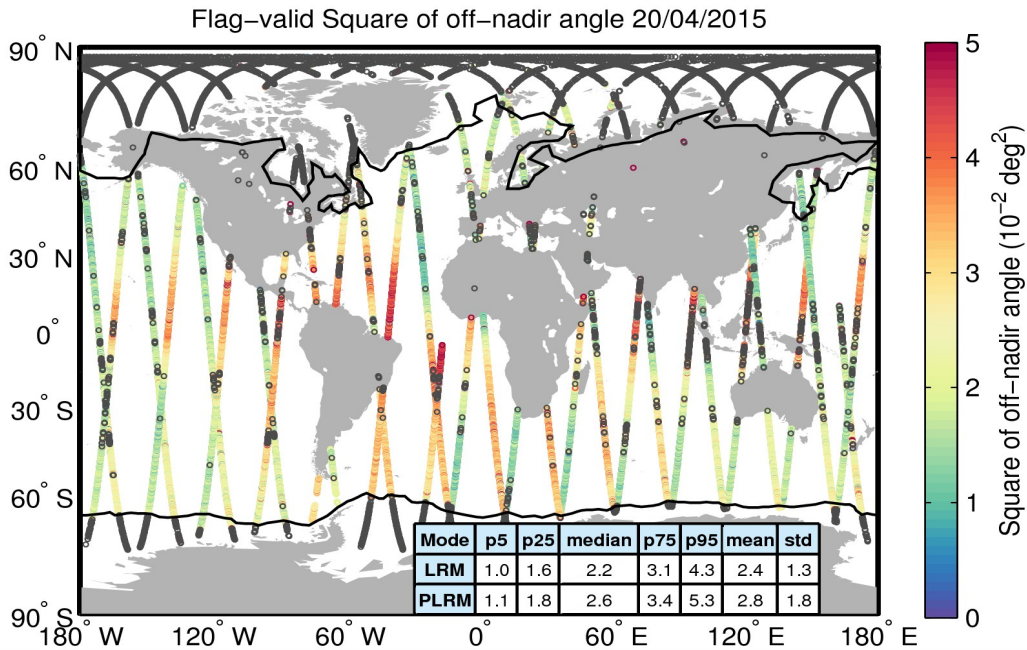
Figure 37. Geographical distribution of flag-valid mispointing data over oceans and lakes for 20/04/2015. The statistical values shown in the table refer to the mispointing in 10^{-2} \text{ deg}^2 and are calculated separately for LRM and PLRM regions. Measurements taken over polar polygons have been excluded from the computation of the statistical values. The black lines mark the outer limit of the Arctic and Antarctic polar polygons. Gray circles denote negative values.
