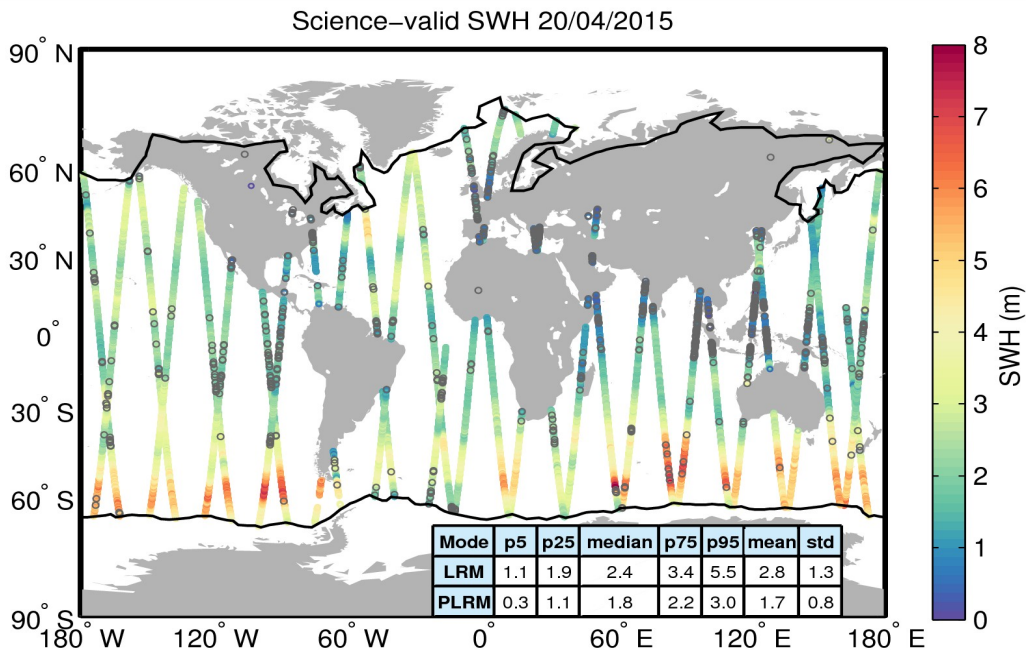
Figure 19. Geographical distribution of science-valid SWH data over oceans and lakes for 20/04/2015. The statistical values shown in the table refer to the SWH in m and are calculated separately for LRM and PLRM regions. The black lines mark the outer limit of the Arctic and Antarctic polar polygons. Gray circles denote records that have been rejected based on the editing criteria described in Table 3.
