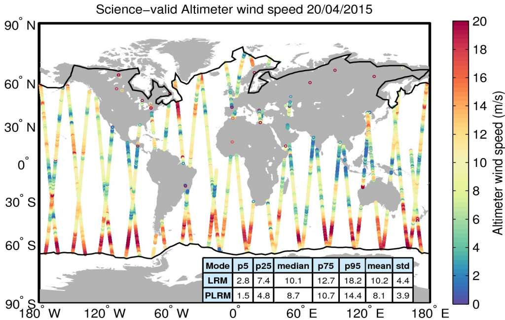
Figure 34. Geographical distribution of science-valid wind data over oceans and lakes for 20/04/2015. The statistical values shown in the table refer to the wind in m/s and are calculated separately for LRM and PLRM regions. The black lines mark the outer limit of the Arctic and Antarctic polar polygons. Gray circles denote records that have been rejected based on the editing criteria described in Table 5.
