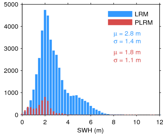
Figure 17. Histogram of flag-valid SWH over oceans and lakes for LRM (blue) and PLRM (red) for 20/04/2015. The mean ( \mu ) and standard deviation ( \sigma ) are also shown. Note that values larger than 12 m are excluded from the histogram for the sake of readability but not from the computation of \mu and \sigma .
