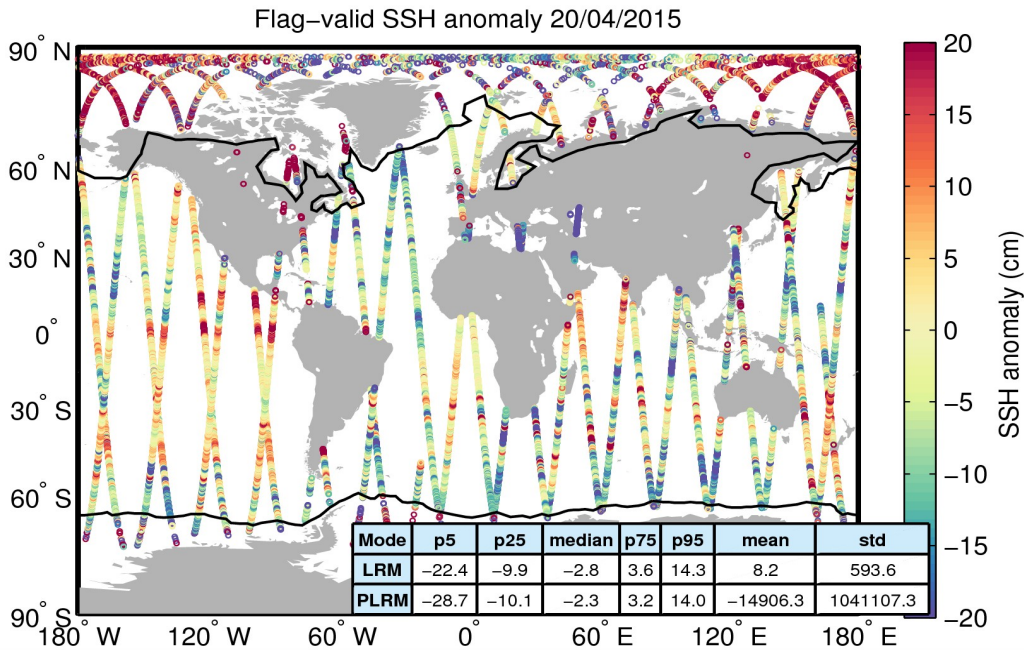
Figure 5. Geographical distribution of flag-valid 1-Hz SSH anomaly data over oceans and lakes for 20/04/2015. The statistical values shown in the table refer to the SSH anomaly in cm and are calculated separately for LRM and PLRM regions. Measurements taken over polar polygons have been excluded from the computation of the statistical values. The black lines mark the outer limit of the Arctic and Antarctic polar polygons.
