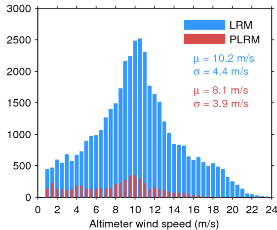
Figure 33. Histogram of flag-valid wind over oceans and lakes for LRM (blue) and PLRM (red) for 20/04/2015. The mean ( \mu ) and standard deviation ( \sigma ) are also shown. Note that values larger than 24 m/s are excluded from the histogram for the sake of readability but not from the computation of \mu and \sigma .
