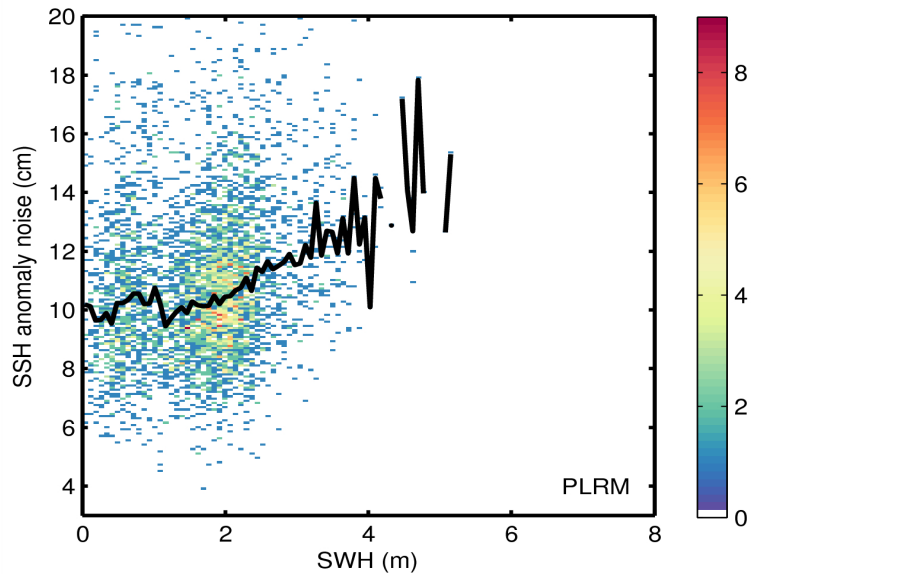
Figure 9. 2D histogram showing flag-valid SSH anomaly noise as a function of SWH for LRM (top) and PLRM (bottom) for 20/04/2015. The black line denotes the median SSH anomaly as a function of SWH.
