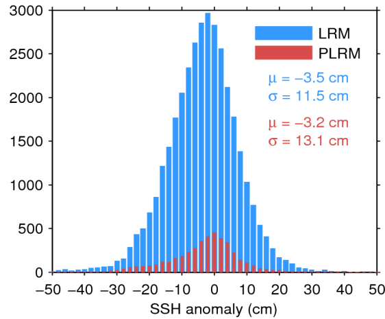
Figure 11. Histogram of science-valid SSH anomaly over oceans and lakes for LRM (blue) and PLRM (red) for 20/04/2015. The mean ( \mu ) and standard deviation ( \sigma ) are also shown. Note that values outside [-50\ 50] cm are excluded from the histogram for the sake of readability but not from the computation of \mu and \sigma .
