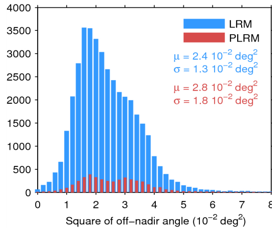
Figure 39. Histogram of flag-valid mispointing over oceans and lakes for LRM (blue) and PLRM (red) for 20/04/2015. Only positive values have been considered. The mean ( \mu ) and standard deviation ( \sigma ) are also shown. Note that values larger than 8 \cdot 10^{-2} \text{ deg}^2 are excluded from the histogram for the sake of readability but not from the computation of \mu and \sigma .
