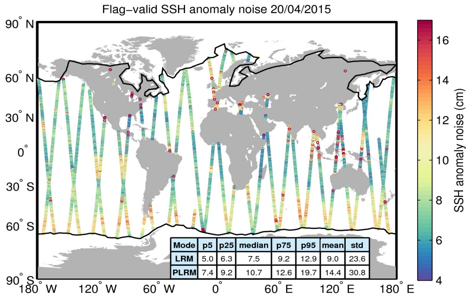
Figure 8. Geographical distribution of flag-valid 20-Hz SSH anomaly measurement noise over oceans and lakes for 20/04/2015. The statistical values shown in the table refer to the SSH anomaly noise and are calculated separately for LRM and PLRM regions. Measurements taken over polar polygons have been excluded from the computation of the statistical values. The black lines mark the outer limit of the Arctic and Antarctic polar polygons.
