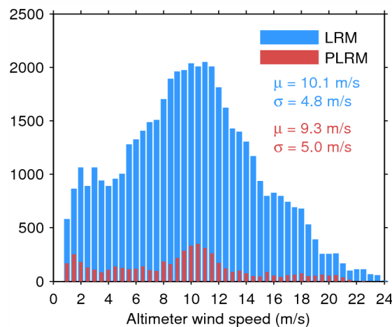
Figure 35. Histogram of science-valid wind over oceans and lakes for LRM (blue) and PLRM (red) for 13/04/2015. The mean ( \mu ) and standard deviation ( \sigma ) are also shown. Note that values larger than 24 m/s are excluded from the histogram for the sake of readability but not from the computation of \mu and \sigma .
