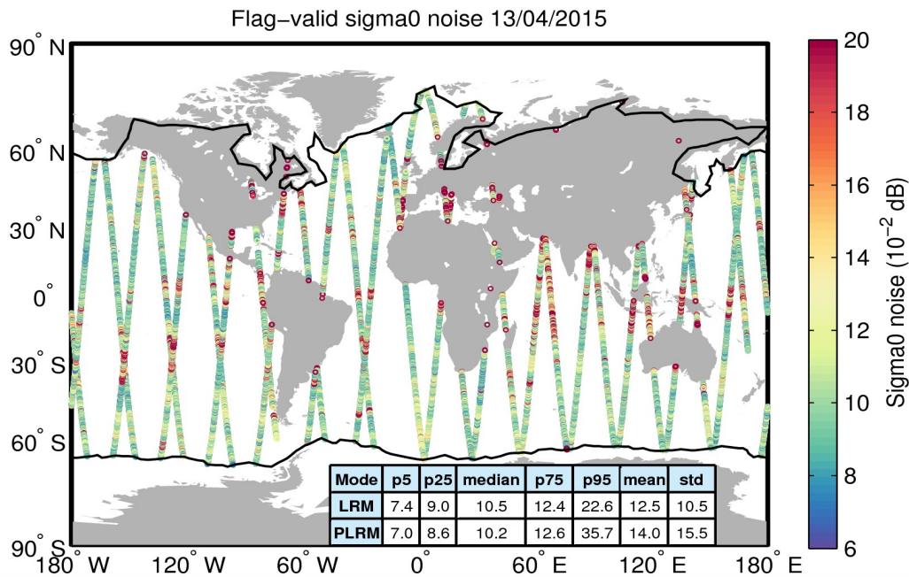
Figure 26. Geographical distribution of flag-valid 20-Hz sigma0 measurement noise over oceans and lakes for 13/04/2015. The statistical values shown in the table refer to the sigma0 noise and are calculated separately for LRM and PLRM regions. Measurements taken over polar polygons have been excluded from the computation of the statistical values. The black lines mark the outer limit of the Arctic and Antarctic polar polygons.
