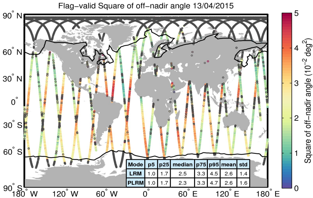
Figure 37. Geographical distribution of flag-valid mispointing data over oceans and lakes for 13/04/2015. The statistical values shown in the table refer to the mispointing in 10^{-2} \text{ deg}^2 and are calculated separately for LRM and PLRM regions. Measurements taken over polar polygons have been excluded from the computation of the statistical values. The black lines mark the outer limit of the Arctic and Antarctic polar polygons. Gray circles denote negative values.
