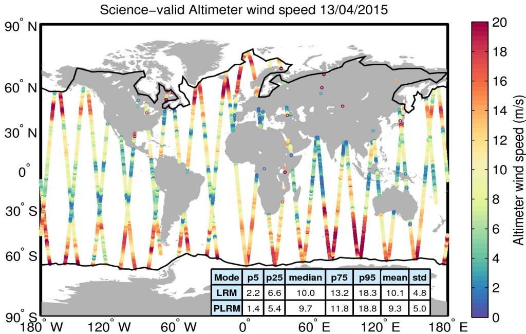
Figure 34. Geographical distribution of science-valid wind data over oceans and lakes for 13/04/2015. The statistical values shown in the table refer to the wind in m/s and are calculated separately for LRM and PLRM regions. The black lines mark the outer limit of the Arctic and Antarctic polar polygons. Gray circles denote records that have been rejected based on the editing criteria described in Table 5.
