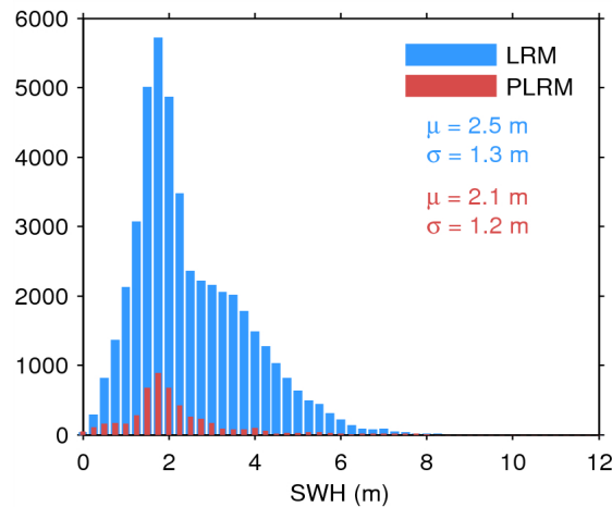
Figure 20. Histogram of science-valid SWH over oceans and lakes for LRM (blue) and PLRM (red) for 13/04/2015. The mean ( \mu ) and standard deviation ( \sigma ) are also shown. Note that values larger than 12 m are excluded from the histogram for the sake of readability but not from the computation of \mu and \sigma .
