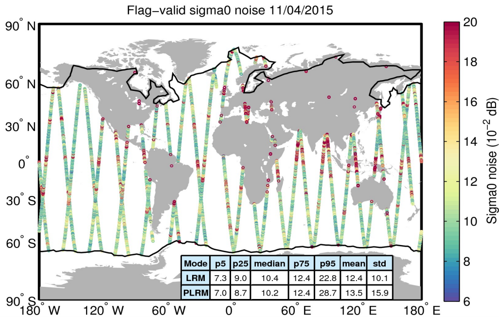
Figure 26. Geographical distribution of flag-valid 20-Hz sigma0 measurement noise over oceans and lakes for 11/04/2015. The statistical values shown in the table refer to the sigma0 noise and are calculated separately for LRM and PLRM regions. Measurements taken over polar polygons have been excluded from the computation of the statistical values. The black lines mark the outer limit of the Arctic and Antarctic polar polygons.
