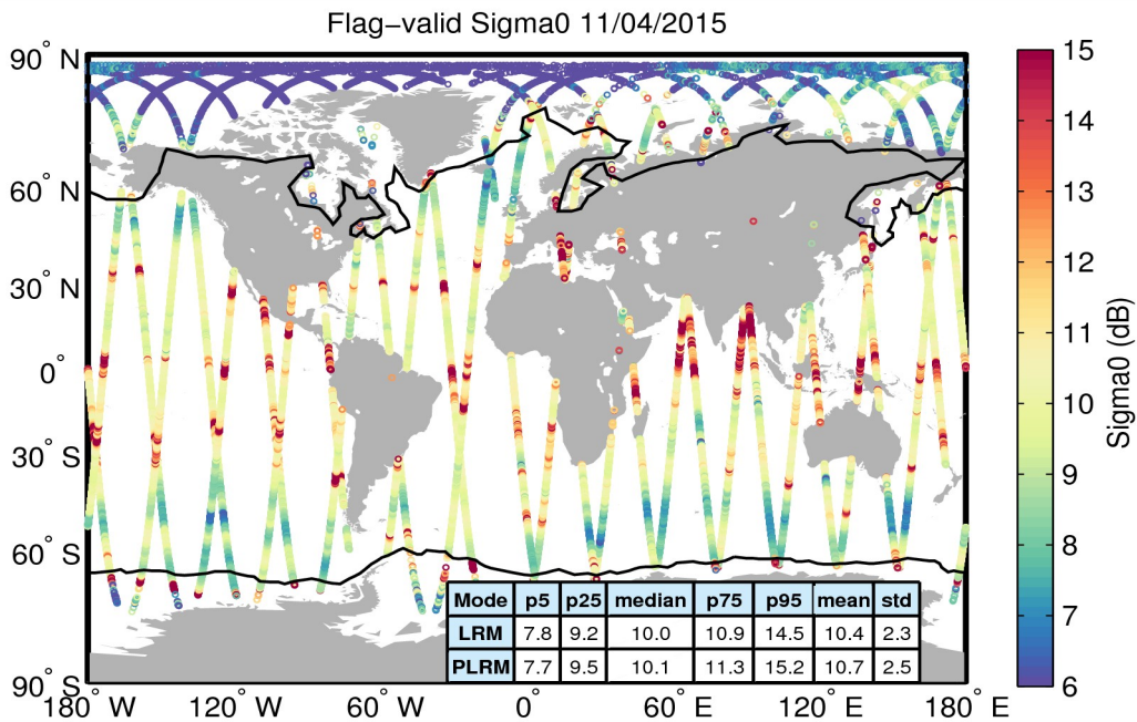
Figure 23. Geographical distribution of flag-valid sigma0 data over oceans and lakes for 11/04/2015. The statistical values shown in the table refer to the sigma0 in dB and are calculated separately for LRM and PLRM regions. Measurements taken over polar polygons have been excluded from the computation of the statistical values. The black lines mark the outer limit of the Arctic and Antarctic polar polygons.
