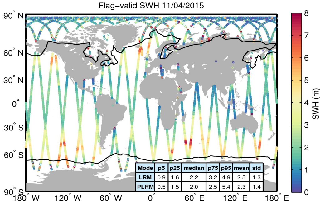
Figure 15. Geographical distribution of flag-valid SWH data over oceans and lakes for 11/04/2015. The statistical values shown in the table refer to the SWH in m and are calculated separately for LRM and PLRM regions. Measurements taken over polar polygons have been excluded from the computation of the statistical values. The black lines mark the outer limit of the Arctic and Antarctic polar polygons.
