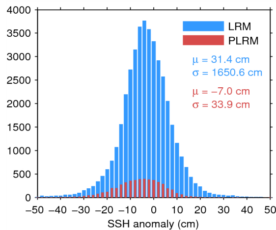
Figure 7. Histogram of flag-valid SSH anomaly over oceans and lakes for LRM (blue) and PLRM (red) for 11/04/2015. The mean ( \mu ) and standard deviation ( \sigma ) are also shown. Note that values outside [-50 \ 50] cm are excluded from the histogram for the sake of readability but not from the computation of \mu and \sigma .
