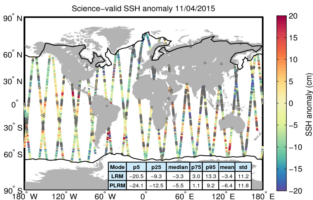
Figure 10. Geographical distribution of science-valid SSH anomaly data over oceans and lakes for 11/04/2015. The statistical values shown in the table refer to the SSH anomaly in cm and are calculated separately for LRM and PLRM regions. The black lines mark the outer limit of the Arctic and Antarctic polar polygons. Gray circles denote records that have been rejected based on the editing criteria described in Table 2.
