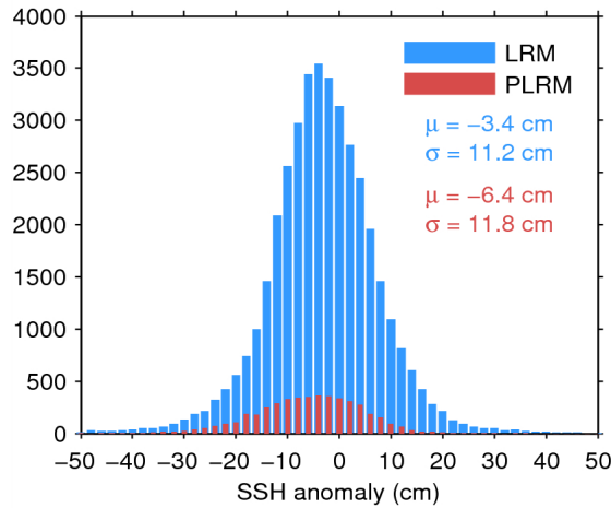
Figure 11. Histogram of science-valid SSH anomaly over oceans and lakes for LRM (blue) and PLRM (red) for 11/04/2015. The mean ( \mu ) and standard deviation ( \sigma ) are also shown. Note that values outside [-50 50] cm are excluded from the histogram for the sake of readability but not from the computation of \mu and \sigma .
