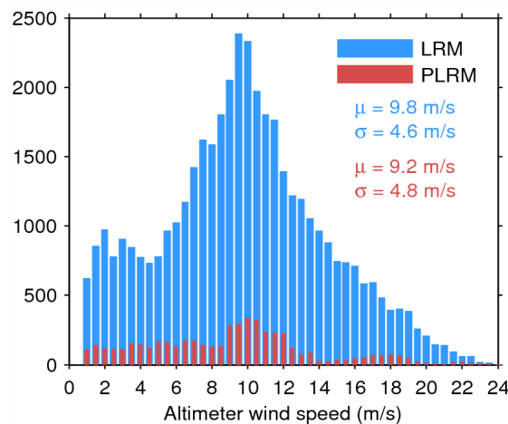
Figure 35. Histogram of science-valid wind over oceans and lakes for LRM (blue) and PLRM (red) for 11/04/2015. The mean ( \mu ) and standard deviation ( \sigma ) are also shown. Note that values larger than 24 m/s are excluded from the histogram for the sake of readability but not from the computation of \mu and \sigma .
