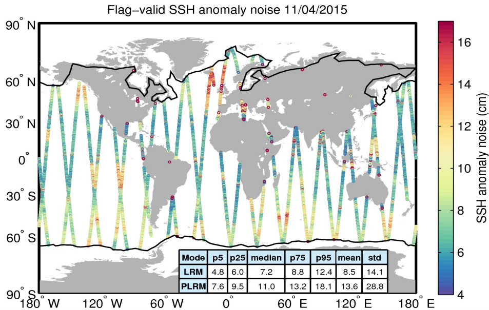
Figure 8. Geographical distribution of flag-valid 20-Hz SSH anomaly measurement noise over oceans and lakes for 11/04/2015. The statistical values shown in the table refer to the SSH anomaly noise and are calculated separately for LRM and PLRM regions. Measurements taken over polar polygons have been excluded from the computation of the statistical values. The black lines mark the outer limit of the Arctic and Antarctic polar polygons.
