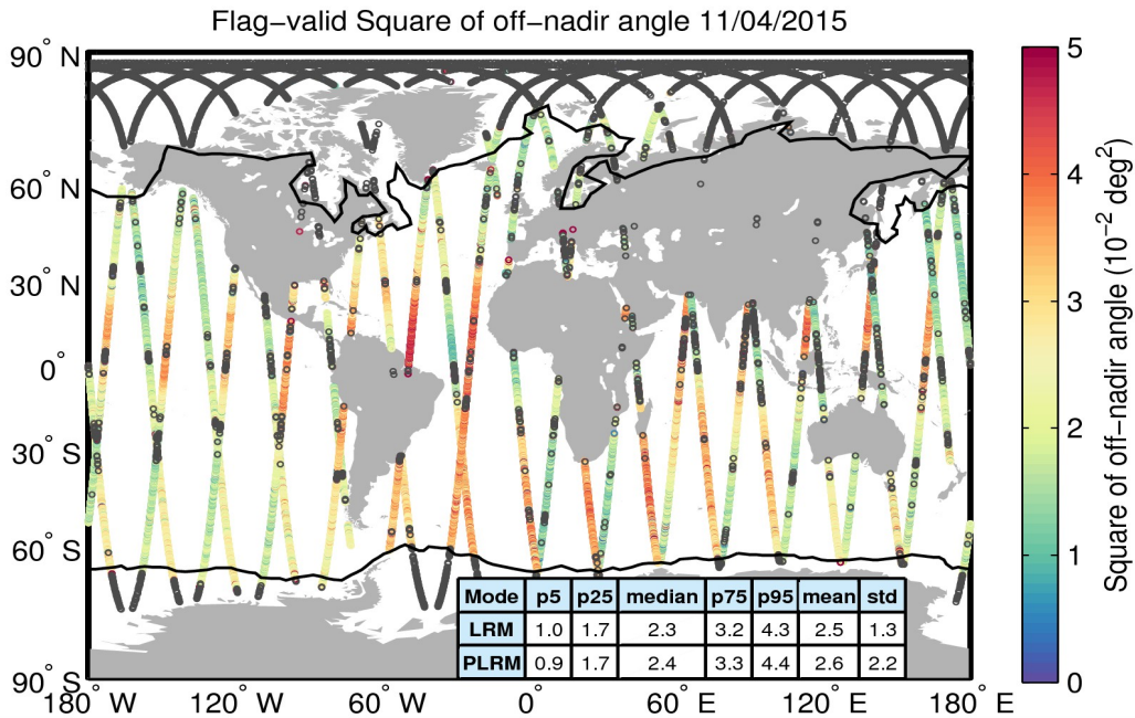
Figure 37. Geographical distribution of flag-valid mispointing data over oceans and lakes for 11/04/2015. The statistical values shown in the table refer to the mispointing in 10^{-2} \text{ deg}^2 and are calculated separately for LRM and PLRM regions. Measurements taken over polar polygons have been excluded from the computation of the statistical values. The black lines mark the outer limit of the Arctic and Antarctic polar polygons. Gray circles denote negative values.
