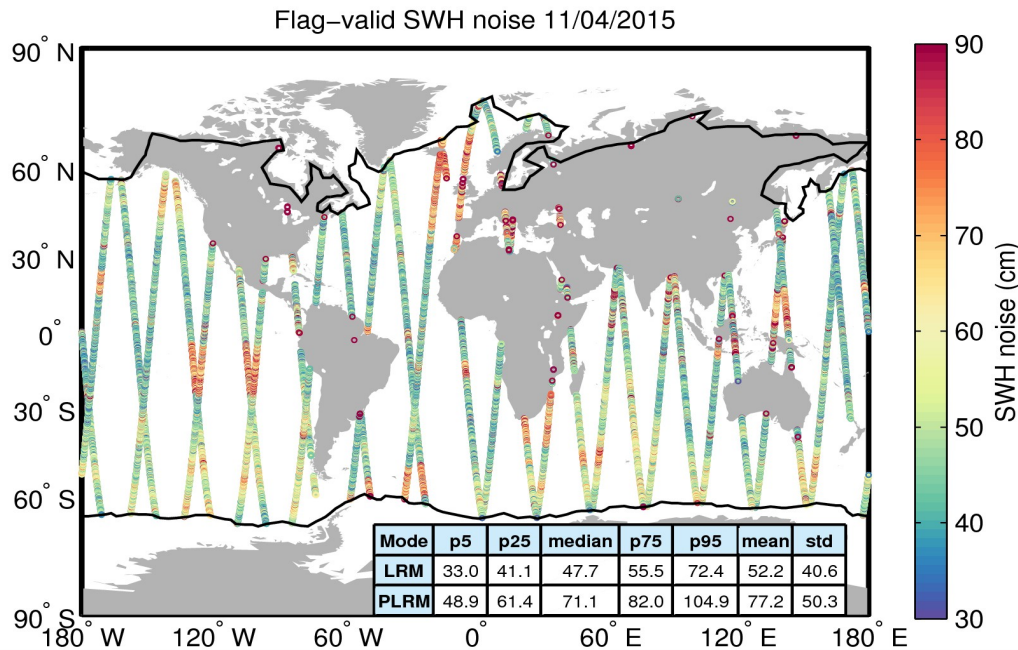
Figure 18. Geographical distribution of flag-valid 20-Hz SWH measurement noise over oceans and lakes for 11/04/2015. The statistical values shown in the table refer to the SWH noise and are calculated separately for LRM and PLRM regions. Measurements taken over polar polygons have been excluded from the computation of the statistical values. The black lines mark the outer limit of the Arctic and Antarctic polar polygons.
