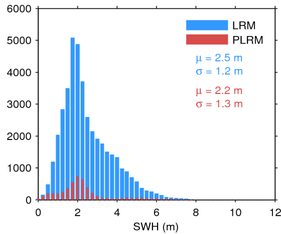
Figure 20. Histogram of science-valid SWH over oceans and lakes for LRM (blue) and PLRM (red) for 11/04/2015. The mean ( \mu ) and standard deviation ( \sigma ) are also shown. Note that values larger than 12 m are excluded from the histogram for the sake of readability but not from the computation of \mu and \sigma .
