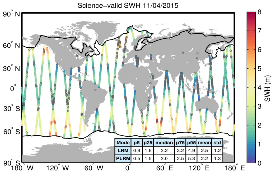
Figure 19. Geographical distribution of science-valid SWH data over oceans and lakes for 11/04/2015. The statistical values shown in the table refer to the SWH in m and are calculated separately for LRM and PLRM regions. The black lines mark the outer limit of the Arctic and Antarctic polar polygons. Gray circles denote records that have been rejected based on the editing criteria described in Table 3.
