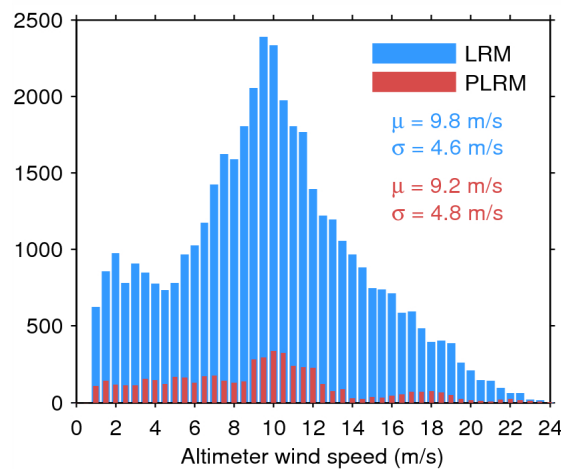
Figure 33. Histogram of flag-valid wind over oceans and lakes for LRM (blue) and PLRM (red) for 11/04/2015. The mean ( \mu ) and standard deviation ( \sigma ) are also shown. Note that values larger than 24 m/s are excluded from the histogram for the sake of readability but not from the computation of \mu and \sigma .
