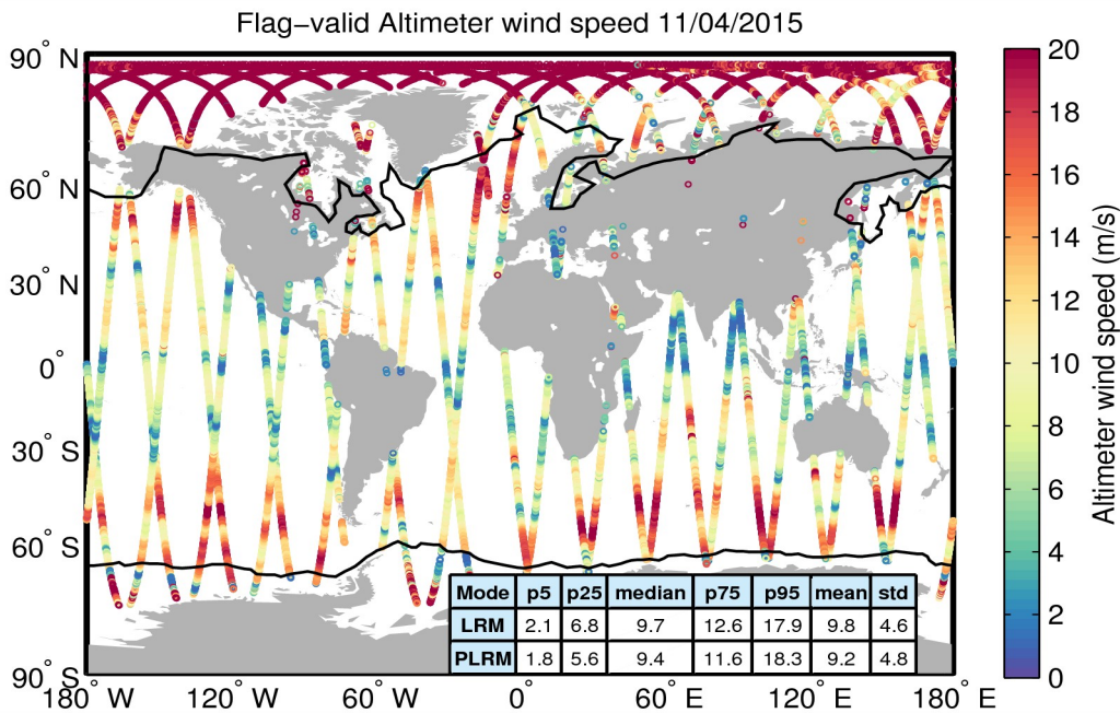
Figure 31. Geographical distribution of flag-valid wind data over oceans and lakes for 11/04/2015. The statistical values shown in the table refer to the wind in m/s and are calculated separately for LRM and PLRM regions. Measurements taken over polar polygons have been excluded from the computation of the statistical values. The black lines mark the outer limit of the Arctic and Antarctic polar polygons.
