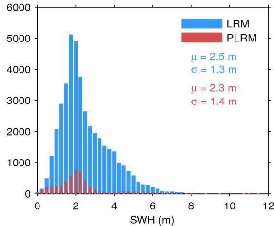
Figure 17. Histogram of flag-valid SWH over oceans and lakes for LRM (blue) and PLRM (red) for 11/04/2015. The mean ( \mu ) and standard deviation ( \sigma ) are also shown. Note that values larger than 12 m are excluded from the histogram for the sake of readability but not from the computation of \mu and \sigma .
