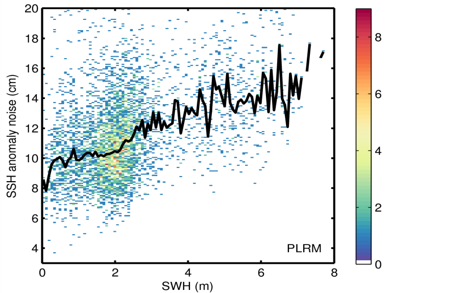
Figure 9. 2D histogram showing flag-valid SSH anomaly noise as a function of SWH for LRM (top) and PLRM (bottom) for 11/04/2015. The black line denotes the median SSH anomaly as a function of SWH.
