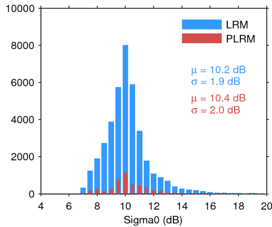
Figure 28. Histogram of science-valid sigma0 over oceans and lakes for LRM (blue) and PLRM (red) for 11/04/2015. The mean ( \mu ) and standard deviation ( \sigma ) are also shown. Note that values outside [4 20] dB are excluded from the histogram for the sake of readability but not from the computation of \mu and \sigma .
