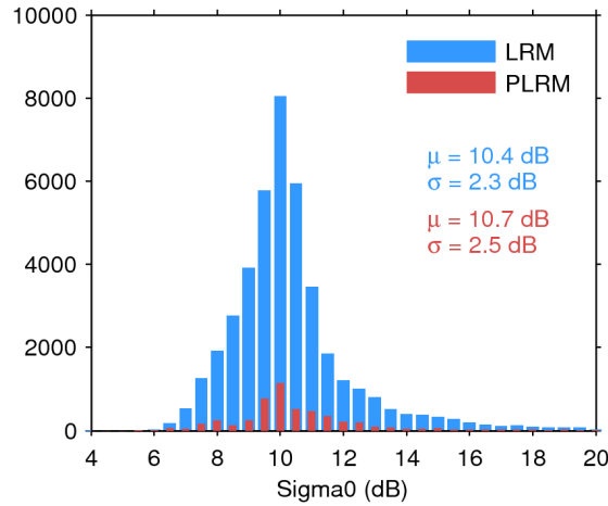
Figure 25. Histogram of flag-valid sigma0 over oceans and lakes for LRM (blue) and PLRM (red) for 11/04/2015. The mean ( \mu ) and standard deviation ( \sigma ) are also shown. Note that values outside [4 20] dB are excluded from the histogram for the sake of readability but not from the computation of \mu and \sigma .
