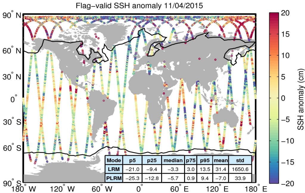
Figure 5. Geographical distribution of flag-valid 1-Hz SSH anomaly data over oceans and lakes for 11/04/2015. The statistical values shown in the table refer to the SSH anomaly in cm and are calculated separately for LRM and PLRM regions. Measurements taken over polar polygons have been excluded from the computation of the statistical values. The black lines mark the outer limit of the Arctic and Antarctic polar polygons.
