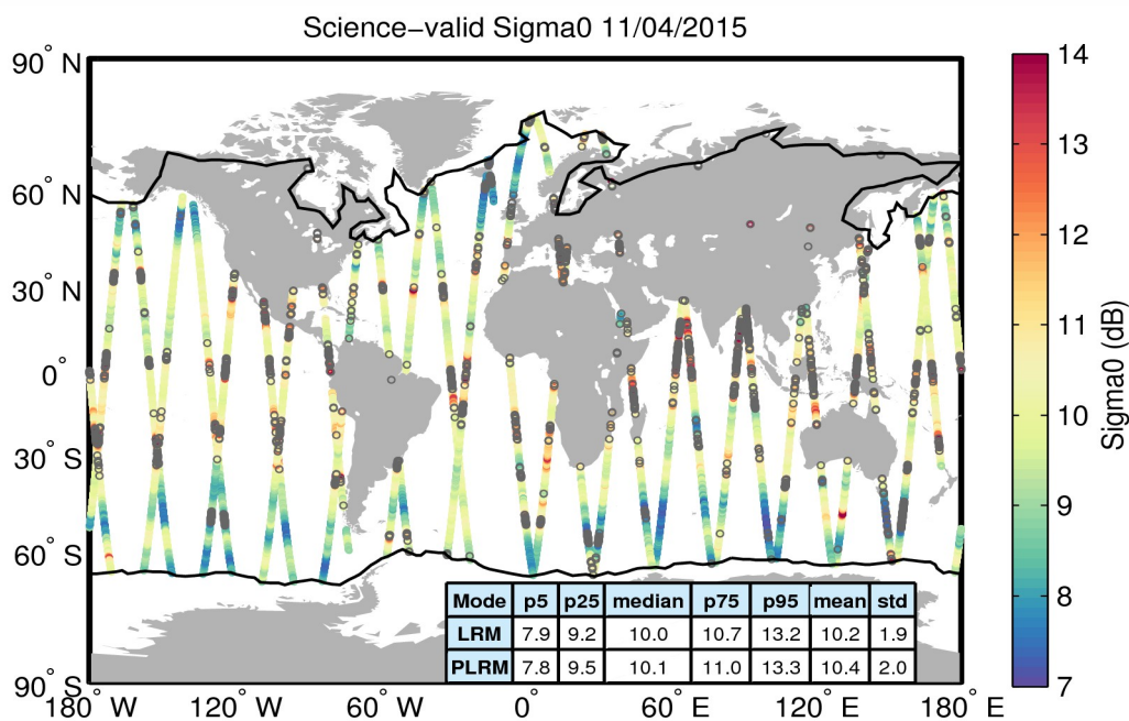
Figure 27. Geographical distribution of science-valid sigma0 data over oceans and lakes for 11/04/2015. The statistical values shown in the table refer to the sigma0 in dB and are calculated separately for LRM and PLRM regions. The black lines mark the outer limit of the Arctic and Antarctic polar polygons. Gray circles denote records that have been rejected based on the editing criteria described in Table 4.
