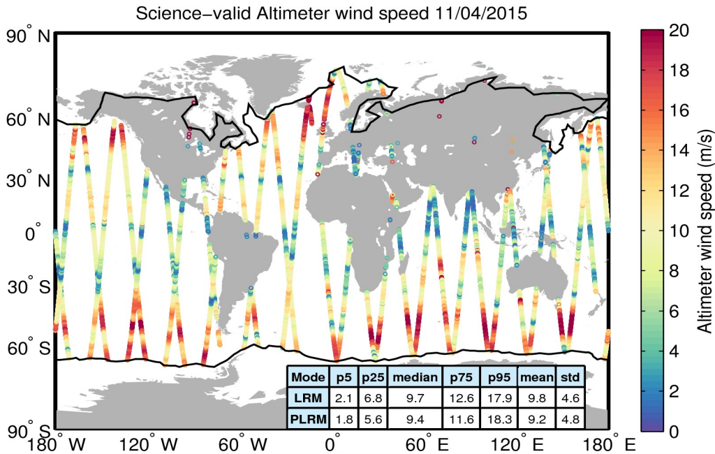
Figure 34. Geographical distribution of science-valid wind data over oceans and lakes for 11/04/2015. The statistical values shown in the table refer to the wind in m/s and are calculated separately for LRM and PLRM regions. The black lines mark the outer limit of the Arctic and Antarctic polar polygons. Gray circles denote records that have been rejected based on the editing criteria described in Table 5.
