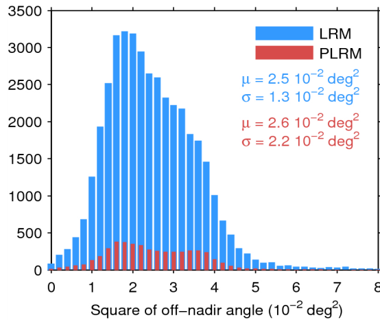
Figure 39. Histogram of flag-valid mispointing over oceans and lakes for LRM (blue) and PLRM (red) for 11/04/2015. Only positive values have been considered. The mean ( \mu ) and standard deviation ( \sigma ) are also shown. Note that values larger than 8 \cdot 10^{-2} \text{ deg}^2 are excluded from the histogram for the sake of readability but not from the computation of \mu and \sigma .
