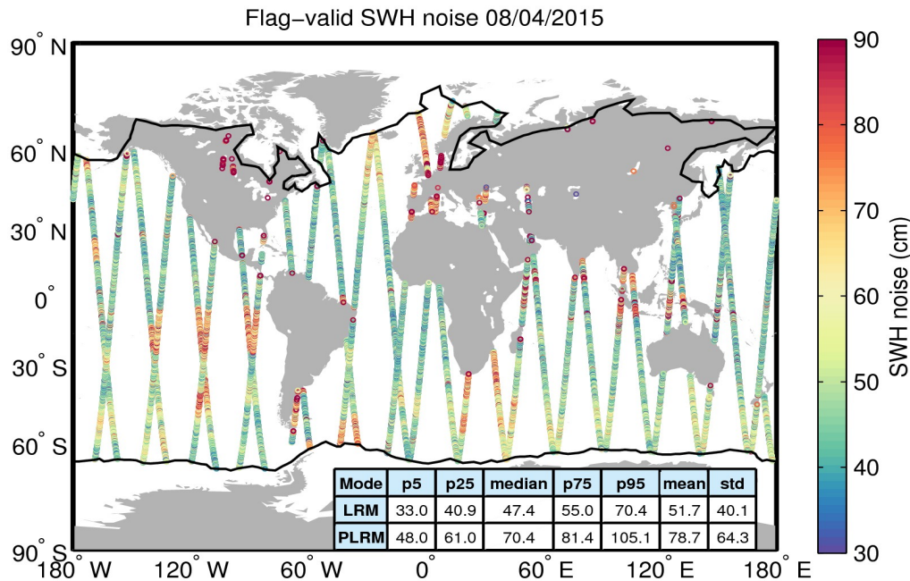
Figure 18. Geographical distribution of flag-valid 20-Hz SWH measurement noise over oceans and lakes for 08/04/2015. The statistical values shown in the table refer to the SWH noise and are calculated separately for LRM and PLRM regions. Measurements taken over polar polygons have been excluded from the computation of the statistical values. The black lines mark the outer limit of the Arctic and Antarctic polar polygons.
