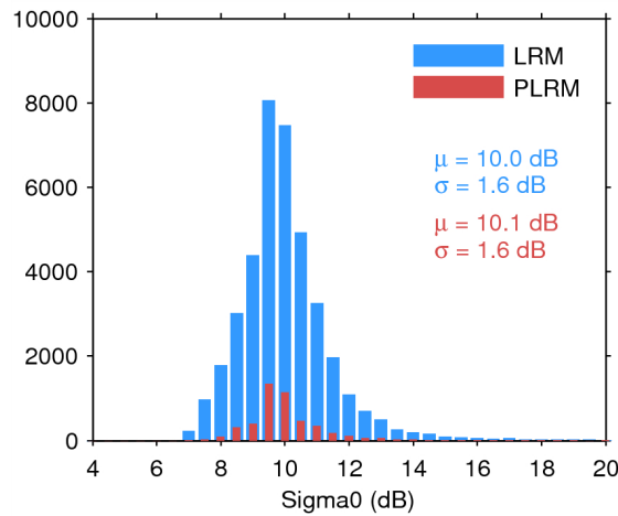
Figure 28. Histogram of science-valid sigma0 over oceans and lakes for LRM (blue) and PLRM (red) for 08/04/2015. The mean ( \mu ) and standard deviation ( \sigma ) are also shown. Note that values outside [4 20] dB are excluded from the histogram for the sake of readability but not from the computation of \mu and \sigma .
