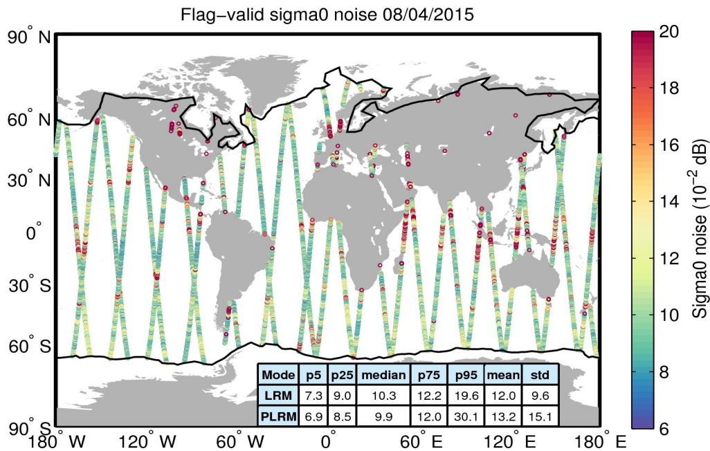
Figure 26. Geographical distribution of flag-valid 20-Hz sigma0 measurement noise over oceans and lakes for 08/04/2015. The statistical values shown in the table refer to the sigma0 noise and are calculated separately for LRM and PLRM regions. Measurements taken over polar polygons have been excluded from the computation of the statistical values. The black lines mark the outer limit of the Arctic and Antarctic polar polygons.
