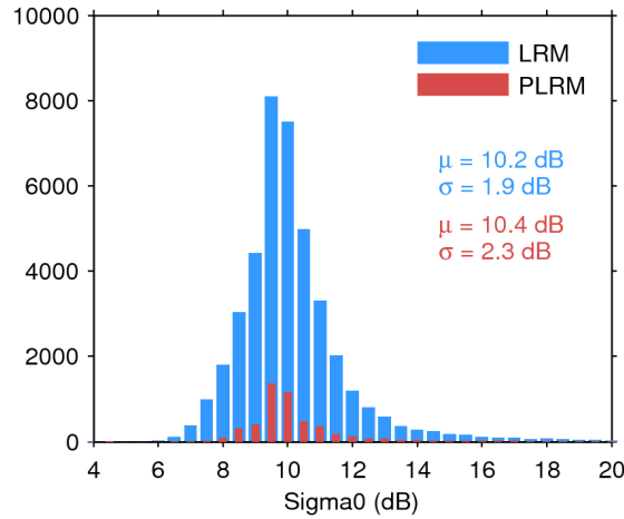
Figure 25. Histogram of flag-valid sigma0 over oceans and lakes for LRM (blue) and PLRM (red) for 08/04/2015. The mean ( \mu ) and standard deviation ( \sigma ) are also shown. Note that values outside [4 20] dB are excluded from the histogram for the sake of readability but not from the computation of \mu and \sigma .
