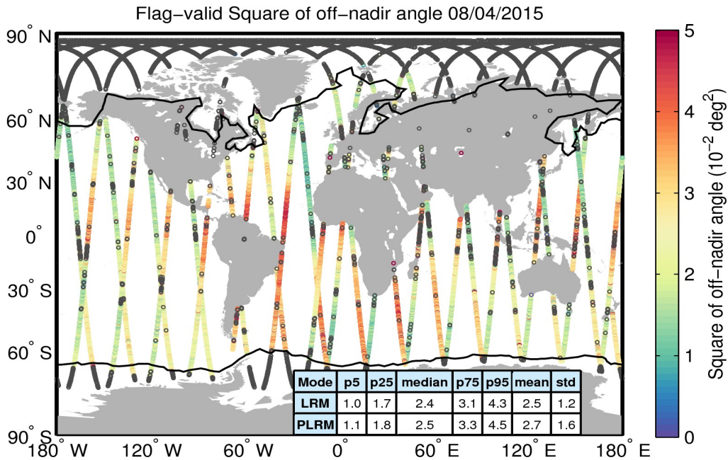
Figure 37. Geographical distribution of flag-valid mispointing data over oceans and lakes for 08/04/2015. The statistical values shown in the table refer to the mispointing in 10^{-2} \text{ deg}^2 and are calculated separately for LRM and PLRM regions. Measurements taken over polar polygons have been excluded from the computation of the statistical values. The black lines mark the outer limit of the Arctic and Antarctic polar polygons. Gray circles denote negative values.
