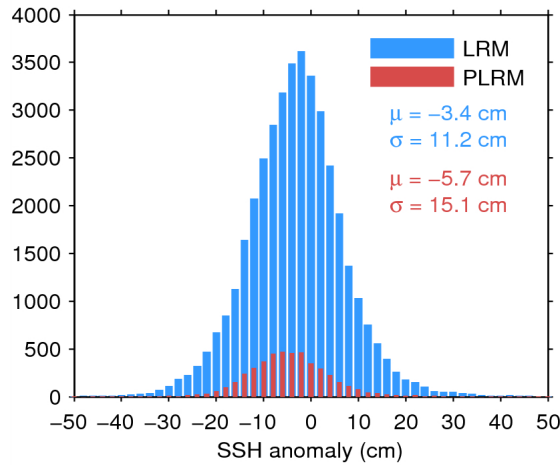
Figure 11. Histogram of science-valid SSH anomaly over oceans and lakes for LRM (blue) and PLRM (red) for 08/04/2015. The mean ( \mu ) and standard deviation ( \sigma ) are also shown. Note that values outside [-50 50] cm are excluded from the histogram for the sake of readability but not from the computation of \mu and \sigma .
