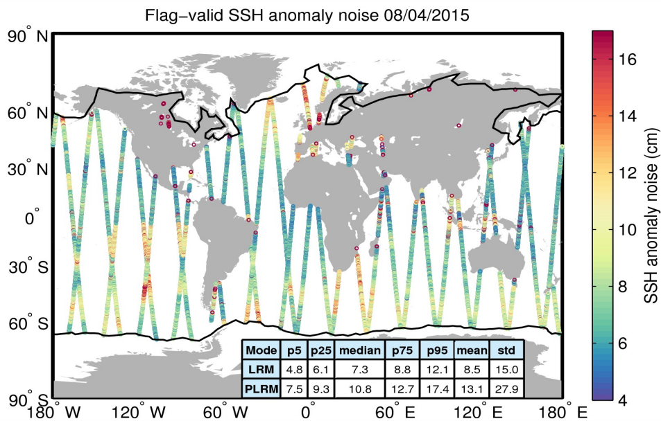
Figure 8. Geographical distribution of flag-valid 20-Hz SSH anomaly measurement noise over oceans and lakes for 08/04/2015. The statistical values shown in the table refer to the SSH anomaly noise and are calculated separately for LRM and PLRM regions. Measurements taken over polar polygons have been excluded from the computation of the statistical values. The black lines mark the outer limit of the Arctic and Antarctic polar polygons.
