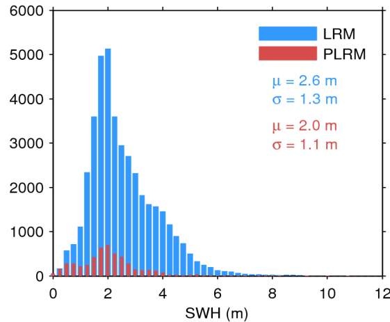
Figure 17. Histogram of flag-valid SWH over oceans and lakes for LRM (blue) and PLRM (red) for 08/04/2015. The mean ( \mu ) and standard deviation ( \sigma ) are also shown. Note that values larger than 12 m are excluded from the histogram for the sake of readability but not from the computation of \mu and \sigma .
