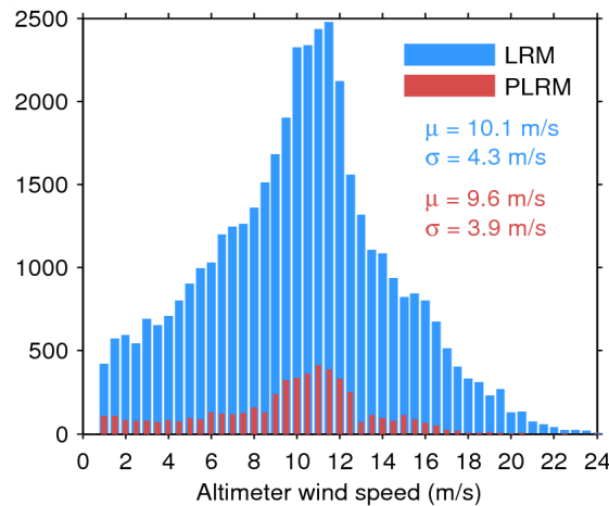
Figure 33. Histogram of flag-valid wind over oceans and lakes for LRM (blue) and PLRM (red) for 08/04/2015. The mean ( \mu ) and standard deviation ( \sigma ) are also shown. Note that values larger than 24 m/s are excluded from the histogram for the sake of readability but not from the computation of \mu and \sigma .
