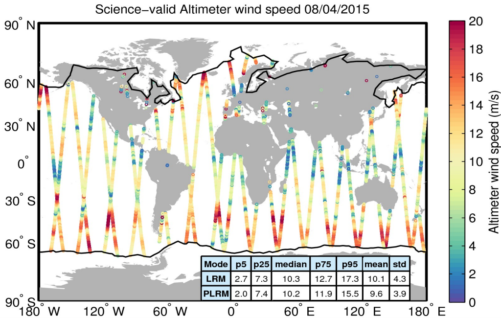
Figure 34. Geographical distribution of science-valid wind data over oceans and lakes for 08/04/2015. The statistical values shown in the table refer to the wind in m/s and are calculated separately for LRM and PLRM regions. The black lines mark the outer limit of the Arctic and Antarctic polar polygons. Gray circles denote records that have been rejected based on the editing criteria described in Table 5.
