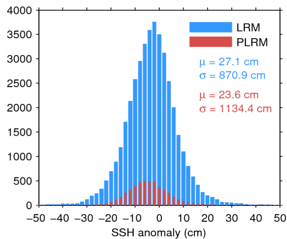
Figure 7. Histogram of flag-valid SSH anomaly over oceans and lakes for LRM (blue) and PLRM (red) for 08/04/2015. The mean ( \mu ) and standard deviation ( \sigma ) are also shown. Note that values outside [-50\ 50] cm are excluded from the histogram for the sake of readability but not from the computation of \mu and \sigma .
