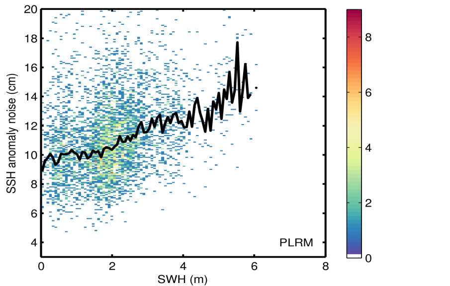
Figure 9. 2D histogram showing flag-valid SSH anomaly noise as a function of SWH for LRM (top) and PLRM (bottom) for 08/04/2015. The black line denotes the median SSH anomaly as a function of SWH.
