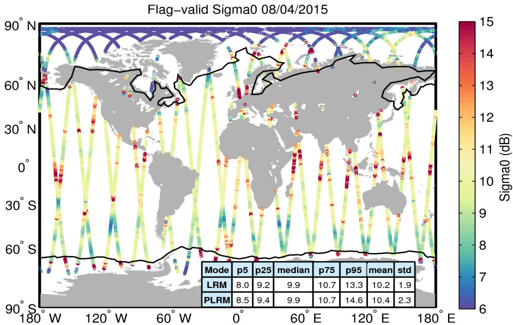
Figure 23. Geographical distribution of flag-valid sigma0 data over oceans and lakes for 08/04/2015. The statistical values shown in the table refer to the sigma0 in dB and are calculated separately for LRM and PLRM regions. Measurements taken over polar polygons have been excluded from the computation of the statistical values. The black lines mark the outer limit of the Arctic and Antarctic polar polygons.
