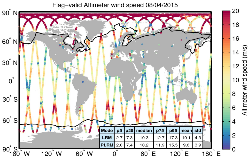
Figure 31. Geographical distribution of flag-valid wind data over oceans and lakes for 08/04/2015. The statistical values shown in the table refer to the wind in m/s and are calculated separately for LRM and PLRM regions. Measurements taken over polar polygons have been excluded from the computation of the statistical values. The black lines mark the outer limit of the Arctic and Antarctic polar polygons.
