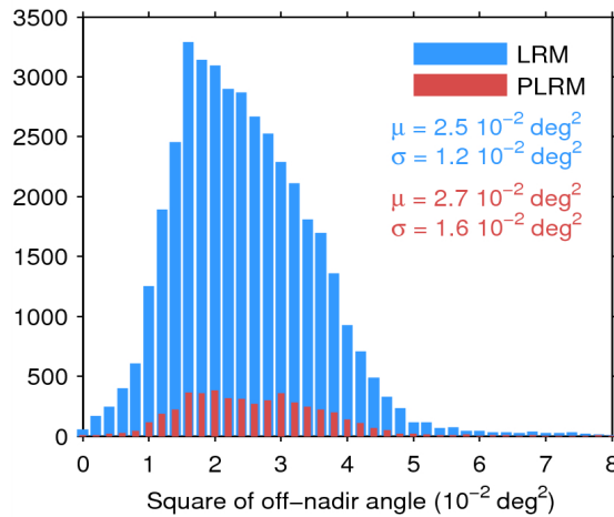
Figure 39. Histogram of flag-valid mispointing over oceans and lakes for LRM (blue) and PLRM (red) for 08/04/2015. Only positive values have been considered. The mean ( \mu ) and standard deviation ( \sigma ) are also shown. Note that values larger than 8 \cdot 10^{-2} \text{ deg}^2 are excluded from the histogram for the sake of readability but not from the computation of \mu and \sigma .
