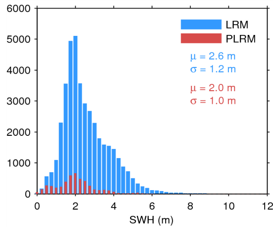
Figure 20. Histogram of science-valid SWH over oceans and lakes for LRM (blue) and PLRM (red) for 08/04/2015. The mean ( \mu ) and standard deviation ( \sigma ) are also shown. Note that values larger than 12 m are excluded from the histogram for the sake of readability but not from the computation of \mu and \sigma .
