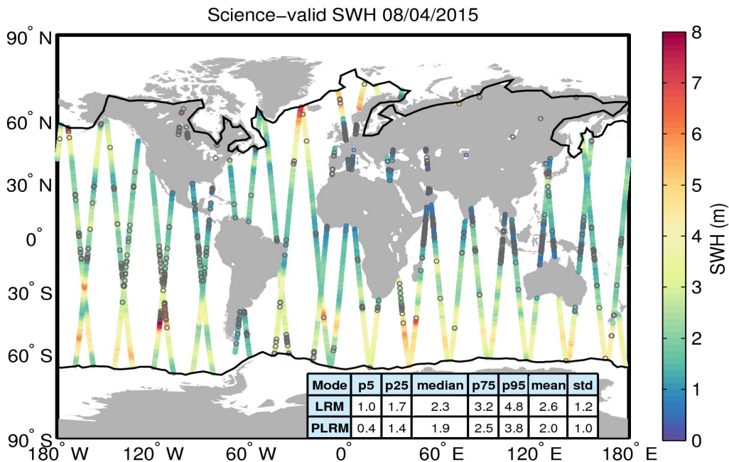
Figure 19. Geographical distribution of science-valid SWH data over oceans and lakes for 08/04/2015. The statistical values shown in the table refer to the SWH in m and are calculated separately for LRM and PLRM regions. The black lines mark the outer limit of the Arctic and Antarctic polar polygons. Gray circles denote records that have been rejected based on the editing criteria described in Table 3.
