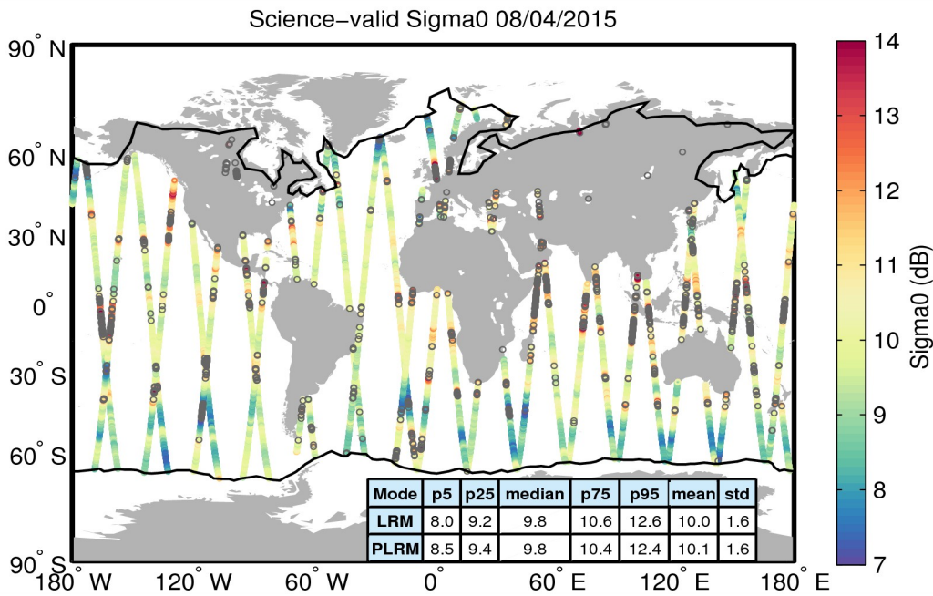
Figure 27. Geographical distribution of science-valid sigma0 data over oceans and lakes for 08/04/2015. The statistical values shown in the table refer to the sigma0 in dB and are calculated separately for LRM and PLRM regions. The black lines mark the outer limit of the Arctic and Antarctic polar polygons. Gray circles denote records that have been rejected based on the editing criteria described in Table 4.
