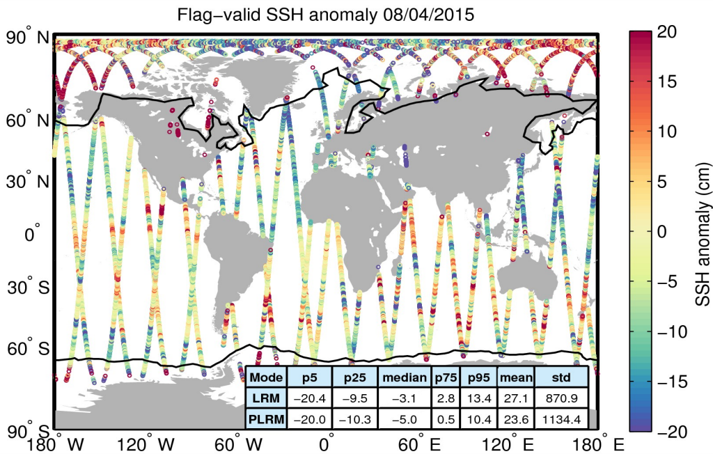
Figure 5. Geographical distribution of flag-valid 1-Hz SSH anomaly data over oceans and lakes for 08/04/2015. The statistical values shown in the table refer to the SSH anomaly in cm and are calculated separately for LRM and PLRM regions. Measurements taken over polar polygons have been excluded from the computation of the statistical values. The black lines mark the outer limit of the Arctic and Antarctic polar polygons.
