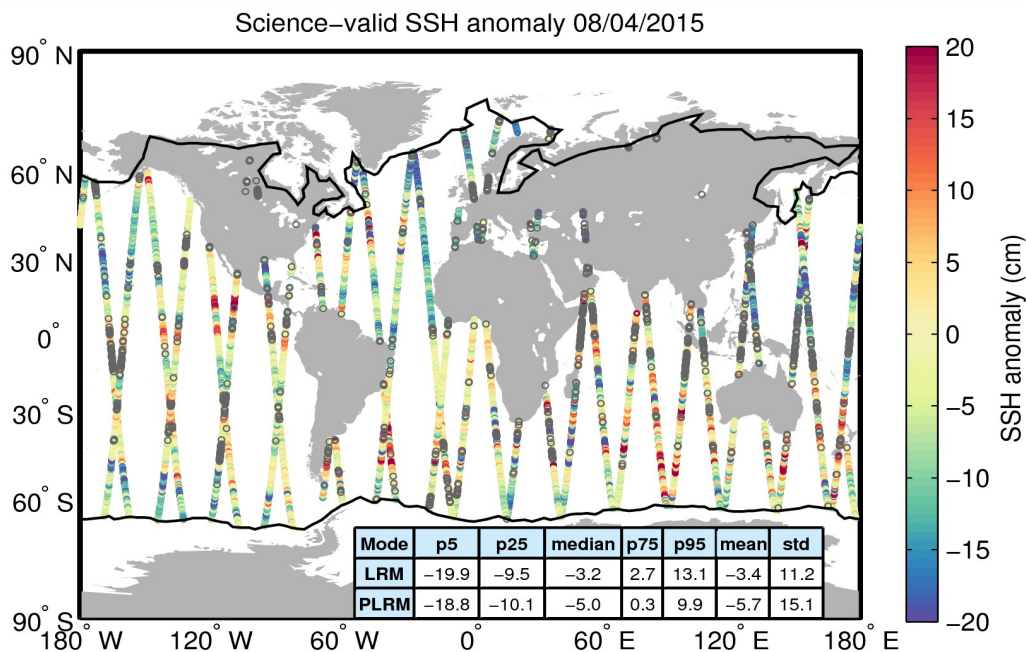
Figure 10. Geographical distribution of science-valid SSH anomaly data over oceans and lakes for 08/04/2015. The statistical values shown in the table refer to the SSH anomaly in cm and are calculated separately for LRM and PLRM regions. The black lines mark the outer limit of the Arctic and Antarctic polar polygons. Gray circles denote records that have been rejected based on the editing criteria described in Table 2.
