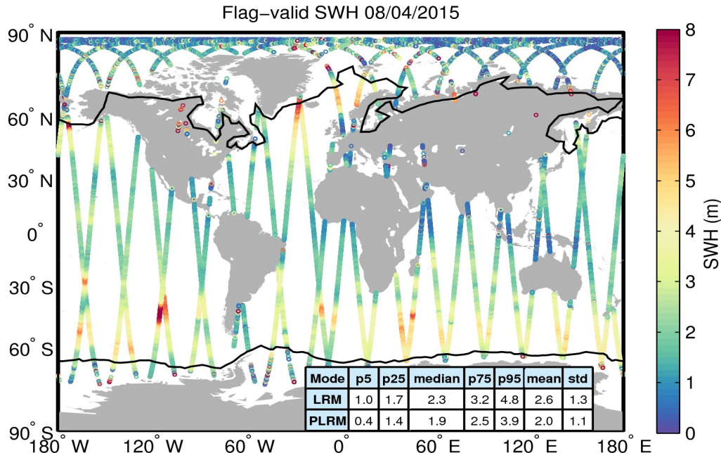
Figure 15. Geographical distribution of flag-valid SWH data over oceans and lakes for 08/04/2015. The statistical values shown in the table refer to the SWH in m and are calculated separately for LRM and PLRM regions. Measurements taken over polar polygons have been excluded from the computation of the statistical values. The black lines mark the outer limit of the Arctic and Antarctic polar polygons.
