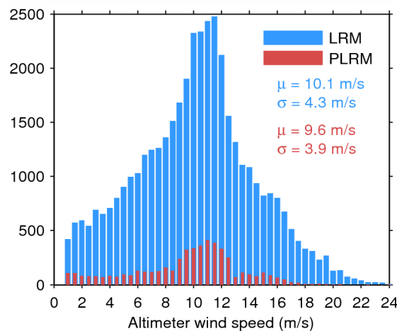
Figure 35. Histogram of science-valid wind over oceans and lakes for LRM (blue) and PLRM (red) for 08/04/2015. The mean ( \mu ) and standard deviation ( \sigma ) are also shown. Note that values larger than 24 m/s are excluded from the histogram for the sake of readability but not from the computation of \mu and \sigma .
