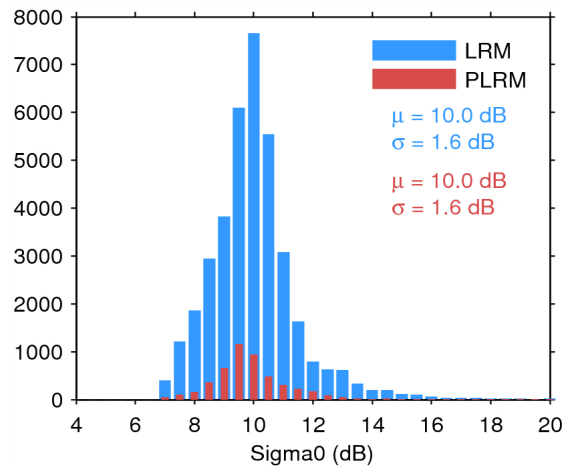
Figure 28. Histogram of science-valid sigma0 over oceans and lakes for LRM (blue) and PLRM (red) for 07/04/2015. The mean ( \mu ) and standard deviation ( \sigma ) are also shown. Note that values outside [4 20] dB are excluded from the histogram for the sake of readability but not from the computation of \mu and \sigma .
