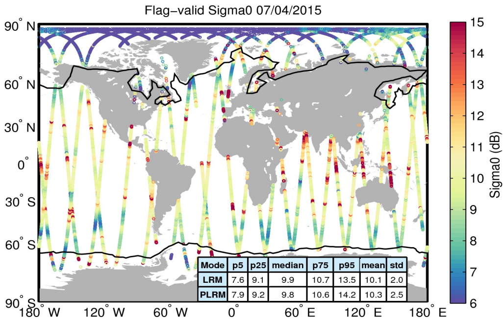
Figure 23. Geographical distribution of flag-valid sigma0 data over oceans and lakes for 07/04/2015. The statistical values shown in the table refer to the sigma0 in dB and are calculated separately for LRM and PLRM regions. Measurements taken over polar polygons have been excluded from the computation of the statistical values. The black lines mark the outer limit of the Arctic and Antarctic polar polygons.
