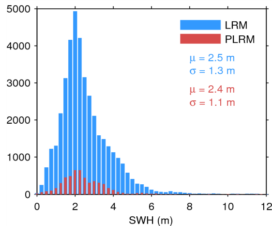
Figure 17. Histogram of flag-valid SWH over oceans and lakes for LRM (blue) and PLRM (red) for 07/04/2015. The mean ( \mu ) and standard deviation ( \sigma ) are also shown. Note that values larger than 12 m are excluded from the histogram for the sake of readability but not from the computation of \mu and \sigma .
