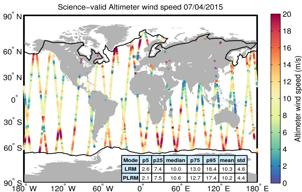
Figure 34. Geographical distribution of science-valid wind data over oceans and lakes for 07/04/2015. The statistical values shown in the table refer to the wind in m/s and are calculated separately for LRM and PLRM regions. The black lines mark the outer limit of the Arctic and Antarctic polar polygons. Gray circles denote records that have been rejected based on the editing criteria described in Table 5.
