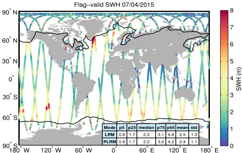
Figure 15. Geographical distribution of flag-valid SWH data over oceans and lakes for 07/04/2015. The statistical values shown in the table refer to the SWH in m and are calculated separately for LRM and PLRM regions. Measurements taken over polar polygons have been excluded from the computation of the statistical values. The black lines mark the outer limit of the Arctic and Antarctic polar polygons.
