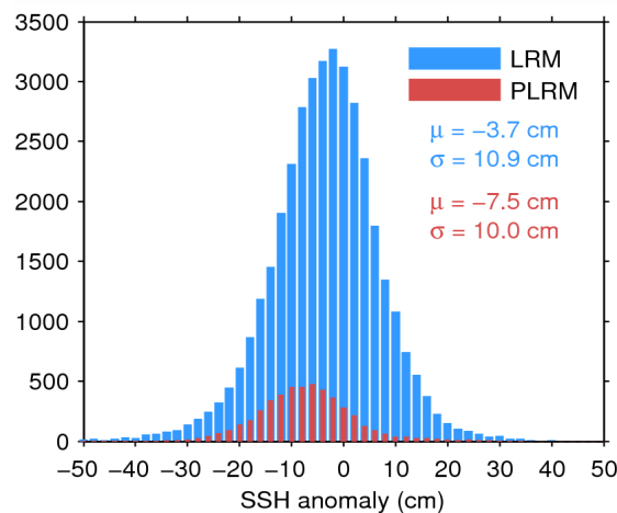
Figure 11. Histogram of science-valid SSH anomaly over oceans and lakes for LRM (blue) and PLRM (red) for 07/04/2015. The mean ( \mu ) and standard deviation ( \sigma ) are also shown. Note that values outside [-50 50] cm are excluded from the histogram for the sake of readability but not from the computation of \mu and \sigma .
