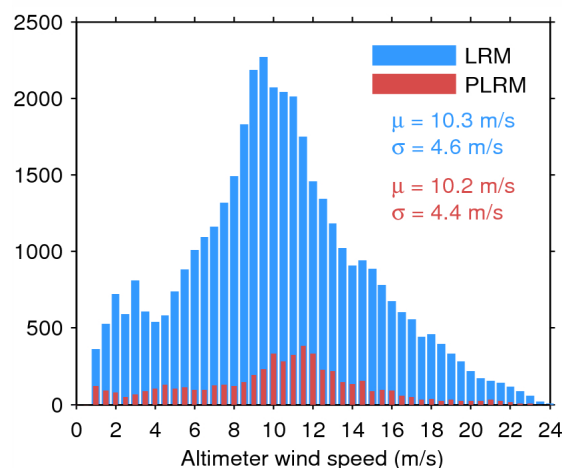
Figure 35. Histogram of science-valid wind over oceans and lakes for LRM (blue) and PLRM (red) for 07/04/2015. The mean ( \mu ) and standard deviation ( \sigma ) are also shown. Note that values larger than 24 m/s are excluded from the histogram for the sake of readability but not from the computation of \mu and \sigma .
