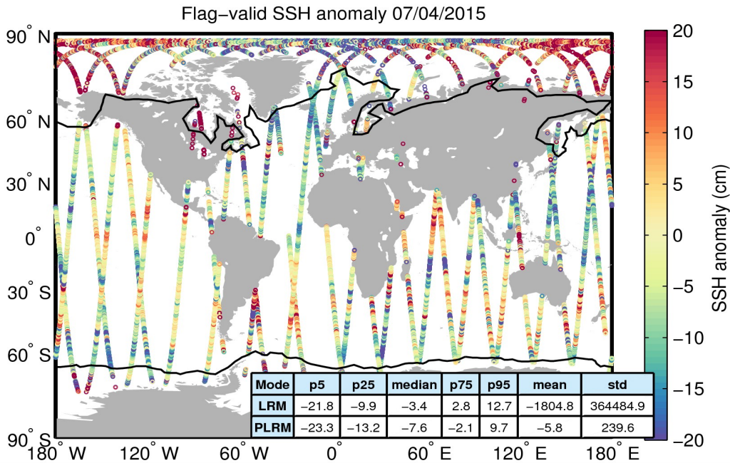
Figure 5. Geographical distribution of flag-valid 1-Hz SSH anomaly data over oceans and lakes for 07/04/2015. The statistical values shown in the table refer to the SSH anomaly in cm and are calculated separately for LRM and PLRM regions. Measurements taken over polar polygons have been excluded from the computation of the statistical values. The black lines mark the outer limit of the Arctic and Antarctic polar polygons.
