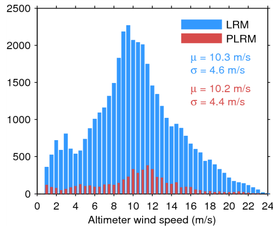
Figure 33. Histogram of flag-valid wind over oceans and lakes for LRM (blue) and PLRM (red) for 07/04/2015. The mean ( \mu ) and standard deviation ( \sigma ) are also shown. Note that values larger than 24 m/s are excluded from the histogram for the sake of readability but not from the computation of \mu and \sigma .
