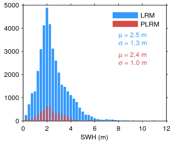
Figure 20. Histogram of science-valid SWH over oceans and lakes for LRM (blue) and PLRM (red) for 07/04/2015. The mean ( \mu ) and standard deviation ( \sigma ) are also shown. Note that values larger than 12 m are excluded from the histogram for the sake of readability but not from the computation of \mu and \sigma .
