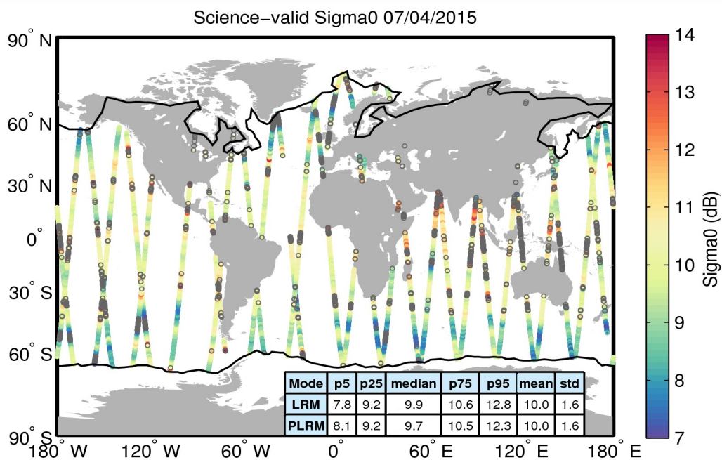
Figure 27. Geographical distribution of science-valid sigma0 data over oceans and lakes for 07/04/2015. The statistical values shown in the table refer to the sigma0 in dB and are calculated separately for LRM and PLRM regions. The black lines mark the outer limit of the Arctic and Antarctic polar polygons. Gray circles denote records that have been rejected based on the editing criteria described in Table 4.
