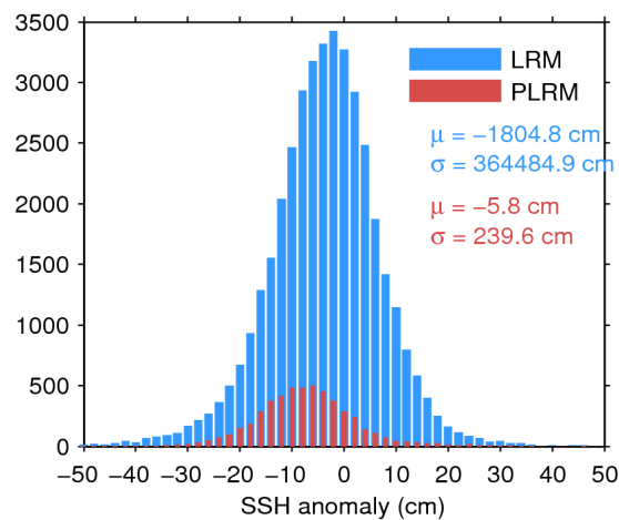
Figure 7. Histogram of flag-valid SSH anomaly over oceans and lakes for LRM (blue) and PLRM (red) for 07/04/2015. The mean ( \mu ) and standard deviation ( \sigma ) are also shown. Note that values outside [-50\ 50] cm are excluded from the histogram for the sake of readability but not from the computation of \mu and \sigma .
