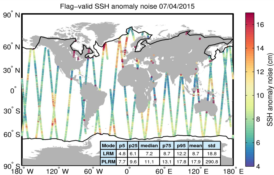
Figure 8. Geographical distribution of flag-valid 20-Hz SSH anomaly measurement noise over oceans and lakes for 07/04/2015. The statistical values shown in the table refer to the SSH anomaly noise and are calculated separately for LRM and PLRM regions. Measurements taken over polar polygons have been excluded from the computation of the statistical values. The black lines mark the outer limit of the Arctic and Antarctic polar polygons.
