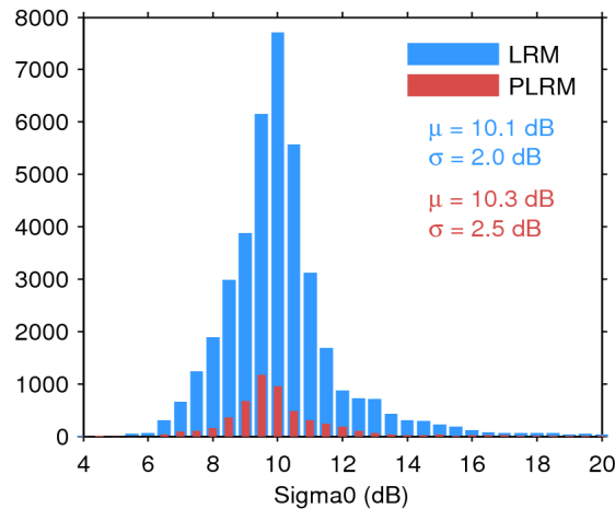
Figure 25. Histogram of flag-valid sigma0 over oceans and lakes for LRM (blue) and PLRM (red) for 07/04/2015. The mean ( \mu ) and standard deviation ( \sigma ) are also shown. Note that values outside [4 20] dB are excluded from the histogram for the sake of readability but not from the computation of \mu and \sigma .
