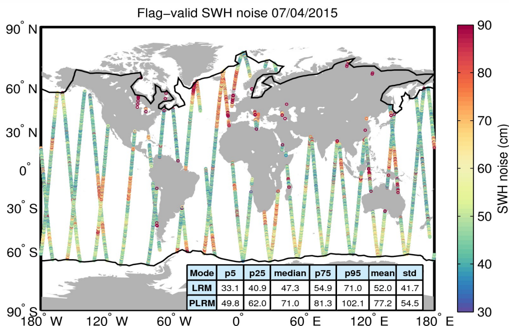
Figure 18. Geographical distribution of flag-valid 20-Hz SWH measurement noise over oceans and lakes for 07/04/2015. The statistical values shown in the table refer to the SWH noise and are calculated separately for LRM and PLRM regions. Measurements taken over polar polygons have been excluded from the computation of the statistical values. The black lines mark the outer limit of the Arctic and Antarctic polar polygons.
