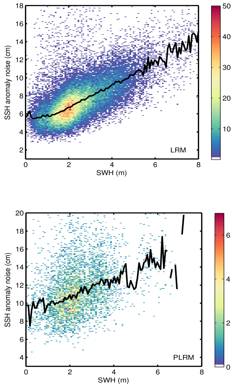
Figure 9. 2D histogram showing flag-valid SSH anomaly noise as a function of SWH for LRM (top) and PLRM (bottom) for 07/04/2015. The black line denotes the median SSH anomaly as a function of SWH.
