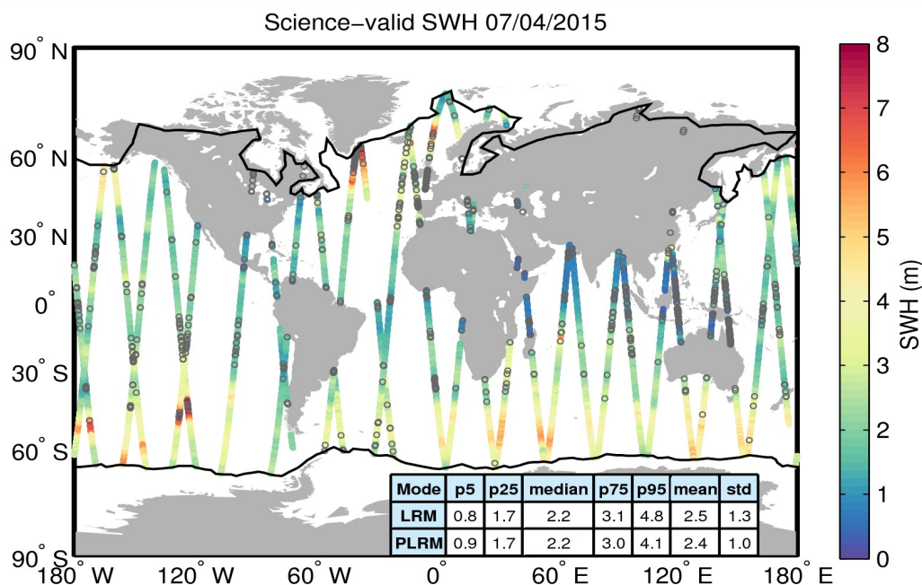
Figure 19. Geographical distribution of science-valid SWH data over oceans and lakes for 07/04/2015. The statistical values shown in the table refer to the SWH in m and are calculated separately for LRM and PLRM regions. The black lines mark the outer limit of the Arctic and Antarctic polar polygons. Gray circles denote records that have been rejected based on the editing criteria described in Table 3.
