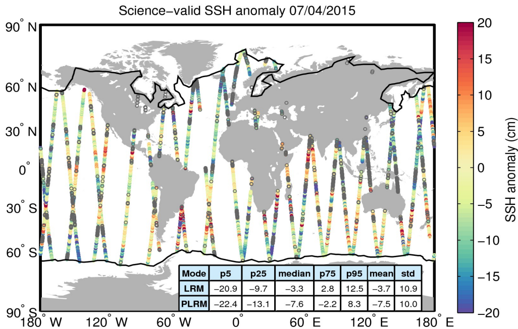
Figure 10. Geographical distribution of science-valid SSH anomaly data over oceans and lakes for 07/04/2015. The statistical values shown in the table refer to the SSH anomaly in cm and are calculated separately for LRM and PLRM regions. The black lines mark the outer limit of the Arctic and Antarctic polar polygons. Gray circles denote records that have been rejected based on the editing criteria described in Table 2.
