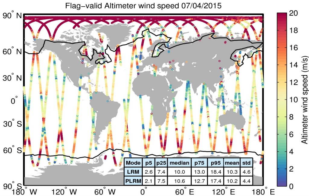
Figure 31. Geographical distribution of flag-valid wind data over oceans and lakes for 07/04/2015. The statistical values shown in the table refer to the wind in m/s and are calculated separately for LRM and PLRM regions. Measurements taken over polar polygons have been excluded from the computation of the statistical values. The black lines mark the outer limit of the Arctic and Antarctic polar polygons.
