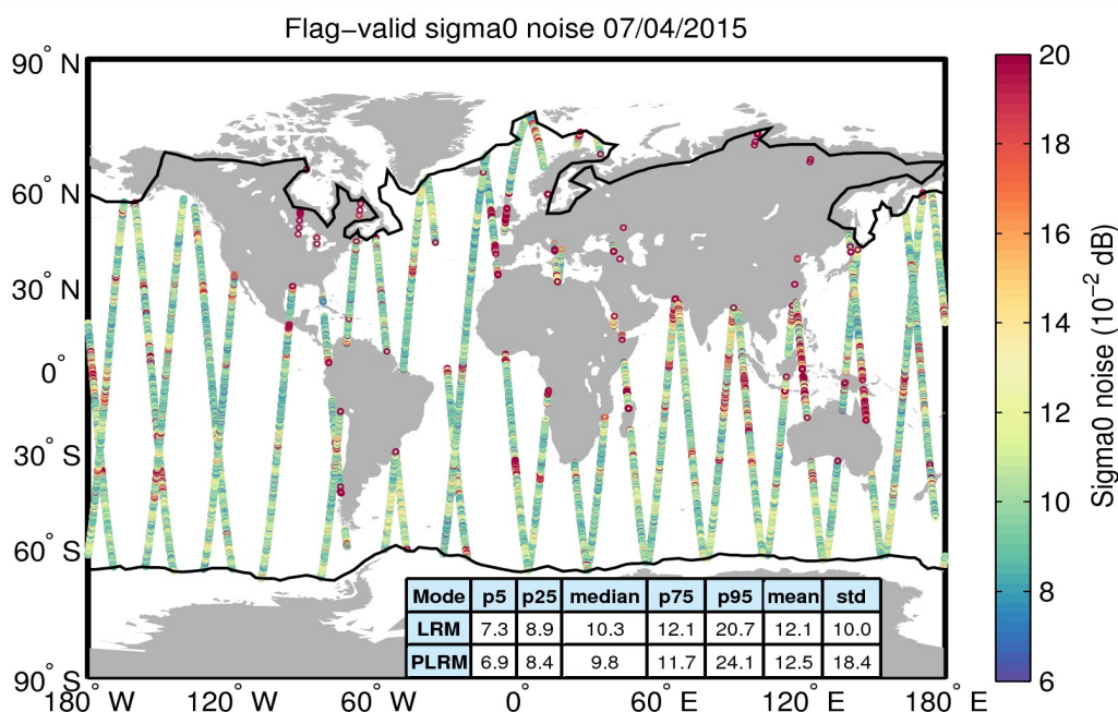
Figure 26. Geographical distribution of flag-valid 20-Hz sigma0 measurement noise over oceans and lakes for 07/04/2015. The statistical values shown in the table refer to the sigma0 noise and are calculated separately for LRM and PLRM regions. Measurements taken over polar polygons have been excluded from the computation of the statistical values. The black lines mark the outer limit of the Arctic and Antarctic polar polygons.
