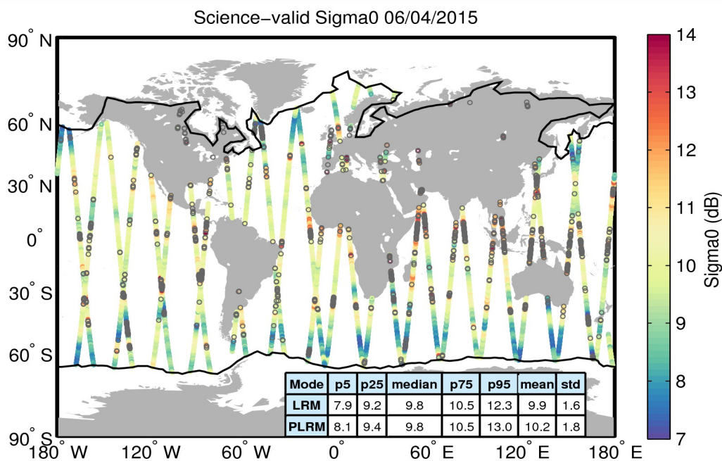
Figure 27. Geographical distribution of science-valid sigma0 data over oceans and lakes for 06/04/2015. The statistical values shown in the table refer to the sigma0 in dB and are calculated separately for LRM and PLRM regions. The black lines mark the outer limit of the Arctic and Antarctic polar polygons. Gray circles denote records that have been rejected based on the editing criteria described in Table 4.
