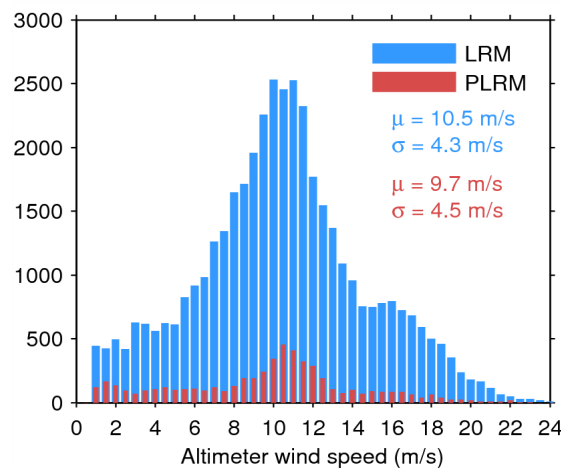
Figure 35. Histogram of science-valid wind over oceans and lakes for LRM (blue) and PLRM (red) for 06/04/2015. The mean ( \mu ) and standard deviation ( \sigma ) are also shown. Note that values larger than 24 m/s are excluded from the histogram for the sake of readability but not from the computation of \mu and \sigma .
