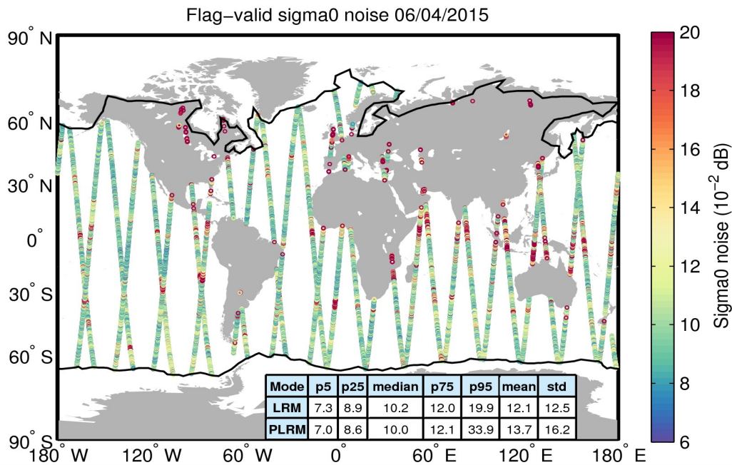
Figure 26. Geographical distribution of flag-valid 20-Hz sigma0 measurement noise over oceans and lakes for 06/04/2015. The statistical values shown in the table refer to the sigma0 noise and are calculated separately for LRM and PLRM regions. Measurements taken over polar polygons have been excluded from the computation of the statistical values. The black lines mark the outer limit of the Arctic and Antarctic polar polygons.
