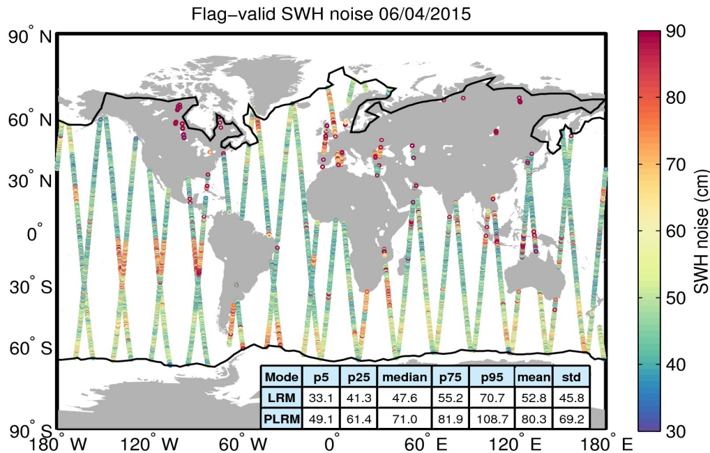
Figure 18. Geographical distribution of flag-valid 20-Hz SWH measurement noise over oceans and lakes for 06/04/2015. The statistical values shown in the table refer to the SWH noise and are calculated separately for LRM and PLRM regions. Measurements taken over polar polygons have been excluded from the computation of the statistical values. The black lines mark the outer limit of the Arctic and Antarctic polar polygons.
