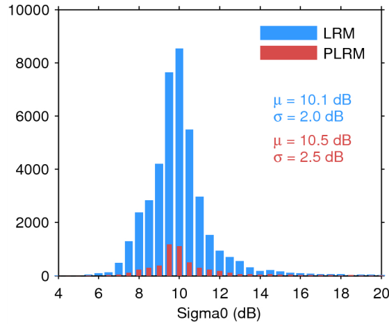
Figure 25. Histogram of flag-valid sigma0 over oceans and lakes for LRM (blue) and PLRM (red) for 06/04/2015. The mean ( \mu ) and standard deviation ( \sigma ) are also shown. Note that values outside [4 20] dB are excluded from the histogram for the sake of readability but not from the computation of \mu and \sigma .
