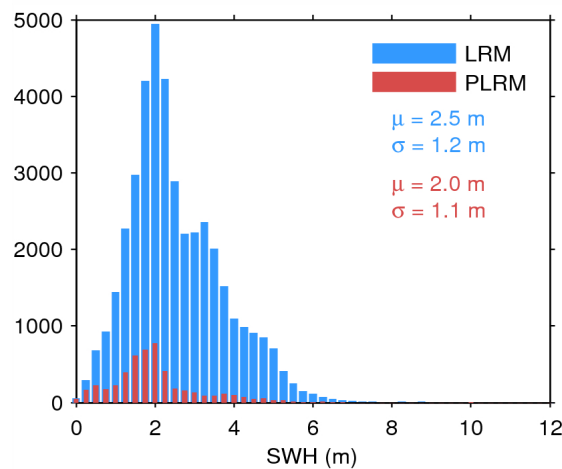
Figure 20. Histogram of science-valid SWH over oceans and lakes for LRM (blue) and PLRM (red) for 06/04/2015. The mean ( \mu ) and standard deviation ( \sigma ) are also shown. Note that values larger than 12 m are excluded from the histogram for the sake of readability but not from the computation of \mu and \sigma .
