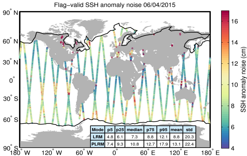
Figure 8. Geographical distribution of flag-valid 20-Hz SSH anomaly measurement noise over oceans and lakes for 06/04/2015. The statistical values shown in the table refer to the SSH anomaly noise and are calculated separately for LRM and PLRM regions. Measurements taken over polar polygons have been excluded from the computation of the statistical values. The black lines mark the outer limit of the Arctic and Antarctic polar polygons.
