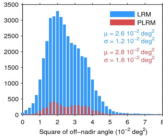
Figure 39. Histogram of flag-valid mispointing over oceans and lakes for LRM (blue) and PLRM (red) for 06/04/2015. Only positive values have been considered. The mean ( \mu ) and standard deviation ( \sigma ) are also shown. Note that values larger than 8 \cdot 10^{-2} \text{ deg}^2 are excluded from the histogram for the sake of readability but not from the computation of \mu and \sigma .
