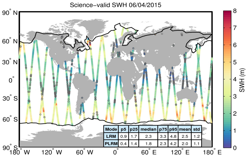
Figure 19. Geographical distribution of science-valid SWH data over oceans and lakes for 06/04/2015. The statistical values shown in the table refer to the SWH in m and are calculated separately for LRM and PLRM regions. The black lines mark the outer limit of the Arctic and Antarctic polar polygons. Gray circles denote records that have been rejected based on the editing criteria described in Table 3.
