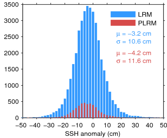
Figure 11. Histogram of science-valid SSH anomaly over oceans and lakes for LRM (blue) and PLRM (red) for 06/04/2015. The mean ( \mu ) and standard deviation ( \sigma ) are also shown. Note that values outside [-50\ 50] cm are excluded from the histogram for the sake of readability but not from the computation of \mu and \sigma .
