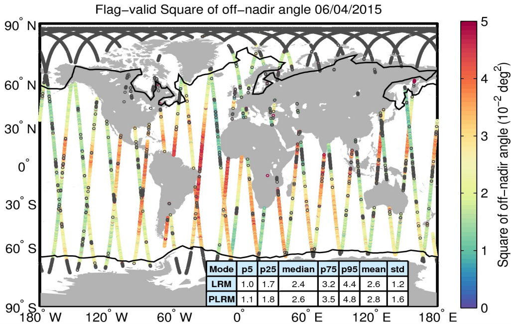
Figure 37. Geographical distribution of flag-valid mispointing data over oceans and lakes for 06/04/2015. The statistical values shown in the table refer to the mispointing in 10^{-2} \text{ deg}^2 and are calculated separately for LRM and PLRM regions. Measurements taken over polar polygons have been excluded from the computation of the statistical values. The black lines mark the outer limit of the Arctic and Antarctic polar polygons. Gray circles denote negative values.
