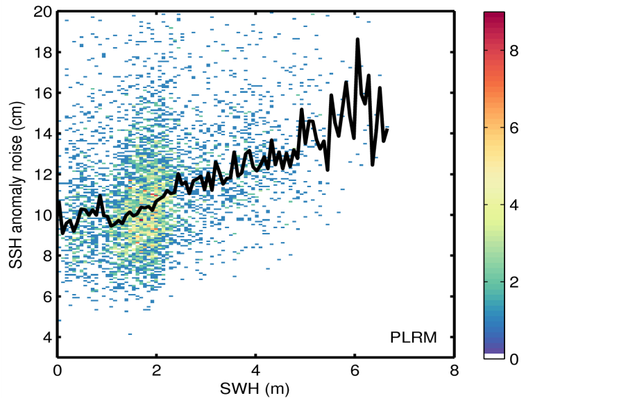
Figure 9. 2D histogram showing flag-valid SSH anomaly noise as a function of SWH for LRM (top) and PLRM (bottom) for 06/04/2015. The black line denotes the median SSH anomaly as a function of SWH.
