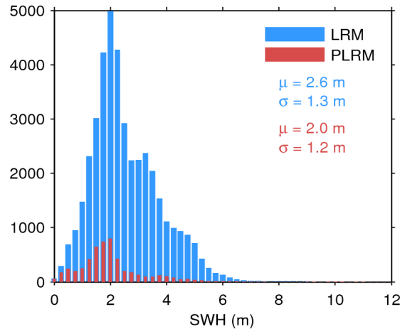
Figure 17. Histogram of flag-valid SWH over oceans and lakes for LRM (blue) and PLRM (red) for 06/04/2015. The mean ( \mu ) and standard deviation ( \sigma ) are also shown. Note that values larger than 12 m are excluded from the histogram for the sake of readability but not from the computation of \mu and \sigma .
