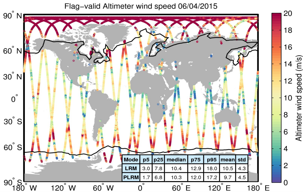
Figure 31. Geographical distribution of flag-valid wind data over oceans and lakes for 06/04/2015. The statistical values shown in the table refer to the wind in m/s and are calculated separately for LRM and PLRM regions. Measurements taken over polar polygons have been excluded from the computation of the statistical values. The black lines mark the outer limit of the Arctic and Antarctic polar polygons.
