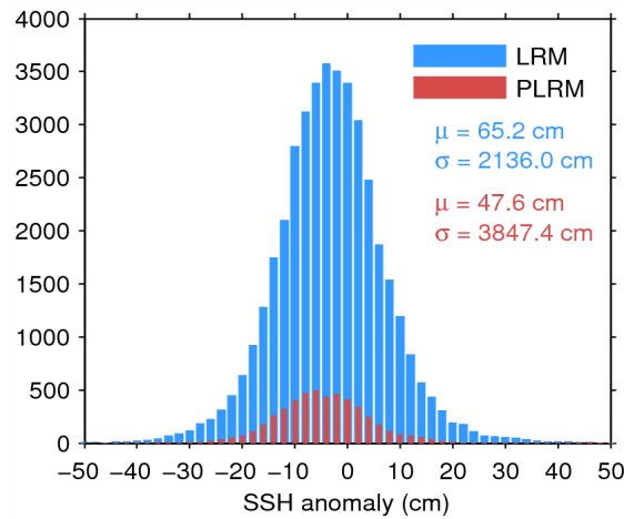
Figure 7. Histogram of flag-valid SSH anomaly over oceans and lakes for LRM (blue) and PLRM (red) for 06/04/2015. The mean ( \mu ) and standard deviation ( \sigma ) are also shown. Note that values outside [-50\ 50] cm are excluded from the histogram for the sake of readability but not from the computation of \mu and \sigma .
