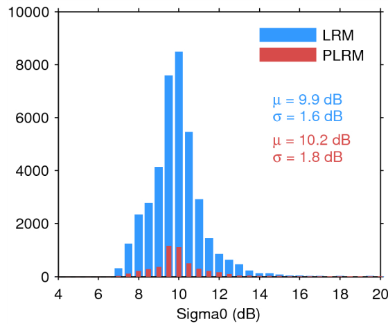
Figure 28. Histogram of science-valid sigma0 over oceans and lakes for LRM (blue) and PLRM (red) for 06/04/2015. The mean ( \mu ) and standard deviation ( \sigma ) are also shown. Note that values outside [4 20] dB are excluded from the histogram for the sake of readability but not from the computation of \mu and \sigma .
