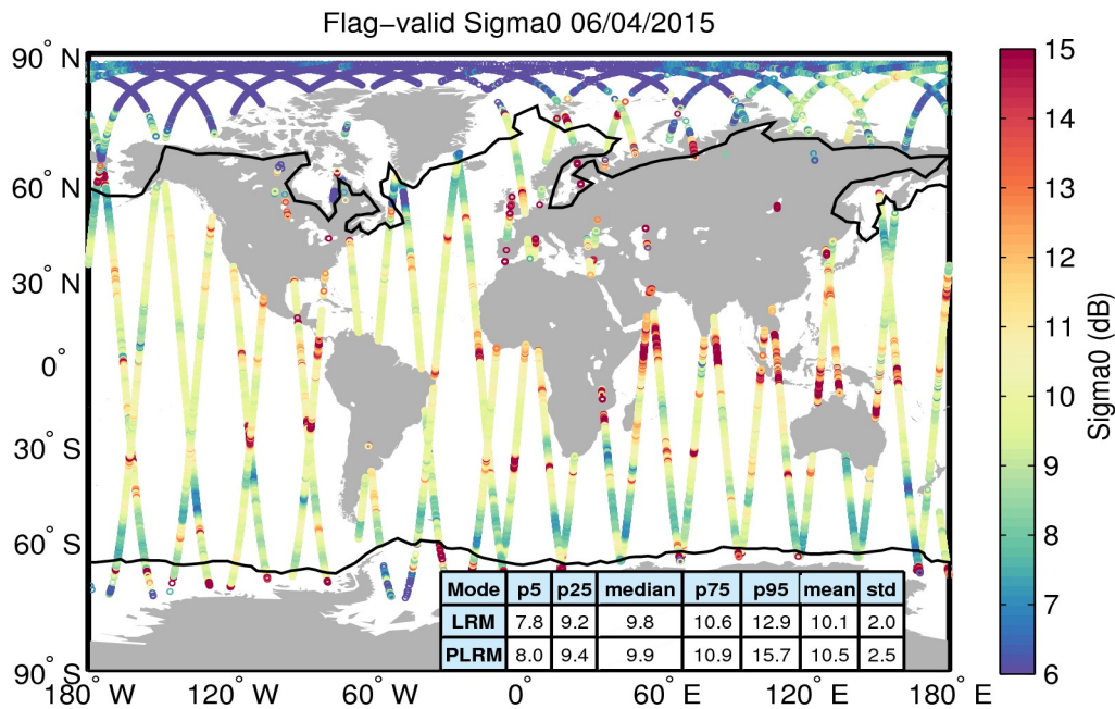
Figure 23. Geographical distribution of flag-valid sigma0 data over oceans and lakes for 06/04/2015. The statistical values shown in the table refer to the sigma0 in dB and are calculated separately for LRM and PLRM regions. Measurements taken over polar polygons have been excluded from the computation of the statistical values. The black lines mark the outer limit of the Arctic and Antarctic polar polygons.
