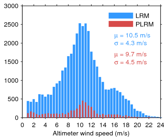
Figure 33. Histogram of flag-valid wind over oceans and lakes for LRM (blue) and PLRM (red) for 06/04/2015. The mean ( \mu ) and standard deviation ( \sigma ) are also shown. Note that values larger than 24 m/s are excluded from the histogram for the sake of readability but not from the computation of \mu and \sigma .
