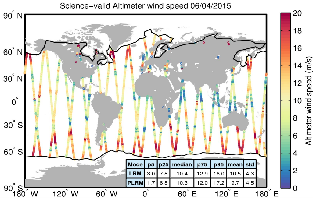
Figure 34. Geographical distribution of science-valid wind data over oceans and lakes for 06/04/2015. The statistical values shown in the table refer to the wind in m/s and are calculated separately for LRM and PLRM regions. The black lines mark the outer limit of the Arctic and Antarctic polar polygons. Gray circles denote records that have been rejected based on the editing criteria described in Table 5.
