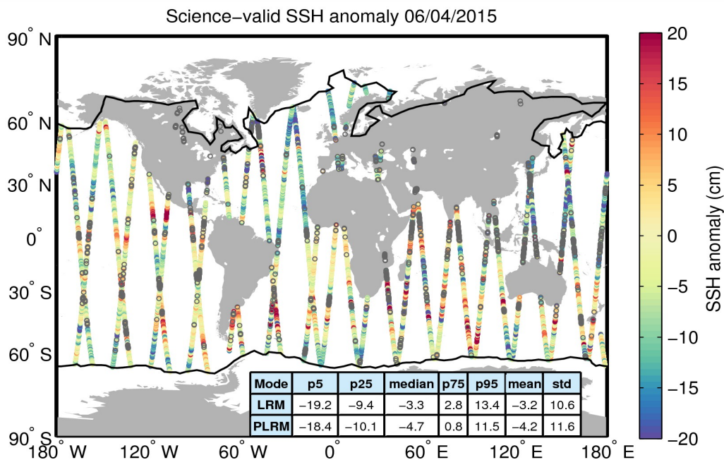
Figure 10. Geographical distribution of science-valid SSH anomaly data over oceans and lakes for 06/04/2015. The statistical values shown in the table refer to the SSH anomaly in cm and are calculated separately for LRM and PLRM regions. The black lines mark the outer limit of the Arctic and Antarctic polar polygons. Gray circles denote records that have been rejected based on the editing criteria described in Table 2.
