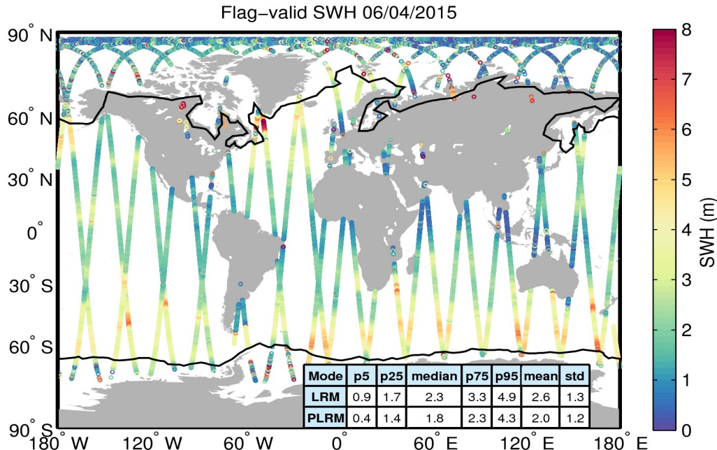
Figure 15. Geographical distribution of flag-valid SWH data over oceans and lakes for 06/04/2015. The statistical values shown in the table refer to the SWH in m and are calculated separately for LRM and PLRM regions. Measurements taken over polar polygons have been excluded from the computation of the statistical values. The black lines mark the outer limit of the Arctic and Antarctic polar polygons.
