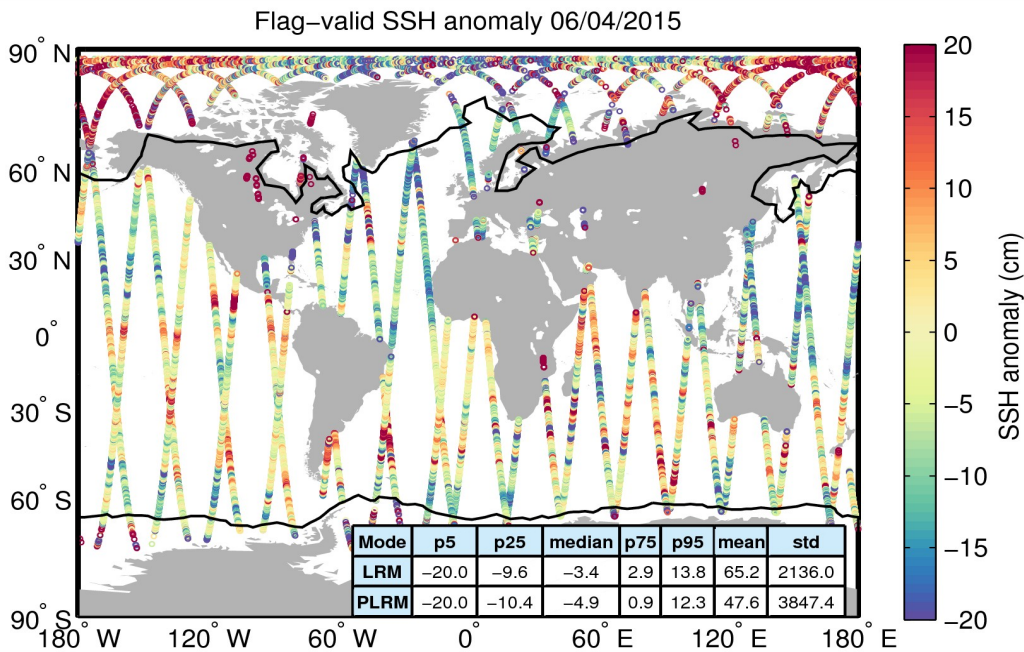
Figure 5. Geographical distribution of flag-valid 1-Hz SSH anomaly data over oceans and lakes for 06/04/2015. The statistical values shown in the table refer to the SSH anomaly in cm and are calculated separately for LRM and PLRM regions. Measurements taken over polar polygons have been excluded from the computation of the statistical values. The black lines mark the outer limit of the Arctic and Antarctic polar polygons.
