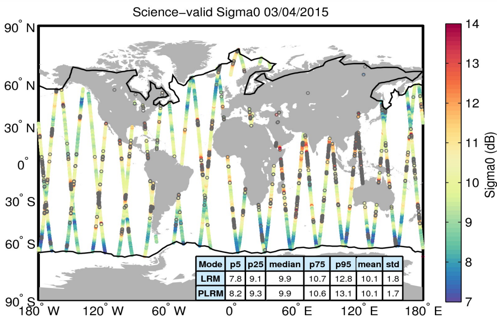
Figure 27. Geographical distribution of science-valid sigma0 data over oceans and lakes for 03/04/2015. The statistical values shown in the table refer to the sigma0 in dB and are calculated separately for LRM and PLRM regions. The black lines mark the outer limit of the Arctic and Antarctic polar polygons. Gray circles denote records that have been rejected based on the editing criteria described in Table 4.
