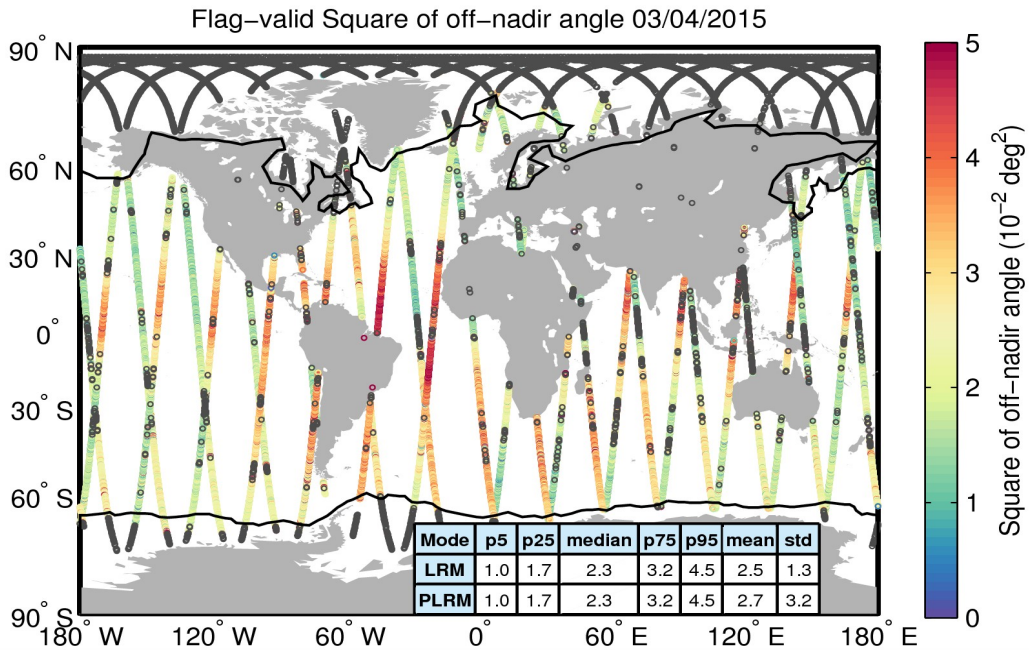
Figure 37. Geographical distribution of flag-valid mispointing data over oceans and lakes for 03/04/2015. The statistical values shown in the table refer to the mispointing in 10^{-2} \text{ deg}^2 and are calculated separately for LRM and PLRM regions. Measurements taken over polar polygons have been excluded from the computation of the statistical values. The black lines mark the outer limit of the Arctic and Antarctic polar polygons. Gray circles denote negative values.
