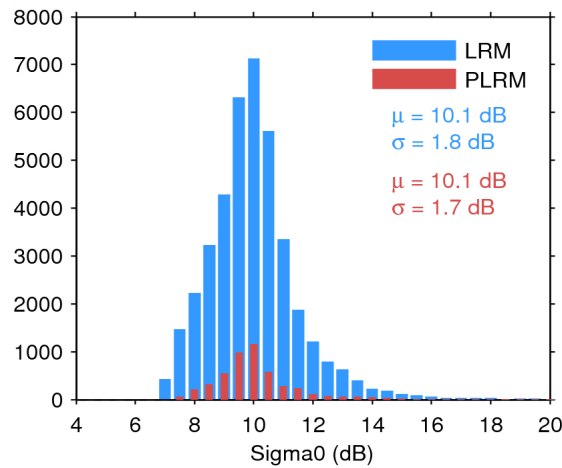
Figure 28. Histogram of science-valid sigma0 over oceans and lakes for LRM (blue) and PLRM (red) for 03/04/2015. The mean ( \mu ) and standard deviation ( \sigma ) are also shown. Note that values outside [4 20] dB are excluded from the histogram for the sake of readability but not from the computation of \mu and \sigma .
