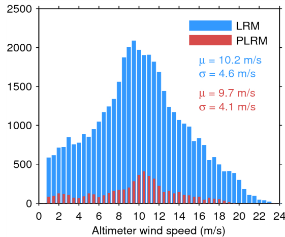
Figure 33. Histogram of flag-valid wind over oceans and lakes for LRM (blue) and PLRM (red) for 03/04/2015. The mean ( \mu ) and standard deviation ( \sigma ) are also shown. Note that values larger than 24 m/s are excluded from the histogram for the sake of readability but not from the computation of \mu and \sigma .
