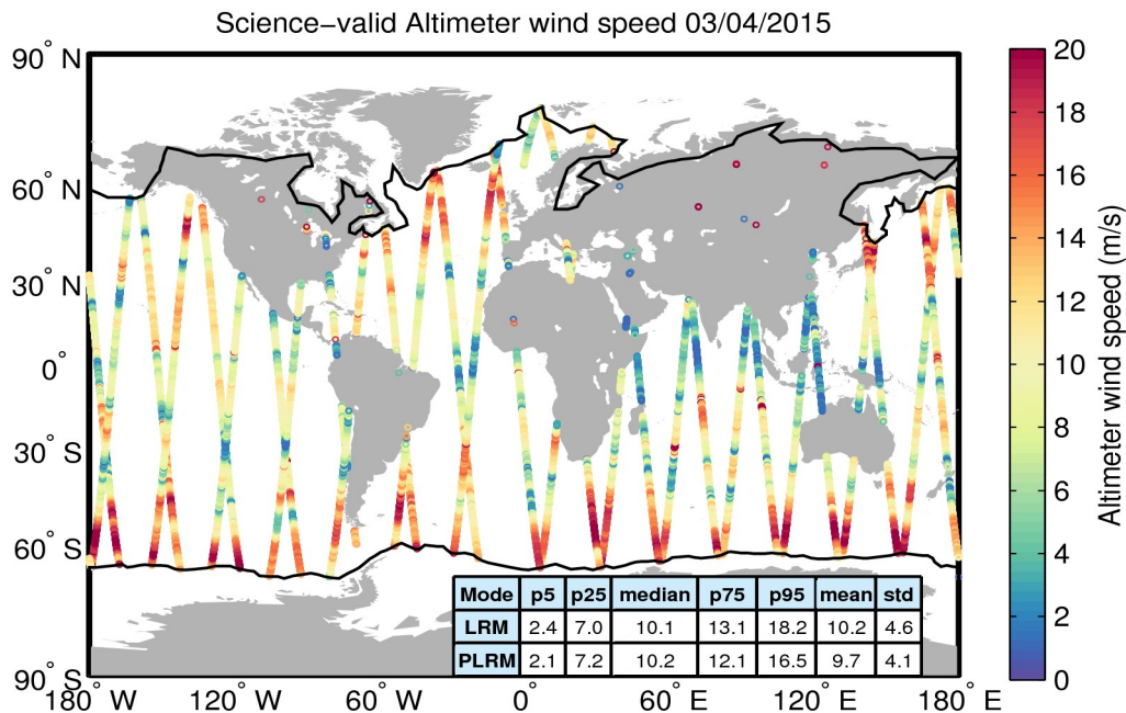
Figure 34. Geographical distribution of science-valid wind data over oceans and lakes for 03/04/2015. The statistical values shown in the table refer to the wind in m/s and are calculated separately for LRM and PLRM regions. The black lines mark the outer limit of the Arctic and Antarctic polar polygons. Gray circles denote records that have been rejected based on the editing criteria described in Table 5.
