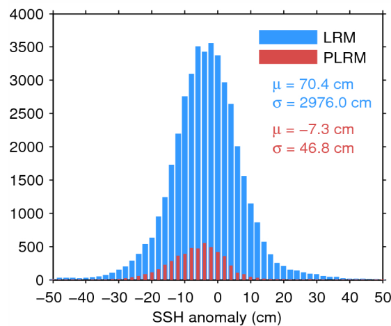
Figure 7. Histogram of flag-valid SSH anomaly over oceans and lakes for LRM (blue) and PLRM (red) for 03/04/2015. The mean ( \mu ) and standard deviation ( \sigma ) are also shown. Note that values outside [-50\ 50] cm are excluded from the histogram for the sake of readability but not from the computation of \mu and \sigma .
