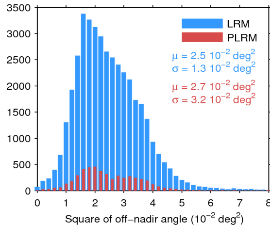
Figure 39. Histogram of flag-valid mispointing over oceans and lakes for LRM (blue) and PLRM (red) for 03/04/2015. Only positive values have been considered. The mean ( \mu ) and standard deviation ( \sigma ) are also shown. Note that values larger than 8 \cdot 10^{-2} \text{ deg}^2 are excluded from the histogram for the sake of readability but not from the computation of \mu and \sigma .
