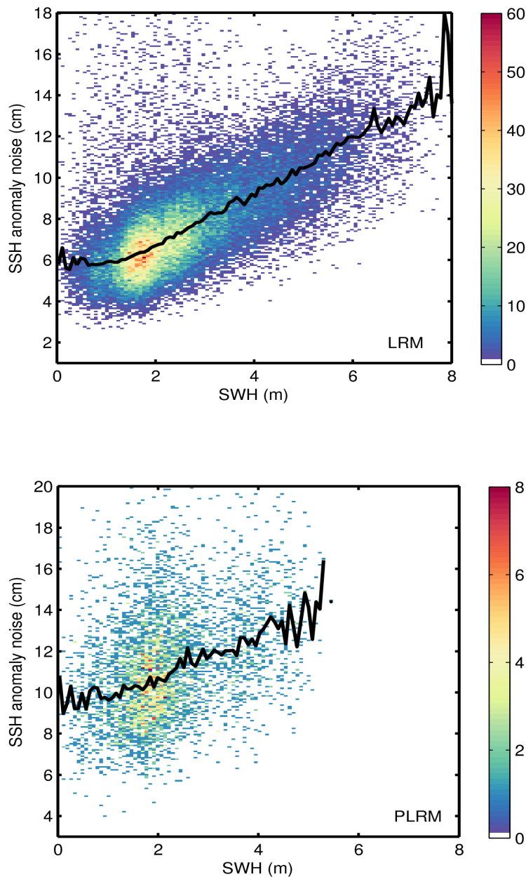
Figure 9. 2D histogram showing flag-valid SSH anomaly noise as a function of SWH for LRM (top) and PLRM (bottom) for 03/04/2015. The black line denotes the median SSH anomaly as a function of SWH.
