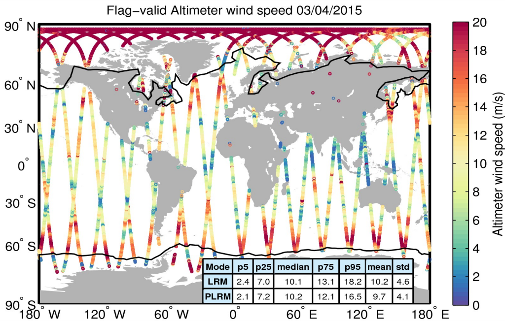
Figure 31. Geographical distribution of flag-valid wind data over oceans and lakes for 03/04/2015. The statistical values shown in the table refer to the wind in m/s and are calculated separately for LRM and PLRM regions. Measurements taken over polar polygons have been excluded from the computation of the statistical values. The black lines mark the outer limit of the Arctic and Antarctic polar polygons.
