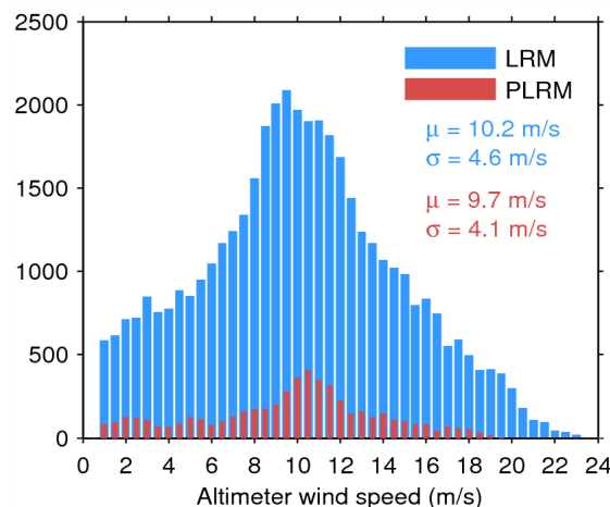
Figure 35. Histogram of science-valid wind over oceans and lakes for LRM (blue) and PLRM (red) for 03/04/2015. The mean ( \mu ) and standard deviation ( \sigma ) are also shown. Note that values larger than 24 m/s are excluded from the histogram for the sake of readability but not from the computation of \mu and \sigma .
