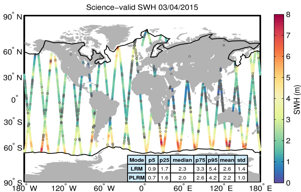
Figure 19. Geographical distribution of science-valid SWH data over oceans and lakes for 03/04/2015. The statistical values shown in the table refer to the SWH in m and are calculated separately for LRM and PLRM regions. The black lines mark the outer limit of the Arctic and Antarctic polar polygons. Gray circles denote records that have been rejected based on the editing criteria described in Table 3.
