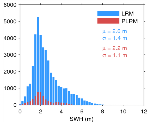
Figure 17. Histogram of flag-valid SWH over oceans and lakes for LRM (blue) and PLRM (red) for 03/04/2015. The mean ( \mu ) and standard deviation ( \sigma ) are also shown. Note that values larger than 12 m are excluded from the histogram for the sake of readability but not from the computation of \mu and \sigma .
