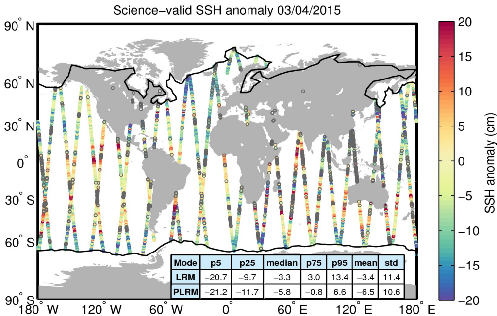
Figure 10. Geographical distribution of science-valid SSH anomaly data over oceans and lakes for 03/04/2015. The statistical values shown in the table refer to the SSH anomaly in cm and are calculated separately for LRM and PLRM regions. The black lines mark the outer limit of the Arctic and Antarctic polar polygons. Gray circles denote records that have been rejected based on the editing criteria described in Table 2.
