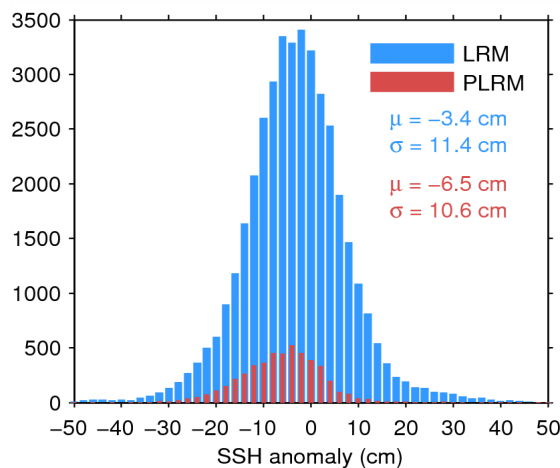
Figure 11. Histogram of science-valid SSH anomaly over oceans and lakes for LRM (blue) and PLRM (red) for 03/04/2015. The mean ( \mu ) and standard deviation ( \sigma ) are also shown. Note that values outside [-50 50] cm are excluded from the histogram for the sake of readability but not from the computation of \mu and \sigma .
