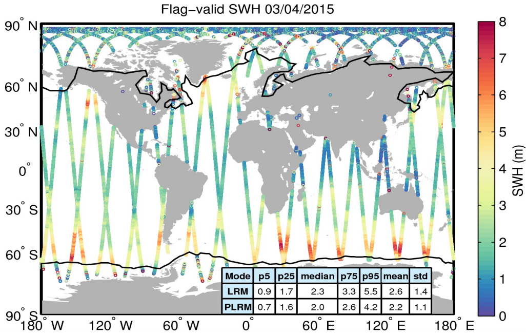
Figure 15. Geographical distribution of flag-valid SWH data over oceans and lakes for 03/04/2015. The statistical values shown in the table refer to the SWH in m and are calculated separately for LRM and PLRM regions. Measurements taken over polar polygons have been excluded from the computation of the statistical values. The black lines mark the outer limit of the Arctic and Antarctic polar polygons.
