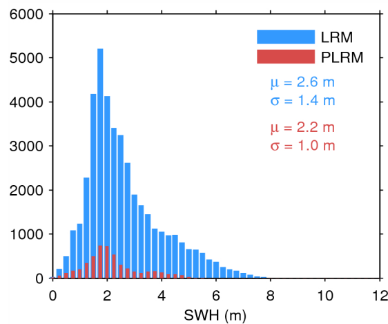
Figure 20. Histogram of science-valid SWH over oceans and lakes for LRM (blue) and PLRM (red) for 03/04/2015. The mean ( \mu ) and standard deviation ( \sigma ) are also shown. Note that values larger than 12 m are excluded from the histogram for the sake of readability but not from the computation of \mu and \sigma .
