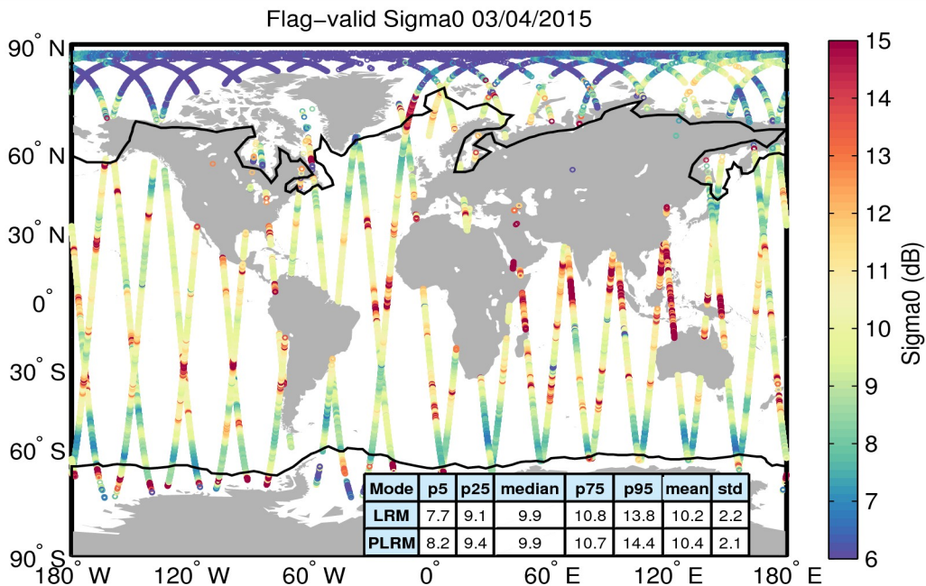
Figure 23. Geographical distribution of flag-valid sigma0 data over oceans and lakes for 03/04/2015. The statistical values shown in the table refer to the sigma0 in dB and are calculated separately for LRM and PLRM regions. Measurements taken over polar polygons have been excluded from the computation of the statistical values. The black lines mark the outer limit of the Arctic and Antarctic polar polygons.
