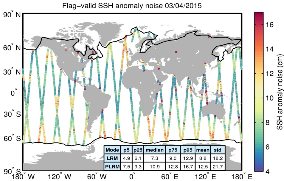
Figure 8. Geographical distribution of flag-valid 20-Hz SSH anomaly measurement noise over oceans and lakes for 03/04/2015. The statistical values shown in the table refer to the SSH anomaly noise and are calculated separately for LRM and PLRM regions. Measurements taken over polar polygons have been excluded from the computation of the statistical values. The black lines mark the outer limit of the Arctic and Antarctic polar polygons.
