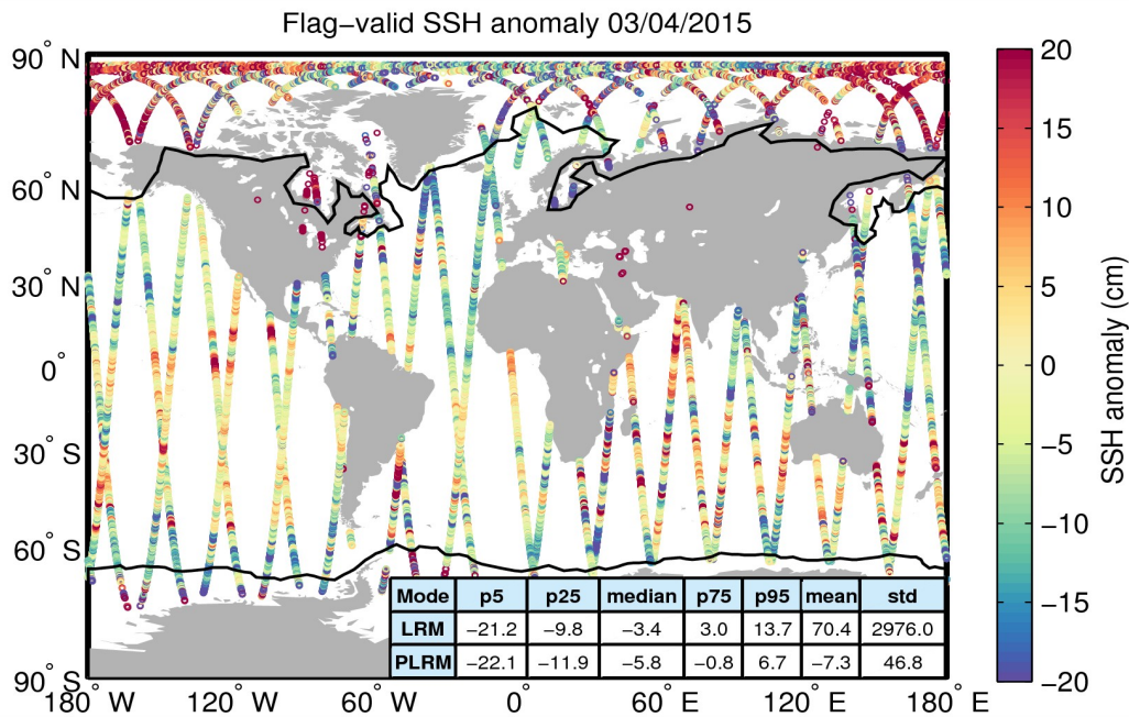
Figure 5. Geographical distribution of flag-valid 1-Hz SSH anomaly data over oceans and lakes for 03/04/2015. The statistical values shown in the table refer to the SSH anomaly in cm and are calculated separately for LRM and PLRM regions. Measurements taken over polar polygons have been excluded from the computation of the statistical values. The black lines mark the outer limit of the Arctic and Antarctic polar polygons.
