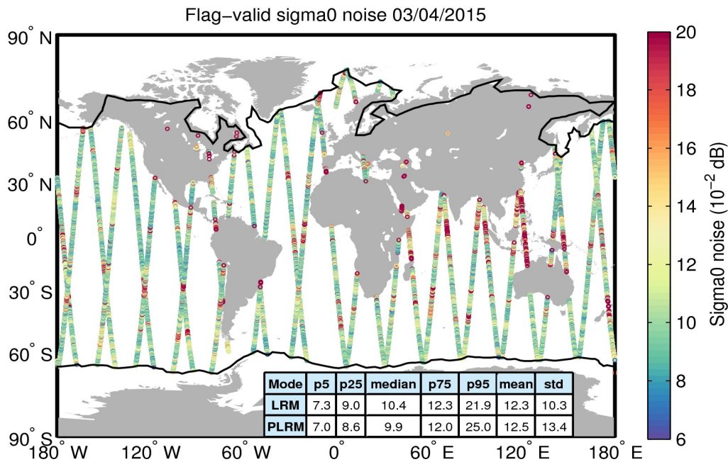
Figure 26. Geographical distribution of flag-valid 20-Hz sigma0 measurement noise over oceans and lakes for 03/04/2015. The statistical values shown in the table refer to the sigma0 noise and are calculated separately for LRM and PLRM regions. Measurements taken over polar polygons have been excluded from the computation of the statistical values. The black lines mark the outer limit of the Arctic and Antarctic polar polygons.
