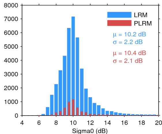
Figure 25. Histogram of flag-valid sigma0 over oceans and lakes for LRM (blue) and PLRM (red) for 03/04/2015. The mean ( \mu ) and standard deviation ( \sigma ) are also shown. Note that values outside [4 20] dB are excluded from the histogram for the sake of readability but not from the computation of \mu and \sigma .
