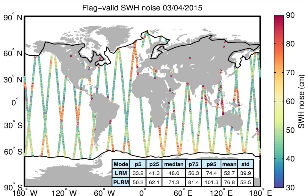
Figure 18. Geographical distribution of flag-valid 20-Hz SWH measurement noise over oceans and lakes for 03/04/2015. The statistical values shown in the table refer to the SWH noise and are calculated separately for LRM and PLRM regions. Measurements taken over polar polygons have been excluded from the computation of the statistical values. The black lines mark the outer limit of the Arctic and Antarctic polar polygons.
