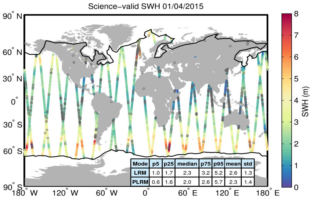
Figure 19. Geographical distribution of science-valid SWH data over oceans and lakes for 01/04/2015. The statistical values shown in the table refer to the SWH in m and are calculated separately for LRM and PLRM regions. The black lines mark the outer limit of the Arctic and Antarctic polar polygons. Gray circles denote records that have been rejected based on the editing criteria described in Table 3.
