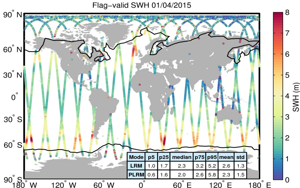
Figure 15. Geographical distribution of flag-valid SWH data over oceans and lakes for 01/04/2015. The statistical values shown in the table refer to the SWH in m and are calculated separately for LRM and PLRM regions. Measurements taken over polar polygons have been excluded from the computation of the statistical values. The black lines mark the outer limit of the Arctic and Antarctic polar polygons.
