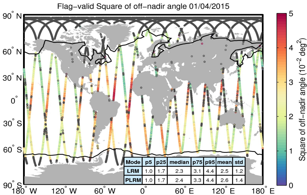
Figure 37. Geographical distribution of flag-valid mispointing data over oceans and lakes for 01/04/2015. The statistical values shown in the table refer to the mispointing in 10^{-2} \text{ deg}^2 and are calculated separately for LRM and PLRM regions. Measurements taken over polar polygons have been excluded from the computation of the statistical values. The black lines mark the outer limit of the Arctic and Antarctic polar polygons. Gray circles denote negative values.
