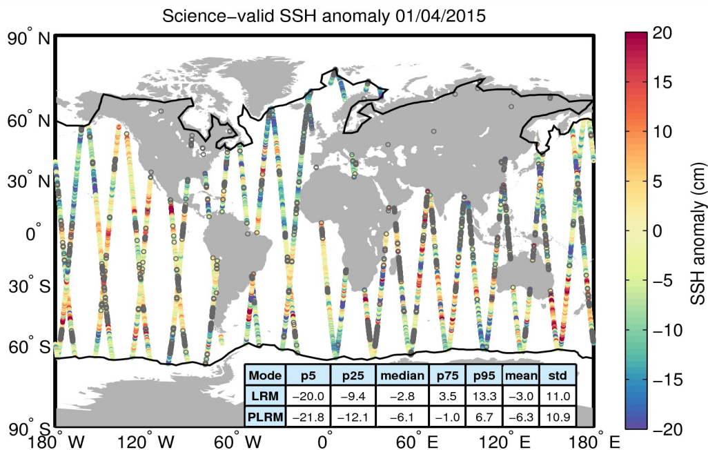
Figure 10. Geographical distribution of science-valid SSH anomaly data over oceans and lakes for 01/04/2015. The statistical values shown in the table refer to the SSH anomaly in cm and are calculated separately for LRM and PLRM regions. The black lines mark the outer limit of the Arctic and Antarctic polar polygons. Gray circles denote records that have been rejected based on the editing criteria described in Table 2.
