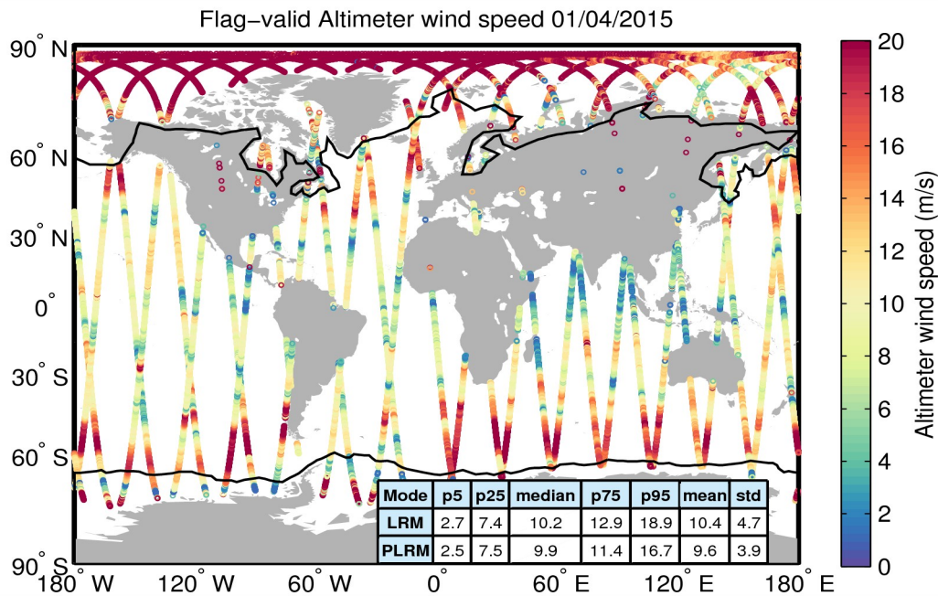
Figure 31. Geographical distribution of flag-valid wind data over oceans and lakes for 01/04/2015. The statistical values shown in the table refer to the wind in m/s and are calculated separately for LRM and PLRM regions. Measurements taken over polar polygons have been excluded from the computation of the statistical values. The black lines mark the outer limit of the Arctic and Antarctic polar polygons.
