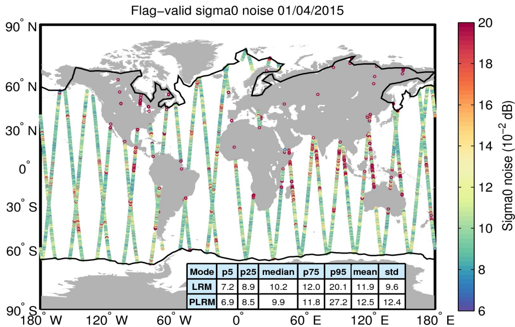
Figure 26. Geographical distribution of flag-valid 20-Hz sigma0 measurement noise over oceans and lakes for 01/04/2015. The statistical values shown in the table refer to the sigma0 noise and are calculated separately for LRM and PLRM regions. Measurements taken over polar polygons have been excluded from the computation of the statistical values. The black lines mark the outer limit of the Arctic and Antarctic polar polygons.
