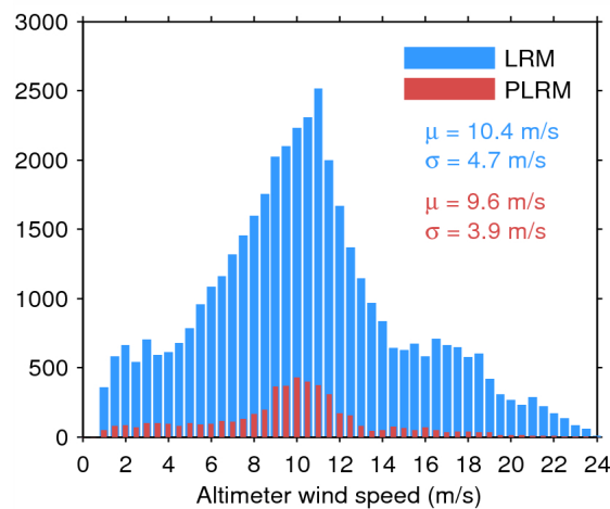
Figure 33. Histogram of flag-valid wind over oceans and lakes for LRM (blue) and PLRM (red) for 01/04/2015. The mean ( \mu ) and standard deviation ( \sigma ) are also shown. Note that values larger than 24 m/s are excluded from the histogram for the sake of readability but not from the computation of \mu and \sigma .
