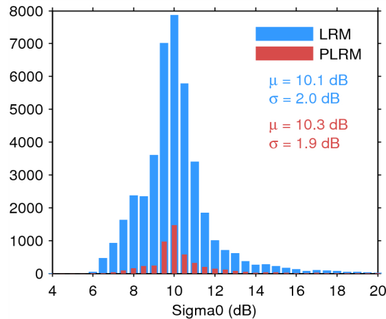
Figure 25. Histogram of flag-valid sigma0 over oceans and lakes for LRM (blue) and PLRM (red) for 01/04/2015. The mean ( \mu ) and standard deviation ( \sigma ) are also shown. Note that values outside [4 20] dB are excluded from the histogram for the sake of readability but not from the computation of \mu and \sigma .
