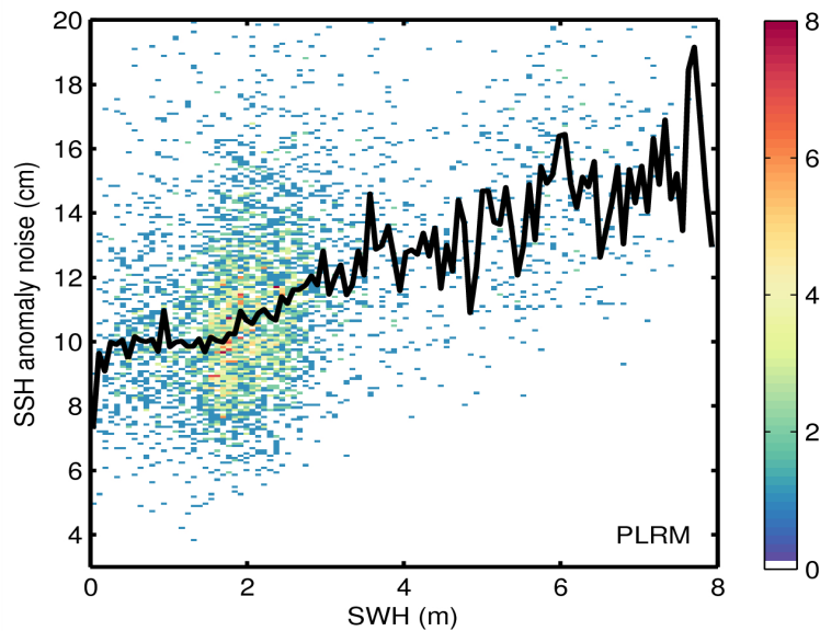
Figure 9. 2D histogram showing flag-valid SSH anomaly noise as a function of SWH for LRM (top) and PLRM (bottom) for 01/04/2015. The black line denotes the median SSH anomaly as a function of SWH.
