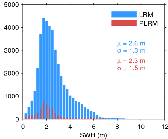
Figure 17. Histogram of flag-valid SWH over oceans and lakes for LRM (blue) and PLRM (red) for 01/04/2015. The mean ( \mu ) and standard deviation ( \sigma ) are also shown. Note that values larger than 12 m are excluded from the histogram for the sake of readability but not from the computation of \mu and \sigma .
