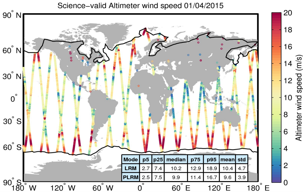
Figure 34. Geographical distribution of science-valid wind data over oceans and lakes for 01/04/2015. The statistical values shown in the table refer to the wind in m/s and are calculated separately for LRM and PLRM regions. The black lines mark the outer limit of the Arctic and Antarctic polar polygons. Gray circles denote records that have been rejected based on the editing criteria described in Table 5.
