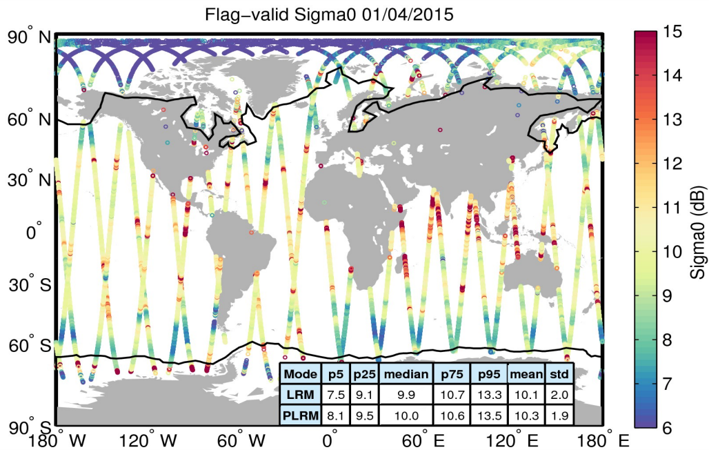
Figure 23. Geographical distribution of flag-valid sigma0 data over oceans and lakes for 01/04/2015. The statistical values shown in the table refer to the sigma0 in dB and are calculated separately for LRM and PLRM regions. Measurements taken over polar polygons have been excluded from the computation of the statistical values. The black lines mark the outer limit of the Arctic and Antarctic polar polygons.
