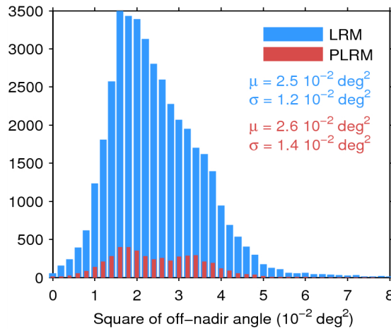
Figure 39. Histogram of flag-valid mispointing over oceans and lakes for LRM (blue) and PLRM (red) for 01/04/2015. Only positive values have been considered. The mean ( \mu ) and standard deviation ( \sigma ) are also shown. Note that values larger than 8 \cdot 10^{-2} \text{ deg}^2 are excluded from the histogram for the sake of readability but not from the computation of \mu and \sigma .
