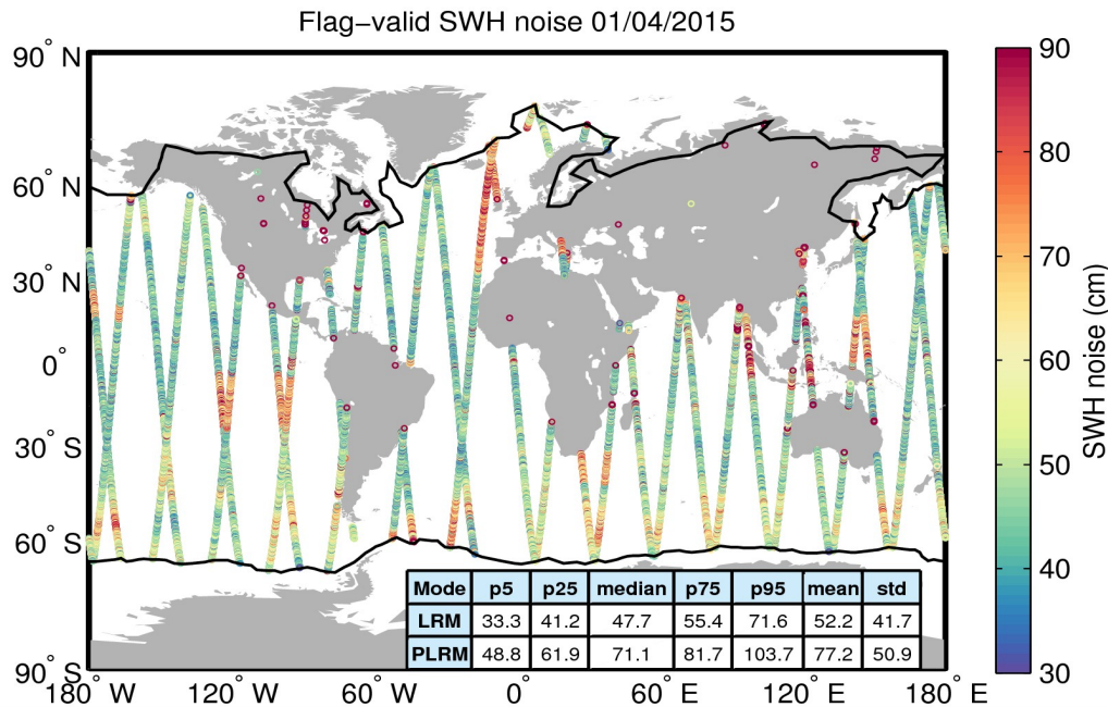
Figure 18. Geographical distribution of flag-valid 20-Hz SWH measurement noise over oceans and lakes for 01/04/2015. The statistical values shown in the table refer to the SWH noise and are calculated separately for LRM and PLRM regions. Measurements taken over polar polygons have been excluded from the computation of the statistical values. The black lines mark the outer limit of the Arctic and Antarctic polar polygons.
