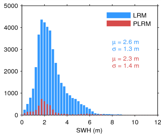
Figure 20. Histogram of science-valid SWH over oceans and lakes for LRM (blue) and PLRM (red) for 01/04/2015. The mean ( \mu ) and standard deviation ( \sigma ) are also shown. Note that values larger than 12 m are excluded from the histogram for the sake of readability but not from the computation of \mu and \sigma .
