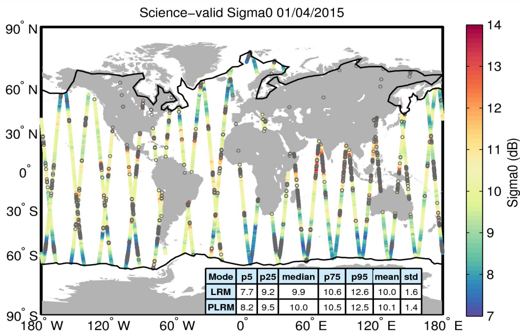
Figure 27. Geographical distribution of science-valid sigma0 data over oceans and lakes for 01/04/2015. The statistical values shown in the table refer to the sigma0 in dB and are calculated separately for LRM and PLRM regions. The black lines mark the outer limit of the Arctic and Antarctic polar polygons. Gray circles denote records that have been rejected based on the editing criteria described in Table 4.
