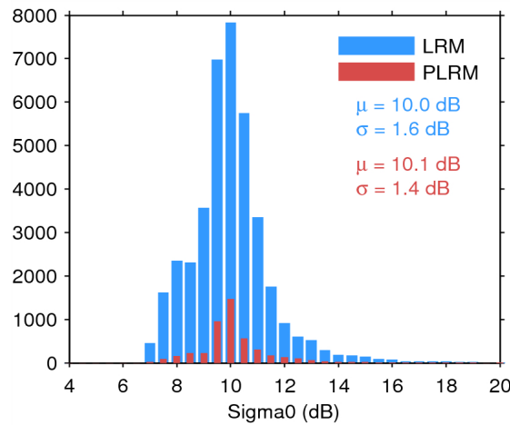
Figure 28. Histogram of science-valid sigma0 over oceans and lakes for LRM (blue) and PLRM (red) for 01/04/2015. The mean ( \mu ) and standard deviation ( \sigma ) are also shown. Note that values outside [4 20] dB are excluded from the histogram for the sake of readability but not from the computation of \mu and \sigma .
