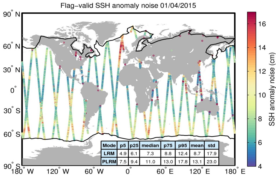
Figure 8. Geographical distribution of flag-valid 20-Hz SSH anomaly measurement noise over oceans and lakes for 01/04/2015. The statistical values shown in the table refer to the SSH anomaly noise and are calculated separately for LRM and PLRM regions. Measurements taken over polar polygons have been excluded from the computation of the statistical values. The black lines mark the outer limit of the Arctic and Antarctic polar polygons.
