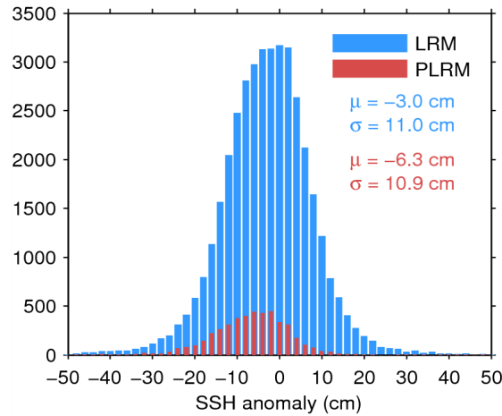
Figure 11. Histogram of science-valid SSH anomaly over oceans and lakes for LRM (blue) and PLRM (red) for 01/04/2015. The mean ( \mu ) and standard deviation ( \sigma ) are also shown. Note that values outside [-50\ 50] cm are excluded from the histogram for the sake of readability but not from the computation of \mu and \sigma .
