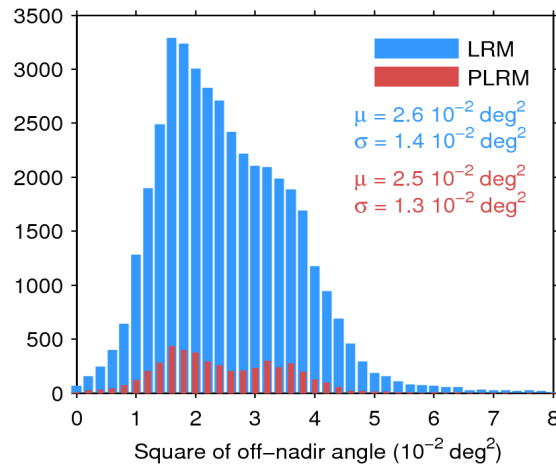
Figure 39. Histogram of flag-valid mispointing over oceans and lakes for LRM (blue) and PLRM (red) for 31/03/2015. Only positive values have been considered. The mean ( \mu ) and standard deviation ( \sigma ) are also shown. Note that values larger than 8 \cdot 10^{-2} \text{ deg}^2 are excluded from the histogram for the sake of readability but not from the computation of \mu and \sigma .
