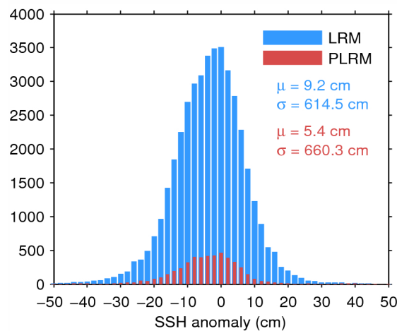
Figure 7. Histogram of flag-valid SSH anomaly over oceans and lakes for LRM (blue) and PLRM (red) for 31/03/2015. The mean ( \mu ) and standard deviation ( \sigma ) are also shown. Note that values outside [-50\ 50] cm are excluded from the histogram for the sake of readability but not from the computation of \mu and \sigma .
