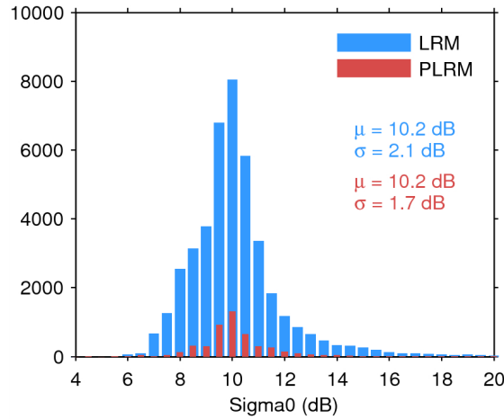
Figure 25. Histogram of flag-valid sigma0 over oceans and lakes for LRM (blue) and PLRM (red) for 31/03/2015. The mean ( \mu ) and standard deviation ( \sigma ) are also shown. Note that values outside [4 20] dB are excluded from the histogram for the sake of readability but not from the computation of \mu and \sigma .
