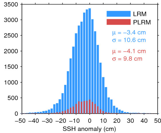
Figure 11. Histogram of science-valid SSH anomaly over oceans and lakes for LRM (blue) and PLRM (red) for 31/03/2015. The mean ( \mu ) and standard deviation ( \sigma ) are also shown. Note that values outside [-50\ 50] cm are excluded from the histogram for the sake of readability but not from the computation of \mu and \sigma .
