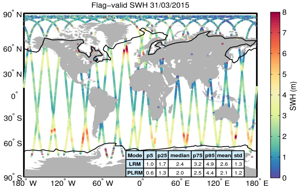
Figure 15. Geographical distribution of flag-valid SWH data over oceans and lakes for 31/03/2015. The statistical values shown in the table refer to the SWH in m and are calculated separately for LRM and PLRM regions. Measurements taken over polar polygons have been excluded from the computation of the statistical values. The black lines mark the outer limit of the Arctic and Antarctic polar polygons.
