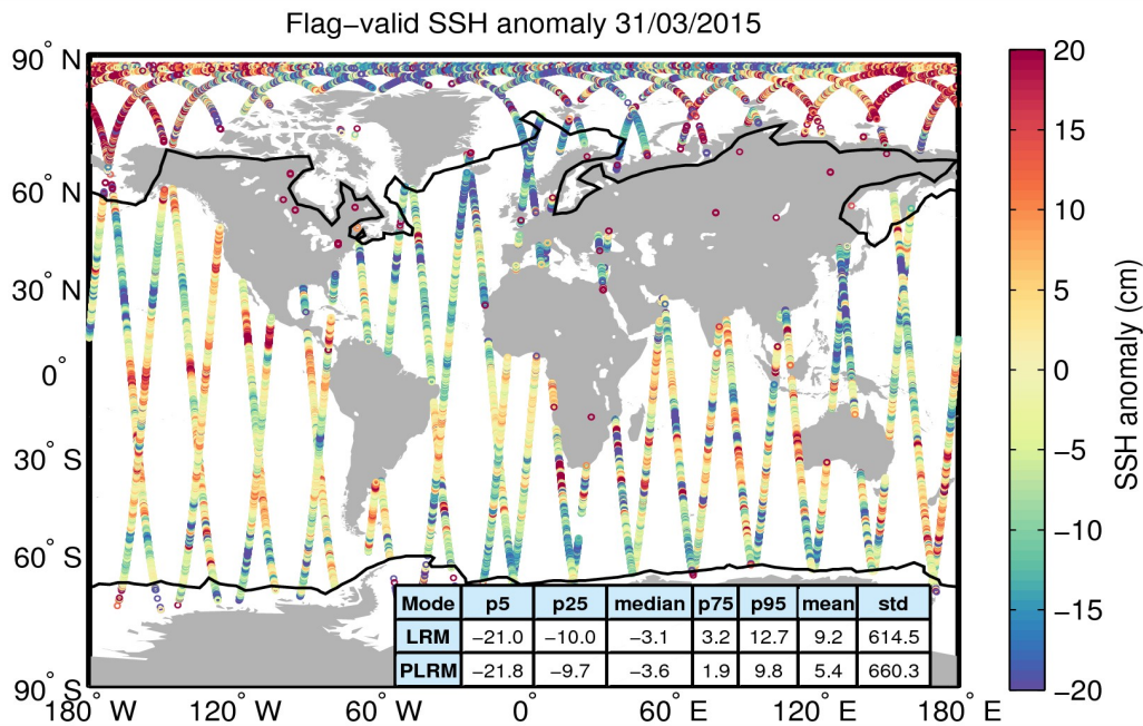
Figure 5. Geographical distribution of flag-valid 1-Hz SSH anomaly data over oceans and lakes for 31/03/2015. The statistical values shown in the table refer to the SSH anomaly in cm and are calculated separately for LRM and PLRM regions. Measurements taken over polar polygons have been excluded from the computation of the statistical values. The black lines mark the outer limit of the Arctic and Antarctic polar polygons.
