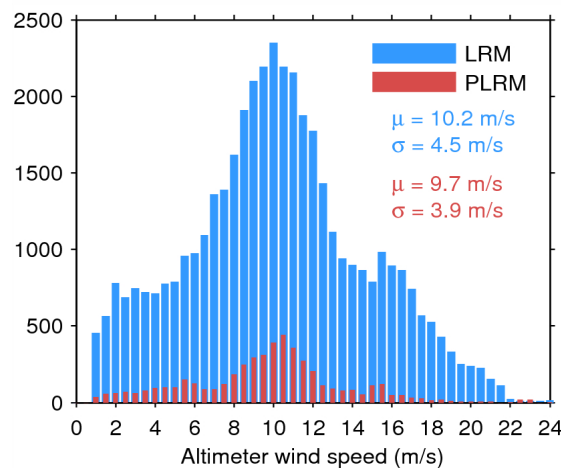
Figure 35. Histogram of science-valid wind over oceans and lakes for LRM (blue) and PLRM (red) for 31/03/2015. The mean ( \mu ) and standard deviation ( \sigma ) are also shown. Note that values larger than 24 m/s are excluded from the histogram for the sake of readability but not from the computation of \mu and \sigma .
