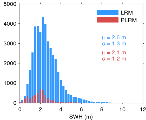
Figure 17. Histogram of flag-valid SWH over oceans and lakes for LRM (blue) and PLRM (red) for 31/03/2015. The mean ( \mu ) and standard deviation ( \sigma ) are also shown. Note that values larger than 12 m are excluded from the histogram for the sake of readability but not from the computation of \mu and \sigma .
