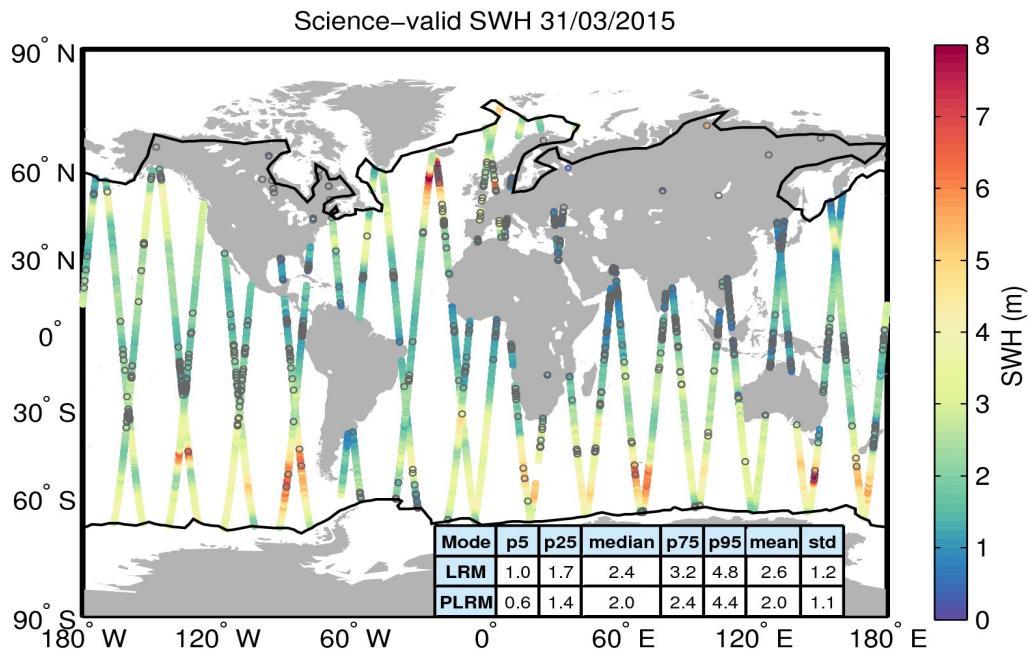
Figure 19. Geographical distribution of science-valid SWH data over oceans and lakes for 31/03/2015. The statistical values shown in the table refer to the SWH in m and are calculated separately for LRM and PLRM regions. The black lines mark the outer limit of the Arctic and Antarctic polar polygons. Gray circles denote records that have been rejected based on the editing criteria described in Table 3.
