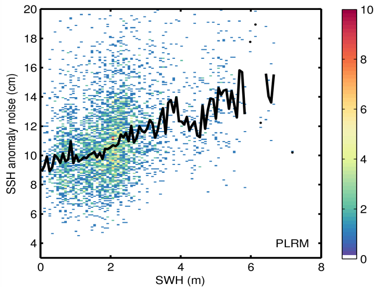
Figure 9. 2D histogram showing flag-valid SSH anomaly noise as a function of SWH for LRM (top) and PLRM (bottom) for 31/03/2015. The black line denotes the median SSH anomaly as a function of SWH.
