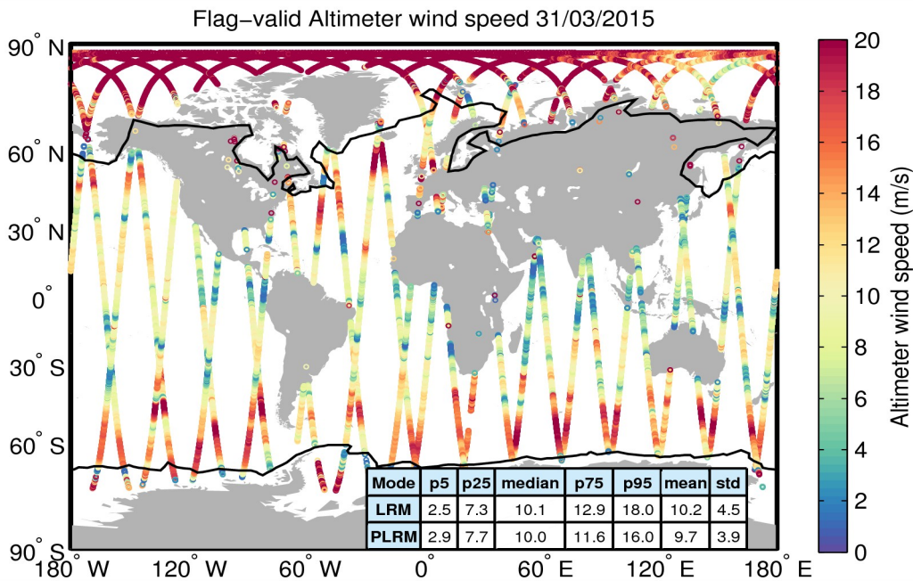
Figure 31. Geographical distribution of flag-valid wind data over oceans and lakes for 31/03/2015. The statistical values shown in the table refer to the wind in m/s and are calculated separately for LRM and PLRM regions. Measurements taken over polar polygons have been excluded from the computation of the statistical values. The black lines mark the outer limit of the Arctic and Antarctic polar polygons.
