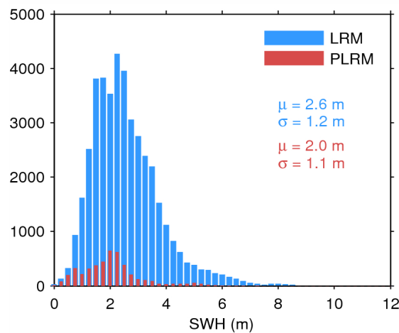
Figure 20. Histogram of science-valid SWH over oceans and lakes for LRM (blue) and PLRM (red) for 31/03/2015. The mean ( \mu ) and standard deviation ( \sigma ) are also shown. Note that values larger than 12 m are excluded from the histogram for the sake of readability but not from the computation of \mu and \sigma .
