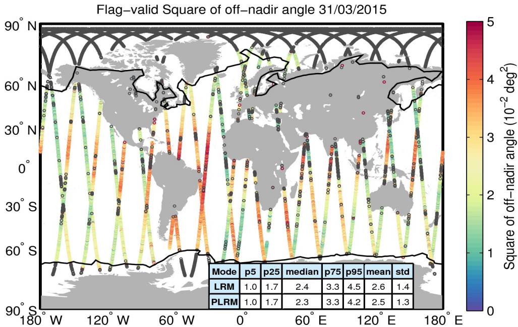
Figure 37. Geographical distribution of flag-valid mispointing data over oceans and lakes for 31/03/2015. The statistical values shown in the table refer to the mispointing in 10^{-2} \text{ deg}^2 and are calculated separately for LRM and PLRM regions. Measurements taken over polar polygons have been excluded from the computation of the statistical values. The black lines mark the outer limit of the Arctic and Antarctic polar polygons. Gray circles denote negative values.
