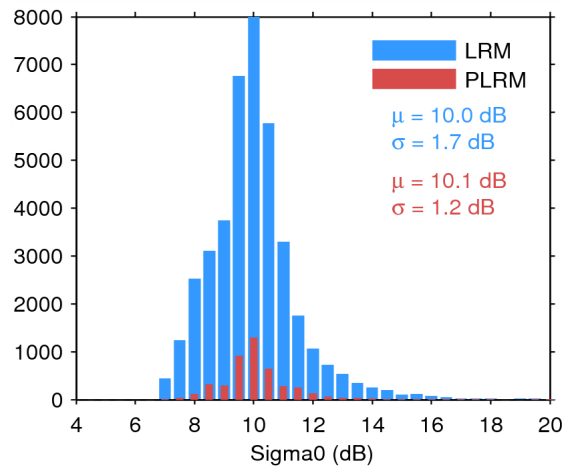
Figure 28. Histogram of science-valid sigma0 over oceans and lakes for LRM (blue) and PLRM (red) for 31/03/2015. The mean ( \mu ) and standard deviation ( \sigma ) are also shown. Note that values outside [4 20] dB are excluded from the histogram for the sake of readability but not from the computation of \mu and \sigma .
