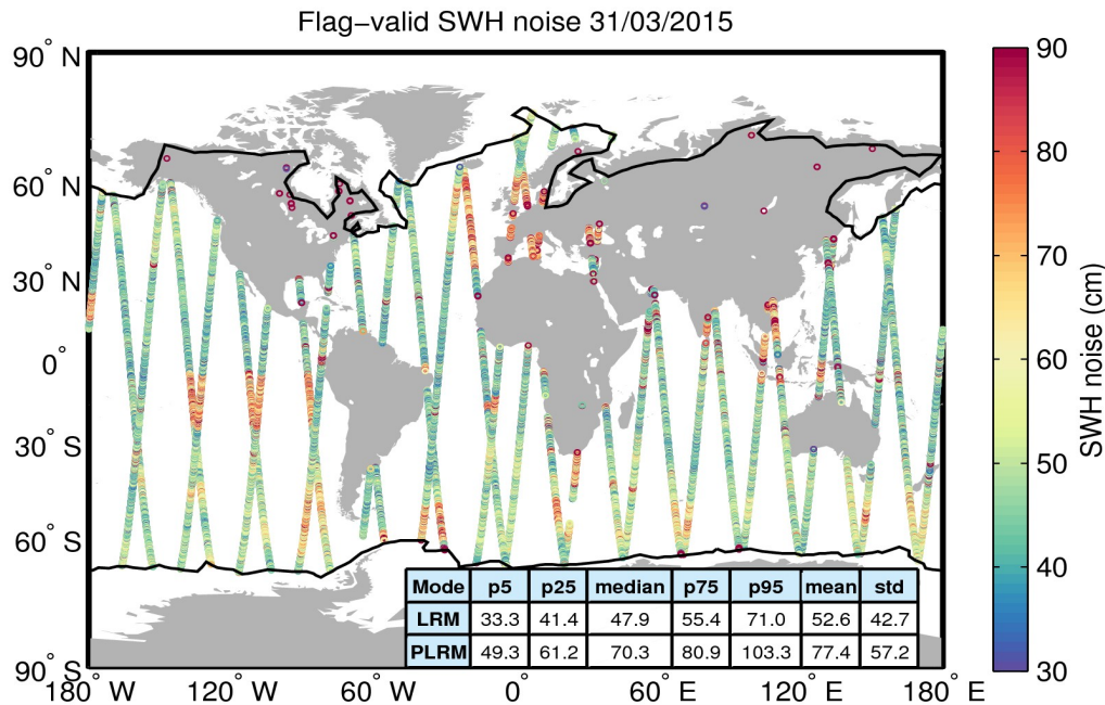
Figure 18. Geographical distribution of flag-valid 20-Hz SWH measurement noise over oceans and lakes for 31/03/2015. The statistical values shown in the table refer to the SWH noise and are calculated separately for LRM and PLRM regions. Measurements taken over polar polygons have been excluded from the computation of the statistical values. The black lines mark the outer limit of the Arctic and Antarctic polar polygons.
