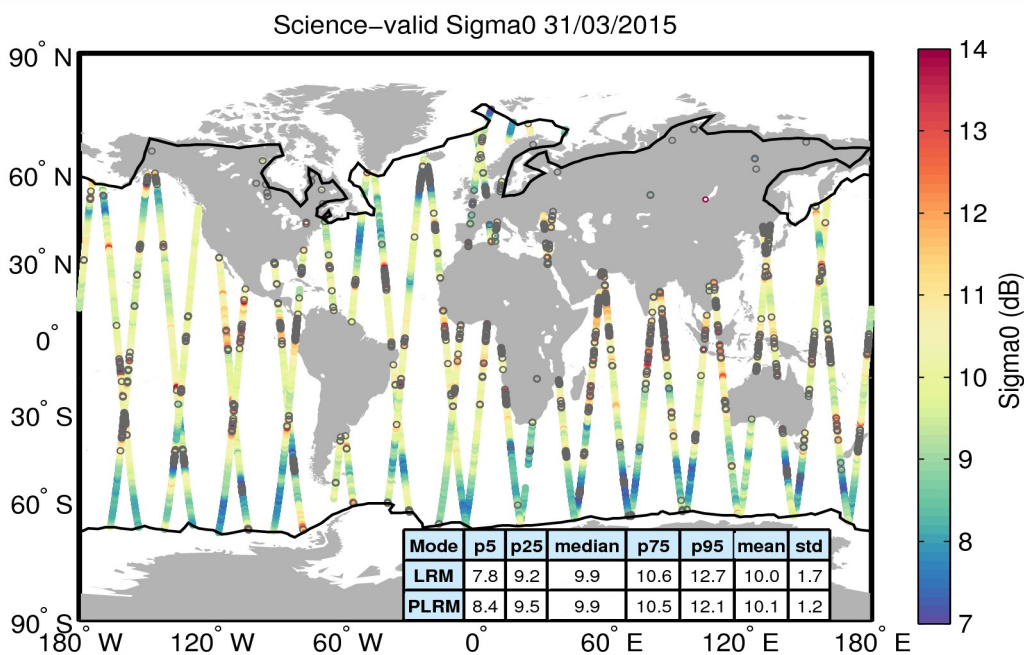
Figure 27. Geographical distribution of science-valid sigma0 data over oceans and lakes for 31/03/2015. The statistical values shown in the table refer to the sigma0 in dB and are calculated separately for LRM and PLRM regions. The black lines mark the outer limit of the Arctic and Antarctic polar polygons. Gray circles denote records that have been rejected based on the editing criteria described in Table 4.
