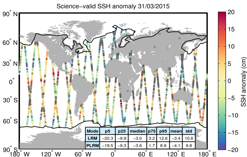
Figure 10. Geographical distribution of science-valid SSH anomaly data over oceans and lakes for 31/03/2015. The statistical values shown in the table refer to the SSH anomaly in cm and are calculated separately for LRM and PLRM regions. The black lines mark the outer limit of the Arctic and Antarctic polar polygons. Gray circles denote records that have been rejected based on the editing criteria described in Table 2.
