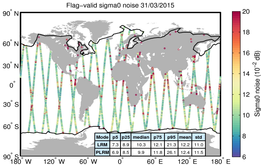
Figure 26. Geographical distribution of flag-valid 20-Hz sigma0 measurement noise over oceans and lakes for 31/03/2015. The statistical values shown in the table refer to the sigma0 noise and are calculated separately for LRM and PLRM regions. Measurements taken over polar polygons have been excluded from the computation of the statistical values. The black lines mark the outer limit of the Arctic and Antarctic polar polygons.
