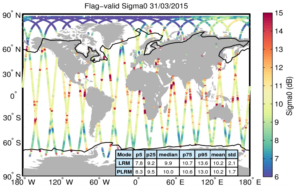
Figure 23. Geographical distribution of flag-valid sigma0 data over oceans and lakes for 31/03/2015. The statistical values shown in the table refer to the sigma0 in dB and are calculated separately for LRM and PLRM regions. Measurements taken over polar polygons have been excluded from the computation of the statistical values. The black lines mark the outer limit of the Arctic and Antarctic polar polygons.
