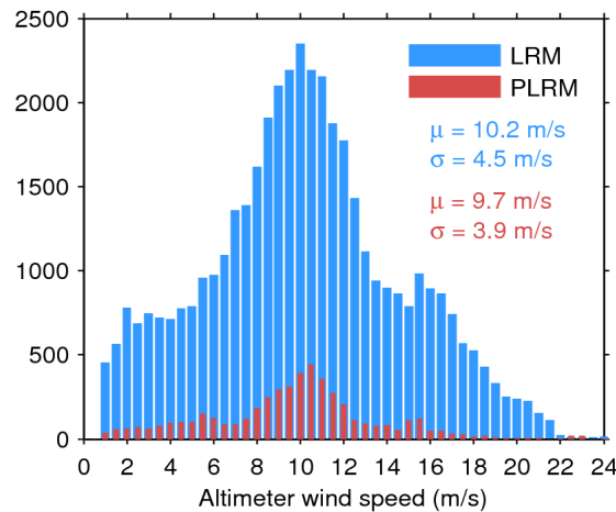
Figure 33. Histogram of flag-valid wind over oceans and lakes for LRM (blue) and PLRM (red) for 31/03/2015. The mean ( \mu ) and standard deviation ( \sigma ) are also shown. Note that values larger than 24 m/s are excluded from the histogram for the sake of readability but not from the computation of \mu and \sigma .
