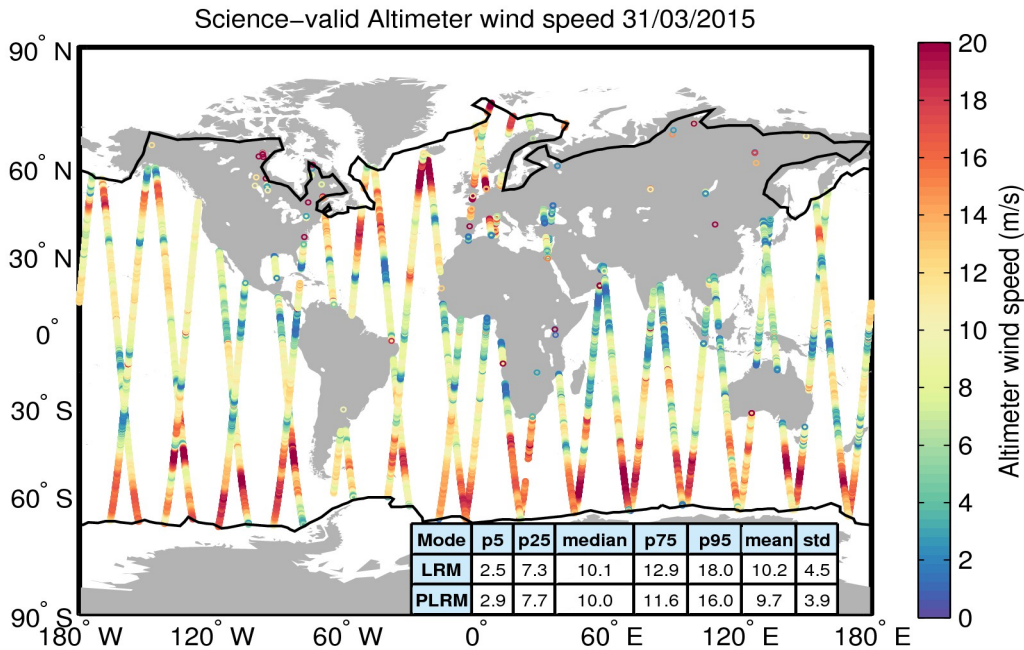
Figure 34. Geographical distribution of science-valid wind data over oceans and lakes for 31/03/2015. The statistical values shown in the table refer to the wind in m/s and are calculated separately for LRM and PLRM regions. The black lines mark the outer limit of the Arctic and Antarctic polar polygons. Gray circles denote records that have been rejected based on the editing criteria described in Table 5.
