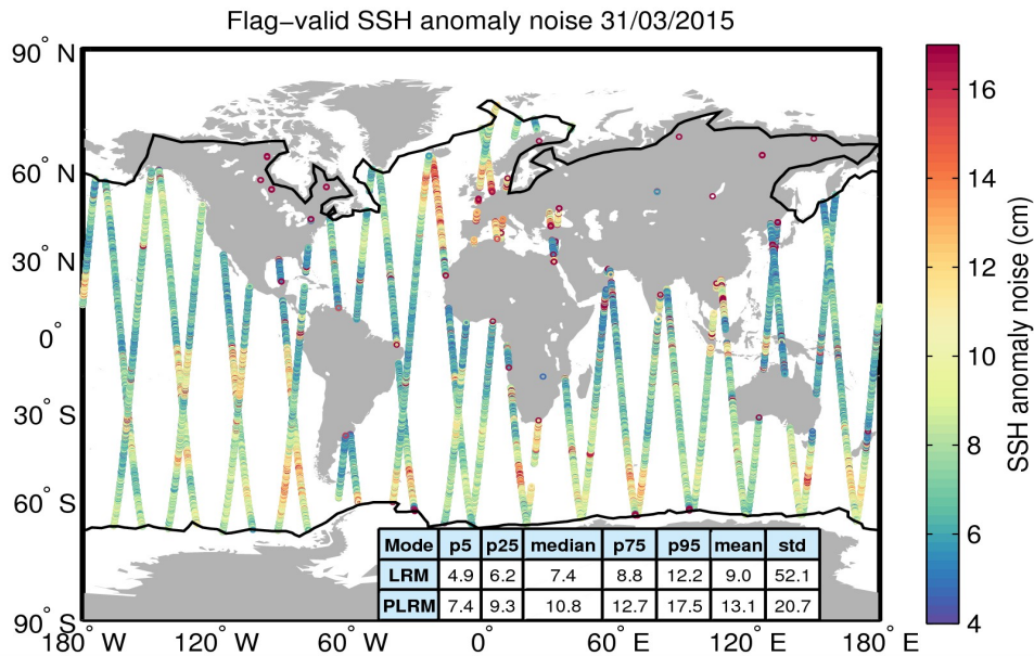
Figure 8. Geographical distribution of flag-valid 20-Hz SSH anomaly measurement noise over oceans and lakes for 31/03/2015. The statistical values shown in the table refer to the SSH anomaly noise and are calculated separately for LRM and PLRM regions. Measurements taken over polar polygons have been excluded from the computation of the statistical values. The black lines mark the outer limit of the Arctic and Antarctic polar polygons.
