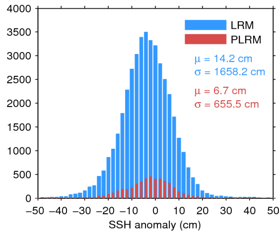
Figure 7. Histogram of flag-valid SSH anomaly over oceans and lakes for LRM (blue) and PLRM (red) for 29/03/2015. The mean ( \mu ) and standard deviation ( \sigma ) are also shown. Note that values outside [-50\ 50] cm are excluded from the histogram for the sake of readability but not from the computation of \mu and \sigma .
