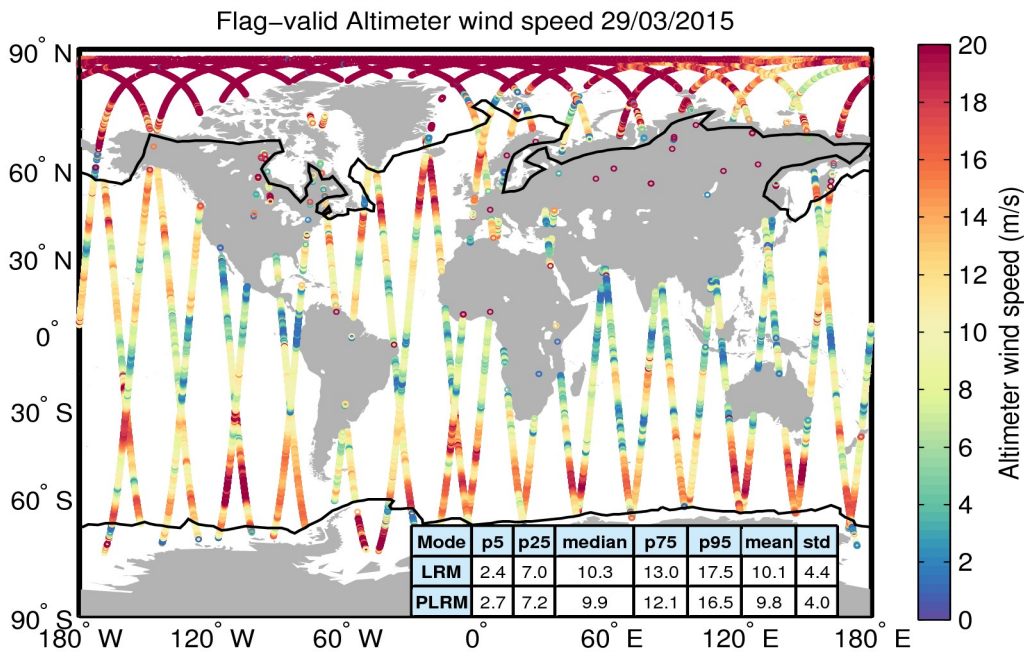
Figure 31. Geographical distribution of flag-valid wind data over oceans and lakes for 29/03/2015. The statistical values shown in the table refer to the wind in m/s and are calculated separately for LRM and PLRM regions. Measurements taken over polar polygons have been excluded from the computation of the statistical values. The black lines mark the outer limit of the Arctic and Antarctic polar polygons.
