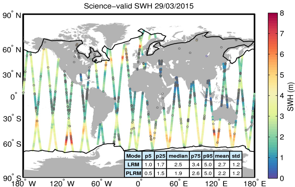
Figure 19. Geographical distribution of science-valid SWH data over oceans and lakes for 29/03/2015. The statistical values shown in the table refer to the SWH in m and are calculated separately for LRM and PLRM regions. The black lines mark the outer limit of the Arctic and Antarctic polar polygons. Gray circles denote records that have been rejected based on the editing criteria described in Table 3.
