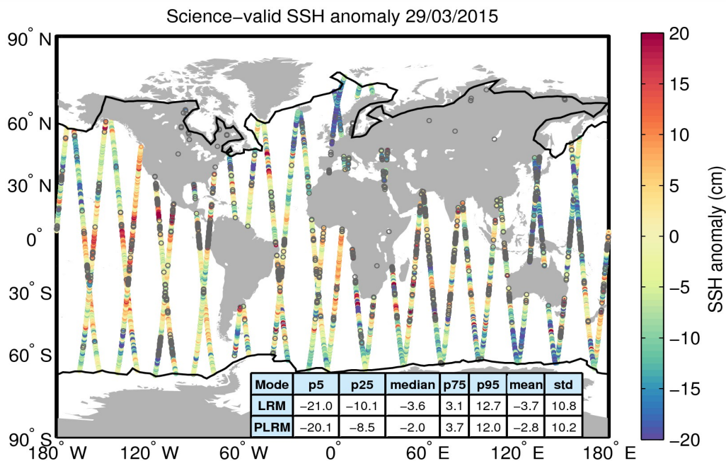
Figure 10. Geographical distribution of science-valid SSH anomaly data over oceans and lakes for 29/03/2015. The statistical values shown in the table refer to the SSH anomaly in cm and are calculated separately for LRM and PLRM regions. The black lines mark the outer limit of the Arctic and Antarctic polar polygons. Gray circles denote records that have been rejected based on the editing criteria described in Table 2.
