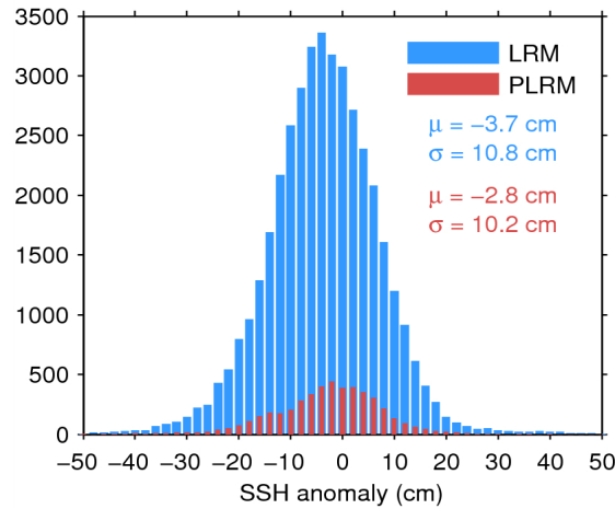
Figure 11. Histogram of science-valid SSH anomaly over oceans and lakes for LRM (blue) and PLRM (red) for 29/03/2015. The mean ( \mu ) and standard deviation ( \sigma ) are also shown. Note that values outside [-50\ 50] cm are excluded from the histogram for the sake of readability but not from the computation of \mu and \sigma .
