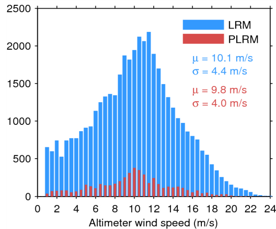
Figure 33. Histogram of flag-valid wind over oceans and lakes for LRM (blue) and PLRM (red) for 29/03/2015. The mean ( \mu ) and standard deviation ( \sigma ) are also shown. Note that values larger than 24 m/s are excluded from the histogram for the sake of readability but not from the computation of \mu and \sigma .
