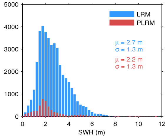
Figure 17. Histogram of flag-valid SWH over oceans and lakes for LRM (blue) and PLRM (red) for 29/03/2015. The mean ( \mu ) and standard deviation ( \sigma ) are also shown. Note that values larger than 12 m are excluded from the histogram for the sake of readability but not from the computation of \mu and \sigma .
