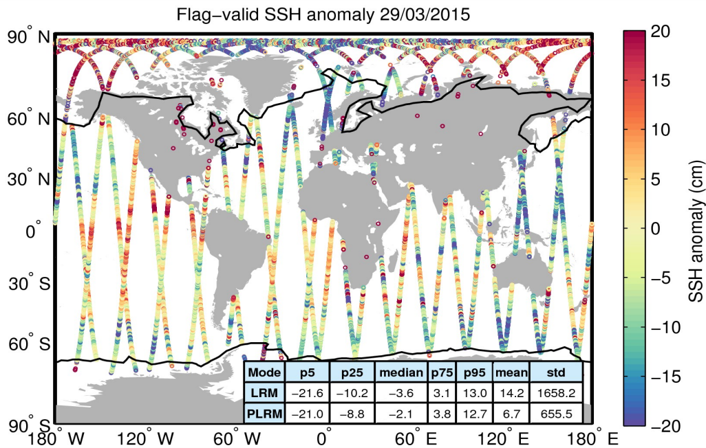
Figure 5. Geographical distribution of flag-valid 1-Hz SSH anomaly data over oceans and lakes for 29/03/2015. The statistical values shown in the table refer to the SSH anomaly in cm and are calculated separately for LRM and PLRM regions. Measurements taken over polar polygons have been excluded from the computation of the statistical values. The black lines mark the outer limit of the Arctic and Antarctic polar polygons.
