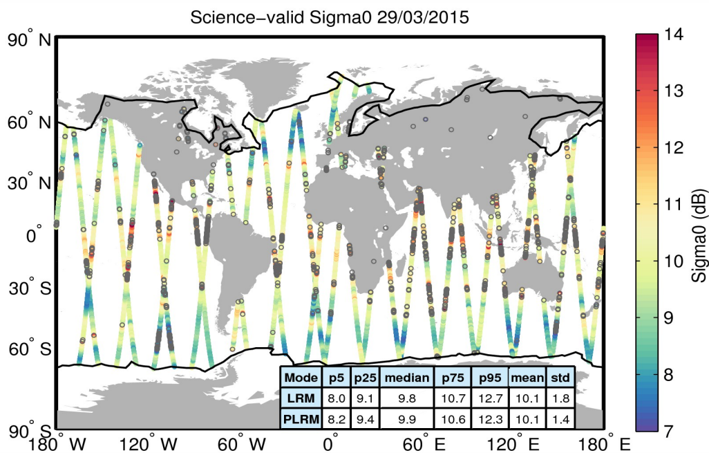
Figure 27. Geographical distribution of science-valid sigma0 data over oceans and lakes for 29/03/2015. The statistical values shown in the table refer to the sigma0 in dB and are calculated separately for LRM and PLRM regions. The black lines mark the outer limit of the Arctic and Antarctic polar polygons. Gray circles denote records that have been rejected based on the editing criteria described in Table 4.
