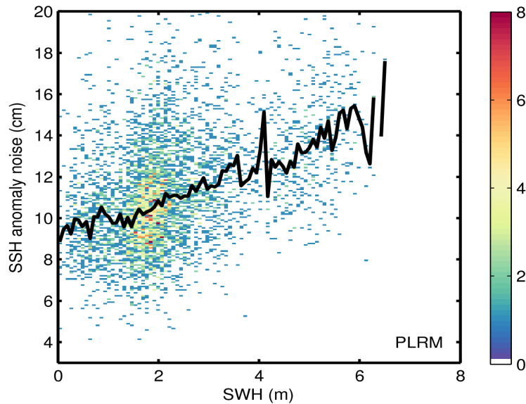
Figure 9. 2D histogram showing flag-valid SSH anomaly noise as a function of SWH for LRM (top) and PLRM (bottom) for 29/03/2015. The black line denotes the median SSH anomaly as a function of SWH.
