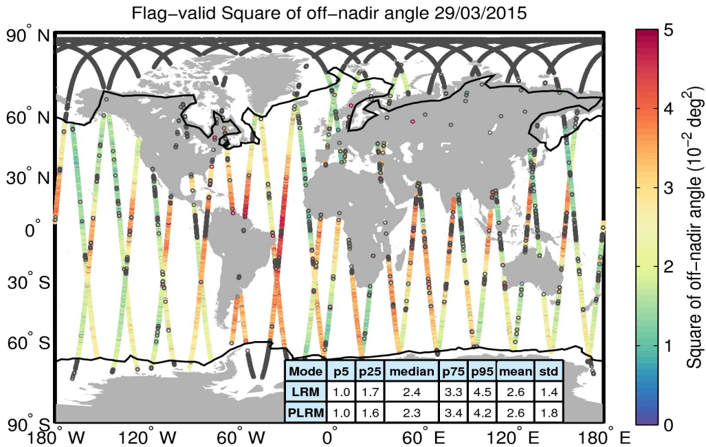
Figure 37. Geographical distribution of flag-valid mispointing data over oceans and lakes for 29/03/2015. The statistical values shown in the table refer to the mispointing in 10^{-2} \text{ deg}^2 and are calculated separately for LRM and PLRM regions. Measurements taken over polar polygons have been excluded from the computation of the statistical values. The black lines mark the outer limit of the Arctic and Antarctic polar polygons. Gray circles denote negative values.
