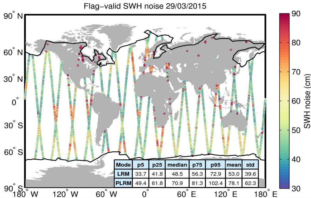
Figure 18. Geographical distribution of flag-valid 20-Hz SWH measurement noise over oceans and lakes for 29/03/2015. The statistical values shown in the table refer to the SWH noise and are calculated separately for LRM and PLRM regions. Measurements taken over polar polygons have been excluded from the computation of the statistical values. The black lines mark the outer limit of the Arctic and Antarctic polar polygons.
