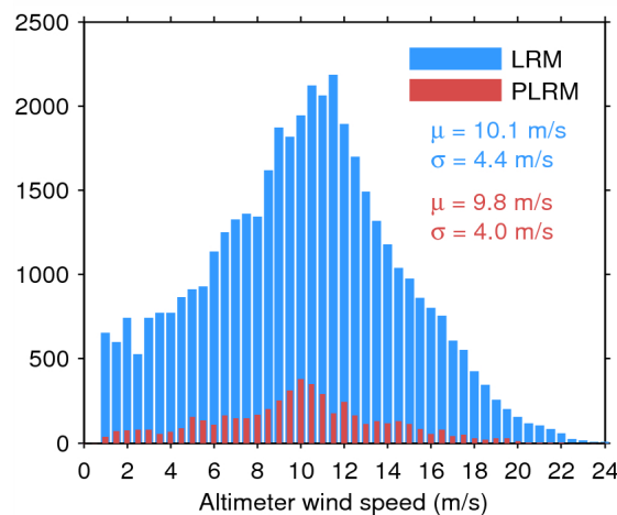
Figure 35. Histogram of science-valid wind over oceans and lakes for LRM (blue) and PLRM (red) for 29/03/2015. The mean ( \mu ) and standard deviation ( \sigma ) are also shown. Note that values larger than 24 m/s are excluded from the histogram for the sake of readability but not from the computation of \mu and \sigma .
