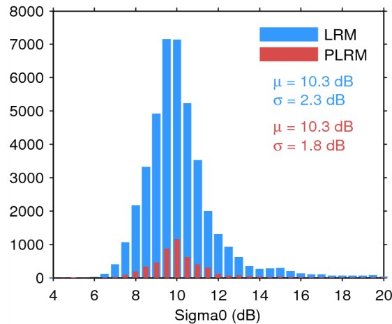
Figure 25. Histogram of flag-valid sigma0 over oceans and lakes for LRM (blue) and PLRM (red) for 29/03/2015. The mean ( \mu ) and standard deviation ( \sigma ) are also shown. Note that values outside [4 20] dB are excluded from the histogram for the sake of readability but not from the computation of \mu and \sigma .
