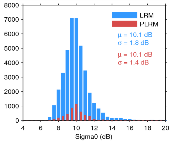
Figure 28. Histogram of science-valid sigma0 over oceans and lakes for LRM (blue) and PLRM (red) for 29/03/2015. The mean ( \mu ) and standard deviation ( \sigma ) are also shown. Note that values outside [4 20] dB are excluded from the histogram for the sake of readability but not from the computation of \mu and \sigma .
