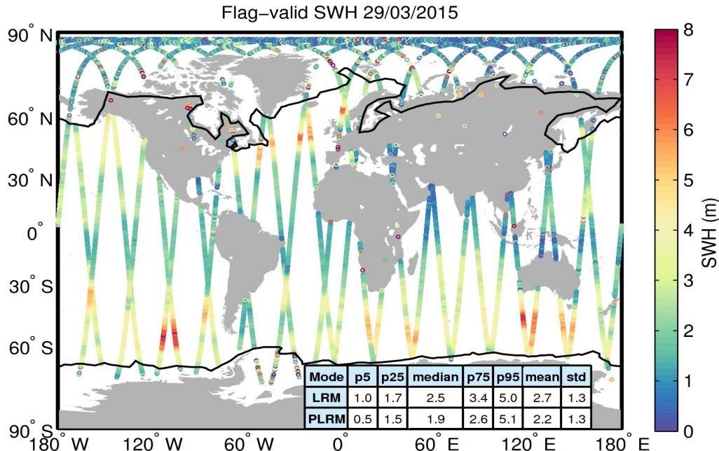
Figure 15. Geographical distribution of flag-valid SWH data over oceans and lakes for 29/03/2015. The statistical values shown in the table refer to the SWH in m and are calculated separately for LRM and PLRM regions. Measurements taken over polar polygons have been excluded from the computation of the statistical values. The black lines mark the outer limit of the Arctic and Antarctic polar polygons.
