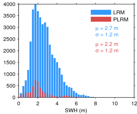
Figure 20. Histogram of science-valid SWH over oceans and lakes for LRM (blue) and PLRM (red) for 29/03/2015. The mean ( \mu ) and standard deviation ( \sigma ) are also shown. Note that values larger than 12 m are excluded from the histogram for the sake of readability but not from the computation of \mu and \sigma .
