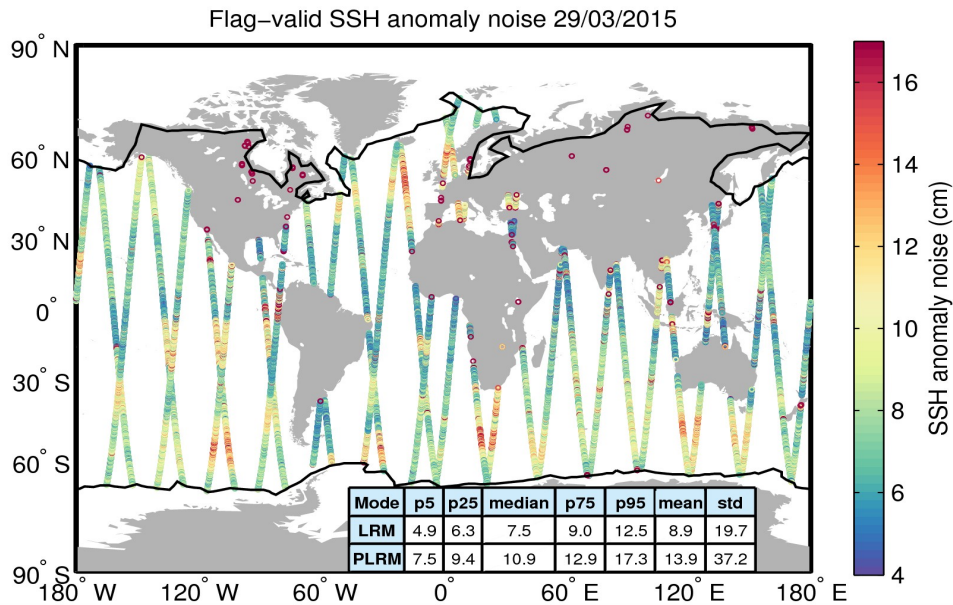
Figure 8. Geographical distribution of flag-valid 20-Hz SSH anomaly measurement noise over oceans and lakes for 29/03/2015. The statistical values shown in the table refer to the SSH anomaly noise and are calculated separately for LRM and PLRM regions. Measurements taken over polar polygons have been excluded from the computation of the statistical values. The black lines mark the outer limit of the Arctic and Antarctic polar polygons.
