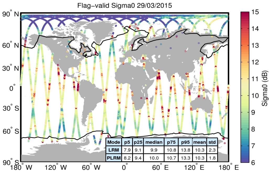
Figure 23. Geographical distribution of flag-valid sigma0 data over oceans and lakes for 29/03/2015. The statistical values shown in the table refer to the sigma0 in dB and are calculated separately for LRM and PLRM regions. Measurements taken over polar polygons have been excluded from the computation of the statistical values. The black lines mark the outer limit of the Arctic and Antarctic polar polygons.
