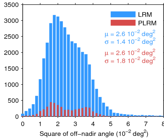
Figure 39. Histogram of flag-valid mispointing over oceans and lakes for LRM (blue) and PLRM (red) for 29/03/2015. Only positive values have been considered. The mean ( \mu ) and standard deviation ( \sigma ) are also shown. Note that values larger than 8 \cdot 10^{-2} \text{ deg}^2 are excluded from the histogram for the sake of readability but not from the computation of \mu and \sigma .
