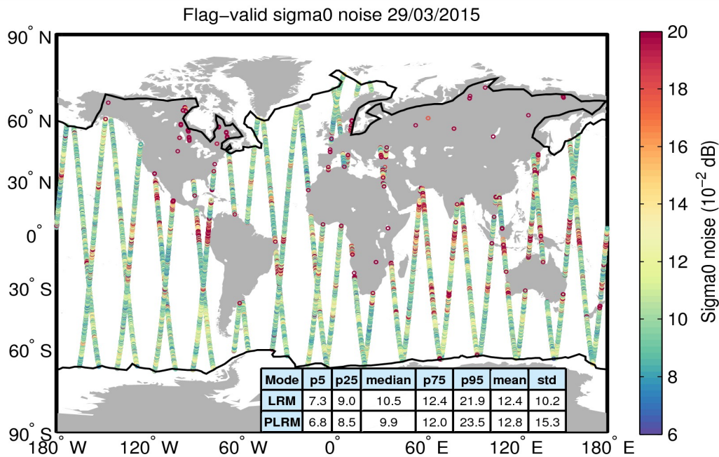
Figure 26. Geographical distribution of flag-valid 20-Hz sigma0 measurement noise over oceans and lakes for 29/03/2015. The statistical values shown in the table refer to the sigma0 noise and are calculated separately for LRM and PLRM regions. Measurements taken over polar polygons have been excluded from the computation of the statistical values. The black lines mark the outer limit of the Arctic and Antarctic polar polygons.
