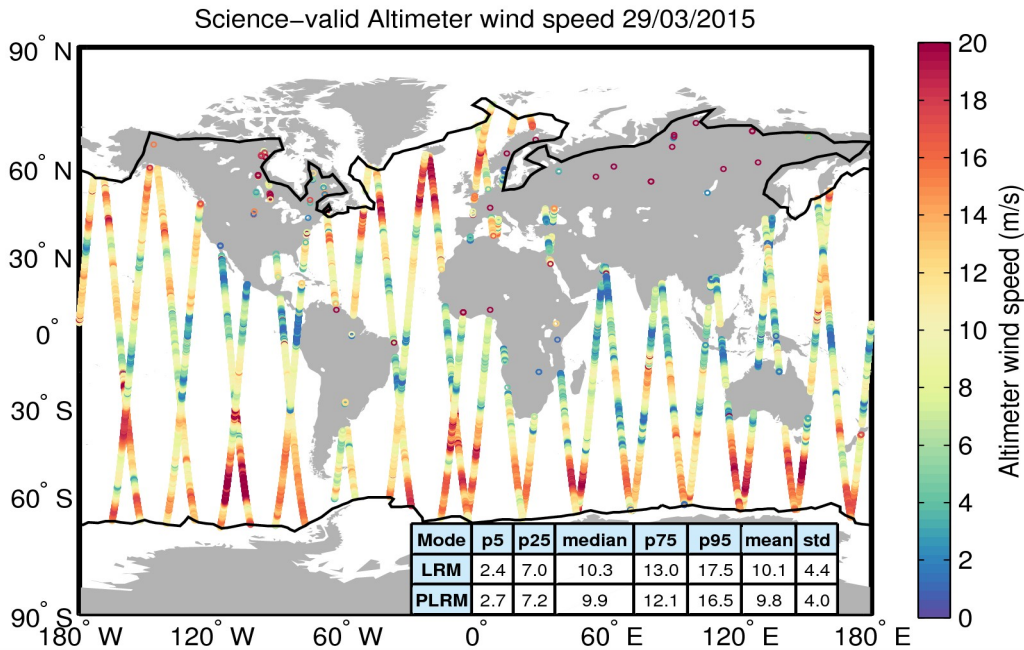
Figure 34. Geographical distribution of science-valid wind data over oceans and lakes for 29/03/2015. The statistical values shown in the table refer to the wind in m/s and are calculated separately for LRM and PLRM regions. The black lines mark the outer limit of the Arctic and Antarctic polar polygons. Gray circles denote records that have been rejected based on the editing criteria described in Table 5.
