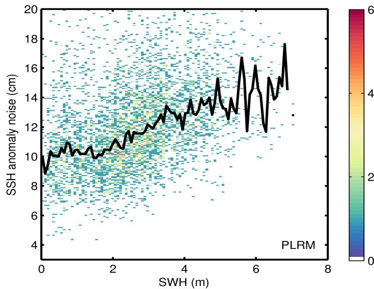
Figure 9. 2D histogram showing flag-valid SSH anomaly noise as a function of SWH for LRM (top) and PLRM (bottom) for 26/03/2015. The black line denotes the median SSH anomaly as a function of SWH.
