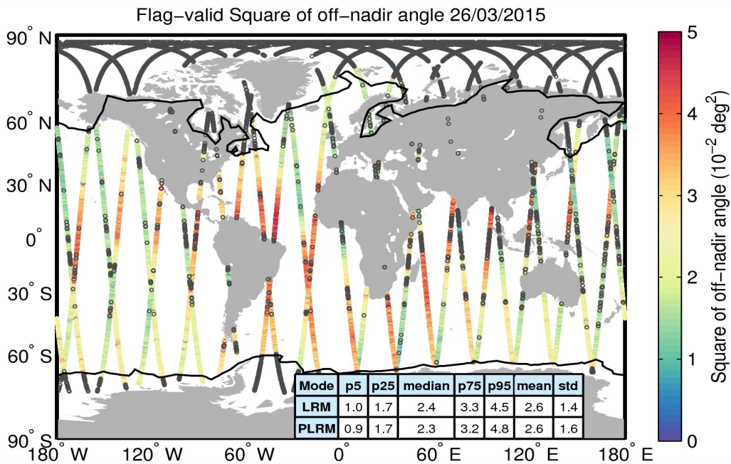
Figure 37. Geographical distribution of flag-valid mispointing data over oceans and lakes for 26/03/2015. The statistical values shown in the table refer to the mispointing in 10^{-2} \text{ deg}^2 and are calculated separately for LRM and PLRM regions. Measurements taken over polar polygons have been excluded from the computation of the statistical values. The black lines mark the outer limit of the Arctic and Antarctic polar polygons. Gray circles denote negative values.
