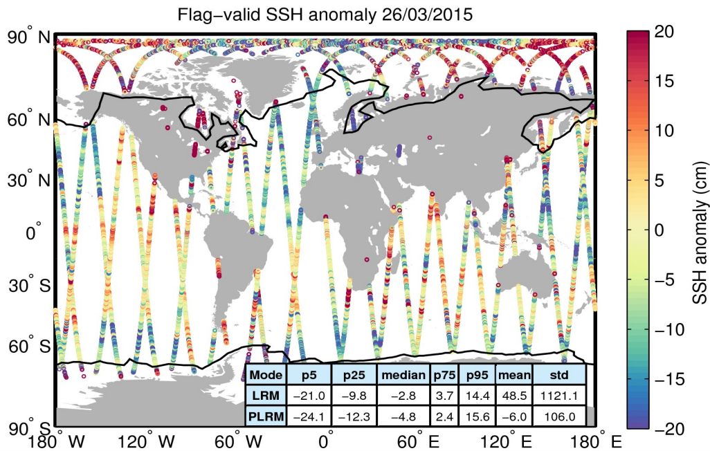
Figure 5. Geographical distribution of flag-valid 1-Hz SSH anomaly data over oceans and lakes for 26/03/2015. The statistical values shown in the table refer to the SSH anomaly in cm and are calculated separately for LRM and PLRM regions. Measurements taken over polar polygons have been excluded from the computation of the statistical values. The black lines mark the outer limit of the Arctic and Antarctic polar polygons.
