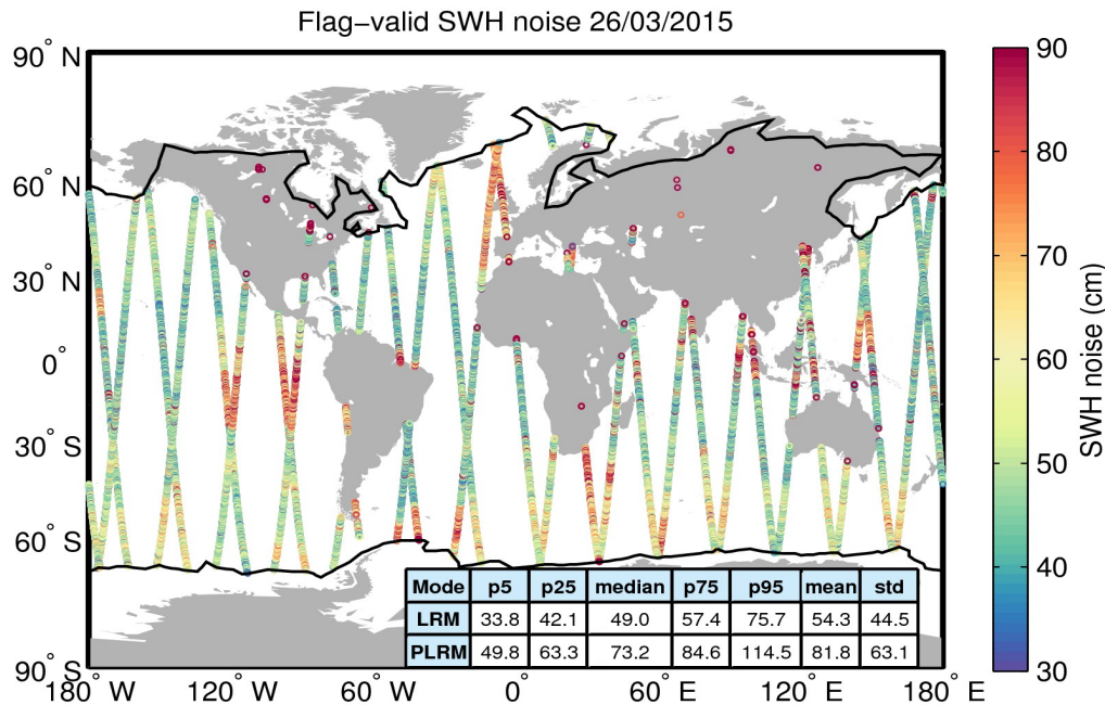
Figure 18. Geographical distribution of flag-valid 20-Hz SWH measurement noise over oceans and lakes for 26/03/2015. The statistical values shown in the table refer to the SWH noise and are calculated separately for LRM and PLRM regions. Measurements taken over polar polygons have been excluded from the computation of the statistical values. The black lines mark the outer limit of the Arctic and Antarctic polar polygons.
