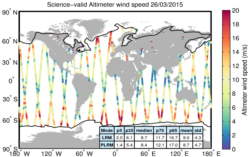
Figure 34. Geographical distribution of science-valid wind data over oceans and lakes for 26/03/2015. The statistical values shown in the table refer to the wind in m/s and are calculated separately for LRM and PLRM regions. The black lines mark the outer limit of the Arctic and Antarctic polar polygons. Gray circles denote records that have been rejected based on the editing criteria described in Table 5.
