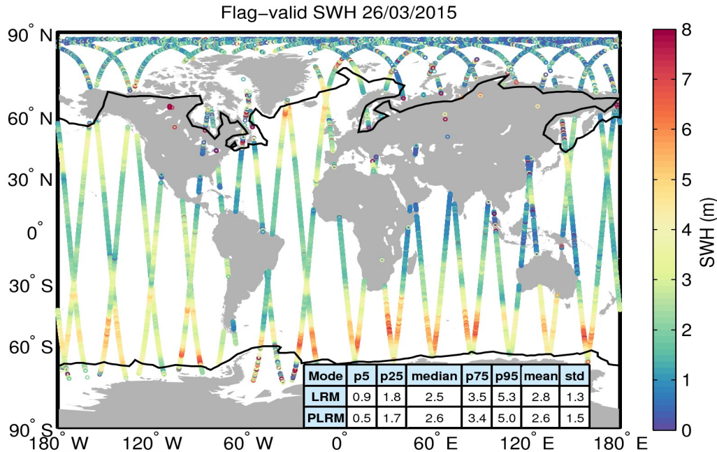
Figure 15. Geographical distribution of flag-valid SWH data over oceans and lakes for 26/03/2015. The statistical values shown in the table refer to the SWH in m and are calculated separately for LRM and PLRM regions. Measurements taken over polar polygons have been excluded from the computation of the statistical values. The black lines mark the outer limit of the Arctic and Antarctic polar polygons.
