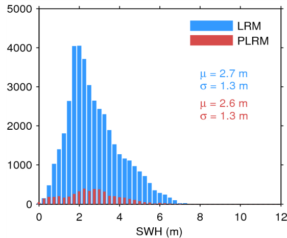
Figure 20. Histogram of science-valid SWH over oceans and lakes for LRM (blue) and PLRM (red) for 26/03/2015. The mean ( \mu ) and standard deviation ( \sigma ) are also shown. Note that values larger than 12 m are excluded from the histogram for the sake of readability but not from the computation of \mu and \sigma .
