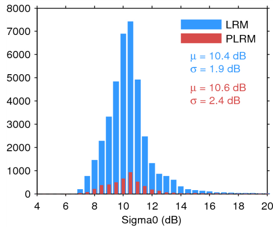
Figure 28. Histogram of science-valid sigma0 over oceans and lakes for LRM (blue) and PLRM (red) for 26/03/2015. The mean ( \mu ) and standard deviation ( \sigma ) are also shown. Note that values outside [4 20] dB are excluded from the histogram for the sake of readability but not from the computation of \mu and \sigma .
