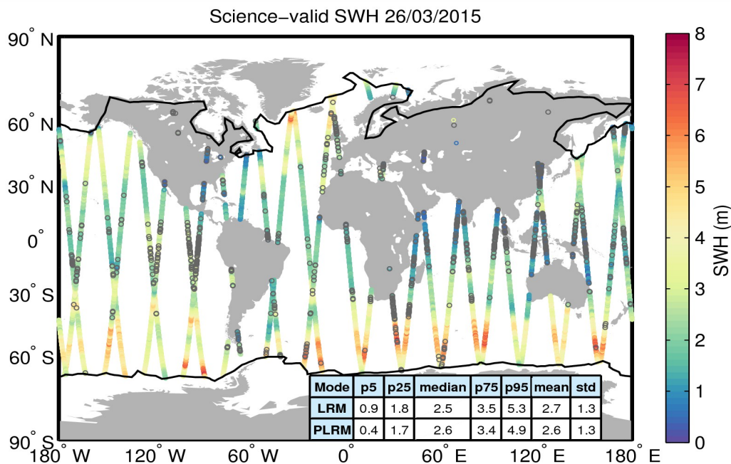
Figure 19. Geographical distribution of science-valid SWH data over oceans and lakes for 26/03/2015. The statistical values shown in the table refer to the SWH in m and are calculated separately for LRM and PLRM regions. The black lines mark the outer limit of the Arctic and Antarctic polar polygons. Gray circles denote records that have been rejected based on the editing criteria described in Table 3.
