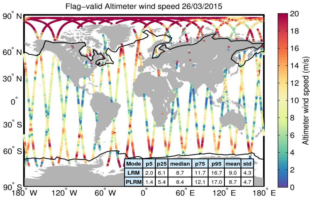
Figure 31. Geographical distribution of flag-valid wind data over oceans and lakes for 26/03/2015. The statistical values shown in the table refer to the wind in m/s and are calculated separately for LRM and PLRM regions. Measurements taken over polar polygons have been excluded from the computation of the statistical values. The black lines mark the outer limit of the Arctic and Antarctic polar polygons.
