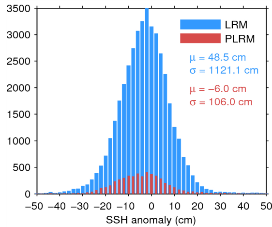
Figure 7. Histogram of flag-valid SSH anomaly over oceans and lakes for LRM (blue) and PLRM (red) for 26/03/2015. The mean ( \mu ) and standard deviation ( \sigma ) are also shown. Note that values outside [-50\ 50] cm are excluded from the histogram for the sake of readability but not from the computation of \mu and \sigma .
