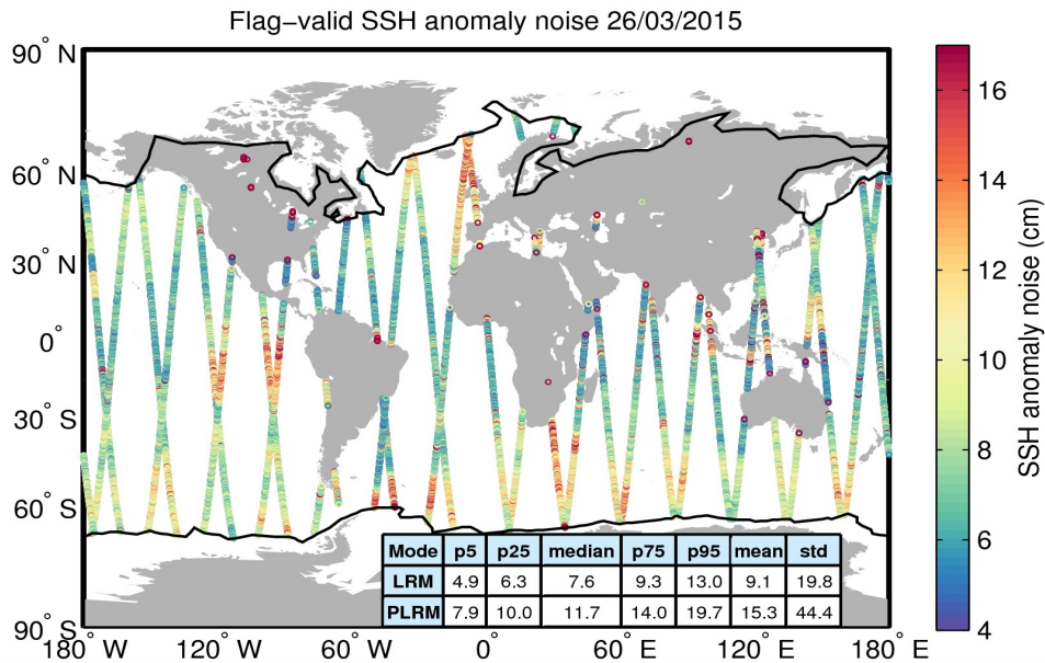
Figure 8. Geographical distribution of flag-valid 20-Hz SSH anomaly measurement noise over oceans and lakes for 26/03/2015. The statistical values shown in the table refer to the SSH anomaly noise and are calculated separately for LRM and PLRM regions. Measurements taken over polar polygons have been excluded from the computation of the statistical values. The black lines mark the outer limit of the Arctic and Antarctic polar polygons.
