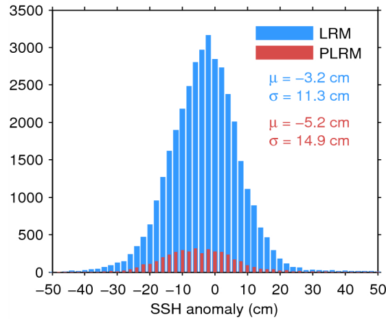
Figure 11. Histogram of science-valid SSH anomaly over oceans and lakes for LRM (blue) and PLRM (red) for 26/03/2015. The mean ( \mu ) and standard deviation ( \sigma ) are also shown. Note that values outside [-50 50] cm are excluded from the histogram for the sake of readability but not from the computation of \mu and \sigma .
