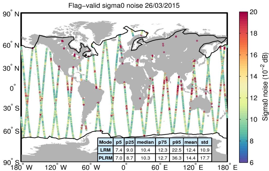
Figure 26. Geographical distribution of flag-valid 20-Hz sigma0 measurement noise over oceans and lakes for 26/03/2015. The statistical values shown in the table refer to the sigma0 noise and are calculated separately for LRM and PLRM regions. Measurements taken over polar polygons have been excluded from the computation of the statistical values. The black lines mark the outer limit of the Arctic and Antarctic polar polygons.
