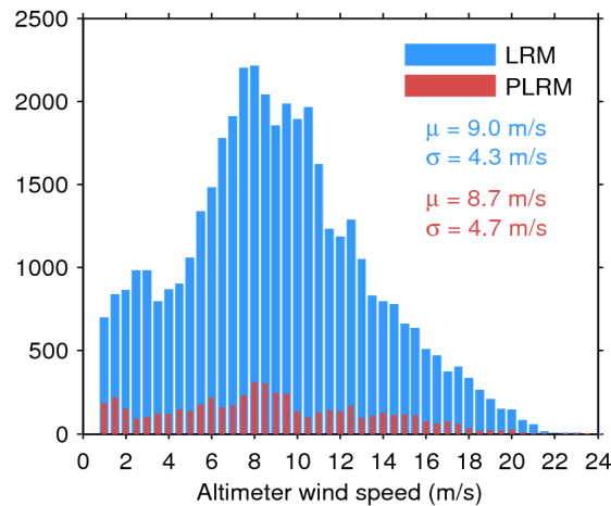
Figure 33. Histogram of flag-valid wind over oceans and lakes for LRM (blue) and PLRM (red) for 26/03/2015. The mean ( \mu ) and standard deviation ( \sigma ) are also shown. Note that values larger than 24 m/s are excluded from the histogram for the sake of readability but not from the computation of \mu and \sigma .
