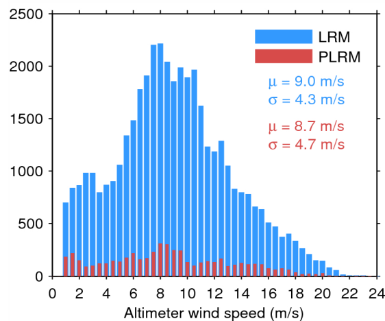
Figure 35. Histogram of science-valid wind over oceans and lakes for LRM (blue) and PLRM (red) for 26/03/2015. The mean ( \mu ) and standard deviation ( \sigma ) are also shown. Note that values larger than 24 m/s are excluded from the histogram for the sake of readability but not from the computation of \mu and \sigma .
