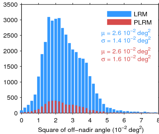
Figure 39. Histogram of flag-valid mispointing over oceans and lakes for LRM (blue) and PLRM (red) for 26/03/2015. Only positive values have been considered. The mean ( \mu ) and standard deviation ( \sigma ) are also shown. Note that values larger than 8 \cdot 10^{-2} \text{ deg}^2 are excluded from the histogram for the sake of readability but not from the computation of \mu and \sigma .
