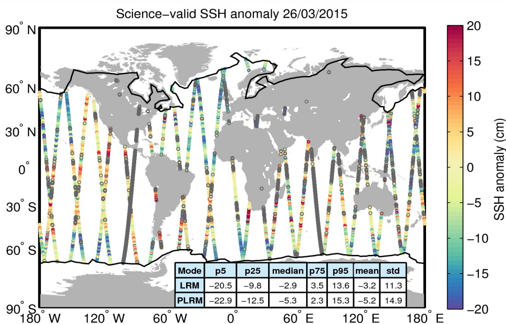
Figure 10. Geographical distribution of science-valid SSH anomaly data over oceans and lakes for 26/03/2015. The statistical values shown in the table refer to the SSH anomaly in cm and are calculated separately for LRM and PLRM regions. The black lines mark the outer limit of the Arctic and Antarctic polar polygons. Gray circles denote records that have been rejected based on the editing criteria described in Table 2.
