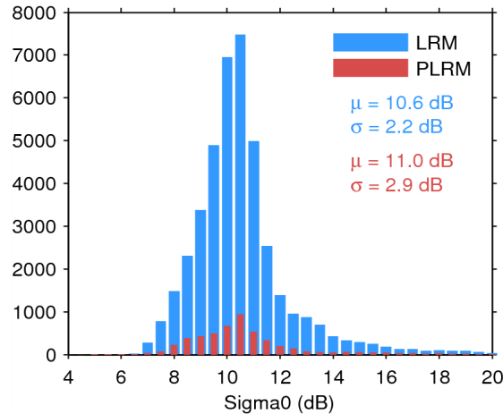
Figure 25. Histogram of flag-valid sigma0 over oceans and lakes for LRM (blue) and PLRM (red) for 26/03/2015. The mean ( \mu ) and standard deviation ( \sigma ) are also shown. Note that values outside [4 20] dB are excluded from the histogram for the sake of readability but not from the computation of \mu and \sigma .
