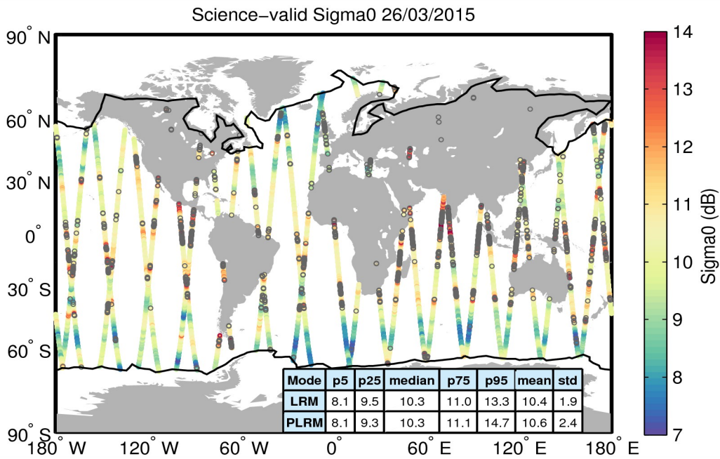
Figure 27. Geographical distribution of science-valid sigma0 data over oceans and lakes for 26/03/2015. The statistical values shown in the table refer to the sigma0 in dB and are calculated separately for LRM and PLRM regions. The black lines mark the outer limit of the Arctic and Antarctic polar polygons. Gray circles denote records that have been rejected based on the editing criteria described in Table 4.
