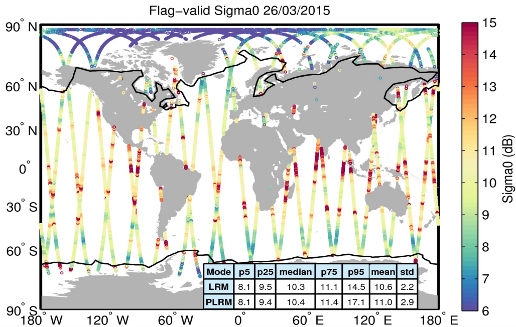
Figure 23. Geographical distribution of flag-valid sigma0 data over oceans and lakes for 26/03/2015. The statistical values shown in the table refer to the sigma0 in dB and are calculated separately for LRM and PLRM regions. Measurements taken over polar polygons have been excluded from the computation of the statistical values. The black lines mark the outer limit of the Arctic and Antarctic polar polygons.
