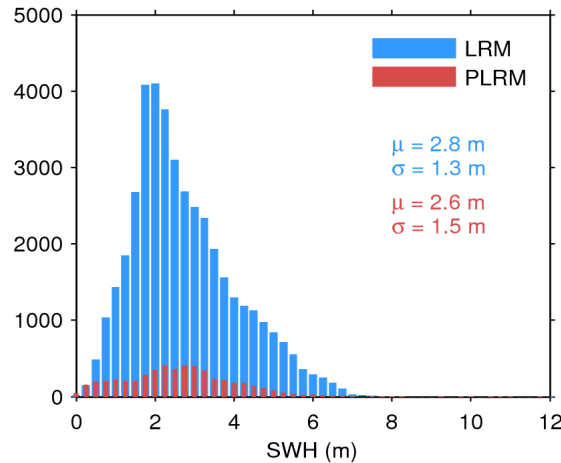
Figure 17. Histogram of flag-valid SWH over oceans and lakes for LRM (blue) and PLRM (red) for 26/03/2015. The mean ( \mu ) and standard deviation ( \sigma ) are also shown. Note that values larger than 12 m are excluded from the histogram for the sake of readability but not from the computation of \mu and \sigma .
