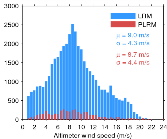
Figure 35. Histogram of science-valid wind over oceans and lakes for LRM (blue) and PLRM (red) for 25/03/2015. The mean ( \mu ) and standard deviation ( \sigma ) are also shown. Note that values larger than 24 m/s are excluded from the histogram for the sake of readability but not from the computation of \mu and \sigma .
