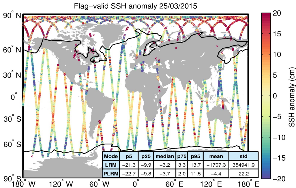
Figure 5. Geographical distribution of flag-valid 1-Hz SSH anomaly data over oceans and lakes for 25/03/2015. The statistical values shown in the table refer to the SSH anomaly in cm and are calculated separately for LRM and PLRM regions. Measurements taken over polar polygons have been excluded from the computation of the statistical values. The black lines mark the outer limit of the Arctic and Antarctic polar polygons.
