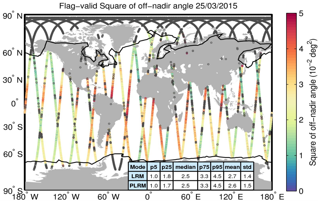
Figure 37. Geographical distribution of flag-valid mispointing data over oceans and lakes for 25/03/2015. The statistical values shown in the table refer to the mispointing in 10^{-2} \text{ deg}^2 and are calculated separately for LRM and PLRM regions. Measurements taken over polar polygons have been excluded from the computation of the statistical values. The black lines mark the outer limit of the Arctic and Antarctic polar polygons. Gray circles denote negative values.
