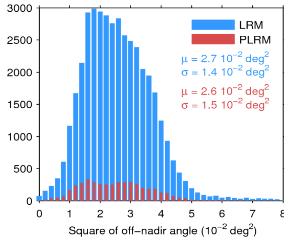
Figure 39. Histogram of flag-valid mispointing over oceans and lakes for LRM (blue) and PLRM (red) for 25/03/2015. Only positive values have been considered. The mean ( \mu ) and standard deviation ( \sigma ) are also shown. Note that values larger than 8 \cdot 10^{-2} \text{ deg}^2 are excluded from the histogram for the sake of readability but not from the computation of \mu and \sigma .
