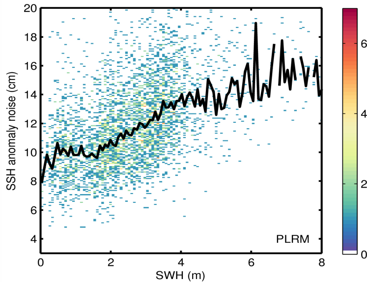
Figure 9. 2D histogram showing flag-valid SSH anomaly noise as a function of SWH for LRM (top) and PLRM (bottom) for 25/03/2015. The black line denotes the median SSH anomaly as a function of SWH.
