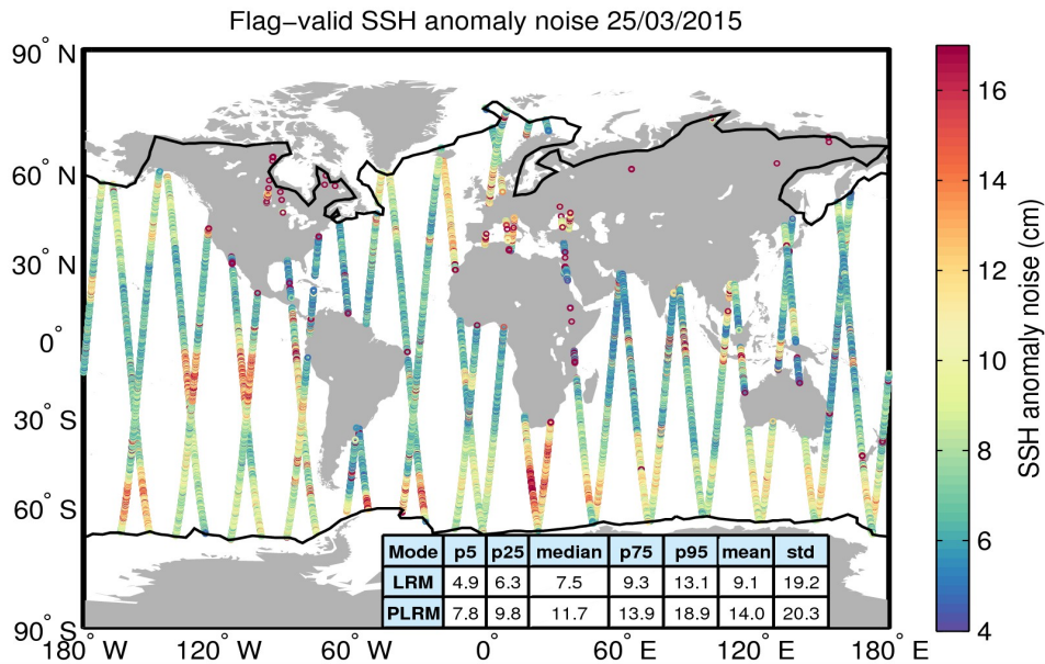
Figure 8. Geographical distribution of flag-valid 20-Hz SSH anomaly measurement noise over oceans and lakes for 25/03/2015. The statistical values shown in the table refer to the SSH anomaly noise and are calculated separately for LRM and PLRM regions. Measurements taken over polar polygons have been excluded from the computation of the statistical values. The black lines mark the outer limit of the Arctic and Antarctic polar polygons.
