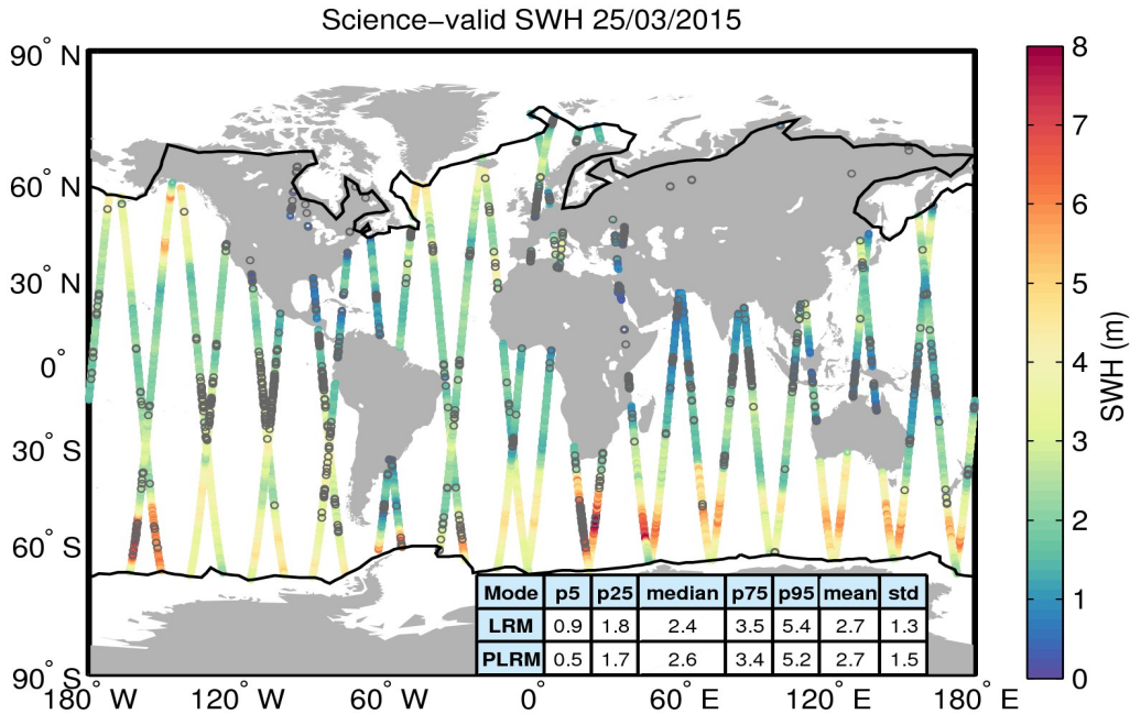
Figure 19. Geographical distribution of science-valid SWH data over oceans and lakes for 25/03/2015. The statistical values shown in the table refer to the SWH in m and are calculated separately for LRM and PLRM regions. The black lines mark the outer limit of the Arctic and Antarctic polar polygons. Gray circles denote records that have been rejected based on the editing criteria described in Table 3.
