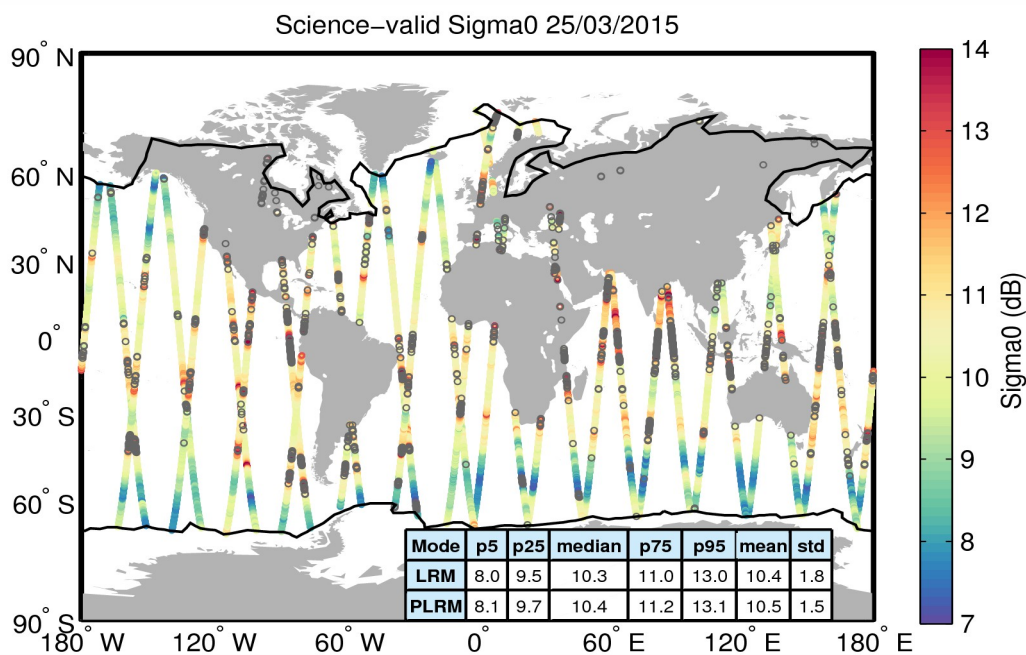
Figure 27. Geographical distribution of science-valid sigma0 data over oceans and lakes for 25/03/2015. The statistical values shown in the table refer to the sigma0 in dB and are calculated separately for LRM and PLRM regions. The black lines mark the outer limit of the Arctic and Antarctic polar polygons. Gray circles denote records that have been rejected based on the editing criteria described in Table 4.
