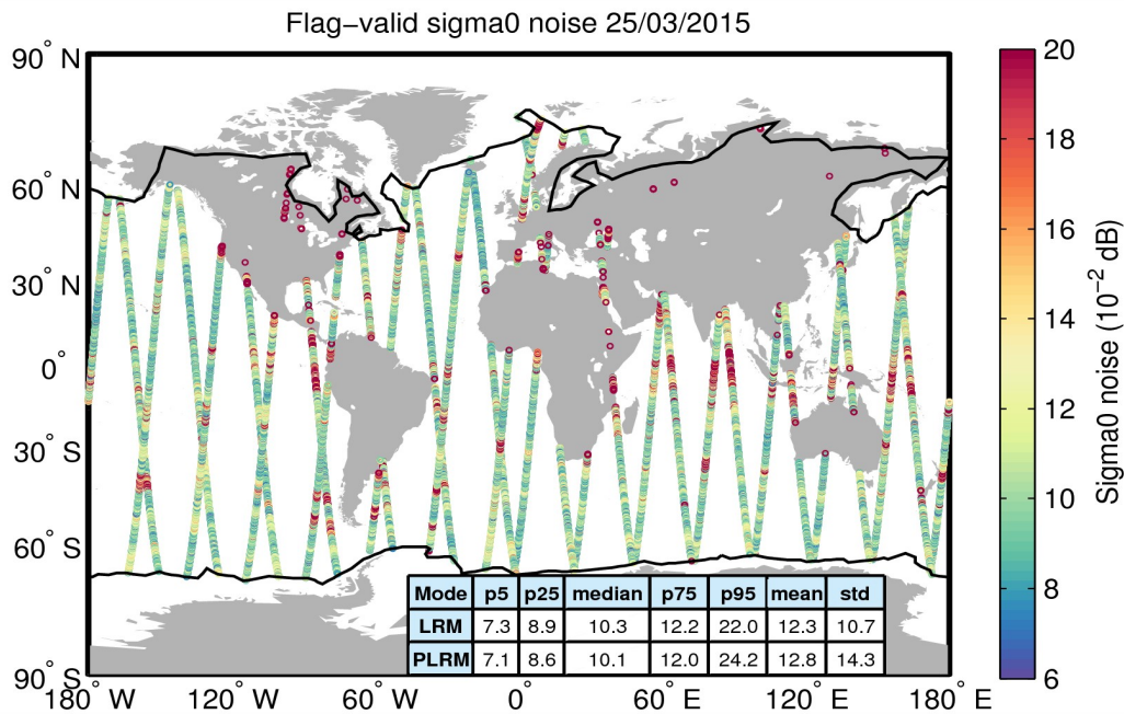
Figure 26. Geographical distribution of flag-valid 20-Hz sigma0 measurement noise over oceans and lakes for 25/03/2015. The statistical values shown in the table refer to the sigma0 noise and are calculated separately for LRM and PLRM regions. Measurements taken over polar polygons have been excluded from the computation of the statistical values. The black lines mark the outer limit of the Arctic and Antarctic polar polygons.
