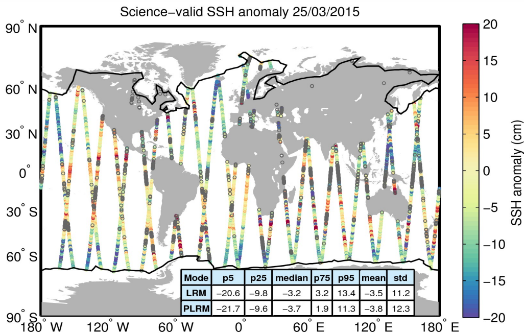
Figure 10. Geographical distribution of science-valid SSH anomaly data over oceans and lakes for 25/03/2015. The statistical values shown in the table refer to the SSH anomaly in cm and are calculated separately for LRM and PLRM regions. The black lines mark the outer limit of the Arctic and Antarctic polar polygons. Gray circles denote records that have been rejected based on the editing criteria described in Table 2.
