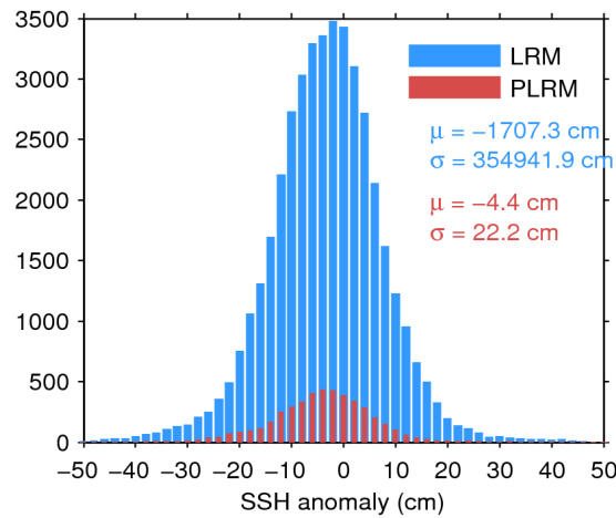
Figure 7. Histogram of flag-valid SSH anomaly over oceans and lakes for LRM (blue) and PLRM (red) for 25/03/2015. The mean ( \mu ) and standard deviation ( \sigma ) are also shown. Note that values outside [-50\ 50] cm are excluded from the histogram for the sake of readability but not from the computation of \mu and \sigma .
