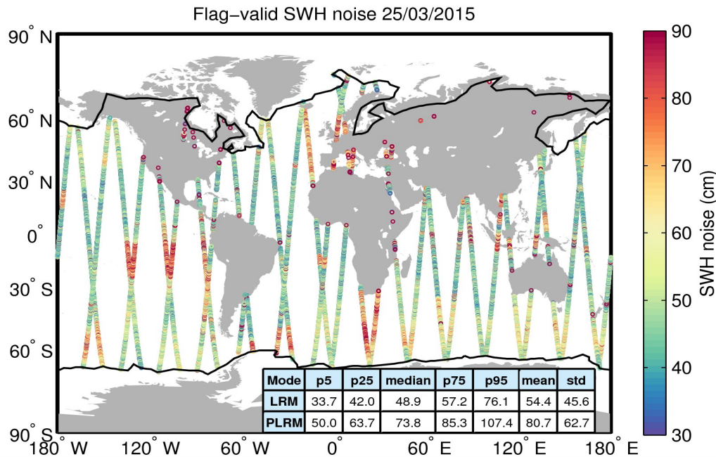
Figure 18. Geographical distribution of flag-valid 20-Hz SWH measurement noise over oceans and lakes for 25/03/2015. The statistical values shown in the table refer to the SWH noise and are calculated separately for LRM and PLRM regions. Measurements taken over polar polygons have been excluded from the computation of the statistical values. The black lines mark the outer limit of the Arctic and Antarctic polar polygons.
