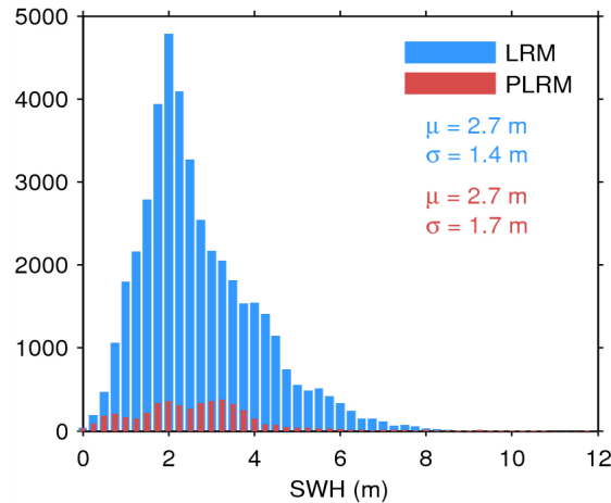
Figure 17. Histogram of flag-valid SWH over oceans and lakes for LRM (blue) and PLRM (red) for 25/03/2015. The mean ( \mu ) and standard deviation ( \sigma ) are also shown. Note that values larger than 12 m are excluded from the histogram for the sake of readability but not from the computation of \mu and \sigma .
