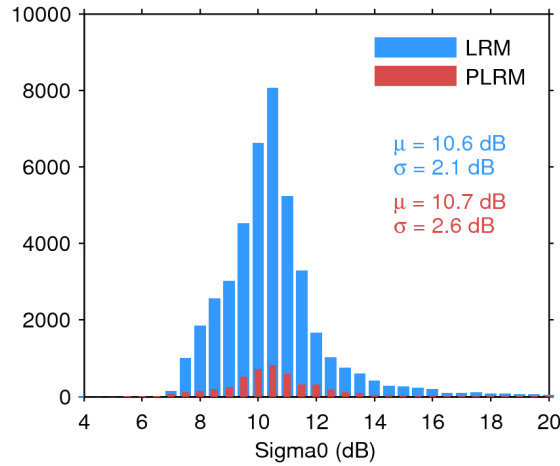
Figure 25. Histogram of flag-valid sigma0 over oceans and lakes for LRM (blue) and PLRM (red) for 25/03/2015. The mean ( \mu ) and standard deviation ( \sigma ) are also shown. Note that values outside [4 20] dB are excluded from the histogram for the sake of readability but not from the computation of \mu and \sigma .
