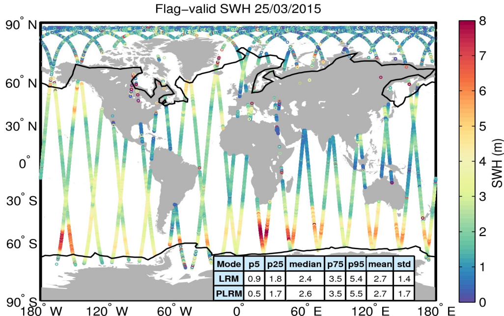
Figure 15. Geographical distribution of flag-valid SWH data over oceans and lakes for 25/03/2015. The statistical values shown in the table refer to the SWH in m and are calculated separately for LRM and PLRM regions. Measurements taken over polar polygons have been excluded from the computation of the statistical values. The black lines mark the outer limit of the Arctic and Antarctic polar polygons.
