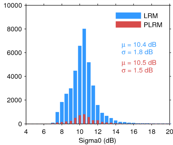
Figure 28. Histogram of science-valid sigma0 over oceans and lakes for LRM (blue) and PLRM (red) for 25/03/2015. The mean ( \mu ) and standard deviation ( \sigma ) are also shown. Note that values outside [4 20] dB are excluded from the histogram for the sake of readability but not from the computation of \mu and \sigma .
