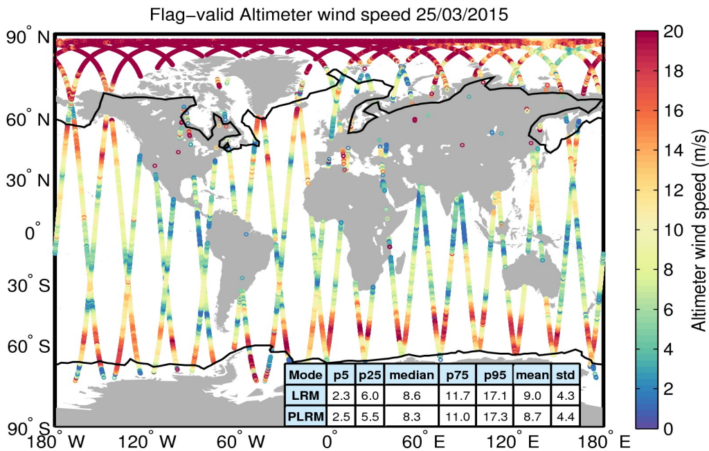
Figure 31. Geographical distribution of flag-valid wind data over oceans and lakes for 25/03/2015. The statistical values shown in the table refer to the wind in m/s and are calculated separately for LRM and PLRM regions. Measurements taken over polar polygons have been excluded from the computation of the statistical values. The black lines mark the outer limit of the Arctic and Antarctic polar polygons.
