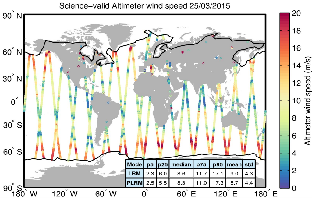
Figure 34. Geographical distribution of science-valid wind data over oceans and lakes for 25/03/2015. The statistical values shown in the table refer to the wind in m/s and are calculated separately for LRM and PLRM regions. The black lines mark the outer limit of the Arctic and Antarctic polar polygons. Gray circles denote records that have been rejected based on the editing criteria described in Table 5.
