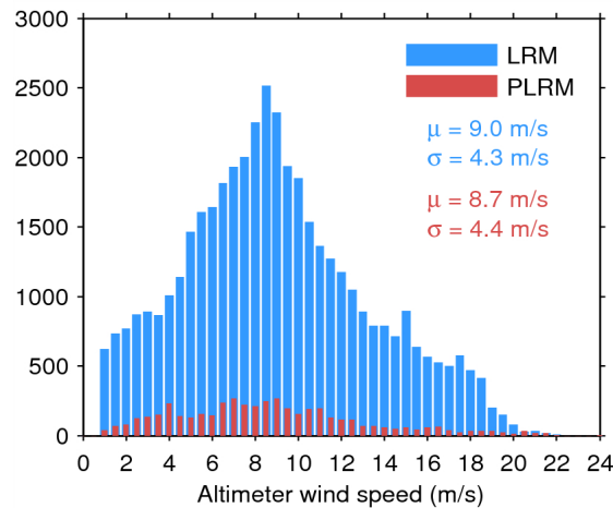
Figure 33. Histogram of flag-valid wind over oceans and lakes for LRM (blue) and PLRM (red) for 25/03/2015. The mean ( \mu ) and standard deviation ( \sigma ) are also shown. Note that values larger than 24 m/s are excluded from the histogram for the sake of readability but not from the computation of \mu and \sigma .
