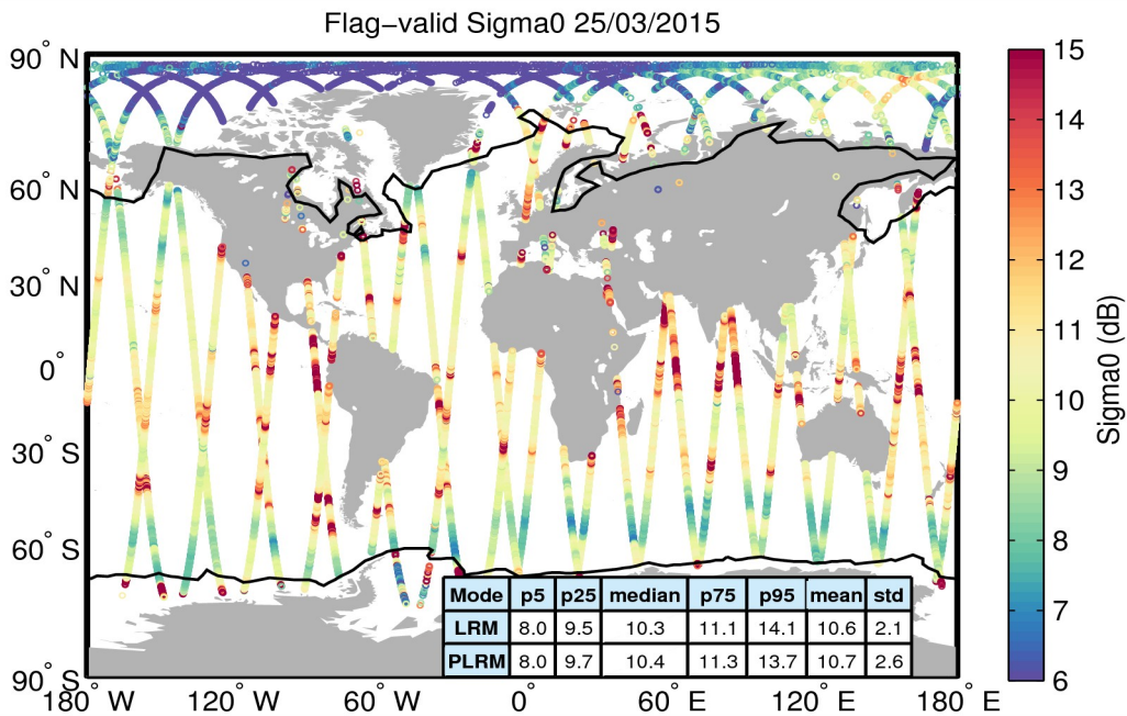
Figure 23. Geographical distribution of flag-valid sigma0 data over oceans and lakes for 25/03/2015. The statistical values shown in the table refer to the sigma0 in dB and are calculated separately for LRM and PLRM regions. Measurements taken over polar polygons have been excluded from the computation of the statistical values. The black lines mark the outer limit of the Arctic and Antarctic polar polygons.
