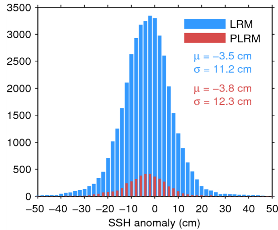
Figure 11. Histogram of science-valid SSH anomaly over oceans and lakes for LRM (blue) and PLRM (red) for 25/03/2015. The mean ( \mu ) and standard deviation ( \sigma ) are also shown. Note that values outside [-50\ 50] cm are excluded from the histogram for the sake of readability but not from the computation of \mu and \sigma .
