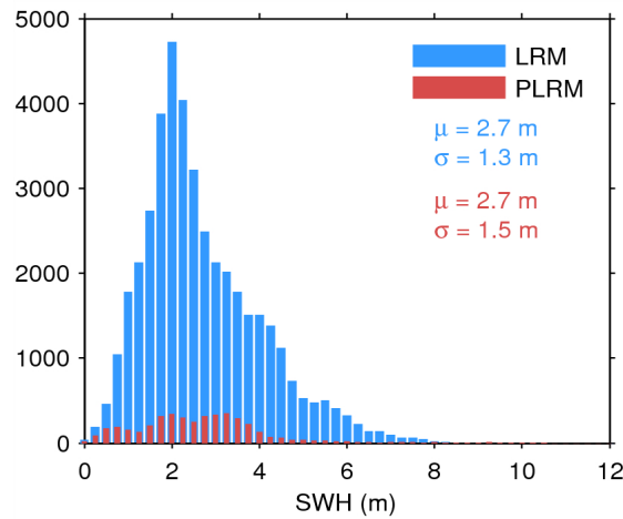
Figure 20. Histogram of science-valid SWH over oceans and lakes for LRM (blue) and PLRM (red) for 25/03/2015. The mean ( \mu ) and standard deviation ( \sigma ) are also shown. Note that values larger than 12 m are excluded from the histogram for the sake of readability but not from the computation of \mu and \sigma .
