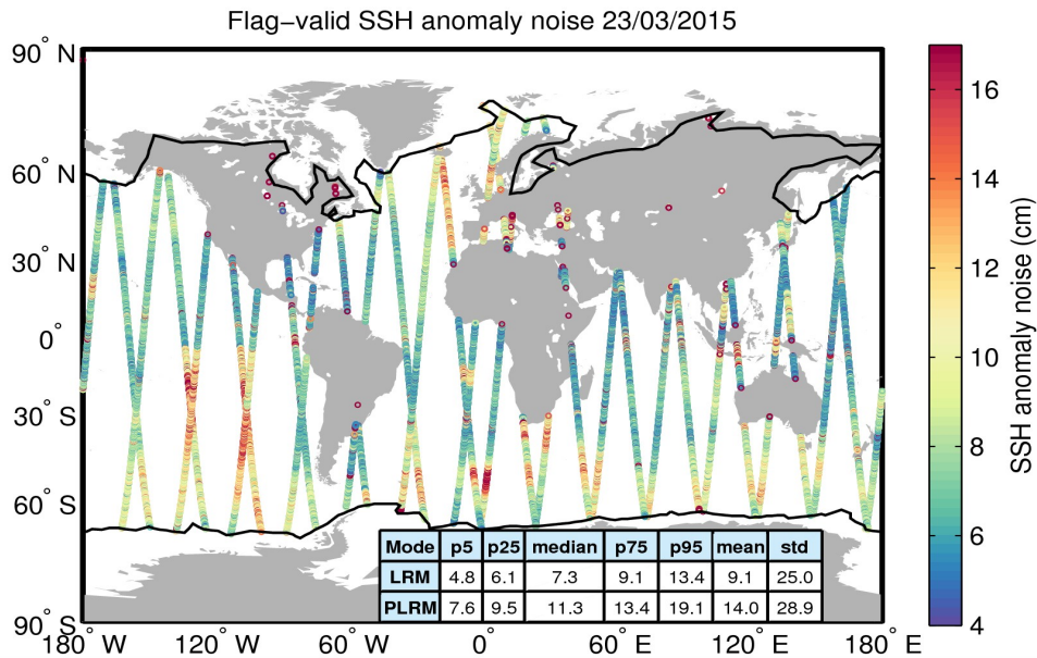
Figure 8. Geographical distribution of flag-valid 20-Hz SSH anomaly measurement noise over oceans and lakes for 23/03/2015. The statistical values shown in the table refer to the SSH anomaly noise and are calculated separately for LRM and PLRM regions. Measurements taken over polar polygons have been excluded from the computation of the statistical values. The black lines mark the outer limit of the Arctic and Antarctic polar polygons.
