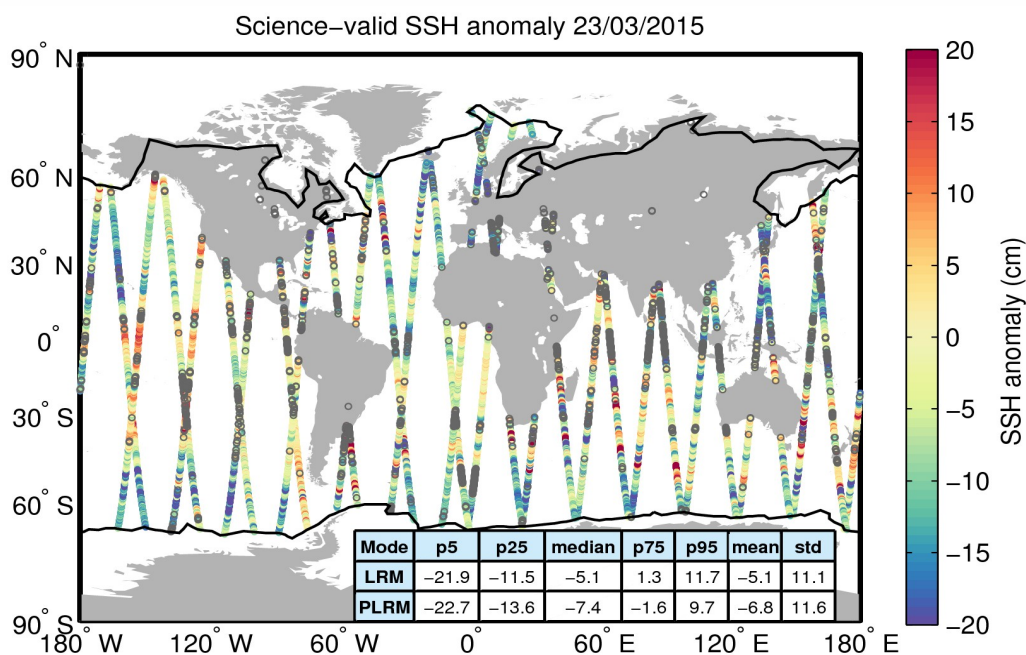
Figure 10. Geographical distribution of science-valid SSH anomaly data over oceans and lakes for 23/03/2015. The statistical values shown in the table refer to the SSH anomaly in cm and are calculated separately for LRM and PLRM regions. The black lines mark the outer limit of the Arctic and Antarctic polar polygons. Gray circles denote records that have been rejected based on the editing criteria described in Table 2.
