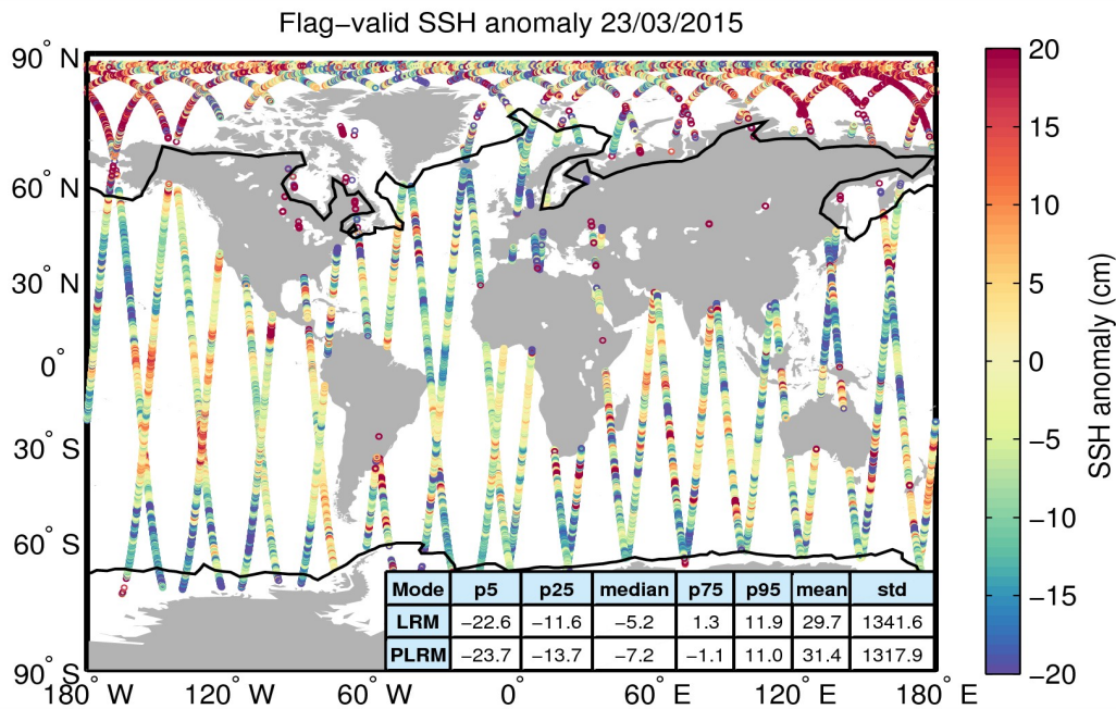
Figure 5. Geographical distribution of flag-valid 1-Hz SSH anomaly data over oceans and lakes for 23/03/2015. The statistical values shown in the table refer to the SSH anomaly in cm and are calculated separately for LRM and PLRM regions. Measurements taken over polar polygons have been excluded from the computation of the statistical values. The black lines mark the outer limit of the Arctic and Antarctic polar polygons.
