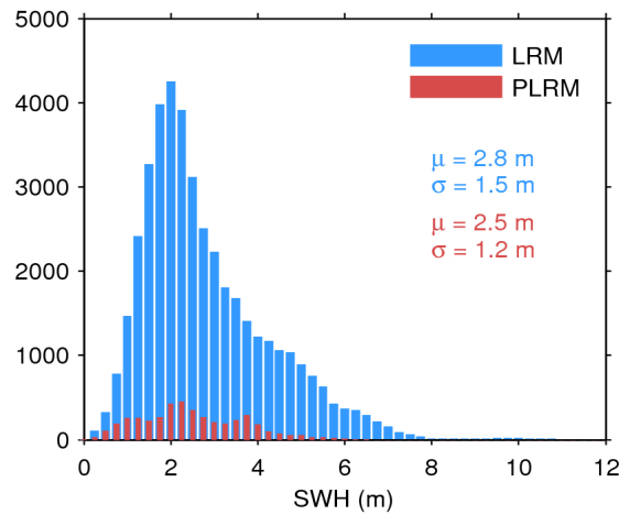
Figure 20. Histogram of science-valid SWH over oceans and lakes for LRM (blue) and PLRM (red) for 23/03/2015. The mean ( \mu ) and standard deviation ( \sigma ) are also shown. Note that values larger than 12 m are excluded from the histogram for the sake of readability but not from the computation of \mu and \sigma .
