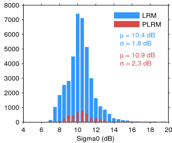
Figure 28. Histogram of science-valid sigma0 over oceans and lakes for LRM (blue) and PLRM (red) for 23/03/2015. The mean ( \mu ) and standard deviation ( \sigma ) are also shown. Note that values outside [4 20] dB are excluded from the histogram for the sake of readability but not from the computation of \mu and \sigma .
