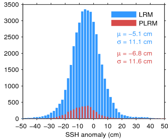
Figure 11. Histogram of science-valid SSH anomaly over oceans and lakes for LRM (blue) and PLRM (red) for 23/03/2015. The mean ( \mu ) and standard deviation ( \sigma ) are also shown. Note that values outside [-50 50] cm are excluded from the histogram for the sake of readability but not from the computation of \mu and \sigma .
