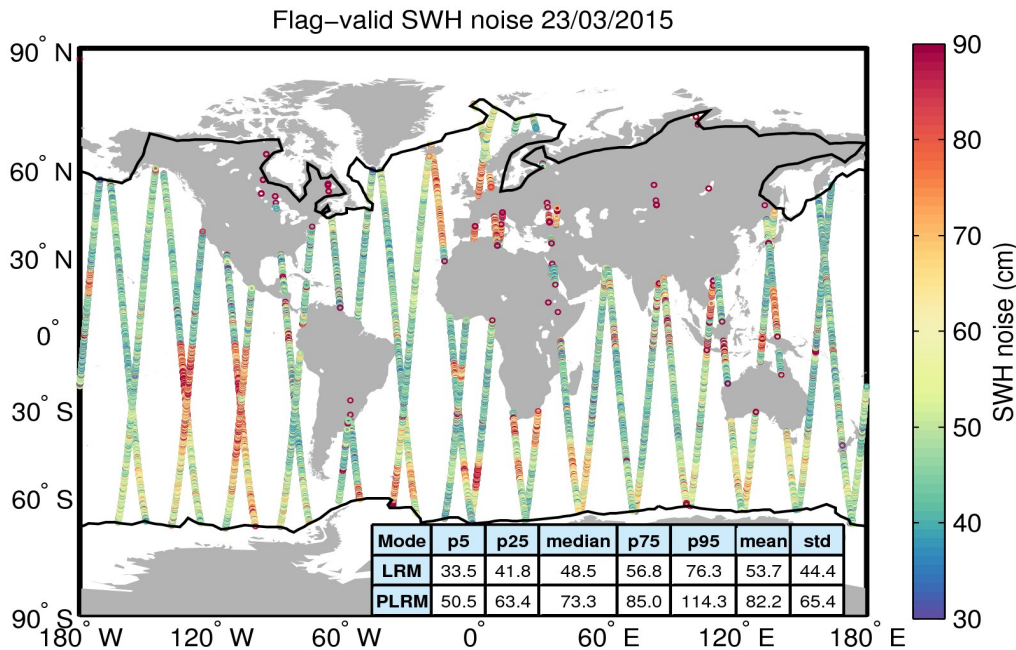
Figure 18. Geographical distribution of flag-valid 20-Hz SWH measurement noise over oceans and lakes for 23/03/2015. The statistical values shown in the table refer to the SWH noise and are calculated separately for LRM and PLRM regions. Measurements taken over polar polygons have been excluded from the computation of the statistical values. The black lines mark the outer limit of the Arctic and Antarctic polar polygons.
