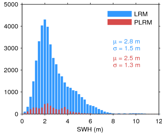
Figure 17. Histogram of flag-valid SWH over oceans and lakes for LRM (blue) and PLRM (red) for 23/03/2015. The mean ( \mu ) and standard deviation ( \sigma ) are also shown. Note that values larger than 12 m are excluded from the histogram for the sake of readability but not from the computation of \mu and \sigma .
