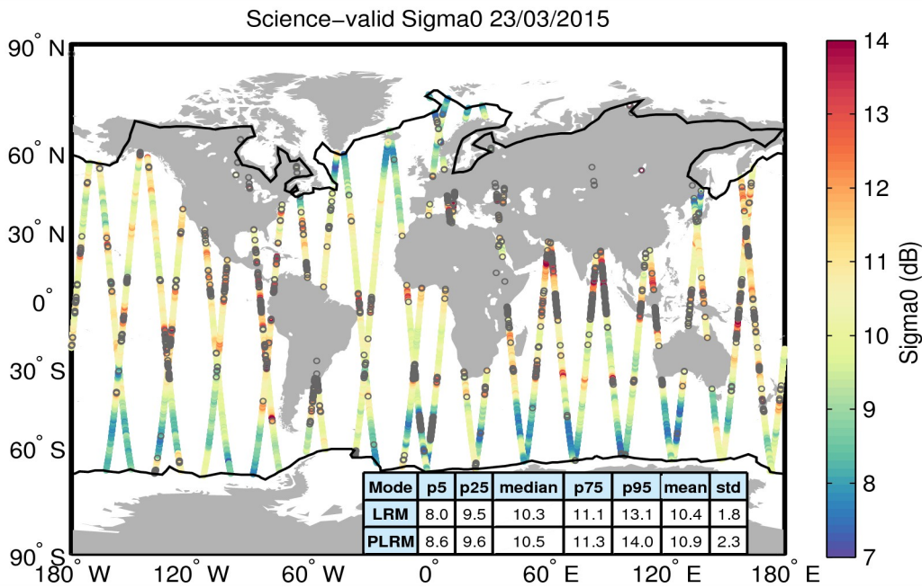
Figure 27. Geographical distribution of science-valid sigma0 data over oceans and lakes for 23/03/2015. The statistical values shown in the table refer to the sigma0 in dB and are calculated separately for LRM and PLRM regions. The black lines mark the outer limit of the Arctic and Antarctic polar polygons. Gray circles denote records that have been rejected based on the editing criteria described in Table 4.
