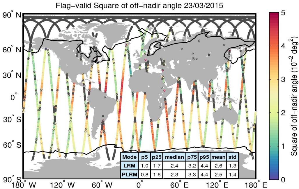
Figure 37. Geographical distribution of flag-valid mispointing data over oceans and lakes for 23/03/2015. The statistical values shown in the table refer to the mispointing in 10^{-2} \text{ deg}^2 and are calculated separately for LRM and PLRM regions. Measurements taken over polar polygons have been excluded from the computation of the statistical values. The black lines mark the outer limit of the Arctic and Antarctic polar polygons. Gray circles denote negative values.
