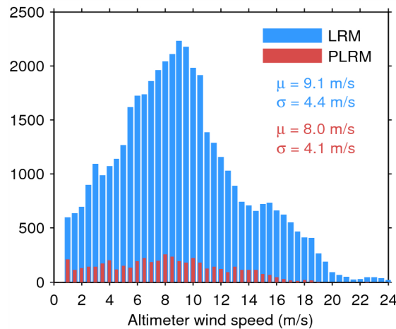
Figure 33. Histogram of flag-valid wind over oceans and lakes for LRM (blue) and PLRM (red) for 23/03/2015. The mean ( \mu ) and standard deviation ( \sigma ) are also shown. Note that values larger than 24 m/s are excluded from the histogram for the sake of readability but not from the computation of \mu and \sigma .
