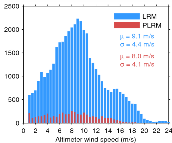
Figure 35. Histogram of science-valid wind over oceans and lakes for LRM (blue) and PLRM (red) for 23/03/2015. The mean ( \mu ) and standard deviation ( \sigma ) are also shown. Note that values larger than 24 m/s are excluded from the histogram for the sake of readability but not from the computation of \mu and \sigma .
