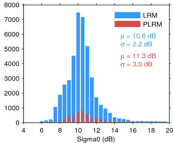
Figure 25. Histogram of flag-valid sigma0 over oceans and lakes for LRM (blue) and PLRM (red) for 23/03/2015. The mean ( \mu ) and standard deviation ( \sigma ) are also shown. Note that values outside [4 20] dB are excluded from the histogram for the sake of readability but not from the computation of \mu and \sigma .
