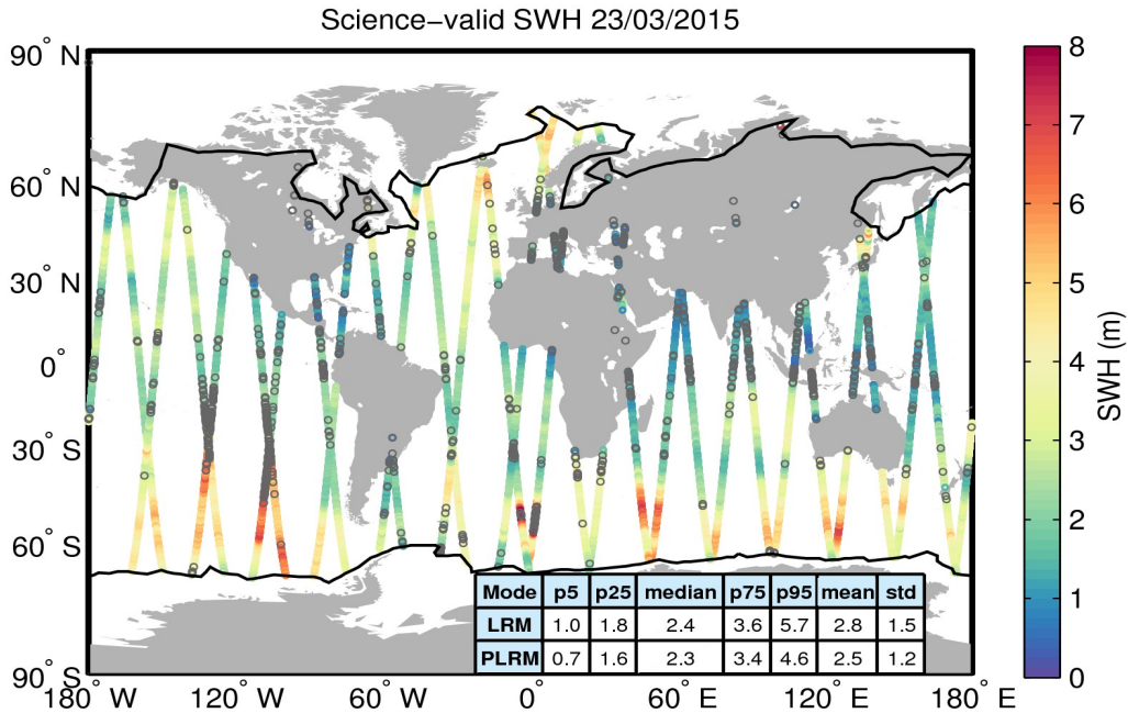
Figure 19. Geographical distribution of science-valid SWH data over oceans and lakes for 23/03/2015. The statistical values shown in the table refer to the SWH in m and are calculated separately for LRM and PLRM regions. The black lines mark the outer limit of the Arctic and Antarctic polar polygons. Gray circles denote records that have been rejected based on the editing criteria described in Table 3.
