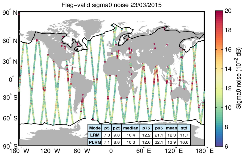
Figure 26. Geographical distribution of flag-valid 20-Hz sigma0 measurement noise over oceans and lakes for 23/03/2015. The statistical values shown in the table refer to the sigma0 noise and are calculated separately for LRM and PLRM regions. Measurements taken over polar polygons have been excluded from the computation of the statistical values. The black lines mark the outer limit of the Arctic and Antarctic polar polygons.
