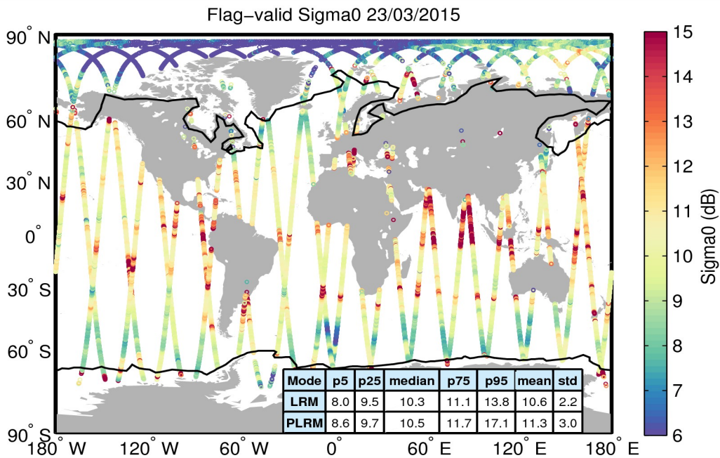
Figure 23. Geographical distribution of flag-valid sigma0 data over oceans and lakes for 23/03/2015. The statistical values shown in the table refer to the sigma0 in dB and are calculated separately for LRM and PLRM regions. Measurements taken over polar polygons have been excluded from the computation of the statistical values. The black lines mark the outer limit of the Arctic and Antarctic polar polygons.
