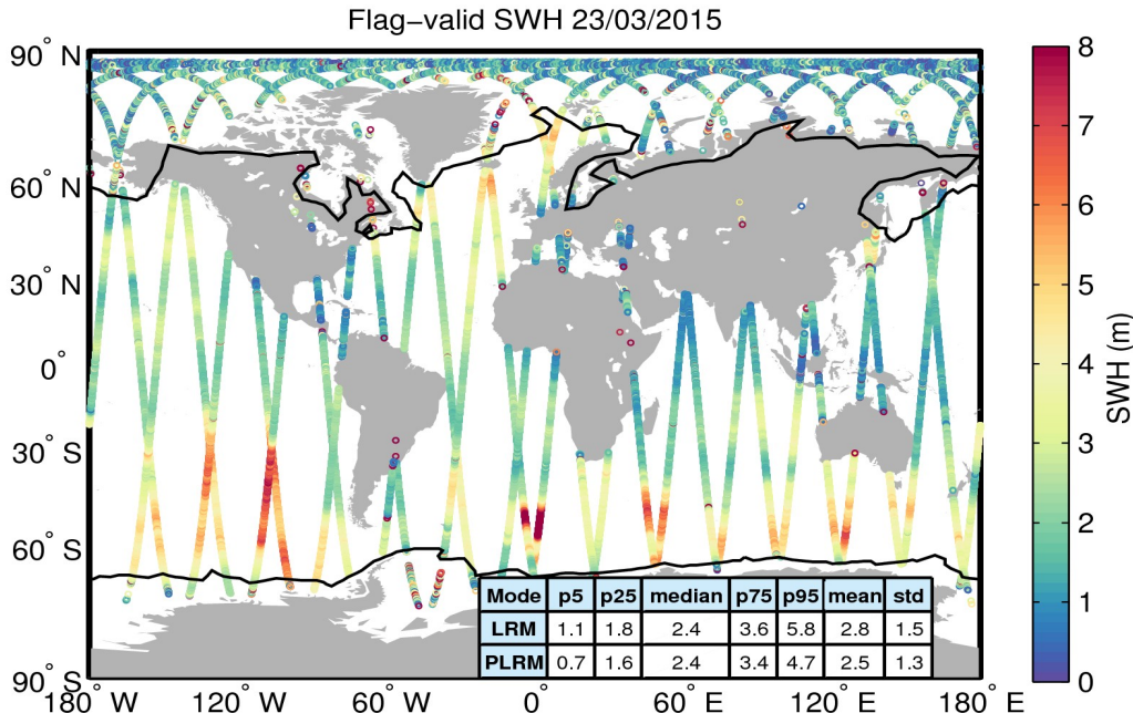
Figure 15. Geographical distribution of flag-valid SWH data over oceans and lakes for 23/03/2015. The statistical values shown in the table refer to the SWH in m and are calculated separately for LRM and PLRM regions. Measurements taken over polar polygons have been excluded from the computation of the statistical values. The black lines mark the outer limit of the Arctic and Antarctic polar polygons.
