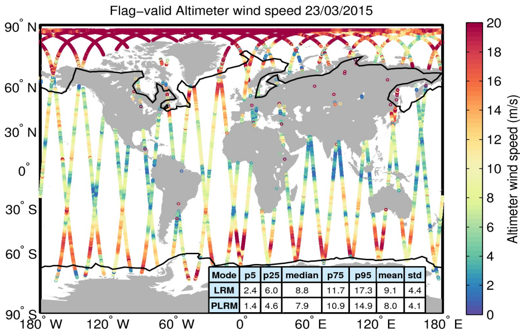
Figure 31. Geographical distribution of flag-valid wind data over oceans and lakes for 23/03/2015. The statistical values shown in the table refer to the wind in m/s and are calculated separately for LRM and PLRM regions. Measurements taken over polar polygons have been excluded from the computation of the statistical values. The black lines mark the outer limit of the Arctic and Antarctic polar polygons.
