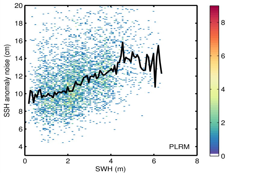
Figure 9. 2D histogram showing flag-valid SSH anomaly noise as a function of SWH for LRM (top) and PLRM (bottom) for 23/03/2015. The black line denotes the median SSH anomaly as a function of SWH.
