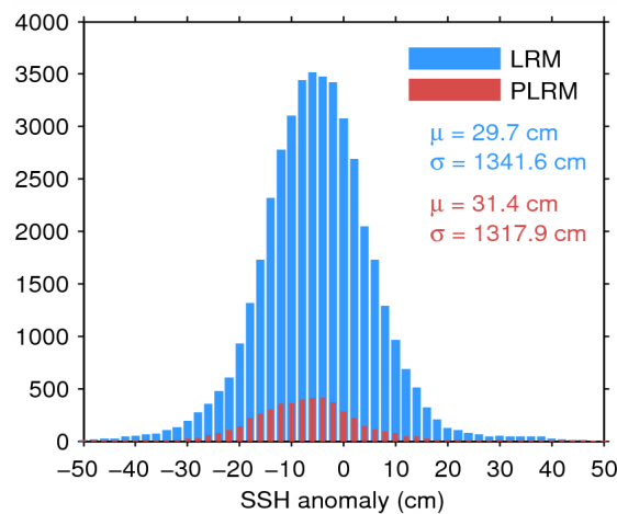
Figure 7. Histogram of flag-valid SSH anomaly over oceans and lakes for LRM (blue) and PLRM (red) for 23/03/2015. The mean ( \mu ) and standard deviation ( \sigma ) are also shown. Note that values outside [-50\ 50] cm are excluded from the histogram for the sake of readability but not from the computation of \mu and \sigma .
