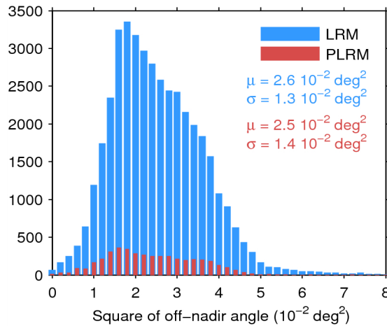
Figure 39. Histogram of flag-valid mispointing over oceans and lakes for LRM (blue) and PLRM (red) for 23/03/2015. Only positive values have been considered. The mean ( \mu ) and standard deviation ( \sigma ) are also shown. Note that values larger than 8 \cdot 10^{-2} \text{ deg}^2 are excluded from the histogram for the sake of readability but not from the computation of \mu and \sigma .
