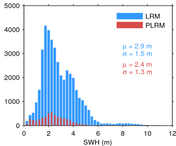
Figure 17. Histogram of flag-valid SWH over oceans and lakes for LRM (blue) and PLRM (red) for 20/03/2015. The mean ( \mu ) and standard deviation ( \sigma ) are also shown. Note that values larger than 12 m are excluded from the histogram for the sake of readability but not from the computation of \mu and \sigma .
