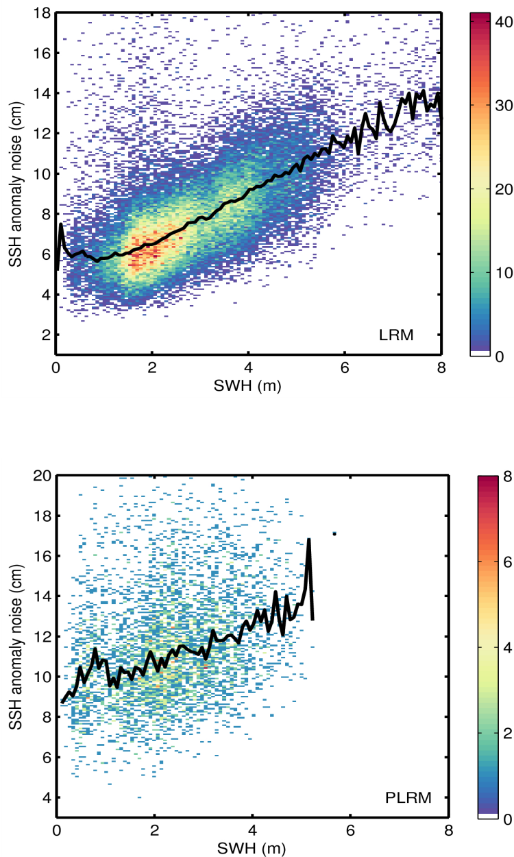
Figure 9. 2D histogram showing flag-valid SSH anomaly noise as a function of SWH for LRM (top) and PLRM (bottom) for 20/03/2015. The black line denotes the median SSH anomaly as a function of SWH.
