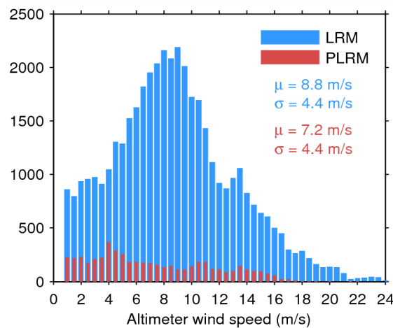
Figure 33. Histogram of flag-valid wind over oceans and lakes for LRM (blue) and PLRM (red) for 20/03/2015. The mean ( \mu ) and standard deviation ( \sigma ) are also shown. Note that values larger than 24 m/s are excluded from the histogram for the sake of readability but not from the computation of \mu and \sigma .
