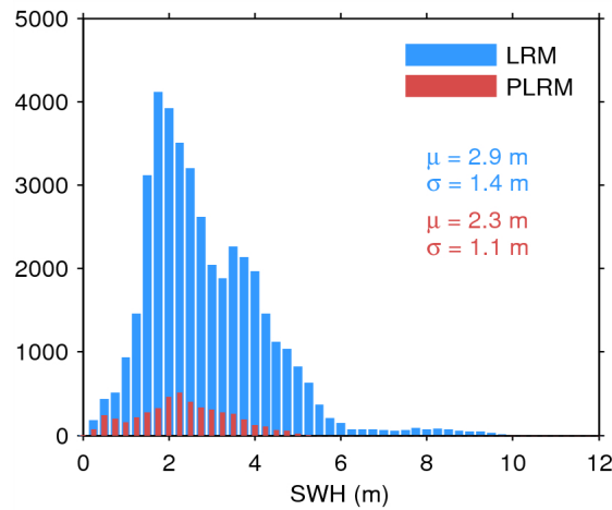
Figure 20. Histogram of science-valid SWH over oceans and lakes for LRM (blue) and PLRM (red) for 20/03/2015. The mean ( \mu ) and standard deviation ( \sigma ) are also shown. Note that values larger than 12 m are excluded from the histogram for the sake of readability but not from the computation of \mu and \sigma .
