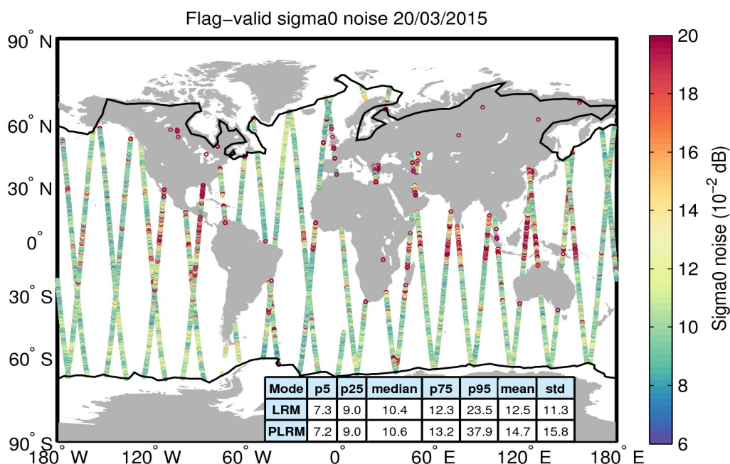
Figure 26. Geographical distribution of flag-valid 20-Hz sigma0 measurement noise over oceans and lakes for 20/03/2015. The statistical values shown in the table refer to the sigma0 noise and are calculated separately for LRM and PLRM regions. Measurements taken over polar polygons have been excluded from the computation of the statistical values. The black lines mark the outer limit of the Arctic and Antarctic polar polygons.
