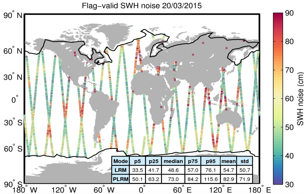
Figure 18. Geographical distribution of flag-valid 20-Hz SWH measurement noise over oceans and lakes for 20/03/2015. The statistical values shown in the table refer to the SWH noise and are calculated separately for LRM and PLRM regions. Measurements taken over polar polygons have been excluded from the computation of the statistical values. The black lines mark the outer limit of the Arctic and Antarctic polar polygons.
