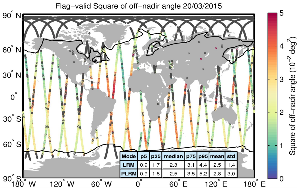
Figure 37. Geographical distribution of flag-valid mispointing data over oceans and lakes for 20/03/2015. The statistical values shown in the table refer to the mispointing in 10^{-2} \text{ deg}^2 and are calculated separately for LRM and PLRM regions. Measurements taken over polar polygons have been excluded from the computation of the statistical values. The black lines mark the outer limit of the Arctic and Antarctic polar polygons. Gray circles denote negative values.
