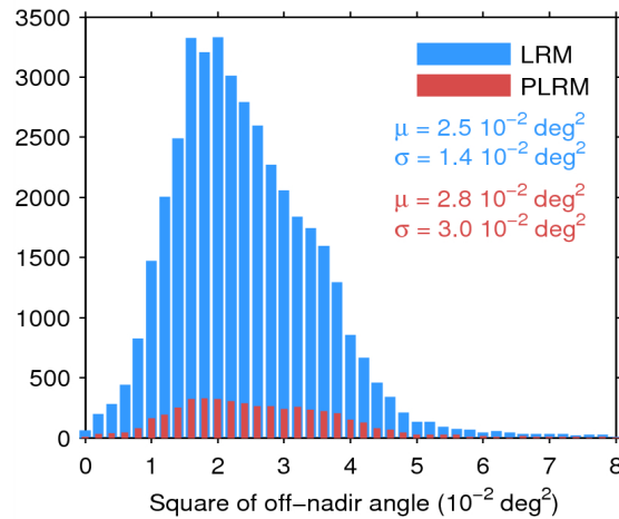
Figure 39. Histogram of flag-valid mispointing over oceans and lakes for LRM (blue) and PLRM (red) for 20/03/2015. Only positive values have been considered. The mean ( \mu ) and standard deviation ( \sigma ) are also shown. Note that values larger than 8 \cdot 10^{-2} \text{ deg}^2 are excluded from the histogram for the sake of readability but not from the computation of \mu and \sigma .
