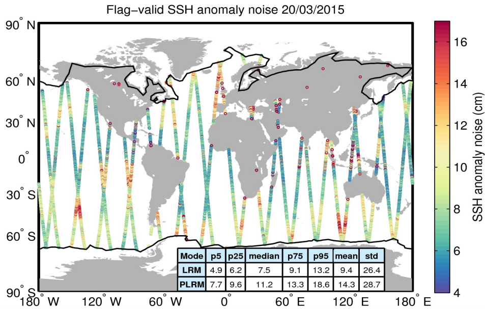
Figure 8. Geographical distribution of flag-valid 20-Hz SSH anomaly measurement noise over oceans and lakes for 20/03/2015. The statistical values shown in the table refer to the SSH anomaly noise and are calculated separately for LRM and PLRM regions. Measurements taken over polar polygons have been excluded from the computation of the statistical values. The black lines mark the outer limit of the Arctic and Antarctic polar polygons.
