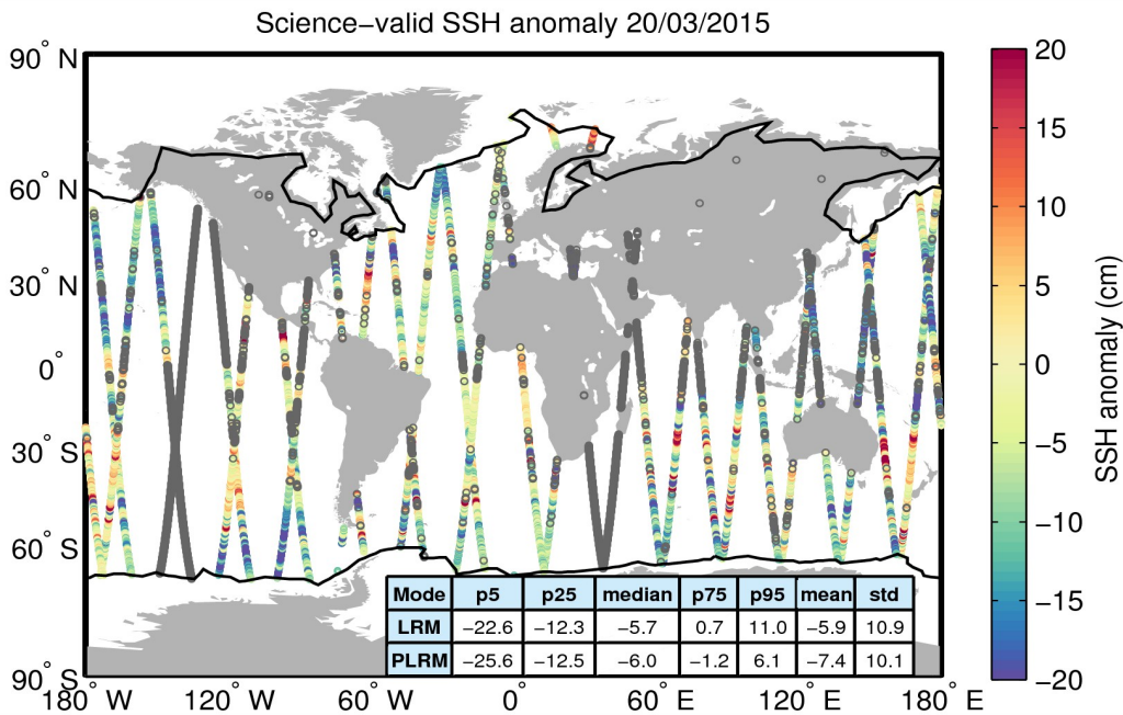
Figure 10. Geographical distribution of science-valid SSH anomaly data over oceans and lakes for 20/03/2015. The statistical values shown in the table refer to the SSH anomaly in cm and are calculated separately for LRM and PLRM regions. The black lines mark the outer limit of the Arctic and Antarctic polar polygons. Gray circles denote records that have been rejected based on the editing criteria described in Table 2.
