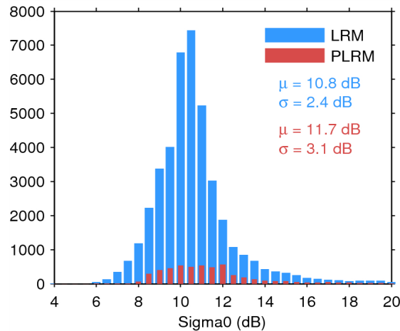
Figure 25. Histogram of flag-valid sigma0 over oceans and lakes for LRM (blue) and PLRM (red) for 20/03/2015. The mean ( \mu ) and standard deviation ( \sigma ) are also shown. Note that values outside [4 20] dB are excluded from the histogram for the sake of readability but not from the computation of \mu and \sigma .
