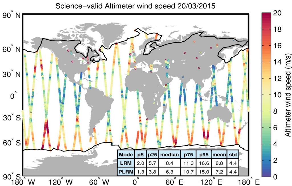
Figure 34. Geographical distribution of science-valid wind data over oceans and lakes for 20/03/2015. The statistical values shown in the table refer to the wind in m/s and are calculated separately for LRM and PLRM regions. The black lines mark the outer limit of the Arctic and Antarctic polar polygons. Gray circles denote records that have been rejected based on the editing criteria described in Table 5.
