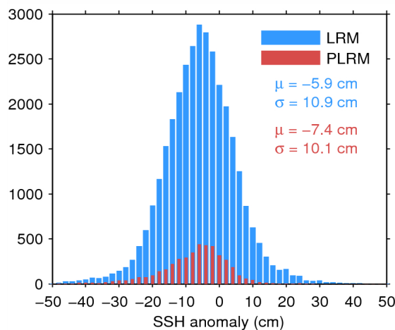
Figure 11. Histogram of science-valid SSH anomaly over oceans and lakes for LRM (blue) and PLRM (red) for 20/03/2015. The mean ( \mu ) and standard deviation ( \sigma ) are also shown. Note that values outside [-50 50] cm are excluded from the histogram for the sake of readability but not from the computation of \mu and \sigma .
