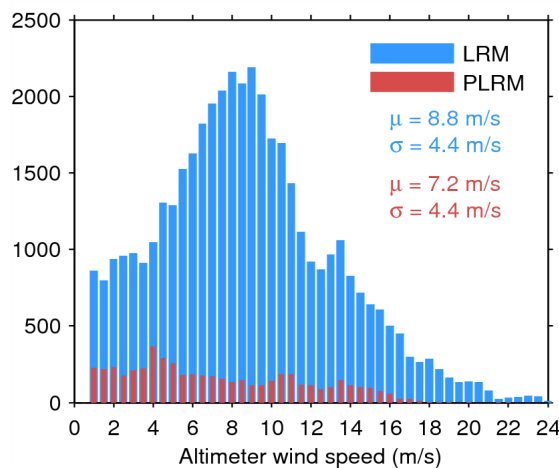
Figure 35. Histogram of science-valid wind over oceans and lakes for LRM (blue) and PLRM (red) for 20/03/2015. The mean ( \mu ) and standard deviation ( \sigma ) are also shown. Note that values larger than 24 m/s are excluded from the histogram for the sake of readability but not from the computation of \mu and \sigma .
