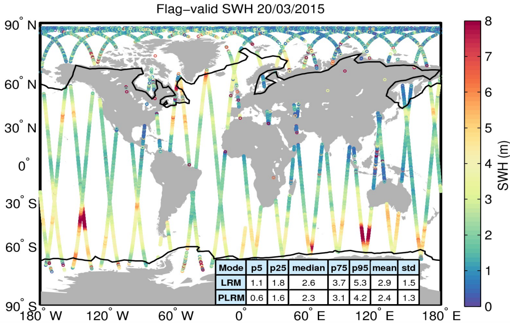
Figure 15. Geographical distribution of flag-valid SWH data over oceans and lakes for 20/03/2015. The statistical values shown in the table refer to the SWH in m and are calculated separately for LRM and PLRM regions. Measurements taken over polar polygons have been excluded from the computation of the statistical values. The black lines mark the outer limit of the Arctic and Antarctic polar polygons.
