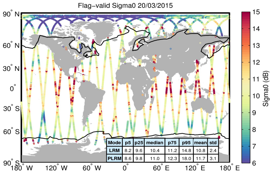
Figure 23. Geographical distribution of flag-valid sigma0 data over oceans and lakes for 20/03/2015. The statistical values shown in the table refer to the sigma0 in dB and are calculated separately for LRM and PLRM regions. Measurements taken over polar polygons have been excluded from the computation of the statistical values. The black lines mark the outer limit of the Arctic and Antarctic polar polygons.
