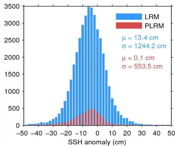
Figure 7. Histogram of flag-valid SSH anomaly over oceans and lakes for LRM (blue) and PLRM (red) for 20/03/2015. The mean ( \mu ) and standard deviation ( \sigma ) are also shown. Note that values outside [-50\ 50] cm are excluded from the histogram for the sake of readability but not from the computation of \mu and \sigma .
