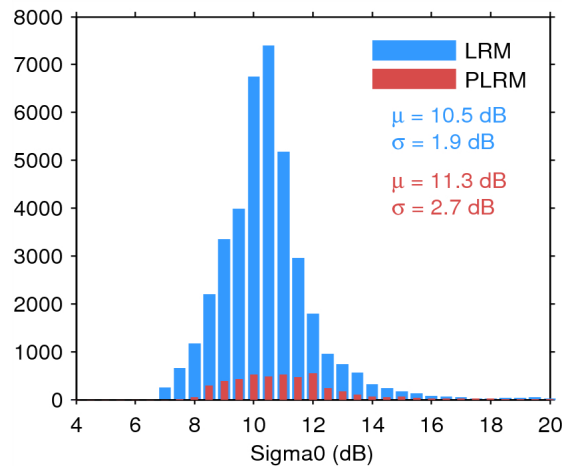
Figure 28. Histogram of science-valid sigma0 over oceans and lakes for LRM (blue) and PLRM (red) for 20/03/2015. The mean ( \mu ) and standard deviation ( \sigma ) are also shown. Note that values outside [4 20] dB are excluded from the histogram for the sake of readability but not from the computation of \mu and \sigma .
