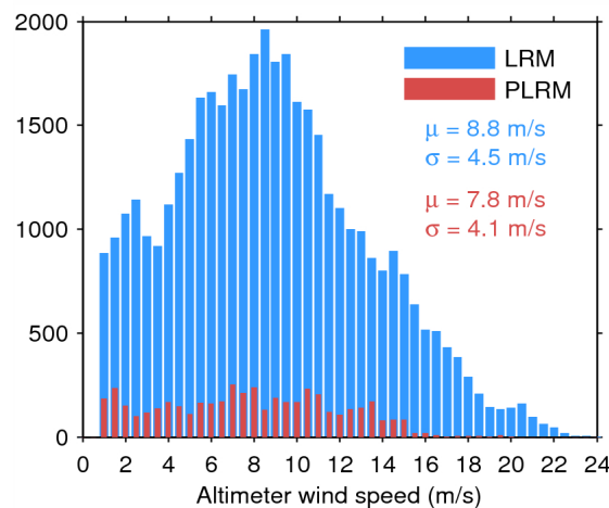
Figure 35. Histogram of science-valid wind over oceans and lakes for LRM (blue) and PLRM (red) for 19/03/2015. The mean ( \mu ) and standard deviation ( \sigma ) are also shown. Note that values larger than 24 m/s are excluded from the histogram for the sake of readability but not from the computation of \mu and \sigma .
