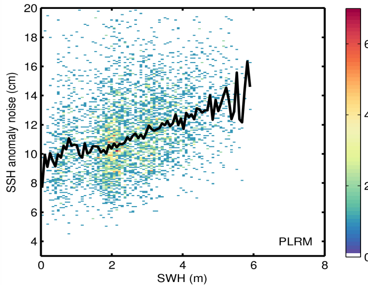
Figure 9. 2D histogram showing flag-valid SSH anomaly noise as a function of SWH for LRM (top) and PLRM (bottom) for 19/03/2015. The black line denotes the median SSH anomaly as a function of SWH.
