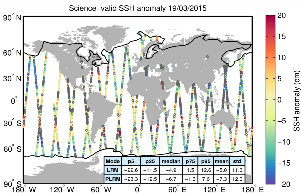
Figure 10. Geographical distribution of science-valid SSH anomaly data over oceans and lakes for 19/03/2015. The statistical values shown in the table refer to the SSH anomaly in cm and are calculated separately for LRM and PLRM regions. The black lines mark the outer limit of the Arctic and Antarctic polar polygons. Gray circles denote records that have been rejected based on the editing criteria described in Table 2.
