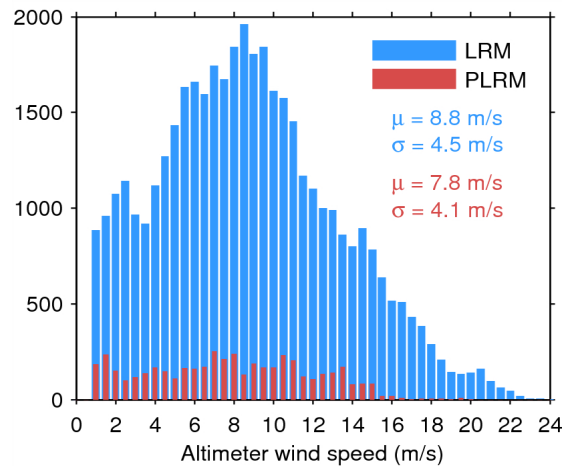
Figure 33. Histogram of flag-valid wind over oceans and lakes for LRM (blue) and PLRM (red) for 19/03/2015. The mean ( \mu ) and standard deviation ( \sigma ) are also shown. Note that values larger than 24 m/s are excluded from the histogram for the sake of readability but not from the computation of \mu and \sigma .
