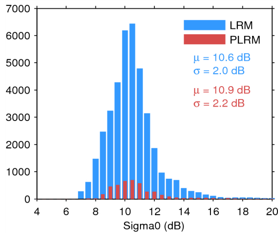
Figure 28. Histogram of science-valid sigma0 over oceans and lakes for LRM (blue) and PLRM (red) for 19/03/2015. The mean ( \mu ) and standard deviation ( \sigma ) are also shown. Note that values outside [4 20] dB are excluded from the histogram for the sake of readability but not from the computation of \mu and \sigma .
