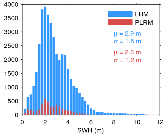
Figure 17. Histogram of flag-valid SWH over oceans and lakes for LRM (blue) and PLRM (red) for 19/03/2015. The mean ( \mu ) and standard deviation ( \sigma ) are also shown. Note that values larger than 12 m are excluded from the histogram for the sake of readability but not from the computation of \mu and \sigma .
