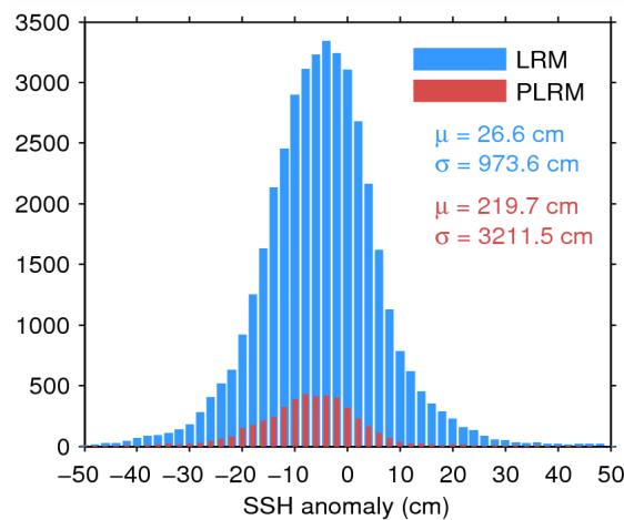
Figure 7. Histogram of flag-valid SSH anomaly over oceans and lakes for LRM (blue) and PLRM (red) for 19/03/2015. The mean ( \mu ) and standard deviation ( \sigma ) are also shown. Note that values outside [-50\ 50] cm are excluded from the histogram for the sake of readability but not from the computation of \mu and \sigma .
