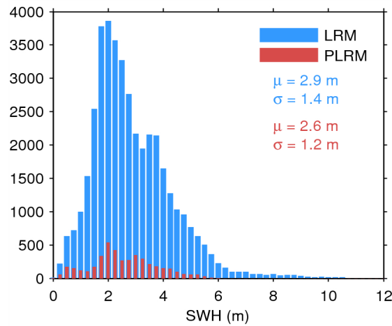
Figure 20. Histogram of science-valid SWH over oceans and lakes for LRM (blue) and PLRM (red) for 19/03/2015. The mean ( \mu ) and standard deviation ( \sigma ) are also shown. Note that values larger than 12 m are excluded from the histogram for the sake of readability but not from the computation of \mu and \sigma .
