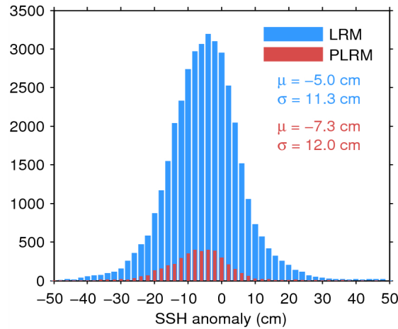
Figure 11. Histogram of science-valid SSH anomaly over oceans and lakes for LRM (blue) and PLRM (red) for 19/03/2015. The mean ( \mu ) and standard deviation ( \sigma ) are also shown. Note that values outside [-50\ 50] cm are excluded from the histogram for the sake of readability but not from the computation of \mu and \sigma .
