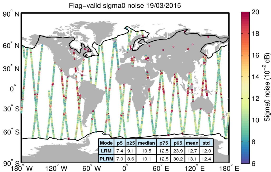
Figure 26. Geographical distribution of flag-valid 20-Hz sigma0 measurement noise over oceans and lakes for 19/03/2015. The statistical values shown in the table refer to the sigma0 noise and are calculated separately for LRM and PLRM regions. Measurements taken over polar polygons have been excluded from the computation of the statistical values. The black lines mark the outer limit of the Arctic and Antarctic polar polygons.
