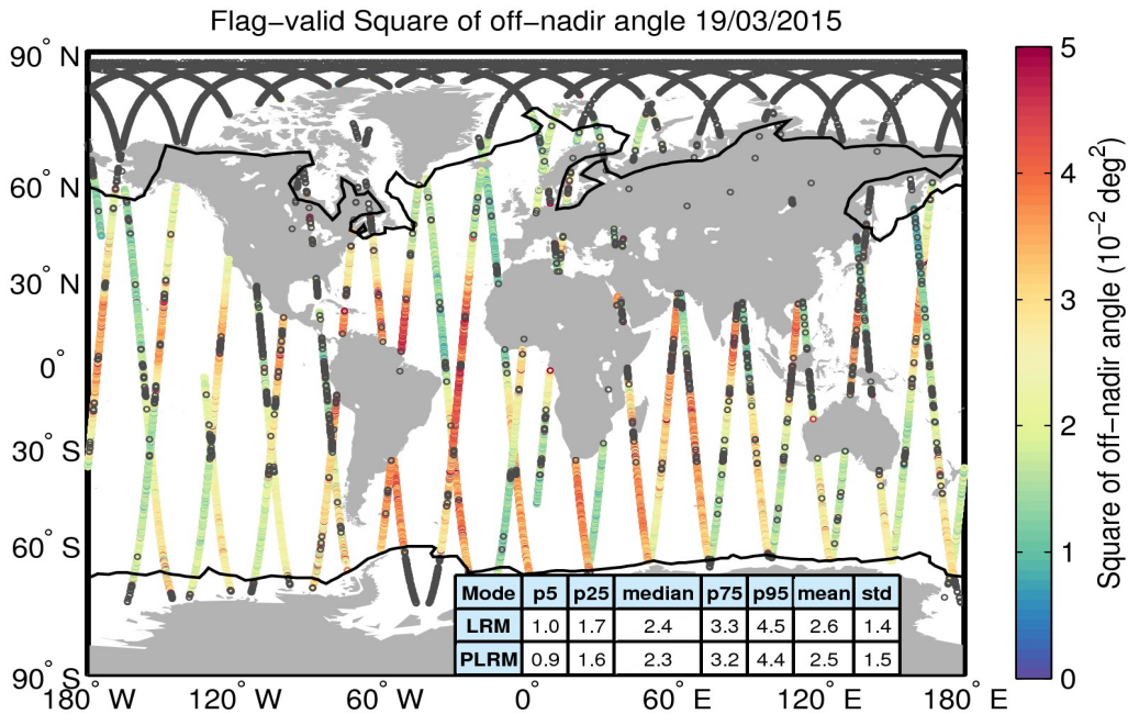
Figure 37. Geographical distribution of flag-valid mispointing data over oceans and lakes for 19/03/2015. The statistical values shown in the table refer to the mispointing in 10^{-2} \text{ deg}^2 and are calculated separately for LRM and PLRM regions. Measurements taken over polar polygons have been excluded from the computation of the statistical values. The black lines mark the outer limit of the Arctic and Antarctic polar polygons. Gray circles denote negative values.
