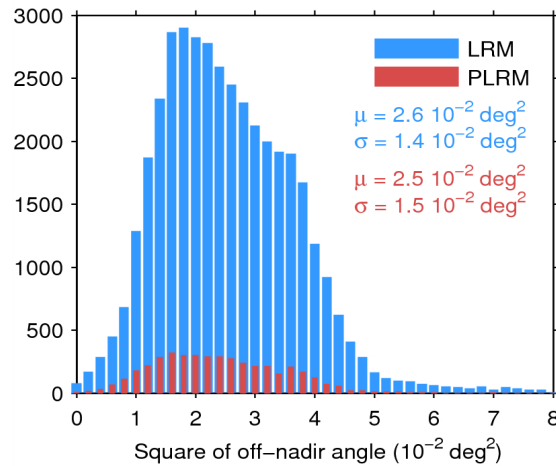
Figure 39. Histogram of flag-valid mispointing over oceans and lakes for LRM (blue) and PLRM (red) for 19/03/2015. Only positive values have been considered. The mean ( \mu ) and standard deviation ( \sigma ) are also shown. Note that values larger than 8 \cdot 10^{-2} \text{ deg}^2 are excluded from the histogram for the sake of readability but not from the computation of \mu and \sigma .
