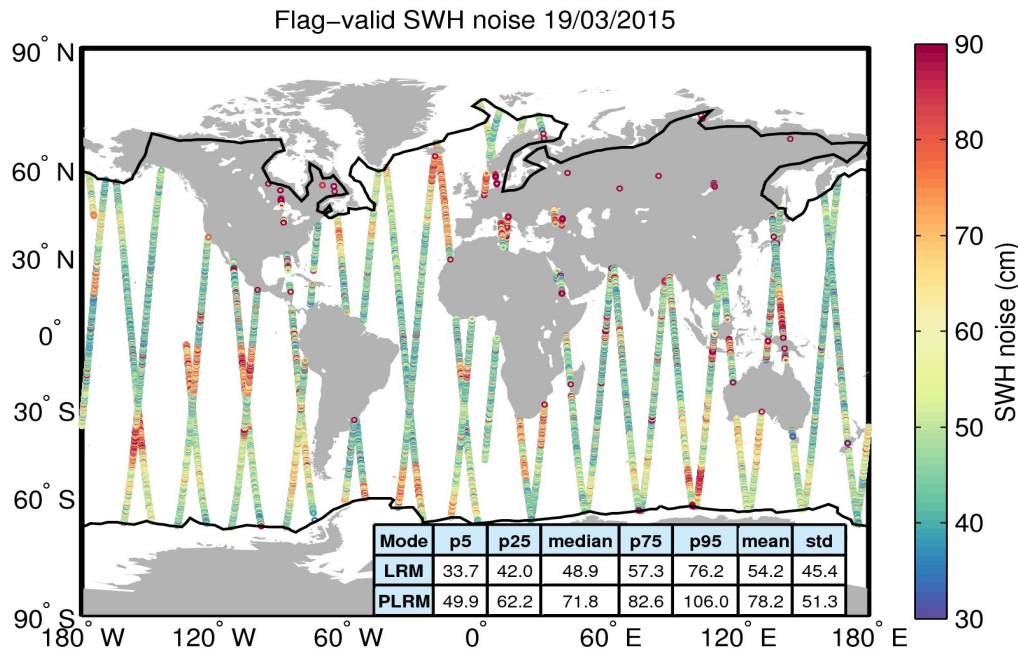
Figure 18. Geographical distribution of flag-valid 20-Hz SWH measurement noise over oceans and lakes for 19/03/2015. The statistical values shown in the table refer to the SWH noise and are calculated separately for LRM and PLRM regions. Measurements taken over polar polygons have been excluded from the computation of the statistical values. The black lines mark the outer limit of the Arctic and Antarctic polar polygons.
