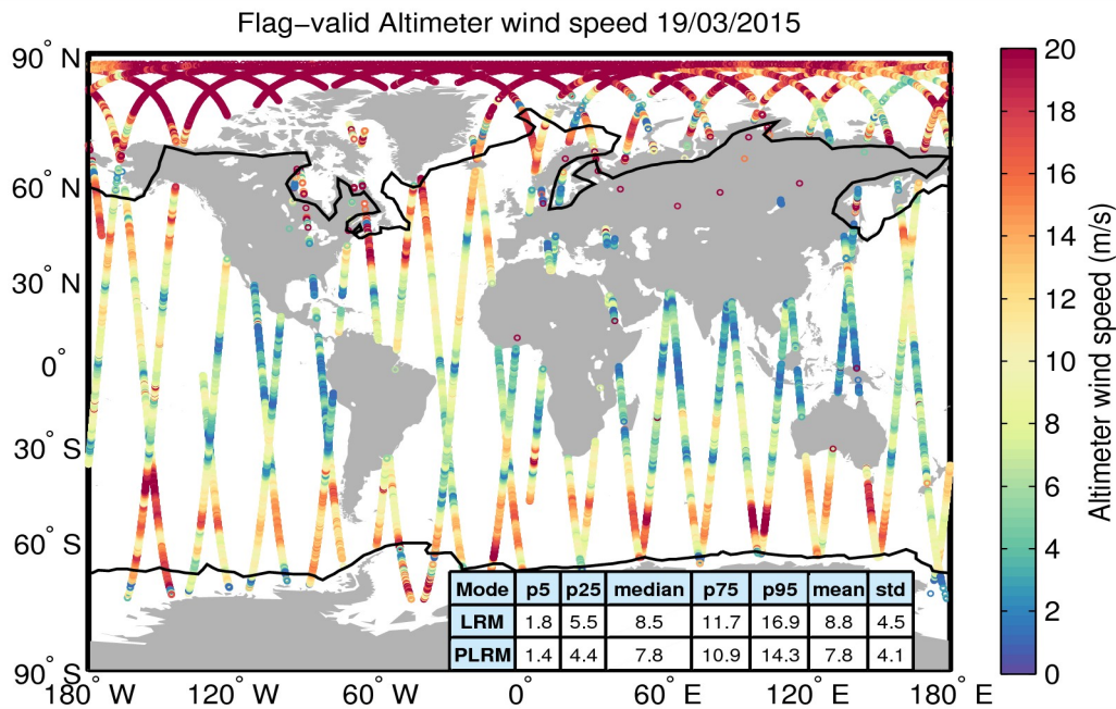
Figure 31. Geographical distribution of flag-valid wind data over oceans and lakes for 19/03/2015. The statistical values shown in the table refer to the wind in m/s and are calculated separately for LRM and PLRM regions. Measurements taken over polar polygons have been excluded from the computation of the statistical values. The black lines mark the outer limit of the Arctic and Antarctic polar polygons.
