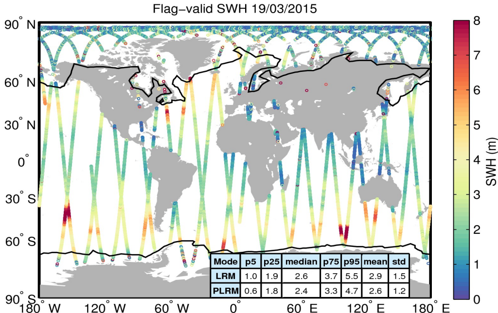
Figure 15. Geographical distribution of flag-valid SWH data over oceans and lakes for 19/03/2015. The statistical values shown in the table refer to the SWH in m and are calculated separately for LRM and PLRM regions. Measurements taken over polar polygons have been excluded from the computation of the statistical values. The black lines mark the outer limit of the Arctic and Antarctic polar polygons.
