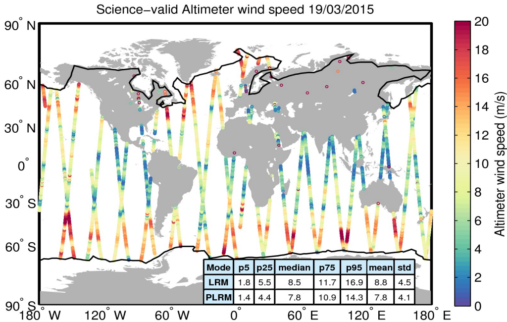
Figure 34. Geographical distribution of science-valid wind data over oceans and lakes for 19/03/2015. The statistical values shown in the table refer to the wind in m/s and are calculated separately for LRM and PLRM regions. The black lines mark the outer limit of the Arctic and Antarctic polar polygons. Gray circles denote records that have been rejected based on the editing criteria described in Table 5.
