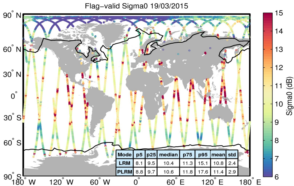
Figure 23. Geographical distribution of flag-valid sigma0 data over oceans and lakes for 19/03/2015. The statistical values shown in the table refer to the sigma0 in dB and are calculated separately for LRM and PLRM regions. Measurements taken over polar polygons have been excluded from the computation of the statistical values. The black lines mark the outer limit of the Arctic and Antarctic polar polygons.
