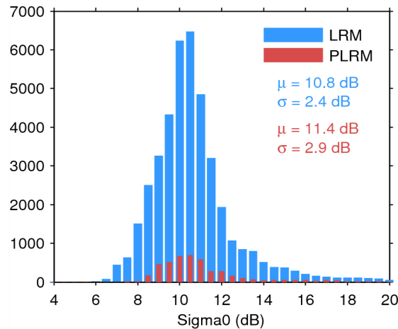
Figure 25. Histogram of flag-valid sigma0 over oceans and lakes for LRM (blue) and PLRM (red) for 19/03/2015. The mean ( \mu ) and standard deviation ( \sigma ) are also shown. Note that values outside [4 20] dB are excluded from the histogram for the sake of readability but not from the computation of \mu and \sigma .
