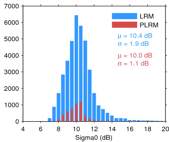
Figure 28. Histogram of science-valid sigma0 over oceans and lakes for LRM (blue) and PLRM (red) for 15/03/2015. The mean ( \mu ) and standard deviation ( \sigma ) are also shown. Note that values outside [4 20] dB are excluded from the histogram for the sake of readability but not from the computation of \mu and \sigma .
