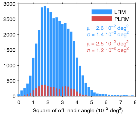
Figure 39. Histogram of flag-valid mispointing over oceans and lakes for LRM (blue) and PLRM (red) for 15/03/2015. Only positive values have been considered. The mean ( \mu ) and standard deviation ( \sigma ) are also shown. Note that values larger than 8 \cdot 10^{-2} \text{ deg}^2 are excluded from the histogram for the sake of readability but not from the computation of \mu and \sigma .
