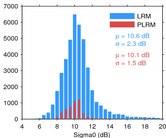
Figure 25. Histogram of flag-valid sigma0 over oceans and lakes for LRM (blue) and PLRM (red) for 15/03/2015. The mean ( \mu ) and standard deviation ( \sigma ) are also shown. Note that values outside [4 20] dB are excluded from the histogram for the sake of readability but not from the computation of \mu and \sigma .
