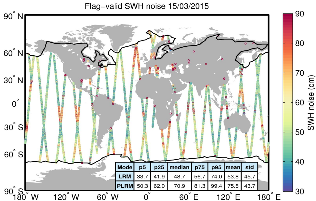
Figure 18. Geographical distribution of flag-valid 20-Hz SWH measurement noise over oceans and lakes for 15/03/2015. The statistical values shown in the table refer to the SWH noise and are calculated separately for LRM and PLRM regions. Measurements taken over polar polygons have been excluded from the computation of the statistical values. The black lines mark the outer limit of the Arctic and Antarctic polar polygons.
