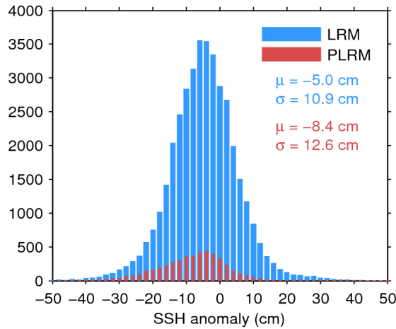
Figure 11. Histogram of science-valid SSH anomaly over oceans and lakes for LRM (blue) and PLRM (red) for 15/03/2015. The mean ( \mu ) and standard deviation ( \sigma ) are also shown. Note that values outside [-50\ 50] cm are excluded from the histogram for the sake of readability but not from the computation of \mu and \sigma .
