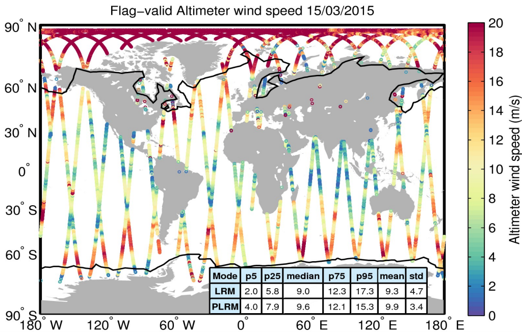
Figure 31. Geographical distribution of flag-valid wind data over oceans and lakes for 15/03/2015. The statistical values shown in the table refer to the wind in m/s and are calculated separately for LRM and PLRM regions. Measurements taken over polar polygons have been excluded from the computation of the statistical values. The black lines mark the outer limit of the Arctic and Antarctic polar polygons.
