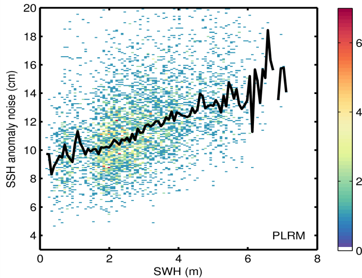
Figure 9. 2D histogram showing flag-valid SSH anomaly noise as a function of SWH for LRM (top) and PLRM (bottom) for 15/03/2015. The black line denotes the median SSH anomaly as a function of SWH.
