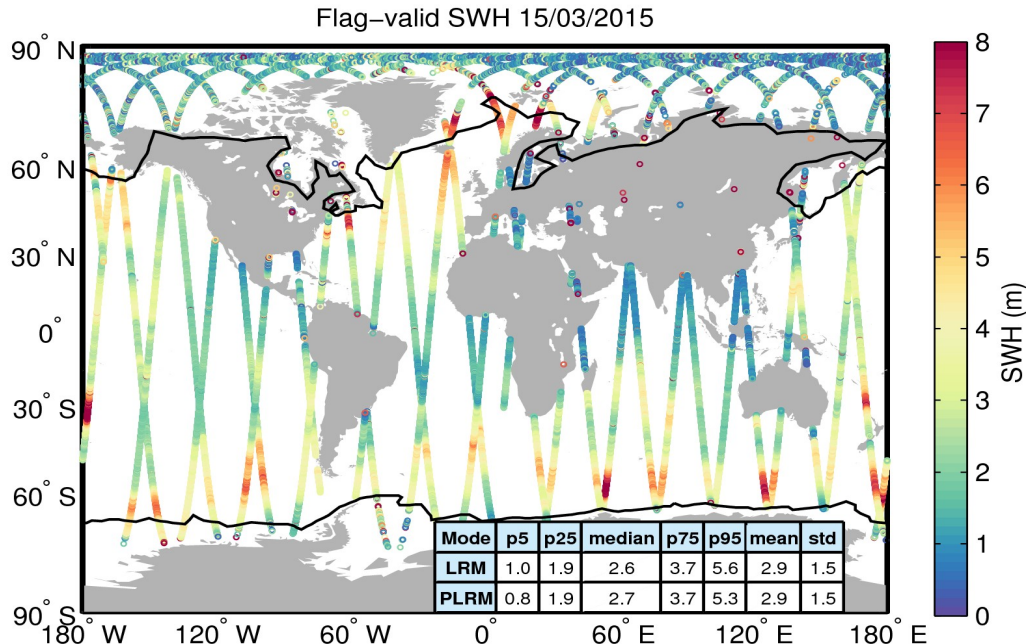
Figure 15. Geographical distribution of flag-valid SWH data over oceans and lakes for 15/03/2015. The statistical values shown in the table refer to the SWH in m and are calculated separately for LRM and PLRM regions. Measurements taken over polar polygons have been excluded from the computation of the statistical values. The black lines mark the outer limit of the Arctic and Antarctic polar polygons.
