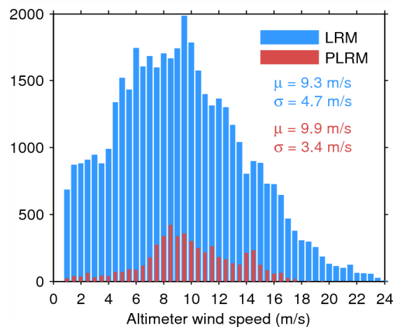
Figure 35. Histogram of science-valid wind over oceans and lakes for LRM (blue) and PLRM (red) for 15/03/2015. The mean ( \mu ) and standard deviation ( \sigma ) are also shown. Note that values larger than 24 m/s are excluded from the histogram for the sake of readability but not from the computation of \mu and \sigma .
