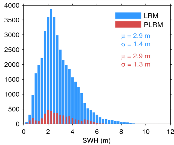
Figure 20. Histogram of science-valid SWH over oceans and lakes for LRM (blue) and PLRM (red) for 15/03/2015. The mean ( \mu ) and standard deviation ( \sigma ) are also shown. Note that values larger than 12 m are excluded from the histogram for the sake of readability but not from the computation of \mu and \sigma .
