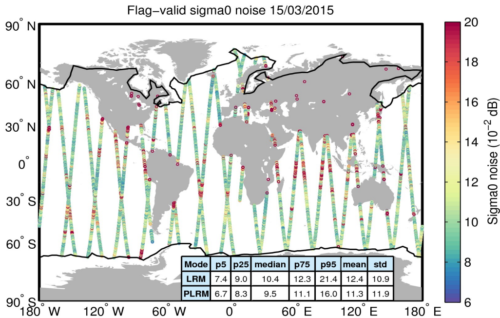
Figure 26. Geographical distribution of flag-valid 20-Hz sigma0 measurement noise over oceans and lakes for 15/03/2015. The statistical values shown in the table refer to the sigma0 noise and are calculated separately for LRM and PLRM regions. Measurements taken over polar polygons have been excluded from the computation of the statistical values. The black lines mark the outer limit of the Arctic and Antarctic polar polygons.
