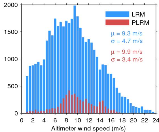
Figure 33. Histogram of flag-valid wind over oceans and lakes for LRM (blue) and PLRM (red) for 15/03/2015. The mean ( \mu ) and standard deviation ( \sigma ) are also shown. Note that values larger than 24 m/s are excluded from the histogram for the sake of readability but not from the computation of \mu and \sigma .
