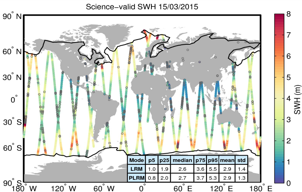
Figure 19. Geographical distribution of science-valid SWH data over oceans and lakes for 15/03/2015. The statistical values shown in the table refer to the SWH in m and are calculated separately for LRM and PLRM regions. The black lines mark the outer limit of the Arctic and Antarctic polar polygons. Gray circles denote records that have been rejected based on the editing criteria described in Table 3.
