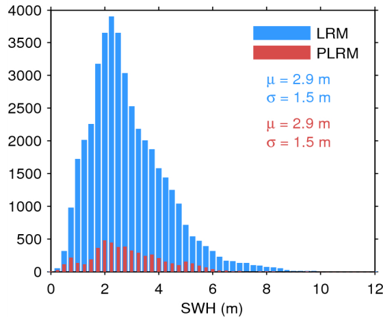
Figure 17. Histogram of flag-valid SWH over oceans and lakes for LRM (blue) and PLRM (red) for 15/03/2015. The mean ( \mu ) and standard deviation ( \sigma ) are also shown. Note that values larger than 12 m are excluded from the histogram for the sake of readability but not from the computation of \mu and \sigma .
