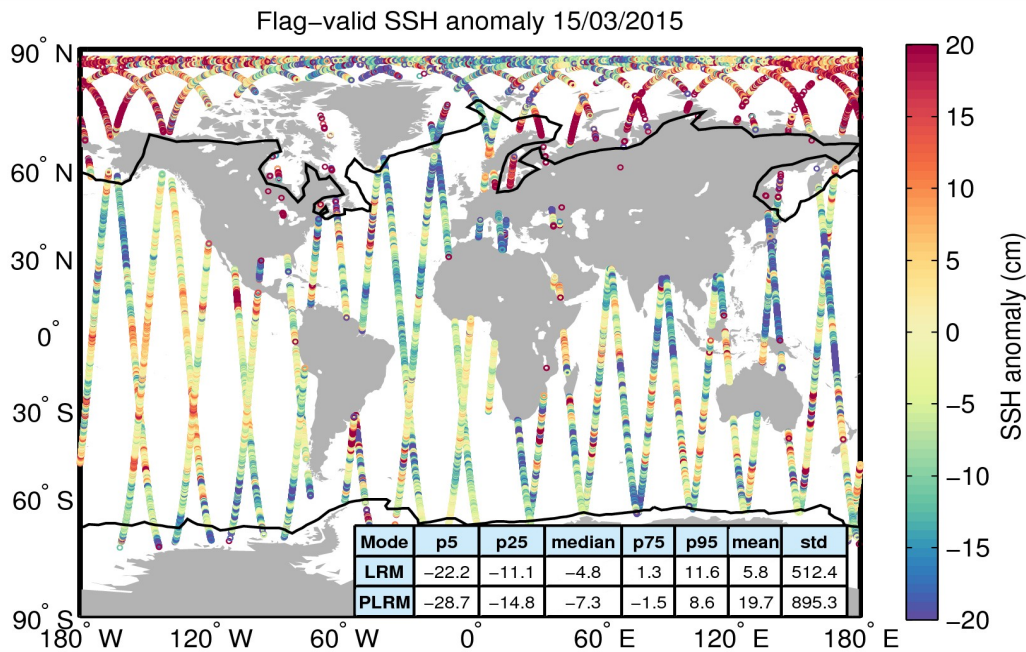
Figure 5. Geographical distribution of flag-valid 1-Hz SSH anomaly data over oceans and lakes for 15/03/2015. The statistical values shown in the table refer to the SSH anomaly in cm and are calculated separately for LRM and PLRM regions. Measurements taken over polar polygons have been excluded from the computation of the statistical values. The black lines mark the outer limit of the Arctic and Antarctic polar polygons.
