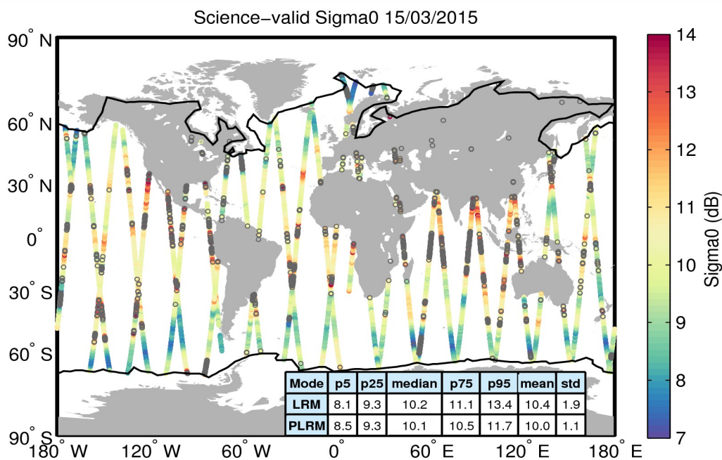
Figure 27. Geographical distribution of science-valid sigma0 data over oceans and lakes for 15/03/2015. The statistical values shown in the table refer to the sigma0 in dB and are calculated separately for LRM and PLRM regions. The black lines mark the outer limit of the Arctic and Antarctic polar polygons. Gray circles denote records that have been rejected based on the editing criteria described in Table 4.
