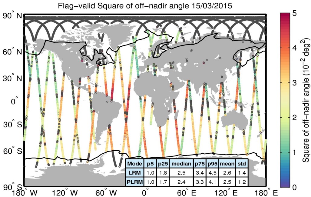
Figure 37. Geographical distribution of flag-valid mispointing data over oceans and lakes for 15/03/2015. The statistical values shown in the table refer to the mispointing in 10^{-2} \text{ deg}^2 and are calculated separately for LRM and PLRM regions. Measurements taken over polar polygons have been excluded from the computation of the statistical values. The black lines mark the outer limit of the Arctic and Antarctic polar polygons. Gray circles denote negative values.
