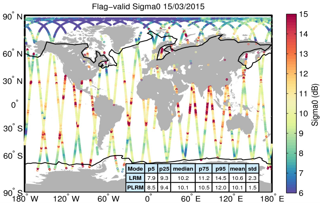
Figure 23. Geographical distribution of flag-valid sigma0 data over oceans and lakes for 15/03/2015. The statistical values shown in the table refer to the sigma0 in dB and are calculated separately for LRM and PLRM regions. Measurements taken over polar polygons have been excluded from the computation of the statistical values. The black lines mark the outer limit of the Arctic and Antarctic polar polygons.
