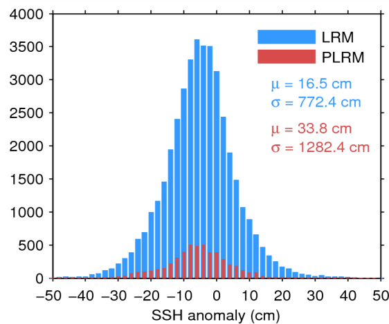
Figure 7. Histogram of flag-valid SSH anomaly over oceans and lakes for LRM (blue) and PLRM (red) for 14/03/2015. The mean ( \mu ) and standard deviation ( \sigma ) are also shown. Note that values outside [-50\ 50] cm are excluded from the histogram for the sake of readability but not from the computation of \mu and \sigma .
