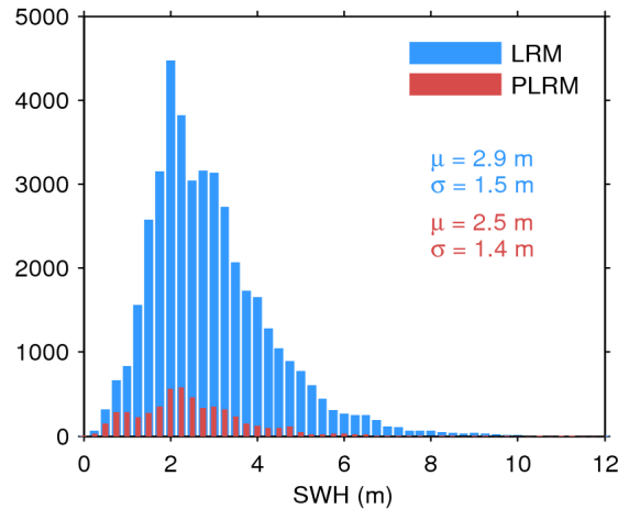
Figure 17. Histogram of flag-valid SWH over oceans and lakes for LRM (blue) and PLRM (red) for 14/03/2015. The mean ( \mu ) and standard deviation ( \sigma ) are also shown. Note that values larger than 12 m are excluded from the histogram for the sake of readability but not from the computation of \mu and \sigma .
