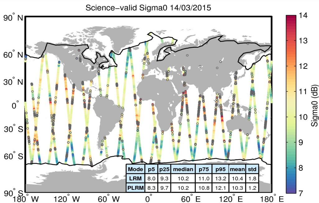
Figure 27. Geographical distribution of science-valid sigma0 data over oceans and lakes for 14/03/2015. The statistical values shown in the table refer to the sigma0 in dB and are calculated separately for LRM and PLRM regions. The black lines mark the outer limit of the Arctic and Antarctic polar polygons. Gray circles denote records that have been rejected based on the editing criteria described in Table 4.
