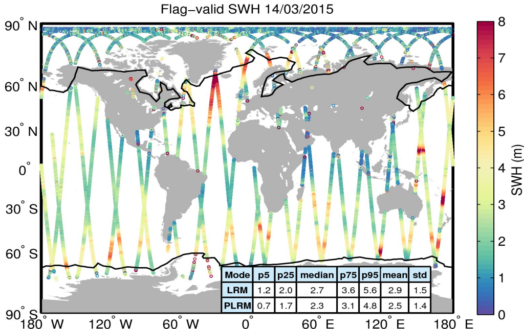
Figure 15. Geographical distribution of flag-valid SWH data over oceans and lakes for 14/03/2015. The statistical values shown in the table refer to the SWH in m and are calculated separately for LRM and PLRM regions. Measurements taken over polar polygons have been excluded from the computation of the statistical values. The black lines mark the outer limit of the Arctic and Antarctic polar polygons.
