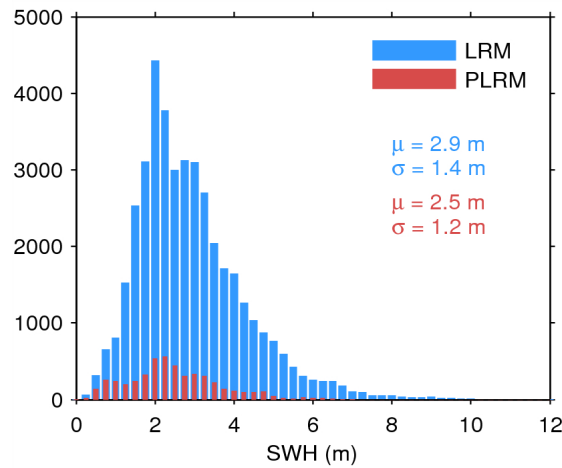
Figure 20. Histogram of science-valid SWH over oceans and lakes for LRM (blue) and PLRM (red) for 14/03/2015. The mean ( \mu ) and standard deviation ( \sigma ) are also shown. Note that values larger than 12 m are excluded from the histogram for the sake of readability but not from the computation of \mu and \sigma .
