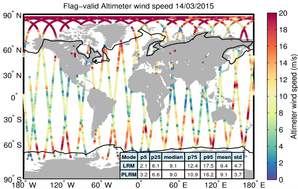
Figure 31. Geographical distribution of flag-valid wind data over oceans and lakes for 14/03/2015. The statistical values shown in the table refer to the wind in m/s and are calculated separately for LRM and PLRM regions. Measurements taken over polar polygons have been excluded from the computation of the statistical values. The black lines mark the outer limit of the Arctic and Antarctic polar polygons.
