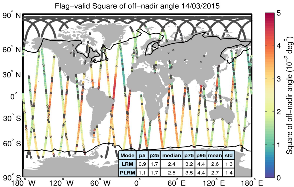
Figure 37. Geographical distribution of flag-valid mispointing data over oceans and lakes for 14/03/2015. The statistical values shown in the table refer to the mispointing in 10^{-2} \text{ deg}^2 and are calculated separately for LRM and PLRM regions. Measurements taken over polar polygons have been excluded from the computation of the statistical values. The black lines mark the outer limit of the Arctic and Antarctic polar polygons. Gray circles denote negative values.
