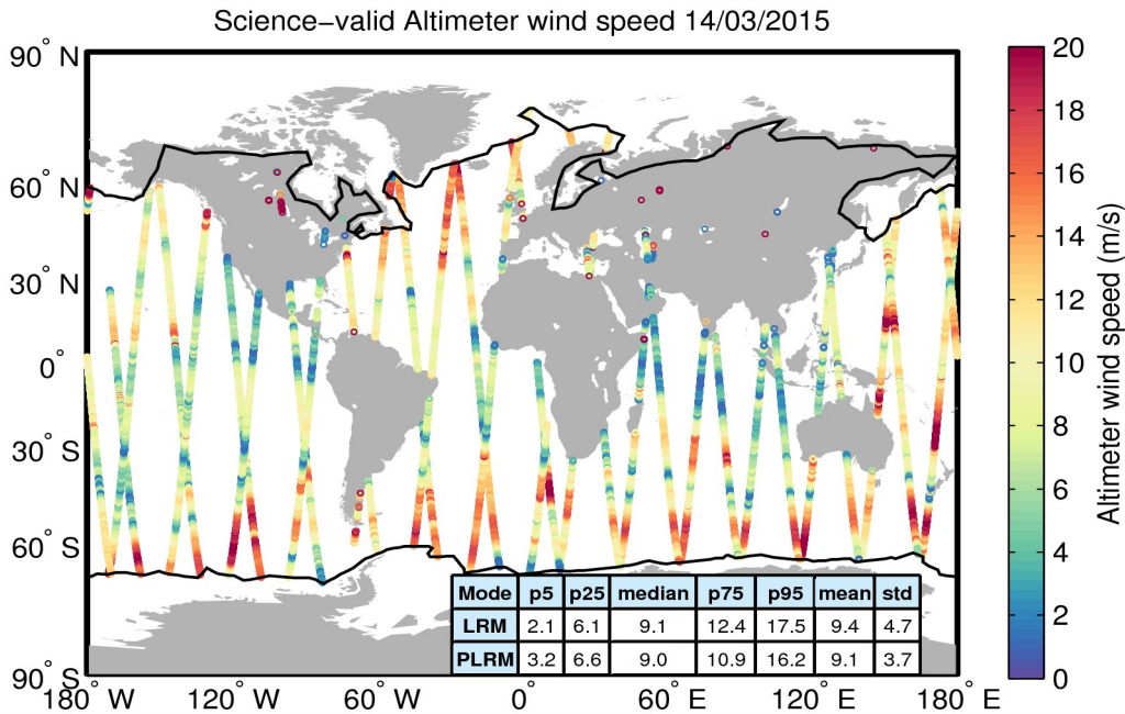
Figure 34. Geographical distribution of science-valid wind data over oceans and lakes for 14/03/2015. The statistical values shown in the table refer to the wind in m/s and are calculated separately for LRM and PLRM regions. The black lines mark the outer limit of the Arctic and Antarctic polar polygons. Gray circles denote records that have been rejected based on the editing criteria described in Table 5.
