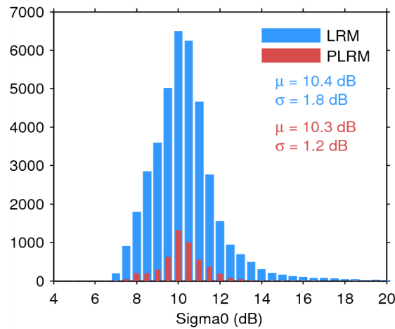
Figure 28. Histogram of science-valid sigma0 over oceans and lakes for LRM (blue) and PLRM (red) for 14/03/2015. The mean ( \mu ) and standard deviation ( \sigma ) are also shown. Note that values outside [4 20] dB are excluded from the histogram for the sake of readability but not from the computation of \mu and \sigma .
