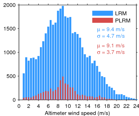
Figure 35. Histogram of science-valid wind over oceans and lakes for LRM (blue) and PLRM (red) for 14/03/2015. The mean ( \mu ) and standard deviation ( \sigma ) are also shown. Note that values larger than 24 m/s are excluded from the histogram for the sake of readability but not from the computation of \mu and \sigma .
