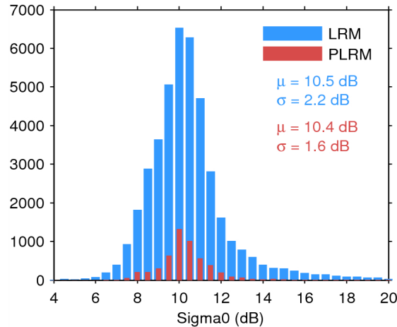
Figure 25. Histogram of flag-valid sigma0 over oceans and lakes for LRM (blue) and PLRM (red) for 14/03/2015. The mean ( \mu ) and standard deviation ( \sigma ) are also shown. Note that values outside [4 20] dB are excluded from the histogram for the sake of readability but not from the computation of \mu and \sigma .
