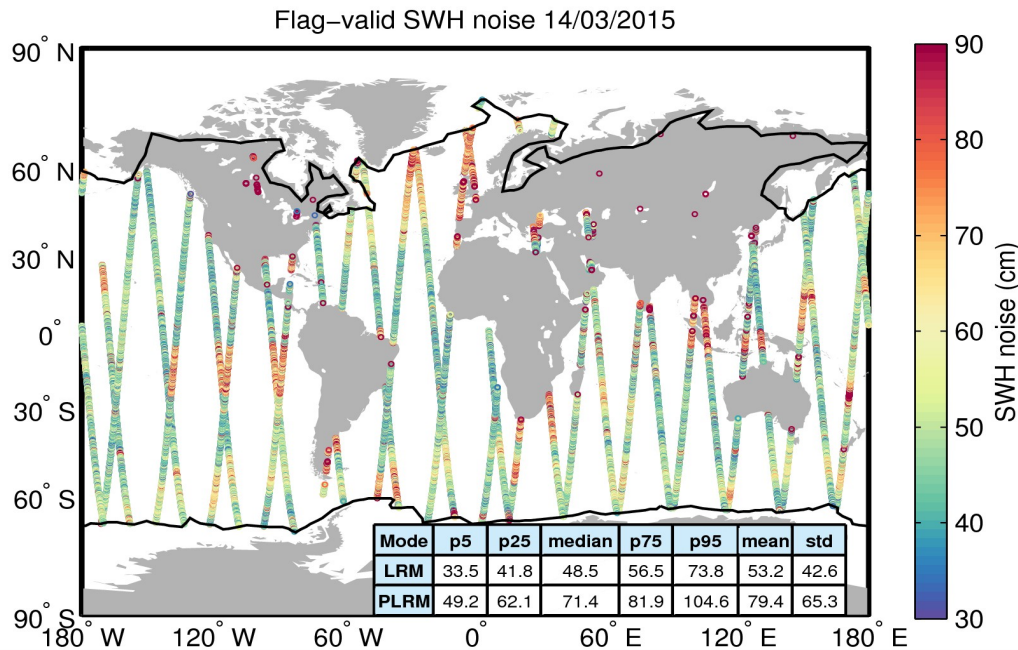
Figure 18. Geographical distribution of flag-valid 20-Hz SWH measurement noise over oceans and lakes for 14/03/2015. The statistical values shown in the table refer to the SWH noise and are calculated separately for LRM and PLRM regions. Measurements taken over polar polygons have been excluded from the computation of the statistical values. The black lines mark the outer limit of the Arctic and Antarctic polar polygons.
