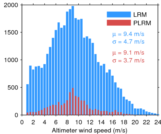
Figure 33. Histogram of flag-valid wind over oceans and lakes for LRM (blue) and PLRM (red) for 14/03/2015. The mean ( \mu ) and standard deviation ( \sigma ) are also shown. Note that values larger than 24 m/s are excluded from the histogram for the sake of readability but not from the computation of \mu and \sigma .
