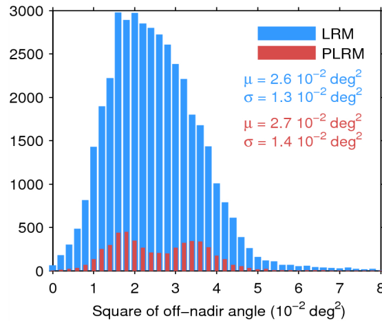
Figure 39. Histogram of flag-valid mispointing over oceans and lakes for LRM (blue) and PLRM (red) for 14/03/2015. Only positive values have been considered. The mean ( \mu ) and standard deviation ( \sigma ) are also shown. Note that values larger than 8 \cdot 10^{-2} \text{ deg}^2 are excluded from the histogram for the sake of readability but not from the computation of \mu and \sigma .
