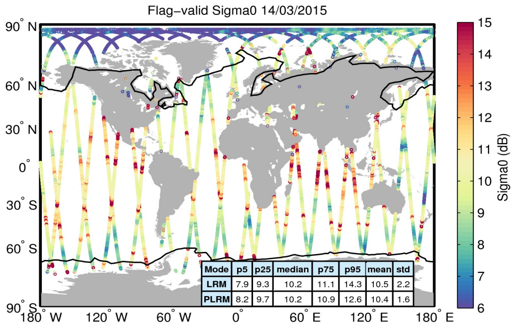
Figure 23. Geographical distribution of flag-valid sigma0 data over oceans and lakes for 14/03/2015. The statistical values shown in the table refer to the sigma0 in dB and are calculated separately for LRM and PLRM regions. Measurements taken over polar polygons have been excluded from the computation of the statistical values. The black lines mark the outer limit of the Arctic and Antarctic polar polygons.
