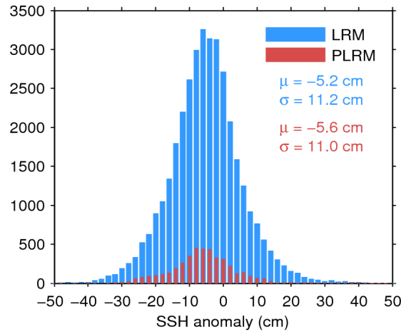
Figure 11. Histogram of science-valid SSH anomaly over oceans and lakes for LRM (blue) and PLRM (red) for 14/03/2015. The mean ( \mu ) and standard deviation ( \sigma ) are also shown. Note that values outside [-50 50] cm are excluded from the histogram for the sake of readability but not from the computation of \mu and \sigma .
