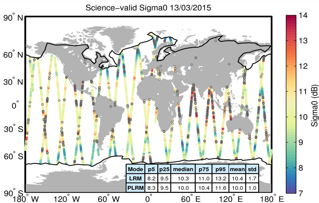
Figure 27. Geographical distribution of science-valid sigma0 data over oceans and lakes for 13/03/2015. The statistical values shown in the table refer to the sigma0 in dB and are calculated separately for LRM and PLRM regions. The black lines mark the outer limit of the Arctic and Antarctic polar polygons. Gray circles denote records that have been rejected based on the editing criteria described in Table 4.
