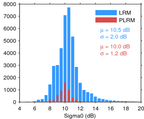
Figure 25. Histogram of flag-valid sigma0 over oceans and lakes for LRM (blue) and PLRM (red) for 13/03/2015. The mean ( \mu ) and standard deviation ( \sigma ) are also shown. Note that values outside [4 20] dB are excluded from the histogram for the sake of readability but not from the computation of \mu and \sigma .
