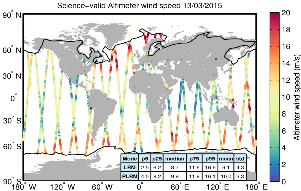
Figure 34. Geographical distribution of science-valid wind data over oceans and lakes for 13/03/2015. The statistical values shown in the table refer to the wind in m/s and are calculated separately for LRM and PLRM regions. The black lines mark the outer limit of the Arctic and Antarctic polar polygons. Gray circles denote records that have been rejected based on the editing criteria described in Table 5.
