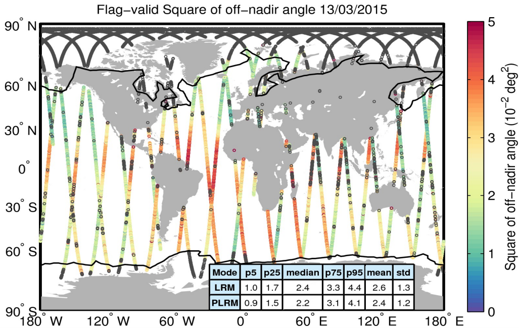
Figure 37. Geographical distribution of flag-valid mispointing data over oceans and lakes for 13/03/2015. The statistical values shown in the table refer to the mispointing in 10^{-2} \text{ deg}^2 and are calculated separately for LRM and PLRM regions. Measurements taken over polar polygons have been excluded from the computation of the statistical values. The black lines mark the outer limit of the Arctic and Antarctic polar polygons. Gray circles denote negative values.
