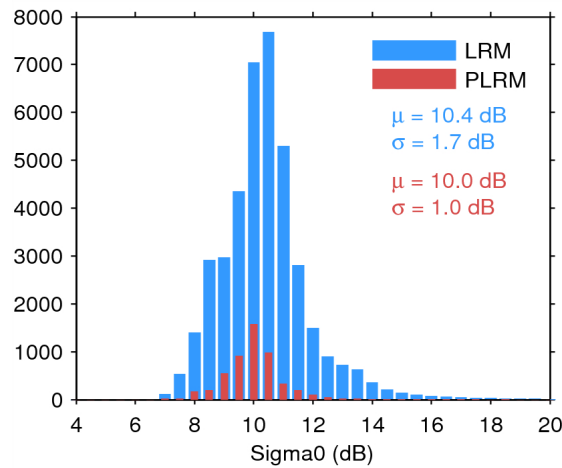
Figure 28. Histogram of science-valid sigma0 over oceans and lakes for LRM (blue) and PLRM (red) for 13/03/2015. The mean ( \mu ) and standard deviation ( \sigma ) are also shown. Note that values outside [4 20] dB are excluded from the histogram for the sake of readability but not from the computation of \mu and \sigma .
