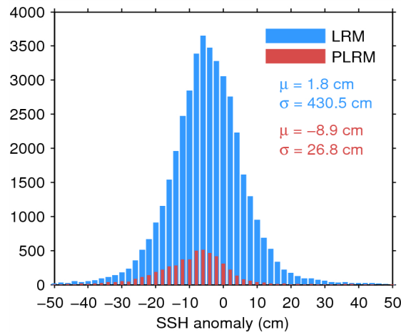
Figure 7. Histogram of flag-valid SSH anomaly over oceans and lakes for LRM (blue) and PLRM (red) for 13/03/2015. The mean ( \mu ) and standard deviation ( \sigma ) are also shown. Note that values outside [-50\ 50] cm are excluded from the histogram for the sake of readability but not from the computation of \mu and \sigma .
