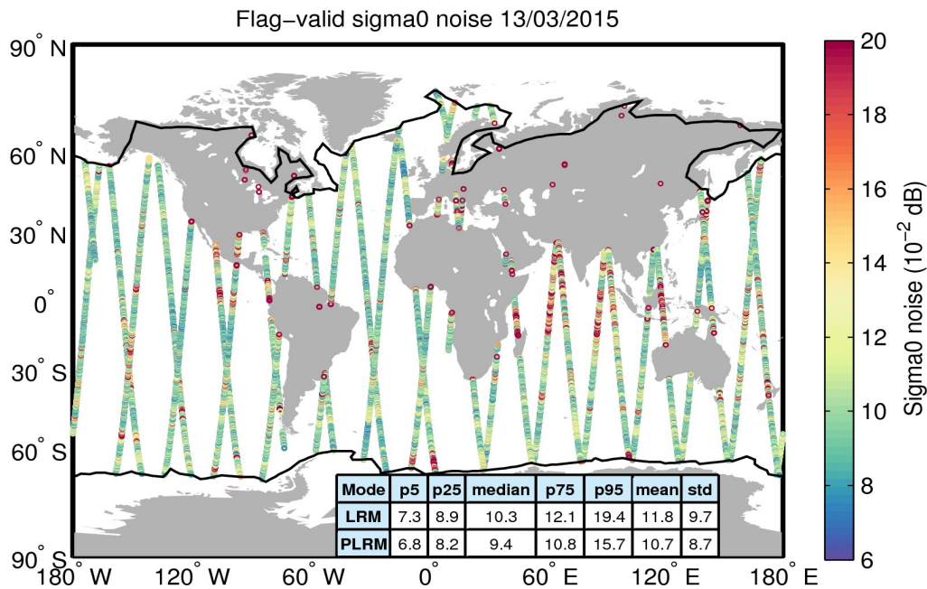
Figure 26. Geographical distribution of flag-valid 20-Hz sigma0 measurement noise over oceans and lakes for 13/03/2015. The statistical values shown in the table refer to the sigma0 noise and are calculated separately for LRM and PLRM regions. Measurements taken over polar polygons have been excluded from the computation of the statistical values. The black lines mark the outer limit of the Arctic and Antarctic polar polygons.
