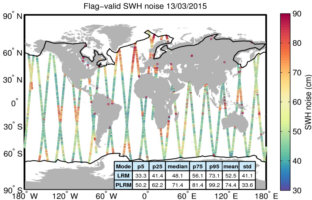
Figure 18. Geographical distribution of flag-valid 20-Hz SWH measurement noise over oceans and lakes for 13/03/2015. The statistical values shown in the table refer to the SWH noise and are calculated separately for LRM and PLRM regions. Measurements taken over polar polygons have been excluded from the computation of the statistical values. The black lines mark the outer limit of the Arctic and Antarctic polar polygons.
