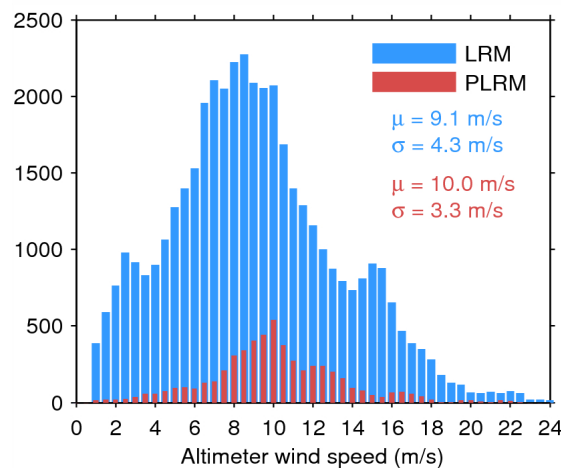
Figure 35. Histogram of science-valid wind over oceans and lakes for LRM (blue) and PLRM (red) for 13/03/2015. The mean ( \mu ) and standard deviation ( \sigma ) are also shown. Note that values larger than 24 m/s are excluded from the histogram for the sake of readability but not from the computation of \mu and \sigma .
