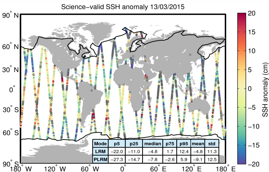
Figure 10. Geographical distribution of science-valid SSH anomaly data over oceans and lakes for 13/03/2015. The statistical values shown in the table refer to the SSH anomaly in cm and are calculated separately for LRM and PLRM regions. The black lines mark the outer limit of the Arctic and Antarctic polar polygons. Gray circles denote records that have been rejected based on the editing criteria described in Table 2.
