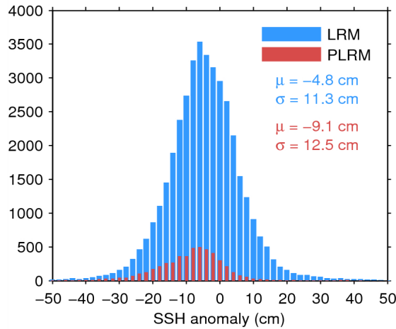
Figure 11. Histogram of science-valid SSH anomaly over oceans and lakes for LRM (blue) and PLRM (red) for 13/03/2015. The mean ( \mu ) and standard deviation ( \sigma ) are also shown. Note that values outside [-50 50] cm are excluded from the histogram for the sake of readability but not from the computation of \mu and \sigma .
