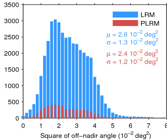
Figure 39. Histogram of flag-valid mispointing over oceans and lakes for LRM (blue) and PLRM (red) for 13/03/2015. Only positive values have been considered. The mean ( \mu ) and standard deviation ( \sigma ) are also shown. Note that values larger than 8 \cdot 10^{-2} \text{ deg}^2 are excluded from the histogram for the sake of readability but not from the computation of \mu and \sigma .
