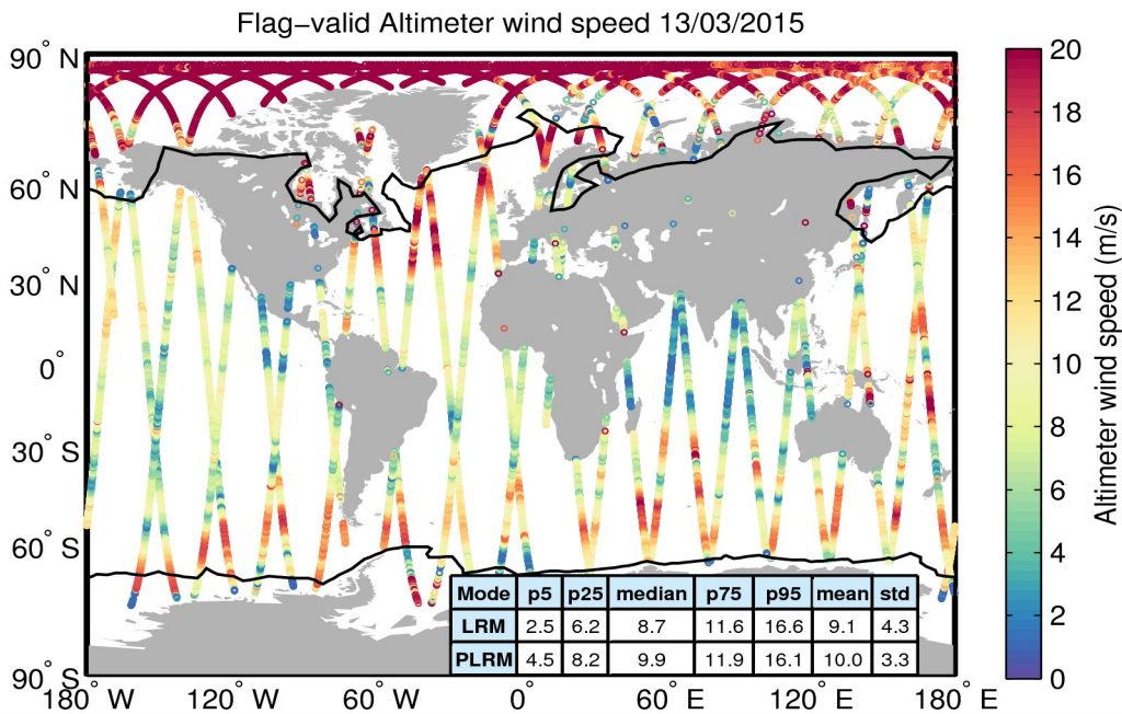
Figure 31. Geographical distribution of flag-valid wind data over oceans and lakes for 13/03/2015. The statistical values shown in the table refer to the wind in m/s and are calculated separately for LRM and PLRM regions. Measurements taken over polar polygons have been excluded from the computation of the statistical values. The black lines mark the outer limit of the Arctic and Antarctic polar polygons.
