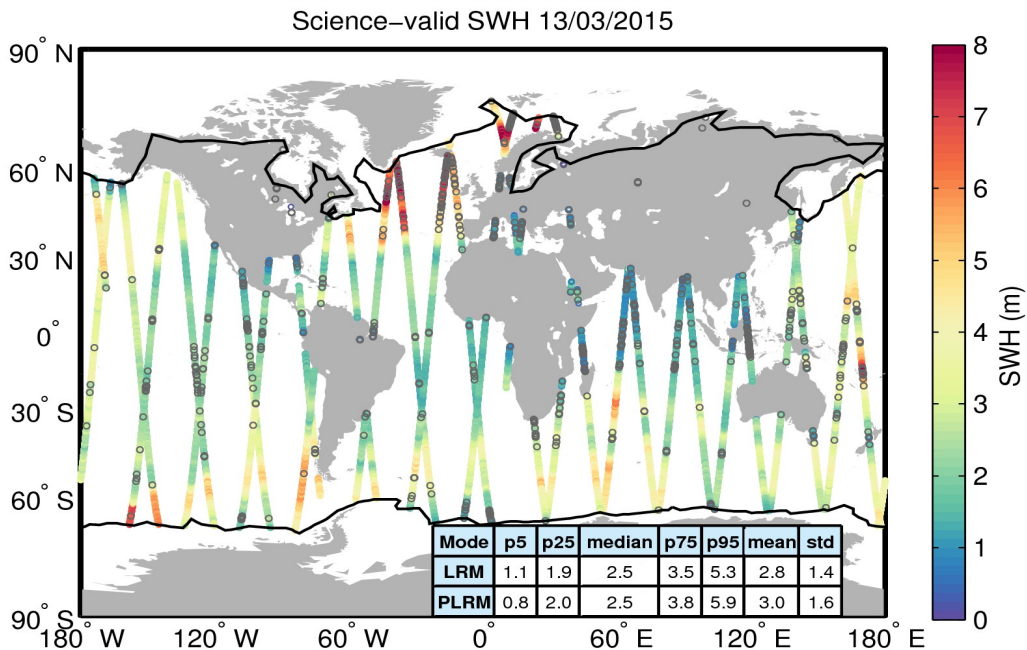
Figure 19. Geographical distribution of science-valid SWH data over oceans and lakes for 13/03/2015. The statistical values shown in the table refer to the SWH in m and are calculated separately for LRM and PLRM regions. The black lines mark the outer limit of the Arctic and Antarctic polar polygons. Gray circles denote records that have been rejected based on the editing criteria described in Table 3.
