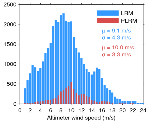
Figure 33. Histogram of flag-valid wind over oceans and lakes for LRM (blue) and PLRM (red) for 13/03/2015. The mean ( \mu ) and standard deviation ( \sigma ) are also shown. Note that values larger than 24 m/s are excluded from the histogram for the sake of readability but not from the computation of \mu and \sigma .
