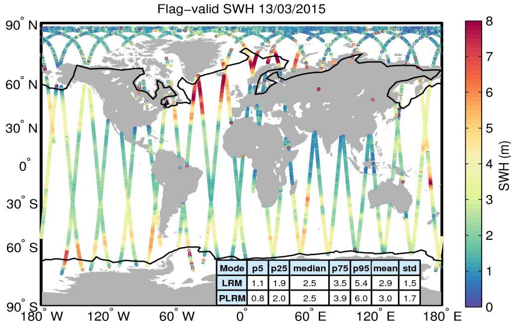
Figure 15. Geographical distribution of flag-valid SWH data over oceans and lakes for 13/03/2015. The statistical values shown in the table refer to the SWH in m and are calculated separately for LRM and PLRM regions. Measurements taken over polar polygons have been excluded from the computation of the statistical values. The black lines mark the outer limit of the Arctic and Antarctic polar polygons.
