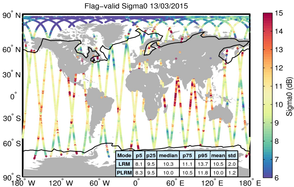
Figure 23. Geographical distribution of flag-valid sigma0 data over oceans and lakes for 13/03/2015. The statistical values shown in the table refer to the sigma0 in dB and are calculated separately for LRM and PLRM regions. Measurements taken over polar polygons have been excluded from the computation of the statistical values. The black lines mark the outer limit of the Arctic and Antarctic polar polygons.
