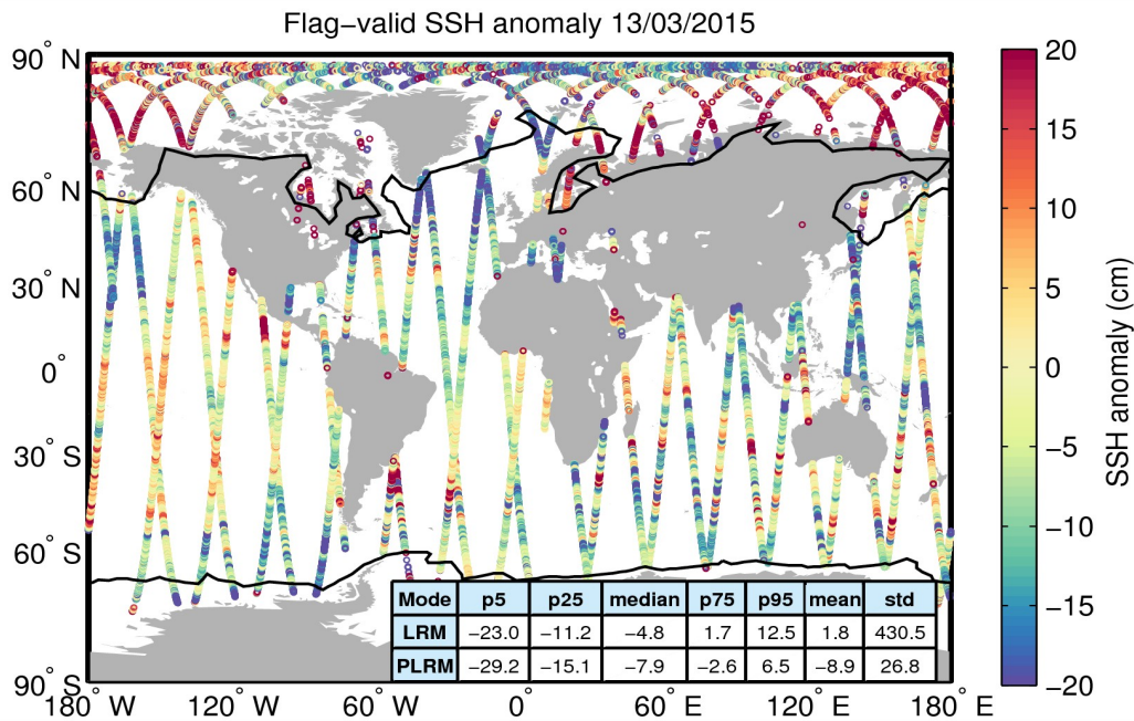
Figure 5. Geographical distribution of flag-valid 1-Hz SSH anomaly data over oceans and lakes for 13/03/2015. The statistical values shown in the table refer to the SSH anomaly in cm and are calculated separately for LRM and PLRM regions. Measurements taken over polar polygons have been excluded from the computation of the statistical values. The black lines mark the outer limit of the Arctic and Antarctic polar polygons.
