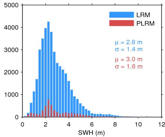
Figure 20. Histogram of science-valid SWH over oceans and lakes for LRM (blue) and PLRM (red) for 13/03/2015. The mean ( \mu ) and standard deviation ( \sigma ) are also shown. Note that values larger than 12 m are excluded from the histogram for the sake of readability but not from the computation of \mu and \sigma .
