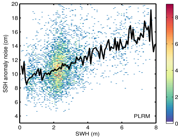
Figure 9. 2D histogram showing flag-valid SSH anomaly noise as a function of SWH for LRM (top) and PLRM (bottom) for 11/03/2015. The black line denotes the median SSH anomaly as a function of SWH.
