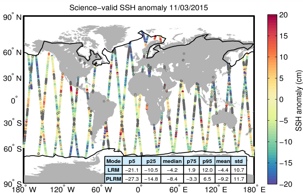
Figure 10. Geographical distribution of science-valid SSH anomaly data over oceans and lakes for 11/03/2015. The statistical values shown in the table refer to the SSH anomaly in cm and are calculated separately for LRM and PLRM regions. The black lines mark the outer limit of the Arctic and Antarctic polar polygons. Gray circles denote records that have been rejected based on the editing criteria described in Table 2.
