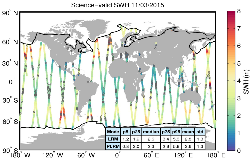
Figure 19. Geographical distribution of science-valid SWH data over oceans and lakes for 11/03/2015. The statistical values shown in the table refer to the SWH in m and are calculated separately for LRM and PLRM regions. The black lines mark the outer limit of the Arctic and Antarctic polar polygons. Gray circles denote records that have been rejected based on the editing criteria described in Table 3.
