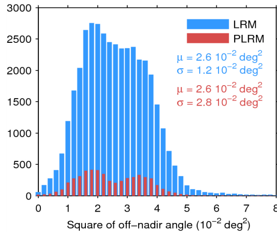
Figure 39. Histogram of flag-valid mispointing over oceans and lakes for LRM (blue) and PLRM (red) for 11/03/2015. Only positive values have been considered. The mean ( \mu ) and standard deviation ( \sigma ) are also shown. Note that values larger than 8 \cdot 10^{-2} \text{ deg}^2 are excluded from the histogram for the sake of readability but not from the computation of \mu and \sigma .
