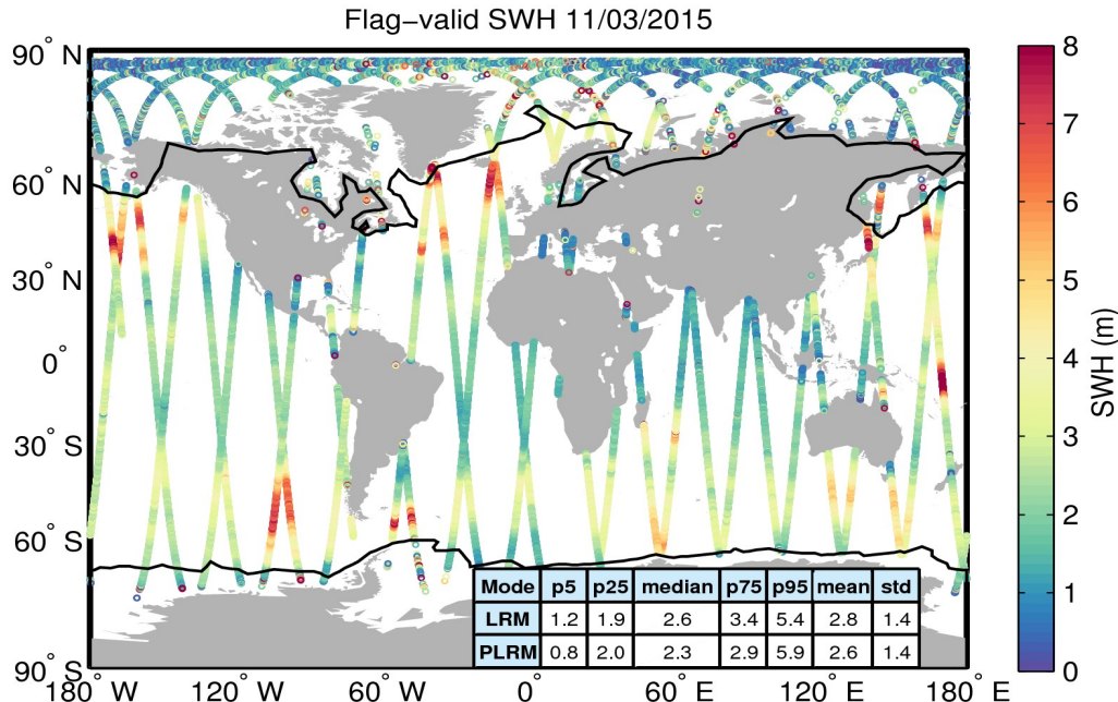
Figure 15. Geographical distribution of flag-valid SWH data over oceans and lakes for 11/03/2015. The statistical values shown in the table refer to the SWH in m and are calculated separately for LRM and PLRM regions. Measurements taken over polar polygons have been excluded from the computation of the statistical values. The black lines mark the outer limit of the Arctic and Antarctic polar polygons.
