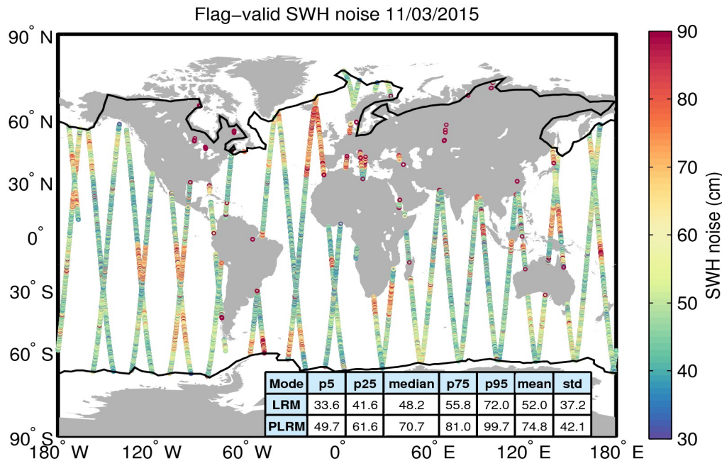
Figure 18. Geographical distribution of flag-valid 20-Hz SWH measurement noise over oceans and lakes for 11/03/2015. The statistical values shown in the table refer to the SWH noise and are calculated separately for LRM and PLRM regions. Measurements taken over polar polygons have been excluded from the computation of the statistical values. The black lines mark the outer limit of the Arctic and Antarctic polar polygons.
