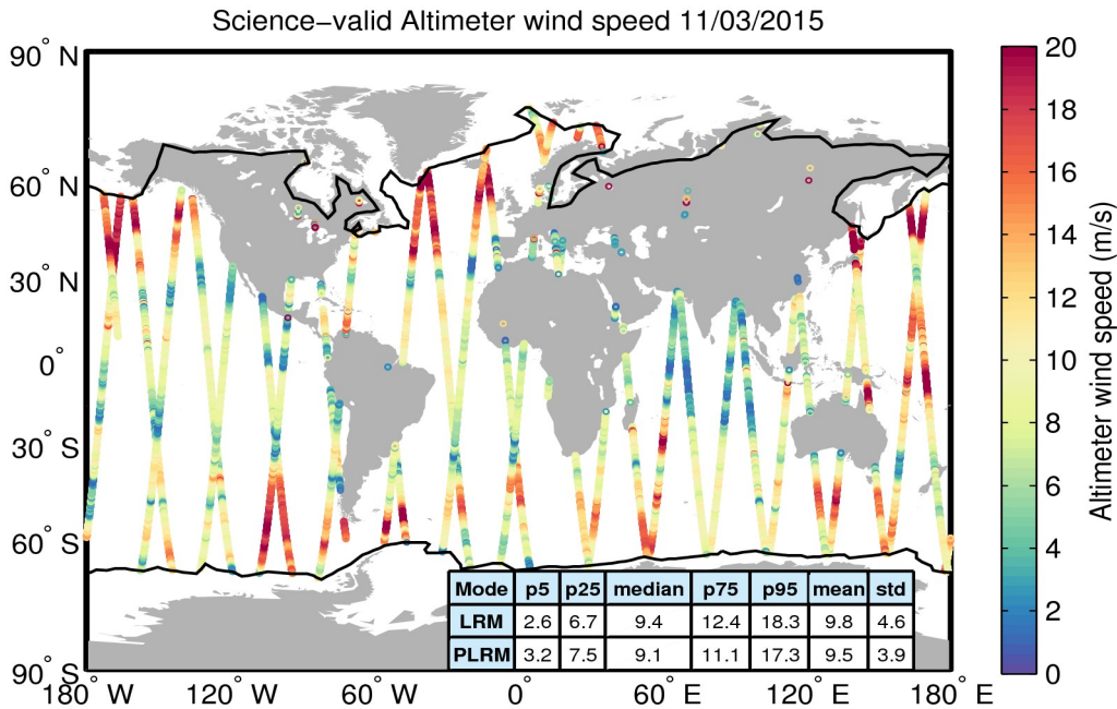
Figure 34. Geographical distribution of science-valid wind data over oceans and lakes for 11/03/2015. The statistical values shown in the table refer to the wind in m/s and are calculated separately for LRM and PLRM regions. The black lines mark the outer limit of the Arctic and Antarctic polar polygons. Gray circles denote records that have been rejected based on the editing criteria described in Table 5.
