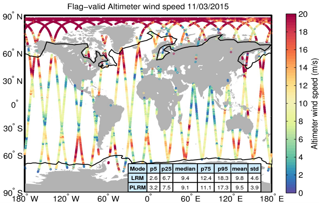
Figure 31. Geographical distribution of flag-valid wind data over oceans and lakes for 11/03/2015. The statistical values shown in the table refer to the wind in m/s and are calculated separately for LRM and PLRM regions. Measurements taken over polar polygons have been excluded from the computation of the statistical values. The black lines mark the outer limit of the Arctic and Antarctic polar polygons.
