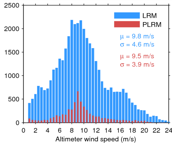
Figure 33. Histogram of flag-valid wind over oceans and lakes for LRM (blue) and PLRM (red) for 11/03/2015. The mean ( \mu ) and standard deviation ( \sigma ) are also shown. Note that values larger than 24 m/s are excluded from the histogram for the sake of readability but not from the computation of \mu and \sigma .
