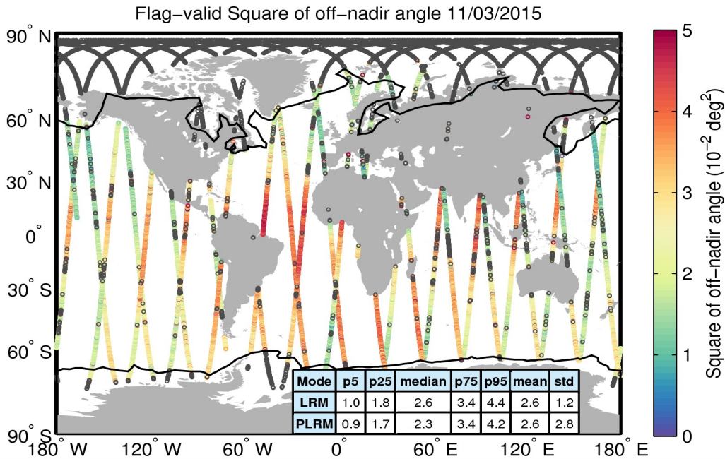
Figure 37. Geographical distribution of flag-valid mispointing data over oceans and lakes for 11/03/2015. The statistical values shown in the table refer to the mispointing in 10^{-2} \text{ deg}^2 and are calculated separately for LRM and PLRM regions. Measurements taken over polar polygons have been excluded from the computation of the statistical values. The black lines mark the outer limit of the Arctic and Antarctic polar polygons. Gray circles denote negative values.
