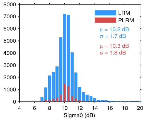
Figure 28. Histogram of science-valid sigma0 over oceans and lakes for LRM (blue) and PLRM (red) for 11/03/2015. The mean ( \mu ) and standard deviation ( \sigma ) are also shown. Note that values outside [4 20] dB are excluded from the histogram for the sake of readability but not from the computation of \mu and \sigma .
