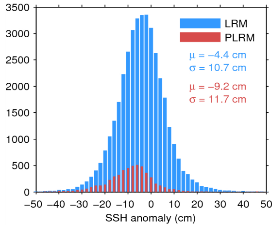
Figure 11. Histogram of science-valid SSH anomaly over oceans and lakes for LRM (blue) and PLRM (red) for 11/03/2015. The mean ( \mu ) and standard deviation ( \sigma ) are also shown. Note that values outside [-50\ 50] cm are excluded from the histogram for the sake of readability but not from the computation of \mu and \sigma .
