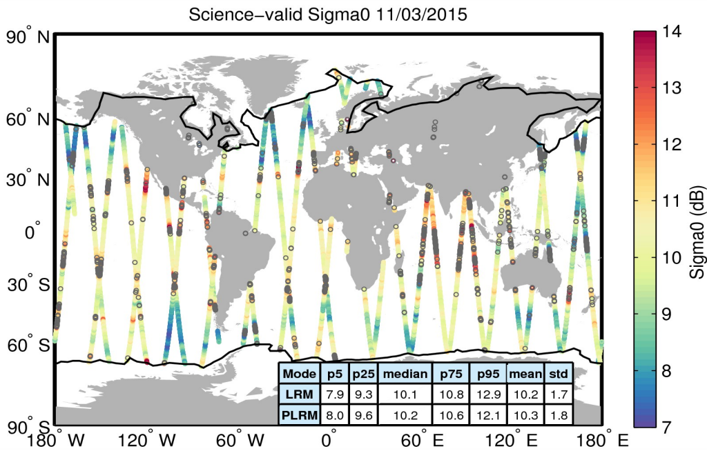
Figure 27. Geographical distribution of science-valid sigma0 data over oceans and lakes for 11/03/2015. The statistical values shown in the table refer to the sigma0 in dB and are calculated separately for LRM and PLRM regions. The black lines mark the outer limit of the Arctic and Antarctic polar polygons. Gray circles denote records that have been rejected based on the editing criteria described in Table 4.
