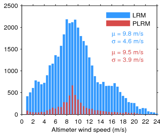
Figure 35. Histogram of science-valid wind over oceans and lakes for LRM (blue) and PLRM (red) for 11/03/2015. The mean ( \mu ) and standard deviation ( \sigma ) are also shown. Note that values larger than 24 m/s are excluded from the histogram for the sake of readability but not from the computation of \mu and \sigma .
