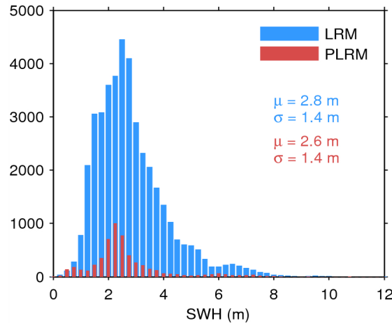
Figure 17. Histogram of flag-valid SWH over oceans and lakes for LRM (blue) and PLRM (red) for 11/03/2015. The mean ( \mu ) and standard deviation ( \sigma ) are also shown. Note that values larger than 12 m are excluded from the histogram for the sake of readability but not from the computation of \mu and \sigma .
