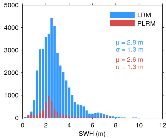
Figure 20. Histogram of science-valid SWH over oceans and lakes for LRM (blue) and PLRM (red) for 11/03/2015. The mean ( \mu ) and standard deviation ( \sigma ) are also shown. Note that values larger than 12 m are excluded from the histogram for the sake of readability but not from the computation of \mu and \sigma .
