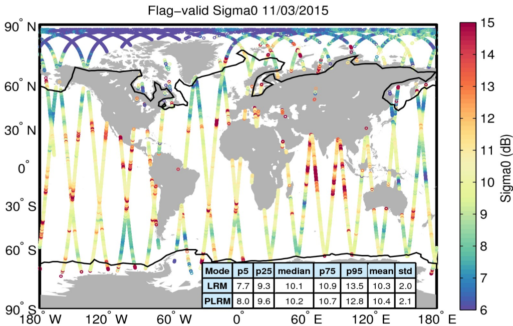
Figure 23. Geographical distribution of flag-valid sigma0 data over oceans and lakes for 11/03/2015. The statistical values shown in the table refer to the sigma0 in dB and are calculated separately for LRM and PLRM regions. Measurements taken over polar polygons have been excluded from the computation of the statistical values. The black lines mark the outer limit of the Arctic and Antarctic polar polygons.
