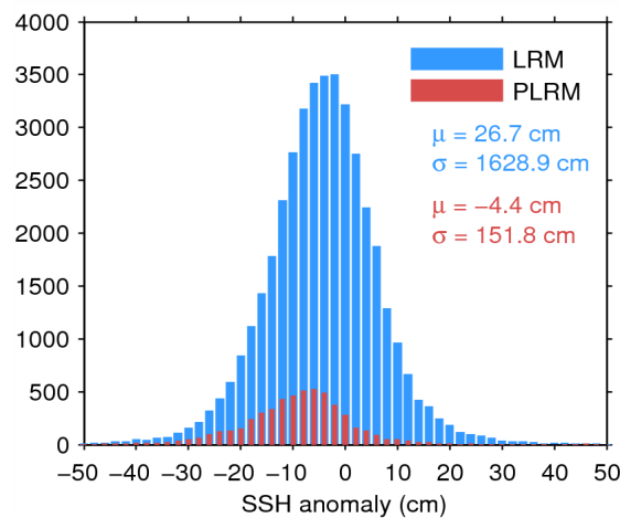
Figure 7. Histogram of flag-valid SSH anomaly over oceans and lakes for LRM (blue) and PLRM (red) for 11/03/2015. The mean ( \mu ) and standard deviation ( \sigma ) are also shown. Note that values outside [-50\ 50] cm are excluded from the histogram for the sake of readability but not from the computation of \mu and \sigma .
