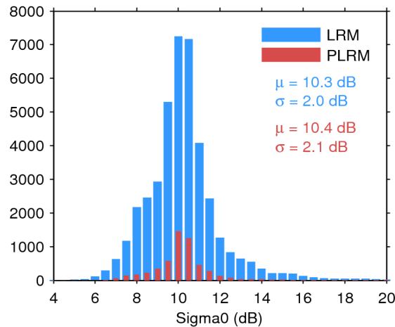
Figure 25. Histogram of flag-valid sigma0 over oceans and lakes for LRM (blue) and PLRM (red) for 11/03/2015. The mean ( \mu ) and standard deviation ( \sigma ) are also shown. Note that values outside [4 20] dB are excluded from the histogram for the sake of readability but not from the computation of \mu and \sigma .
