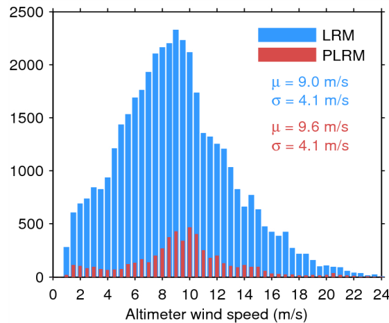
Figure 33. Histogram of flag-valid wind over oceans and lakes for LRM (blue) and PLRM (red) for 09/03/2015. The mean ( \mu ) and standard deviation ( \sigma ) are also shown. Note that values larger than 24 m/s are excluded from the histogram for the sake of readability but not from the computation of \mu and \sigma .
