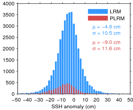
Figure 11. Histogram of science-valid SSH anomaly over oceans and lakes for LRM (blue) and PLRM (red) for 09/03/2015. The mean ( \mu ) and standard deviation ( \sigma ) are also shown. Note that values outside [-50 50] cm are excluded from the histogram for the sake of readability but not from the computation of \mu and \sigma .
