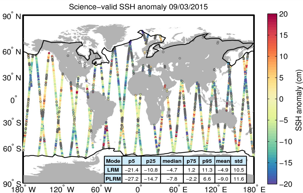
Figure 10. Geographical distribution of science-valid SSH anomaly data over oceans and lakes for 09/03/2015. The statistical values shown in the table refer to the SSH anomaly in cm and are calculated separately for LRM and PLRM regions. The black lines mark the outer limit of the Arctic and Antarctic polar polygons. Gray circles denote records that have been rejected based on the editing criteria described in Table 2.
