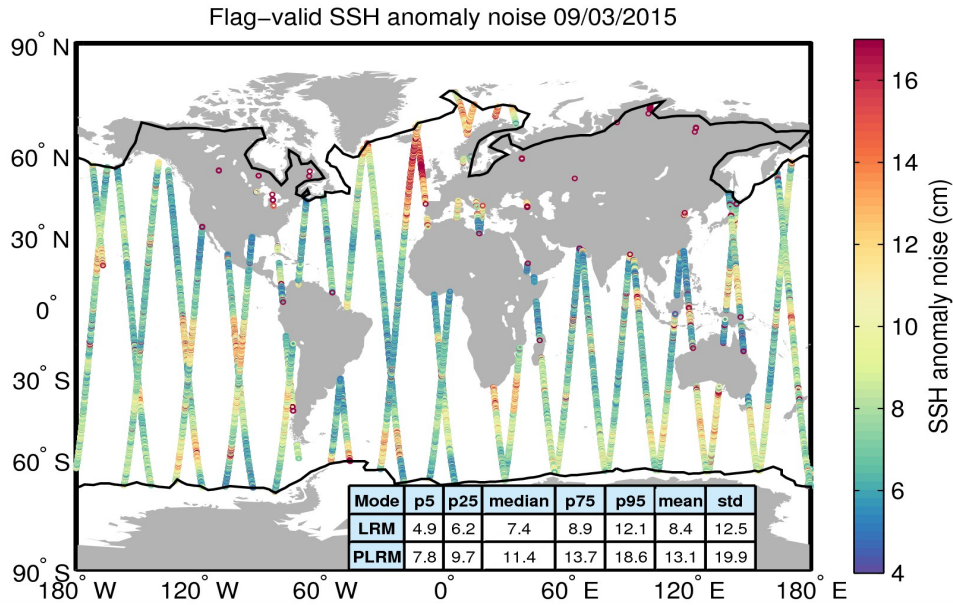
Figure 8. Geographical distribution of flag-valid 20-Hz SSH anomaly measurement noise over oceans and lakes for 09/03/2015. The statistical values shown in the table refer to the SSH anomaly noise and are calculated separately for LRM and PLRM regions. Measurements taken over polar polygons have been excluded from the computation of the statistical values. The black lines mark the outer limit of the Arctic and Antarctic polar polygons.
