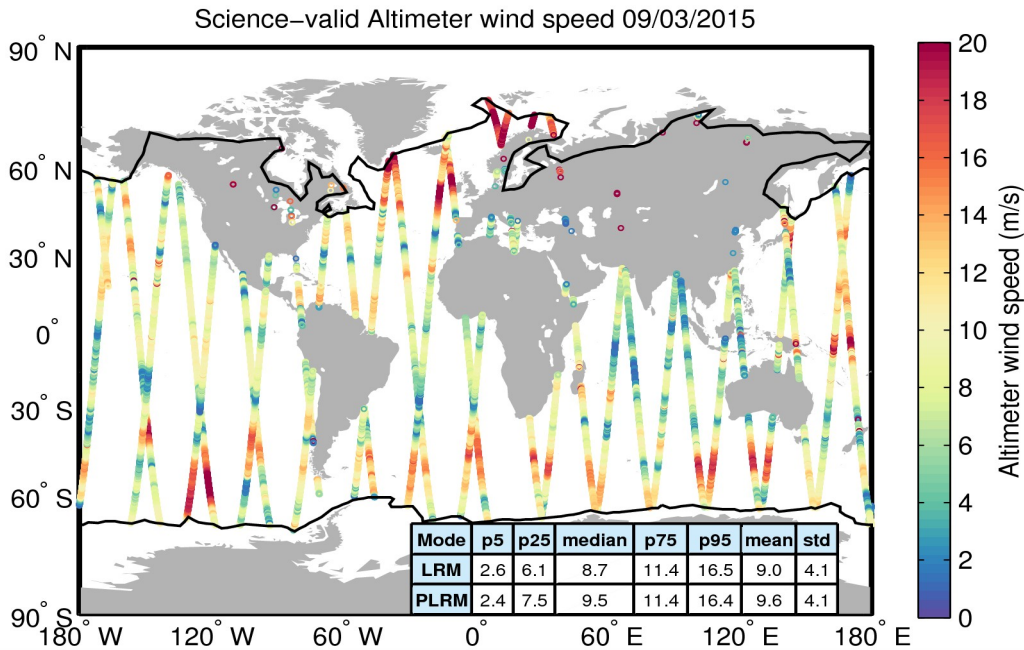
Figure 34. Geographical distribution of science-valid wind data over oceans and lakes for 09/03/2015. The statistical values shown in the table refer to the wind in m/s and are calculated separately for LRM and PLRM regions. The black lines mark the outer limit of the Arctic and Antarctic polar polygons. Gray circles denote records that have been rejected based on the editing criteria described in Table 5.
