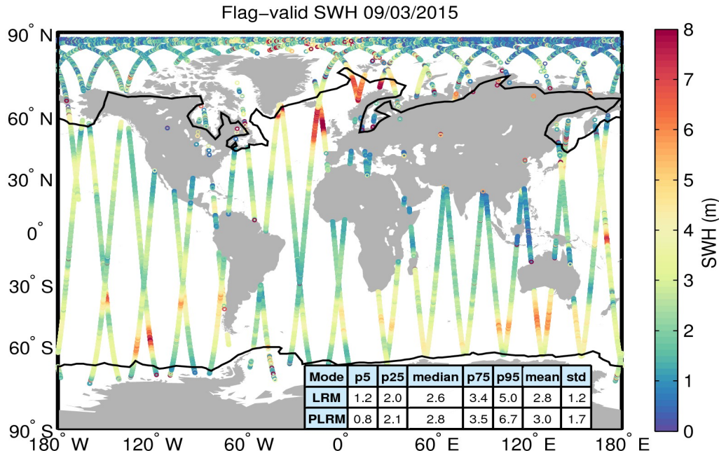
Figure 15. Geographical distribution of flag-valid SWH data over oceans and lakes for 09/03/2015. The statistical values shown in the table refer to the SWH in m and are calculated separately for LRM and PLRM regions. Measurements taken over polar polygons have been excluded from the computation of the statistical values. The black lines mark the outer limit of the Arctic and Antarctic polar polygons.
