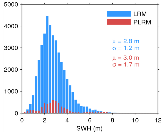
Figure 17. Histogram of flag-valid SWH over oceans and lakes for LRM (blue) and PLRM (red) for 09/03/2015. The mean ( \mu ) and standard deviation ( \sigma ) are also shown. Note that values larger than 12 m are excluded from the histogram for the sake of readability but not from the computation of \mu and \sigma .
