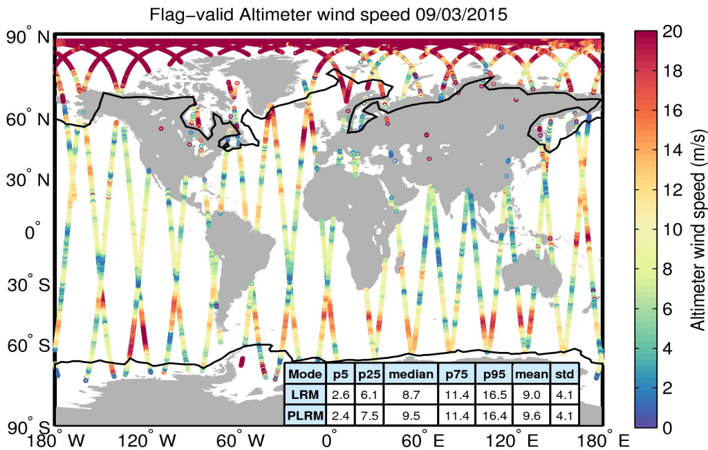
Figure 31. Geographical distribution of flag-valid wind data over oceans and lakes for 09/03/2015. The statistical values shown in the table refer to the wind in m/s and are calculated separately for LRM and PLRM regions. Measurements taken over polar polygons have been excluded from the computation of the statistical values. The black lines mark the outer limit of the Arctic and Antarctic polar polygons.
