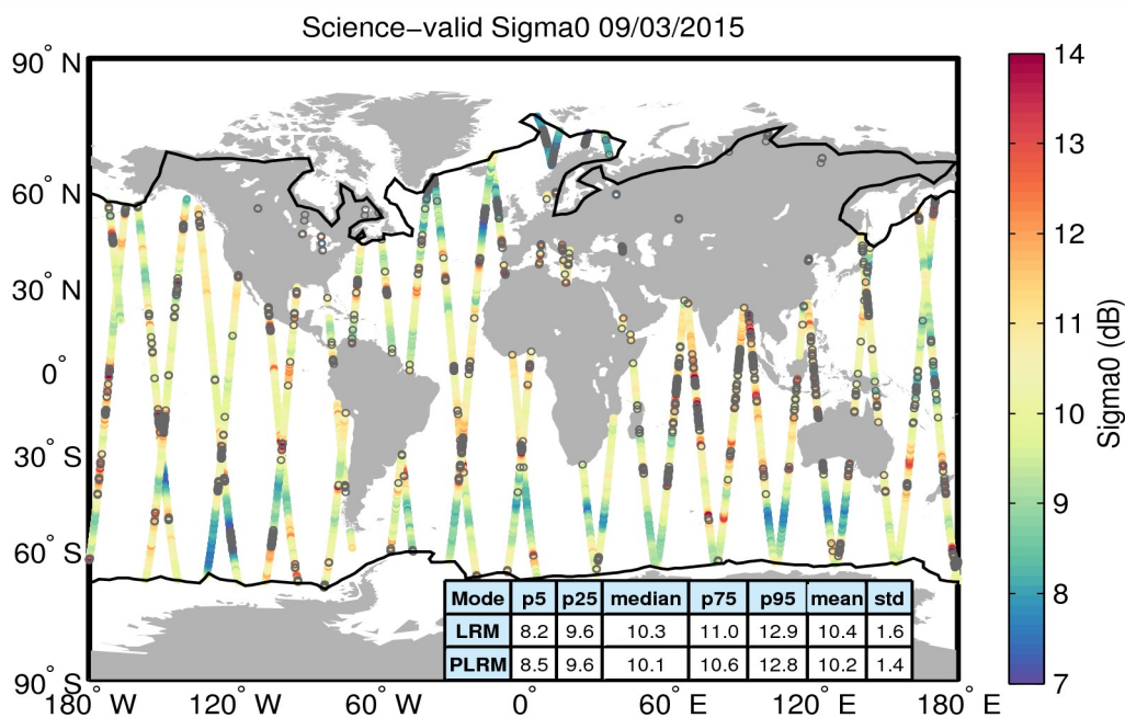
Figure 27. Geographical distribution of science-valid sigma0 data over oceans and lakes for 09/03/2015. The statistical values shown in the table refer to the sigma0 in dB and are calculated separately for LRM and PLRM regions. The black lines mark the outer limit of the Arctic and Antarctic polar polygons. Gray circles denote records that have been rejected based on the editing criteria described in Table 4.
