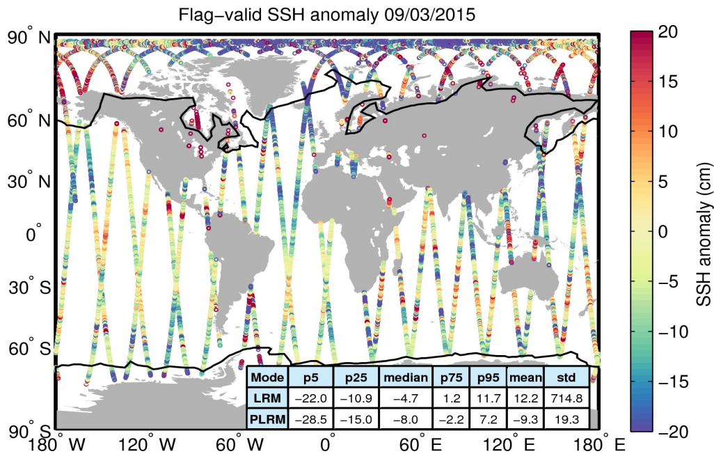
Figure 5. Geographical distribution of flag-valid 1-Hz SSH anomaly data over oceans and lakes for 09/03/2015. The statistical values shown in the table refer to the SSH anomaly in cm and are calculated separately for LRM and PLRM regions. Measurements taken over polar polygons have been excluded from the computation of the statistical values. The black lines mark the outer limit of the Arctic and Antarctic polar polygons.
