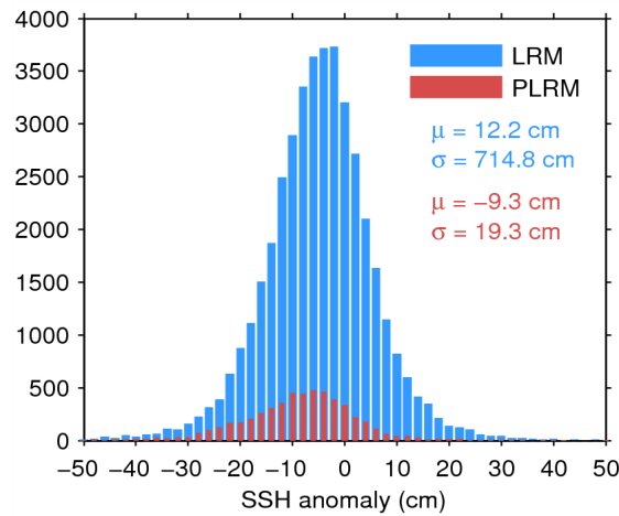
Figure 7. Histogram of flag-valid SSH anomaly over oceans and lakes for LRM (blue) and PLRM (red) for 09/03/2015. The mean ( \mu ) and standard deviation ( \sigma ) are also shown. Note that values outside [-50\ 50] cm are excluded from the histogram for the sake of readability but not from the computation of \mu and \sigma .
