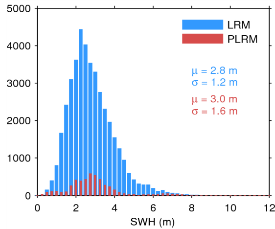
Figure 20. Histogram of science-valid SWH over oceans and lakes for LRM (blue) and PLRM (red) for 09/03/2015. The mean ( \mu ) and standard deviation ( \sigma ) are also shown. Note that values larger than 12 m are excluded from the histogram for the sake of readability but not from the computation of \mu and \sigma .
