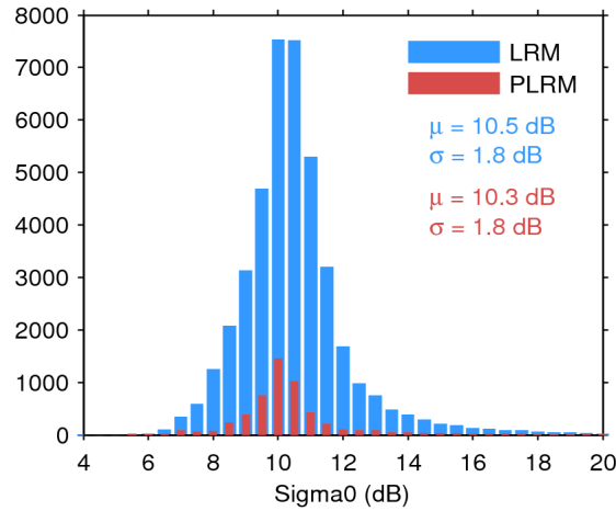
Figure 25. Histogram of flag-valid sigma0 over oceans and lakes for LRM (blue) and PLRM (red) for 09/03/2015. The mean ( \mu ) and standard deviation ( \sigma ) are also shown. Note that values outside [4 20] dB are excluded from the histogram for the sake of readability but not from the computation of \mu and \sigma .
