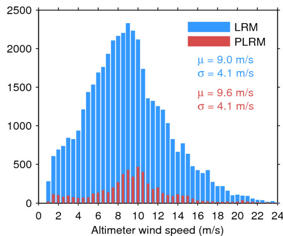
Figure 35. Histogram of science-valid wind over oceans and lakes for LRM (blue) and PLRM (red) for 09/03/2015. The mean ( \mu ) and standard deviation ( \sigma ) are also shown. Note that values larger than 24 m/s are excluded from the histogram for the sake of readability but not from the computation of \mu and \sigma .
