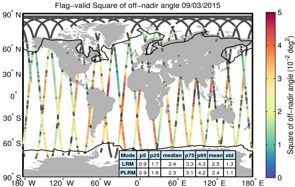
Figure 37. Geographical distribution of flag-valid mispointing data over oceans and lakes for 09/03/2015. The statistical values shown in the table refer to the mispointing in 10^{-2} \text{ deg}^2 and are calculated separately for LRM and PLRM regions. Measurements taken over polar polygons have been excluded from the computation of the statistical values. The black lines mark the outer limit of the Arctic and Antarctic polar polygons. Gray circles denote negative values.
