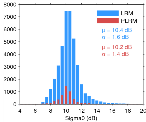
Figure 28. Histogram of science-valid sigma0 over oceans and lakes for LRM (blue) and PLRM (red) for 09/03/2015. The mean ( \mu ) and standard deviation ( \sigma ) are also shown. Note that values outside [4 20] dB are excluded from the histogram for the sake of readability but not from the computation of \mu and \sigma .
