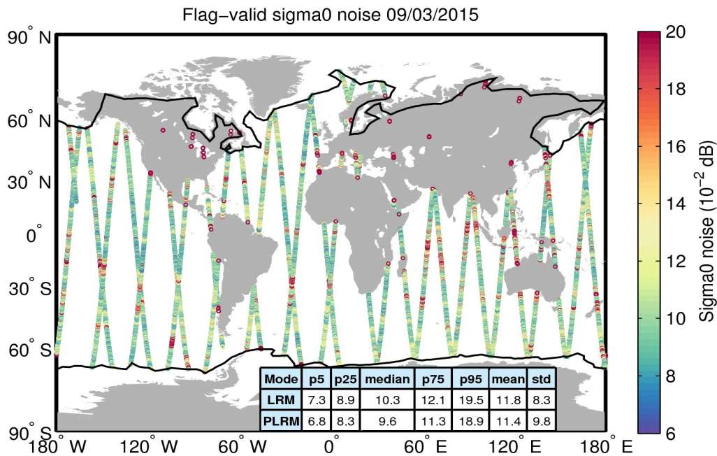
Figure 26. Geographical distribution of flag-valid 20-Hz sigma0 measurement noise over oceans and lakes for 09/03/2015. The statistical values shown in the table refer to the sigma0 noise and are calculated separately for LRM and PLRM regions. Measurements taken over polar polygons have been excluded from the computation of the statistical values. The black lines mark the outer limit of the Arctic and Antarctic polar polygons.
