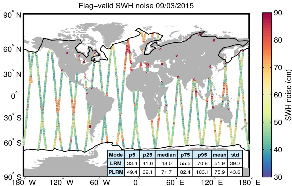
Figure 18. Geographical distribution of flag-valid 20-Hz SWH measurement noise over oceans and lakes for 09/03/2015. The statistical values shown in the table refer to the SWH noise and are calculated separately for LRM and PLRM regions. Measurements taken over polar polygons have been excluded from the computation of the statistical values. The black lines mark the outer limit of the Arctic and Antarctic polar polygons.
