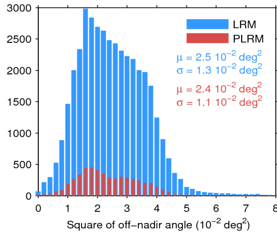
Figure 39. Histogram of flag-valid mispointing over oceans and lakes for LRM (blue) and PLRM (red) for 09/03/2015. Only positive values have been considered. The mean ( \mu ) and standard deviation ( \sigma ) are also shown. Note that values larger than 8 \cdot 10^{-2} \text{ deg}^2 are excluded from the histogram for the sake of readability but not from the computation of \mu and \sigma .
