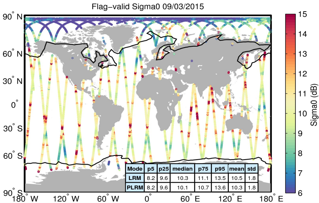
Figure 23. Geographical distribution of flag-valid sigma0 data over oceans and lakes for 09/03/2015. The statistical values shown in the table refer to the sigma0 in dB and are calculated separately for LRM and PLRM regions. Measurements taken over polar polygons have been excluded from the computation of the statistical values. The black lines mark the outer limit of the Arctic and Antarctic polar polygons.
