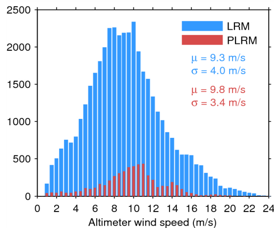
Figure 35. Histogram of science-valid wind over oceans and lakes for LRM (blue) and PLRM (red) for 08/03/2015. The mean ( \mu ) and standard deviation ( \sigma ) are also shown. Note that values larger than 24 m/s are excluded from the histogram for the sake of readability but not from the computation of \mu and \sigma .
