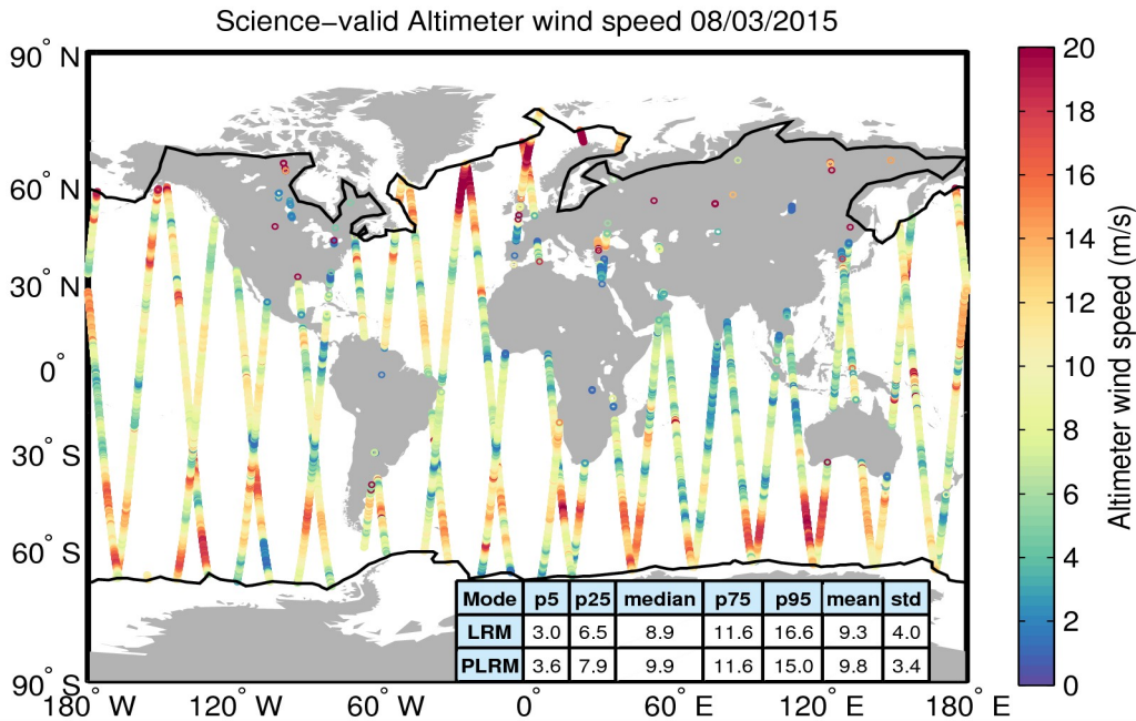
Figure 34. Geographical distribution of science-valid wind data over oceans and lakes for 08/03/2015. The statistical values shown in the table refer to the wind in m/s and are calculated separately for LRM and PLRM regions. The black lines mark the outer limit of the Arctic and Antarctic polar polygons. Gray circles denote records that have been rejected based on the editing criteria described in Table 5.
