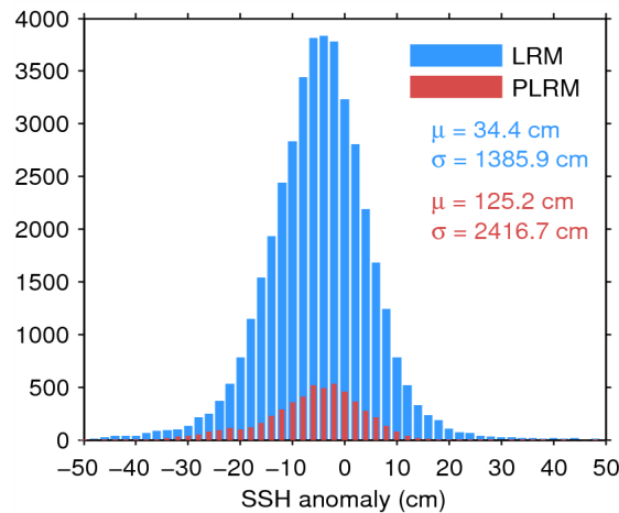
Figure 7. Histogram of flag-valid SSH anomaly over oceans and lakes for LRM (blue) and PLRM (red) for 08/03/2015. The mean ( \mu ) and standard deviation ( \sigma ) are also shown. Note that values outside [-50\ 50] cm are excluded from the histogram for the sake of readability but not from the computation of \mu and \sigma .
