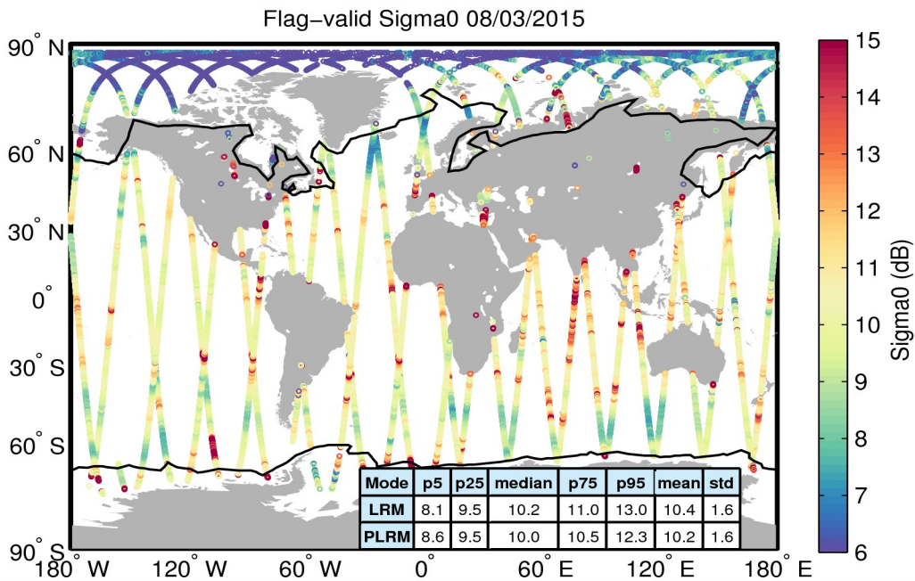
Figure 23. Geographical distribution of flag-valid sigma0 data over oceans and lakes for 08/03/2015. The statistical values shown in the table refer to the sigma0 in dB and are calculated separately for LRM and PLRM regions. Measurements taken over polar polygons have been excluded from the computation of the statistical values. The black lines mark the outer limit of the Arctic and Antarctic polar polygons.
