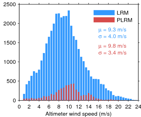
Figure 33. Histogram of flag-valid wind over oceans and lakes for LRM (blue) and PLRM (red) for 08/03/2015. The mean ( \mu ) and standard deviation ( \sigma ) are also shown. Note that values larger than 24 m/s are excluded from the histogram for the sake of readability but not from the computation of \mu and \sigma .
