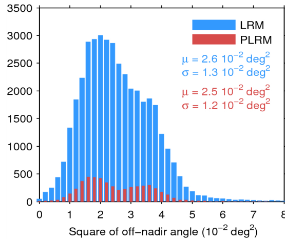
Figure 39. Histogram of flag-valid mispointing over oceans and lakes for LRM (blue) and PLRM (red) for 08/03/2015. Only positive values have been considered. The mean ( \mu ) and standard deviation ( \sigma ) are also shown. Note that values larger than 8 \cdot 10^{-2} \text{ deg}^2 are excluded from the histogram for the sake of readability but not from the computation of \mu and \sigma .
