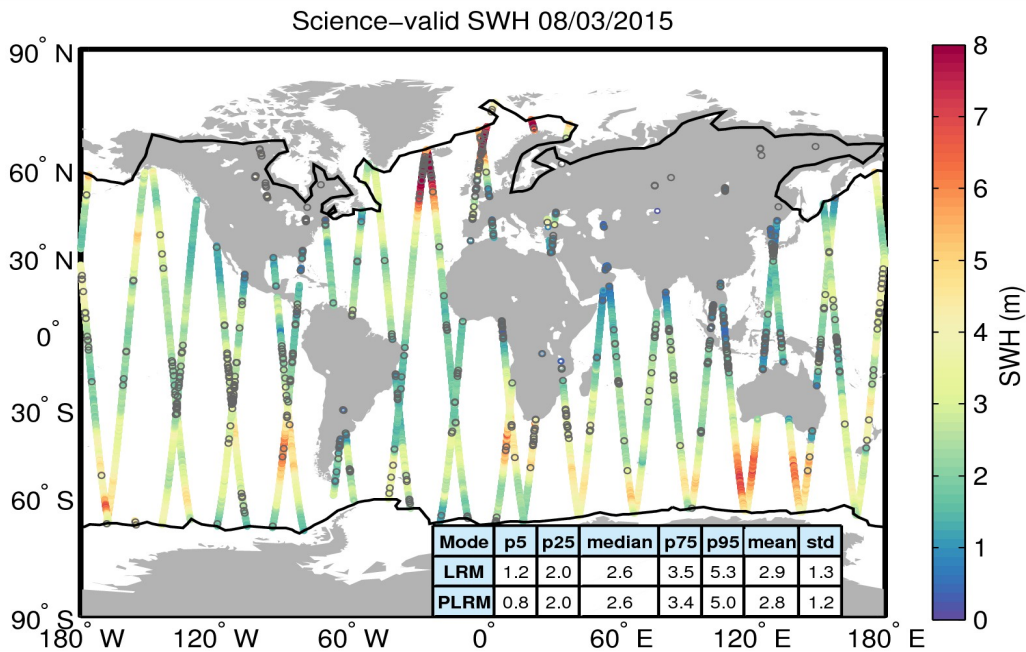
Figure 19. Geographical distribution of science-valid SWH data over oceans and lakes for 08/03/2015. The statistical values shown in the table refer to the SWH in m and are calculated separately for LRM and PLRM regions. The black lines mark the outer limit of the Arctic and Antarctic polar polygons. Gray circles denote records that have been rejected based on the editing criteria described in Table 3.
