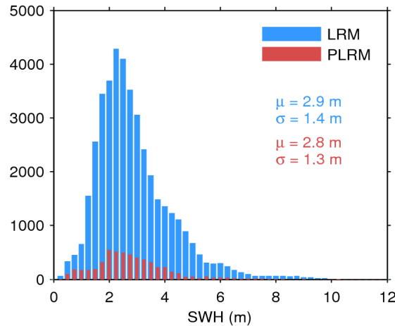
Figure 17. Histogram of flag-valid SWH over oceans and lakes for LRM (blue) and PLRM (red) for 08/03/2015. The mean ( \mu ) and standard deviation ( \sigma ) are also shown. Note that values larger than 12 m are excluded from the histogram for the sake of readability but not from the computation of \mu and \sigma .
