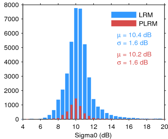
Figure 25. Histogram of flag-valid sigma0 over oceans and lakes for LRM (blue) and PLRM (red) for 08/03/2015. The mean ( \mu ) and standard deviation ( \sigma ) are also shown. Note that values outside [4 20] dB are excluded from the histogram for the sake of readability but not from the computation of \mu and \sigma .
