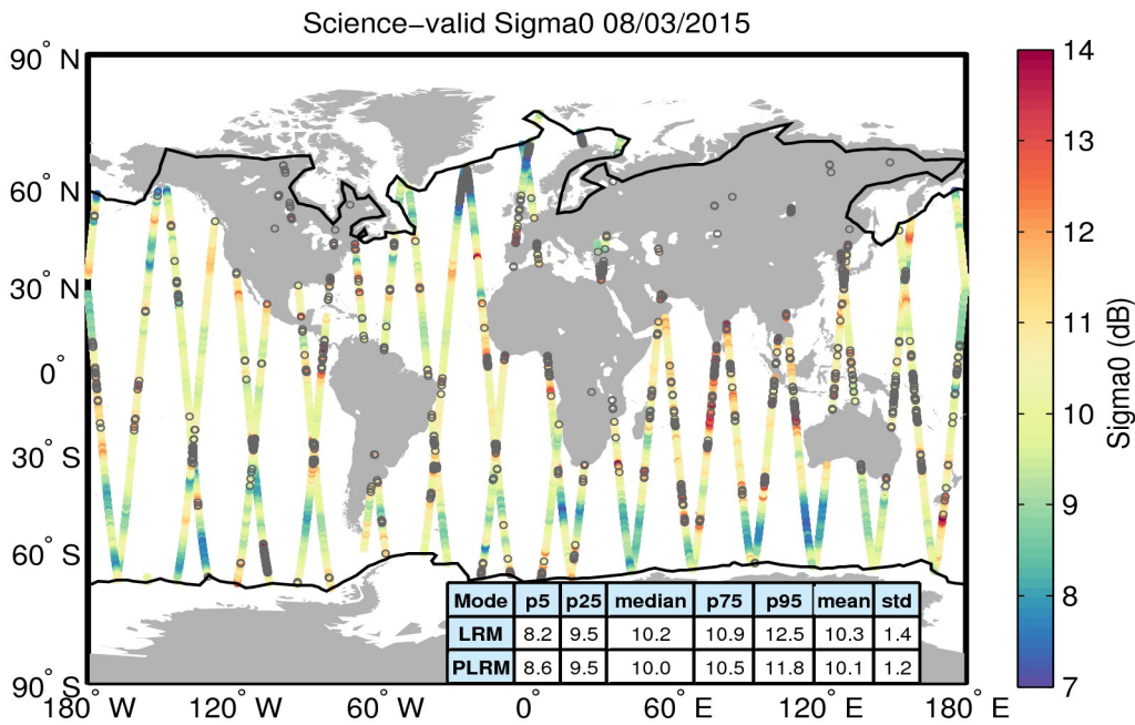
Figure 27. Geographical distribution of science-valid sigma0 data over oceans and lakes for 08/03/2015. The statistical values shown in the table refer to the sigma0 in dB and are calculated separately for LRM and PLRM regions. The black lines mark the outer limit of the Arctic and Antarctic polar polygons. Gray circles denote records that have been rejected based on the editing criteria described in Table 4.
