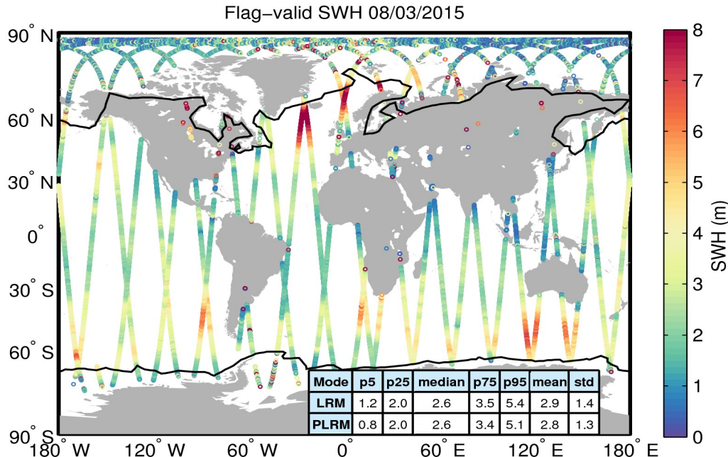
Figure 15. Geographical distribution of flag-valid SWH data over oceans and lakes for 08/03/2015. The statistical values shown in the table refer to the SWH in m and are calculated separately for LRM and PLRM regions. Measurements taken over polar polygons have been excluded from the computation of the statistical values. The black lines mark the outer limit of the Arctic and Antarctic polar polygons.
