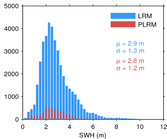
Figure 20. Histogram of science-valid SWH over oceans and lakes for LRM (blue) and PLRM (red) for 08/03/2015. The mean ( \mu ) and standard deviation ( \sigma ) are also shown. Note that values larger than 12 m are excluded from the histogram for the sake of readability but not from the computation of \mu and \sigma .
