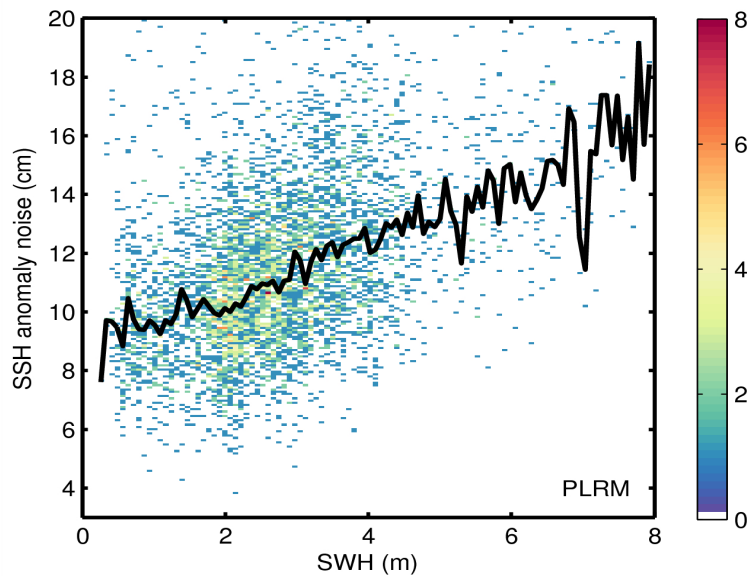
Figure 9. 2D histogram showing flag-valid SSH anomaly noise as a function of SWH for LRM (top) and PLRM (bottom) for 08/03/2015. The black line denotes the median SSH anomaly as a function of SWH.
