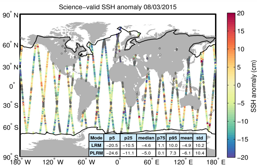
Figure 10. Geographical distribution of science-valid SSH anomaly data over oceans and lakes for 08/03/2015. The statistical values shown in the table refer to the SSH anomaly in cm and are calculated separately for LRM and PLRM regions. The black lines mark the outer limit of the Arctic and Antarctic polar polygons. Gray circles denote records that have been rejected based on the editing criteria described in Table 2.
