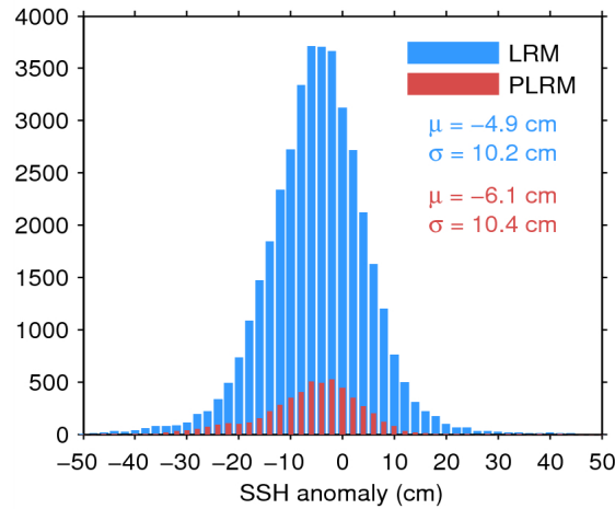
Figure 11. Histogram of science-valid SSH anomaly over oceans and lakes for LRM (blue) and PLRM (red) for 08/03/2015. The mean ( \mu ) and standard deviation ( \sigma ) are also shown. Note that values outside [-50 50] cm are excluded from the histogram for the sake of readability but not from the computation of \mu and \sigma .
