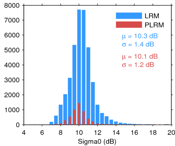
Figure 28. Histogram of science-valid sigma0 over oceans and lakes for LRM (blue) and PLRM (red) for 08/03/2015. The mean ( \mu ) and standard deviation ( \sigma ) are also shown. Note that values outside [4 20] dB are excluded from the histogram for the sake of readability but not from the computation of \mu and \sigma .
