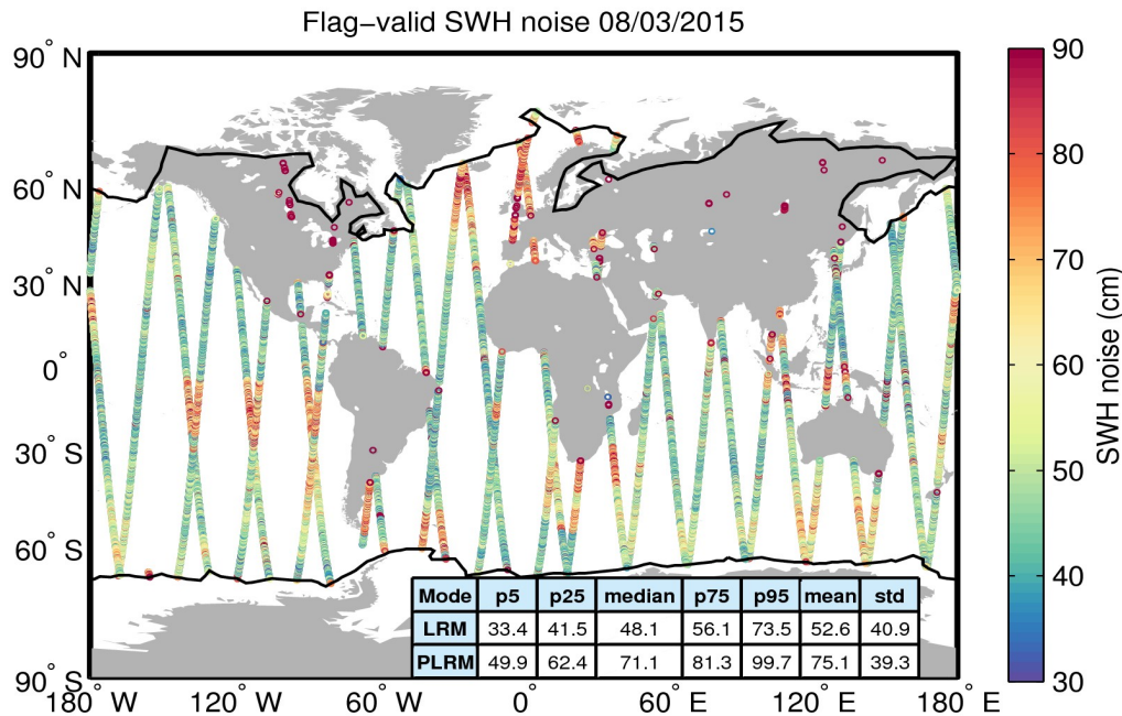
Figure 18. Geographical distribution of flag-valid 20-Hz SWH measurement noise over oceans and lakes for 08/03/2015. The statistical values shown in the table refer to the SWH noise and are calculated separately for LRM and PLRM regions. Measurements taken over polar polygons have been excluded from the computation of the statistical values. The black lines mark the outer limit of the Arctic and Antarctic polar polygons.
